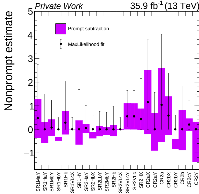
Figure 5.16: The comparison of the nonprompt background estimates based on the simple prompt subtraction and the maximum likelihood fit.
