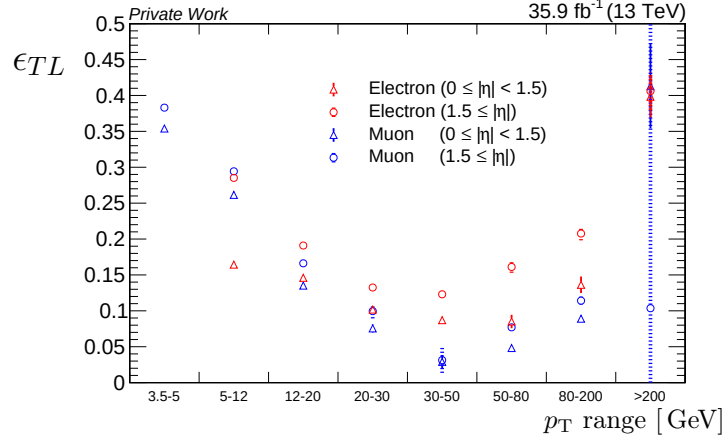
Figure 5.15: Tight-to-loose factors measured in data for electrons and muons.
