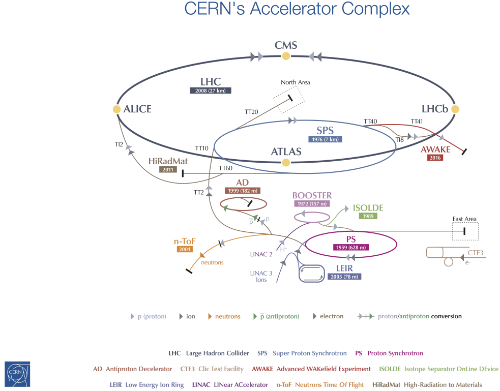
Figure 3.1: CERN accelerator complex [57].
