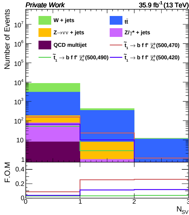
Figure 5.35: The SV multiplicity distribution is shown for the few signal scenarios and the dominant backgrounds. The figure of merit (FOM), shown in the bottom panel, is calculated for each signal scenario based on the methods described in [18].
