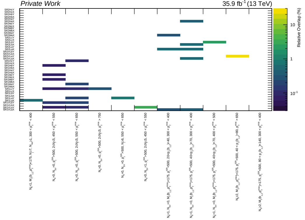
Figure A.7: Relative overlaps, as measured from data events, between the 1\ell SRs and 0\ell SRs normalized to the average sizes of the two regions.
