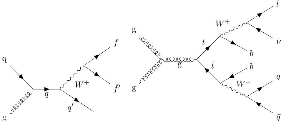
Figure 5.9: Examples of Feynman diagrams for the dominant background processes: the production of a W boson in association with jets (W+jets) on the left and the pair production of top quarks ( t\bar{t} ) on the right.
