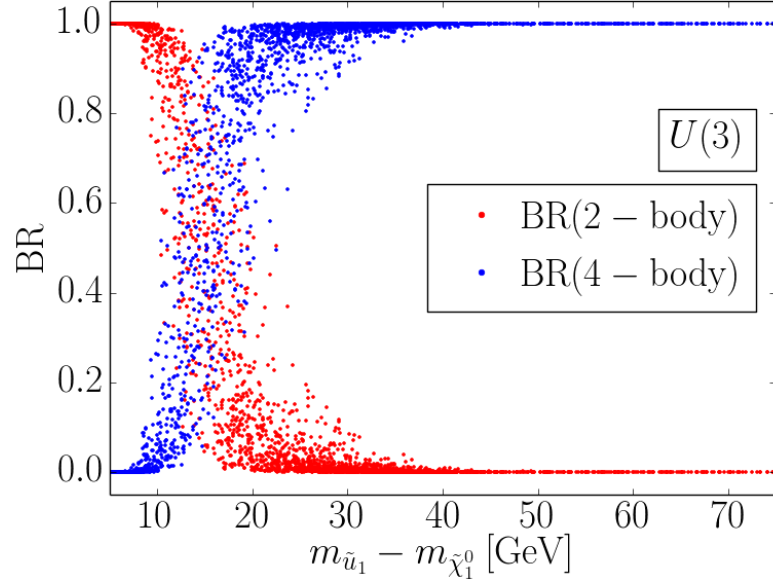
Figure 2.6: Branching ratios for the four-body (blue) and the FCNC (red) decays of the top squark corresponding to a specific flavor symmetry in the squark sector [52].
