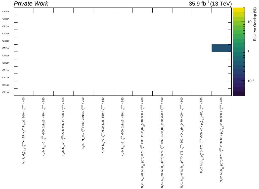
Figure A.8: Relative overlaps, as measured from data events, between the 1\ell CRs and 0\ell SRs normalized to the average sizes of the two regions.
