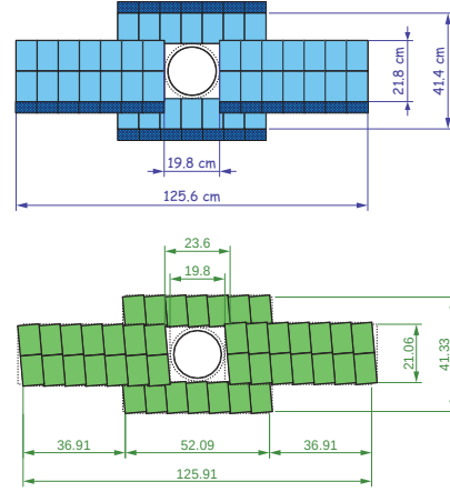
Figure 2.9: Layout of IT layers oriented at 0^\circ (top) and -5^\circ (bottom).
