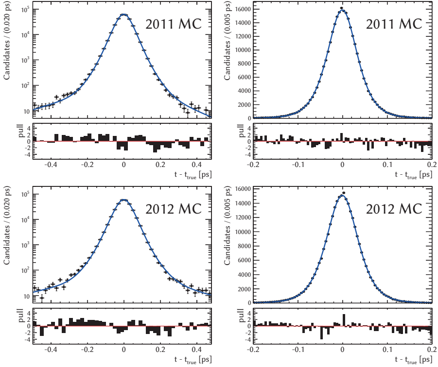
Figure 6.12: Left: result of a likelihood fit to the distribution of t - t_{\text{true}} for samples simulated with 2011 and 2012 conditions containing a B_s \rightarrow J/\psi \phi decay after application of the improved PV refitting. Right: zoomed-in view around t - t_{\text{true}} = 0 .
