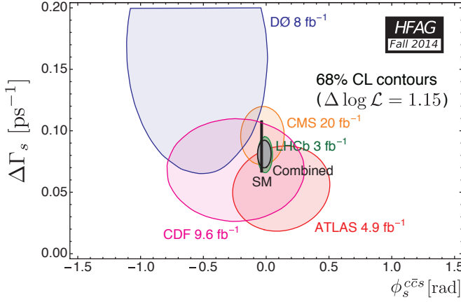
Figure 7.4: Two dimensional contours of -\Delta\log\mathcal{L}=1.15 (“one-sigma”) of \Delta\Gamma_s and \phi_s for all measurements of these observables performed to date. The Standard Model prediction [13, 90], and the combination of all measurements are also shown. Combination performed and figure provided by the Heavy Flavour Averaging Group [91].
