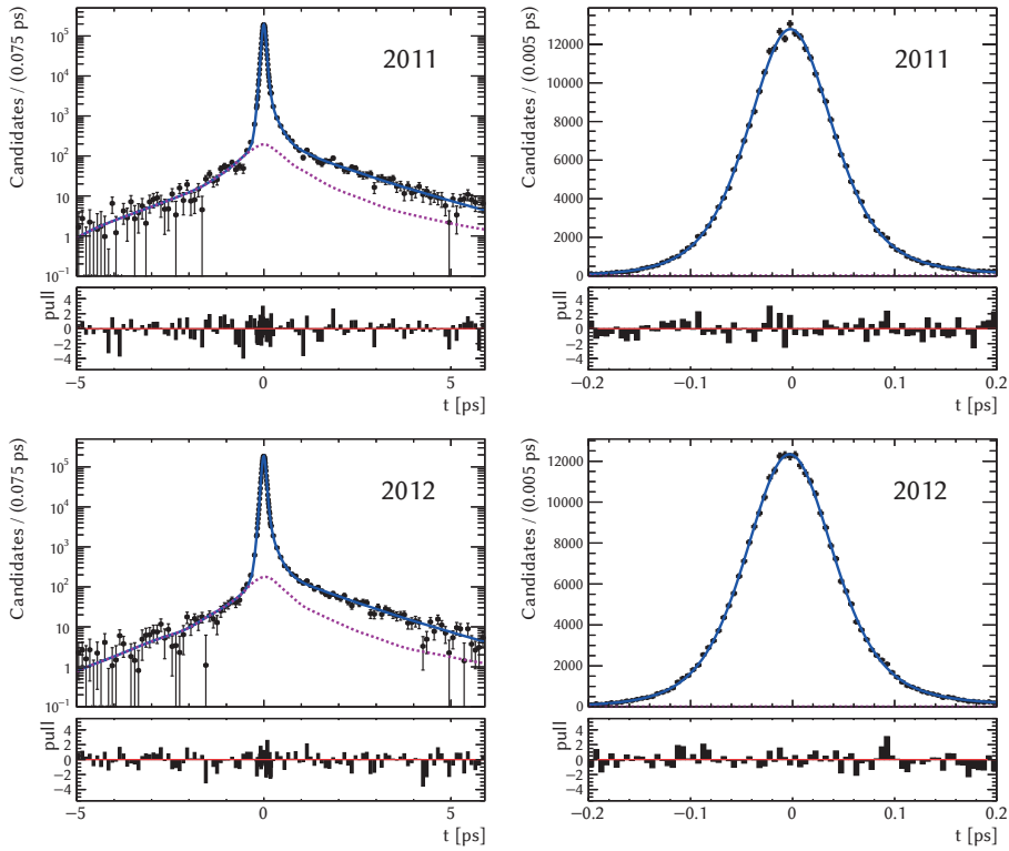
Figure 6.16: Result of a likelihood fit to the 2011 and 2012 real data prompt-background samples, where the next-best- \chi^2_{IP} requirement was omitted and a dedicated distribution (dashed purple line) was included to account for candidates which have been assigned a wrong PV.
