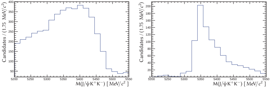
Figure 4.4: Distributions of M_{J/\psi K^+ K^-} for the \Lambda_b \rightarrow J/\psi p K (left) and B^0 \rightarrow J/\psi K^* (right) simulated samples, reconstructed as B_s \rightarrow J/\psi \phi (reproduced from [69]).
