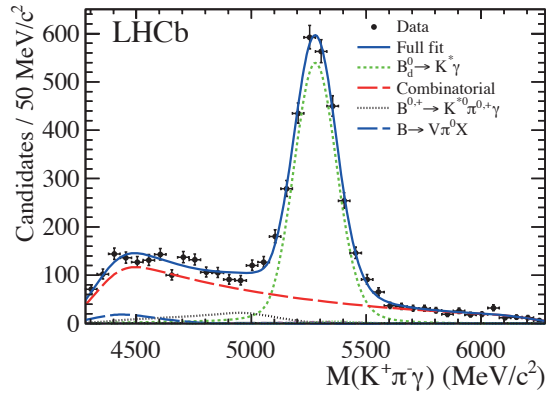
Figure 2.15: Distribution of M_{K\pi\gamma} for a sample of decays of B^0 \rightarrow K^{*0}\gamma selected from 1 \text{ fb}^1 of data collected by LHCb in 2011; reproduced from [40].
