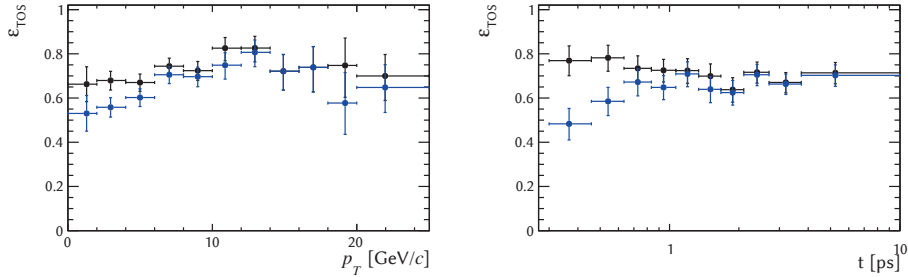
(a) Efficiency as a function of the p_T of the B^+ .
