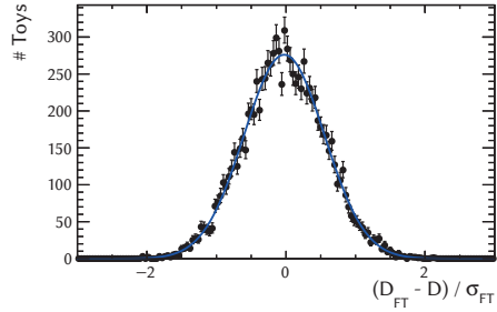
(b) Distribution of the difference between the dilution calculated using either the Fourier transform algorithm or the parameters of the PDF used to generate the toy samples.
