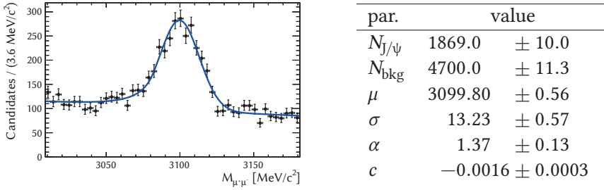
Figure 3.14: Result of a fit to the distribution of M_{\mu^+\mu^-} of a sample of on-line reconstructed J/\psi candidates collected by LHCb during run 133584 on December 3rd 2012; the parameters are described in the text.
