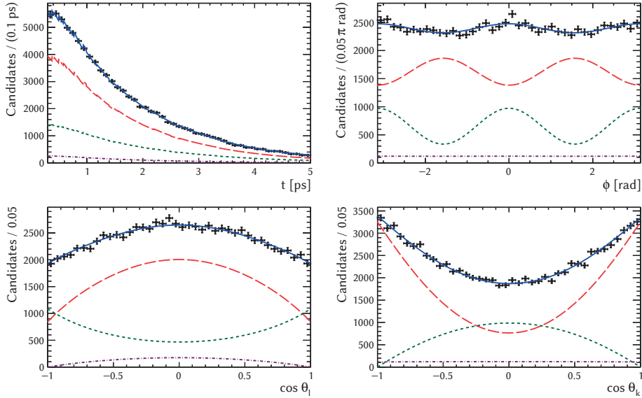
Figure 7.1: Projection of the PDF resulting from the fit to the combined 2011 and 2012 data, superimposed on the data sample as a function of decay-time and decay-angles. The total PDF (blue), CP -even (dashed red), CP -odd (dashed green) and S-wave (dashed purple) components are shown. Figures produced in collaboration with [81].
