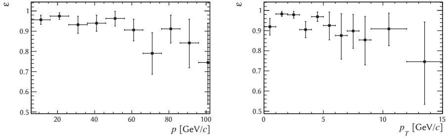
Figure 3.6: Left: efficiency of the HLT1 Velo pattern recognition algorithms for muons from B^+ \rightarrow J/\psi K^+ as a function of p in 2012. Right: efficiency as a function of p_T .
