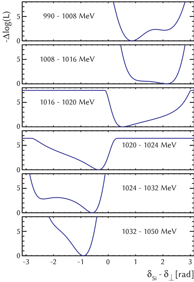
Figure 7.3: Value of -\Delta\log\mathcal{L} as a function of parameter value for the phase differences between the S-wave component and \delta_{\perp} in the bins of M(K^+K^-) . Figures produced in collaboration with [81].
