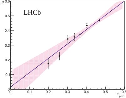
Figure 4.14: Measured ( \omega ) versus estimated ( \eta ) wrong-tag probability obtained from a simultaneous fit in bins of \eta to the decay-time distribution of a sample of B_s \rightarrow D_s^- \pi^+ decays. The line represents a linear parameterisation of the form of eq. (4.31), obtained from a fit to the values of \omega
