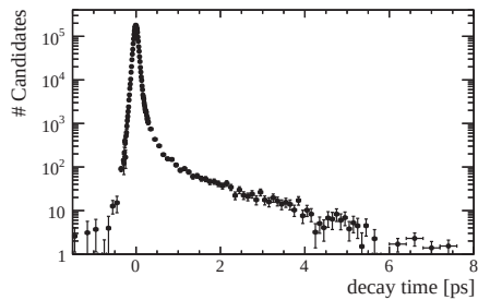
Figure 6.2: Decay-time distribution of prompt-background candidates in 2011 data, weighted using sWeights that have been obtained from a fit to the distribution of M_{\mu^+\mu^-} .
