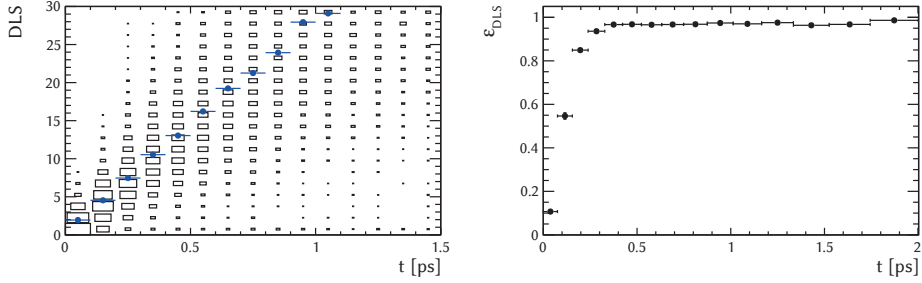
(a) J/\psi DLS versus B_s decay-time; the mean DLS is shown superimposed as the blue points.
