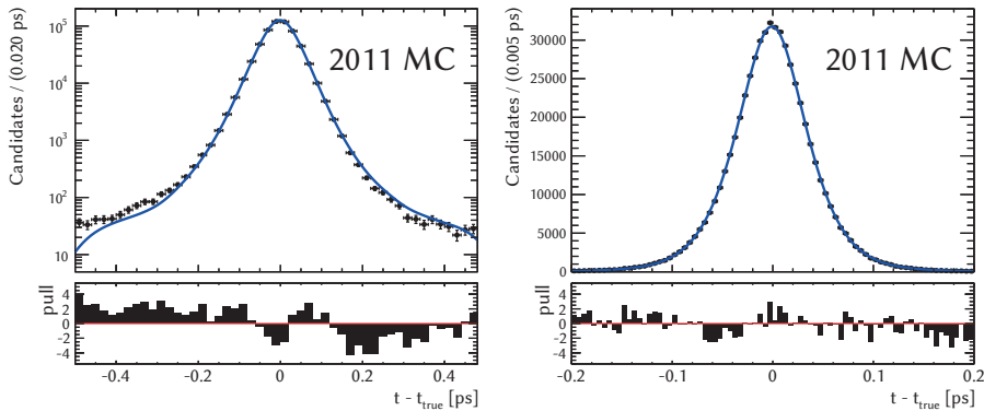
Figure 6.20: Result of a likelihood fit to samples simulated with 2011 conditions which contain a B_s \rightarrow J/\psi \phi decay, where a dedicated distribution has been included to account for candidates which have been associated to the wrong PV. The full PV refitting as described in section 6.4 has been applied to the signal candidates, but not during the event mixing procedure.
