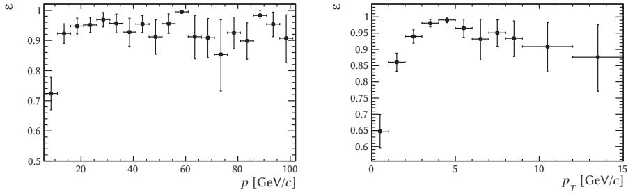
Figure 3.7: Left: efficiency of the matching algorithm for muons from B^+ \rightarrow J/\psi K^+ , whose Velo track segments have been reconstructed by the Velo track finding, as a function of p in 2012. Right: efficiency as a function of p_T .
