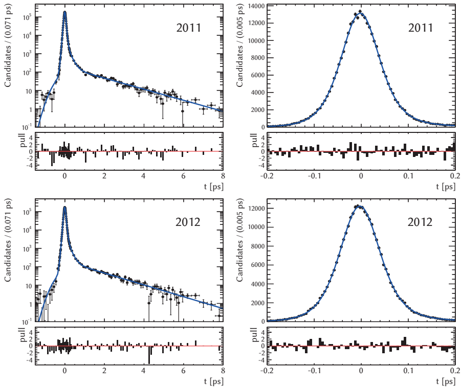
Figure 6.3: Left: results of fits to the decay-time distribution of the 2011 and 2012 sample of prompt-background candidates shown on a log-scale. Right: a linear scale zoomed-in around 0. Below the distributions the pull of the PDF with respect to the data points is shown, demonstrating the good quality of the fit.
