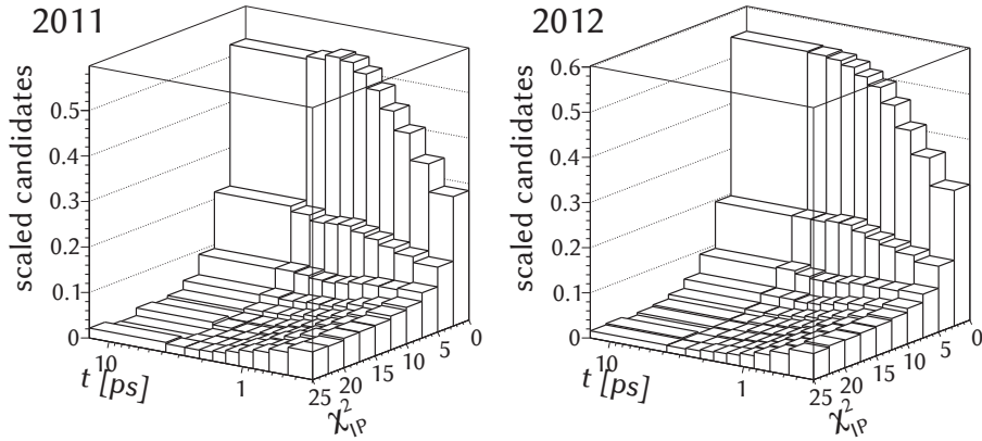
Figure 6.22: Normalised distributions of \chi^2_{\text{IP}}(B_s) in bins of t for 2011 and 2012 signal candidates.
