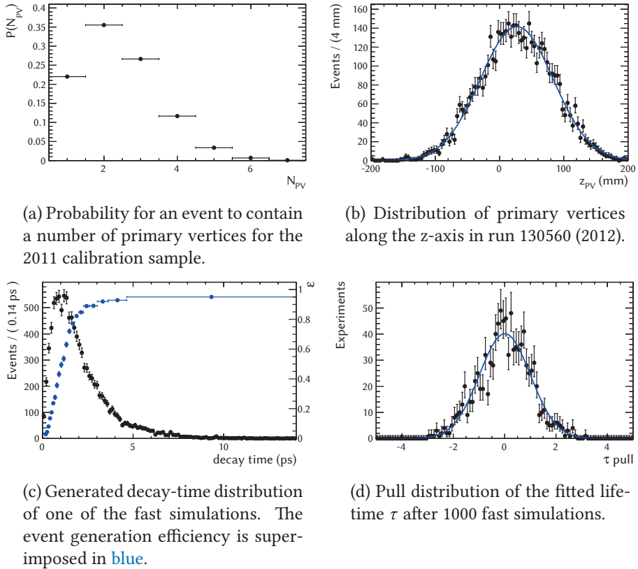
Figure 5.4: Several distributions related to the validation of the per-event decay-time acceptance.
