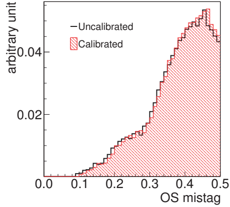
Figure 4.12: Distribution of \eta of the combined opposite-side tagging algorithms for B_s \rightarrow J/\psi \phi signal candidates before and after calibration.
