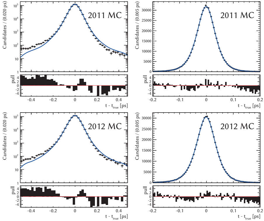
Figure 6.19: Result of a likelihood fit to samples simulated with 2011 and 2012 conditions which contain B_s \rightarrow J/\psi \phi decay, where a dedicated distribution has been included to account for candidates which have been associated to the wrong PV.
