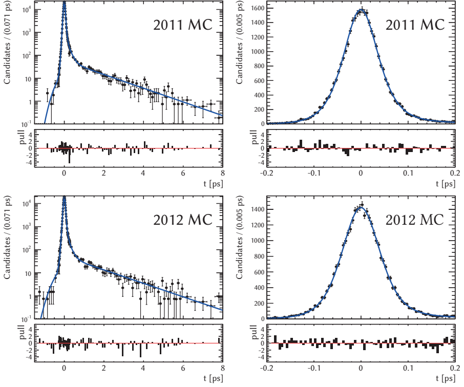
Figure 6.6: Left: result of a likelihood fit to the decay-time distribution of selected B_s \rightarrow J/\psi \phi candidates obtained from the 2011 and 2012 simulated prompt-background samples. The fitted curve is the PDF described in eq. (6.2). Right: zoomed-in view around t = 0 .
