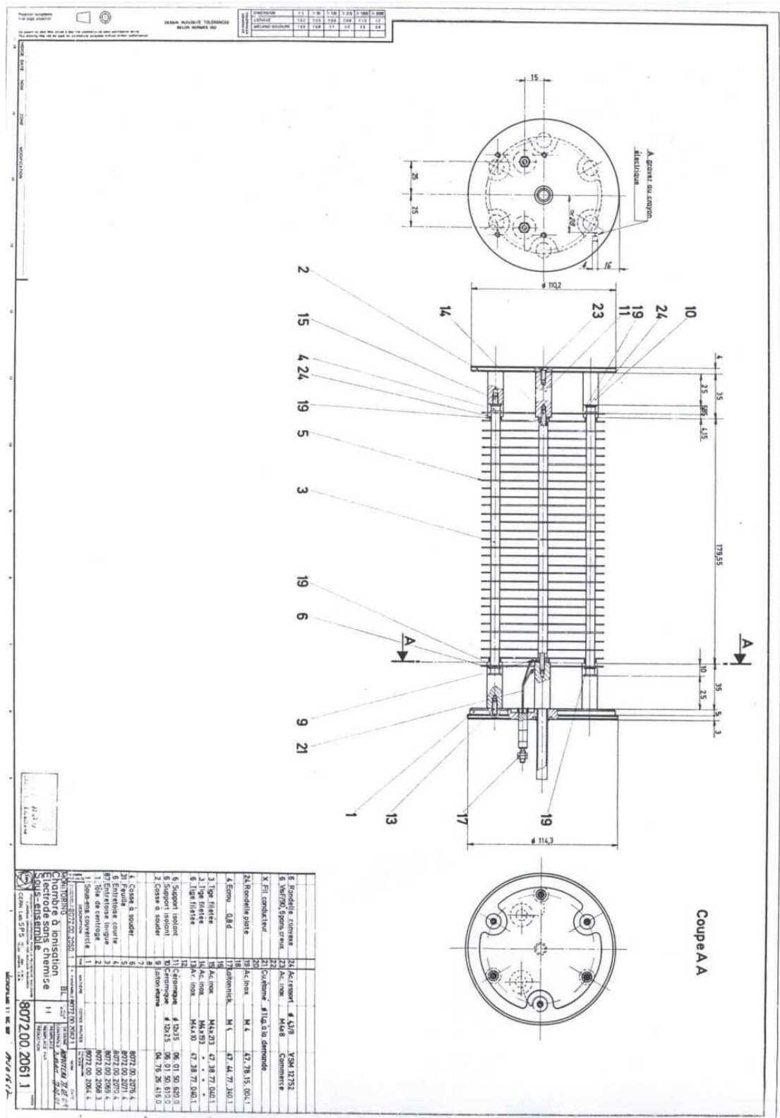
Figure D.1: Technical drawing of the SPS detector
