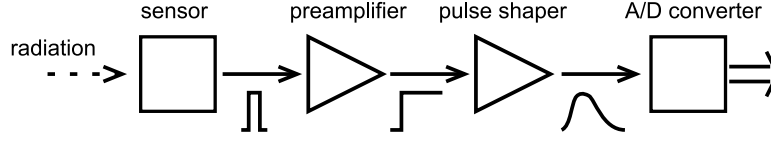
Figure 4.1: Detector system chain
