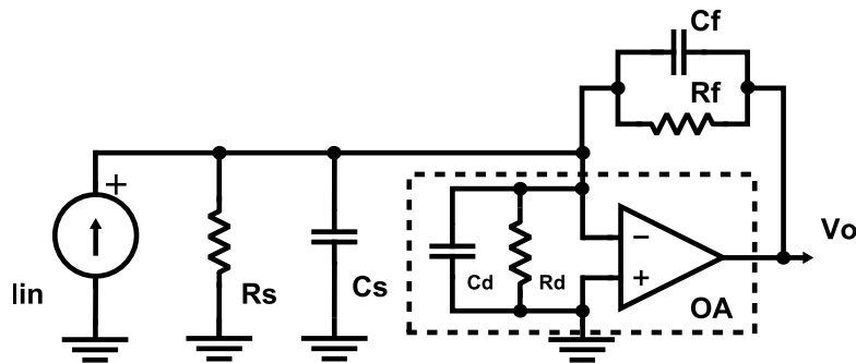
Figure 3.4: Transimpedance amplifier with stray capacitances
