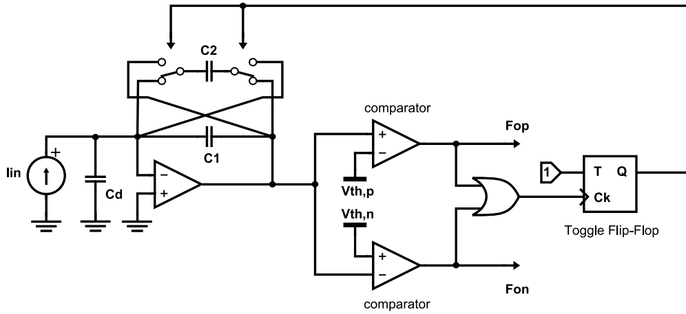
Figure 5.2: CFC implementation through a switched capacitor.
