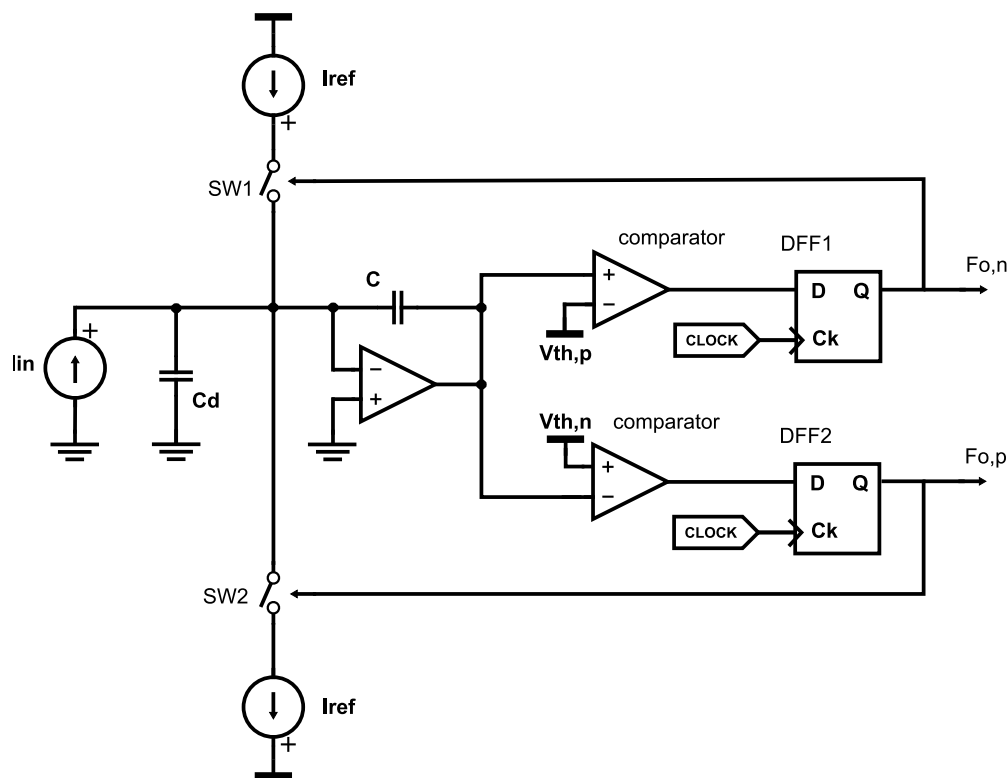
Figure 5.7: Synchronous CFC implementation.
