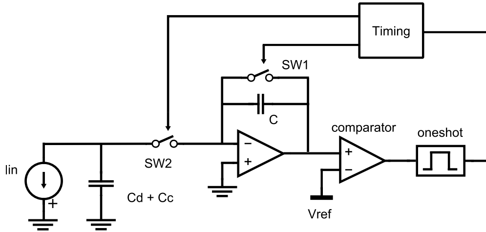
Figure 3.25: Improved CFC with voltage reset.
