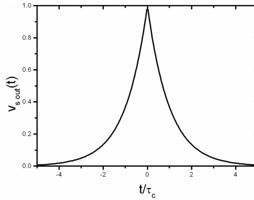
Figure 4.4: Infinite cusp
