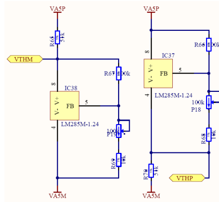
Figure 5.9: Voltage references
