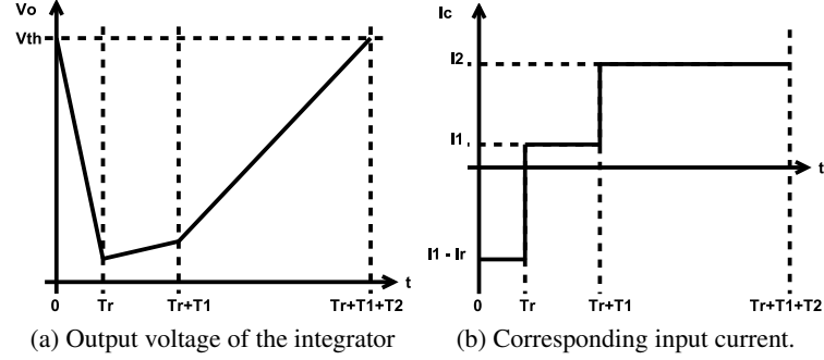
Figure 3.23: Response of the CFC to a current step.
