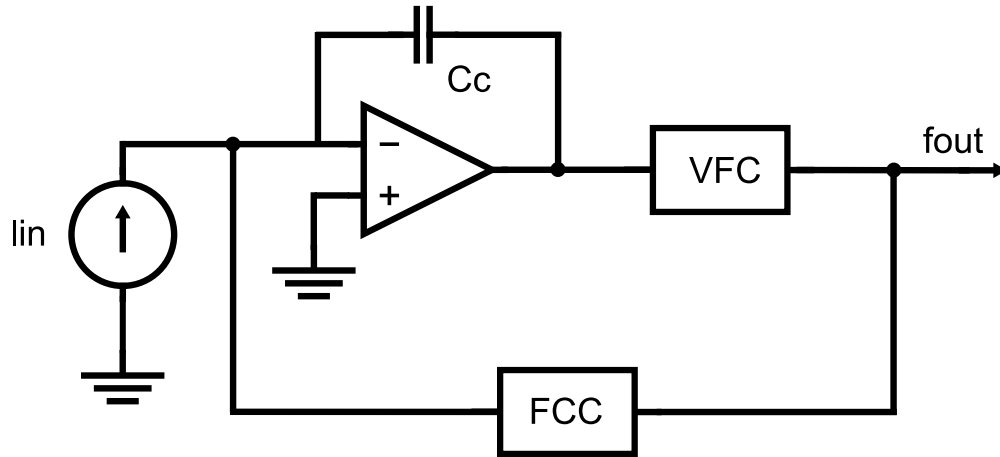
Figure 3.28: Architecture of a CFC with feedback.
