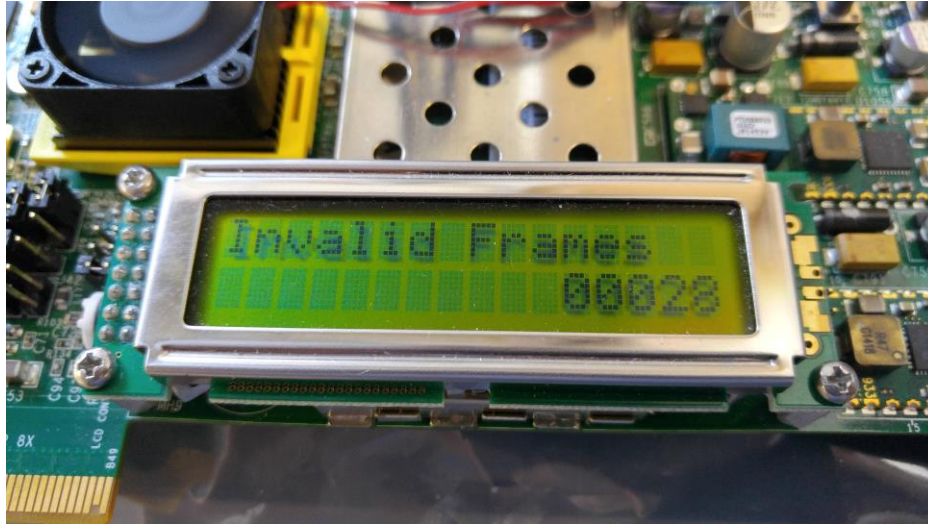
Figure 3.17: Invalid frames displayed on LCD screen. Image depicts invalid frames being sent deliberately to test proper functionality of LCD.
