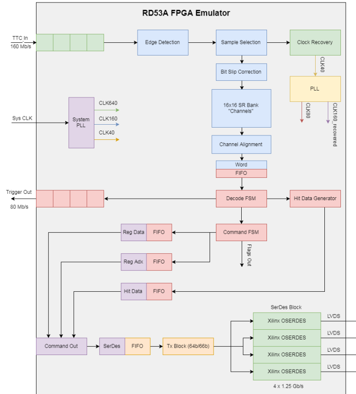
Figure 2.3: RD53A Emulator Block Diagram
