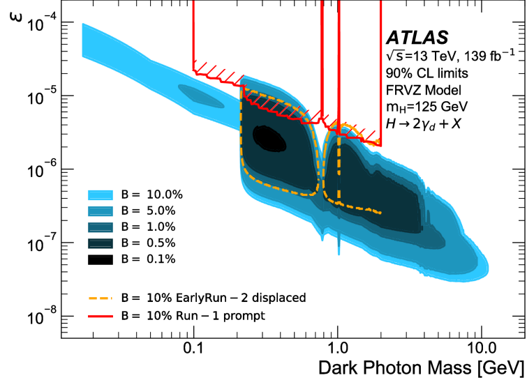
Figure 6.12: The figure shows two-dimensional 90% CL exclusion contours as a function of the dark-photon mass and of the kinetic mixing parameter \epsilon in the context of the FRVZ model hypothesis. In particular the figure refers to the case of the production of SM-like Higgs boson in the H \rightarrow 2\gamma_d + X process. These limits are obtained assuming a decay branching fraction of the Higgs boson into dark-photon ranging between 0.1% and 10%, where each region filled with darker shades of blue correspond to contours obtained considering a lower branching fraction. The figure also shows the respective excluded regions from the previous ATLAS displaced DPJ search [3] (orange line) and ATLAS prompt [4] (red line) DPJ search. Figure from [2].
