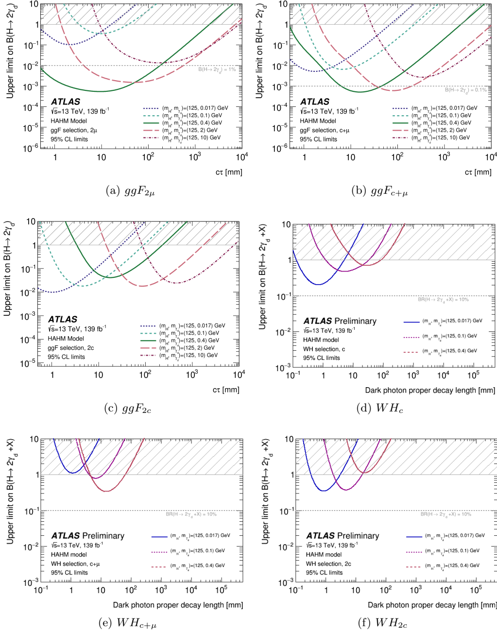
Figure 6.8: Observed upper limits, at the 95% CL, on the branching ratio ( B ) for the process H \rightarrow 2\gamma_d , when considering the HAHM model and the production of a SM-like Higgs boson. Limits in function of the dark-photon c\tau are shown for different choice of the dark-photon mass. The limits for the ggF search channels are reported in separated sub-figures respectively for the ggF_{2\mu} (a), ggF_{c+\mu} (b) and ggF_{2c} (c). For what concerns the results from the WH channels, they are shown in (d) for WH_c , (e) for WH_{c+\mu} and (f) for WH_{2c} . In this interpretation, no limits are set in WH case for dark-photon masses above 400 MeV. In all the sub-figures, the region where the hatched band is present, highlights the fact that the branching ratio considered becomes larger than unity. Figures partially adapted from [2].
