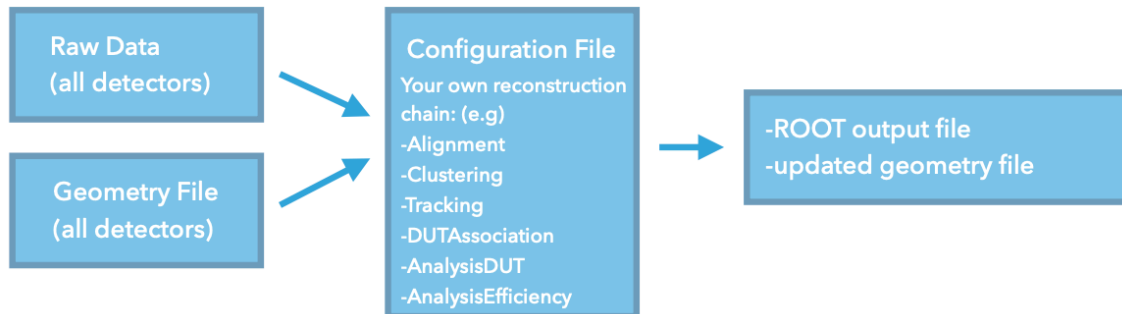
Figure A.5: Schematic illustration of the testbeam data reconstruction workflow when using the Corryvreckan framework [121].
