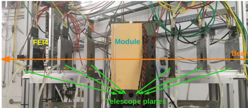
Figure A.4: A photograph of the EUDET telescope [126] and the tested module setup from the April 2019 testbeam. The six telescope planes are visible, with the ITk Long Strip module situated between the two groups of three telescope planes. The FE-I4 timing plane is also visible.
