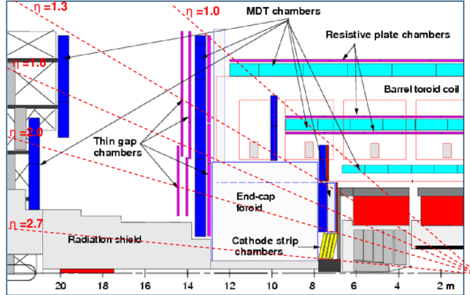
Figure 2.12: Schematic view of the longitudinal projection of the muon spectrometer [54].
