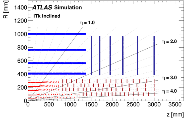
Figure A.1: Schematic layout of one quadrant of the ATLAS ITk detector [120]. The red coloured lines corresponds to the ITk pixel sub-detector layers, while the blue components represent the ITk strip sub-detector layers. The horizontal axis goes along the beam line and the origin of axes lies in the interaction point. The vertical axis corresponds to the radius measured from the beam axis.
