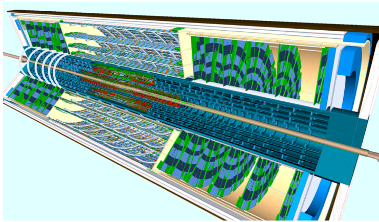
Figure A.2: Simulated layout of the ATLAS ITk tracking detector [120], with the inner pixel sub-detector surrounded by the strip sub-detector.
