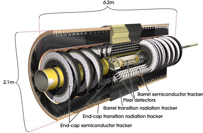
Figure 2.7: Illustration of the ATLAS inner detector system [42].
