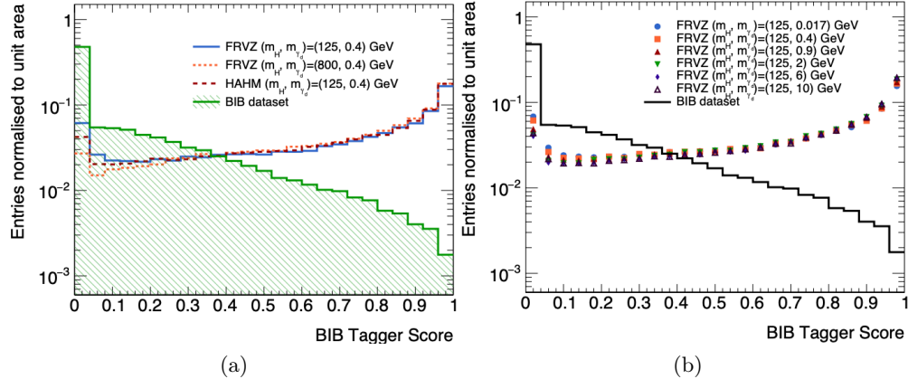
Figure 5.11: Distributions are shown for the output score distribution of the BIB tagger for cDPJs from BIB jets and different set of signals: in (a) different samples with a dark-photon mass of 0.4 GeV are shown, while the distributions relative to different mass points of the FRVZ model are shown in (b).
