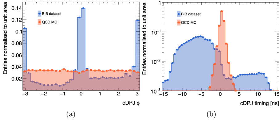
Figure 5.9: Distributions are shown for two relevant variables variables, comparing cDPJs reconstructed from BIBs and multijet simulated events. The \phi distribution is shown in (a) with the characteristic peaks around \phi = 0 and \pm\pi and the timing of the cDPJ is shown in (b).
