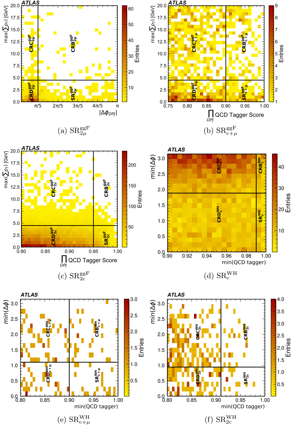
Figure 6.4: The figure shows the per-event distributions in the ABCD planes, for all the six orthogonal ggF and WH category channels, when running on the full Run-II dataset collected by ATLAS. In Figures (a, b, c), the distribution for the ggF category channels is shown, while in figures (d, e, f), the event distribution of the WH category channels is shown. Figures from [2].
