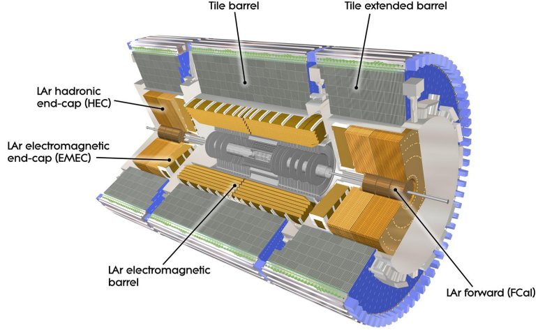
Figure 2.9: Cut-away view of the ATLAS calorimeter system [48].
