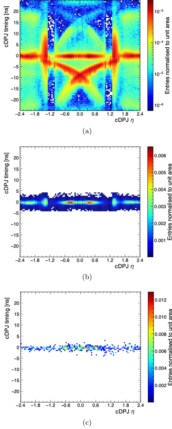
Figure 5.16: 2D distributions of the cDPJs timing vs \eta in the BIB-enhanced sample. (a) shows events entering the ggF_{2c} channel, while (b) shows the events after the timing and BIB tagger cuts. Finally, events entering the ABCD plane are visible in (c), for which no pattern with the characteristic of events originating from BIB is observed.
