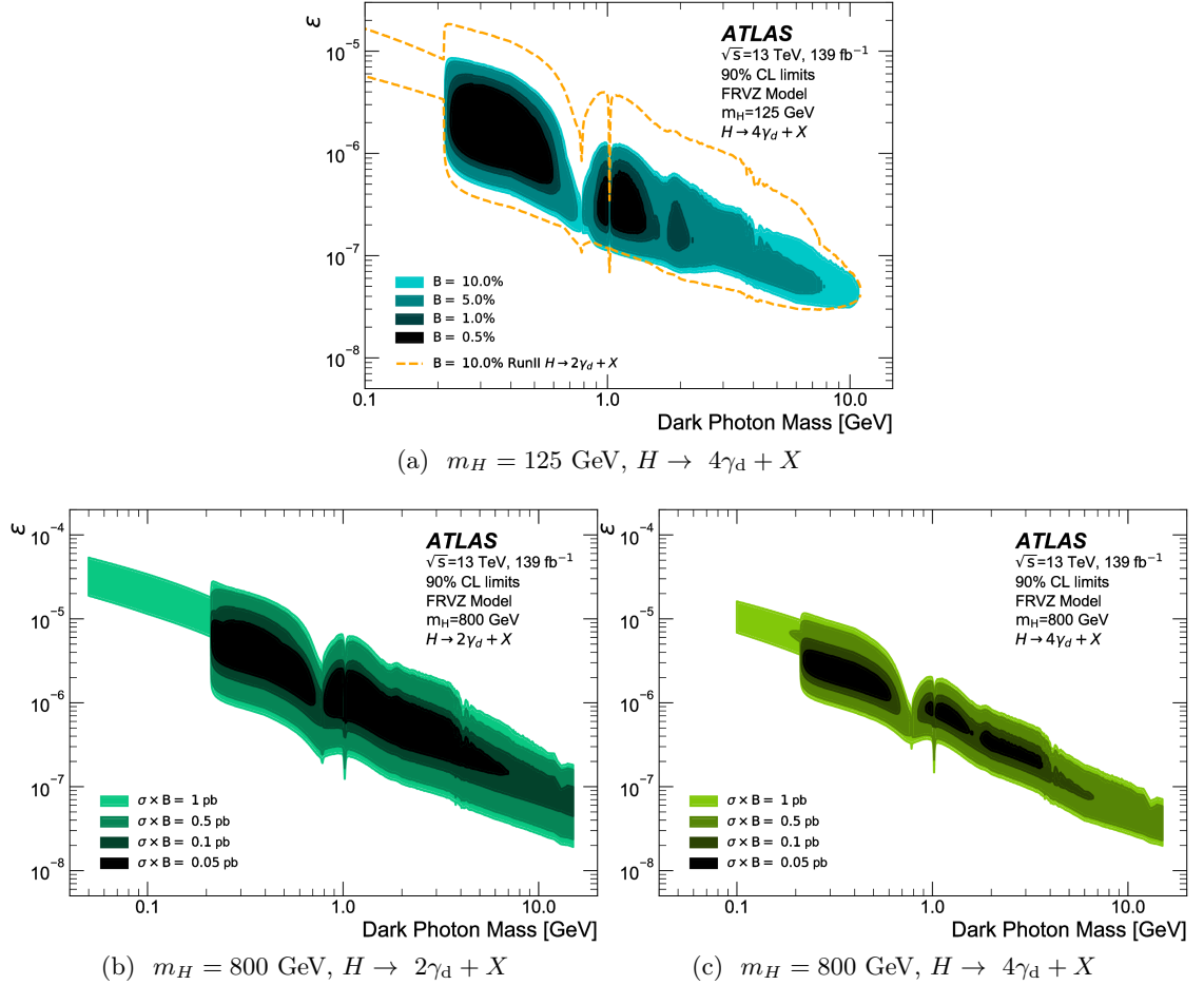
Figure 6.14: Figure showing the two-dimensional exclusion contours for the FRVZ signal model alternative scenarios. In particular, (a) refers to the exclusion contours, as a function of the dark-photon mass and the kinetic mixing parameter, in the case of SM-like Higgs boson production involving the H \rightarrow 4\gamma_d + X process. As a reference is shown also the 10% contour obtained from the H \rightarrow 2\gamma_d + X process (see Figure 6.12), visible as an orange dashed line. In (b) exclusion contours are presented in the case of an 800 GeV Higgs-like boson production involving the production of two dark-photons in the final state. Finally, the exclusion contours presented in (c) are relative to the H \rightarrow 4\gamma_d + X process involving the production of an 800 GeV Higgs-like boson. In (a) the exclusion regions are reported for various choices of the Higgs boson branching fraction into dark-photons, while in (b) and (c) the excluded regions are reported for different choices of the \sigma \times B of the Higgs-like 800 GeV scalar. Figures from [2].
