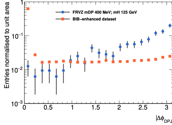
Figure 5.14: Normalised distributions of the \Delta\phi_{DPJ} variable shown for events in the BIB-enhanced dataset and in different signal samples. It can be noticed how a cut at high angular separation between the DPJs in the event is helpful in rejecting the background.
