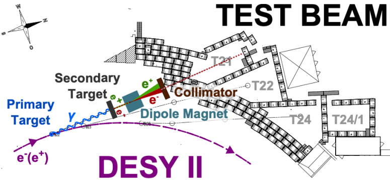
Figure A.3: Scheme illustrating the layout of the DESY-II test beam facility [125].
