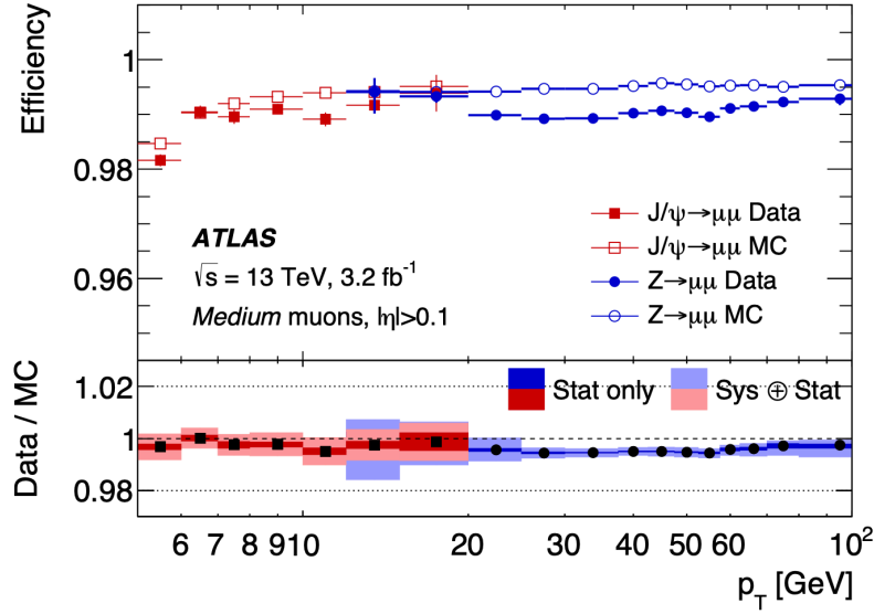
Figure 4.2: Reconstruction efficiency for the medium muon selection as a function of the transverse momentum of the muon, in the region 0.1 < |\eta| < 2.5 obtained with Z \rightarrow \mu^+\mu^- and J/\Psi \rightarrow \mu^+\mu^- events [90].
