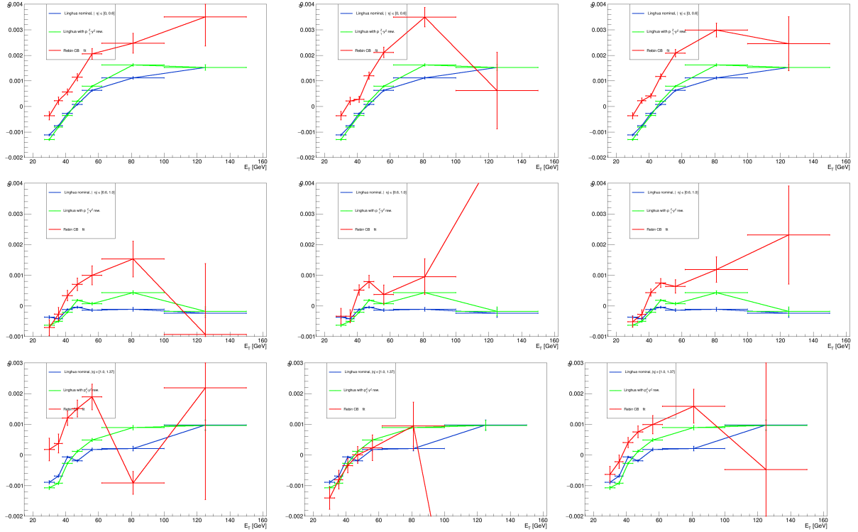
Figure 3.21: Linearity measurements for various |\eta| regions for \eta < 0 (left), \eta > 0 (right) and inclusive in \eta . Red values stand to the ones found in this study with CB fit, green and blue represent m_{ee} linearity found in [71] with and without p_T^Z - y^Z reweighting, respectively. The rows stand for various \eta regions: [0, 0.6] , [0.6, 1.0] and [1.0, 1.37] , respectively. Source: [76].
