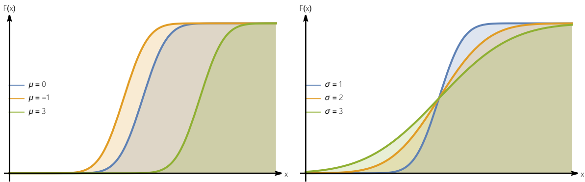
Figure A.2: Examples of cdf of various Gaussian functions.
