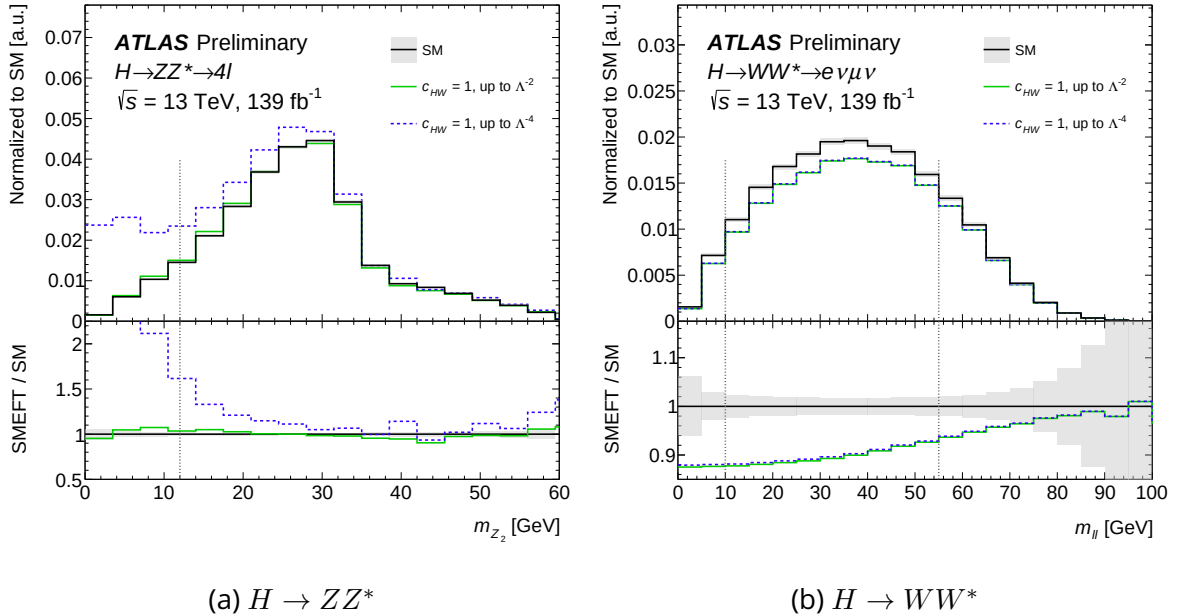
Figure 5.3: Distribution of m_{\ell\ell} observable from (a) H \rightarrow ZZ^* (for the sub-dominant Z ) and (b) H \rightarrow WW^* used in the analysis for the SM prediction and for different values of c_{HW} . Source: [117].
