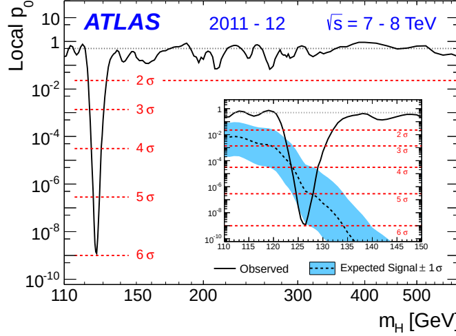
Figure A.11: p -value and the corresponding significance in the historical scan for the search by ATLAS of the Higgs boson signal as a function of its mass. Based on the ATLAS 2011-2012 dataset at \sqrt{s} = 7 and 8 TeV. Source: [146].
