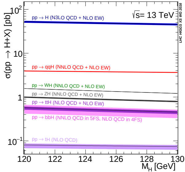
Figure 1.5: Cross-sections of various production modes for the Higgs boson as a function of its mass. The best-known measured value of the mass is \approx 125.11 \pm 0.11 [27]. Source: [28].
