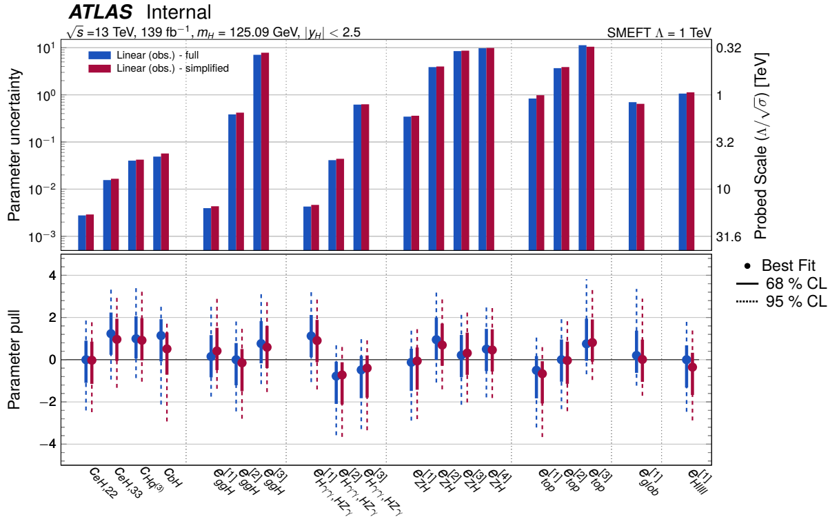
Figure C.16: Comparison of the fit results between the full likelihood (blue) and the simplified one (purple) for the linear parametrisation. Source: [135].
