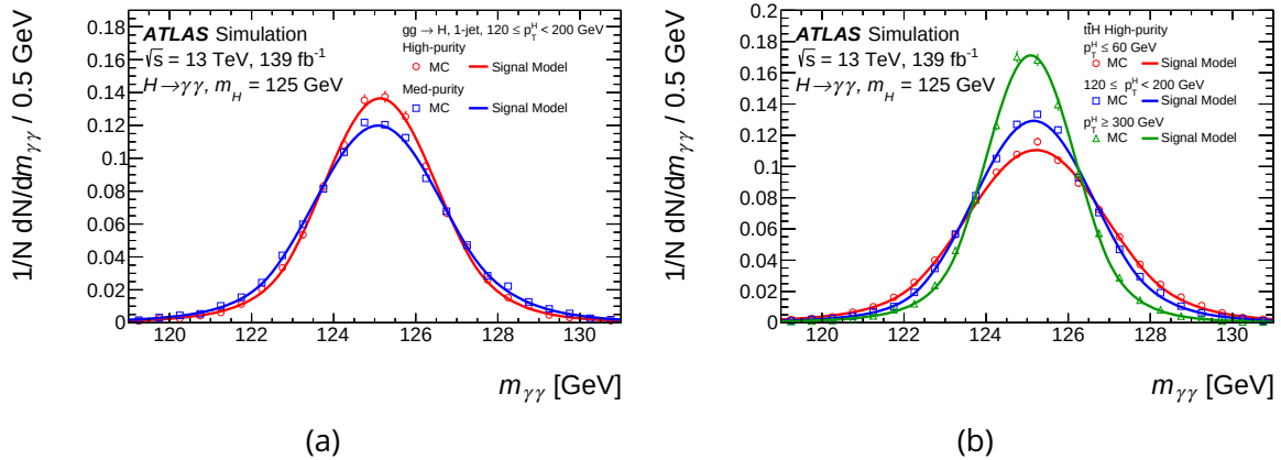
Figure 4.14: Illustrations of signal modelling shape. (a) shows evolution of the spectrum with purity in signal. (b) shows evolution with p_T^H . Source: [39].
