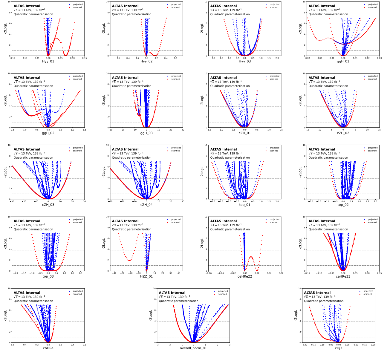
Figure C.11: Nll scans. Source: [135].
