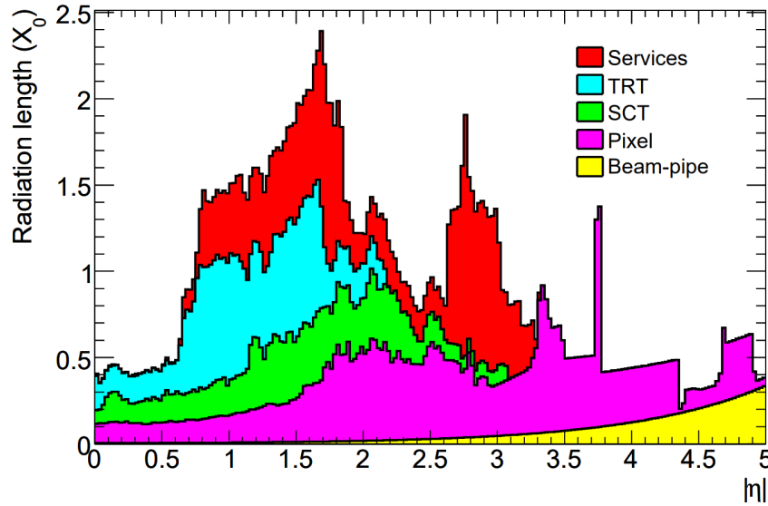
Figure 2.6: Distribution of the material thickness up to the end of ID as a function of |\eta| . Source: [55].
