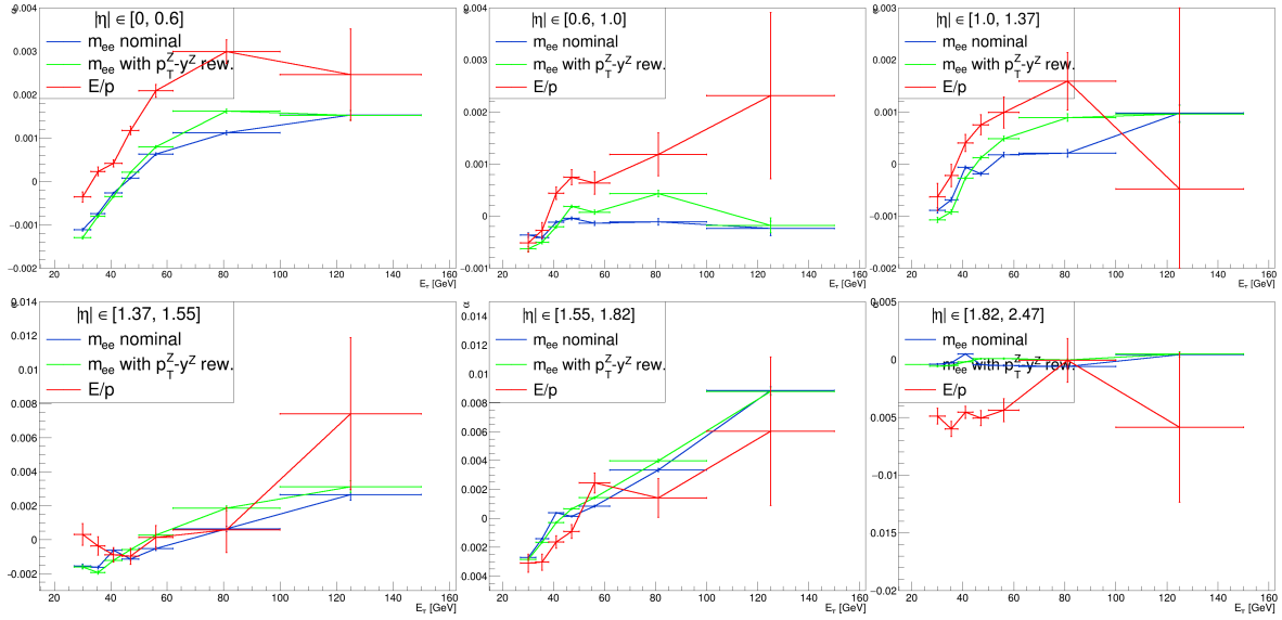
Figure 3.27: Linearity measurements results from E_T/p_T method (red) and nominal m_{ee} template method (blue and green, without and with p_T^Z - y^Z reweighting, respectively). Source: [76].
