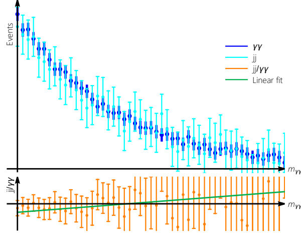
Figure 4.19: Illustration of obtaining linear function for the background reweighting for \gamma\gamma (blue) and j j (cyan) components from data. The j j / \gamma\gamma ratio plot (orange) is fitted with a linear function (green) and this function weights \gamma\gamma MC to emulate the j j component.
