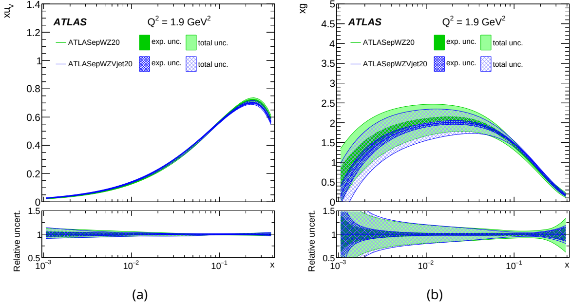
Figure 1.3: Parton distribution function times x (Bjorken scale) of (a) valence up-quark and (b) gluon as a function of x . Source: [25].
