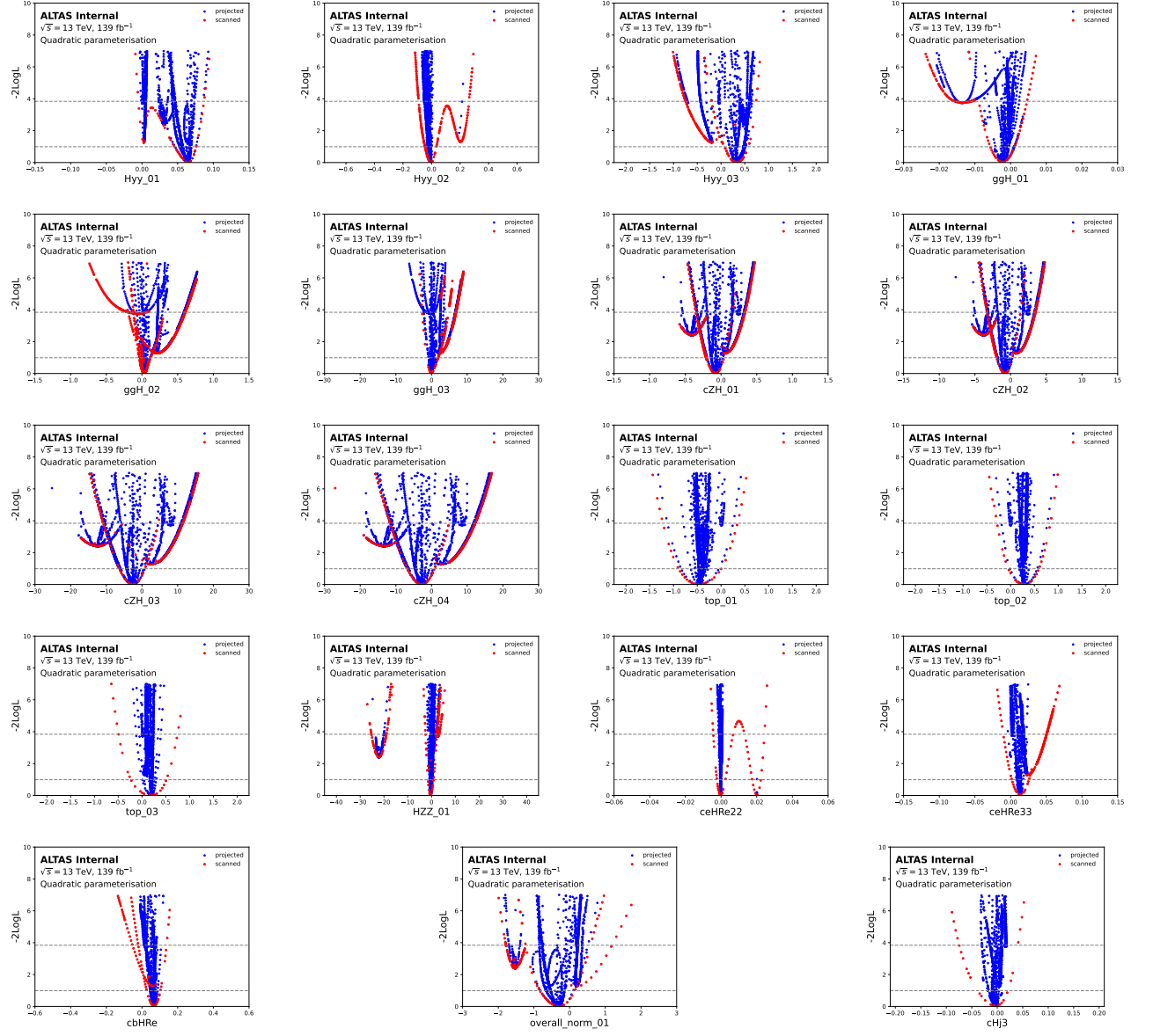
Figure C.12: Nll scans. Source: [135].
