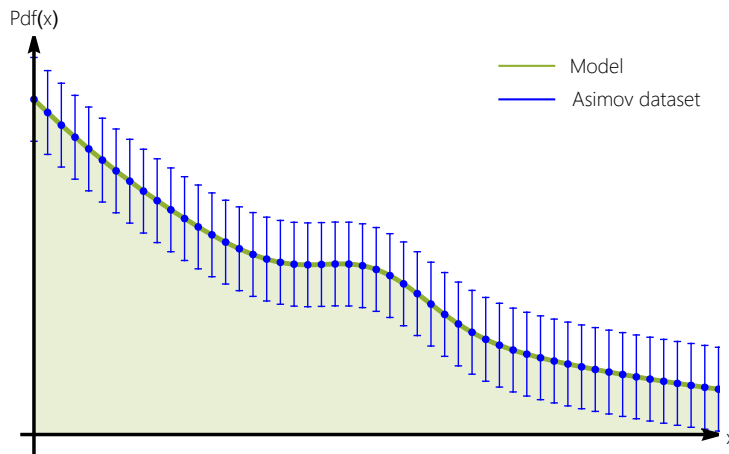
Figure A.12: Example of an Asimov dataset. Generated data (blue) follows exactly the model (green).
