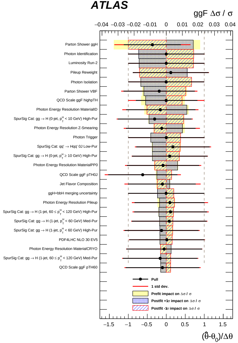
Figure 4.27: Pulls of uncertainties in the 6POI schemes for the ggH production mode. To obtain the pull, signal strength of the other five production modes ( VBF , WH , ZH , ttH and tH ) were kept floating, to match the condition of the combined fit of the production modes signal strength. Source: [39].
