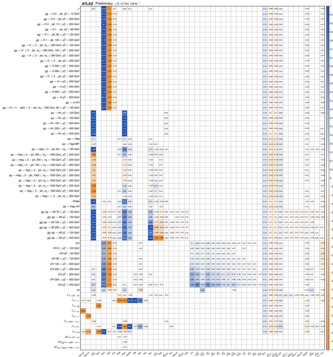
Figure C.18: Linear coefficients \mathcal{A}_{kj}^t , \mathcal{A}_{kj}^f and \mathcal{A}_{kj}^H of the SMEFT parametrisation. The estimated correction factors needed to account for the non-negligible experimental acceptance effects in H \rightarrow ZZ^* and H \rightarrow WW^* decay modes and that affect the impact of certain SMEFT operators are separately provided and labelled as \Delta\Gamma . These correction factors should be added to the corresponding \Gamma term to obtain the parametrisation including acceptance effects. Source: [117].
