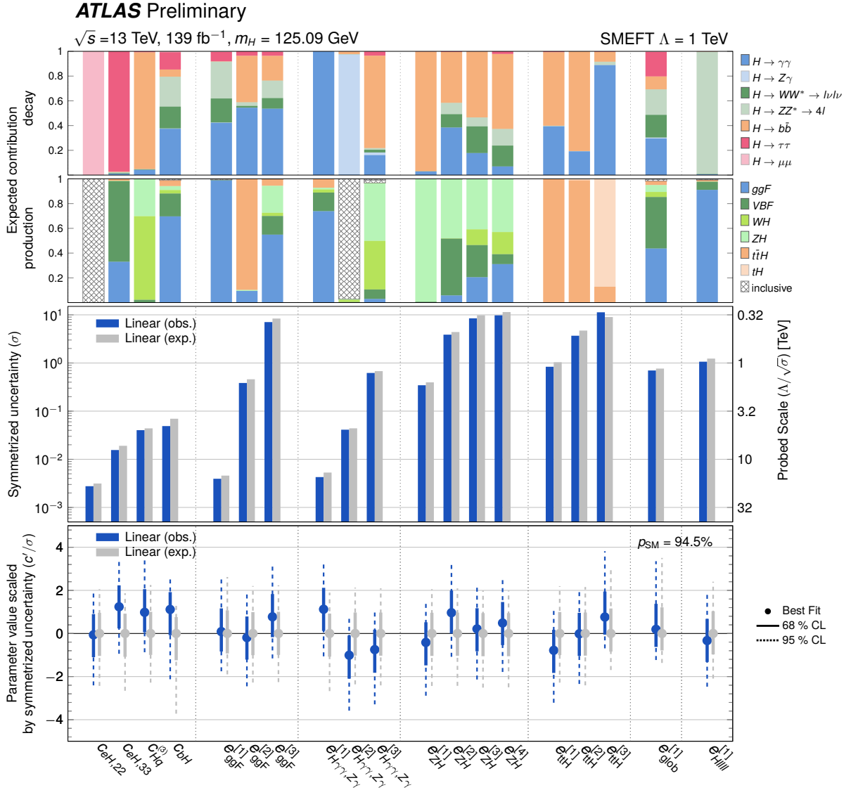
Figure 5.14: Expected (grey) and observe (blue) pull of central values of the Wilson coefficients in the fit-basis (bottom plot), their uncertainties (middle) and relative contributions from each input channel and production mode (top) to the precision of the measurements. The results are obtained under the linear parametrisation. Source: [117].
