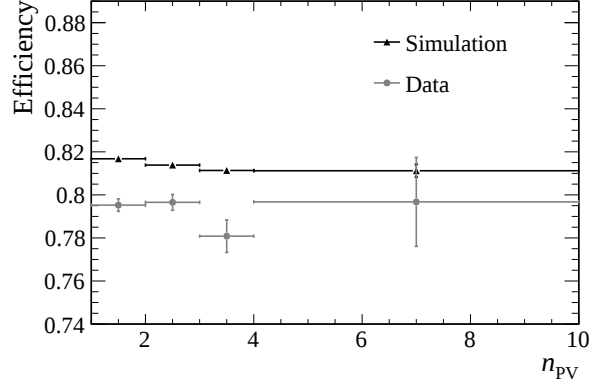
Figure 9.22: Dependence of electron reconstruction efficiency with respect to pile up, i.e. n_{PV} . Both samples in data and simulation have the full kinematic range. A slight dependence is seen in simulation. The uncertainties are too large in data to conform this.
