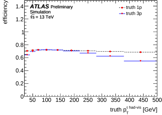
Figure 5.1: Reconstruction efficiency of \tau_{had-vis} , separated in 1p and 3p candidates, as a function of the truth-level p_T of the \tau_{had-vis} object [99].
