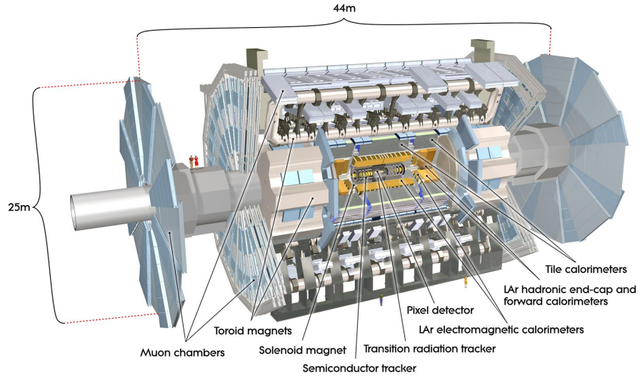
Figure 4.4: Illustration of the ATLAS detector in cut-away view [70].
