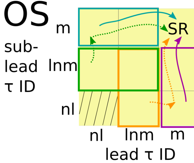
Figure 8.11: Pictorial representation of the fake-factor application for the Fake background estimate in the \tau_{had}\tau_{had} channel. The opposite-sign events are separated into four subregions based on whether the leading and sub-leading \tau_{had-vis} candidate in an event passes the medium (m), the loose but not the medium (lnm) or not the loose (nl) ID working point. Short arrows represent F^{lnm} , while long arrows represent F^{nm} . Positive contributions to the SR are represented by solid arrows, while negative contributions are represented by dotted arrows.
