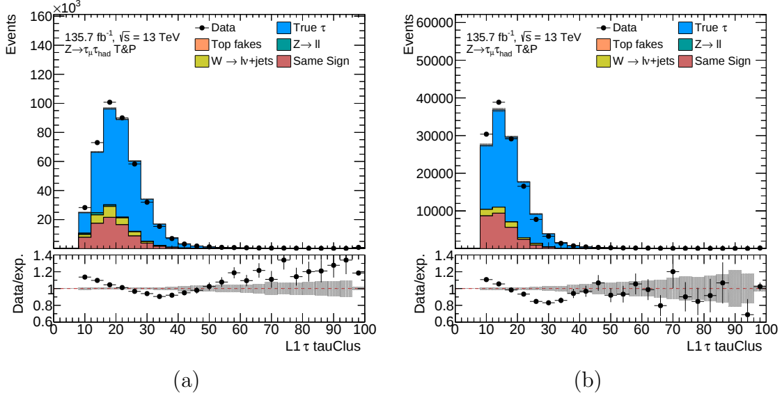
Figure 6.12: SR distributions of the L1 tauClus energy distribution for (a) 1-prong and (b) 3-prong \tau_{\text{had-vis}} candidates.
