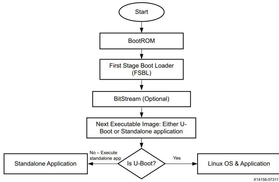
Figure 4.2: Boot process of the Zynq-7000 platform. Figure 4-6 from [40].
