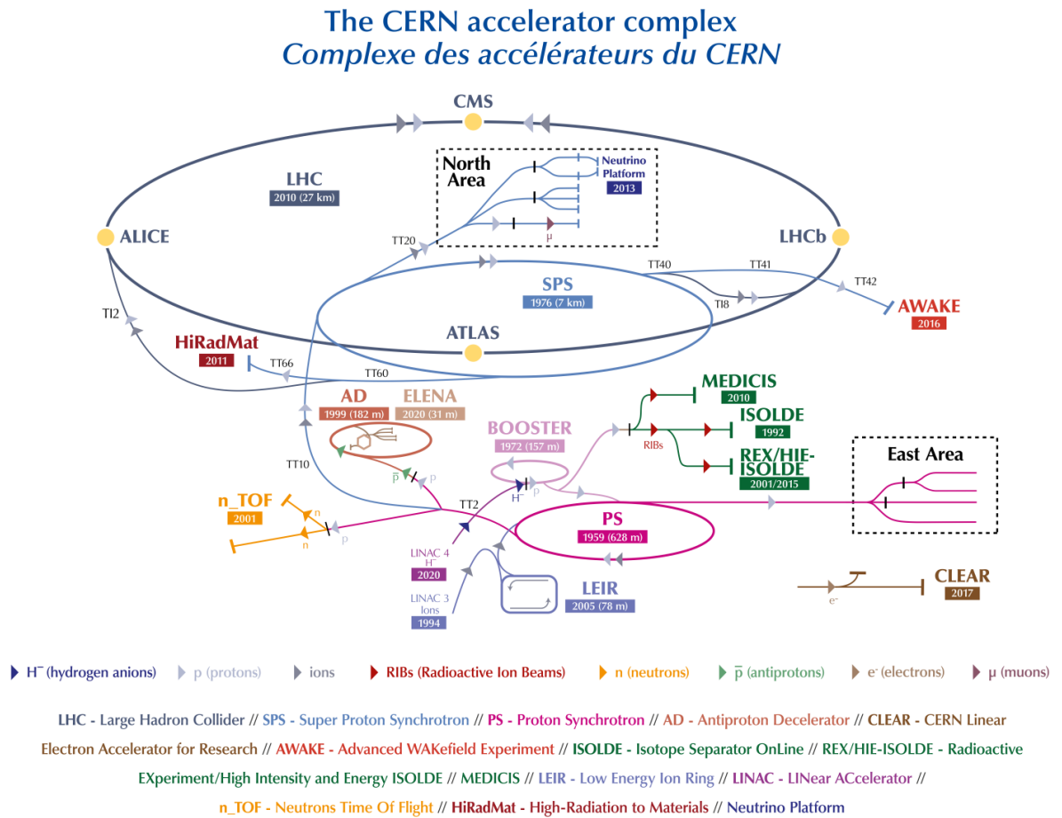
Figure 1.1: CERN accelerator complex diagram, Source: [32]
