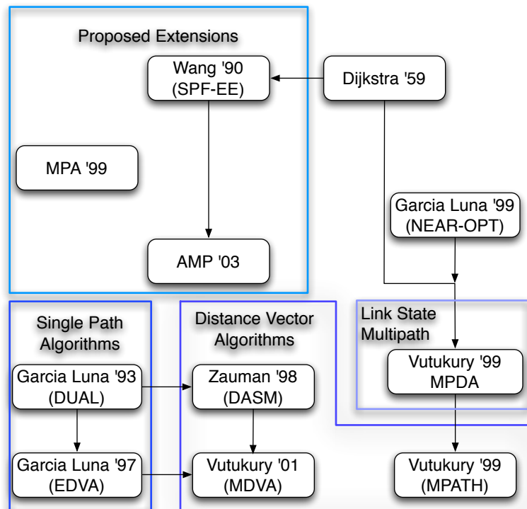
Figure 3.2: The Evolution of multipath algorithms
