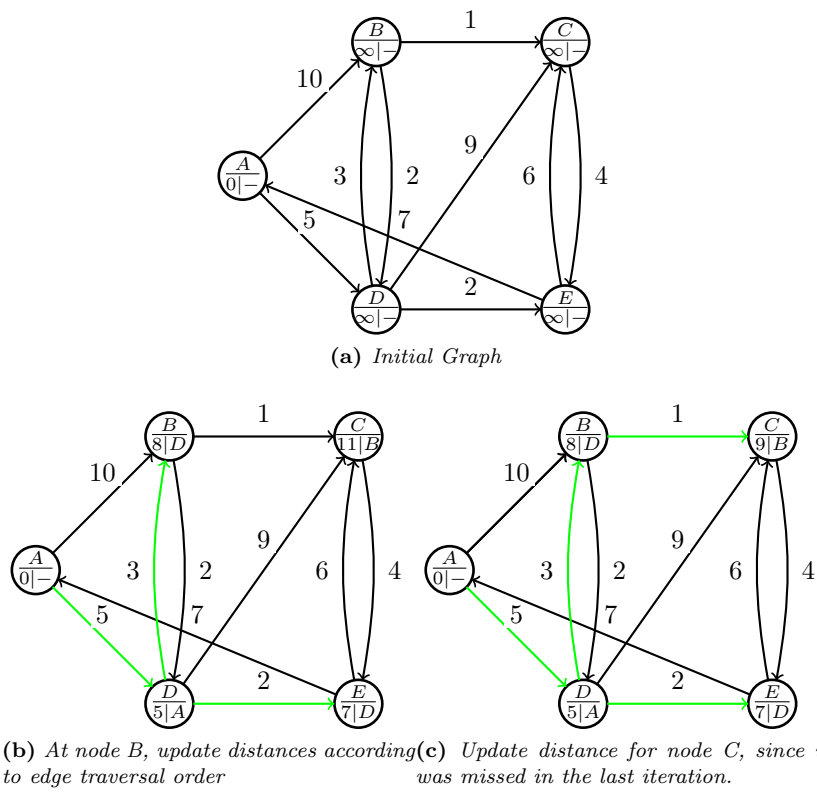
Figure 4.2: Running Example of Bellman-Ford's Algorithm
