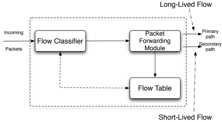
Figure 3.7: The flow classifier.
