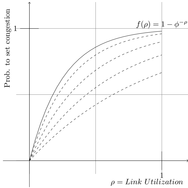
Figure 5.9: The transfer function used in Classical MultiRoute.
