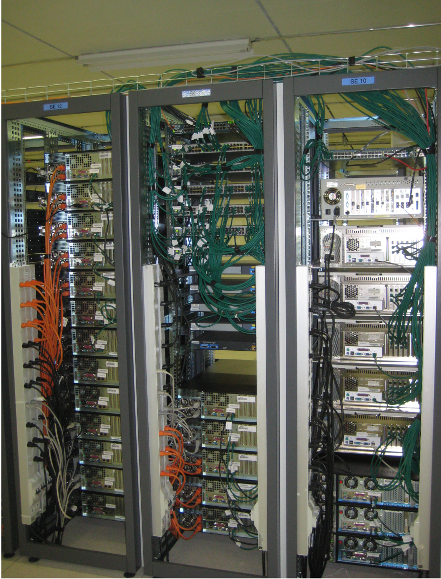
Figure 6.4: The testbed as it is implemented at CERN's computing center.
