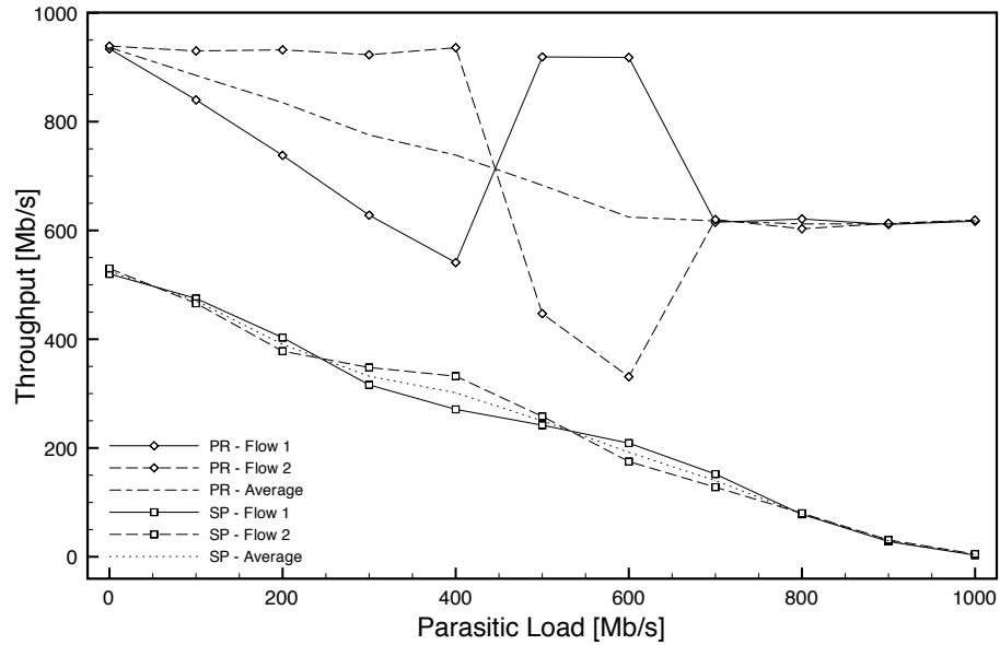
Figure 7.5: Shortest Path versus PathRoute in the presence of Parasitic traffic.
