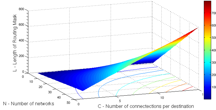
Figure 5.10: Routing Mask Length as a function of N and C .
