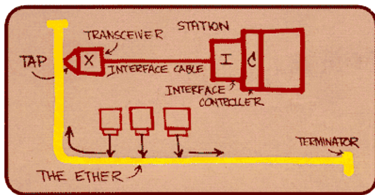
Figure 2.3: The concept of Ethernet, as drawn originally by Bob Metcalfe.
