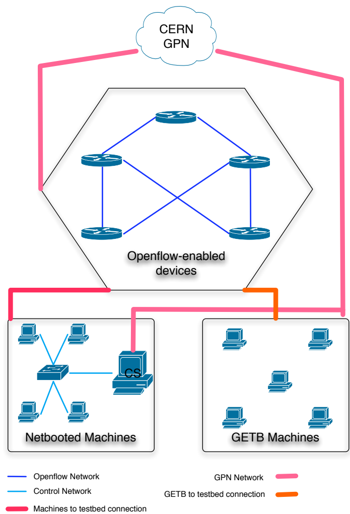
Figure 6.5: The connectivity map of the Testbed.
