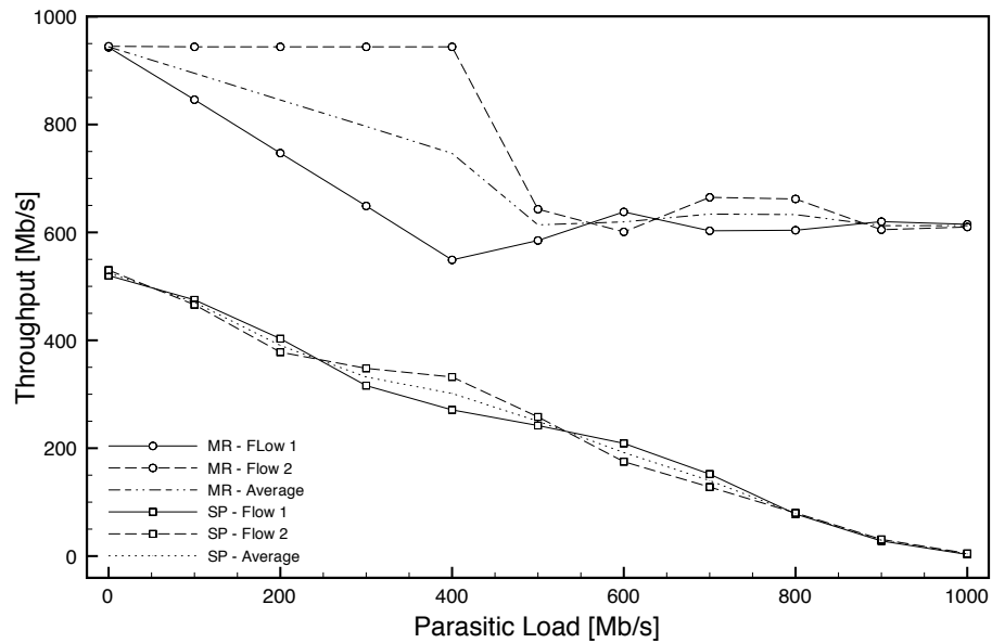
Figure 7.3: Shortest Path versus MultiRoute in the presence of Parasitic traffic.
