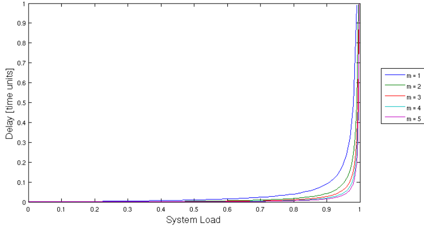
Figure 5.15: Flow delay as function of the load ( = \frac{\lambda}{m\mu} ) and number of servers.
