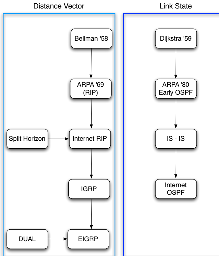
Figure 2.11: Evolution of Implemented Routing Algorithms
