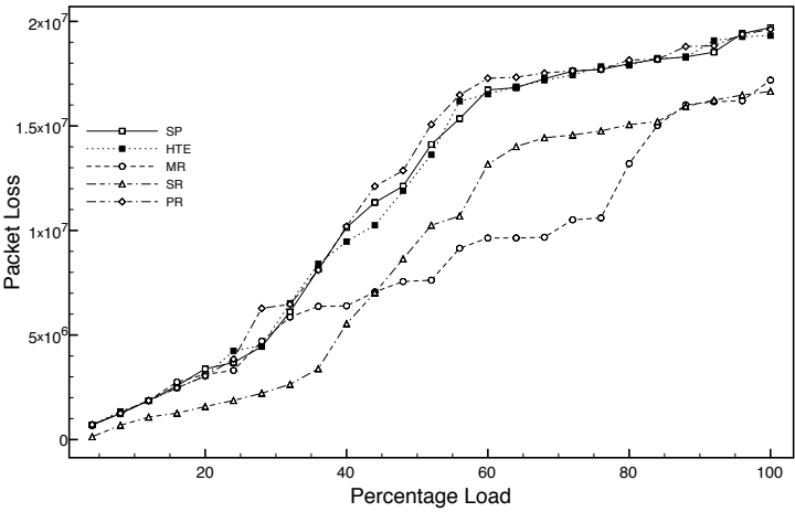
Figure 7.14: Packet Loss for protocols running on the Flower.
