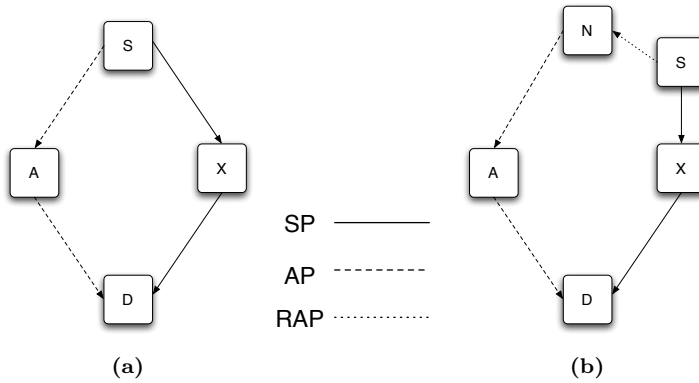
Figure 3.4: An example of SPF-EE
