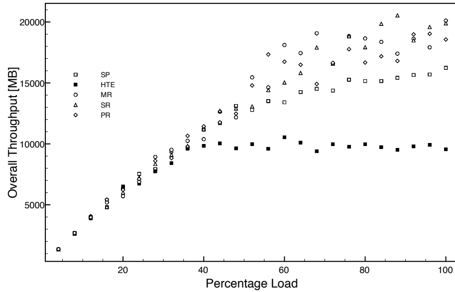
Figure 7.12: Fully-Meshed Traffic running on the Pentagon.
