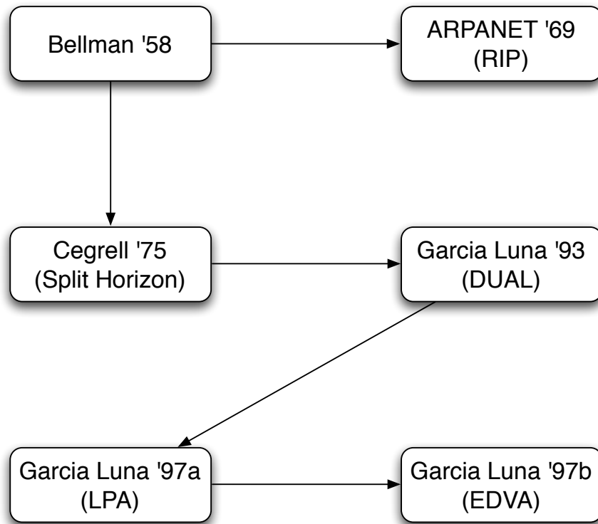
Figure 2.10: Evolution of Distance Vector Algorithms
