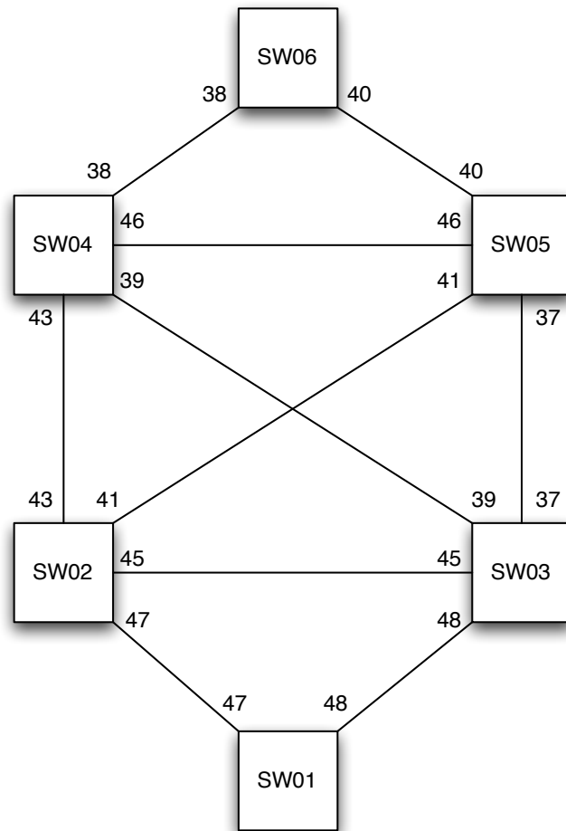
Figure 7.1: The Flower topology.
