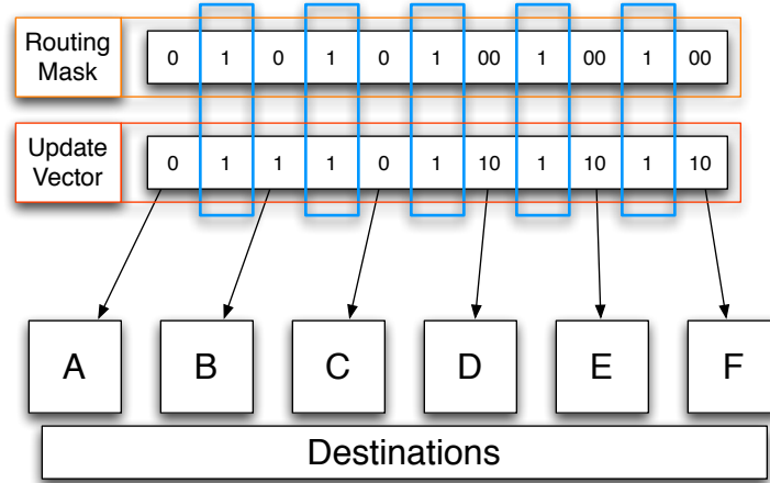
Figure 5.8: Comparing a Routing Mask with its an Update Vector
