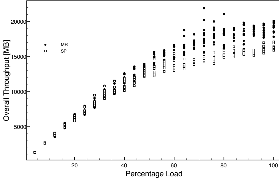
Figure 7.11: Successive Fully-Meshed Traffic running on the Flower.
