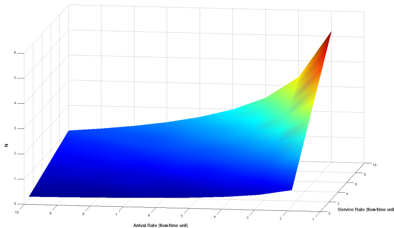
Figure 5.16: Number of flows in each queue
