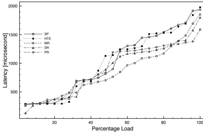
Figure 7.13: Latency plots for protocols running on the Flower.
