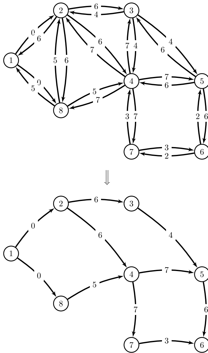
Figure 5.1: Output of the MRPC algorithm
