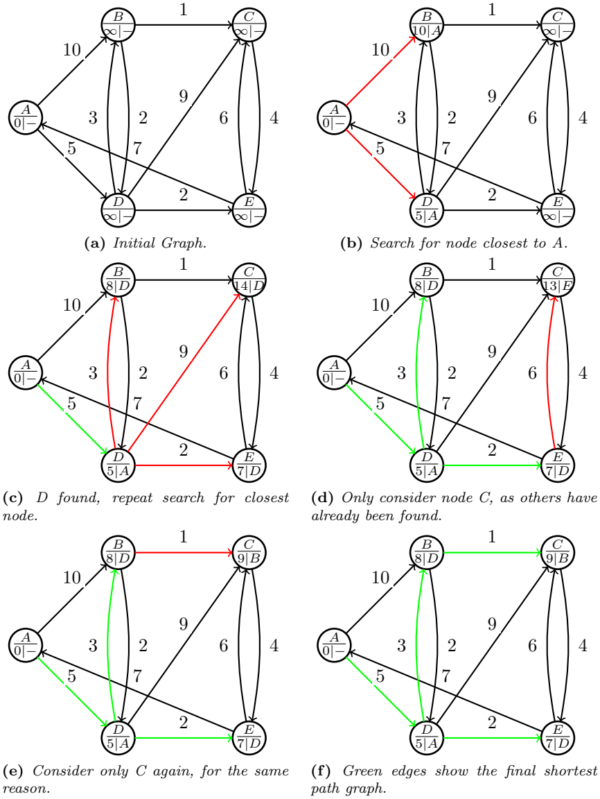
Figure 4.1: Running Example of Dijkstra's Algorithm
