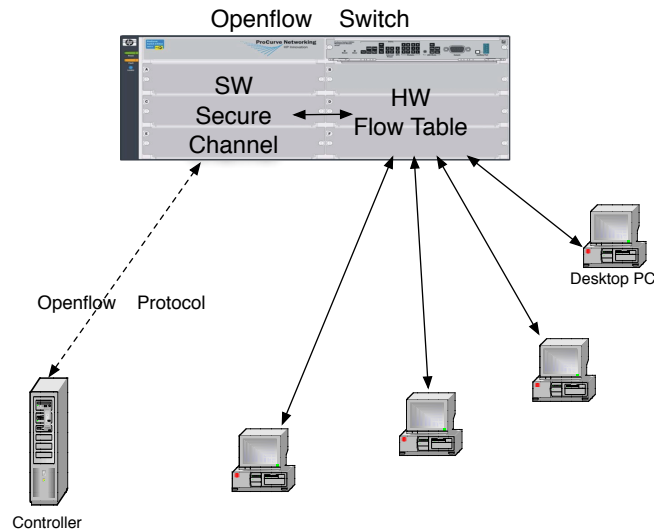
Figure 6.2: The OpenFlow switch.
