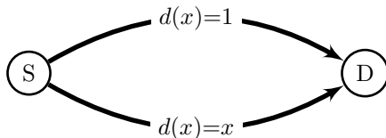
Figure 4.3: Pigou's Example
