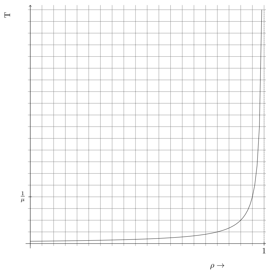
Figure 4.5: Average delay as a function of \rho .
