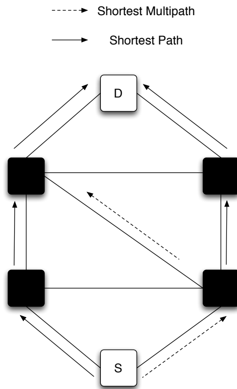
Figure 3.6: An example of Shortest Multipath constructed with DASM.
