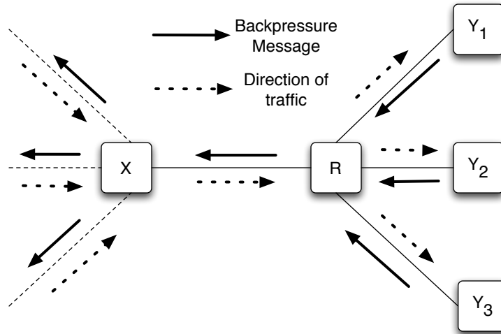
Figure 3.5: An example of AMP.
