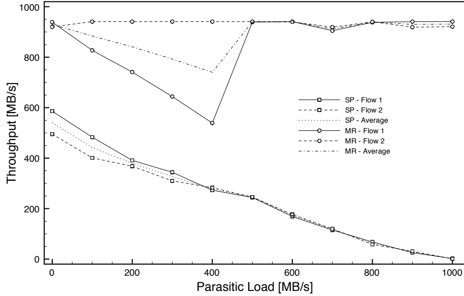
Figure 7.7: Shortest Path versus MultiRoute in the presence of Parasitic Traffic.
