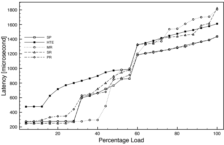
Figure 7.15: Latency plots for protocols running on the Pentagon.
