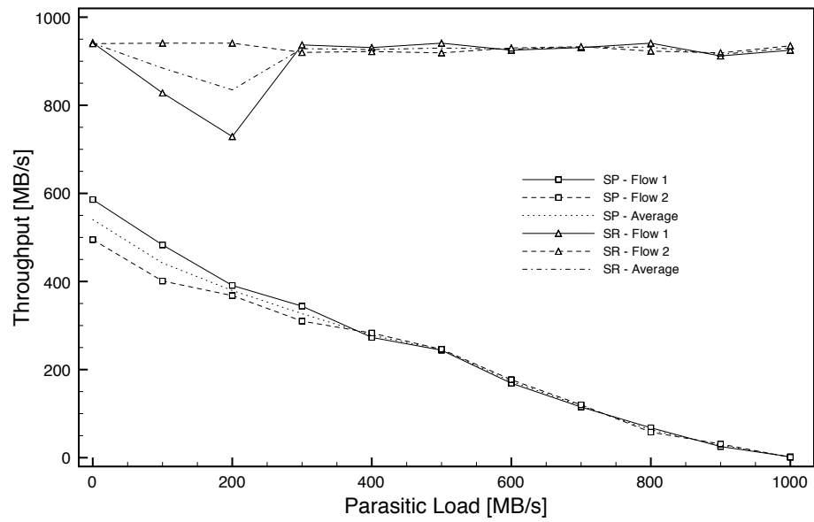
Figure 7.8: Shortest Path versus StepRoute in the presence of Parasitic Traffic.
