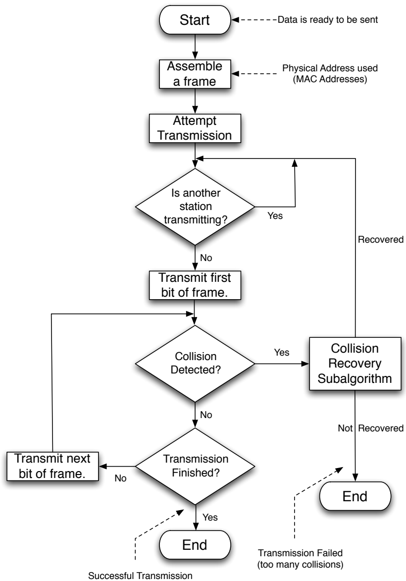
Figure 2.4: A simplified algorithm sketch for CSMA/CD
