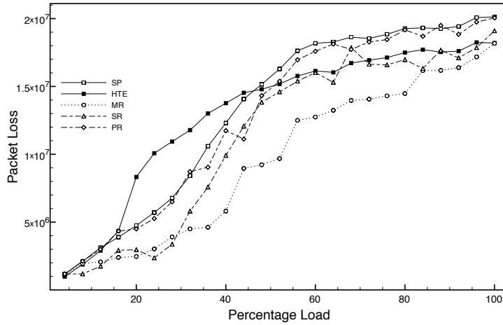
Figure 7.16: Packet Loss for protocols running on the Pentagon.
