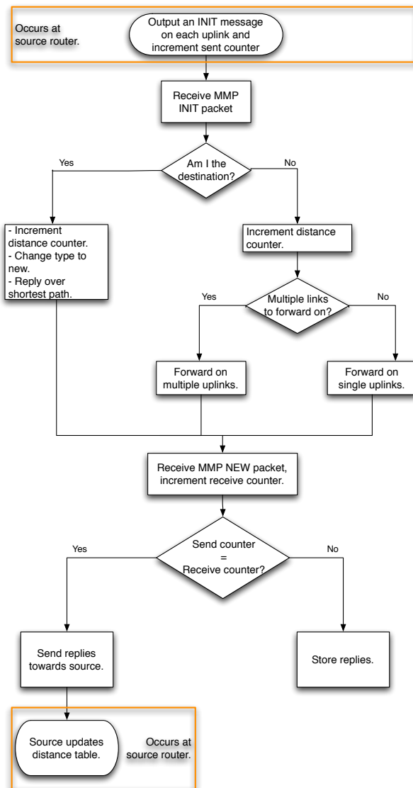
Figure 5.13: Flowgraph of the distance diffusion computation.
