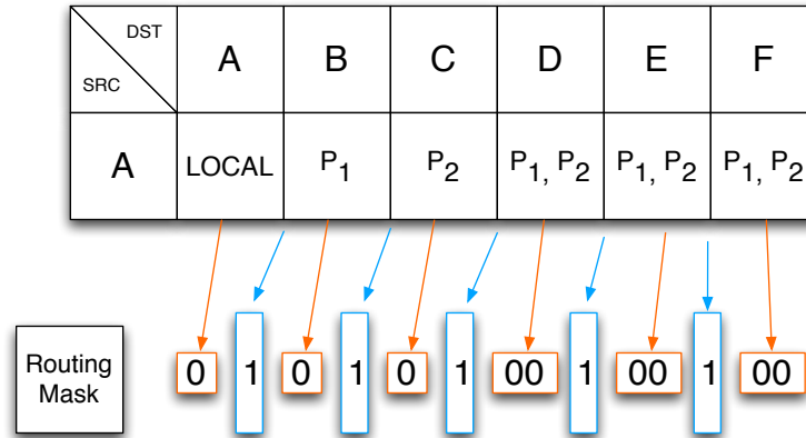
Figure 5.3: A Routing Mask with its associated routing table
