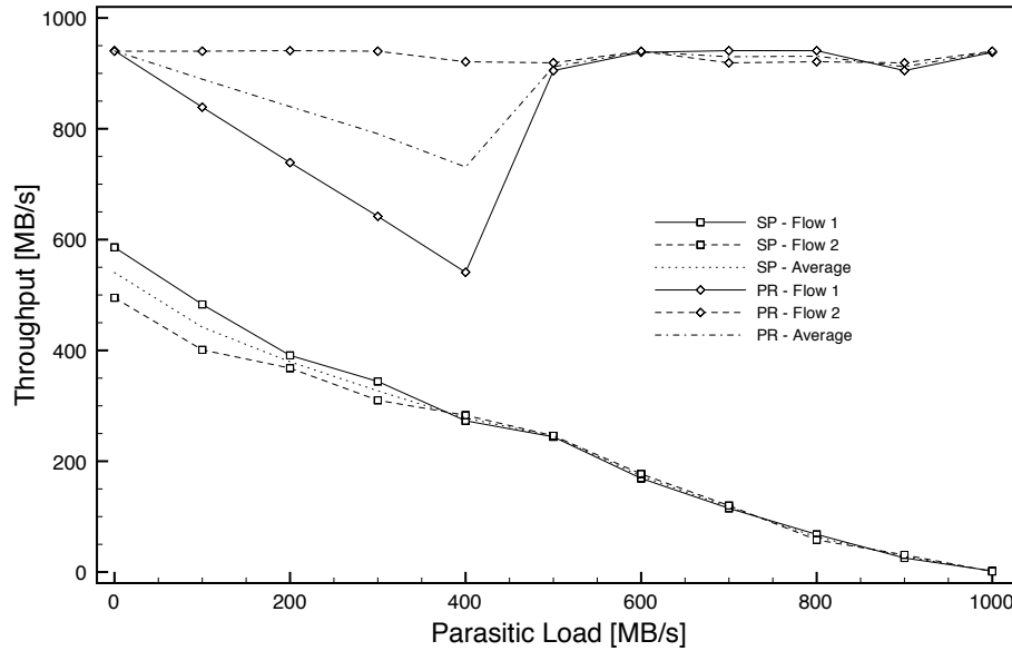
Figure 7.9: Shortest Path versus PathRoute in the presence of Parasitic Traffic.
