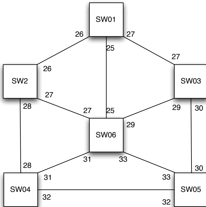
Figure 7.2: The Pentagon topology.
