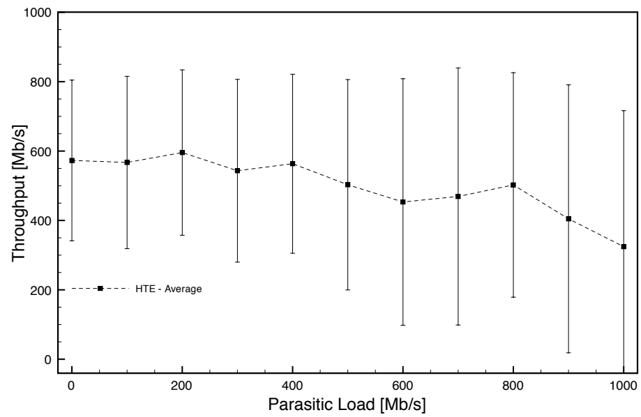
(b) Hash Threshold's throughput variation
