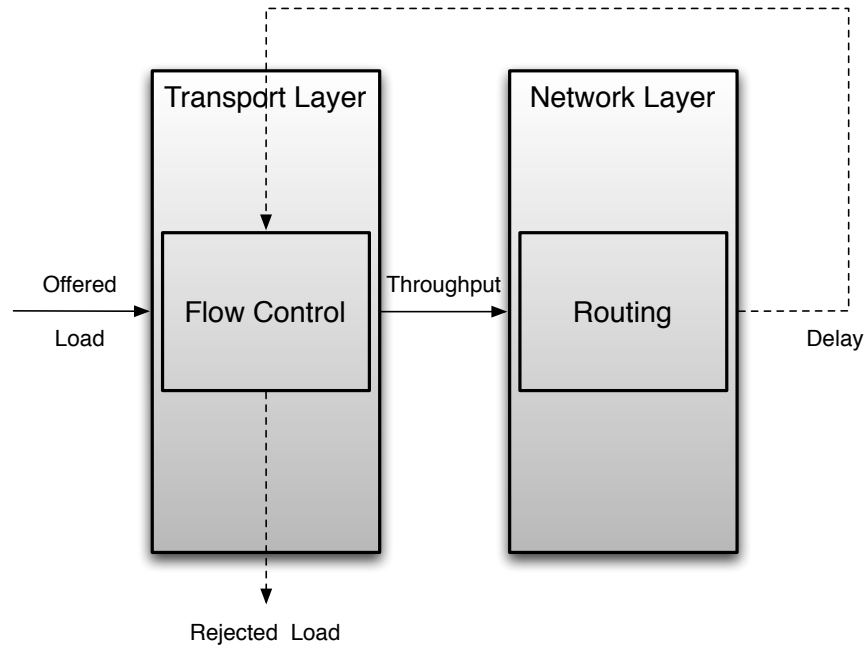
Figure 2.8: Interaction between Transport and Network Layer
