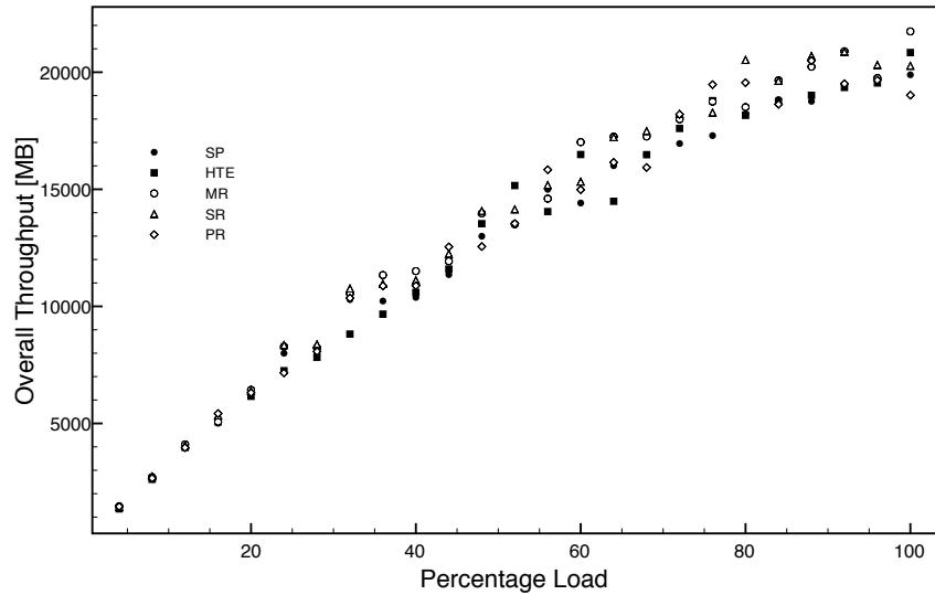
Figure 7.10: Fully-Meshed Traffic running on the Flower.
