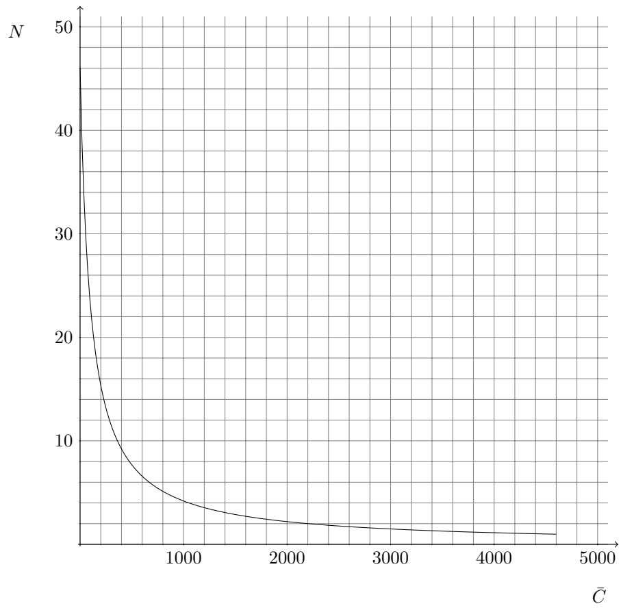
Figure 5.11: Plot of the Routing Mask Limitation
