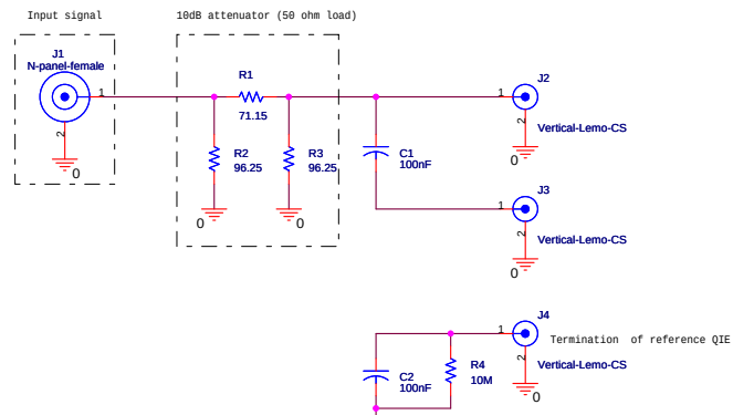
Figure 7.10: Schematic of the splitter used for each BHM channel.
