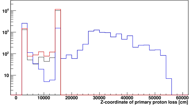
Figure 4.7: Coordinates of the primary proton loss (TCTs are about 148 m from the IP).
