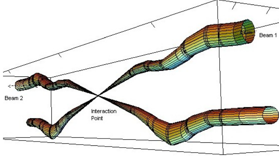
Figure 1.11: The beta function of the two beams near an interaction point [VM].
