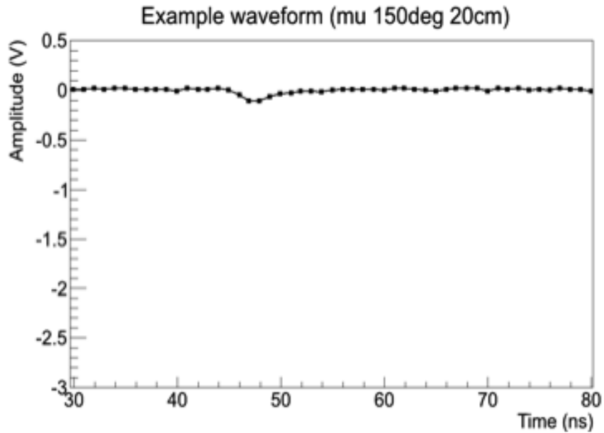
Figure 5.21: Example photomultiplier waveform produced by a relativistic muon passing through the 20 cm quartz bar at 150°, during test beam in T9 area CERN, in 2012 [Amb13].
