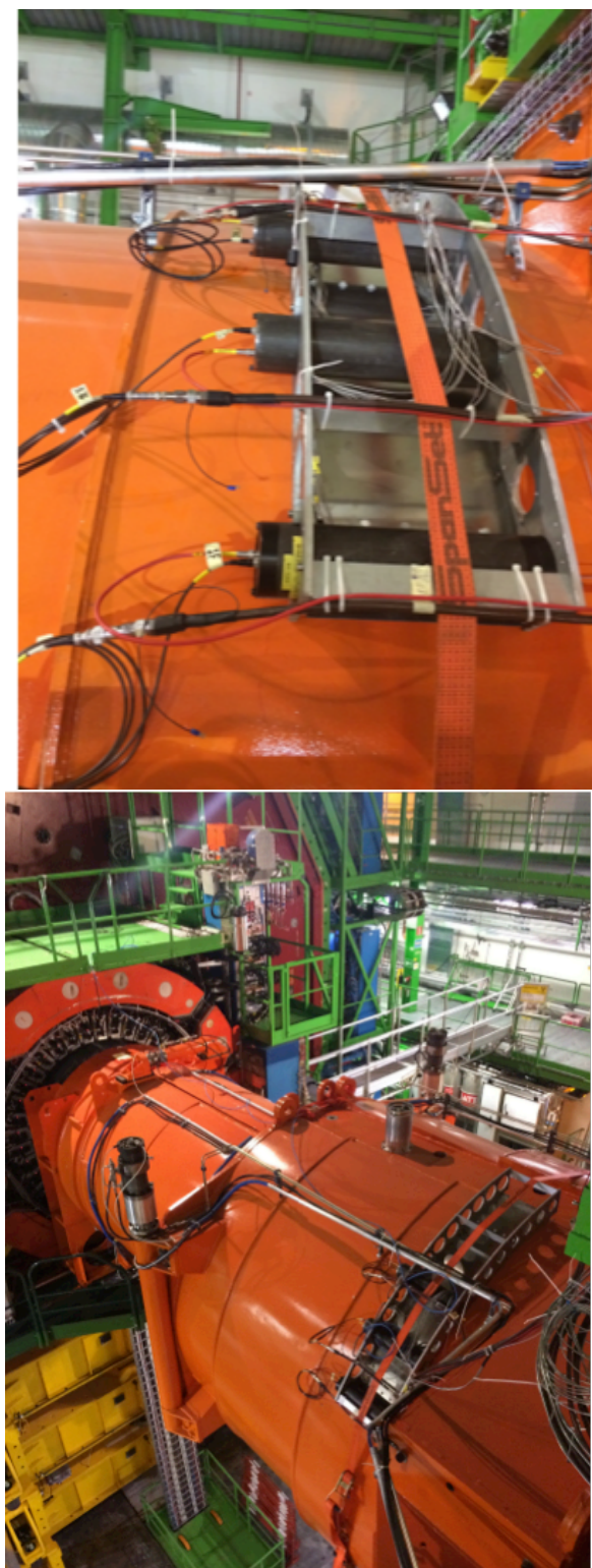
Figure 6.14: Pictures of the installation during the CMS magnet test in November 2014.
