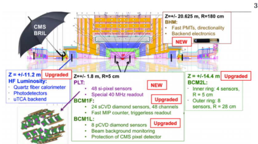
Figure 2.15: The LS1 upgrades of the instrumentation of the BRIL subdetectors [Dab14].
