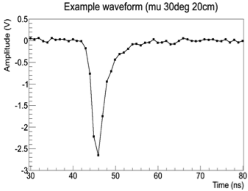
Figure 5.20: Example photomultiplier waveform produced by a relativistic muon passing through the 20 cm quartz bar at 30°, during test beam in T9 area CERN, in 2012 [Amb13].
