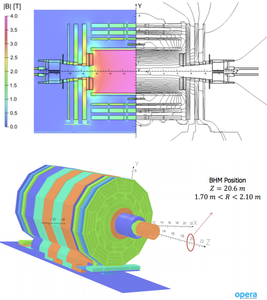
Figure 6.5: The CMS OPERA model before 2014. Value of the field and field lines on the CMS detector for a magnet operation at 3.8 T [Kly13].
