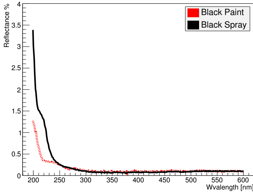
Figure 5.11: The measured reflectance of the two black candidate black materials in the wavelength range of interest.
