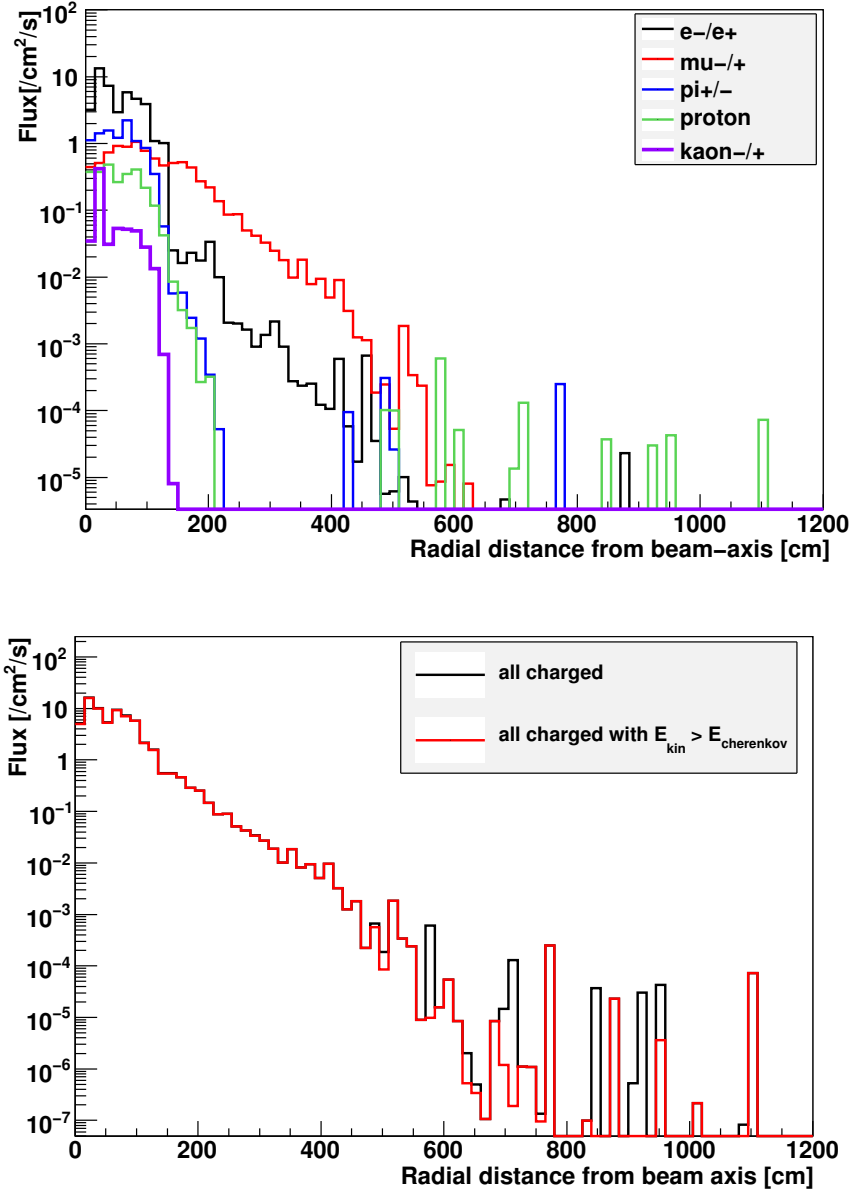
Figure 4.6: Radial particle fluence distributions on the entrance into the experimental area for different particle types (top) and for all charged particles before and after applying the Cherenkov threshold (bottom).
