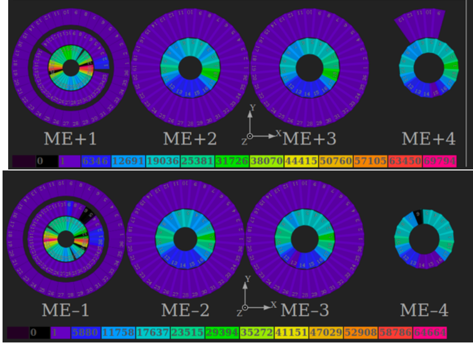
Figure 2.13: The phi distribution of the beam halo rate as seen by the ME stations of the muon system. The numbers in the legend of the two plots need to be divided by 1e6 to get Hz/cm^2 [Ign13].
