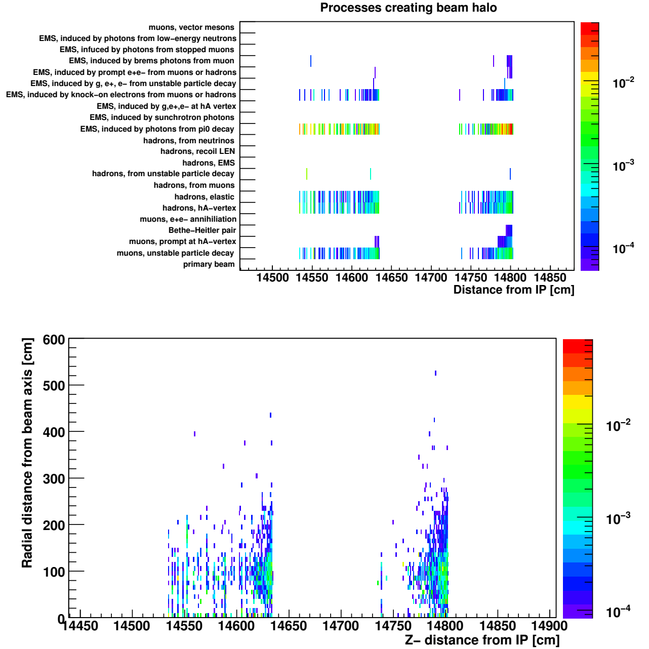
Figure 4.8: The origin processes of hadrons, muons and electromagnetic showers (EMS) resulting to the creation of beam halo (top). The radial distance from the beam pipe on the entrance into the experimental area as a function of the origin location along the LHC tunnel.
