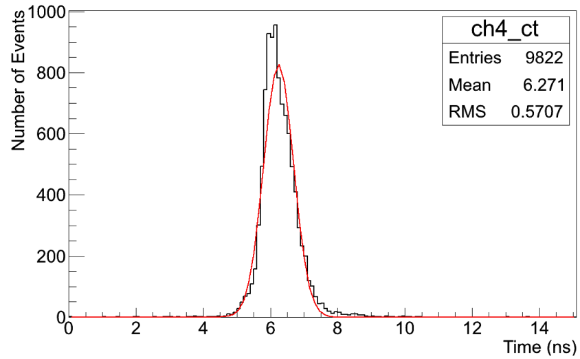
Figure 5.23: The difference of the arrival times of signals from the BHM prototype and a fast trigger scintillator [Amb13].
