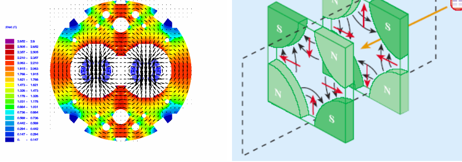
Figure 1.10: The magnetic fields produced by the dipoles and quadrupoles of the LHC. (images courtesy: CERN, [VM])
