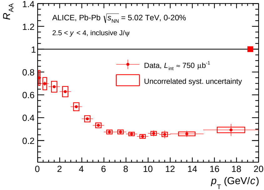
Figure 5.32: J/\psi R_{AA} as a function of p_T for 2.5 < y < 4 in the 0–20% centrality class. The statistical uncertainty is displayed with vertical error bars and the uncorrelated systematic uncertainty is represented by an open box around a point. The global uncertainty is 2% [This thesis].
