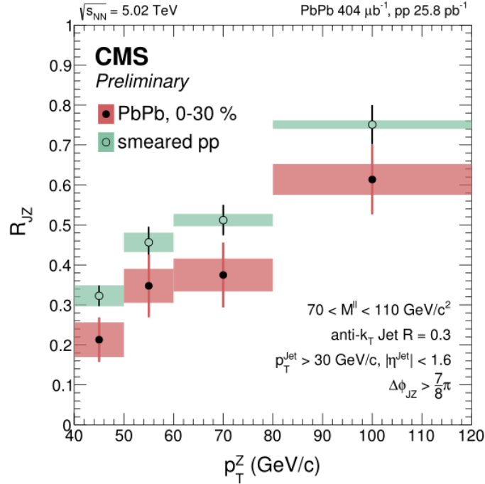
Figure 1.9: The R_{JZ} average number of jet partners per Z boson, measured in Pb-Pb and pp collisions at \sqrt{s_{NN}} = 5.02 TeV by the CMS experiment. Figure from [73].
