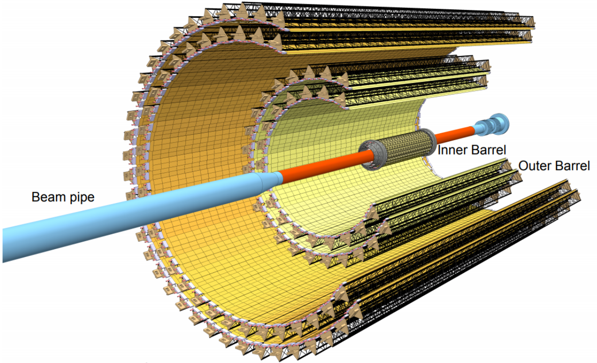
Figure 3.7: Layout of the ITS detector. Figure from [197].
