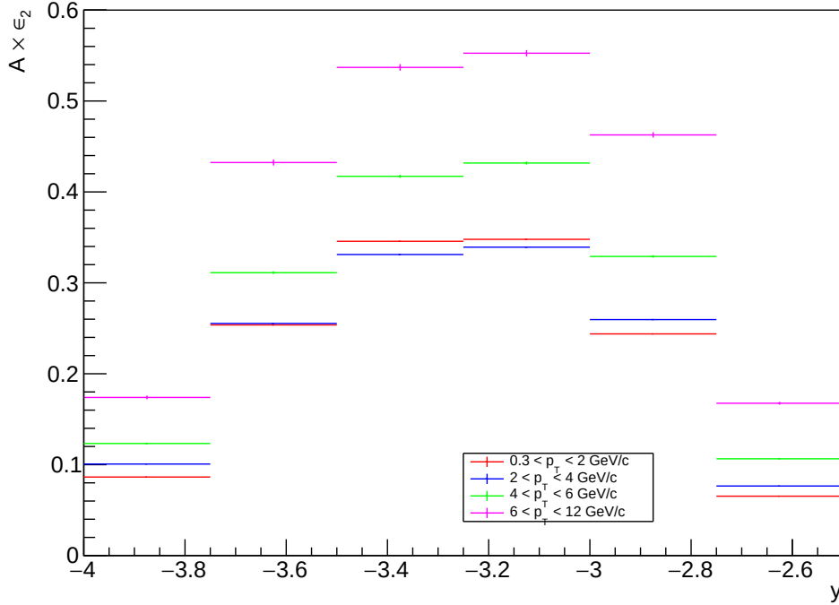
Figure 4.8: J/\psi A \times \epsilon as a function of rapidity in four p_T intervals in 2017 pp collisions at \sqrt{s} = 5.02 TeV.
