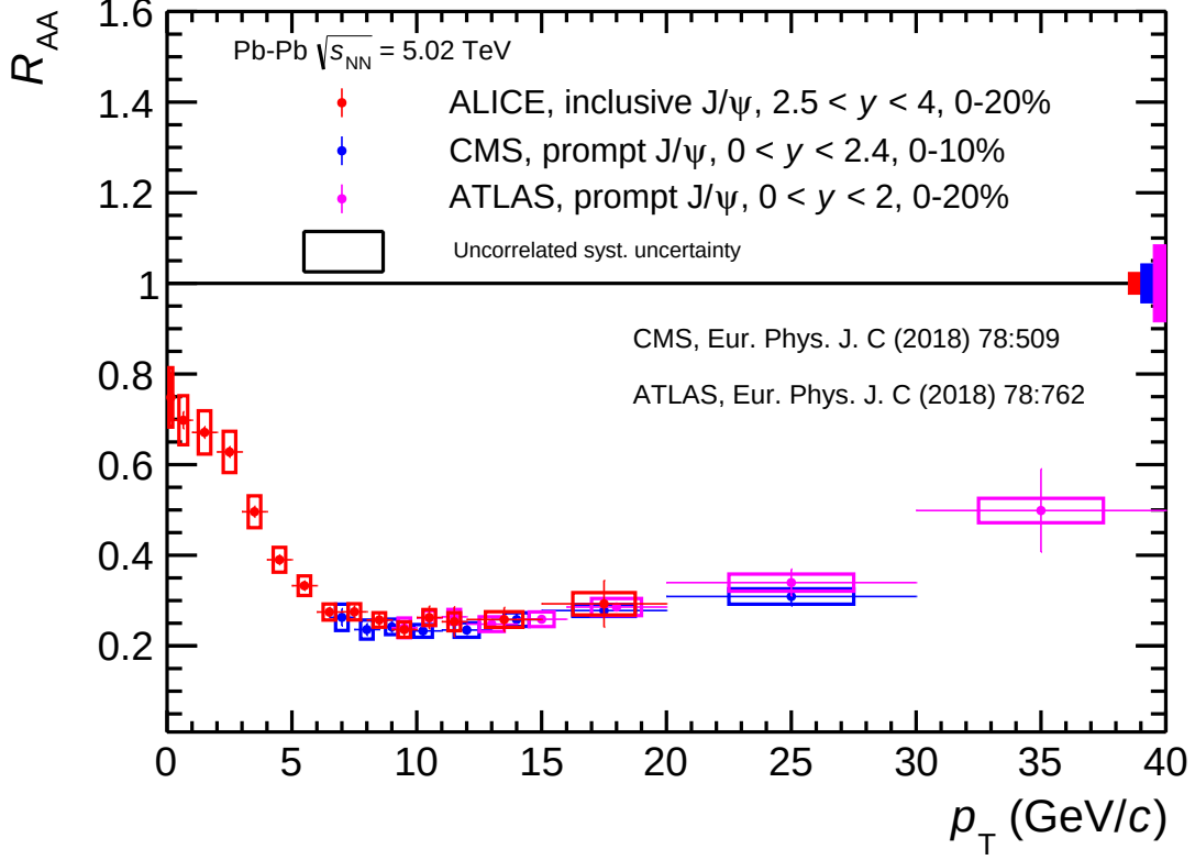
Figure 5.38: J/\psi R_{AA} as a function of p_T for 2.5 < y < 4 in the 0–20% centrality class, compared to the published results from CMS [7] and ATLAS [8]. The statistical uncertainty is displayed with vertical error bars and the uncorrelated systematic uncertainty is represented by an open box around a point [This thesis].
