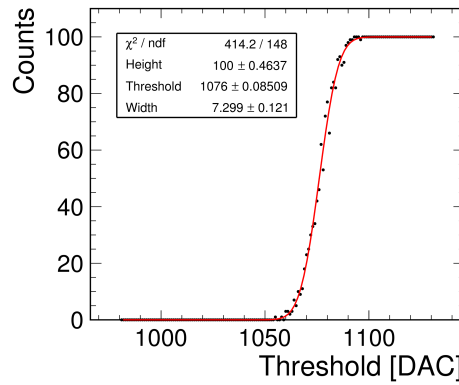
Figure 6.18: An example of a fitted S-curve for one of the pixels of assembly 31 for an injected pulse voltage of 0.03 V.
