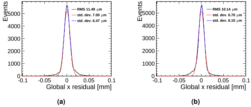
Figure 7.23: Residuals in the x-direction before the eta correction at (a) 0° and (b) 80°. The red line represents a Gaussian fit between \pm 0.1 mm, while the blue line is for a Gaussian fit between \pm 10 \mu\text{m} .
