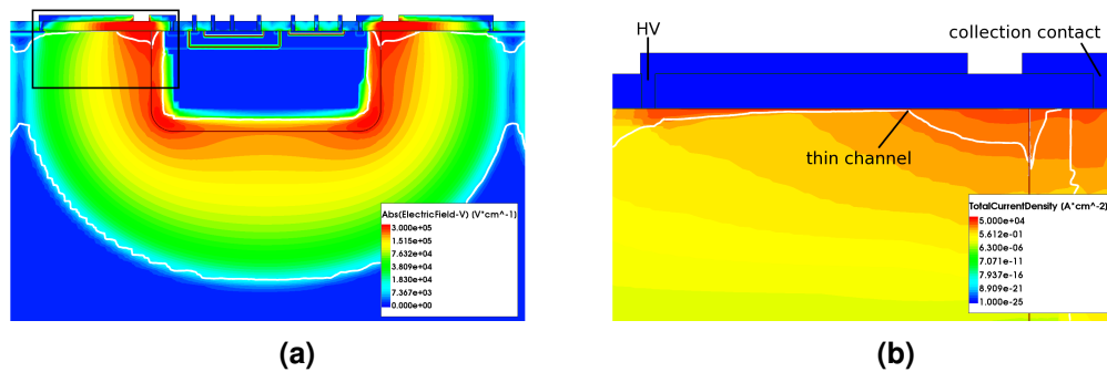
Figure 5.20: Two field maps at the breakdown voltage of -88 V showing (a) the absolute value of the electric field and (b) the total current density in the region near the high-voltage contact and the edge of the deep n-well, represented by the rectangle on (a).
