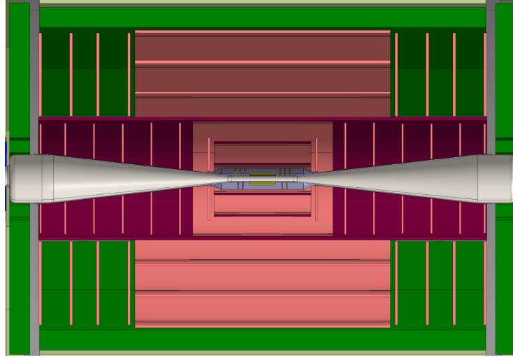
Figure 3.5: The layout of the CLICdet tracker [28].
