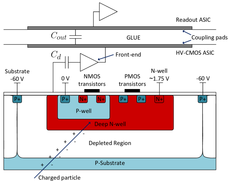
Figure 4.4: A schematic of the cross-section for a capacitively coupled pixel detector with a high-voltage CMOS sensor showing the deep n-well implant in the p-type substrate which hosts the electronics of the sensor [61].
