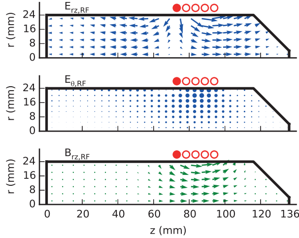
Figure 2.3 – Distribution of the vacuum electromagnetic fields E_{RF} , B_{RF} in the r, z plane. top: E_{rz,RF} , middle: E_{\theta,RF} , bottom: B_{rz,RF} . The RF coil position is indicated, in which the filled dot represents the high voltage connection while the opposite end is grounded. For reference the fields for a coil current I_{RF} = 130 \text{ A} results in maximum values of: E_{r,RF} = 45.8 \text{ kV/m} , E_{\theta,RF} = 2.1 \text{ kV/m} , E_{z,RF} = 62.5 \text{ kV/m} , B_{r,RF} = 9.1 \text{ mT} , B_{\theta,RF} = 0 , B_{z,RF} = 16.9 \text{ mT} .
