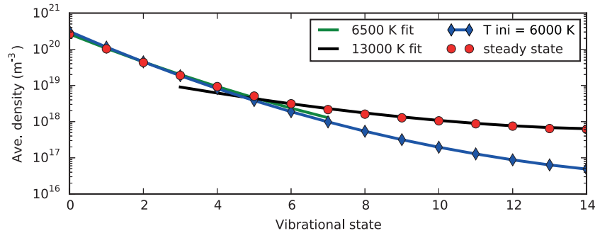
Figure 3.12 – Initial and final H_2(v) population. The initial vibrational temperature is chosen from experimental results. At steady state, the vibrational population is characterized by a two temperature distribution, T_{low} = 6500 K, and T_{high} = 13000 K where T_{low} is representative of the vibrational states v \leq 4 and T_{high} of v \geq 5 .
