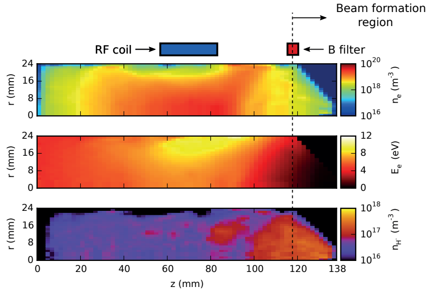
Figure 4.8 – From top to bottom: electron density n_e , electron energy E_e and volume produced H^- density n_{H^-} for the simulation with a magnetic filter field of 18 mT on the center of the plasma chamber, at I_{RF} = 100 A and p_{H_2} = 3 Pa without cusp field. The position of the RF coil and magnetic filter field is indicated. The beam formation region is defined as the region for z > 118 mm. A lower n_e and E_e is observed in the beam formation region, accompanied by an increase of n_{H^-} .
