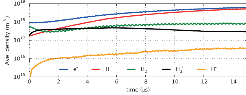
Figure 3.10 – Time evolution of the average charged particles' densities. After 15 \mu s of simulation the ion population is composed of 82% H^+ , 12% H_2^+ , 6% H_3^+ , while negative ions represent \approx 1\% of the negative charges.
