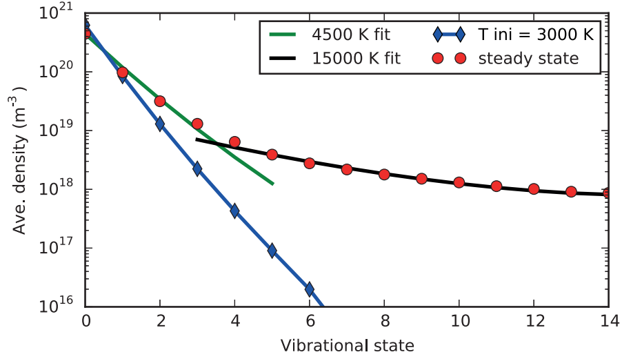
Figure 4.3 – Initial and steady state vibrational temperatures for the simulation without external magnets at p_{\text{H}_2} = 3 \text{ pa} and I_{\text{RF}} = 100 \text{ A} . A two-temperature distribution is observed at steady state.
