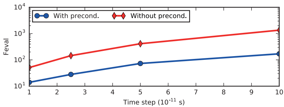
Figure 3.8 – Average number of function evaluations (Feval) required to reach convergence at each time step within JFNK. All simulations are performed with \Delta r \times \Delta z = 1 \times 1 mm and \theta = 0.6 .
