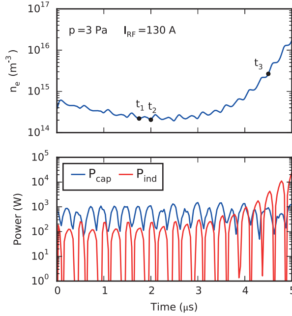
Figure 2.5 – Average electron density (top) and Joule heating power (bottom) as a function of time. t_x correspond to the phase of maximum E_{RF} . Particularly t_1 = 1.75 \mu s and t_2 = 2.00 \mu s correspond to the maximum E-field in opposite direction during the capacitively coupled regime, while t_3 is representative of the inductive coupled regime.
