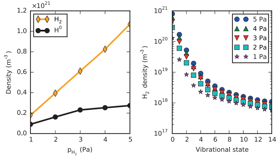
Figure 4.16 – Left) Volume averaged density of H^0 and H_2 (summed over v ) as a function of the hydrogen pressure p_{H_2} . Right) Density of vibrationally excited H_2(v) as a function of the hydrogen pressure p_{H_2} .
