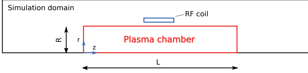
Figure 3.1 – Typical simulation domain: the plasma chamber is a cylinder of radius R and length L , while the calculation of the electromagnetic fields is performed on a larger domain. The RF coil is modelled as a perfect conductor with rectangular cross-section and given input current.
