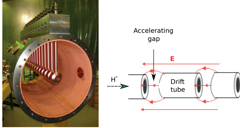
Figure 1.6 – Left) picture of one of Linac4 DTL modules. Right) working principle of a DTL, the particle acceleration takes place within the gaps with a force \vec{F} = q\vec{E} ( q = -1 for H^- ). The electric field is shielded in the metallic drift tubes.
