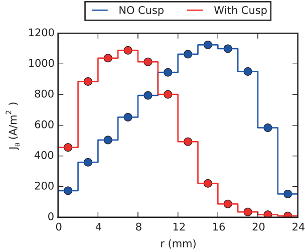
Figure 2.11 – Average plasma current j_{\theta} in the coil region during the first half cycle satisfying equation 2.5. Simulation conditions are p_{H_2} = 3 \text{ Pa} at the E-H transition current I_{EH} = 130 \text{ A} for NO cusp and I_{EH} = 200 \text{ A} with cusp.
