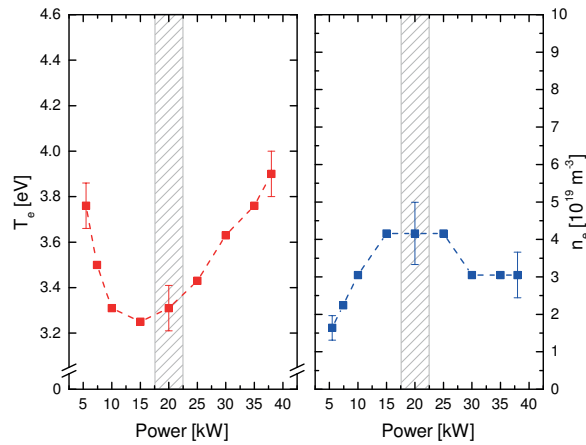
Figure 3.20 – Electron temperature T_e and electron density n_e evaluated from the OES measurements for varying RF power without applying a magnetic cusp field. The grey hatched area shows the region where the optimum source performance is typically achieved.
