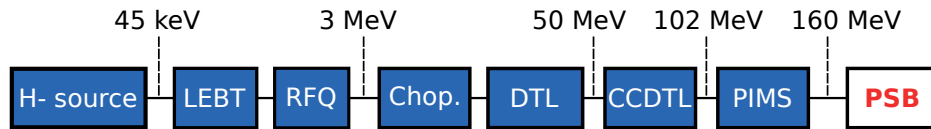
Figure 1.4 – Block diagram of the Linac4 layout with the energy delivered by each accelerating structure. From the H^- source, Linac4 is composed of a Low Energy Beam Transport (LEBT), a Radio-Frequency Quadrupole (RFQ), a chopper and buncher (Chop.), Drift Tube Linac (DTL), Cell Coupled Drift Tube Linac (CCDTL), Pi-mode structures (PIMS) before entering the Proton Synchrotron Booster (PSB).
