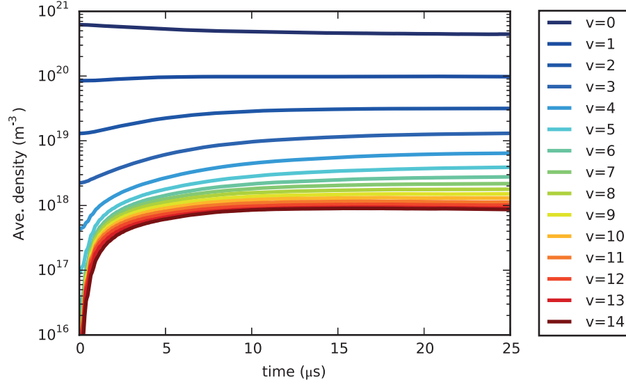
Figure 4.2 – Time evolution of the \text{H}_2(v) vibrational population for the simulation without external magnets at p_{\text{H}_2} = 3 \text{ Pa} and I_{\text{RF}} = 100 \text{ A} .
