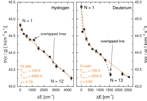
Figure 3.18 – Rotational distribution within the d^3\Pi_u, v' = 0 state evaluated from the Fulcher emission recorded for an RF power of 40 kW in deuterium and hydrogen. The corresponding two-temperature fits are also plotted.
