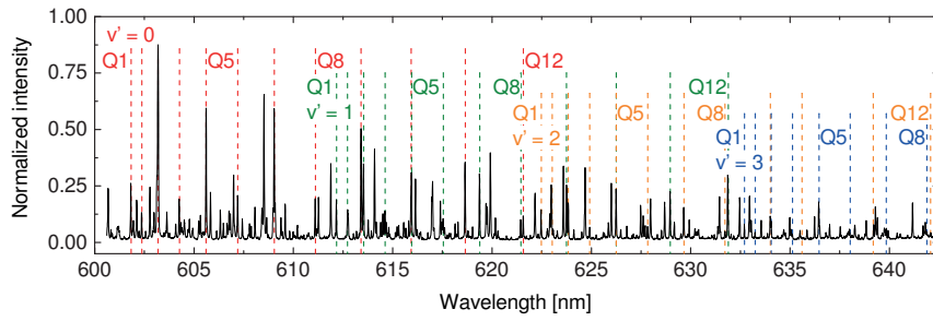
Figure 3.17 – Example spectrum of the molecular Fulcher radiation. The drop lines indicate the position of the Q lines for the first four diagonal vibrational transitions.
