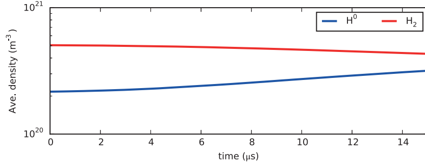
Figure 3.11 – Time evolution of the average neutral densities. The atomic population H^0 increases by a factor 1.5 during the simulation, while the molecular one decreases. We observe that steady state is not reached during the simulation time.
