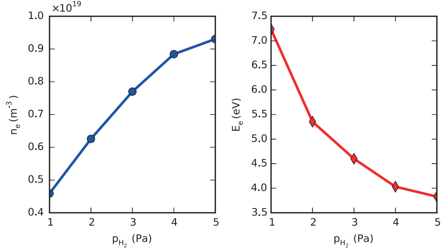
Figure 4.15 – Volume averaged electron density n_e (left) and energy E_e (right) as a function of the hydrogen pressure p_{H_2} .
