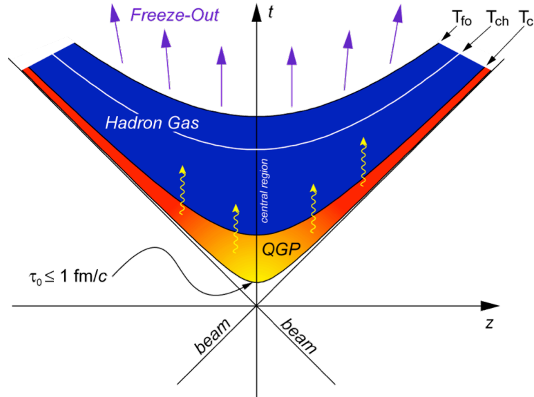
Figure 1.9: Theoretical view of a heavy-ion collision [49].
