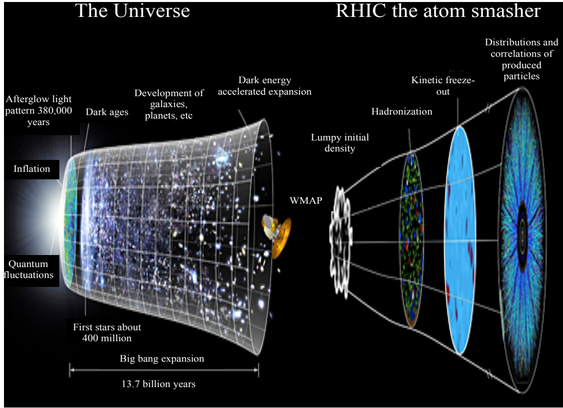
Figure 1.7: Time evolution of the big bang (left) and comparison with a heavy-ion collision (right) [43].
