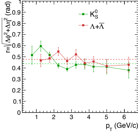
Figure 7.11: Estimation of the near-side jet cone radius for K_S^0 and \Lambda + \bar{\Lambda} .
