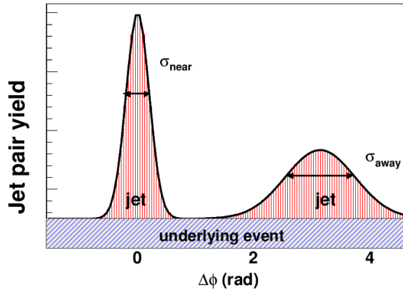
Figure 5.8: Different regions of the correlation function. Narrow near-side and broad away-side with an underlying region are shown (Illustration purposes only).
