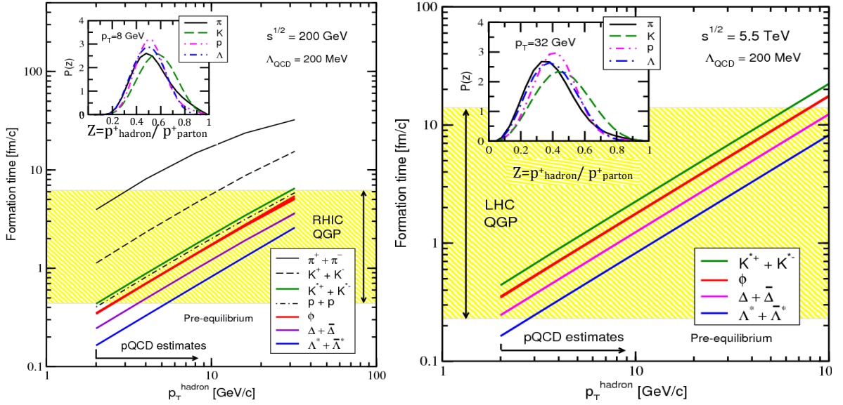
Figure 1.14: RHIC (left) and LHC (right) QGP formation time in different energy regimes [68].
