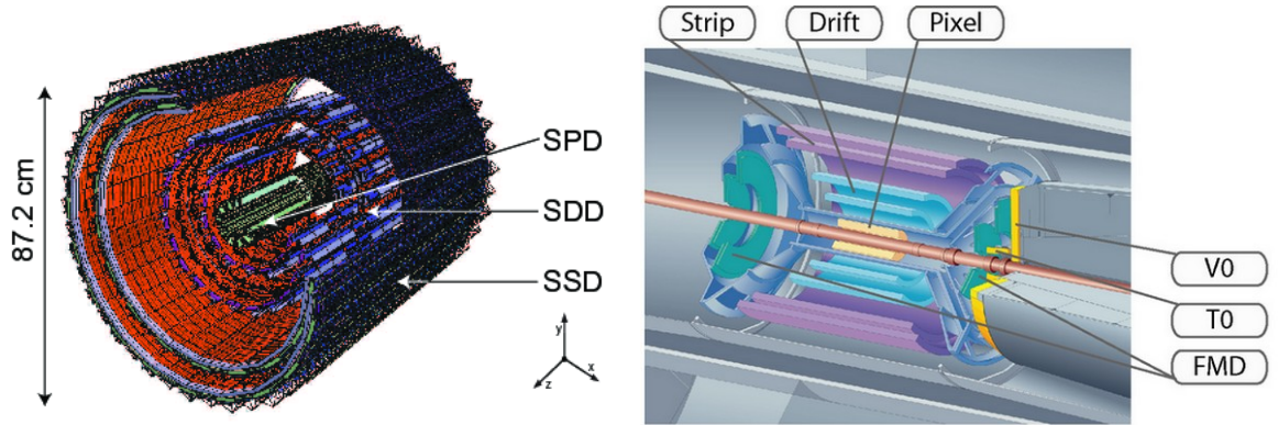
Figure 2.9: Schematic diagram of the ITS (left) and placement of ITS in central tracking region [121].
