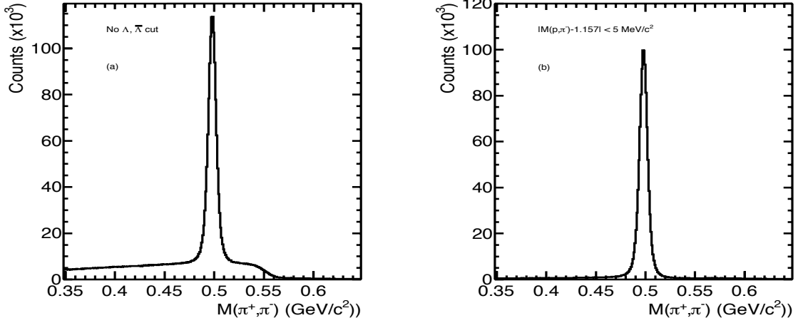
Figure 4.7: Before (a) and after (b) applying a \Lambda invariant mass cut on K_S^0 . The combinatorial background becomes liner, which will be useful in calculating the net signal and background.
