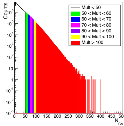
Figure 7.22: Multiplicity intervals after minimum bias trigger and 10cm primary vertex cut.
