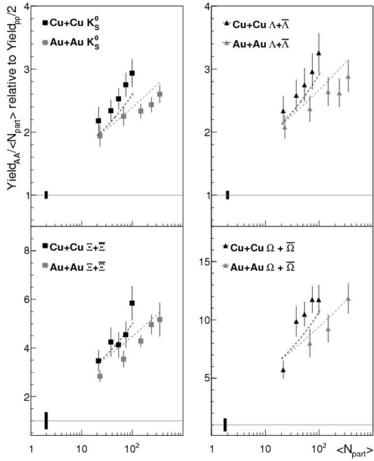
Figure 1.10: The enhancement factor for (multi-) strange particles in Cu+Cu and Au+Au \sqrt{s_{NN}}=200 GeV collisions [54].
