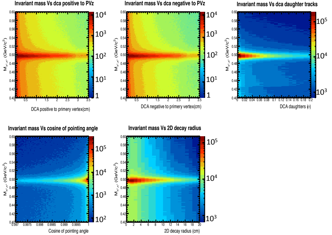
Figure 6.1: Distribution of topological cuts vs invariant mass for K_S^0 .
