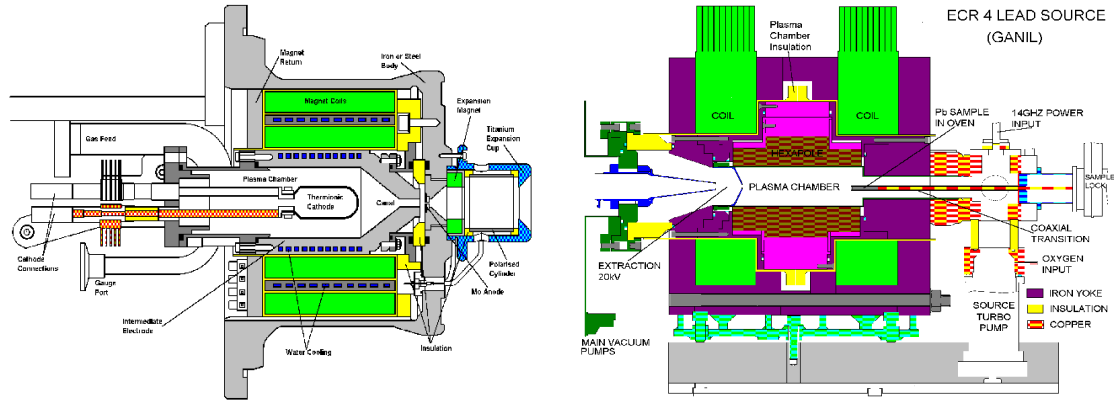
Figure 2.2: Duoplasmatron ion source (left) that provides H^+ ions and the ECR ion source (right) that provides heavy ions( ^{208}_{53}Pb^+ ) [92].
