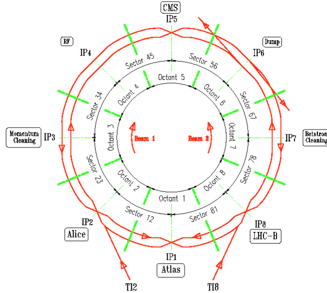
Figure 2.4: Layout of LHC and different activities in eight sectors [101].
