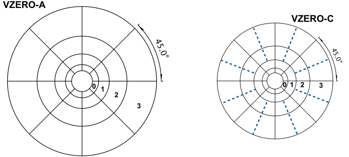
Figure 2.12: Sketches of VZERO-A and VZERO-C arrays showing their segmentation. Scintillator thicknesses are 2.5 and 2 cm, respectively [126].
