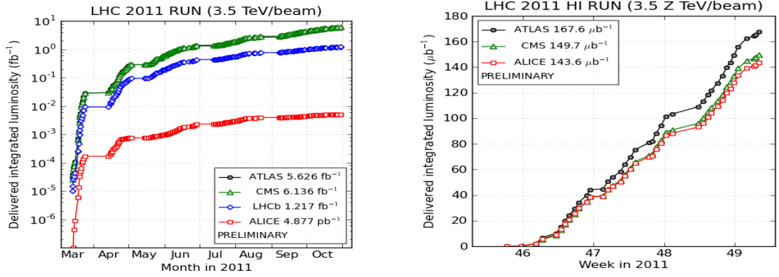
Figure 2.6: Luminosity delivered to each experiment in 2011, left panel shows pp luminosity and right panel shows heavy-ion luminosity. ALICE luminosity is less than that at ATLAS and CMS due to restrictions in readout electronics of the detector. The reduction in luminosity is achieved by defocusing the beam prior to the intersection point [105].
