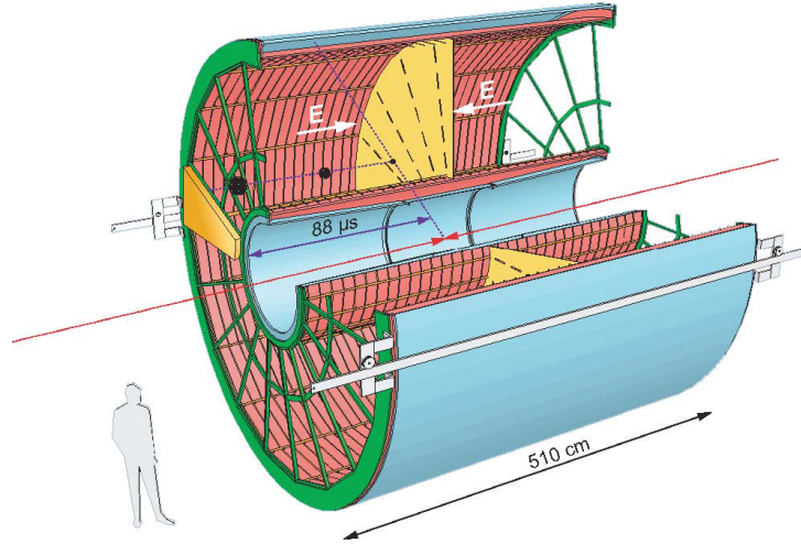
Figure 2.10: The ALICE Time Projection Chamber (TPC) [122].
