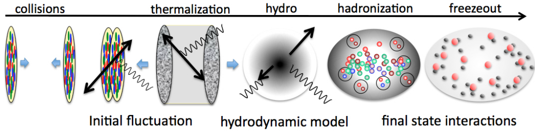
Figure 1.8: Schematic sketch of a relativistic heavy-ion collision. Particles (arrows) and photons (wavy lines) are emitted in several stages of the evolution [48].
