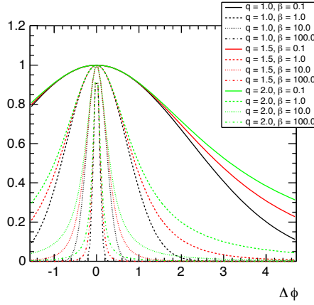
Figure 7.12: Q-Gaussian distributions for four different \beta values in q=1, 1.5, 2 (Illustration purposes only).
