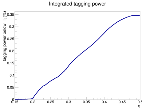
Figure 6.3: The y -axis shows the tagging power (evaluated on MC) as a function of the upper bound on the estimated mistag ( \eta ); the requirement that \eta < 45\% has been removed for illustrative purposes.
