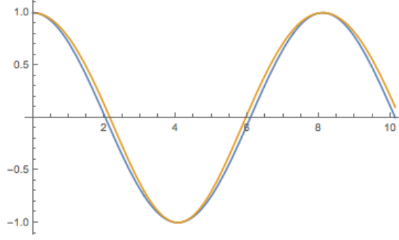
Figure G.2: A plot of the approximation Eq. (G.29) (blue) is compared to Eq. (G.41) (orange) for B^0 oscillation, when \mathcal{A}_0 = 20\% and the observed flavor is B^0 . When the observed flavor is \bar{B}^0 the sign of the correction flips.
