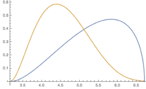
Figure E.6: The q^2 spectra of B_c^+ \rightarrow \psi(2S)\mu^+\nu_\mu are completely distinct in the EFG model (orange) and Kiselev model (blue).
