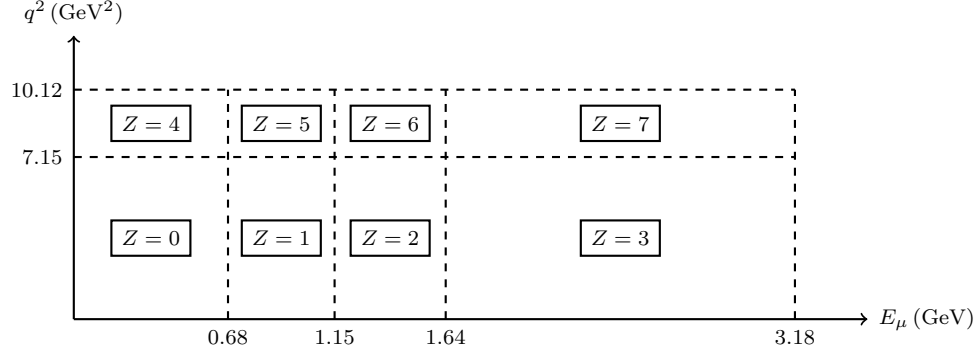
Figure 4.1: Definition of the categorical variable Z in the q^2, E_\mu plane.
