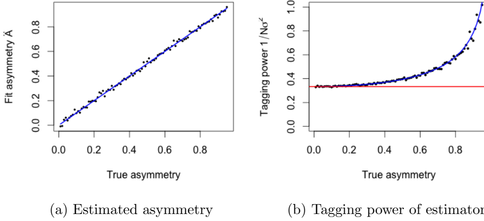
Figure F.1: The asymmetry and estimated numerically from samples of 10k events and associated tagging power (black points) agree very well with the analytic estimates in the asymptotic limit (blue). For small asymmetries the tagging power tends to the canonical tagging power, 1/3 (red).
