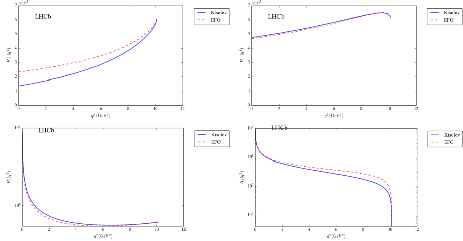
Figure A.2: In the helicity parameterization, closest to the differential decay rate, the Kiselev and EFG hadronic tensor helicity components are in broad agreement, with the biggest difference in H_+ .
