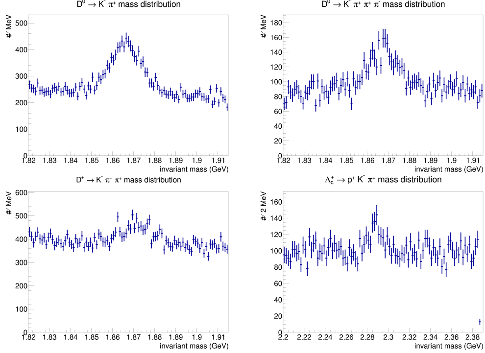
Figure 6.1: Charm hadron mass distributions in data.
