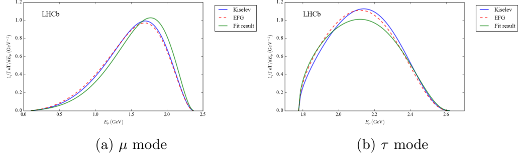
Figure 4.14: The Kiselev, EFG, and BCL E_\ell^* distribution for B_c^+ \rightarrow J/\psi \ell^+ \nu_\ell show that the data prefers a slightly harder E_\mu^* .
