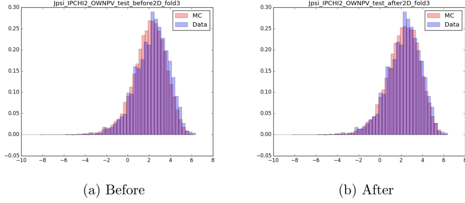
Figure D.4: The J/\psi impact parameter significance is shifted slightly higher to match the data.
