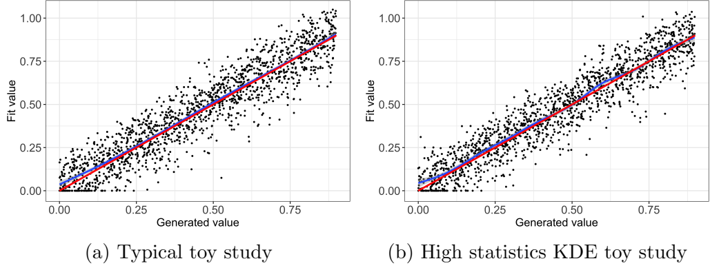
Figure 4.7: There is good agreement in the closure test comparing the high-statistics KDE toy study to the typical toy study. For ease of comparison, the blue curve shows the conditional mean fit value as a function of the generated value.
