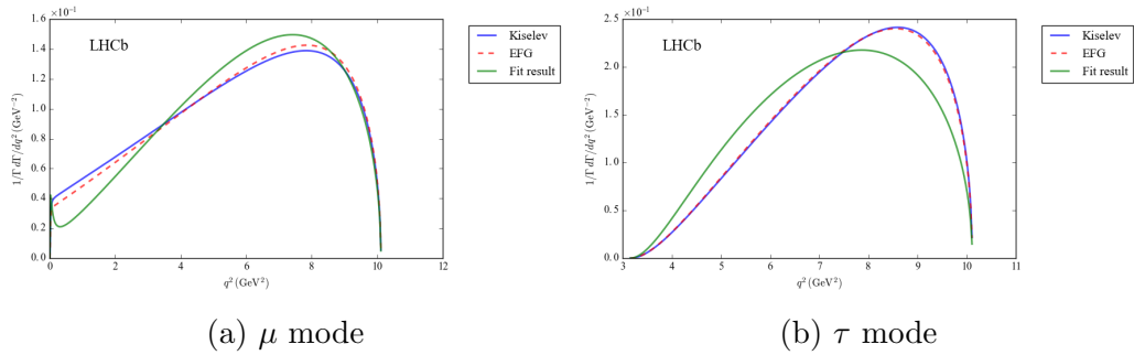
Figure 4.13: The Kiselev, EFG, and BCL q^2 distribution for B_c^+ \rightarrow J/\psi \ell^+ \nu_\ell show that the fit to the data prefers a slightly softer q^2 spectrum.
