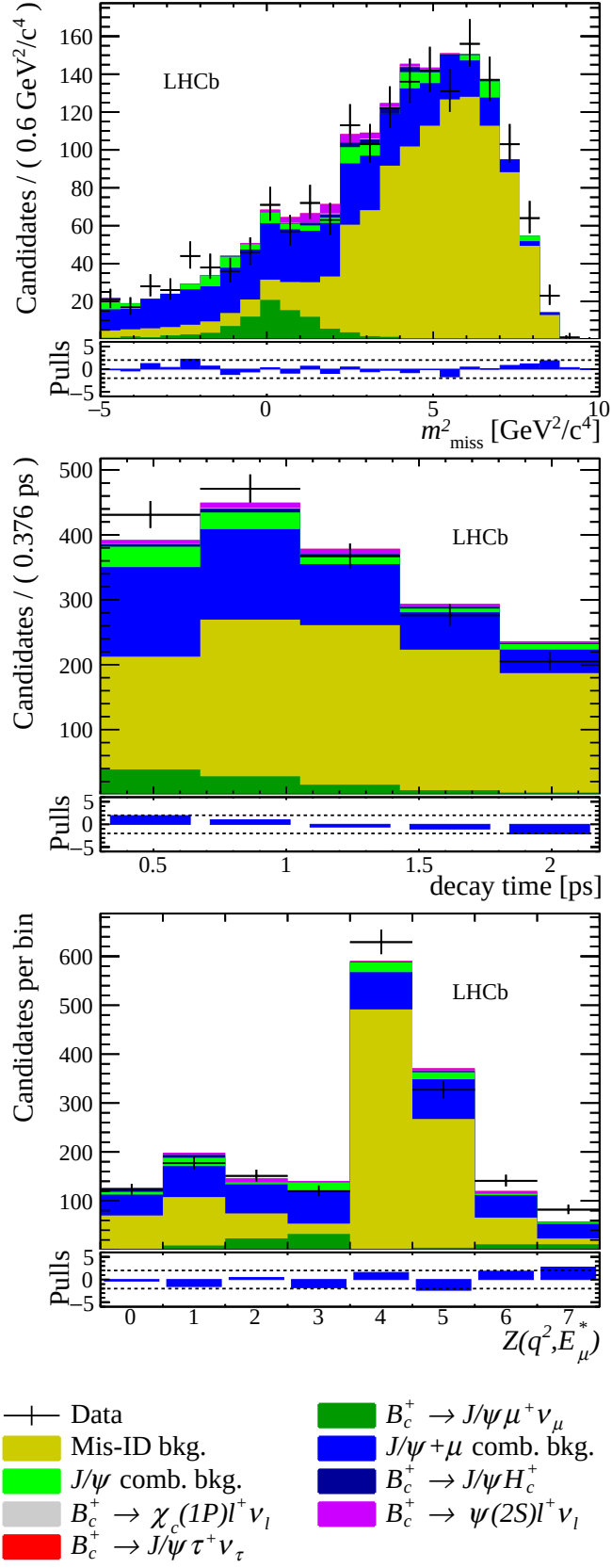
Figure 4.17: Projections of fit to the \psi(2S) enriched sample (including data and the non-signal component templates) onto m^2_{\text{miss}} (top), t (middle), and Z (bottom).
