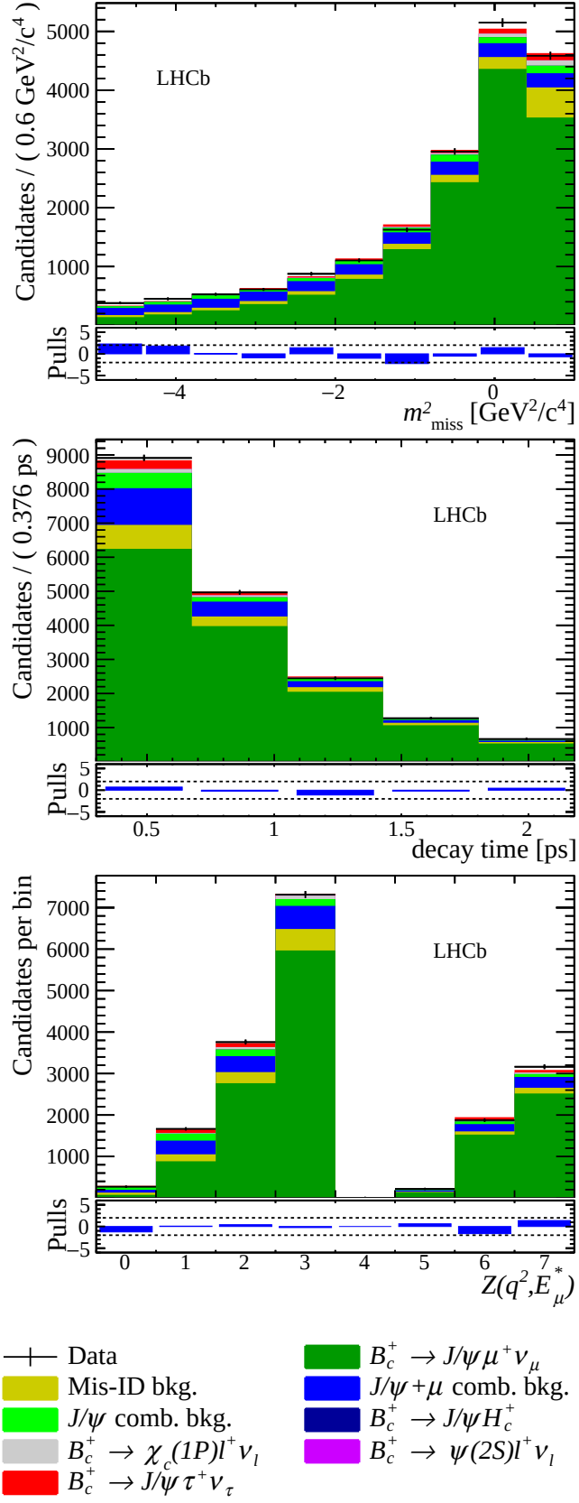
Figure 4.10: Projections of fit to normalization-rich region (including data and the non-signal component templates) onto m^2_{\text{miss}} (top), t (middle), and Z (bottom)
