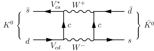
Figure 1.2: K^0 – \bar{K}^0 mixing receives contributions from internal loops with the three up-type quarks ( q = u, c, t ) and shows CP violation due to the phase differences between V_{qs}V_{qs}^* and V_{qs}^*V_{qs} .
