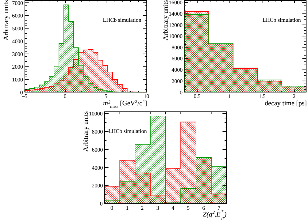
Figure 4.9: Fit templates for normalization B_c^+ \rightarrow J/\psi \mu^+ \nu_\mu ; the signal template is shown in red for comparison.
