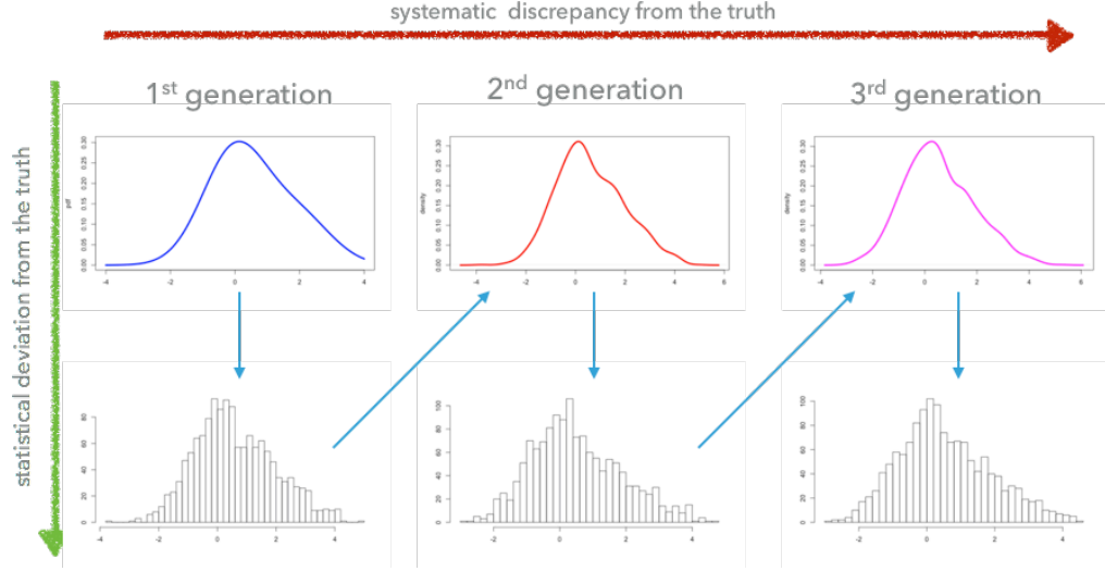
Figure 4.5: Nesting the kernel-smoothing procedure produces third generation distributions f_{i,3}(x) (top right) — indexed by the set of the second-generation histogram templates used to produce them.
