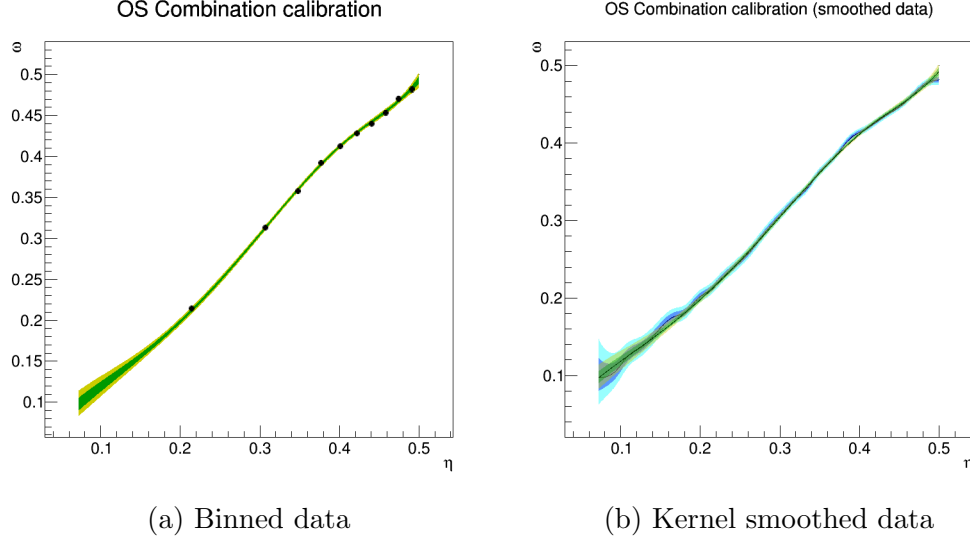
Figure G.5: B-spline calibration to B^\pm \rightarrow J/\psi K^\pm ; the green and yellow areas represent 1\sigma and 2\sigma bands for the calibration, while the blue and light blue areas in the right-hand plot represent 1\sigma and 2\sigma confidence intervals in the kernel-smoothed data.
