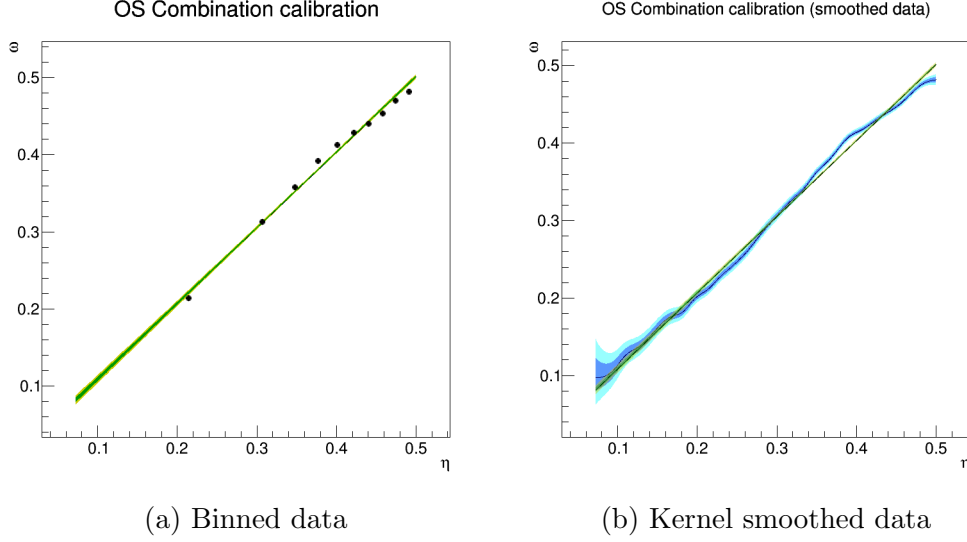
Figure G.3: Linear calibration to B^\pm \rightarrow J/\psi K^\pm ; the green and yellow areas represent 1\sigma and 2\sigma bands for the calibration, while the blue and light blue areas in the right-hand plot represent 1\sigma and 2\sigma confidence intervals in the kernel-smoothed data.
