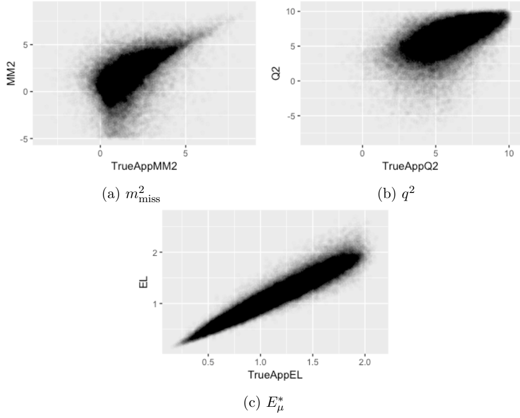
Figure E.7: The distributions of the reconstructed parameters vs. their true values in MC generated \psi(2S) events in the EFT model.
