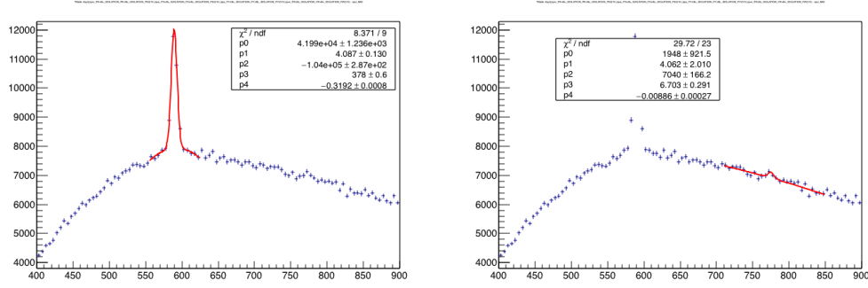
(a) Fit to the mass difference in the \psi(2S) mass window (b) Fit to the mass difference in the X(3872) mass window
