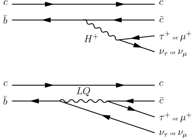
Figure 3.2: Semileptonic B_c^+ decays beyond the SM
