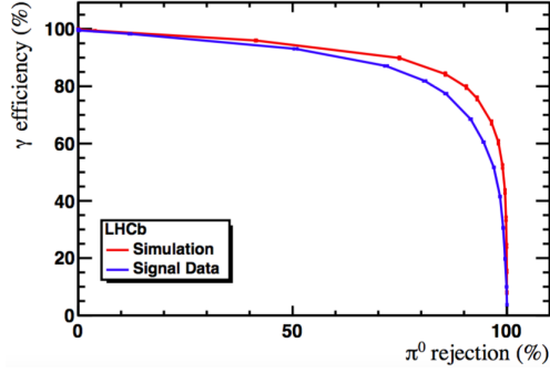
Figure 2.7: Discrimination of \gamma and merged \pi^0 showers in the ECAL
