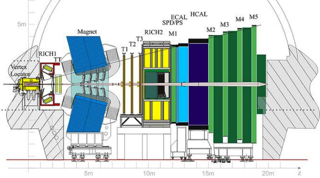
Figure 2.2: The LHCb detector [29]. In the center lies the dipole bending magnet (blue). Upstream (decreasing z ) lie the Vertex Locator (VELO) and TT tracking stations, and the RICH1 station. Downstream (increasing z ) lie the IT and OT trackers (in three layers labelled T1, T2, and T3), RICH2 station, ECAL, HCAL, and muon chamber.
