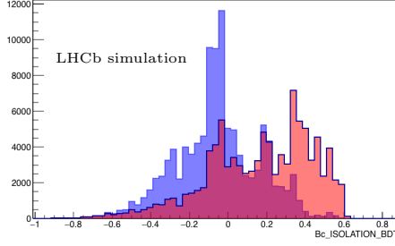
Figure 4.2: The distributions of the isolation BDT score for B_c^+ \rightarrow J/\psi \mu^+ \nu_\mu (blue) and for mis-identified background template, before applying the PID selection (red)
