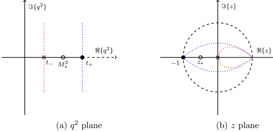
Figure 3.7: Analytic properties of semileptonic form factors in the q^2 and z planes. The branch cuts are represented by dashed lines and the threshold points by solid circles. The pole is represented by an open circle, and the reference point q^2 = t_- by a cross.
