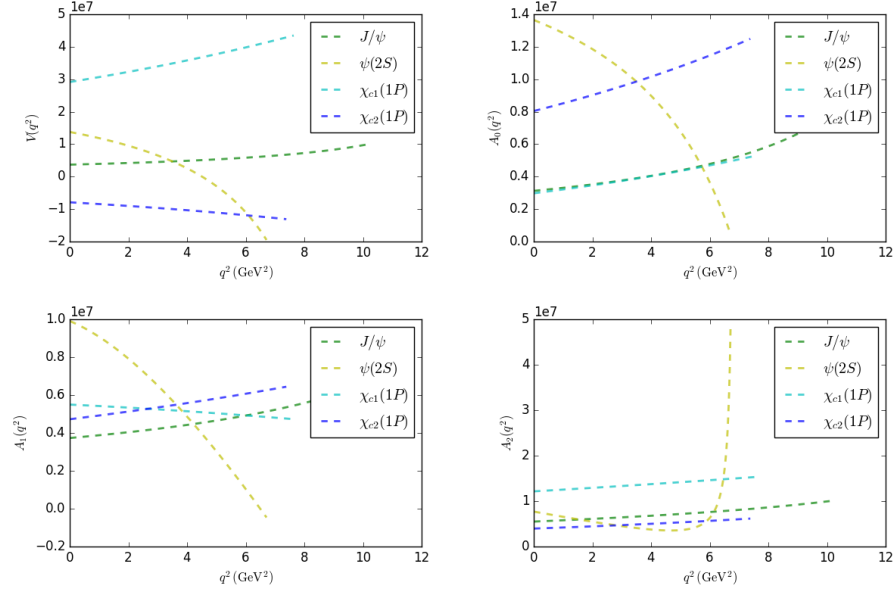
Figure A.5: Form factors for J/\psi and \psi(2S) (from EFG) and \chi_{c1} and \chi_{c2} (from WWL).
