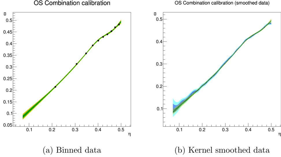
Figure G.6: N-spline calibration to B^\pm \rightarrow J/\psi K^\pm ; the green and yellow areas represent 1 \sigma and 2 \sigma bands for the calibration, while the blue and light blue areas in the right-hand plot represent 1 \sigma and 2 \sigma confidence intervals in the kernel-smoothed data.
