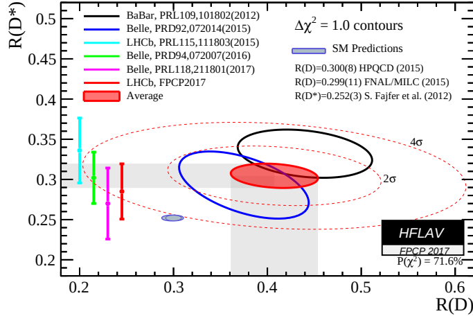
Figure 1.3: Measurements of semitauonic B \rightarrow D^{(*)}\tau\nu branching fractions, reproduced from Ref. [13].
