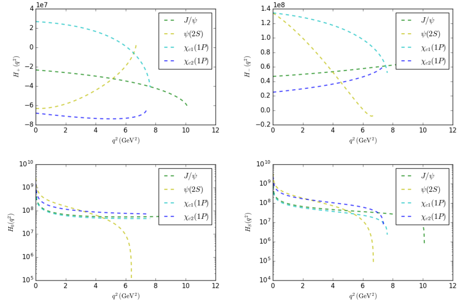
Figure A.6: Helicity form factors for J/\psi and \psi(2S) (from EFG) and \chi_{c1} and \chi_{c2} (from WWL).
