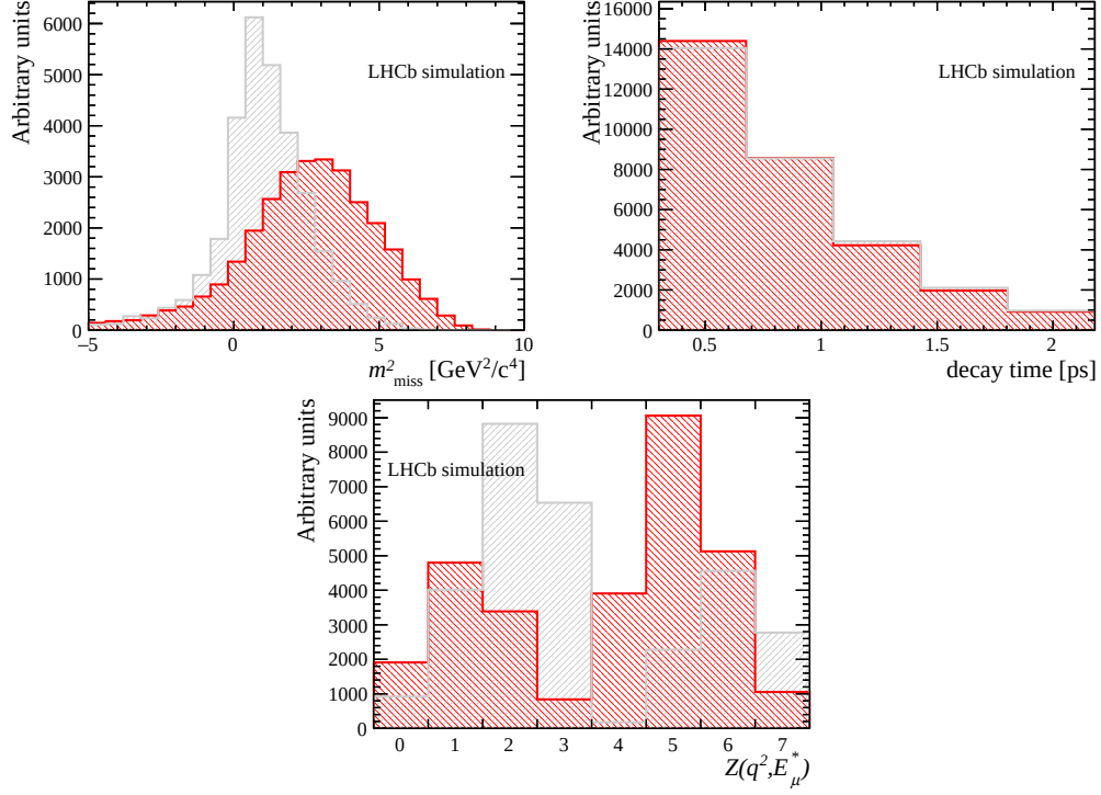
Figure 4.16: Fit templates for muonic feed-down B_c^+ \rightarrow \chi_{c1}\mu^+\nu_\mu and B_c^+ \rightarrow \chi_{c2}\mu^+\nu_\mu ; the signal template is shown in red for comparison.
