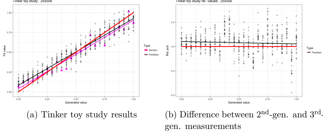
Figure 4.8: The tinker toy test compares a second-generation KDE toy study (purple) to a third-generation study (black). The fits in the third-generation toys generally produce slightly higher estimates than their corresponding second-generation fits, leading to a systematic uncertainty.
