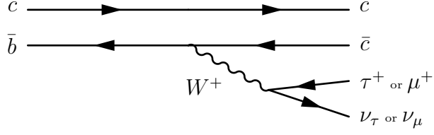
Figure 3.1: Semileptonic B_c^+ decays in the SM
