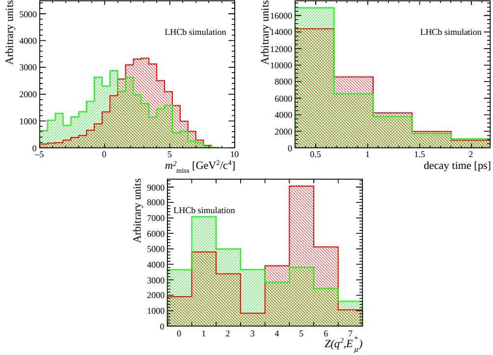
Figure 4.23: Fit templates for combinatorial background from (B^0, B^+, B_s^0) \rightarrow J/\psi X ; the signal template is shown in red for comparison.
