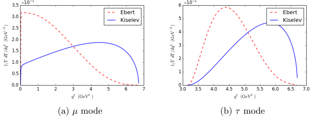
Figure 3.6: The Kiselev and EFG q^2 distribution for B_c^+ \rightarrow \psi(2S)\ell^+\nu_\ell disagree completely.
