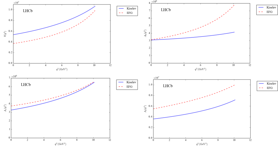
Figure A.1: The Kiselev and EFG form factors do not seem to agree well in the standard parameterization.
