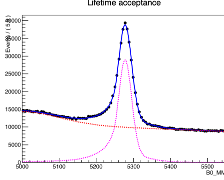
Figure 4.26: Fit to the invariant mass distribution of the B^0 \rightarrow J/\psi K^* sample selected from data.
