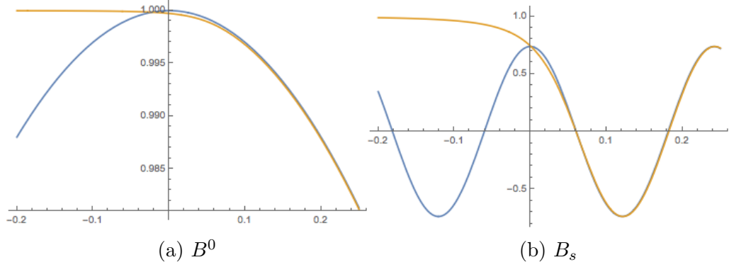
Figure G.1: A plot of the approximation of D_{\text{res}} \cos \Delta m t from Eq. (G.29) (blue) is compared to the analytic result E[\cos(\Delta m t) | t_{\text{obs}}] from Eq. (G.36) (orange) for B^0 mesons (left) and B_s mesons (right). For each plot, the scale of the time axis is chosen such that \Gamma = 1 and \sigma = 0.03 (corresponding to 50 fs decay time resolution), while \Delta m/\Gamma = 0.775 for B^0 and 26 for B_s .
