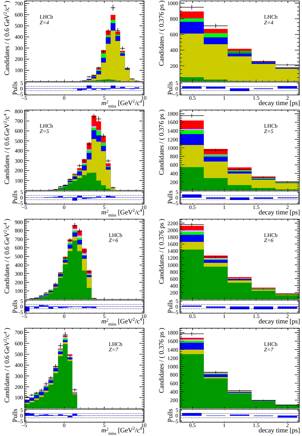
Figure 4.31: Projections of the nominal fit in bins 4–7 of Z , i.e. , individual bins of q^2 and E_\mu^* .
