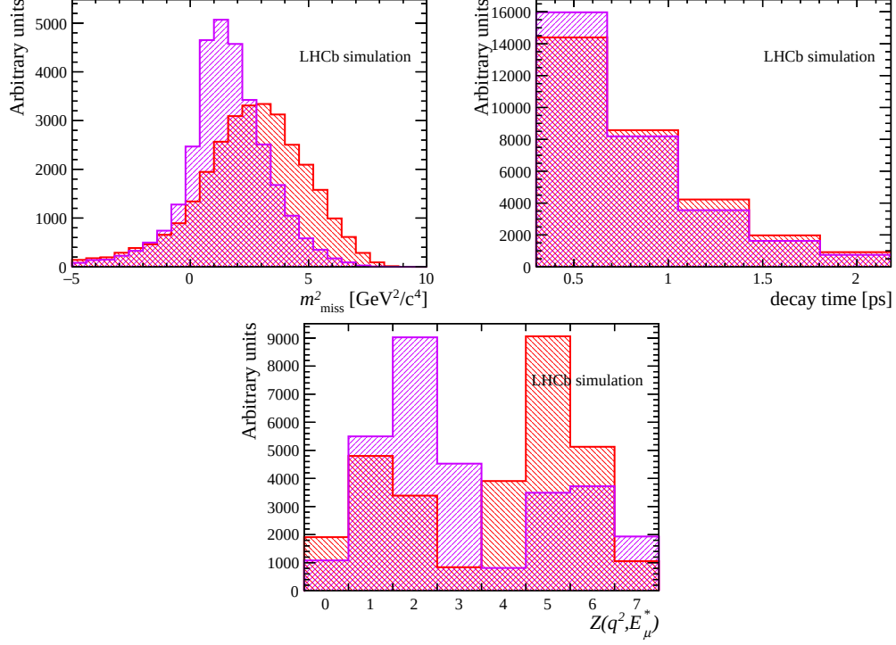
Figure 4.15: Fit templates for feed-down B_c^+ \rightarrow \psi(2S)\mu^+\nu_\mu and B_c^+ \rightarrow \psi(2S)\tau^+\nu_\tau ; the signal template is shown in red for comparison.
