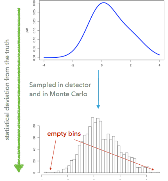
Figure 4.3: The true distributions f_{i,1}(x) (top) has support everywhere, but the high statistics histogram template (bottom) has sparse bins in the tail regions.
