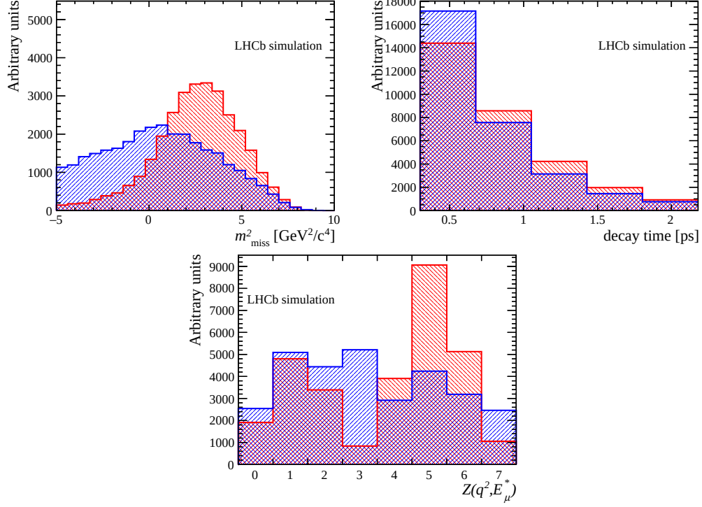
Figure 4.24: Fit templates for combinatorial J/\psi candidates; the signal template is shown in red for comparison.
