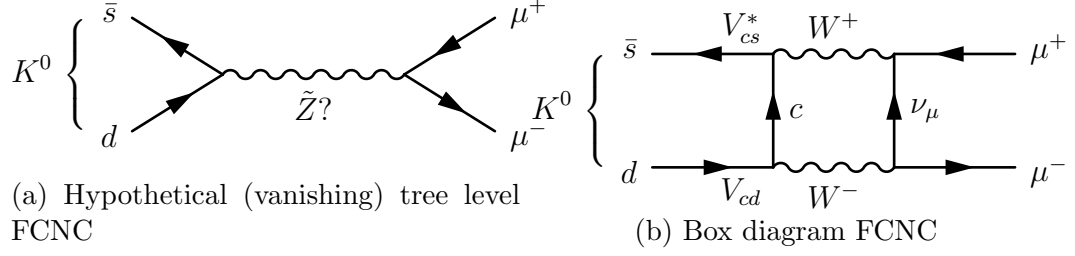
Figure 1.1: FCNCs in K^0 decay
