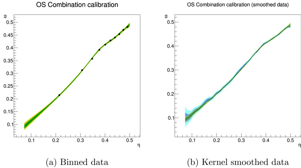
Figure G.7: Enhanced n-spline calibration to B^\pm \rightarrow J/\psi K^\pm ; the green and yellow areas represent 1 \sigma and 2 \sigma bands for the calibration, while the blue and light blue areas in the right-hand plot represent 1 \sigma and 2 \sigma confidence intervals in the kernel-smoothed data.
