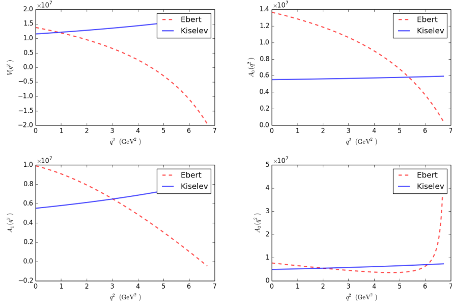
Figure A.3: None of the standard form factors of the Kiselev and EFG models of the B_c^+ \rightarrow \psi(2S) transition agree well.
