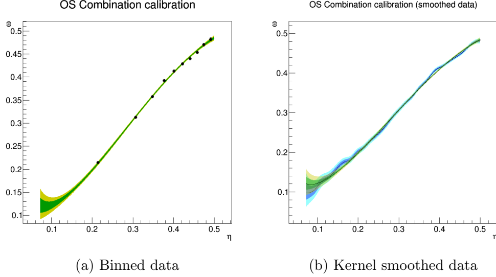
Figure G.4: Cubic calibration to B^\pm \rightarrow J/\psi K^\pm ; the green and yellow areas represent 1\sigma and 2\sigma bands for the calibration, while the blue and light blue areas in the right-hand plot represent 1\sigma and 2\sigma confidence intervals in the kernel-smoothed data.
