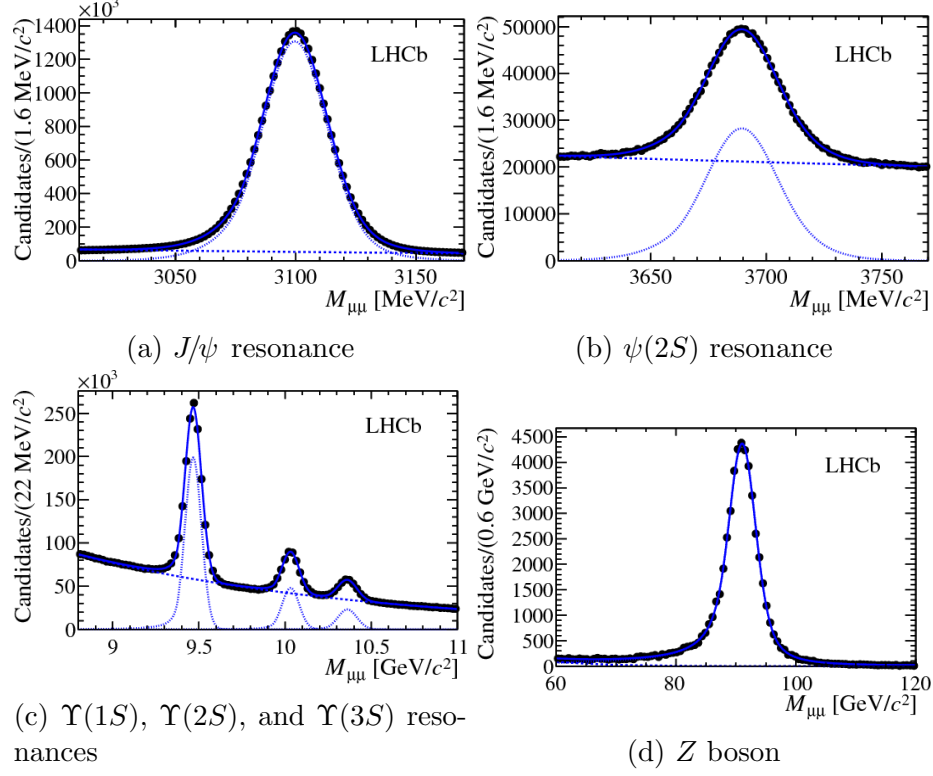
Figure 2.4: Fits to the invariant mass distributions of the J/\psi , \psi(2S) , \Upsilon(nS) , and Z dimuon resonances [42].
