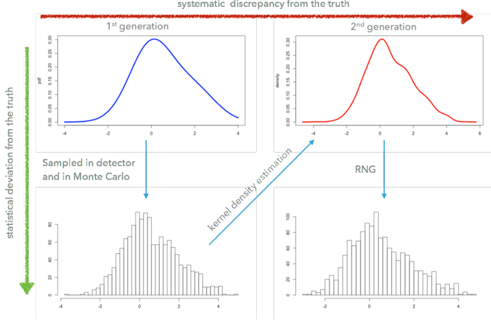
Figure 4.4: Applying a kernel smoothing procedure to sampled simulation data produces second-generation distributions f_{i,2}(x) (top right), which can quickly sampled via RNG (bottom right).
