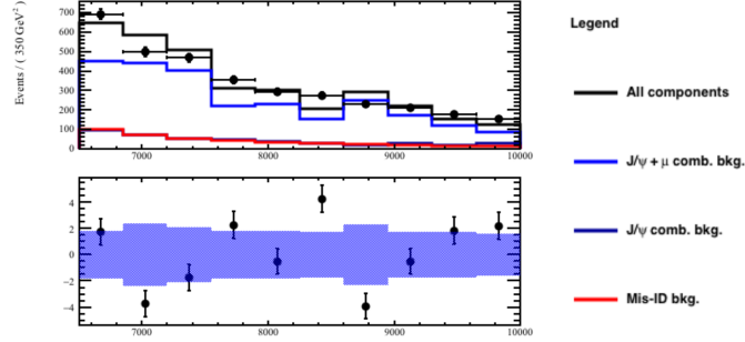
Figure 4.32: Fit to combinatorial-rich high mass sideband region
