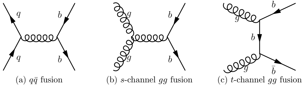
Figure 2.3: Tree-level b\bar{b} pair production in pp collisions
