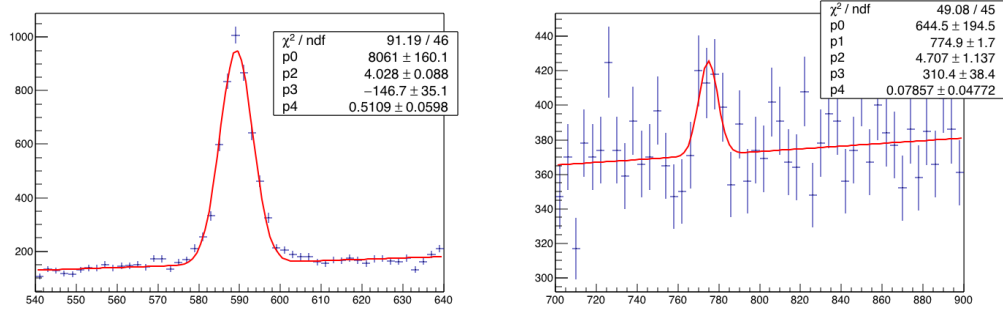
(a) Fit to the mass difference in the \psi(2S) mass window (b) Fit to the mass difference in the X(3872) mass window
