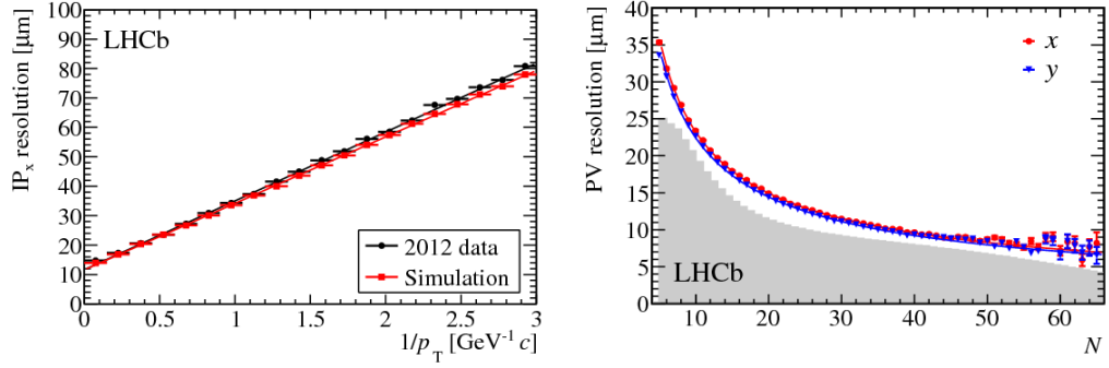
(a) IP resolution dependence on transverse momentum. (b) PV resolution dependence on the number of tracks used in reconstruction.
