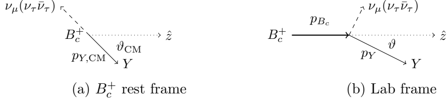
Figure 3.8: Semileptonic B_c^+ decay into a visible J/\psi \mu system and invisible neutrino system
