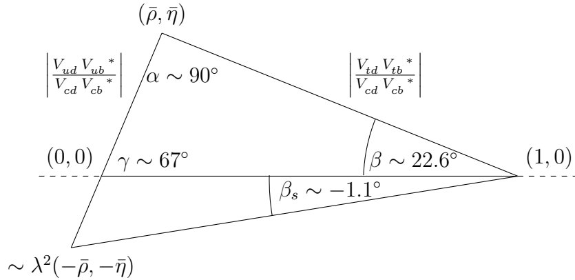
Figure 5.1: Standard unitarity triangles [87]
