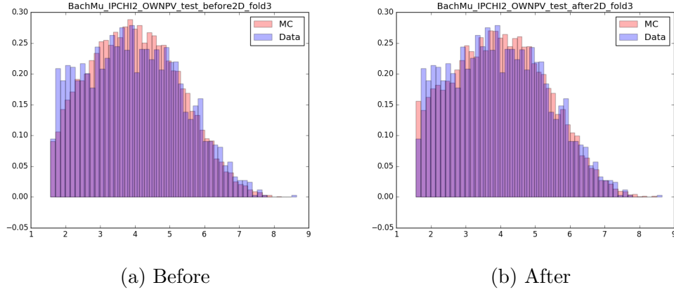
Figure D.5: The \mu^+ impact parameter significance distribution is weighted up slightly at small values.
