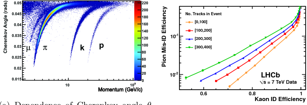
(a) Dependence of Cherenkov angle \theta_c on particle species and momentum, for (b) K^+\pi^+ classification curve, showing dependence on track multiplicity
