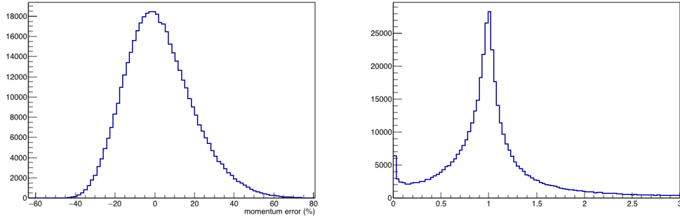
(a) Fractional error on the B_c^+ momentum (b) Ratio of squared kinematic error (from Eq. (3.37)) to the total squared error
