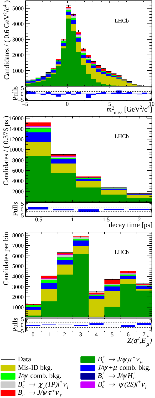
Figure 4.28: Projections of nominal fit onto m_{\text{miss}}^2 (top), t (middle), and Z (bottom).
