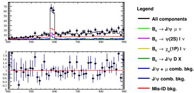
Figure 4.19: Comparison of the invariant mass in the \psi(2S) window in data and in the simulation model corresponding to the best fit point, for the \psi(2S) enriched control sample. The invariant mass of the J/\psi candidate is subtracted to sharpen the \psi(2S) \rightarrow J/\psi \pi^+ \pi^- peak.
