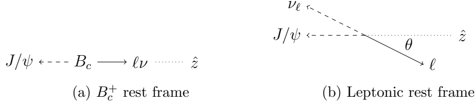
Figure 3.3: Diagram of the semileptonic decay of a B_c^+ into a hadronic part ( J/\psi ) and leptonic part ( \ell and \nu_\ell ). As shown, \theta is the angle between the lepton and the leptonic ( i.e. , lepton-neutrino) flight direction in the leptonic rest frame.
