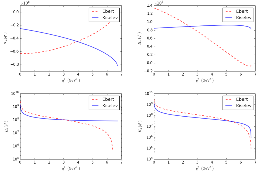
Figure A.4: The huge difference in the Kiselev and EFG models of the B_c^+ \rightarrow \psi(2S) transition is due to their H_+ and H_- hadronic tensor helicity components.
