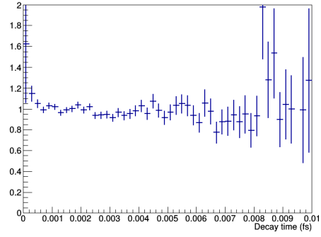
(b) p_\pi/p_{B_c} between 12.5% and 25%
