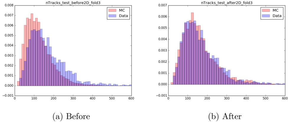
Figure D.3: The track multiplicity is corrected to match the higher activity distribution observed in data.
