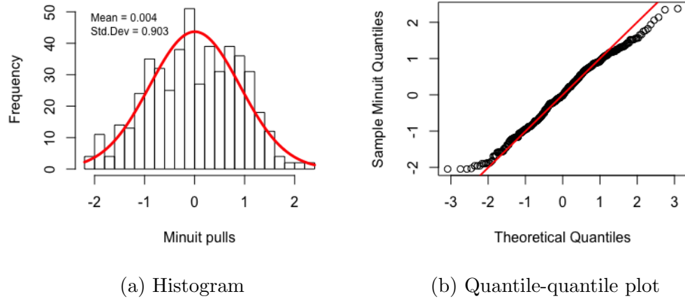
Figure 4.33: The Minuit pull distribution is unbiased and is close to normal between -2 and 1. It has thinner tails than a standard normal distribution.
