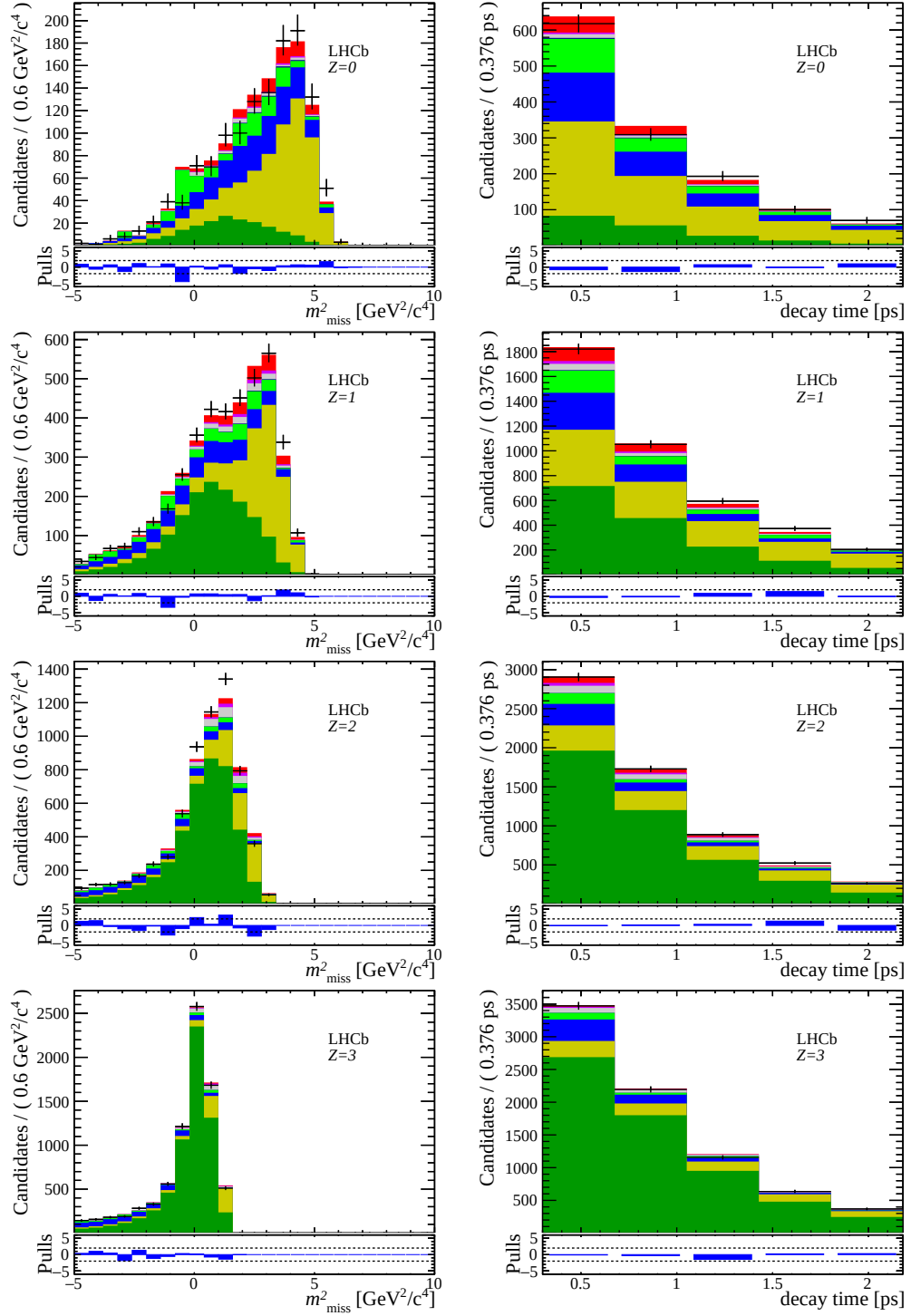
Figure 4.30: Projections of the nominal fit in bins 0–3 of Z , i.e. , individual bins of q^2 and E_\mu^* .
