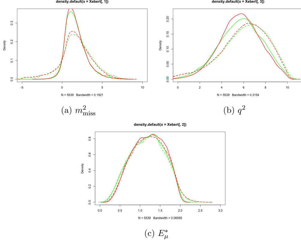
Figure E.8: The results of the kNN resampling closure test. Shown, from both the EFG generator-level MC (green) and independent full MC (red), are the distributions of the true variables (solid line) and the resampled or directly reconstructed distributions, respectively (dashed).
