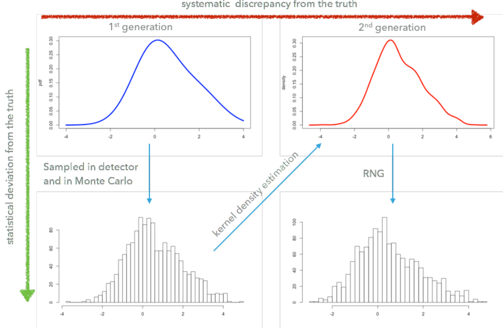
Figure 4.4: Applying a kernel smoothing procedure to sampled simulation data produces second-generation distributions f_{i,2}(x) (top right), which can quickly sampled via RNG (bottom right).
