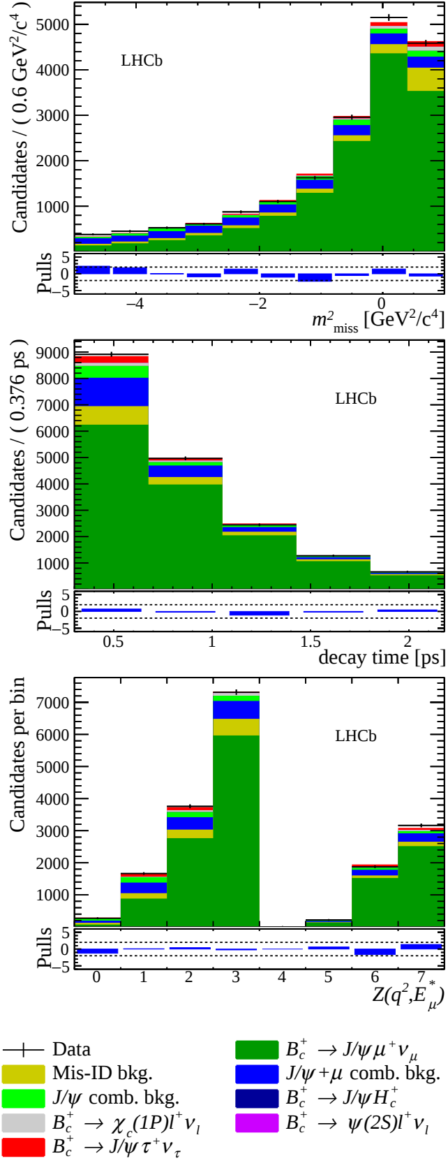
Figure 4.10: Projections of fit to normalization-rich region (including data and the non-signal component templates) onto m_{\text{miss}}^2 (top), t (middle), and Z (bottom)
