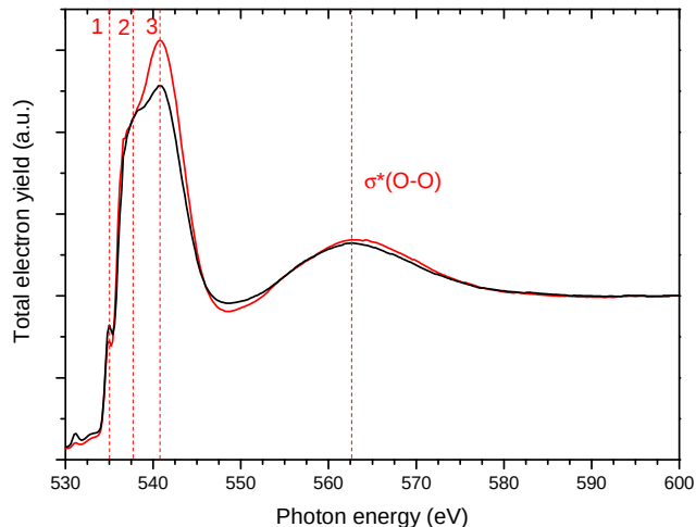
FIG. 1. Total electron yield (TEY) as a function of photon energy at 15 K (black trace) and 90 K (red trace) from c-ASW grown at 90 K. The curves have been normalized at 600 eV. The water features are indicated by vertical dashed red lines (see the text for attributions).
