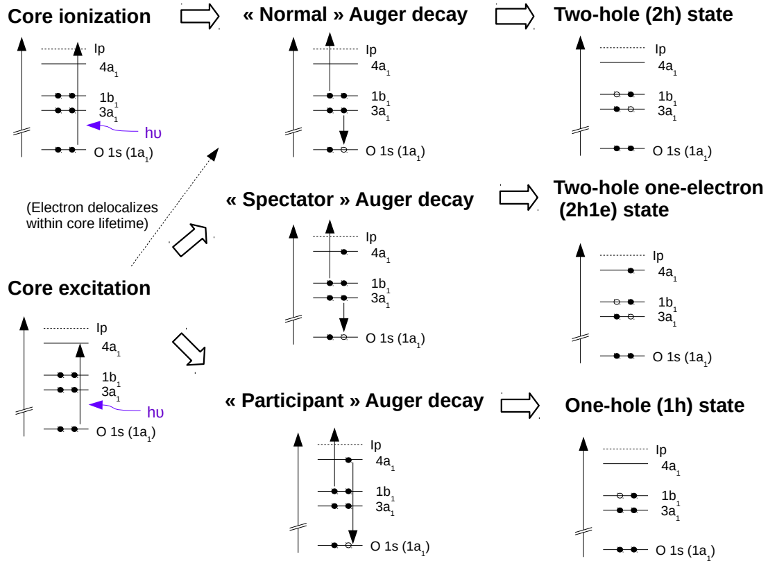
Figure II.10: Schematic representation of the Auger decay process. The example is given using the molecular orbitals of H 2 O: the 1a 1 is the core oxygen orbital, the 1b 1 and 3a 1 are occupied valence orbitals and the 4a 1 is an empty molecular orbital. "Ip" indicates the ionization threshold. Two cases are distinguished, core excitation and core ionization. The valence holes were arbitrarily chosen: other possible final states with different valence holes are possible. See the text for more details.
