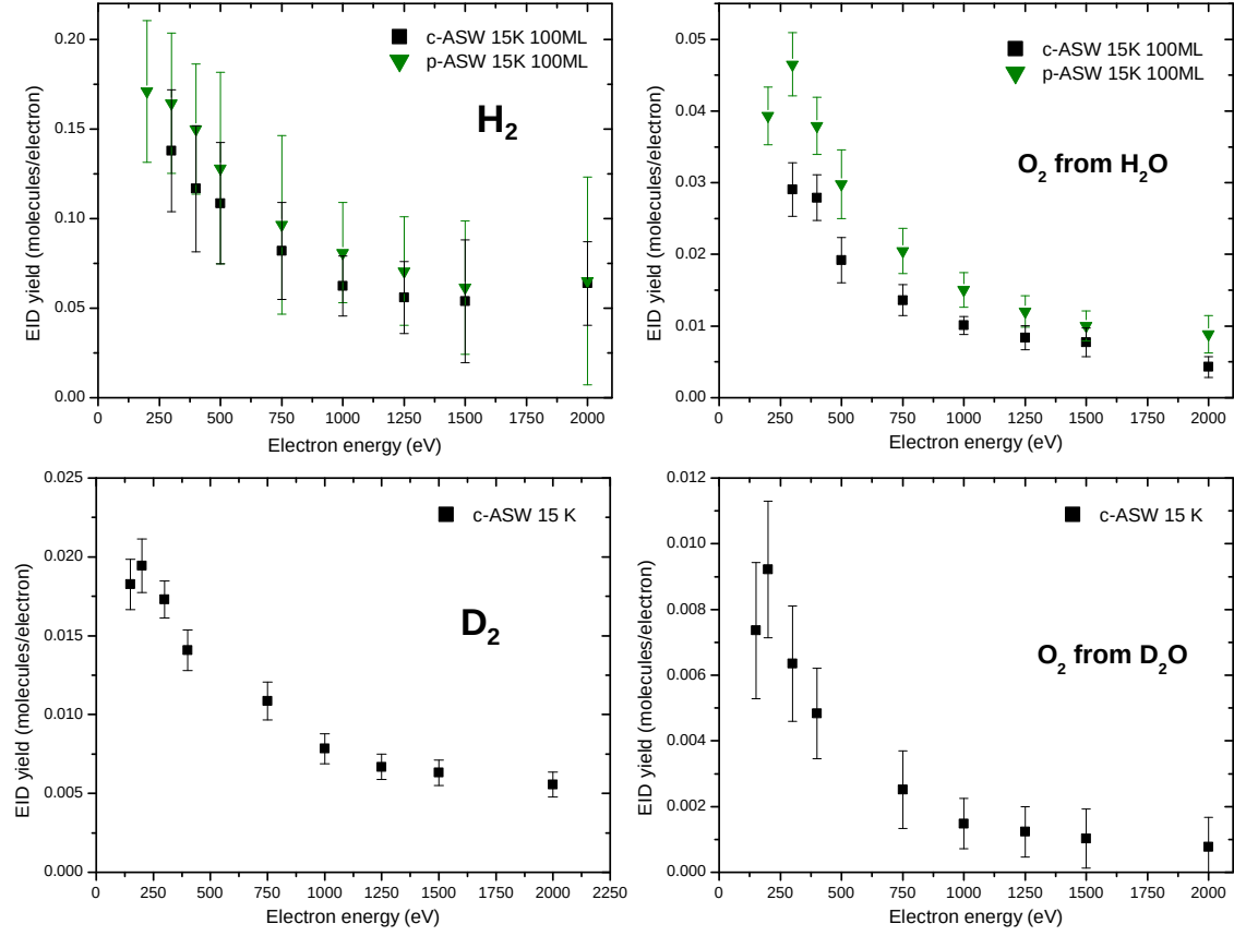
Figure V.14: EID yield curves of H 2 (top left) and O 2 (top right) from H 2 O ice for c-ASW and p-ASW at 15 K, and D 2 (bottom left) and O 2 (bottom right) from D 2 O ice for c-ASW at 15 K.
