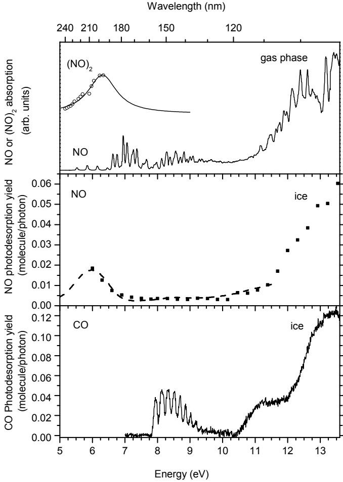
Fig. 1. Upper panel: electronic spectrum of gas-phase NO from Chang et al. (1993) and electronic spectrum of gas-phase (NO) 2 from Forte & Van Den Bergh (1978, open dots) and its Lorentzian fit (solid line). Middle panel: NO photodesorption spectrum of 10 ML thick NO ice on HOPG at 10 K between 6 and 13.6 eV (filled squares). Large energy steps of 0.3 eV were used to avoid ice ageing. Absorption spectrum of pure solid NO from Lu et al. (2008) between 5 and 11.7 eV (dashed line). The absorption spectrum is scaled to the photodesorption spectrum. Lower panel: CO photodesorption spectrum of a 20 ML thick CO ice on gold at 10 K between 7 and 13.6 eV (Dupuy et al. 2017).
