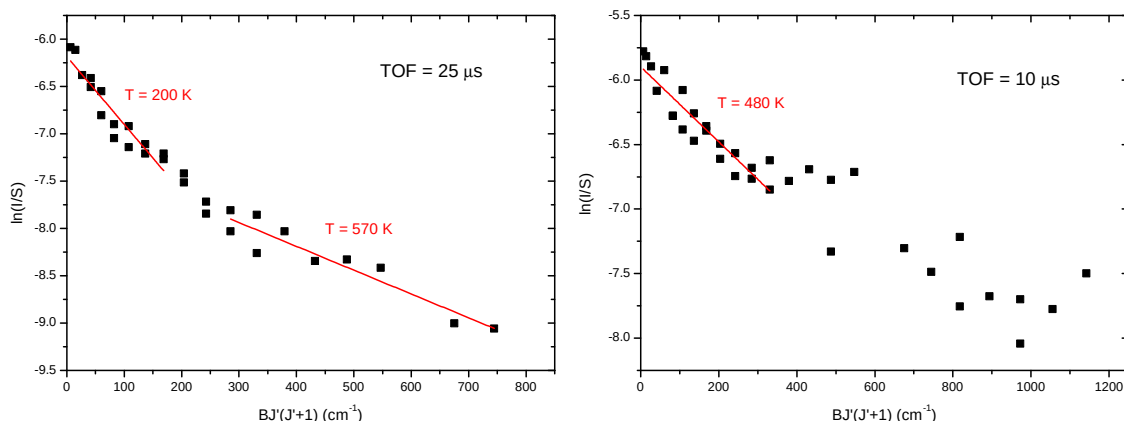
Figure IV.17: Rotational populations (similar to fig. IV.14) of desorbed NO for a TOF of 25\ \mu\text{s} (on the left) or 10\ \mu\text{s} (on the right). In red fits with Maxwell-Boltzmann distributions and the fitted temperatures are indicated. Desorption laser energy \sim 80\ \mu\text{J}/\text{pulse} , REMPI laser energy \sim 50\text{-}70\ \mu\text{J}/\text{pulse} .
