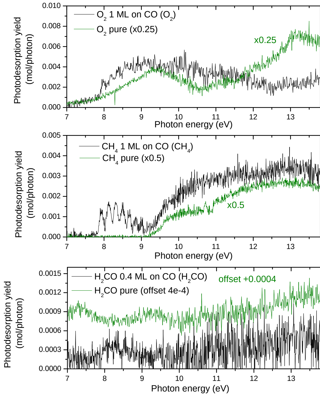
Figure IV.35: Photodesorption spectra of \text{O}_2 , \text{CH}_4 and \text{H}_2\text{CO} single layers on CO. Top: photodesorption of \text{O}_2 from 1 ML \text{O}_2 on CO and from pure \text{O}_2 . Middle: photodesorption of \text{CH}_4 from 1 ML \text{CH}_4 on CO and from pure \text{CH}_4 . Bottom: photodesorption of \text{H}_2\text{CO} from 0.4 ML \text{H}_2\text{CO} on CO and from pure \text{H}_2\text{CO} .
