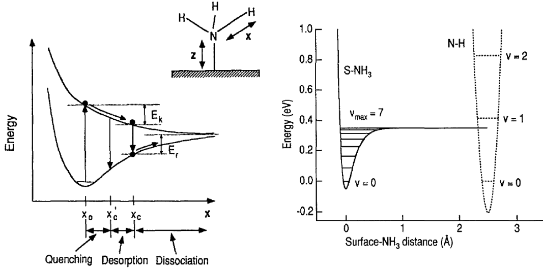
Figure II.12: Principle of the desorption mechanism of NH 3 on GaAs. Adapted directly from ref. [159]
