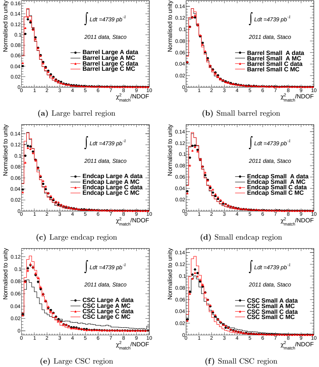
Figure 5.22: \chi^2_{\text{match}} distributions for muon probes with 10 \text{ GeV} < p_T < 30 \text{ GeV} normalised to unity area evaluated in 2011 data and simulations for different MS regions. Regions in side A ( \eta > 0 ) are drawn in black, regions in side C ( \eta < 0 ) in red (see Section 5.1.1).
