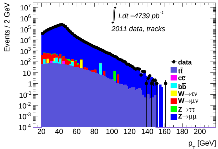
Figure 5.11: p_T distribution of ID probe muons selected for MS reconstruction efficiency measurement.
