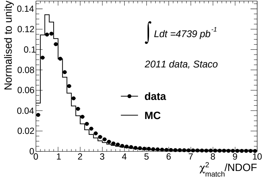
Figure 5.20: \chi^2_{match} distribution of muon probes from Z \rightarrow \mu\mu events in 2011 data and simulation normalised to unity.
