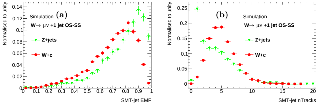
Figure 7.6: Electromagnetic energy fraction EMF (a) and track multiplicity nTracks (b) distributions normalised to unity for SMT tagged jet in Monte Carlo Z + jets (green) and W + c (red) muon channel events. No dilepton invariant mass cut is applied to the events in the plots. Only statistical errors are shown.
