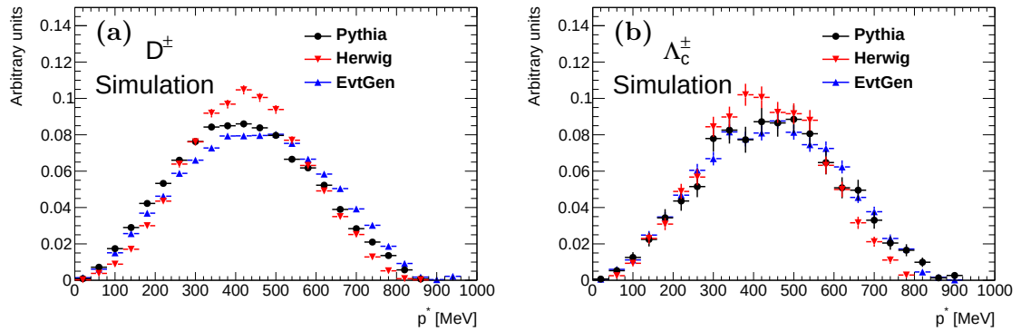
Figure 7.13: Normalised distributions of the momentum p^* of the soft muons from decays of c -hadrons D^\pm (a) and \Lambda_c^\pm (b) at rest, as predicted by PYTHIA (black), HERWIG (red) and EVTGEN (blue).
