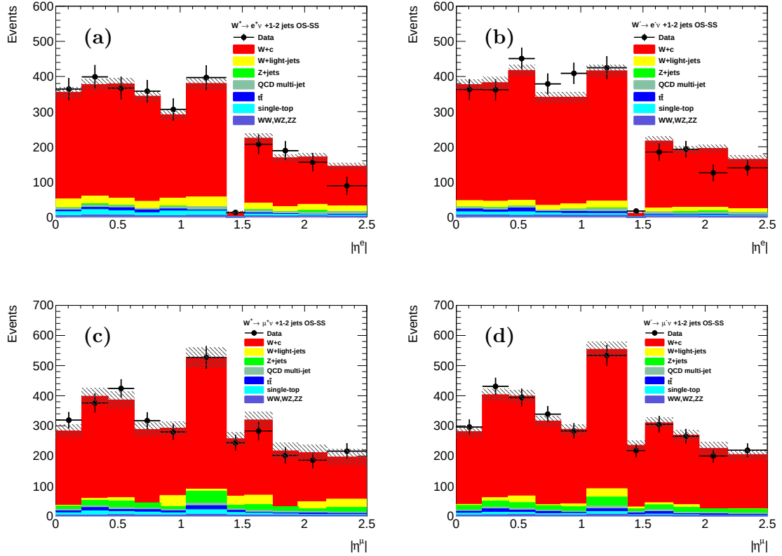
Figure 7.11: W^+ + c -jet (a, c) and W^- + c -jet (b, d) event yields as a function of |\eta^\ell| of the lepton from the W decay in the electron (a, b) and muon (c, d) channels for the combined 1+2-jet sample. The signal and background contributions are described in the text.
