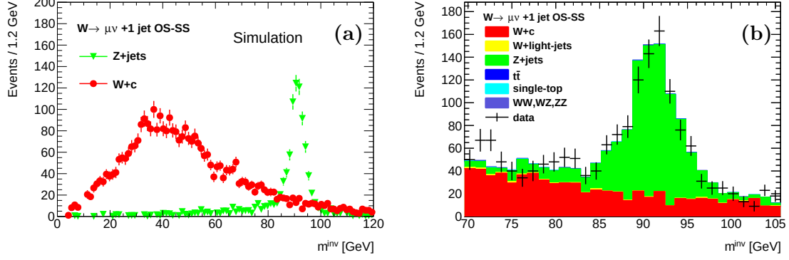
Figure 7.7: (a) Distributions of the invariant mass m(\mu, \text{soft-}\mu) of hard and soft muons in Monte Carlo Z + \text{jets} and W + c events after the selection. (b) data m(\mu, \text{soft-}\mu) distribution near the Z peak with the estimated background contributions. The W + c normalisation from simulations is increased by 27% as determined by the procedure described in the text, the Z + \text{jets} simulated distributions is corrected for the results of the data-driven estimation discussed in this section. The QCD multi-jet contribution is expected to be negligible and is therefore not considered in the plot, the t\bar{t} , single-top and diboson contributions are predicted to be small.
