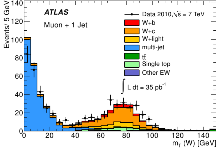
Figure 6.4: W transverse mass distribution in the W + b -jets signal region for the muon channel in the 1-jet category without cut on m_T^W [1]. The multi-jet contribution is normalised using the data-driven technique while all other contributions are from Monte Carlo simulations.
