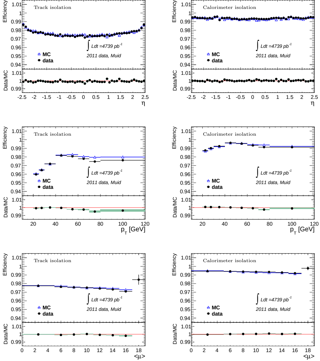
Figure 5.19: Muon isolation efficiency measurement for 2011 data and simulation for a track isolation cut of \sum^{\Delta R=0.3} p_T^{tracks} < 2.5 GeV (left plots) and a calorimeter isolation cut of \sum^{\Delta R=0.2} E_T^{calo} < 4 GeV (right plots). Only statistical errors are shown.
