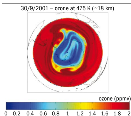
The ozone-mixing ratio in the southern hemisphere on 30 September 2001, measured using an application that will be run completely on EGEE. (Courtesy S Godin-Beekmann IPSL/Service d'Aéronomie.)
