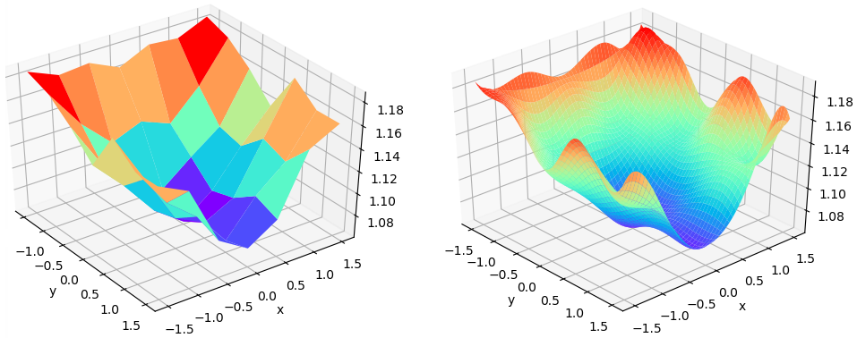
Figure 9: The second weighing function considered. The left graph shows to the data from the simulation and the right graph its cubic interpolation. The x and y coordinates represents the shifts of the screening conductors' effective center. The corresponding z coordinates represent the maximum electric field measured in the tube for that configuration. This is the weighing function chosen to be used in the optimisation process.
