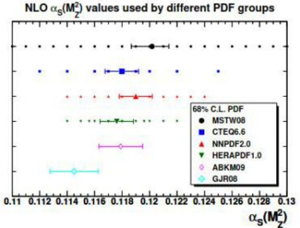
Figure 3.12: Fits for which \alpha_s values are available. Each group's default values and uncertainties are also displayed. G. Watt's plot[45]
