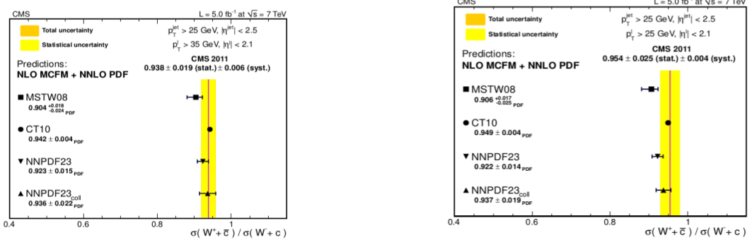
Figure 3.9: Comparison of the average of the experimental data with the theoretical predictions for (\frac{W^+ + \bar{c}}{W + c}) calculated with MCFM and other sets of PDFs. The predictions for a transverse momentum threshold of the lepton, p_T^l > 25 \text{ GeV} for W-boson decay are shown in the right plot and the left plot presents the predictions for p_T^l > 35 \text{ GeV} . The uncertainty associated with the scale variation is \pm 1\%
