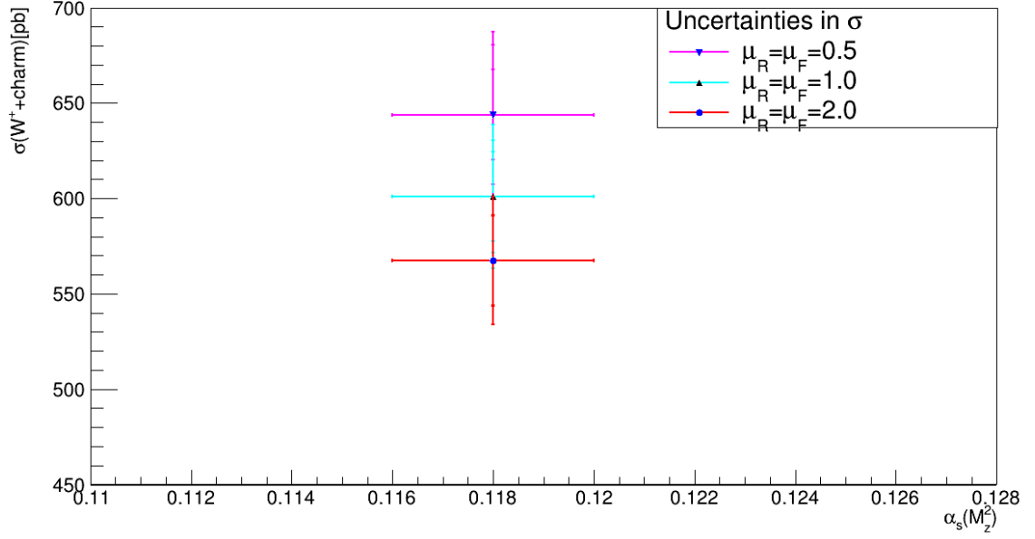
Uncertainty in the \sigma at 14 TeV using NNPDF :305000
