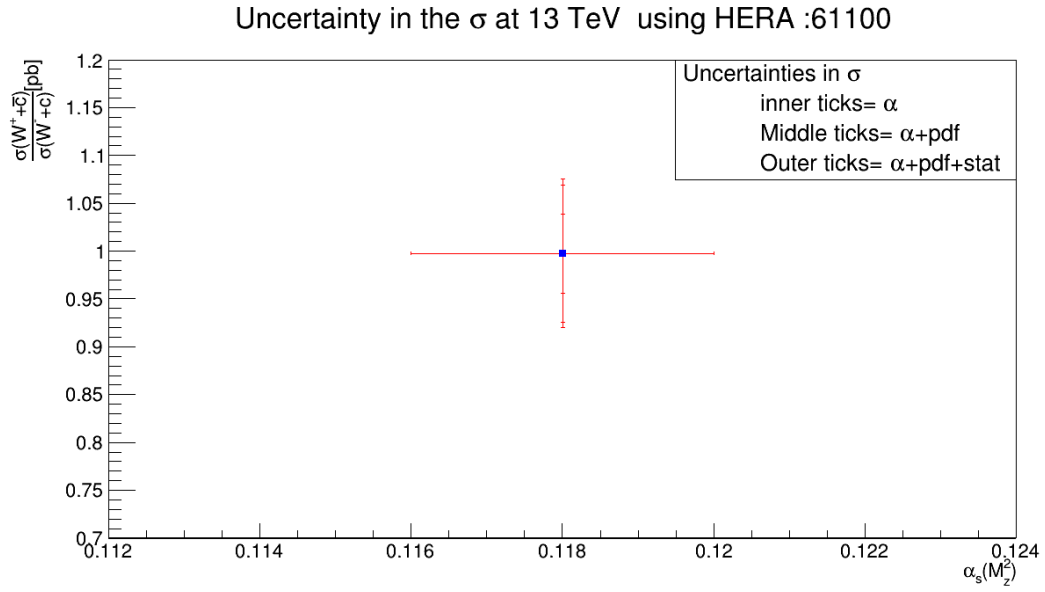
Figure 4.5: Plots (a) and (b) show predicted cross section and uncertainties in the cross section of W + c , (c) and (d) show predicted cross section and uncertainties in the cross section of W^+ + \bar{c} , (e) and (f) show predicted cross section and uncertainties in the cross section of W^- + c while (g) and (h) show predicted cross section and uncertainties in the cross section of \frac{W^+ + \bar{c}}{W^- + c} by using NNPDF31 and HERAPDF at 13 TeV .
