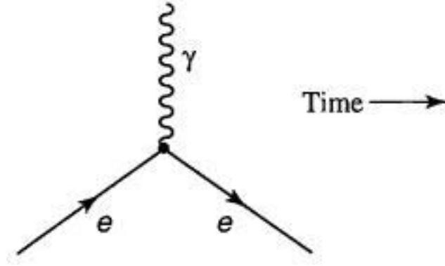
Figure 1.3: Feynman Diagram
