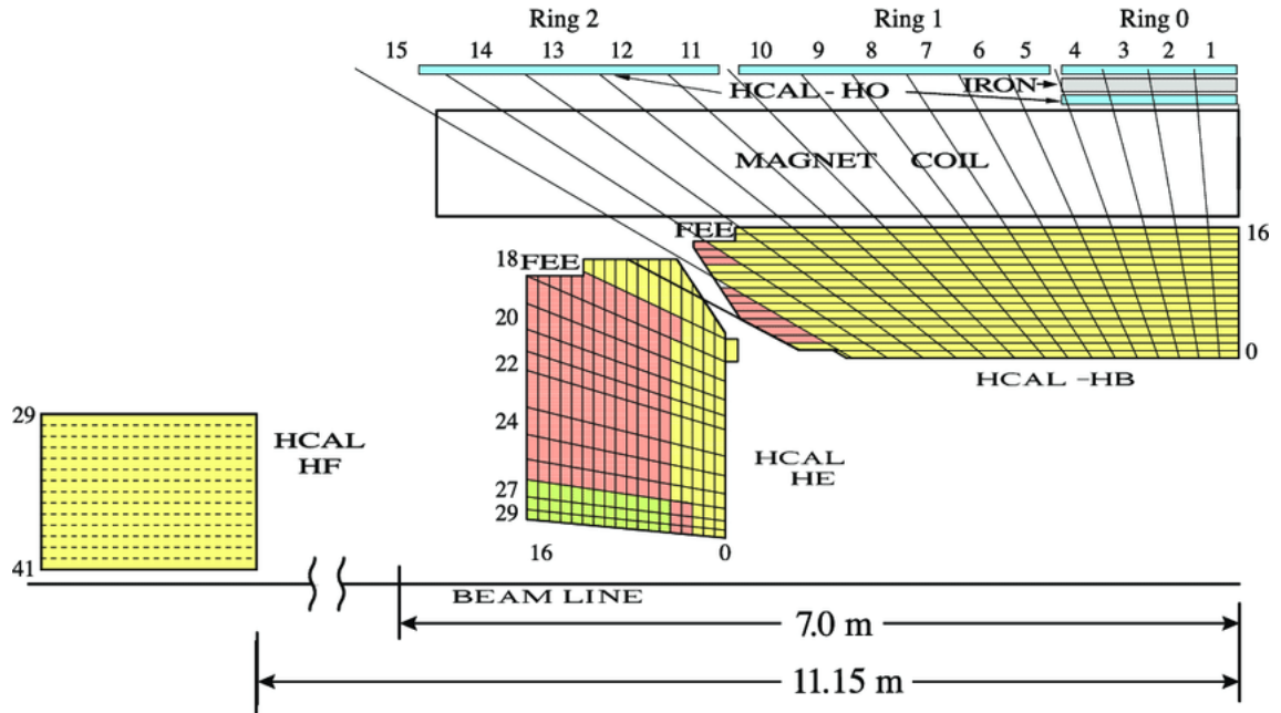
Figure 2.7: Hadron Calorimeter
