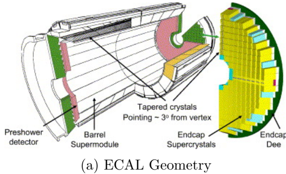
Figure 2.6: Electromagnetic Calorimeter
