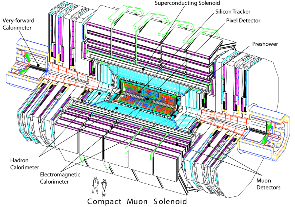
Figure 2.3: CMS detector and its different components [7]
