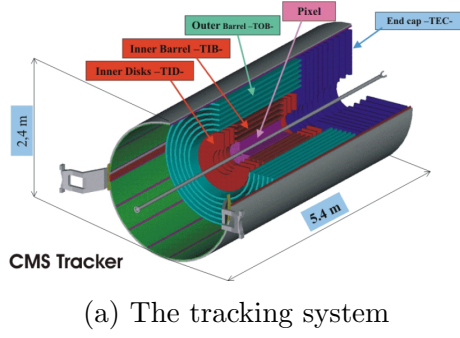
Figure 2.5: Visualization of CMS Tracker
