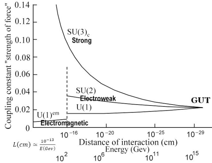
Figure 1.7: Merging of Coupling constant at High Energy
