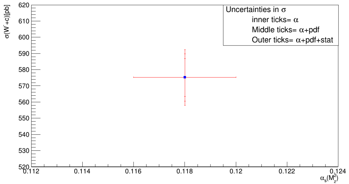
Uncertainty in the \sigma at 13 TeV using HERA :61100
