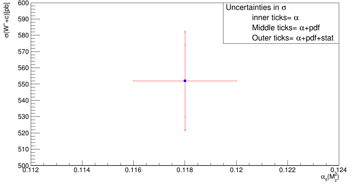
Uncertainty in the \sigma at 13 TeV using NNPDF31 :305000
