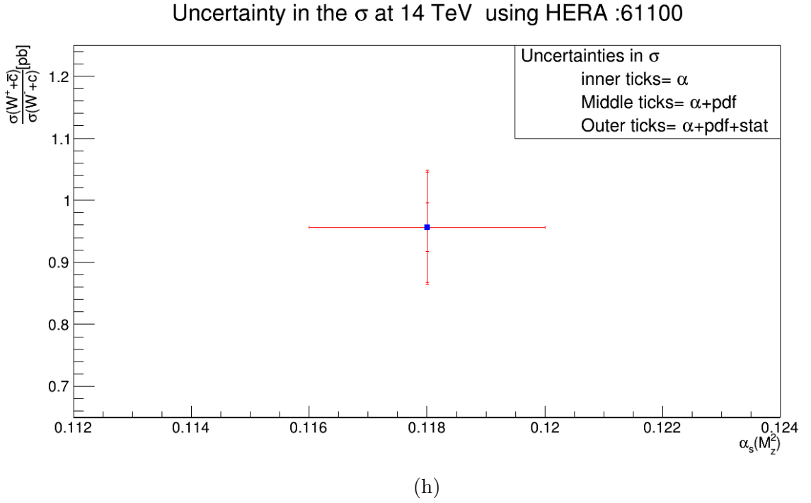
Figure 4.7: Plots (a) and (b) show predicted cross section and uncertainties in the cross section of W + c , (c) and (d) show predicted cross section and uncertainties in the cross section of W^+ + \bar{c} , (e) and (f) show predicted cross section and uncertainties in the cross section of W^- + c while (g) and (h) show predicted cross section and uncertainties in the ratio of \frac{\sigma(W^+ + \bar{c})}{\sigma(W^- + c)} by using NNPDF31 and HERAPDF at 14 TeV .
