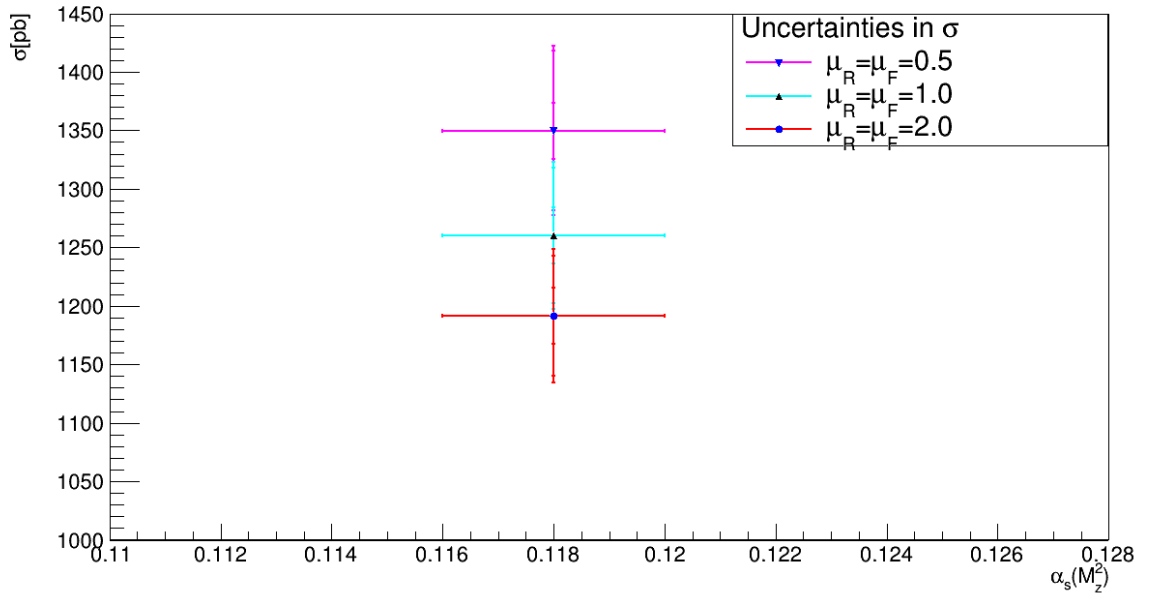
Uncertainty in the \sigma at 14 TeV using HERAPDF :61100
