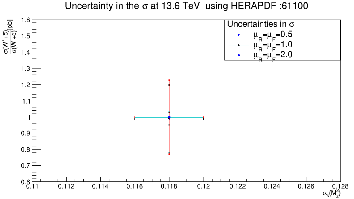
Figure 4.10: Plots (a) and (b) show the predicted change in cross section of W + c , (c) and (d) show the predicted change in the cross section of W^+ + \bar{c} , (e) and (f) show the predicted change in cross section of W^- + c while (g) and (h) show the predicted change in cross section at different QCD scale ( \mu_R and \mu_F ) at 13.6 TeV. The vertical error bars represent: inner (PDF), middle ( \alpha_s ), outer (PDF+ \alpha_s combined) errors.
