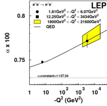
(b) Running coupling constant of QCD with energy Q^2
