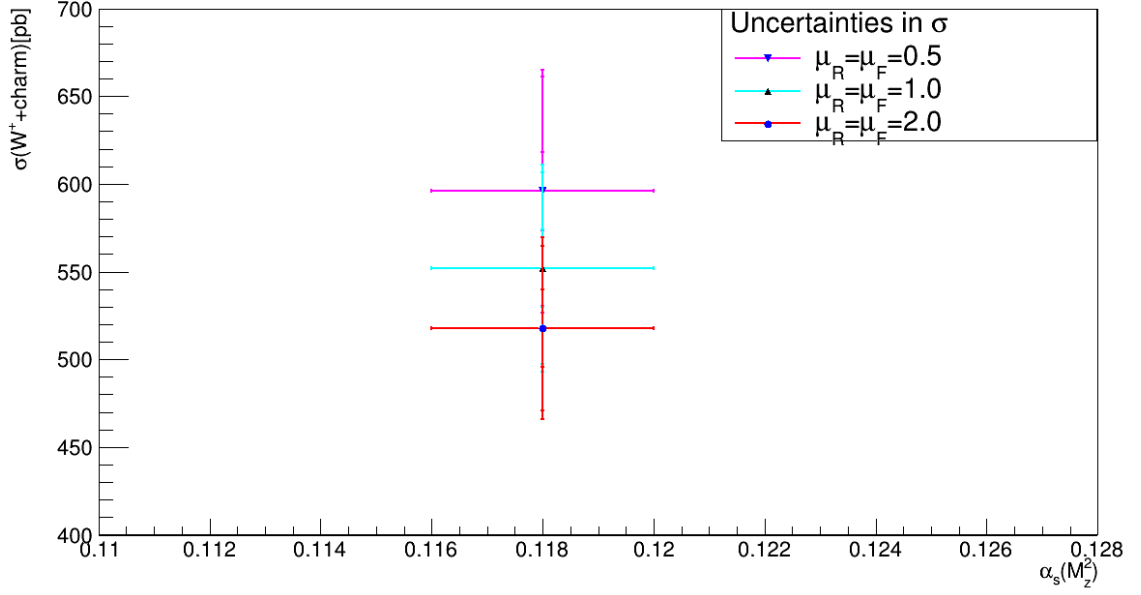
Uncertainty in the \sigma at 13 TeV using NNPDF :305000
