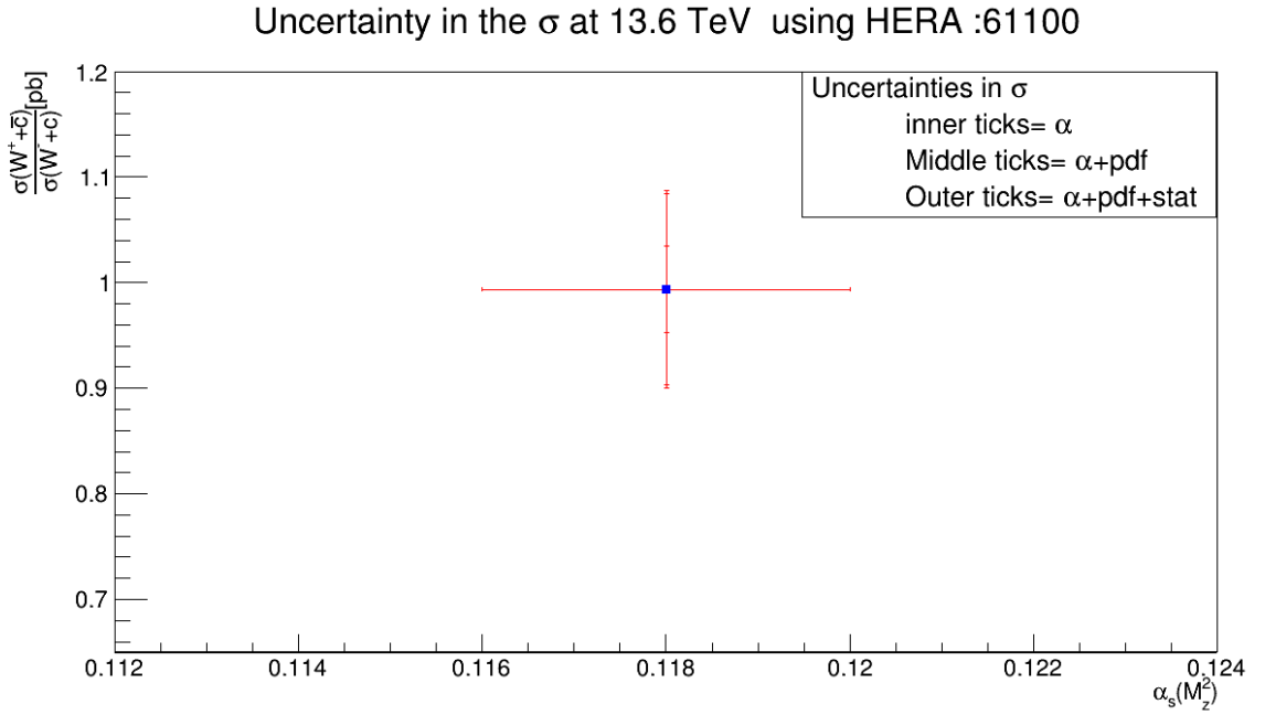
Figure 4.6: Plots (a) and (b) show predicted cross section and uncertainties in the cross section of W + c , (c) and (d) show predicted cross section and uncertainties in the cross section of W^+ + \bar{c} , (e) and (f) show predicted cross section and uncertainties in the cross section of W^- + c while (g) and (h) show predicted cross section and uncertainties in the cross section of \frac{W^+ + \bar{c}}{W^- + c} by using NNPDF31 and HERAPDF at 13.6 TeV.
