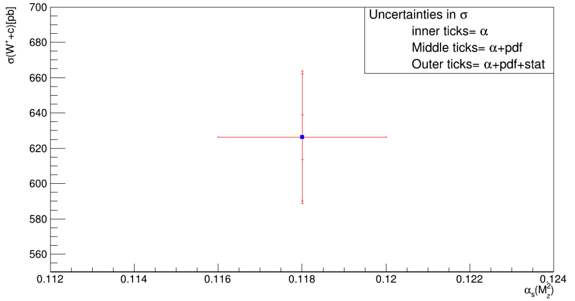
Uncertainty in the \sigma at 14 TeV using HERA :61100
