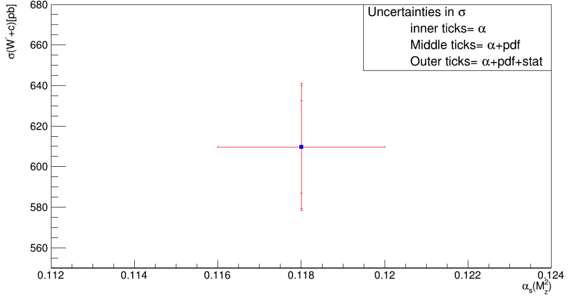
Uncertainty in the \sigma at 14 TeV using NNPDF31 :305000
