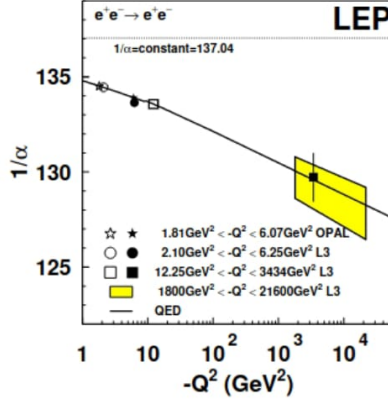
(a) Running coupling constant of QED with energy Q^2
