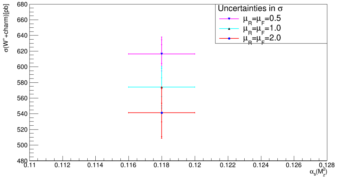
Uncertainty in the \sigma at 13 TeV using HERAPDF :61100
