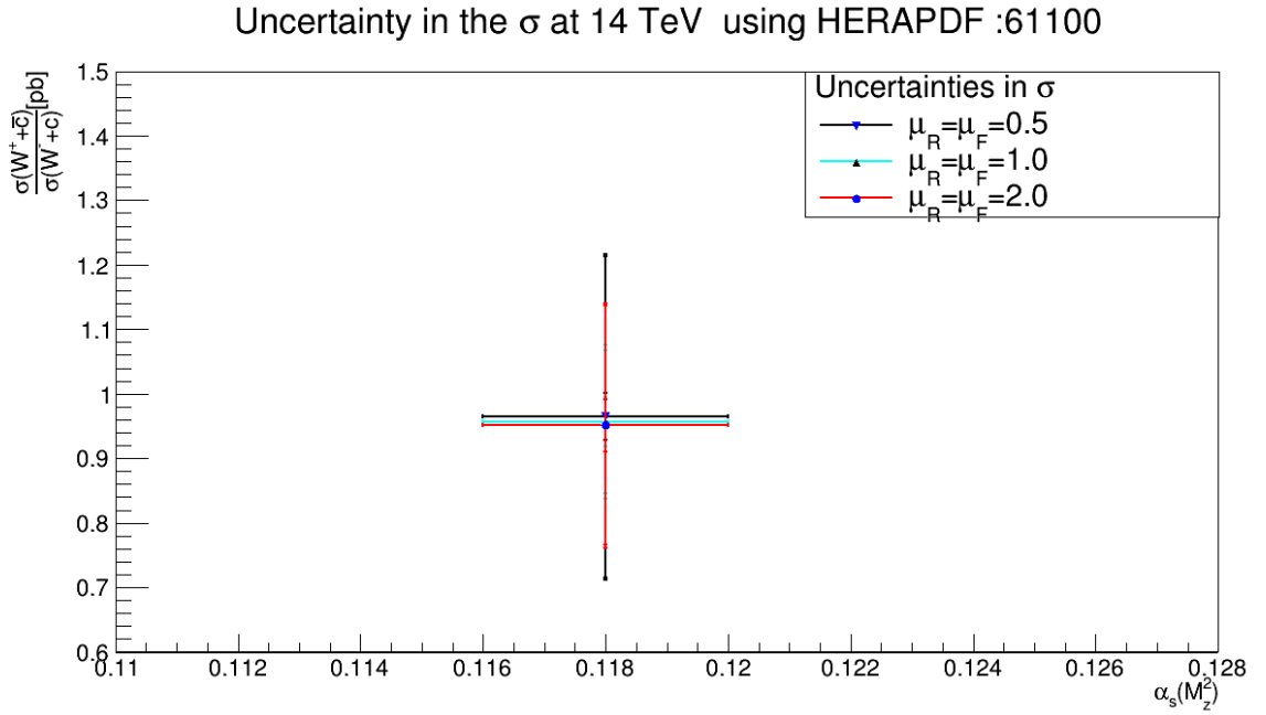
Figure 4.12: Plots (a) and (b) show the predicted change in cross section of W + c , (c) and (d) show the predicted change in the cross section of W^+ + \bar{c} , (e) and (f) show the predicted change in cross section of W^- + c while plots (g) and (h) show the predicted change in cross section at different QCD scale ( \mu_R and \mu_F ) at 14 TeV. The vertical error bars represent: inner (PDF), middle ( \alpha_s ), outer (PDF+ \alpha_s combined) errors.
