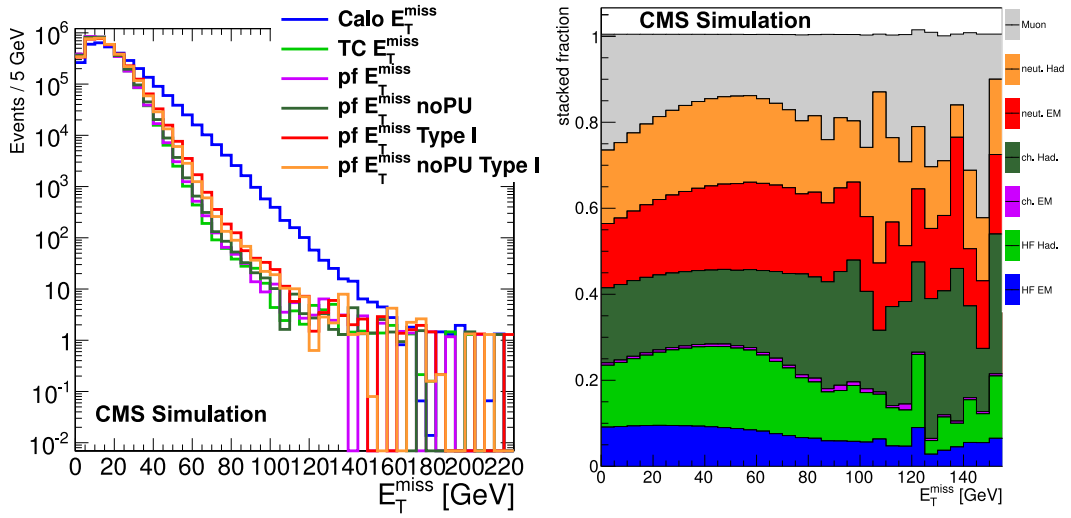
Figure 4.6.: The left Figure shows different reconstruction algorithms for E_T^{\text{miss}} . The different \text{pf}E_T^{\text{miss}} algorithms have a similar description of the Drell-Yan \mu -events where \text{Calo}E_T^{\text{miss}} and \text{TCE}_T^{\text{miss}} have a slightly worse E_T^{\text{miss}} resolution. The right Figure shows the \text{pf}E_T^{\text{miss}} composition for Drell-Yan \mu -events.
