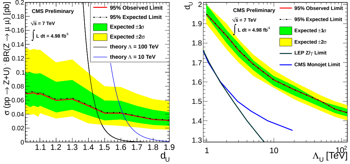
Figure 8.1.: The expected and observed \text{CL}_s limits as a function of d_U (left). The \text{CL}_s limit translated into the plane of \Lambda_U and d_U (right). For the parameter values below the limit curve the 95% CL cross section limit is less than the theoretical cross section.
