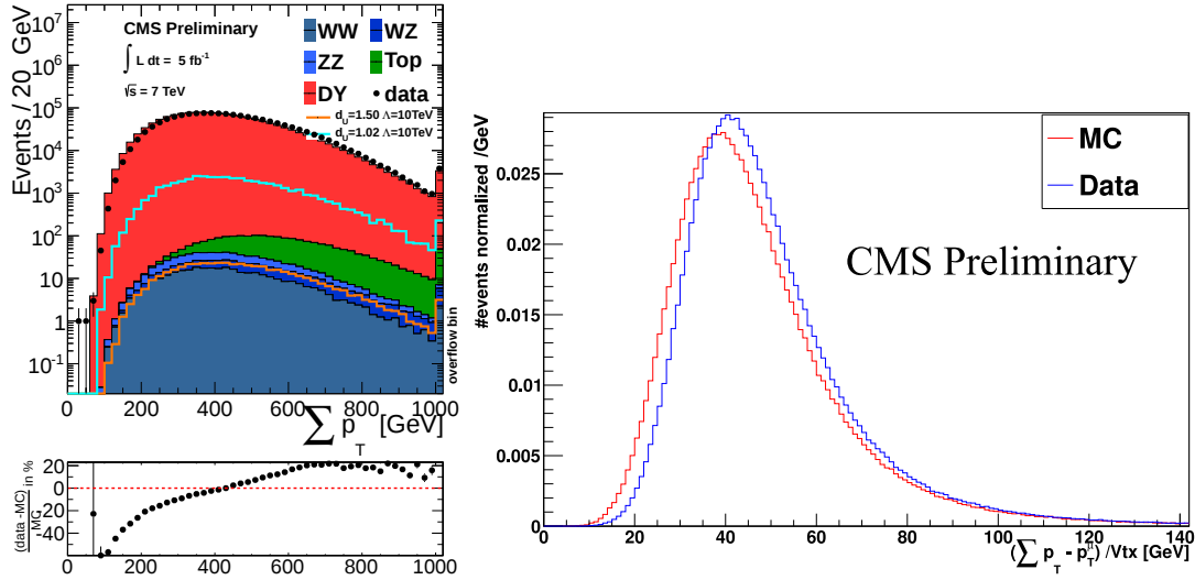
Figure 7.14.: More \Sigma p_T is observed in data than in simulation (left). The shift can be seen more clearly when the muons are subtracted from \Sigma p_T and divided by the number of observed vertices (right). The mean shifts 2.52 GeV in MC with respect to data.
