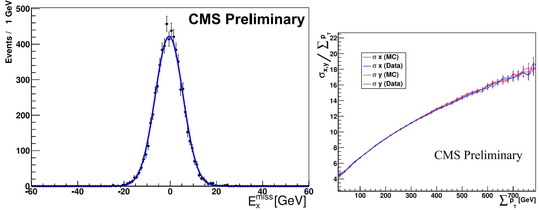
Figure 7.13.: In the left plot an example fit of E_T^{\text{miss}} is shown, on the right side the results of all fits for simulation and data. A good agreement is observed.
