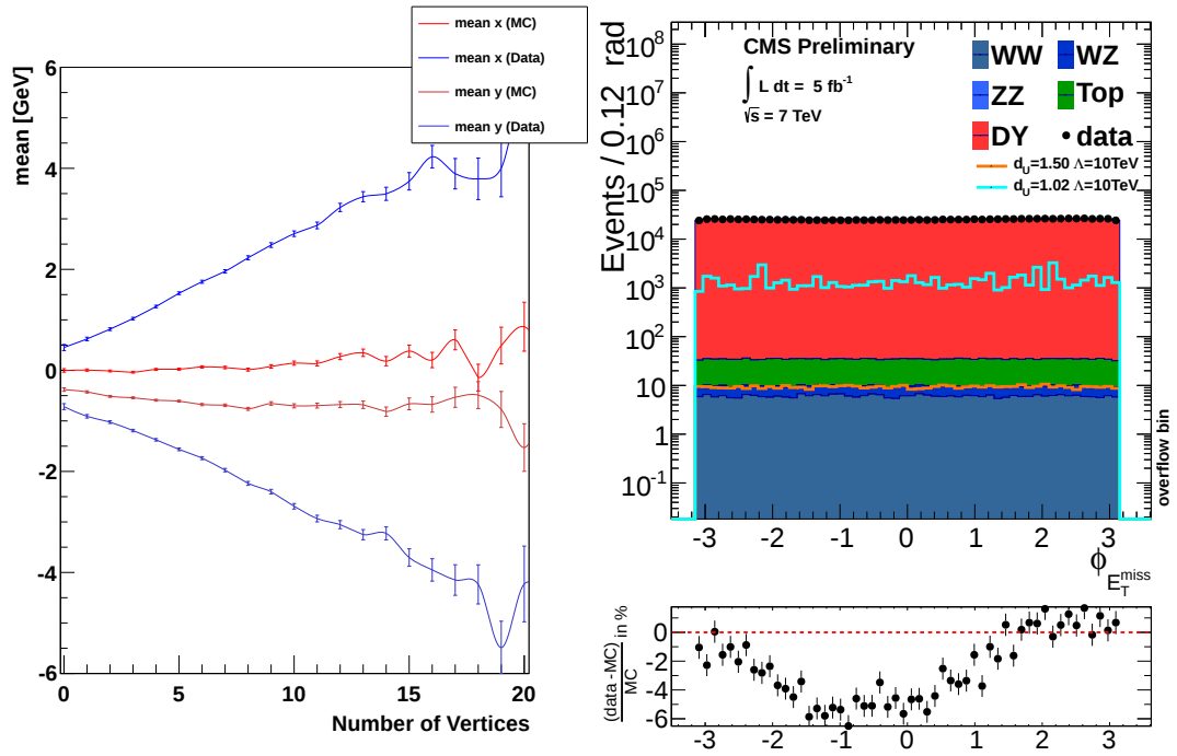
Figure 4.12.: The mean of the x and y component of E_T^{\text{miss}} is plotted in the left against the number of vertices. The corrected E_T^{\text{miss}}-\phi in the right shows less disagreement between data and MC.
