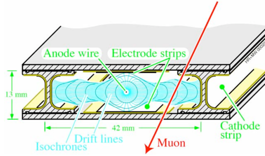
Figure 3.5.: Sketch of a drift tube cell showing drift lines and isochrones [40].
