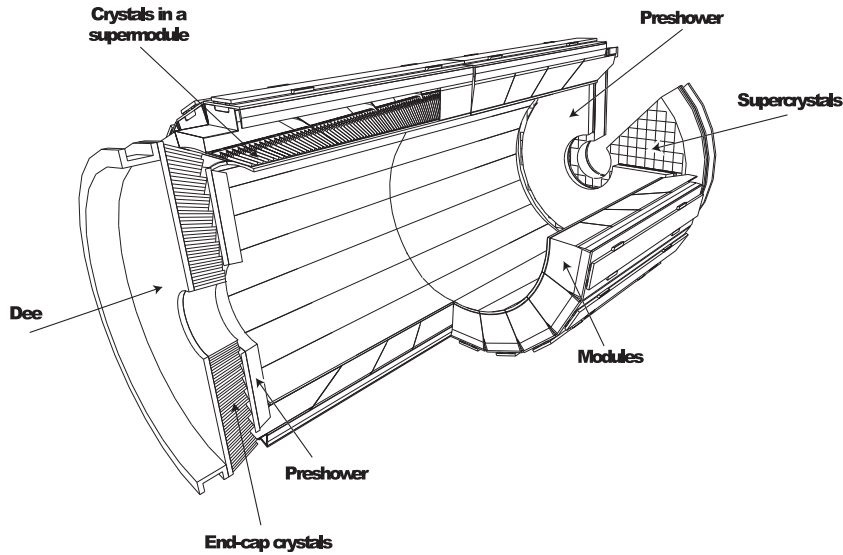
Figure 3.3.: The CMS electro magnetic calorimeter [40].
