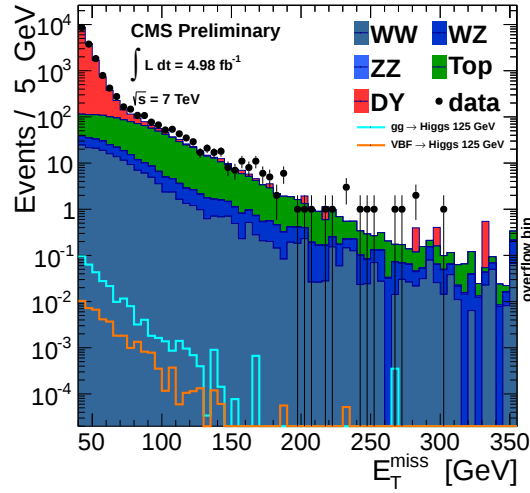
Figure 7.5.: The Higgs contribution from the H \rightarrow (ZZ \rightarrow 2\mu 2\nu) channel has no significant effect on the signal.
