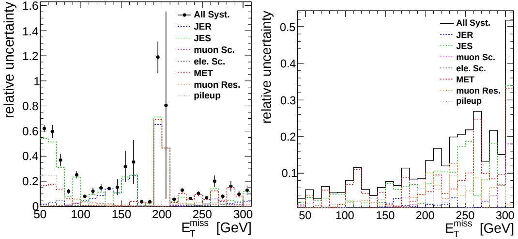
Figure 7.11.: The influences of the various systematic uncertainties depending on the E_T^{\text{miss}} distribution for the backgrounds used from simulation is shown in the left plot. The added systematic uncertainties show that for high E_T^{\text{miss}} the statistical significance of the simulation is low. This is due to missing Drell Yan statistics, which is the main source of the systematic uncertainties. A detailed discussion can be found in Section 7.4. For the signal with d_U = 1.1 the systematic uncertainties are shown in the right plot. The systematic uncertainties increase with higher E_T^{\text{miss}} values.
