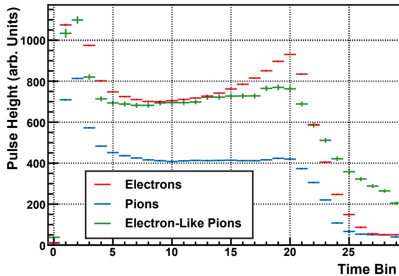
Figure 7.21: Average pulse height distributions for electrons (red), pions (blue), and pions with an electron likelihood larger than 0.99 (green). Pions with large electron likelihood show in contrast to the other particle classes a clear signal at time bins larger than 24.
