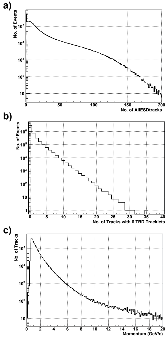
Figure 8.7: Results of simulation of 4.5 million 10 TeV pp collisions. a) number of ESDtracks per event, b) number of TRDtracks traversing six chambers, and c) number of TRDtracks traversing six chambers versus momentum.
