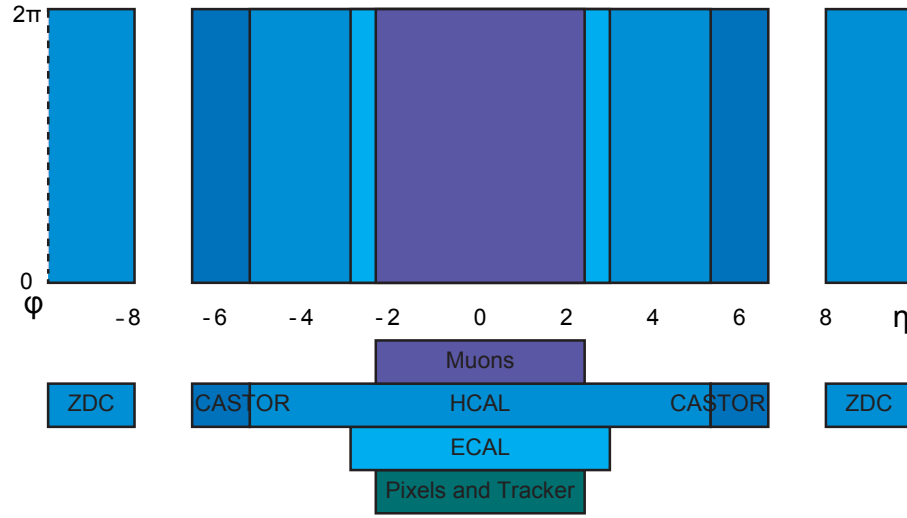
Figure 9.10: The acceptance of the CMS detector systems [d'E08].
