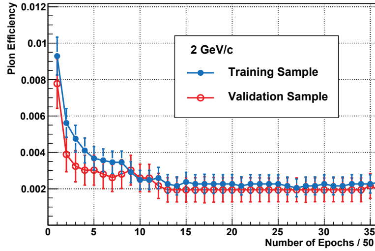
Figure 8.1: Monitoring of the training performance of simulated data with a momentum of 2 GeV/c. The pion efficiency for training (blue) and validation data (red) is plotted versus the number of training epochs.
