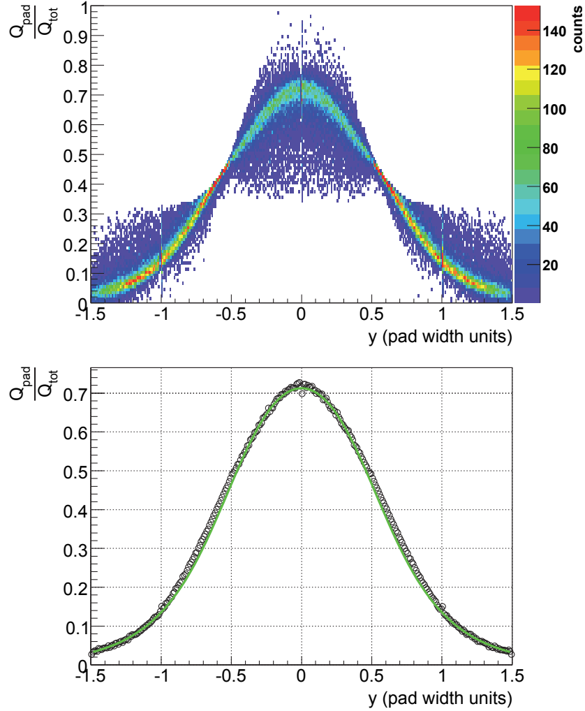
Figure 4.15: Pad Response Function measured with cosmic rays in Münster. The upper plot shows the ratio of pad charge to the total amount of charge versus the distance of the cluster to the pad center. The lower plot shows the measured pad response function (dark dots) and a fit using the Mathieson parametrization [Wul09].
