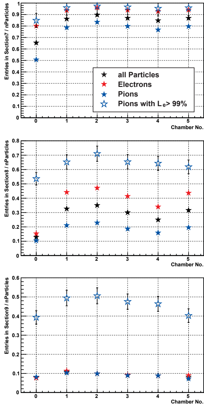
Figure 7.22: Probability for the occurrence of clusters in time bins 22-24 (upper plot), 25-27 (middle plot), and 28-30 (lower plot) versus TRD layer. Shown are the probabilities for electrons, pions, and pions with electron likelihood > 0.99 . Electron-like pions show a clearly larger probability for occurrence of clusters at high time bins compared to the other particle classes.
