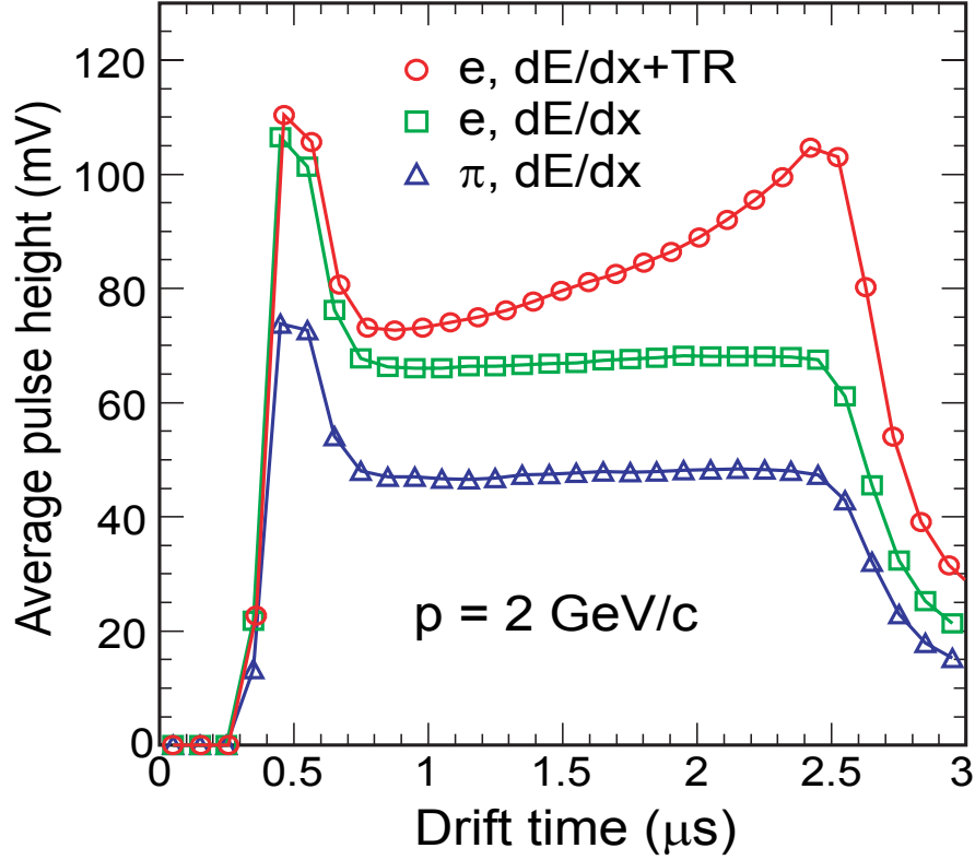
Figure 4.13: The average pulse height in the Transition Radiation Detector for electrons (with and without TR) and pions [Aam08]. The peak at small drift time originates from the amplification region. At larger drift time a plateau can be seen for pions and electrons without TR. The electron signal is about 1.4 times larger than that of pions. In case transition radiation is produced instead of the plateau a second peak can be identified at large drift times. Transition radiation photons are dominantly absorbed within the first few millimeters in the chamber gas and result in the TR peak.
