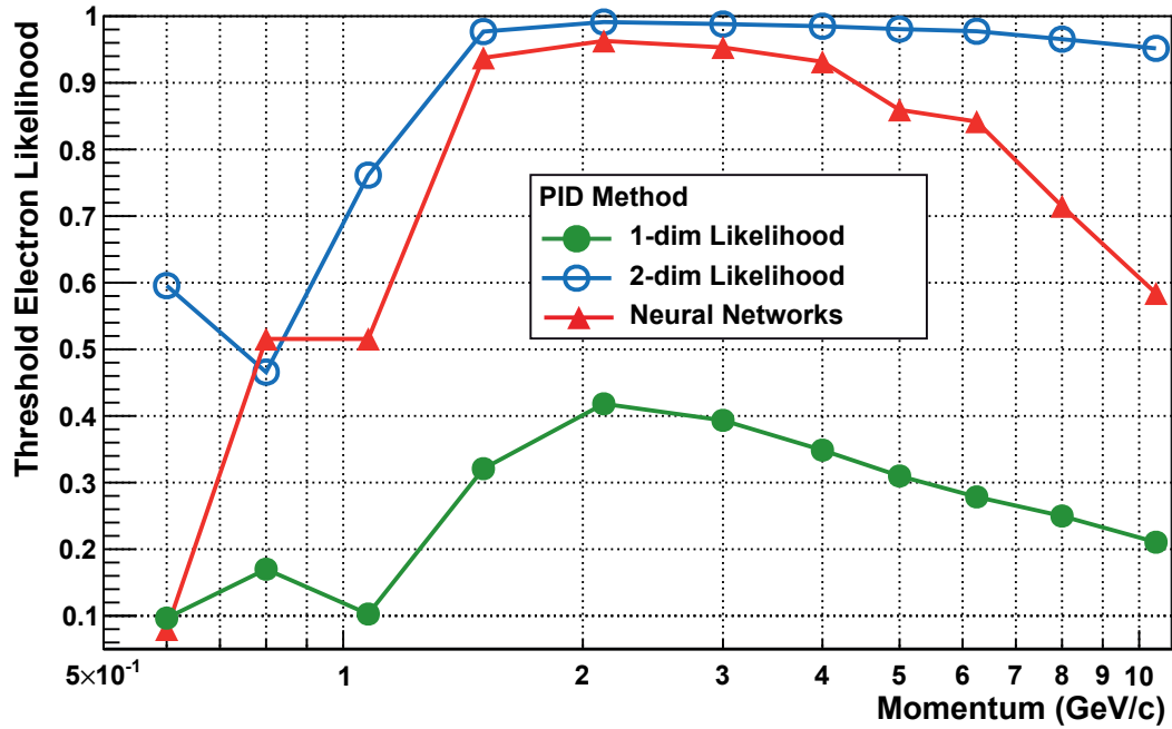
Figure 8.5: Threshold for 90% electron efficiency versus momentum for neural networks (red triangles), 1-dim likelihood (green dots, and 2-dim likelihood (blue circles).
