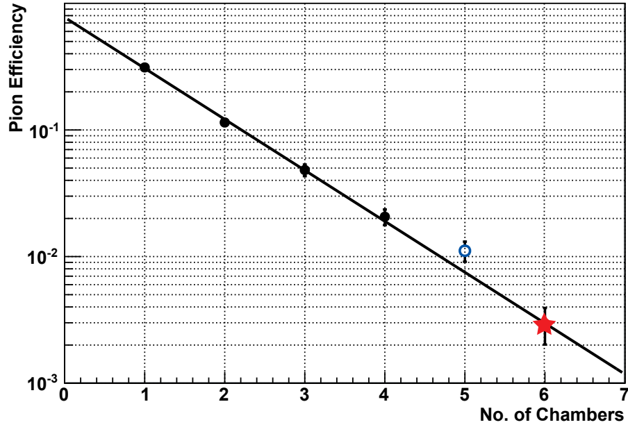
Figure 7.4: Visualization of the extrapolation method. The pion efficiency using artificial neural networks versus the number of TRD layers taken into account for 2 GeV/c particles of 2002 test beam data is shown. Black dots are the calculated pion efficiencies for one, two, three, and four small prototype chambers. The blue circle is the calculated pion efficiency for the small chambers together with a real-size chamber. The red star represents the extrapolated value of pion efficiency using an exponential fit function. The real-size chamber is not taken into account for the extrapolation.
