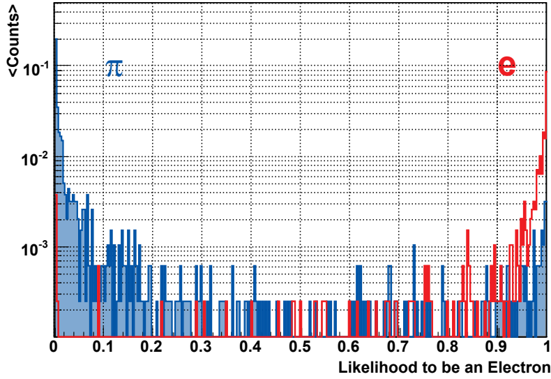
Figure 7.19: Likelihood distribution of electrons (red) and pions (blue) with a nominal momentum of 2 GeV/c. A large contamination of pions at large electron likelihoods is clearly visible.
