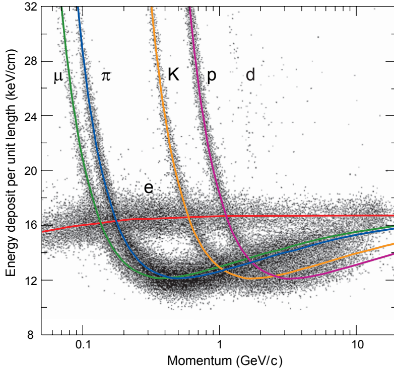
Figure 4.6: The most probable values of the ionization of electrons (red), muons (green), pions (blue), kaons (yellow), and protons (pink) are compared to energy deposit measurements in the PEP4/9-TPC [Ams08].
