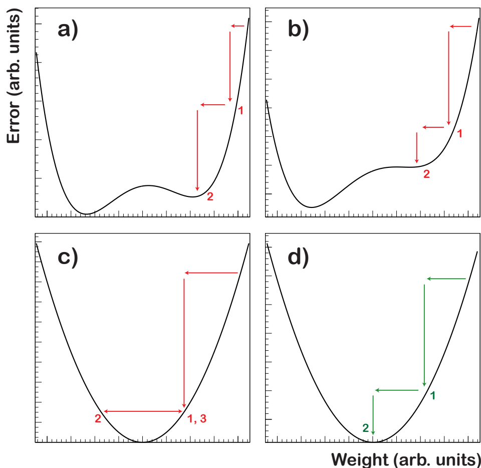
Figure 5.5: Examples of error development of the backpropagation algorithm. In each diagram the error is plotted versus the weight of one synapse. a) : After two steps only a local minimum is found. The learning parameter is too small to reach the global minimum. b) : The procedure stops at a plateau after two steps. The step size of the backpropagation algorithm depends on the gradient. In case of being zero the procedure stops. c) : The learning parameter is too large to reach the minimum. The algorithm oscillates between steps 1, 3 and 2. d) : The learning parameter is optimal. The global minimum is reached after two steps.
