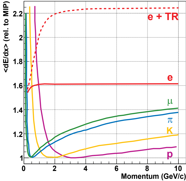
Figure 6.2: The average deposited charge of electrons (with (red dashed line) and without transition radiation (red solid line)), muons (green), pions (blue), kaons (orange), and protons (purple) [And09b]. The deposited charge is plotted relative to the charge deposited by a minimum ionizing particle.
