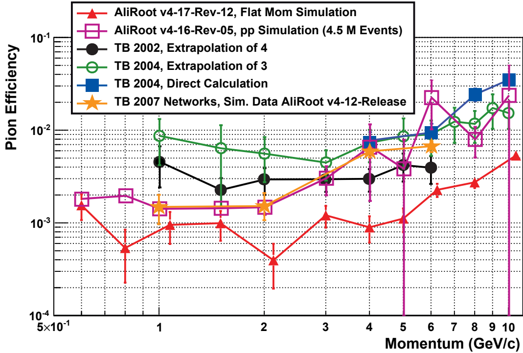
Figure 8.13: Pion efficiency versus momentum for neural networks. The results for simulations using flat-momentum spectra (red triangles) and 10 TeV pp collisions (open purple squares), from test beams 2002 (black dots), 2004 (green circles and blue squares), and simulations applied to networks trained with test beam data (orange stars) are shown.
