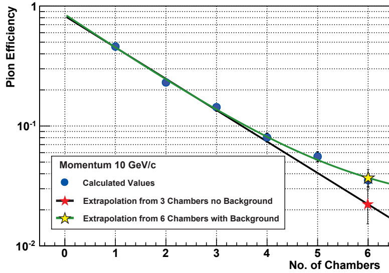
Figure 7.16: Extraction of the shift parameter by fitting the pion efficiencies to an exponential function including a constant shift (green line). The yellow star represents the evaluated pion efficiency using the fit function. The blue dots represent the calculated pion efficiencies versus the number of layers taken into account. The black line is the fit function as used by the extrapolation method, the red star is the corresponding pion efficiency.
