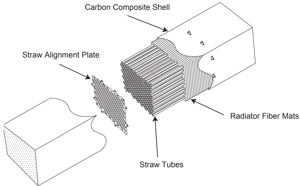
Figure 6.4: A module of the barrel part of the ATLAS Transition Radiation Tracker [Ake98]. The active detector parts is made of small proportional tubes (straw tubes). They are embedded into the radiator material. This detector is optimized for cluster counting methods.
