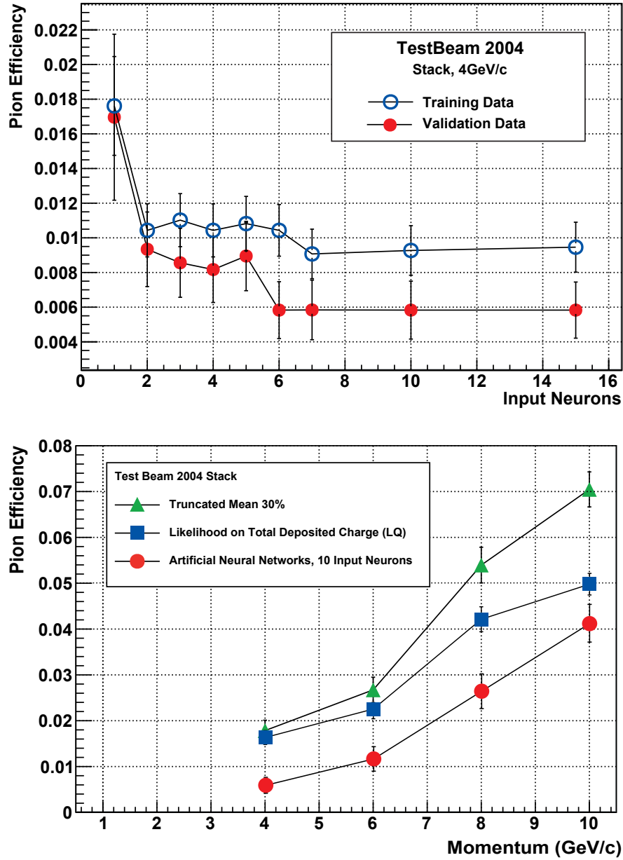
Figure 7.13: Pion efficiency of the stack. a): Pion efficiency versus number of input neurons for 4 GeV/c data. b): Pion efficiency versus momentum.
