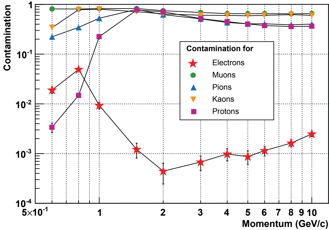
Figure 8.10: Contamination versus momentum for neural networks and different particle species. The results for electron (red stars), muon (green dots), pion (blue triangles), kaon (orange triangles), and proton (purple squares) identification are shown.
