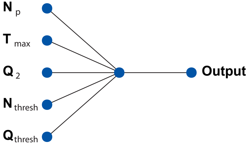
Figure 6.12: The neural network used with preprocessed variables (plot based on Reference [Kim08]). The network uses five input neurons (see text for explanation), one hidden neuron, and one output neuron. This is an untrained net, therefore the connections between the neurons have all the same thickness.
