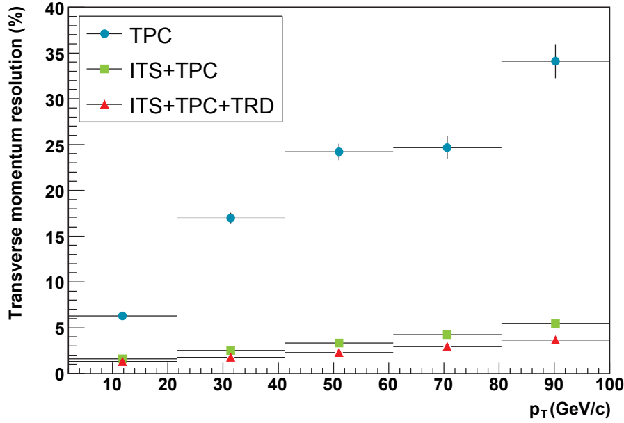
Figure 4.1: Momentum Resolution using the three tracking detectors of the ALICE central barrel for central PbPb collisions [Aam08]. Especially for tracks with high transverse momentum the momentum resolution is improved significantly by adding the Transition Radiation Detector to the combined tracking of the Time Projection Chamber and the Inner Tracking System.
