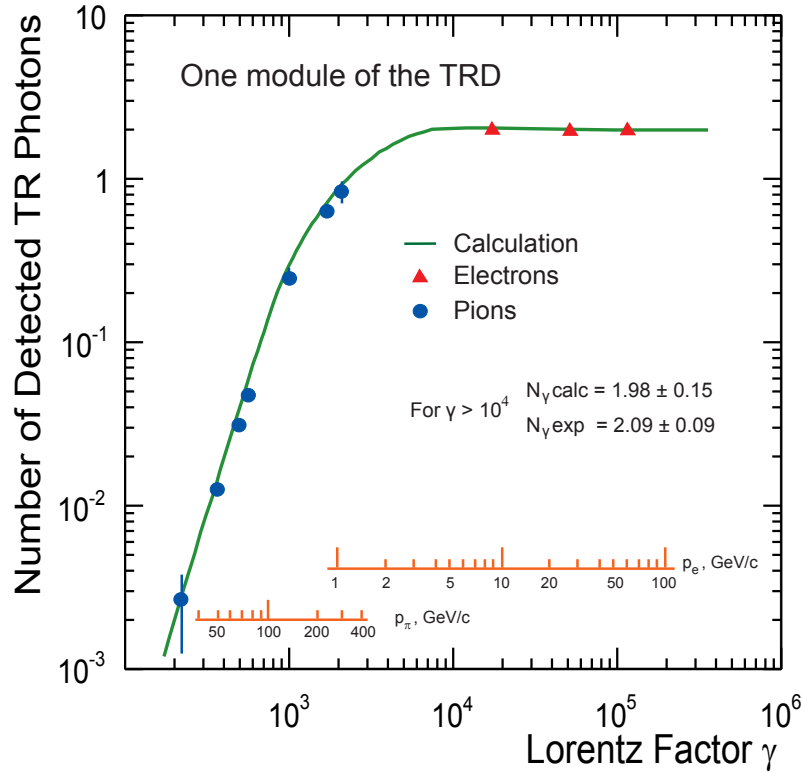
Figure 4.8: Number of detected TR photons versus Lorentz factor \gamma measured with the E715 TRD at Fermilab and compared to calculations [Den84]. With rising \gamma the number of produced TR photons increases. At \gamma \gtrsim 6000 the yield reaches a plateau. Also shown are the momenta of electrons and pions for different values of \gamma . It can be seen that transition radiation is well suited to separate electrons and pions with high momenta.
