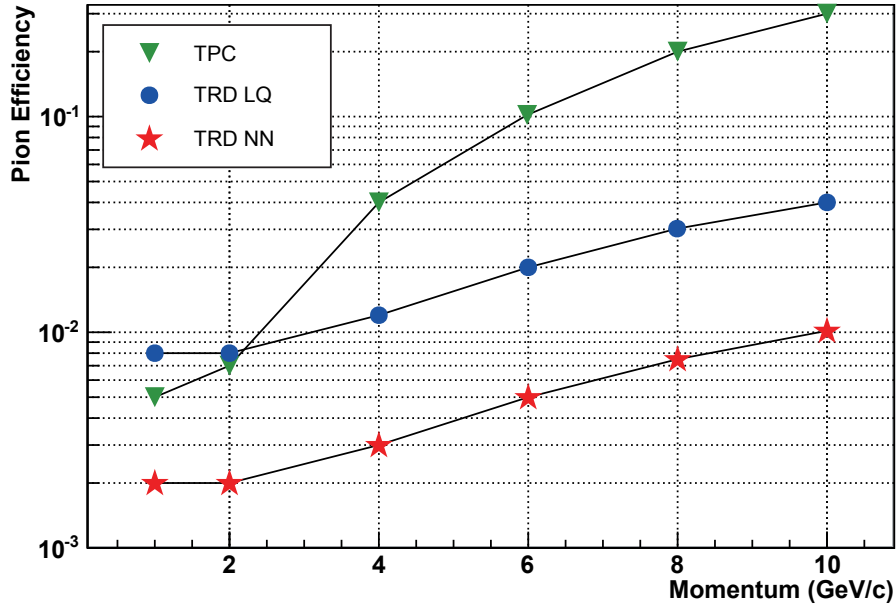
Figure 9.14: Pion efficiency response functions for the TPC (green triangles) and for the TRD are depicted. For the TRD the responses of two PID methods are shown: likelihood on total charge (blue dots) and neural networks (red stars). The pion efficiencies are shown for 90% electron efficiency.
