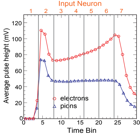
Figure 7.7: Illustration of the input for the artificial neural networks using the deposited charge in seven slices of a TRD module. Analogously to the two-dimensional likelihood method on deposited charge the chamber is divided into several slices.
