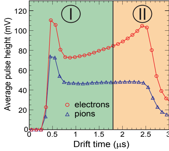
Figure 6.8: Illustration of the two-dimensional likelihood method. The chamber is subdivided into two sectors. In sector II transition radiation is preferably absorbed. The measurement of deposited charge in sector I additionally helps to discriminate electrons from pions.
