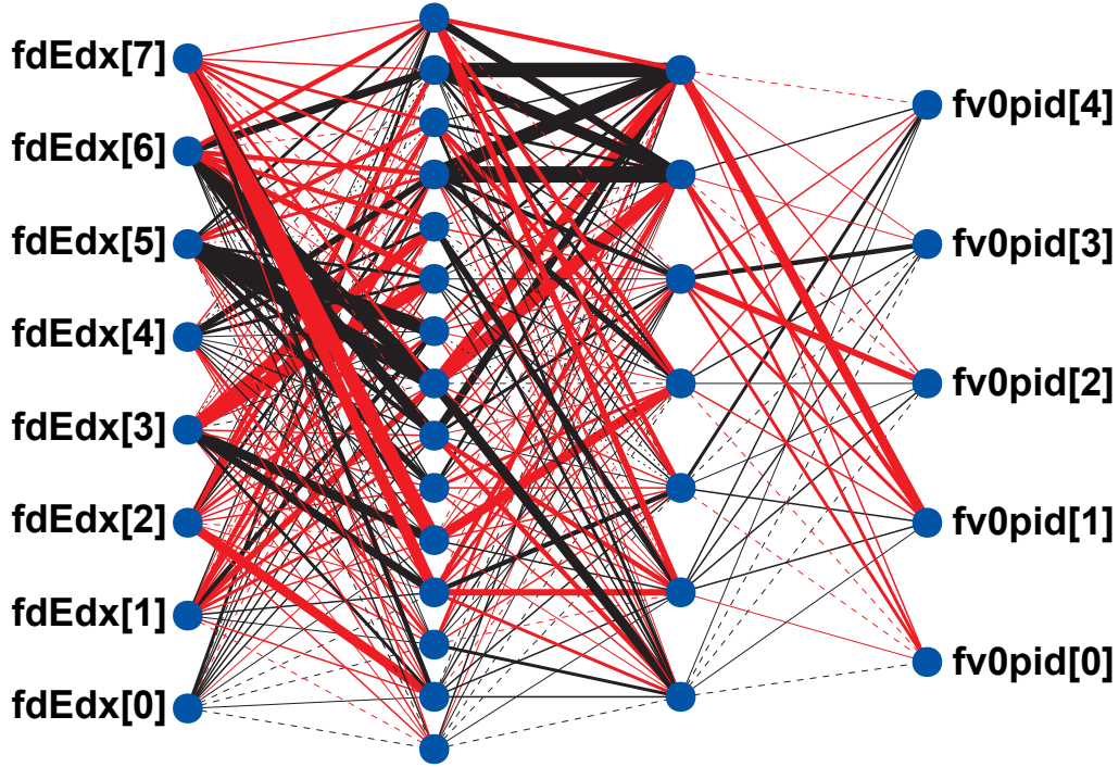
Figure 6.11: Reference network as used in AliRoot v4-17-Rev12 for Layer 1 and particles of 2 GeV/c. The input layer has eight input neurons, corresponding to the eight deposited charges which are presented to the neural network. The output layer has five output neurons, one for each particle type that is taken into account. The particle types are from the bottom neuron to the top neuron electron, muon, pion, kaon and proton. The network has two hidden layers with fifteen and seven neurons respectively. The thickness of the connecting synapses represents the absolute value of the weight that is assigned to the connection. Synapses with a positive weight are shown in black, that with a negative weight in red.
