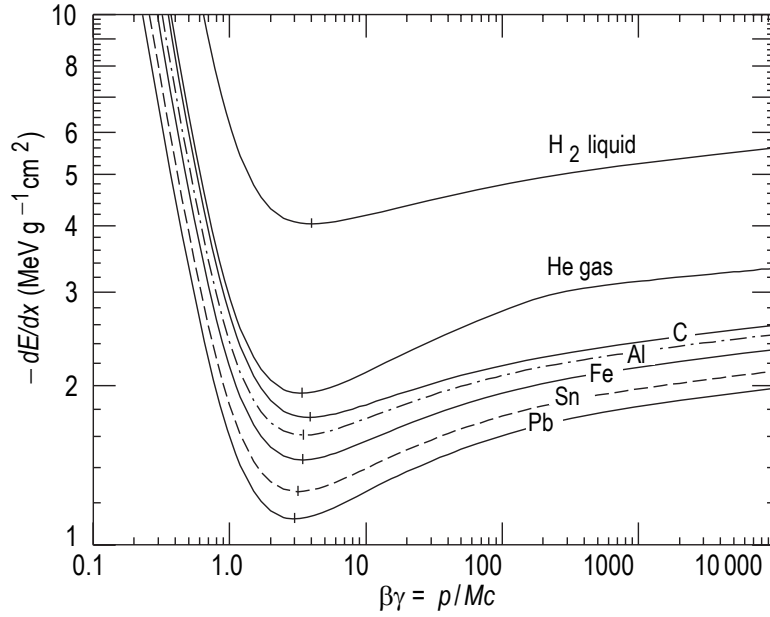
Figure 4.4: Calculated mean energy loss of pions in different materials. Taken into account is only the energy loss by ionization. The curve follows the Bethe-Bloch Formula [Ams08].
