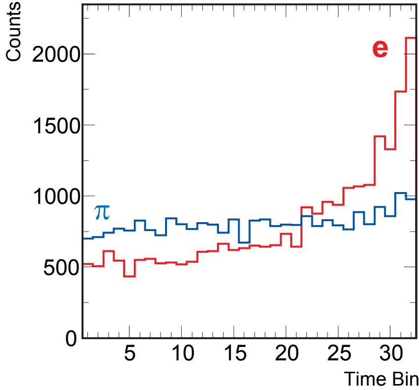
Figure 6.7: Time bin with the largest amount of charge for electrons (red) and pions (blue) in the drift region. The momentum was 1 GeV/c [And01].
