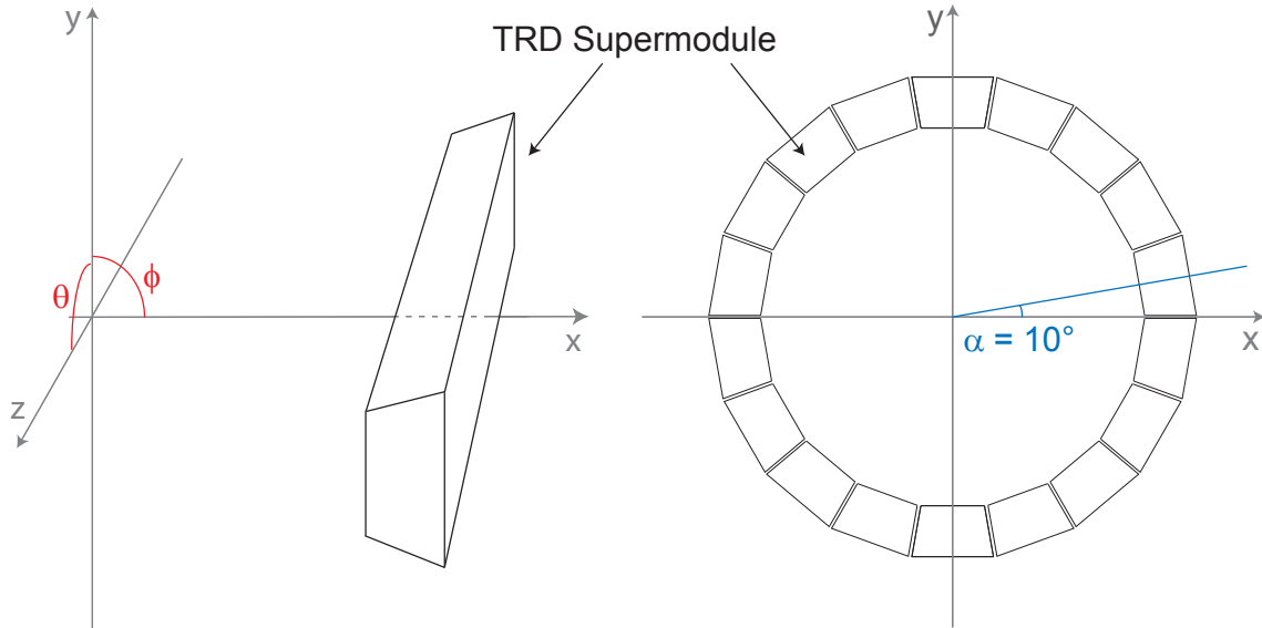
Figure 4.20: Local coordinates of a TRD supermodule. The z axis and the origin are identical to the global coordinate system in ALICE. Local x and local y can be transformed to the global variables by rotation using the angle \alpha .
