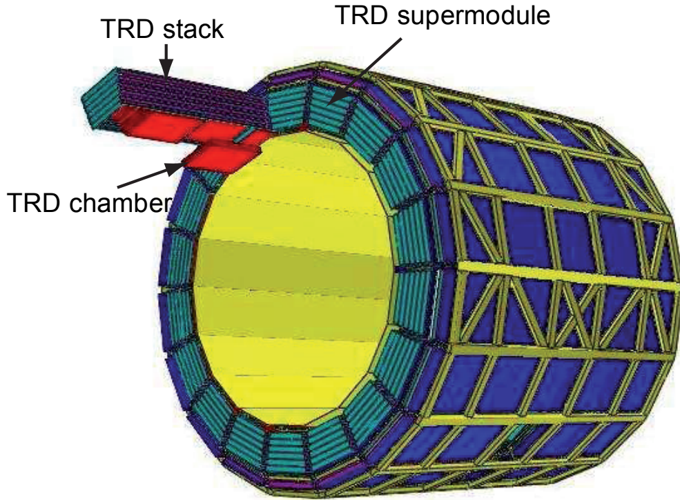
Figure 4.10: The ALICE Transition Radiation Detector [Aam08]. The barrel designed TRD consists of 18 supermodules, which are positioned around the collision point, parallel to the beam axis. Each supermodule is made of 30 single chambers which are arranged in 5 stacks with 6 layers each.
