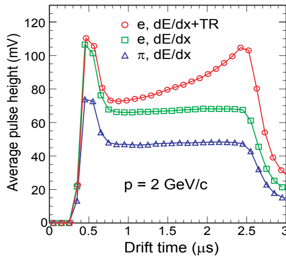
Figure 6.1: The average pulse height in the Transition Radiation Detector for electrons (with and without transition radiation) and pions [Aam08].
