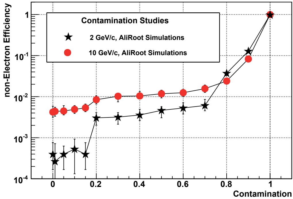
Figure 8.11: Non-electron efficiency versus level of contamination for 2 GeV (black stars) and 10 GeV/c (red dots) particles. For details please refer to the text.
