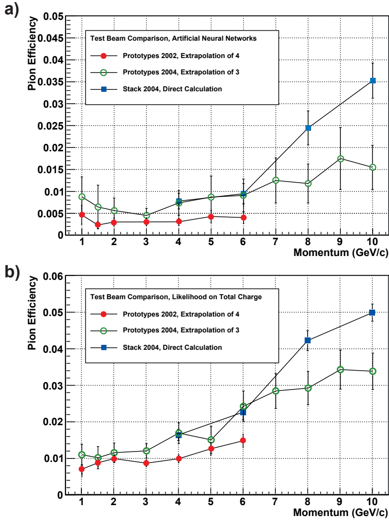
Figure 7.25: Pion efficiencies of the different beam times for neural networks (a) and likelihood on total deposited charge (b).
