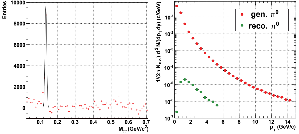
Figure 4.3: Left: Invariant mass spectrum of diphotons after background subtraction extracted with the inner barrel detectors [Mar08]. A clear peak can be seen at the invariant mass of the \pi^0 ( m \approx 135 \text{ MeV}/c^2 ). Right: Comparison of the \pi^0 yield of the inner barrel to the expected total yield. Plotted is the yield per pp event versus the transverse momentum of the neutral pion [Mar08].
