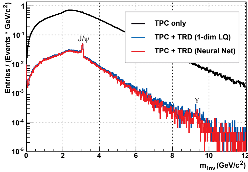
Figure 9.15: Invariant mass spectra of dielectrons in the ALICE central barrel using fast simulations. The spectra are normalized to one event and a bin width of 1 \text{ GeV}/c^2 . The spectrum is shown in case only the TPC is taken into account for electron identification (black line) as well as the spectra for a combined TPC and TRD electron identification. For the TRD PID two different methods were applied, likelihood on total charge (blue line) and neural networks (red line). In case only the TPC is used the electron efficiency is 90%, in case the TRD is taken also into account it is reduced to 81%. A clear peak can be seen at the invariant mass of the J/\psi and an enhancement in the \Upsilon region when the TRD PID information is taken into account.
