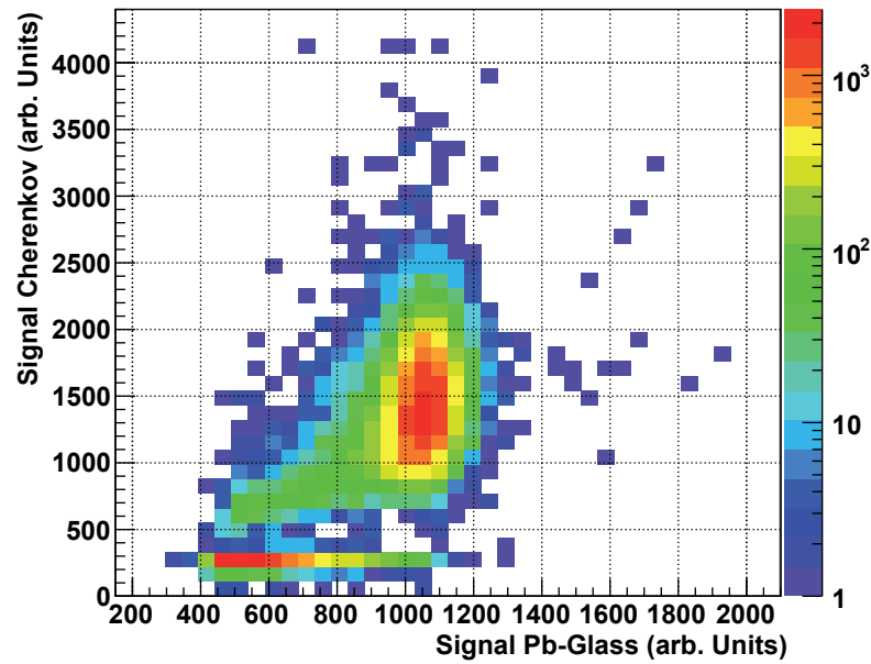
Figure 7.20: Correlation plot for Pb-glass and Cherenkov detector for 2 GeV/c data. Contrary to the correlation plots of 2002's beam time (Figure 7.3), a fraction of particles with a high Cherenkov signal but small energy deposition in the Pb-glass can be seen.
