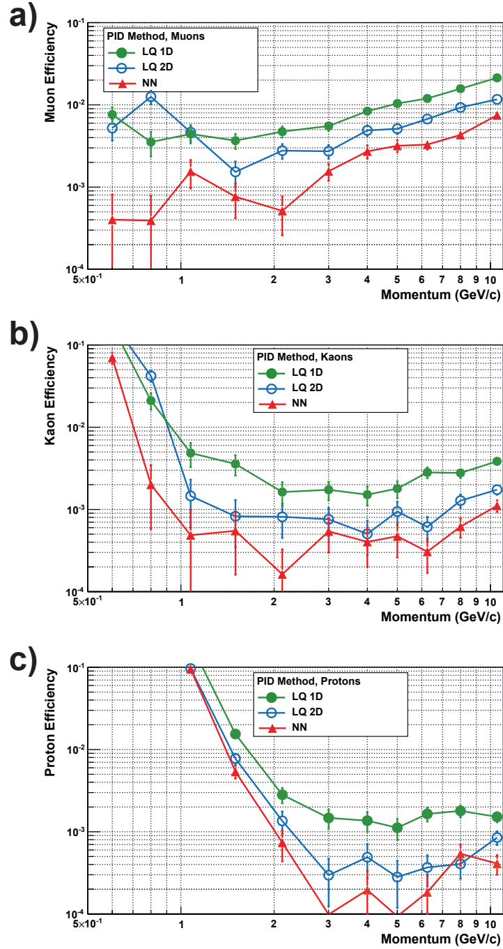
Figure 8.6: a) Muon efficiency, b) kaon efficiency, and c) proton efficiency at 90% electron efficiency versus momentum for neural networks, 1-dim likelihood and 2-dim likelihood.
