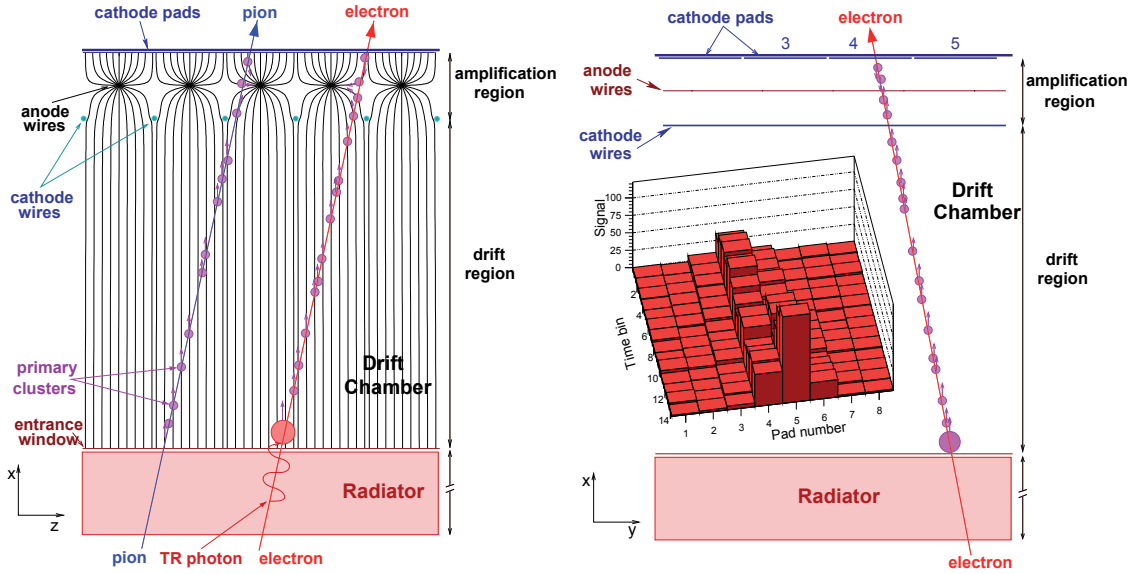
Figure 4.11: The working principle of the ALICE Transition Radiation Detector [Aam08]. A particle that traverses the TRD ionizes the chamber gas. The resulting electron clusters drift to the amplification region. In the amplification region the clusters are accelerated to the anode wires and avalanches are formed out. The avalanches induce charges on the pads which are read out. In case the Lorentz factor of a particle is large enough a transition radiation photon is generated inside of the radiator. This photon is absorbed early in the chamber gas and contributes to the signal.
