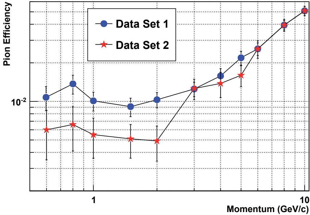
Figure 9.9: Pion efficiency using the look-up tables versus momentum. In each momentum bin results for two data sets are shown. In case of a momentum of 3 GeV/c, data set 1 corresponds to the training set and data set 2 to the validation set.
