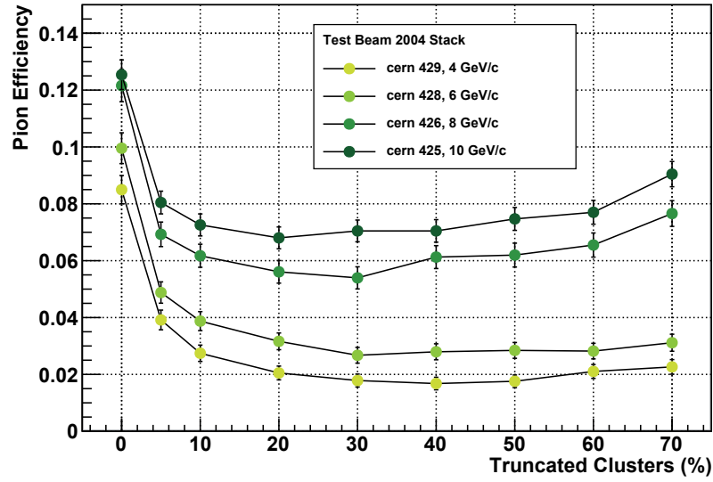
Figure 7.12: Pion efficiency versus rate of truncated clusters for 4, 6, 8, and 10 GeV/c. For all measurement the 5% smallest clusters were rejected. A minimum of pion efficiency is reached if about 30-40% of the largest clusters are truncated.
