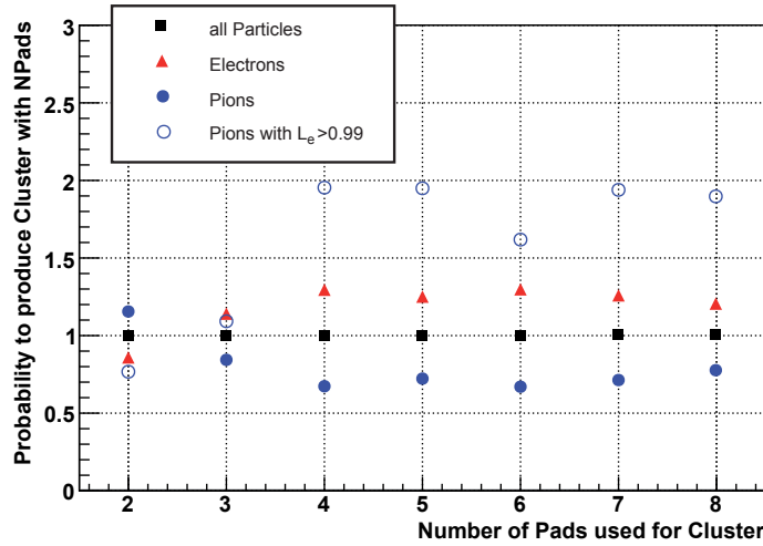
Figure 7.24: Relative probability of occurrence of different cluster sizes for different particle classes. For details please refer to the text.
