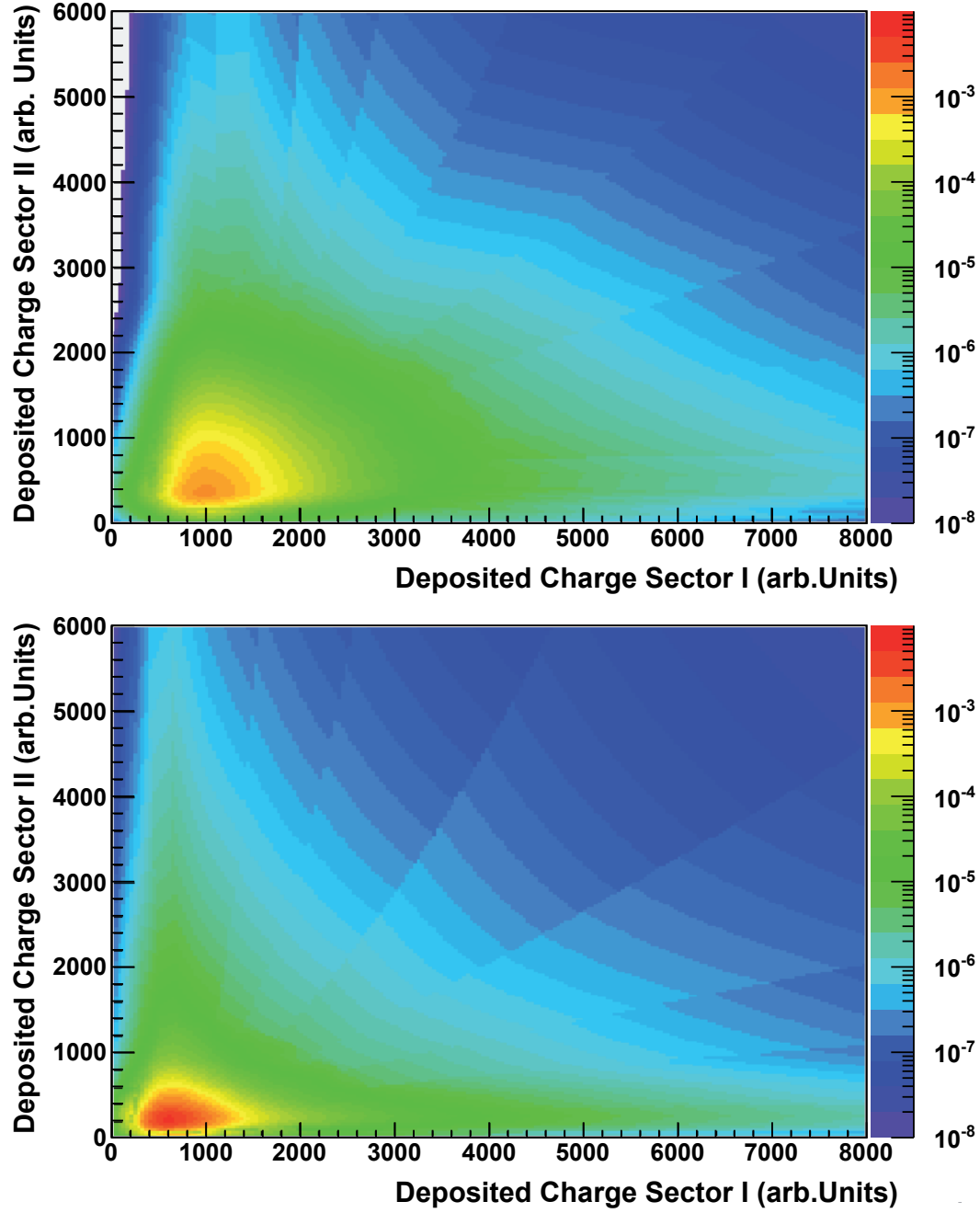
Figure 6.9: Two-dimensional reference histograms for electrons (upper plot) and pions (lower plot) as used in AliRoot (v4-17-Rev-12) for particles with a momentum of 2 \text{ GeV}/c . On the x axis the deposited charge of sector I is plotted, on the y axis that of sector II. It can be seen that the pion distribution is much narrower than the electron distribution, especially in direction of sector II.
