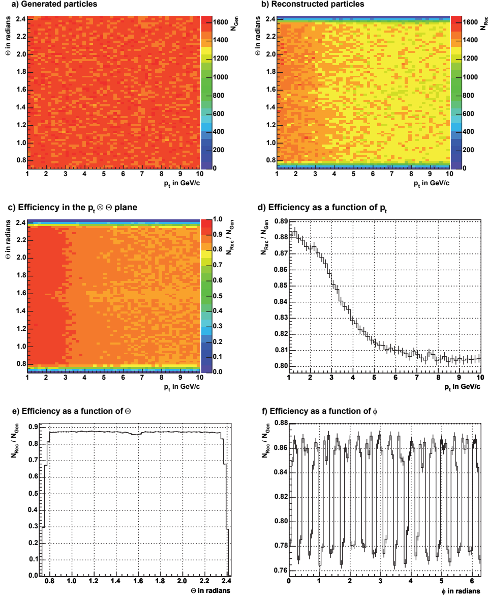
Figure 9.12: Efficiency response functions for the central barrel [GO05]. a) shows the number of simulated particles in the p_T - \theta plane. In b) the number of reconstructed particles and in c) the reconstruction efficiency is presented. In addition the efficiency as a function of d) p_T , e) \theta , and f) \phi is plotted. The small drop around \theta \approx 1.6 is caused by absorption or diversion at the central TPC electrode [TPC00]. The 18 drops for the efficiency as a function of \phi originate from the dead areas of the TPC, the ALICE support structures and the borders between the TRD supermodules.
