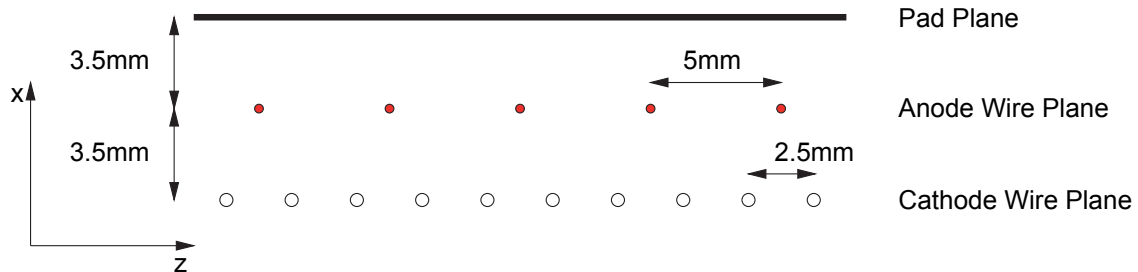
Figure 4.12: Wire geometry of a readout chamber of the Transition Radiation Detector [TRD01].
