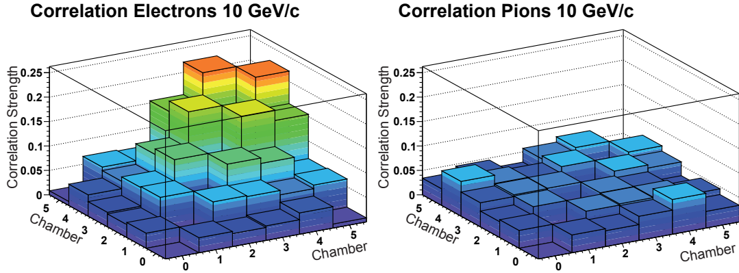
Figure 7.18: Correlation matrix for particles with momenta of 10 GeV/c. The strength of correlation is represented by the color. For electrons correlations between the last chambers are visible, for pions the correlations are smaller. The diagonal representing correlations of the same chambers is suppressed since it is always unity.
