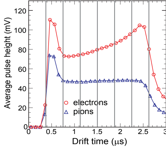
Figure 6.10: Illustration of the input for the artificial neural networks using the deposited charge in eight slices of a TRD module. Analogous to the two-dimensional likelihood method on deposited charge the chamber is divided into several slices.
