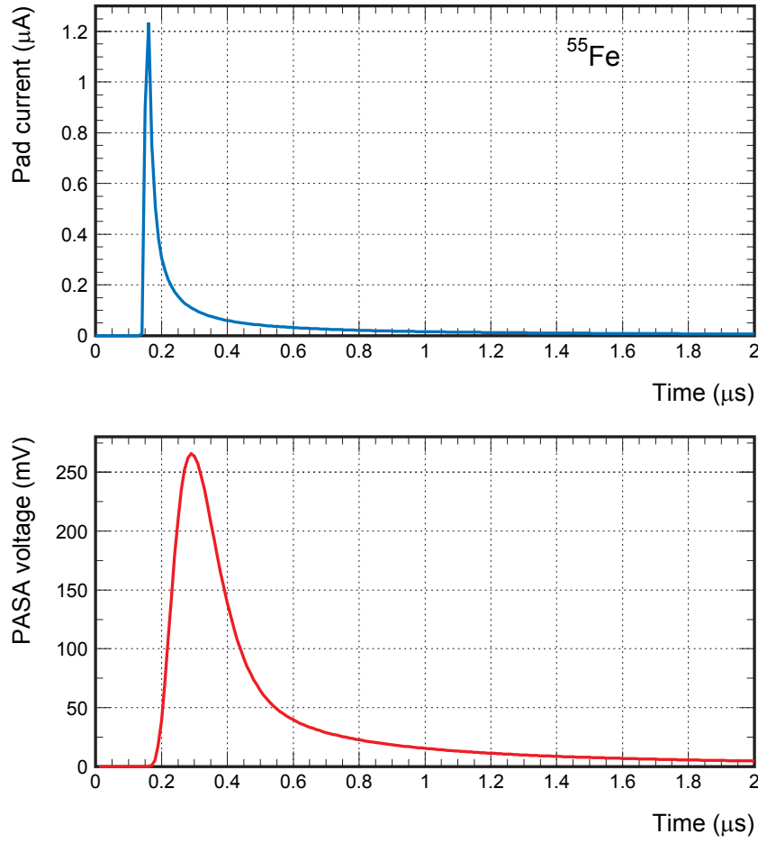
Figure 4.18: The current induced on the readout pads (upper plot) and the electronic response (lower plot), which is the Time Response Function [TRD01].
