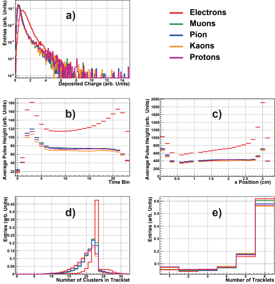
Figure 8.2: Monitoring plots of the AliTRDcheckPID task. The plots are shown for electrons (red), muons (green), pions (blue), kaons (orange), and protons (purple) with a momentum of 2 GeV/c. The plots are a) the deposited charge per tracklet, b) average pulse height versus time bin, c) corrected average pulse height versus x position, d) number of clusters per tracklet, and e) number of tracklets per track.
