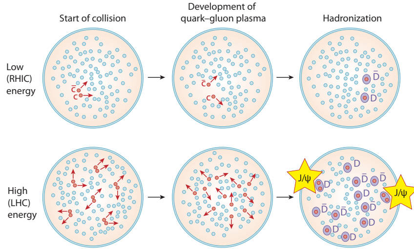
Figure 2.11: The mechanisms of charmonium suppression and enhancement in a quark-gluon plasma. In the upper case (low energy) only small numbers of charm-anticharm pairs (red dots) are produced. The interaction of these two quarks is screened by the other quarks and the gluons of the QGP. In the hadronization phase the charm and the anticharm quark will each form a D meson together with another (light) quark (gray dot) of the medium and the number of observed J/\psi s will be smaller than expected. With increasing collision energy (lower scenario) many more charm-anticharm pairs will be produced. As in the low energy case the medium screens the quark antiquark-pairs from each other, but here, charm and anticharm quarks from different original pairs could form J/\psi s and lead to a higher number of produced charmonia [BM07].
