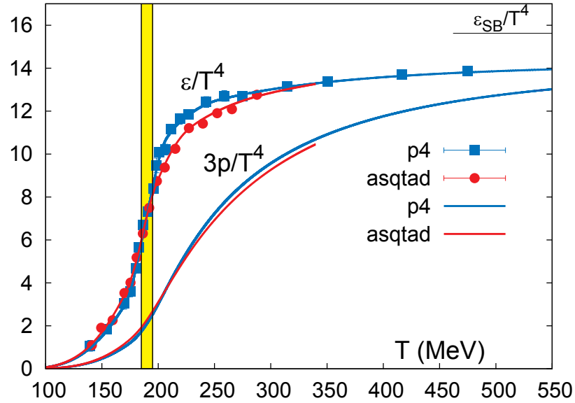
Figure 2.1: Results of lattice QCD calculations for energy density \epsilon/T^4 and pressure 3p/T^4 [Baz09]. The energy density and the pressure are calculated for three quark flavors (two degenerated light quarks and one heavy quark) for two different theoretical models. The Stefan-Boltzmann limit for an ideal gas is also shown. The yellow band indicates a phase transition at a temperature region of 185 < T < 195 MeV.
