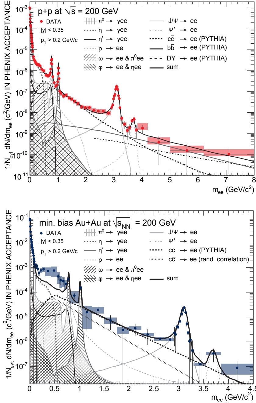
Figure 2.8: Dileptonic signal from Phenix for pp (upper plot) [Ada09b] and AuAu (lower plot) [Afa07]. The spectra are compared to the yield expected from the different contributions. While the data from proton collisions fit well to the model, the extracted signal from heavy ion events shows a significant excess at low dielectron masses over the expectations.
