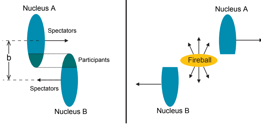
Figure 2.3: Schematic view of the participant-spectator model. The centrality of a collision is described by the impact parameter b . The nucleons in the overlapping regions of the two nuclei are the participants and form the fireball. The particles outside of the overlap are the spectators, they are affected only with comprehensively small excitation energies by the collision. This plot is adapted from Reference [KB04b].
