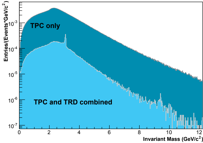
Figure 4.2: Dielectron mass spectrum with the ALICE central detectors [Som08]. Shown is the expected yield for 10^7 central PbPb collisions. The darker area represents the yield of dielectron pairs if the PID information is extracted by the TPC only. With the TRD (lighter area) peaks at the masses of the J/\psi , Y and Y' are visible. This study was done using a parameterization for fast simulations [GO05]. Here, a constant pion efficiency of 1% for the TRD is assumed for all momenta.
