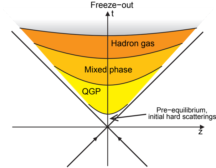
Figure 2.5: Space-time evolution of a central ultrarelativistic heavy-ion collision. After a non-equilibrated phase with initial hard collisions, the system thermalizes and a quark-gluon plasma is formed. With increasing time the system expands and therefore cools. The fireball is transformed to a phase where regions of quark-gluon plasma and hadron gas exist in parallel. Finally the hadronization takes place and the system freezes out. This plot is adapted from Reference [KB04a].
