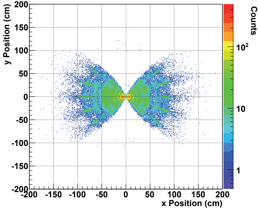
Figure 9.3: Conversions in ALICE for 32 million pp collisions at 10 TeV/c [Hei09]. All conversion points are shown where at least one track can be reconstructed in the Transition Radiation Detector. In this simulation eight TRD Supermodules were active. Since photon conversions occur preferably in material with a high nuclear charge Z , the layers of the ALICE Inner Tracking System as well as the inner part of the Time Projection Chamber can be seen.
