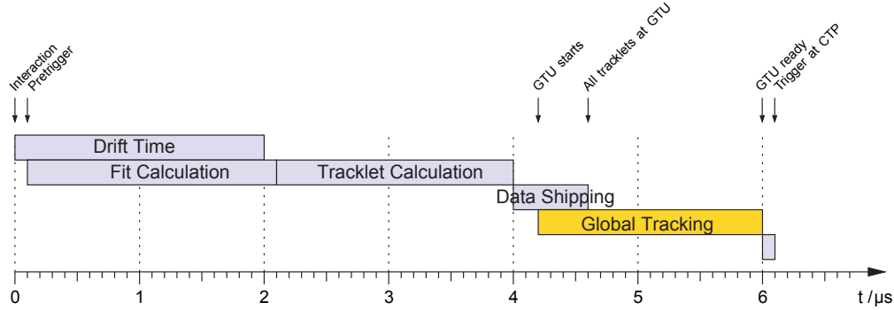
Figure 9.5: Trigger timing for the TRD [dC03].
