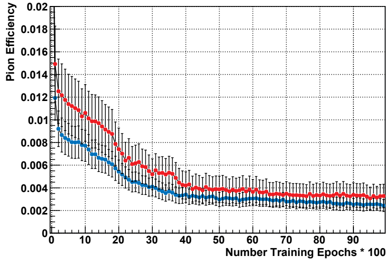
Figure 7.8: Development of pion efficiency versus number of training epochs for 2 GeV/c data. Results achieved with training data are shown in blue, results of validation data are shown in red.
