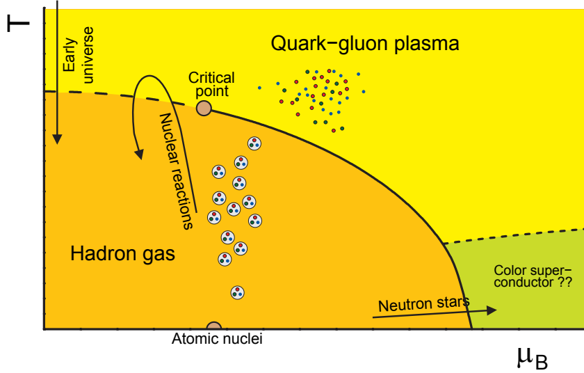
Figure 2.2: A schematic illustration of the phase diagram of strongly interacting matter. Shown are the states of matter as a function of temperature T and baryochemical potential \mu_B . In the orange area quarks and gluons are confined to hadrons, the brown dot at zero temperature represents matter in atomic nuclei. In case the temperature and the baryochemical potential is high enough an other state of matter is formed, the quark-gluon plasma. The solid line represents a first order phase transition, while the dashed line between hadron gas and QGP indicates a crossover transition. The brown dot between the solid and the dashed line stands for the critical endpoint. The green area is a color superconducting phase that is predicted at low temperature but high \mu_B . This plot is adapted from Reference [KB04b].
