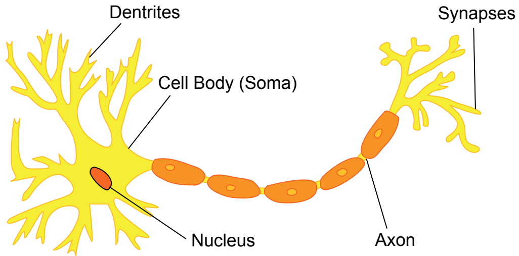
Figure 5.1: Schematic view of a biological neuron. A neuron consists of a cell body including a nucleus (soma), dendrites, an axon, and synapses. The plot is adapted from Reference [Wik10]
