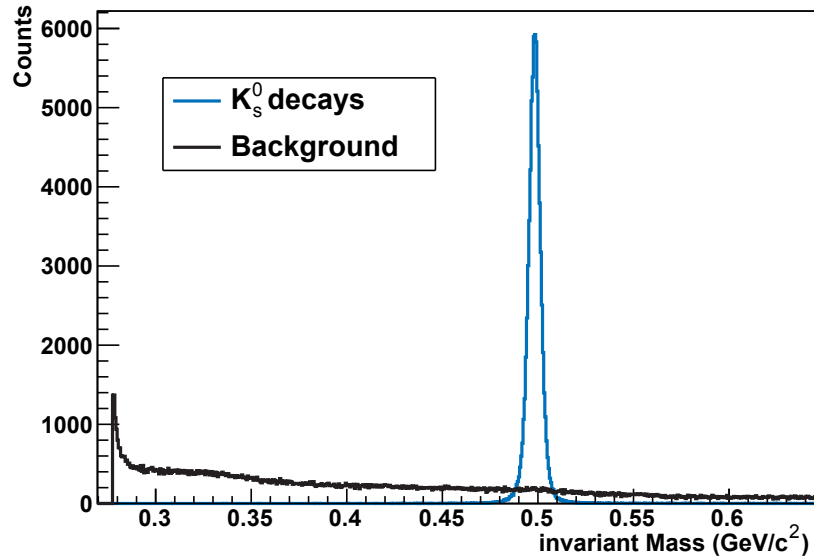
Figure 9.2: Invariant mass of neutral kaons (blue) and background (black) as provided by the ALICE reconstruction V^0 finder [Hei09].
