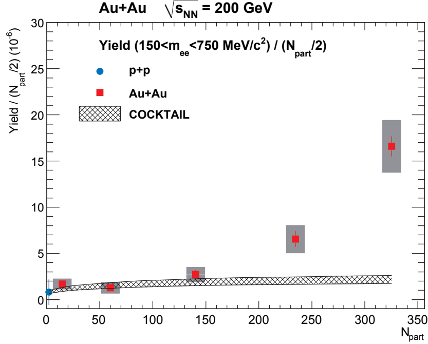
Figure 2.9: Dielectron yield per participating nucleon pair ( N_{part}/2 ) as a function of N_{part} for the invariant mass range 0.15 < m_{inv} < 0.75 \text{ GeV}/c^2 measured by PHENIX [Ada09a]. The yield is compared to the expected dielectron yield from hadron decays (patterned region). It can be seen that the measured yield shows a large excess over the expectations in central collisions.
