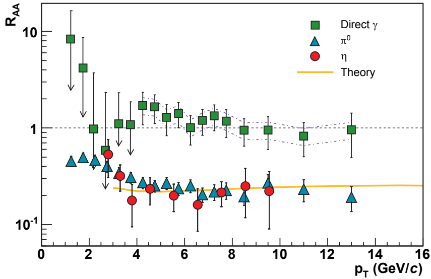
Figure 2.15: Jet quenching at PHENIX for \sqrt{s_{NN}} = 200 GeV [Adl06]. Shown is the suppression of high p_T \pi^0 s and \eta s in AuAu collisions compared to pp events. As predicted for a QGP formation the number of hadrons is smaller than for the non-QGP case. Particles which do not interact strongly as directly produced photons should not be suppressed. The results agree well with the predictions for a quark-gluon plasma formation.
