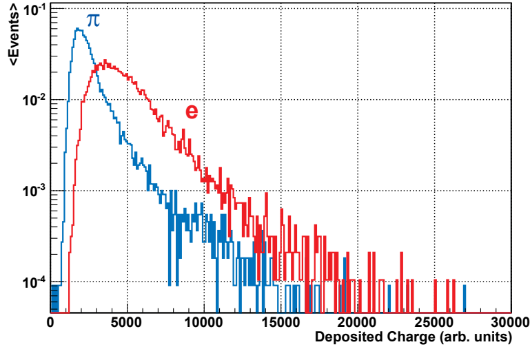
Figure 7.5: Total deposited charge for particles with a momentum of 2 GeV/c. Electrons are shown in red, pions in blue.
