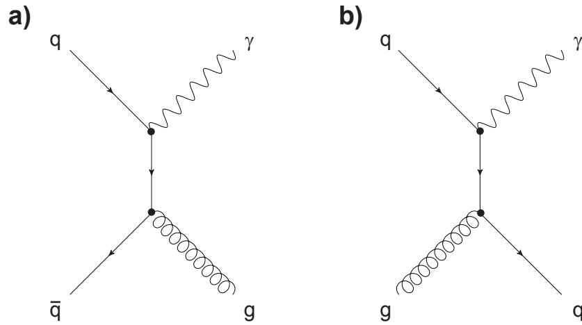
Figure 2.13: Feynman graphs of the main contributions to direct photons: a) quark-antiquark annihilation and b) quark-gluon Compton scattering.
