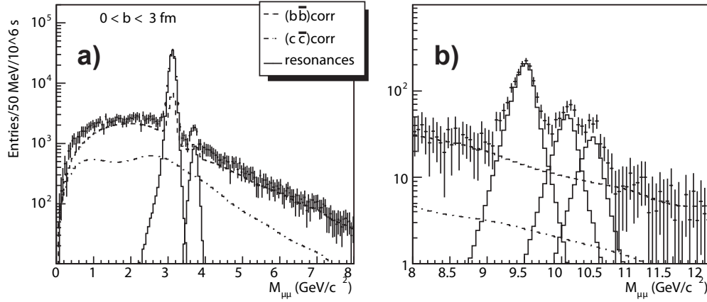
Figure 3.6: The expected invariant mass spectra for one heavy-ion running year of ALICE (about 2 \cdot 10^8 collisions at \sqrt{s_{NN}} = 5.5 TeV) obtained with the muon spectrometer a) in the J/\psi and b) the \Upsilon mass region [Ale06].
