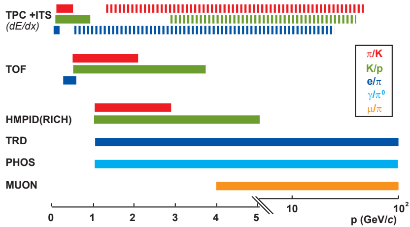
Figure 3.5: Particle identification performance of the ALICE detectors. This plot is based on values presented in Reference [Car04] and is adapted from Reference [Sch04].
