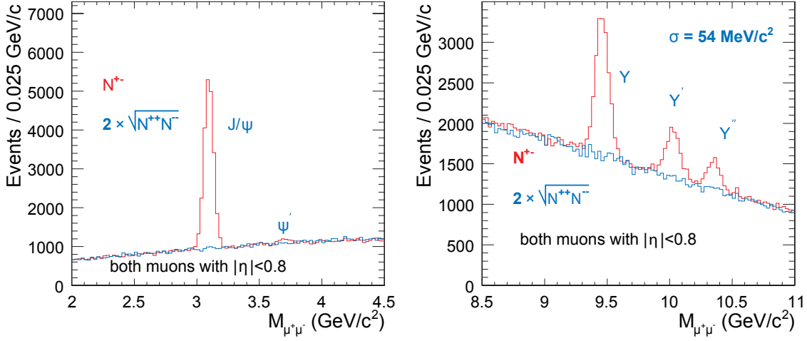
Figure 9.11: Simulated invariant mass spectra of muon pairs in the J/\psi (left) and the \Upsilon region (right) for 5.5 TeV PbPb collisions extracted with the central barrel of CMS ( |\eta| < 0.8 ). Blue are reconstructed masses with like-sign and red are opposite-sign muon pairs. This distribution is expected after one month of data taking. The simulations were done assuming a multiplicity of 5,000 charged particles per pseudo-rapidity unit and no quarkonia suppression [Bed07].
