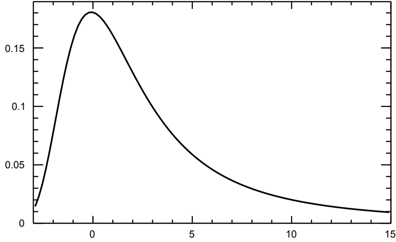
Figure 4.5: Schematic illustration of the Landau distribution.
