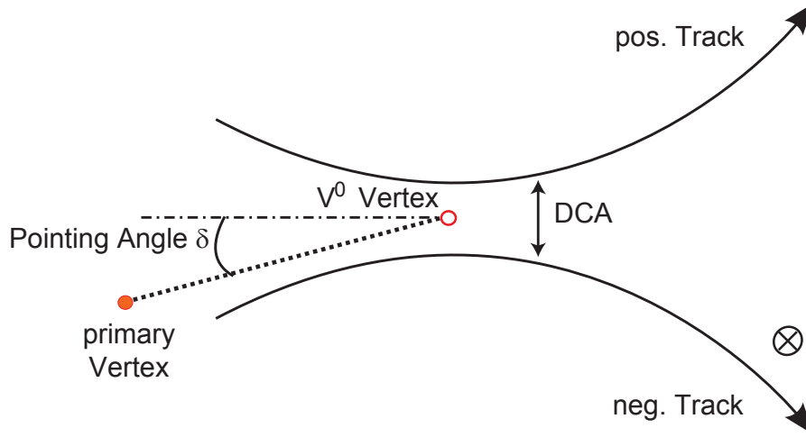
Figure 9.1: Topology of a displaced vertex [Kal08]. A neutral particle does not produce a track in the tracking detectors. In case the uncharged particle decays into a positively and a negatively charged particle, two tracks can be reconstructed. Due to the magnetic field, the tracks are bent in different directions. The reconstructed vertex of the neutral particle decay is the V^0 vertex. Further attributes of a displaced vertex are the Distance of Closest Approach (DCA) between the two reconstructed tracks and the pointing angle \delta . The pointing angle is the angle between the reconstructed momentum of the neutral particle and a straight line between the V^0 vertex and the collision point.
