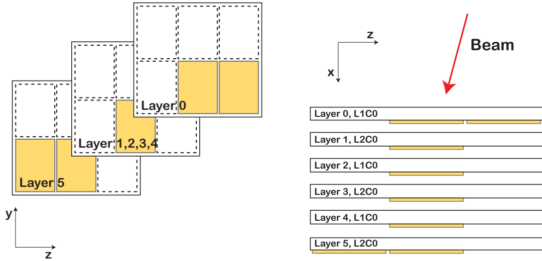
Figure 7.11: Position of the eight readout boards on the different TRD modules. The boards were arranged such that a maximum of possible angles could be measured. The stack consists of two different chambers types (L1C0 and L2C0).
