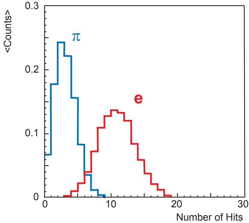
Figure 6.5: Performance of the cluster counting method in the ATLAS Transition Radiation Tracker using an energy threshold of 6 keV [Ake98]. The distribution for electrons is red, that for pions blue. It can be seen that with this method electrons and pions can be well discriminated.
