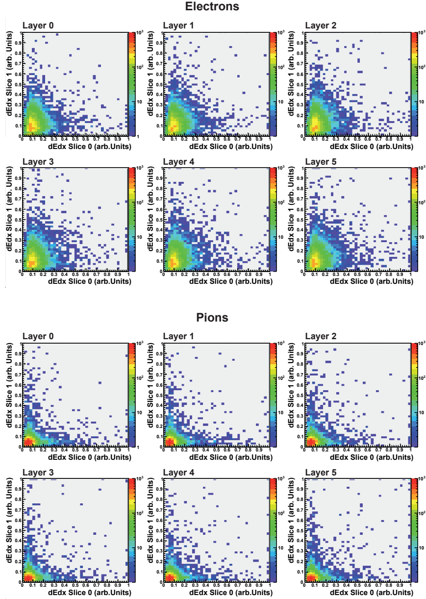
Figure 9.7: Distribution of the deposited charges Q_0 and Q_1 for all six TRD layers. The correlation plots are shown for electrons and pions separately.
