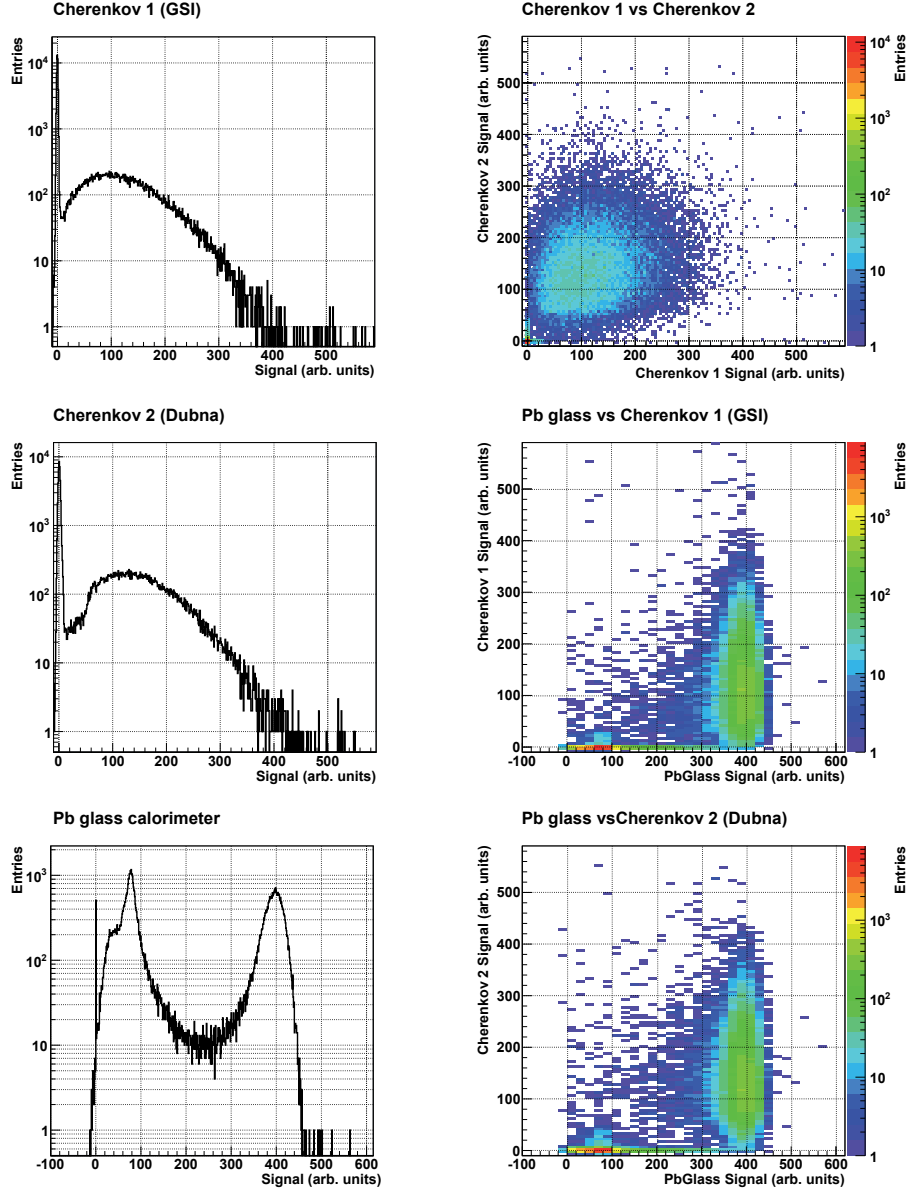
Figure 7.3: The independent particle identification. The detector responses for 2 GeV/c test beam data of 2002 are shown. Pions are expected to produce a signal at zero in the Cherenkov detectors and in addition a smaller signal than electrons in the Pb-glass calorimeter. On the left side the responses of the single detectors are shown. On the right side the correlation plots each with two detectors. In order to be tagged as an electron or a pion, a particle has to pass cuts on all three detectors.
