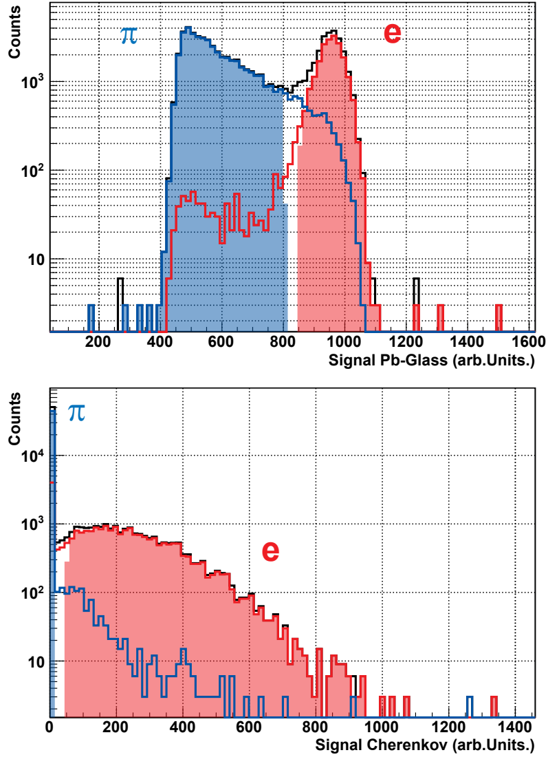
Figure 7.17: Pb-glass (upper plot) and Cherenkov (lower plot) for a run with a nominal momentum of 6 GeV/c. The black line represents all entries, the red and blue areas show the particles tagged as electrons and pions, respectively. The red and blue lines stand for the electrons and pions that are identified by the other PID detector.
