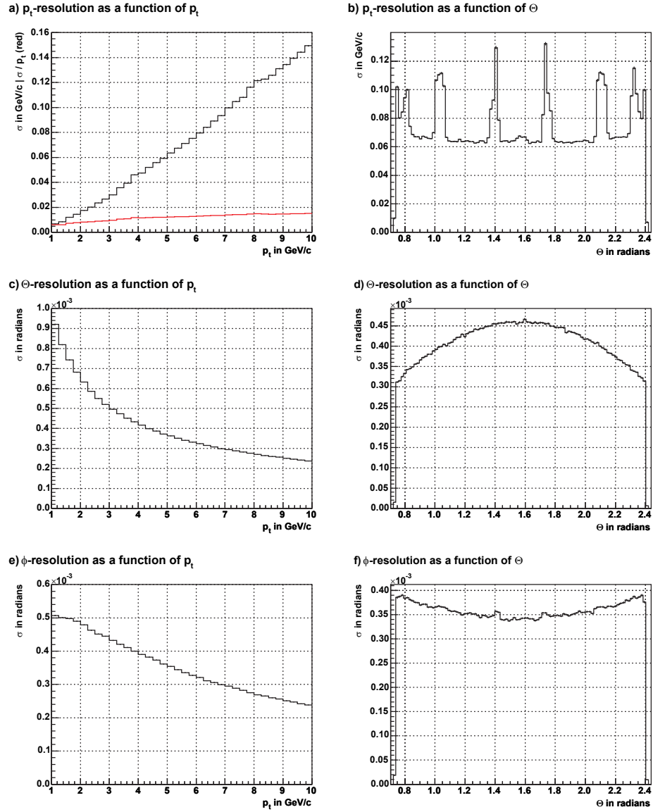
Figure 9.13: Resolution response functions for the central barrel [GO05]. The resolutions in a-b) p_T , c-d) \theta , and e-f) \phi as a function of p_T and \theta are shown. The red line in a) represents the relative resolution p_T ( \sigma/p_T ). It can be seen that for the p_T resolution as a function of \theta the resolution is worse in case no TRD information is available.
