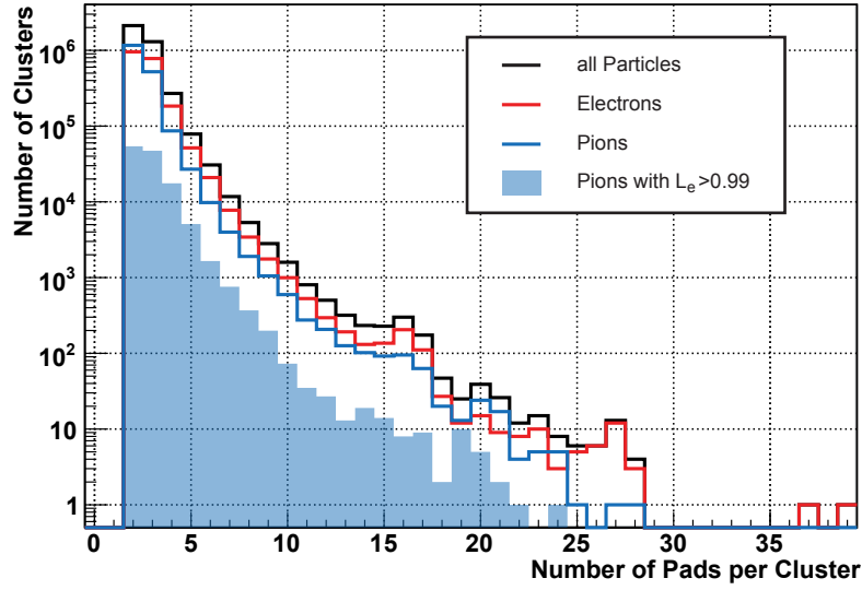
Figure 7.23: Number of Pads used for a cluster. Shown is the total amount of clusters with different size for all particles (black line), electrons (red line), pions (blue line), and fake pions (blue area).
