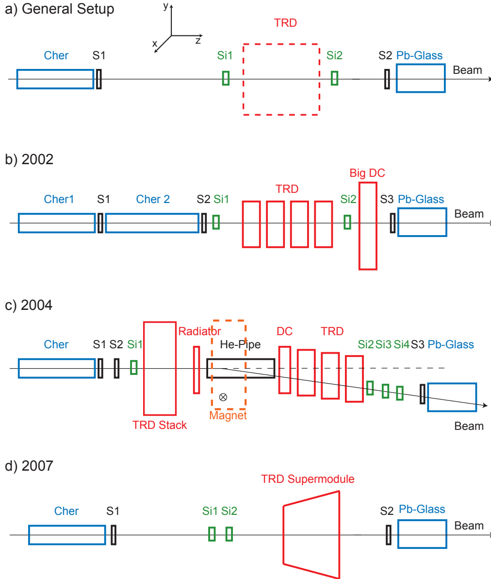
Figure 7.1: Setup of the test beam times [And]. a) The general concept of the setup consisted of two scintillators (S1, S2) working as beam trigger, two silicon strip detectors (Si1, Si2) for beam position monitoring, a Cherenkov threshold counter (Cher) and a lead glass calorimeter (Pb-Glass) for independent particle identification, and finally the Transition Radiation Detector units (TRD). The coordinate system is defined in the following way: x is perpendicular to the beam axis in horizontal direction, y perpendicular to the beam axis and perpendicular to the x axis, and z is parallel to the direction of the particle beam. The setups for the different test beam times ( b ): 2002, ( c ): 2004, and ( d ): 2007) differed in some aspects from the general concept. The details can be found in the dedicated Sections 7.2.1, 7.3.1, and 7.5.1.
