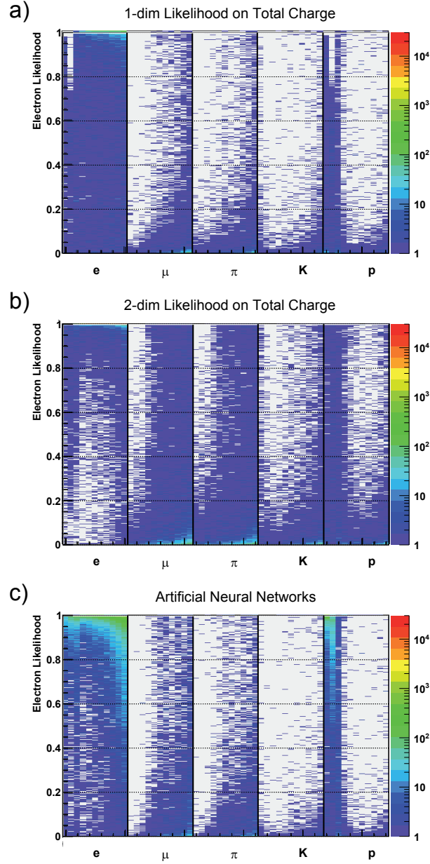
Figure 8.3: Likelihood to be an electron for a) one-dimensional likelihood (LQ), b) two-dimensional likelihood (2-dim LQ), and c) artificial neural networks. The likelihood is plotted versus different particle classes. A particle class is given by one of the eleven default momentum bins and the particle identity. The color represents the frequency of occurrence on a logarithmic scale. The missing entries for 1-dim likelihood for electron and protons at the second momentum bin (0.8 GeV/c) and high electron likelihood is caused by the fact that electrons and protons in this momentum region deposit the same amount of charge and therefore could not be well discriminated.
