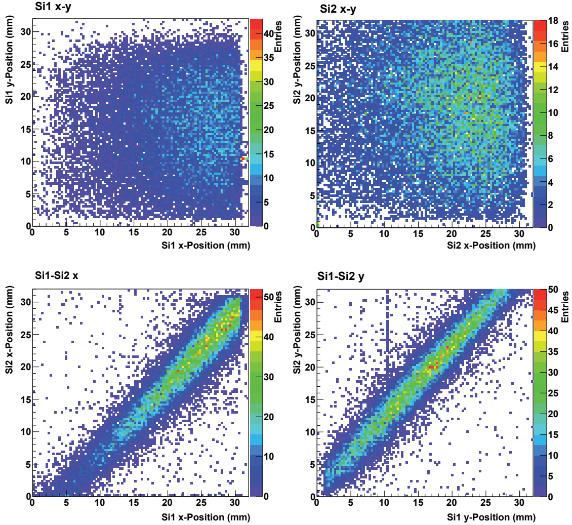
Figure 7.2: The upper plots show the signals of the two silicon strip detectors for 2 GeV/ c beam data from the test beam 2002, Si1 on the left side, Si2 on the right side. The beam profile is visible for both detectors, but they are not centrally hit. The lower plots show the respective correlation between the x position (left) and the y position (right). If both detectors would be perfectly aligned, the entries would lie exactly on a diagonal starting at the origin. It can be seen that the detectors are displaced by about 5 mm in x and about 2 mm in y direction with respect to each other.
