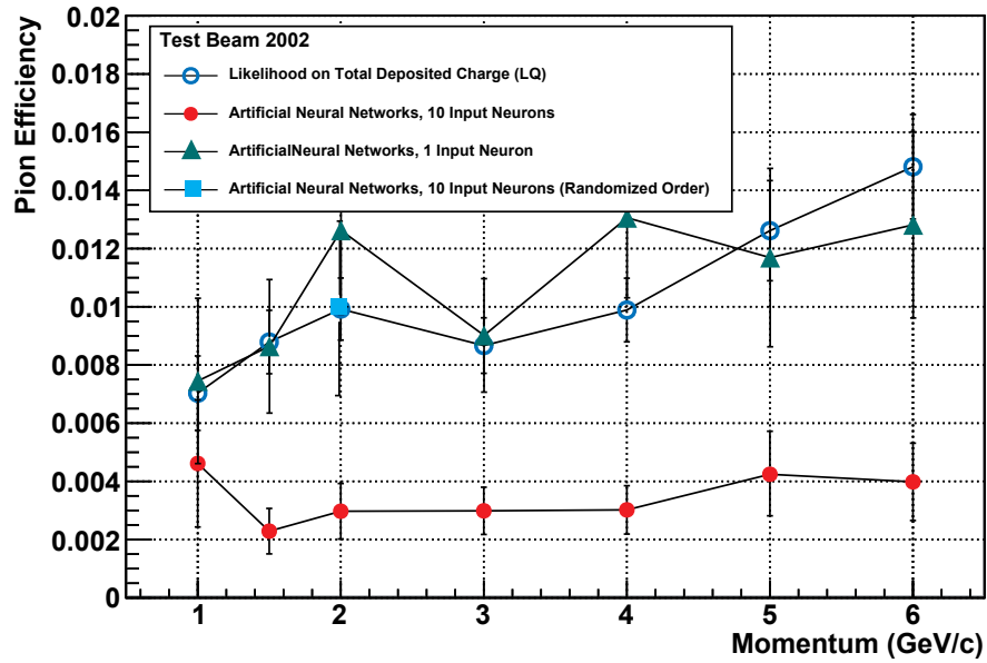
Figure 7.6: a): Pion efficiency (six chambers) at 90% electron efficiency versus number of input neurons for 2 GeV/c data. After a first rapid improvement, the pion efficiency converges. b): Pion efficiency (six chambers) versus momentum. Red dots represent the results of neural networks using 10 input neurons. The neural networks showed an improved pion efficiency by a factor of about three compared to likelihood on total deposited charge.
