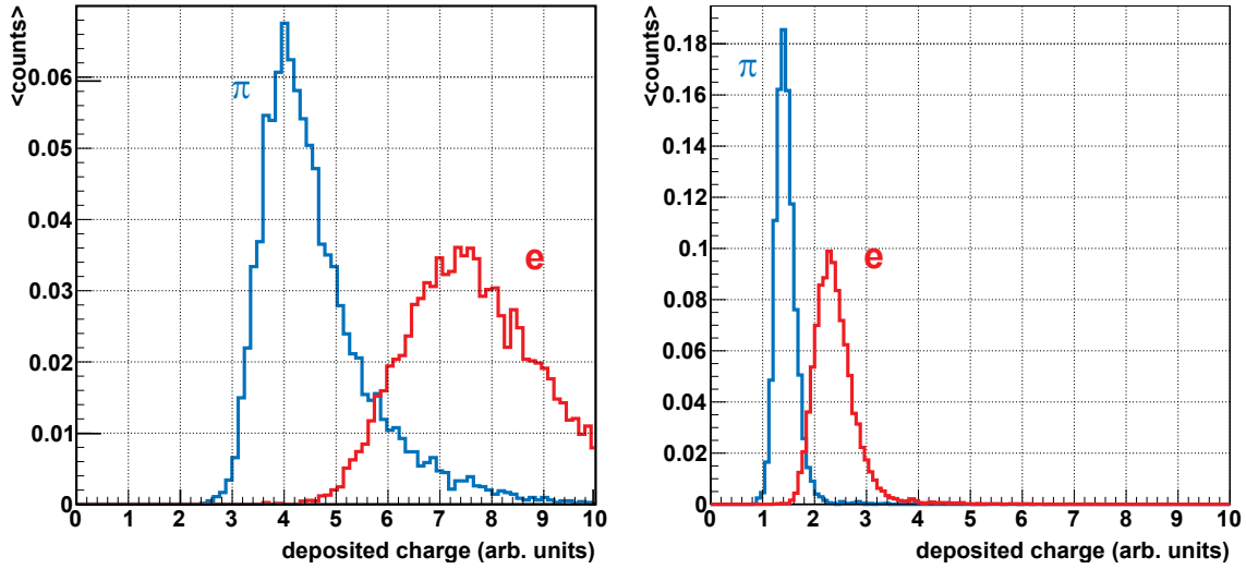
Figure 6.3: Truncated Mean for 4 GeV/c test beam data from 2004. On the left side the deposited charge integrated over all 6 Transition Radiation Detector layers for electrons (red) and pions (blue) are plotted. The pion signal has a long tail towards larger deposited charges. This leads to high contamination of identified electrons. If only the largest 60% of clusters with the smallest deposited charges are taken into account, the contamination decreases significantly.
