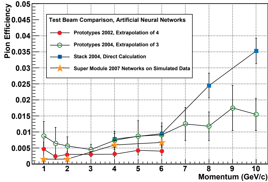
Figure 8.12: Pion efficiency from test beam analyses versus momentum for neural networks. Shown are the results obtained in 2002 (red dots), for prototypes obtained in 2004 (green circles), for a stack of real size chambers in 2004 (blue squares), and simulated data applied to networks trained with data taken in 2007. These results obtained with simulated data fit well with the other test beam pion efficiencies.
