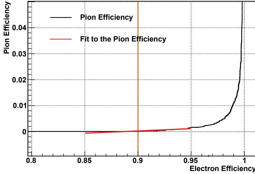
Figure 6.14: Pion efficiency versus electron efficiency for simulated data with a momentum 2\text{ GeV}/c . In order to estimate the error of the pion efficiency, the pion efficiency is plotted versus the electron efficiency. The derivative at 90% electron efficiency is estimated using a fit with a second order polynomial function (red line) and enters the error.
