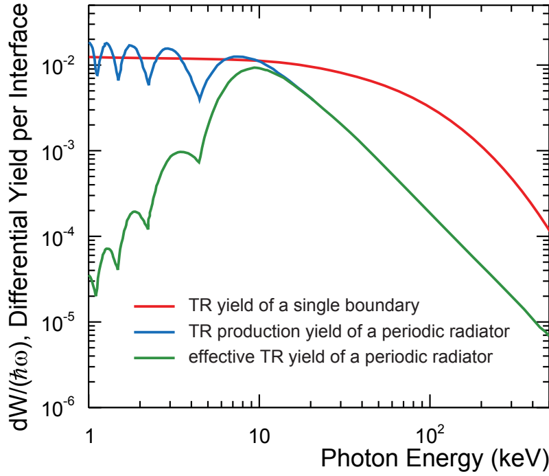
Figure 4.7: The differential yield per interface as a function of TR photon energy [Ego00]. In the case of a single boundary (plotted in red) at low photon energies the yield is constant and then decreases rapidly at higher energies. The photon production in a regular radiator (blue) fluctuates around the value of a single boundary at low energies due to interference effects. Caused by the finite thickness of the foils formation zone effects suppress the yield at higher energies. For a real radiator (green) the absorption of TR photons also plays a role at lower energies.
