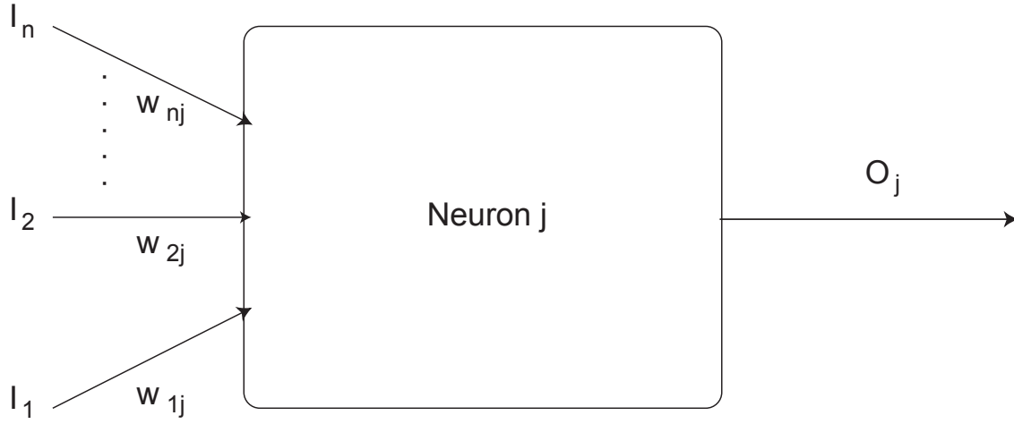
Figure 5.2: Schematic view of an artificial neuron. Input signals I_n are multiplied with associated weights w_{ij} and are transformed by an artificial neuron j into an output O_j .
