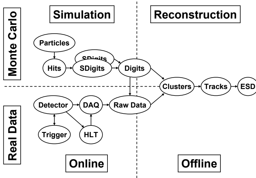
Figure 3.9: Interaction of the reconstruction code with other parts of AliRoot [Aam08]. The reconstruction processes raw data into Event Summary Data. In case of simulations it is also possible to directly use Digits for the reconstruction in order to save computing time.
