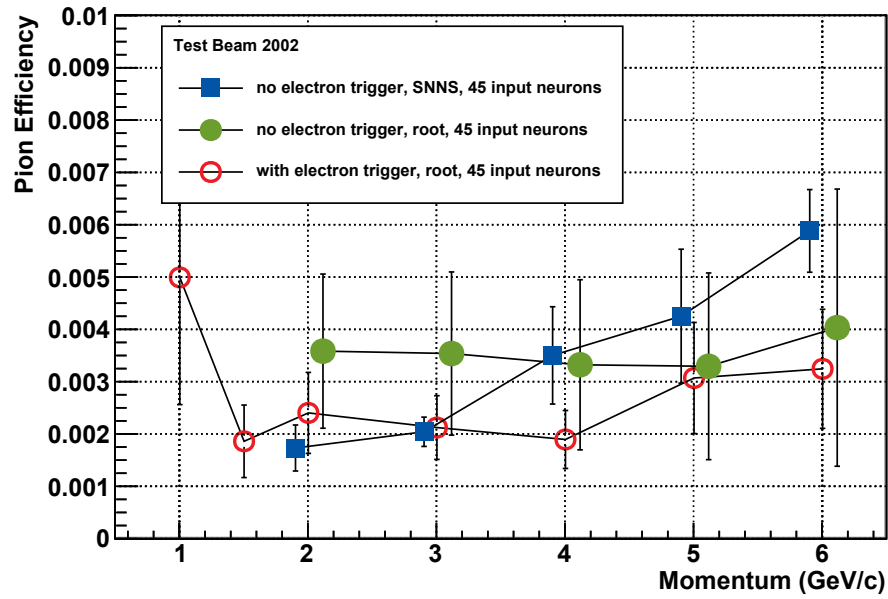
Figure 7.9: Comparison of different results. The results achieved with a different neural network software (SNNS, blue squares) and different validation data (green dots) are shown. They are compared to the results presented in Figure 7.6. In a) the pion efficiencies versus the number of input neurons are shown, in b) the pion efficiencies versus momentum.
