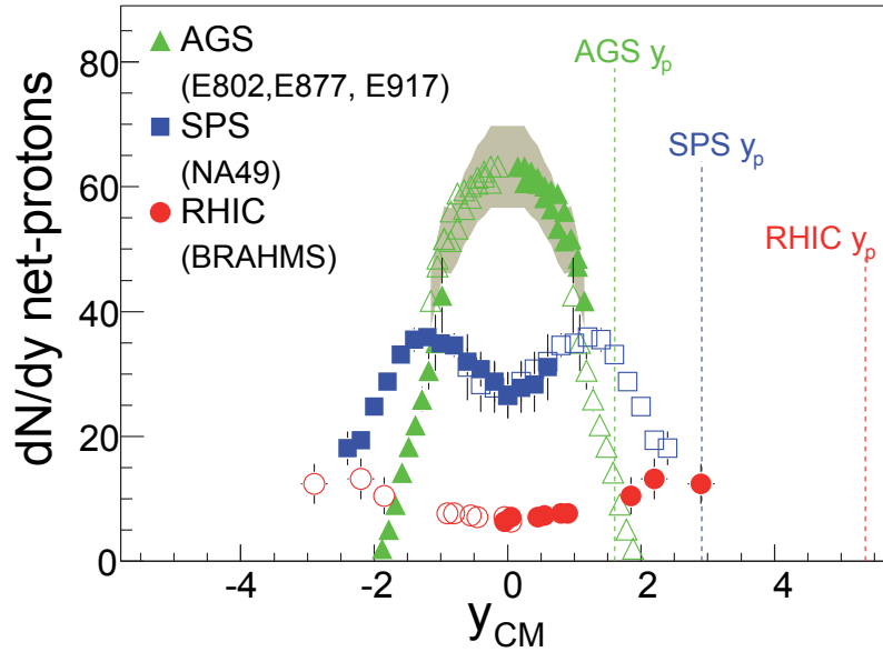
Figure 2.4: Comparison of net proton rapidity distributions for different center of mass energies [Bea04]. For AGS energies the distribution corresponds to the Landau model of nuclear collisions. For higher energies the distribution is better explained by the Bjørken-McLerran picture.
