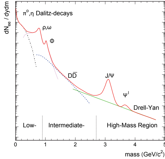
Figure 2.6: Schematic view of the expected invariant mass spectrum of dileptons and its sources in heavy ion collisions [Rap00].
