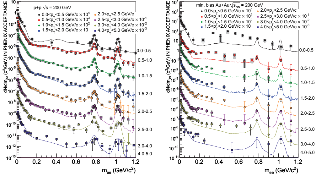
Figure 2.10: Dielectron invariant mass distributions for pp (left) and AuAu collisions (right) [Ada09a]. The distributions are plotted for different intervals of transverse momentum p_T and are compared to the expected spectra from hadron decays.
