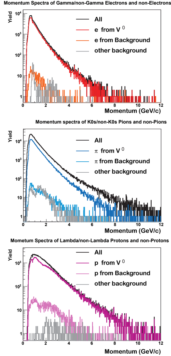
Figure 9.4: Momentum spectra of particles originating from \gamma conversions and from V^0 decays [Hei09]. The complete spectrum as obtained (black) and the intended extracted particles (dark colors: red for electrons, blue for pions, and purple for protons) are shown. The background is plotted, too. It is split into two components: One component is background that consists of the particles of the regarded species which do not originate from a displaced vertex (light colors), the other component consists of all other particles (gray). Only the gray background component influences the purity of a training sample.
