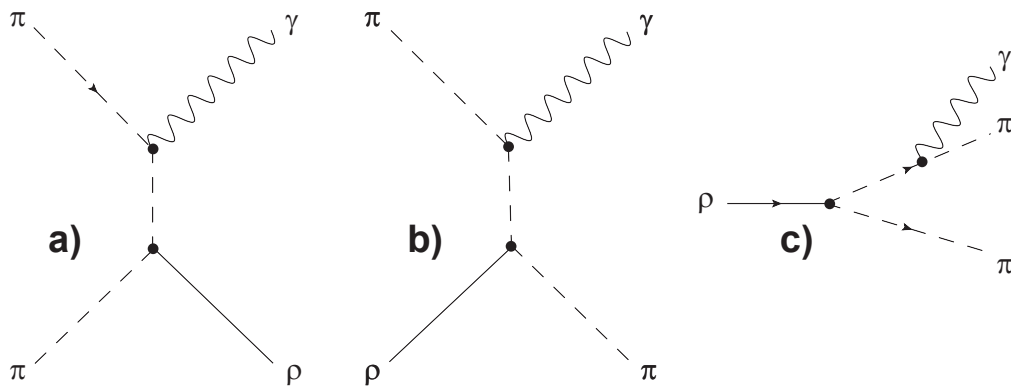
Figure 2.14: Examples of photon production in the hadron gas phase: a) pion annihilation, b) Compton scattering, and c) decays of \rho^0 mesons.
