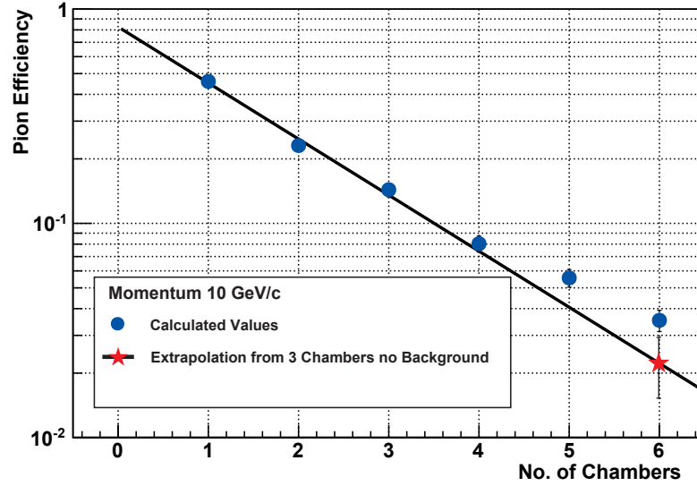
Figure 7.15: Extrapolation method for 10 GeV/c stack data. Shown is pion efficiency versus numbers of chambers that are taken into account. For the fit only the results of the first three chambers were used. A clear difference can be seen for the extrapolated result (red star) and the directly calculated results (blue dots).
