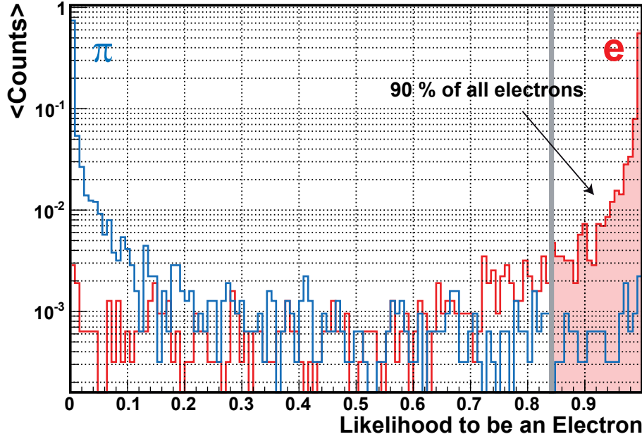
Figure 6.13: Likelihood distribution for electrons (red) and pions (blue) for four TRD layers. This likelihood distribution was extracted from test beam data 2002 using artificial neural networks. In order to determine the pion efficiency at 90% electron efficiency, those 90% of the electrons with the largest electron likelihoods are integrated and a cut is made (grey line). The pion efficiency is the fraction of pions that sits above this integration limit.
