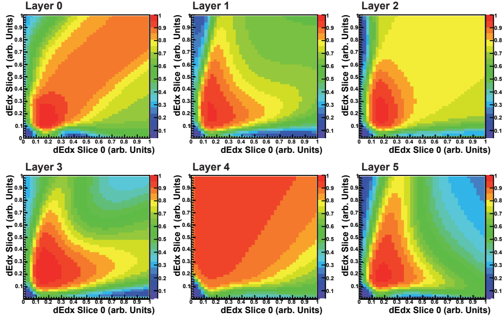
Figure 9.8: Resulting look-up table for the six TRD layers for normalized deposited charges in Slice 0 and Slice 1. The color represents the likelihood to be an electron. The differences in the upper right area are caused by the low statistics in this region. Due to different starting parameters for the training and fluctuations of deposited charge the large differences for the different layers occur. However, due to the limited number of entries in that region (see Figure 9.7) these fluctuations do not have a large influence on the electron identification performance.
