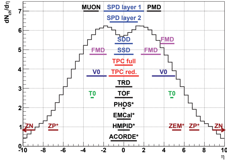
Figure 3.4: Pseudo-rapidity ranges of the ALICE detector systems with a prediction for the charged multiplicity obtained from PYTHIA simulations of pp collisions. The detectors have full azimuthal coverage, unless marked with an asterisk. SPD, SDD, and SSD are subsystems of the ITS, ZN, ZP, and ZEM are parts of the ZDC. For the TPC two \eta ranges are given. "Full" stands for tracks which traverse the TPC over the full radial length, "reduced" means that the track leaves the TPC before reaching the outer radius. The limit is given for tracks which traverse 1/3 of the TPC's radial length. The plot was adapted from Reference [GO09].
