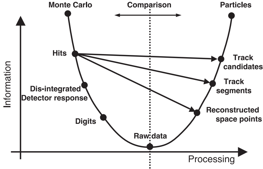
Figure 3.8: Comparison of the simulation (left side) and the reconstruction (right side) in AliRoot [Aam08]. The simulation starts at full event information (Monte Carlo) and is processed to minimum information (Raw data). Minimum information means that no global information of the event is available, just the local detector responses. The reconstruction starts at minimum information and accumulates more information with ongoing processing time, until the properties of the event are reconstructed.
