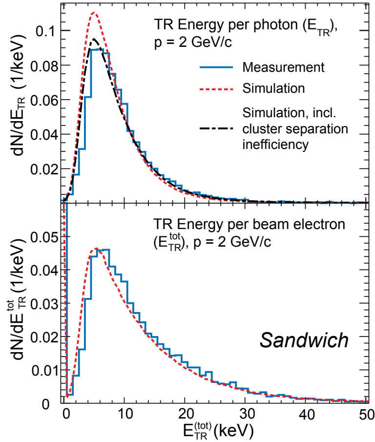
Figure 4.9: Measured and simulated transition radiation spectra [And06b]. The measurement (blue line) was performed with 2 GeV/c electrons during the test beam 2004. The red line represents a simulation using a parameterization for generating transition radiation, the black curve shows the same simulation but with a correction for cluster reconstruction inefficiency. In a ) the transition radiation energy per photon is shown, in b ) the total energy deposit is plotted [And06b].
