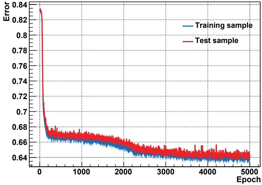
Figure 5.6: Error development of training data (blue) and validation data (red) versus number of epochs. Shown are the curves for the training of one ALICE Transition Radiation Detector prototype chamber from the test beam 2002. It can be seen that after a first fast drop the error reaches a plateau. With increasing number of training epochs the error decreases further and converges. The error curves of training data as well as that of test data fluctuates, which can be understood as noisiness of the error surface.
