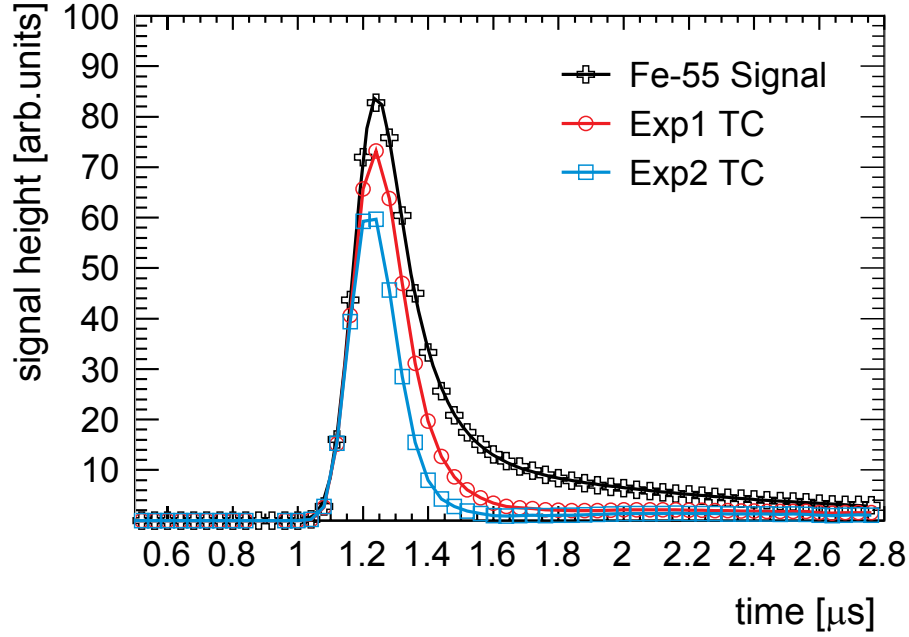
Figure 4.19: Time Response Function measured with an ^{55}\text{Fe} source in black. The effect of tail cancellation can be seen in red and blue. The blue curve shows the resulting time response for a tail cancellation with two exponential functions. The red curve shows the time response if only the long time component is suppressed [Adl05b].
