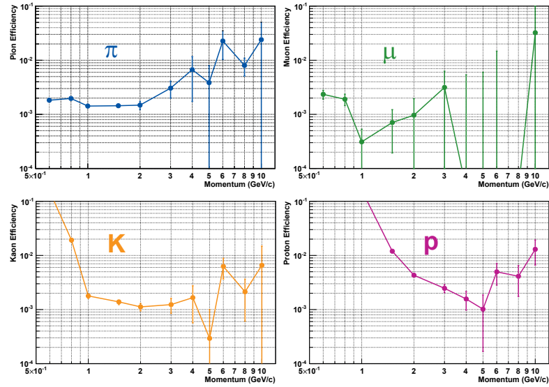
Figure 8.8: a) Pion efficiency, b) muon efficiency, c) kaon, and d) proton efficiency versus momentum for neural networks in pp collisions.
