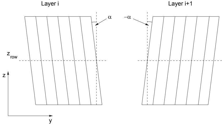
Figure 4.16: In order to improve the position resolution in direction of the long side of the pads ( z direction) the readout pads are tilted by an angle \alpha . The direction of the tilt angle is changed in consecutive layers [TRD01].
