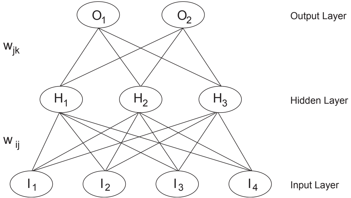
Figure 5.4: A multilayer perceptron with one hidden layer. The network consists of four input neurons I_i which are connected to three hidden neurons H_j . The network has two output neurons O_k . The weights w_{ij} belong to the connections between input neurons and hidden neurons. w_{jk} are the weights of the synapses between hidden layer and output layer.
