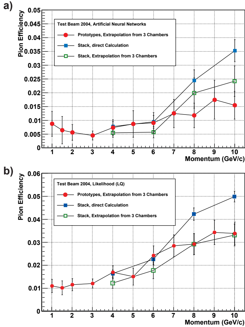
Figure 7.14: Comparison of 2004 prototype results (red dots) on pion efficiency with results achieved with the stack (blue squares) for neural networks a) and likelihood b) . The results at 4 and 6 GeV/c are consistent with each other. The results for higher momenta differ. In addition, the pion efficiencies for the stack using extrapolation are shown (green open squares).
