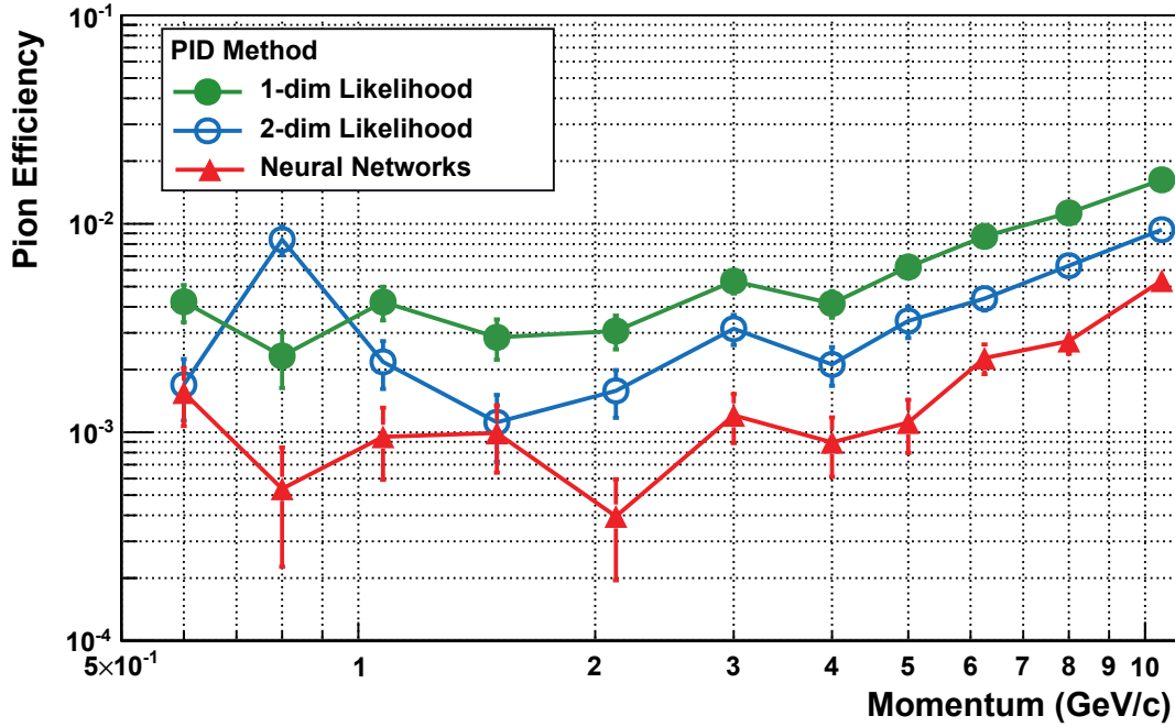
Figure 8.4: Pion efficiency versus momentum for neural networks (red triangles), 1-dim likelihood (green dots) and 2-dim likelihood (blue circles). It can be seen that the pion efficiency depends on the complexity of exploited information. The more information is taken into account the better is the performance.
