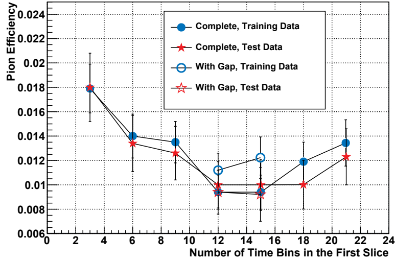
Figure 9.6: Pion efficiency of a neural network with two input neurons versus the number of time bins taken into account for the first slice. The seven different networks were trained for 3,000 epochs. In addition, results are shown for networks with a gap of three time bins. It can be seen that networks with a time bin ratio of 4:4 or 5:3 yield the best pion efficiencies. A gap does not improve the performance of the networks.
