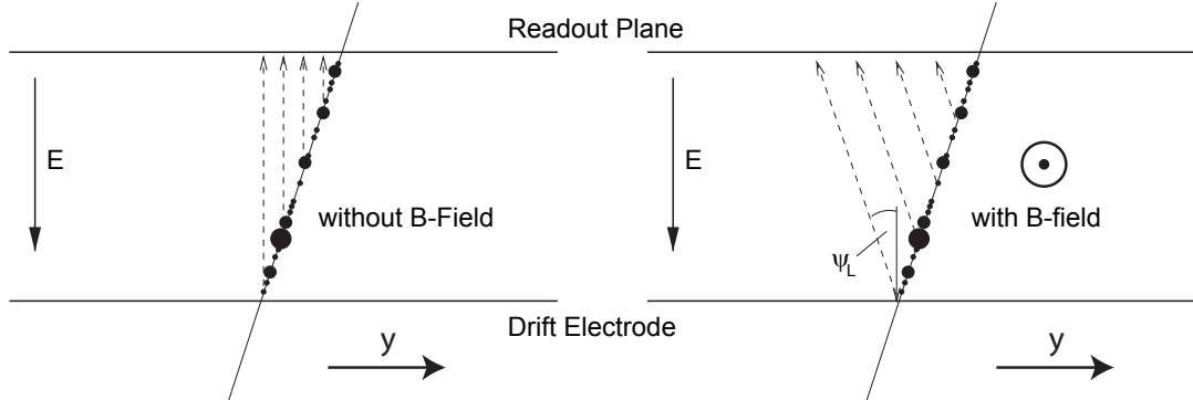
Figure 4.17: The electron clusters in an environment without magnetic field drift directly to the readout plane. In a magnetic field they are deflected in y direction. The deflection angle \psi_L is called Lorentz angle [TRD01].
