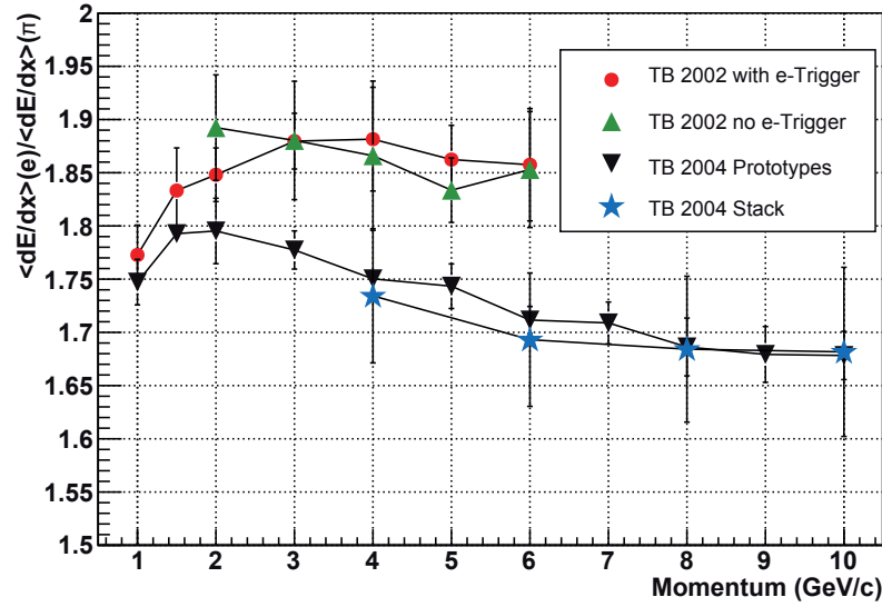
Figure 7.26: Ratio of the mean deposited charge for electrons and pions versus momentum. Ratios for 2002 data (with electron trigger (red dots) and without electron trigger (green triangles)) and 2004 data (prototypes (black triangles) and stack (blue stars)) are shown. The plotted ratios are the average values for all the chambers used in the run.
