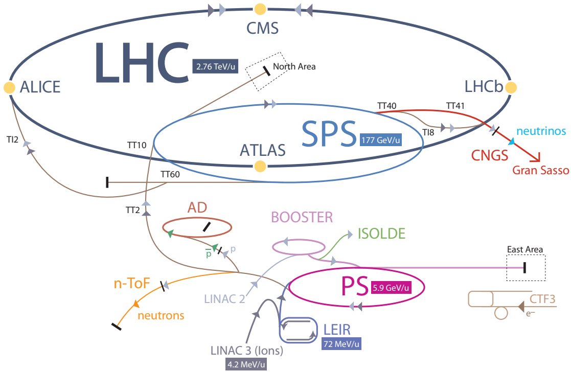
Figure 3.2: The CERN accelerator complex [LHC08]. Shown are the different beam lines and accelerators as well as the corresponding energies for lead ions. Dark grey arrows indicate the beam line for heavy ions, light grey arrows that for protons.
