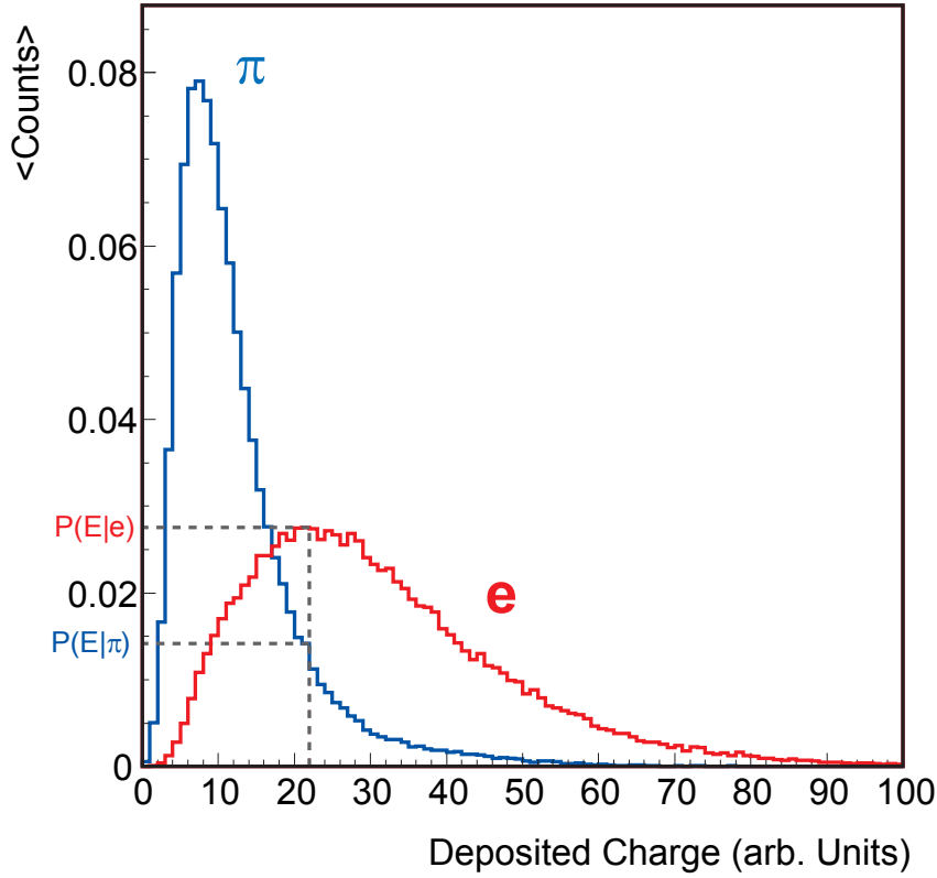
Figure 6.6: Deposited charge for electrons (red) and pions (blue) in one TRD module. This data was taken during the test beam of 2002. The momentum of the particles was 2 GeV/c.
