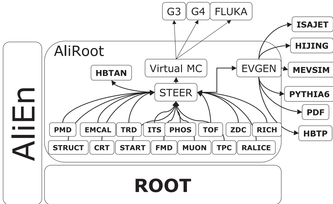
Figure 3.7: Schematic overview of AliRoot [Aam08]. AliRoot is based on the Root framework, the interface to the Grid is AliEn. The central module is STEER, which connects the detector and analysis modules to external event generators, such as HIJING or PYTHIA and to transport packages, like GEANT3.
