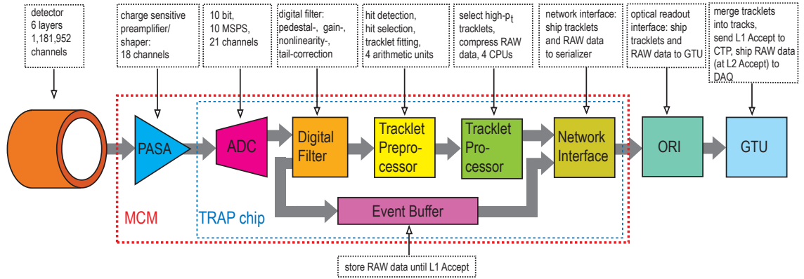
Figure 4.14: Schematic overview of the readout electronics [Aam08].
