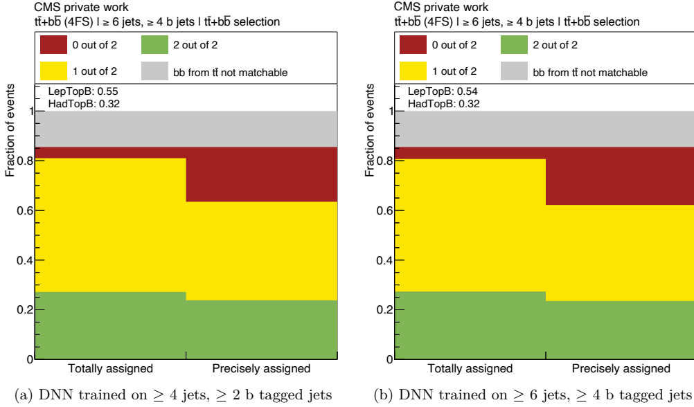
Figure 7.9: DNN performance of the b jets from t\bar{t} system reconstruction. Figure 7.9a shows the DNN performance based on training in the \geq 4 jets, \geq 2 b tagged jets region, Figure 7.9b shows the DNN performance based on training in the \geq 6 jets, \geq 4 b tagged jets region. It is shown how many jets are correctly assigned by the DNN in which fraction of events. The label “precisely assigned” denotes the exact assignment of each jet-type, while “totally assigned” is invariant under a permutation of two or more jet-types.
