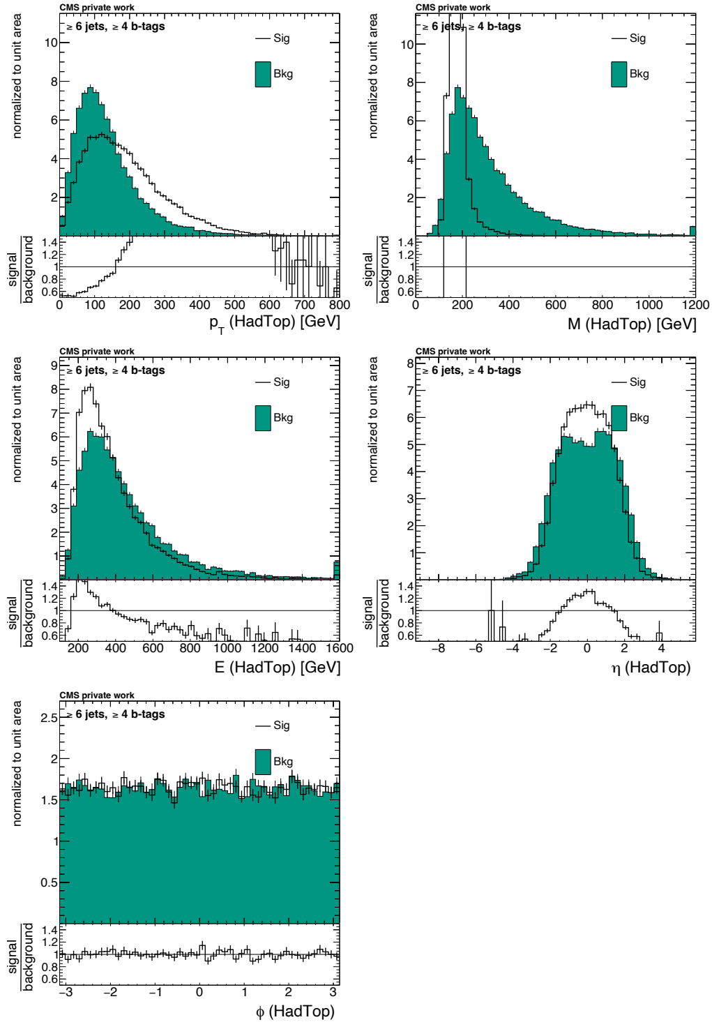
Figure B.31: Input variables of HadTop for DNN training. The solid line (sig) shows the distribution of the given variable for the correct jet assignment. The histogram (bkg) shows a wrong jet assignment.
