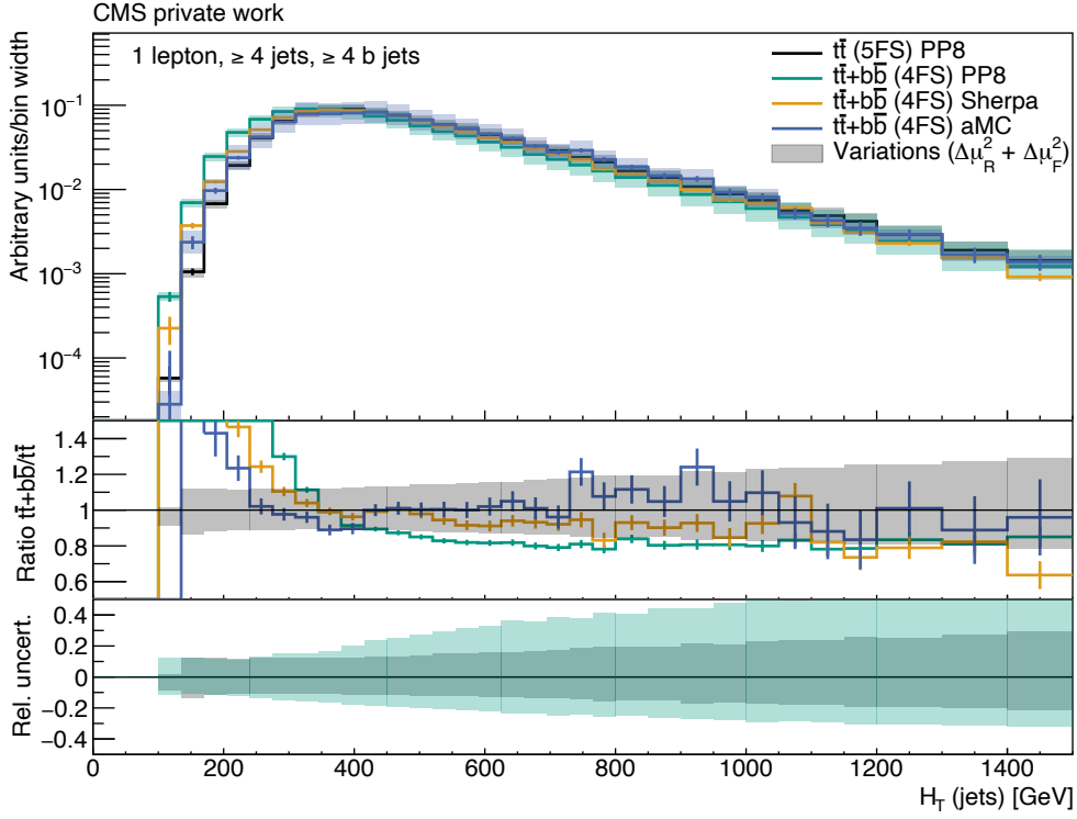
Figure 6.4: H_T (jets) of the t\bar{t} POWHEG+PYTHIA8 (black), t\bar{t}+b\bar{b} POWHEG+PYTHIA8 (green), t\bar{t}+b\bar{b} SHERPA (orange) and t\bar{t}+b\bar{b} MG5AMC(NLO) (blue) simulated events. The statistical uncertainties are shown as bars. The quadratically summed variations of \mu_R and \mu_F are visualized as bands. All distributions are normalized to an integral value of 1. All events pass the selection “1 lepton, \geq 4 jets, \geq 4 b jets”.
