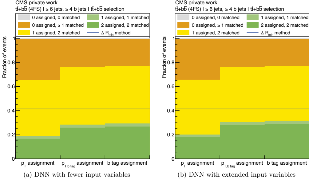
Figure 7.7: Assignment method performance of the t\bar{t} system reconstruction. It is shown how many additional b jets are assigned in which fraction of events depending on the number of jets assigned via the matching algorithm. Figure 7.7a shows the assignment method performance based on the DNN which is trained with the comparably small set of input variables from Table 7.4. Figure 7.7b shows the assignment method performance based on the DNN which is trained with the considerably enlarged set of input variables.
