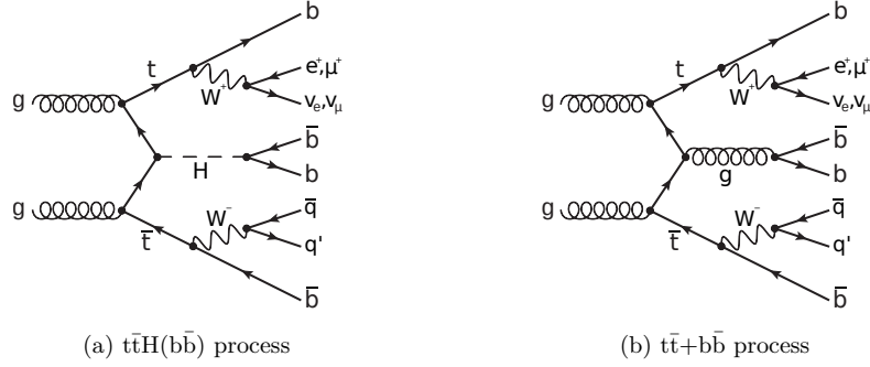
Figure 5.1: Examples of LO Feynman diagrams for the t\bar{t}H(b\bar{b}) and t\bar{t}+b\bar{b} processes.
