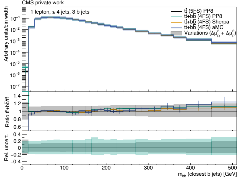
Figure A.13: m_{bb} (closest) of the tt POWHEG+PYTHIA8 (black), tt+bb POWHEG+PYTHIA8 (green), tt+bb SHERPA (orange) and tt+bb MG5AMC-(NLO) (blue) simulated events. The statistical uncertainties are shown as bars. The quadratically summed variations of \mu_R and \mu_F are visualized as bands. All distributions are normalized to an integral value of 1. All events pass the selection “1 lepton, \geq 4 jets, 3 b jets”.
