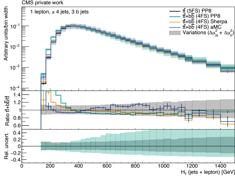
Figure A.7: H_T (jets+lepton) of the tt POWHEG+PYTHIA8 (black), tt+bb POWHEG+PYTHIA8 (green), tt+bb SHERPA (orange) and tt+bb MG5AMC(NLO) (blue) simulated events. The statistical uncertainties are shown as bars. The quadratically summed variations of \mu_R and \mu_F are visualized as bands. All distributions are normalized to an integral value of 1. All events pass the selection “1 lepton, \geq 4 jets, 3 b jets”.
