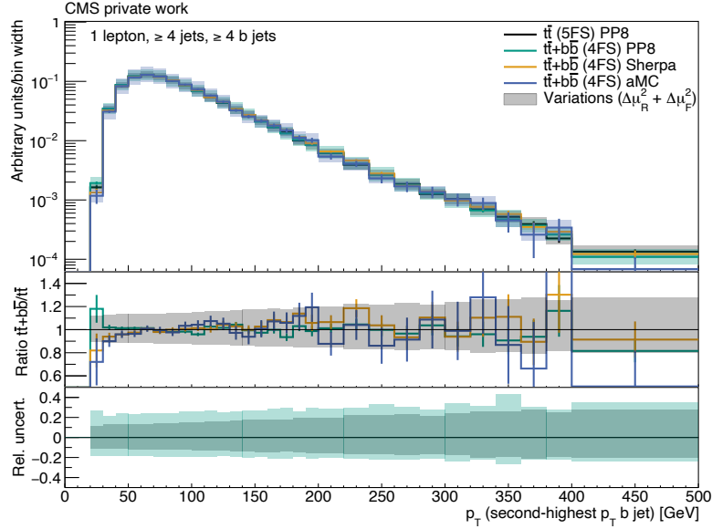
Figure A.18: Sub-leading b jet p_T of the t\bar{t} POWHEG+PYTHIA8 (black), t\bar{t}+b\bar{b} POWHEG+PYTHIA8 (green), t\bar{t}+b\bar{b} SHERPA (orange) and t\bar{t}+b\bar{b} MG5AMC-(NLO) (blue) simulated events. The statistical uncertainties are shown as bars. The quadratically summed variations of \mu_R and \mu_F are visualized as bands. All distributions are normalized to an integral value of 1. All events pass the selection “1 lepton, \geq 4 jets, \geq 4 b jets”.
