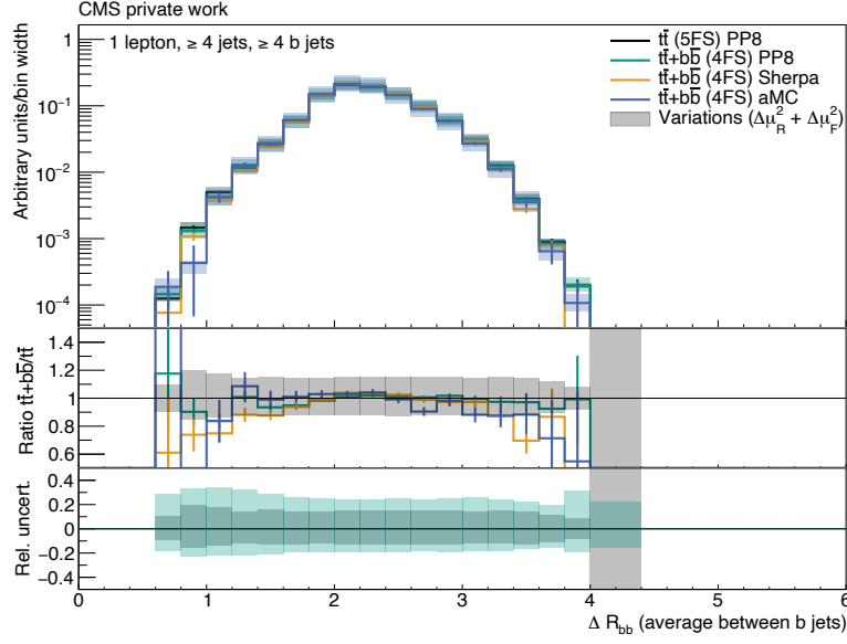
Figure A.23: \Delta R(bb) (average) of the t\bar{t} POWHEG+PYTHIA8 (black), t\bar{t}+b\bar{b} POWHEG+PYTHIA8 (green), t\bar{t}+b\bar{b} SHERPA (orange) and t\bar{t}+b\bar{b} MG5AMC-(NLO) (blue) simulated events. The statistical uncertainties are shown as bars. The quadratically summed variations of \mu_R and \mu_F are visualized as bands. All distributions are normalized to an integral value of 1. All events pass the selection “1 lepton, \geq 4 jets, \geq 4 b jets”.
