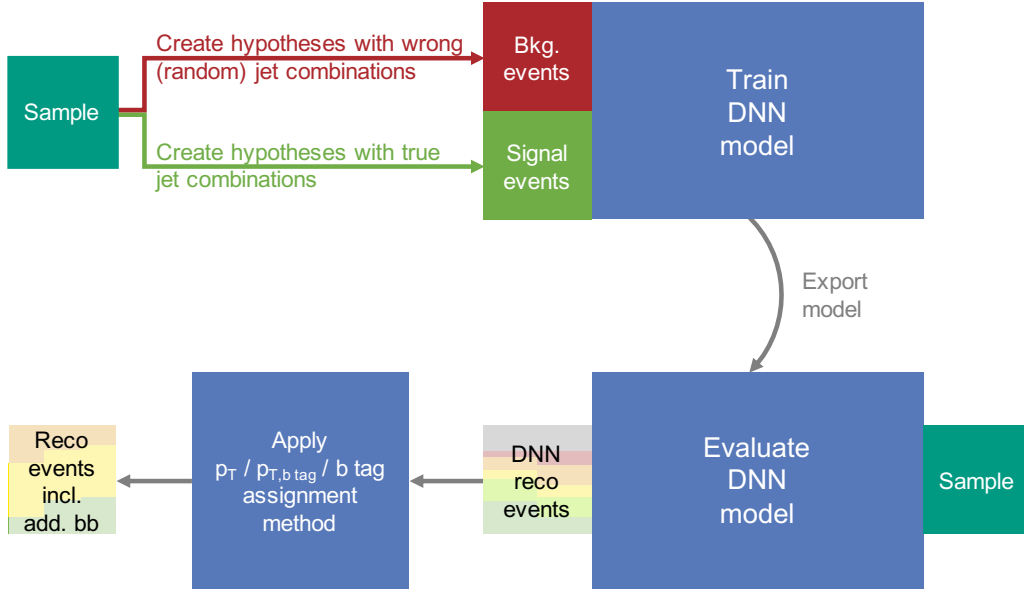
Figure 7.3: Illustration of the analysis process of the DNN based method. The upper part of the figure shows the creation of the hypotheses and the training of the DNN. The lower part of the graphic shows the evaluation of the sample, the application of the assignment methods and the final result, the assignment of the additional b jets.
