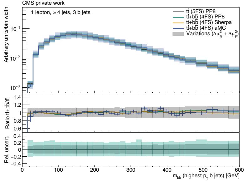
Figure A.14: m_{bb} (leading) of the tt POWHEG+PYTHIA8 (black), tt+bb POWHEG+PYTHIA8 (green), tt+bb SHERPA (orange) and tt+bb MG5AMC-(NLO) (blue) simulated events. The statistical uncertainties are shown as bars. The quadratically summed variations of \mu_R and \mu_F are visualized as bands. All distributions are normalized to an integral value of 1. All events pass the selection “1 lepton, \geq 4 jets, 3 b jets”.
