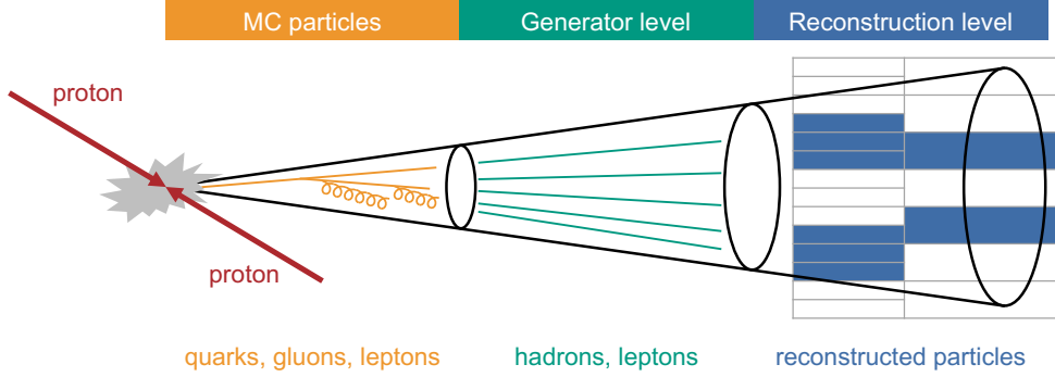
Figure 5.2: Visualization of different simulation levels of a jet. Generator level is shown in the middle of the figure, reconstruction level is shown on the right side. Exemplary physics objects are correspondingly listed at the bottom.
