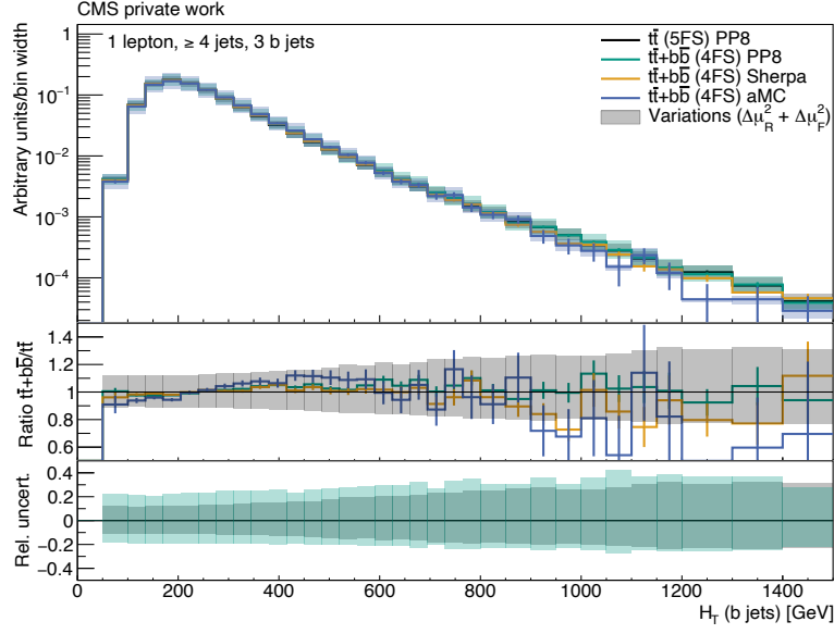
Figure A.9: H_T (b jets) of the t\bar{t} POWHEG+PYTHIA8 (black), t\bar{t}+b\bar{b} POWHEG+PYTHIA8 (green), t\bar{t}+b\bar{b} SHERPA (orange) and t\bar{t}+b\bar{b} MG5AMC(NLO) (blue) simulated events. The statistical uncertainties are shown as bars. The quadratically summed variations of \mu_R and \mu_F are visualized as bands. All distributions are normalized to an integral value of 1. All events pass the selection “1 lepton, \geq 4 jets, 3 b jets”.
