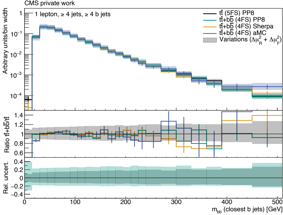
Figure 6.7: m(bb) (closest) of the t\bar{t} POWHEG+PYTHIA8 (black), t\bar{t}+b\bar{b} POWHEG+PYTHIA8 (green), t\bar{t}+b\bar{b} SHERPA (orange) and t\bar{t}+b\bar{b} MG5-AMC(NLO) (blue) simulated events. The statistical uncertainties are shown as bars. The quadratically summed variations of \mu_R and \mu_F are visualized as bands. All distributions are normalized to an integral value of 1. All events pass the selection “1 lepton, \geq 4 jets, \geq 4 b jets”.
