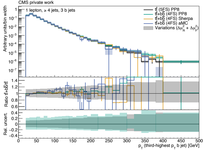
Figure A.6: Third b jet p_T of the t\bar{t} POWHEG+PYTHIA8 (black), t\bar{t}+b\bar{b} POWHEG+PYTHIA8 (green), t\bar{t}+b\bar{b} SHERPA (orange) and t\bar{t}+b\bar{b} MG5AMC(NLO) (blue) simulated events. The statistical uncertainties are shown as bars. The quadratically summed variations of \mu_R and \mu_F are visualized as bands. All distributions are normalized to an integral value of 1. All events pass the selection “1 lepton, \geq 4 jets, 3 b jets”.
