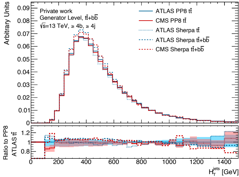
(b) t\bar{t} POWHEG+PYTHIA8 and t\bar{t}/t\bar{t}+b\bar{b} SHERPA simulations
