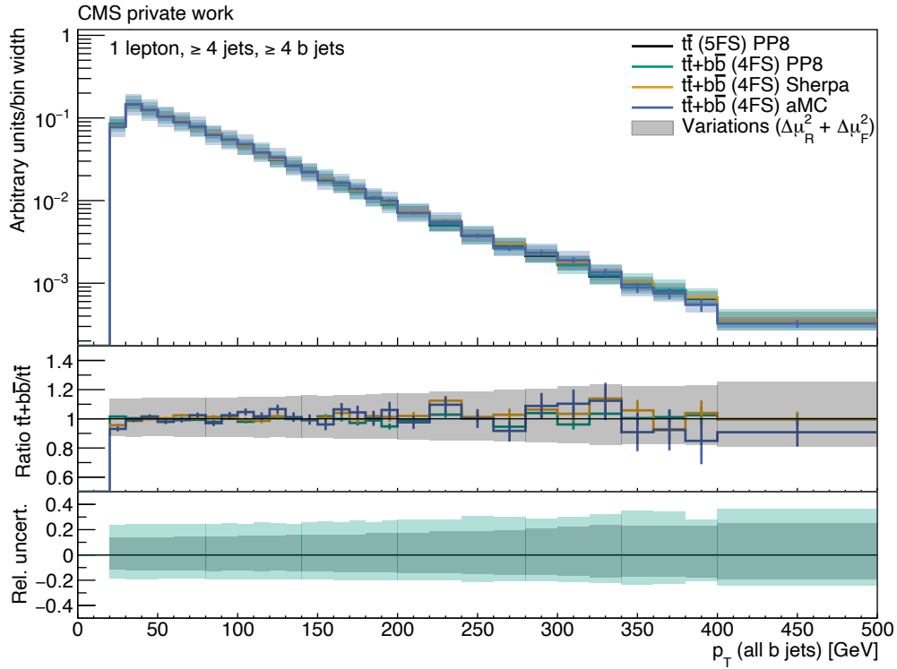
Figure 6.3: p_T (all b jets) of the t\bar{t} POWHEG+PYTHIA8 (black), t\bar{t}+b\bar{b} POWHEG+PYTHIA8 (green), t\bar{t}+b\bar{b} SHERPA (orange) and t\bar{t}+b\bar{b} MG5AMC(NLO) (blue) simulated events. The statistical uncertainties are shown as bars. The quadratically summed variations of \mu_R and \mu_F are visualized as bands. All distributions are normalized to an integral value of 1. All events pass the selection “1 lepton, \geq 4 jets, \geq 4 b jets”.
