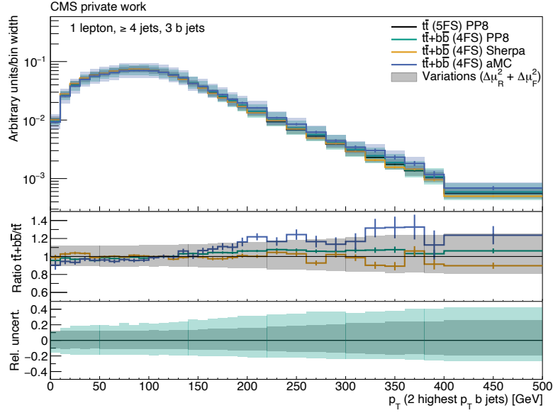
Figure A.16: p_T(\text{bb}) (leading) of the t\bar{t} POWHEG+PYTHIA8 (black), t\bar{t}+b\bar{b} POWHEG+PYTHIA8 (green), t\bar{t}+b\bar{b} SHERPA (orange) and t\bar{t}+b\bar{b} MG5AMC-(NLO) (blue) simulated events. The statistical uncertainties are shown as bars. The quadratically summed variations of \mu_R and \mu_F are visualized as bands. All distributions are normalized to an integral value of 1. All events pass the selection “1 lepton, \geq 4 jets, 3 b jets”.
