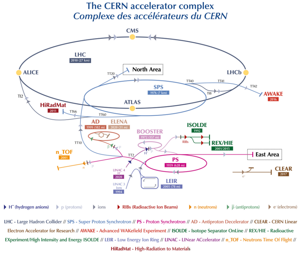
Figure 3.1: The CERN accelerator complex, taken from [42]. The Large Hadron Collider is the last element in the chain of accelerators (dark blue). Also, the experiments at CERN are indicated at the respective positions of the accelerators (yellow dots).
