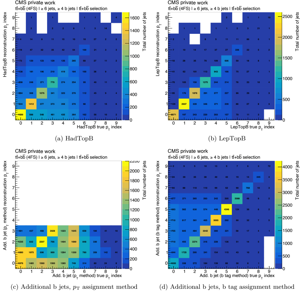
Figure 7.11: Confusion matrices of b jets for the DNN with training in the signal region. Figures 7.11a and 7.11b show the b jets from the top quark decays assigned directly by the DNN. Based on this, Figures 7.11c and 7.11d show the p_T and b tag assignment methods.
