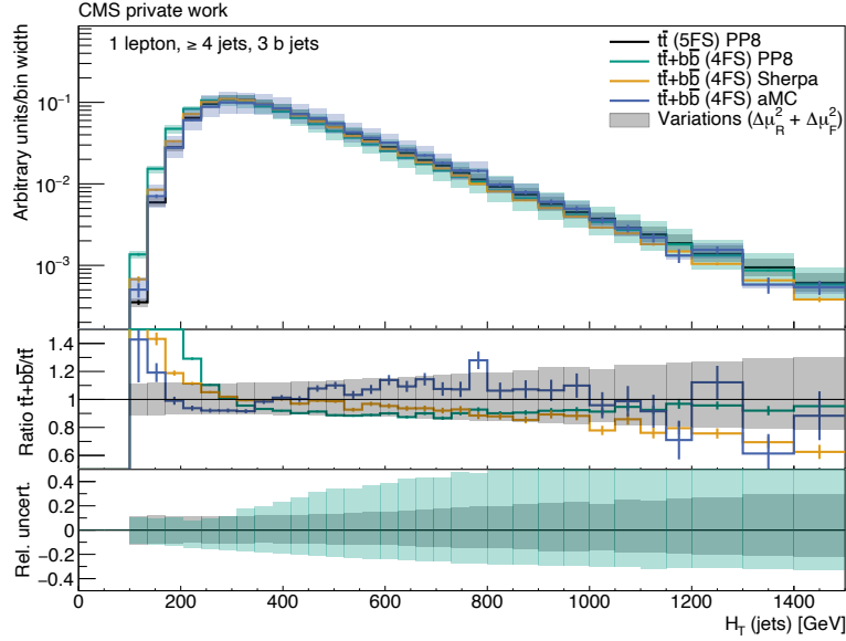
Figure A.8: H_T (jets) of the tt POWHEG+PYTHIA8 (black), tt+bb POWHEG+PYTHIA8 (green), tt+bb SHERPA (orange) and tt+bb MG5AMC(NLO) (blue) simulated events. The statistical uncertainties are shown as bars. The quadratically summed variations of \mu_R and \mu_F are visualized as bands. All distributions are normalized to an integral value of 1. All events pass the selection “1 lepton, \geq 4 jets, 3 b jets”.
