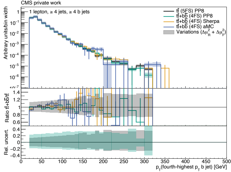
Figure A.20: Fourth b jet p_T of the t\bar{t} POWHEG+PYTHIA8 (black), t\bar{t}+b\bar{b} POWHEG+PYTHIA8 (green), t\bar{t}+b\bar{b} SHERPA (orange) and t\bar{t}+b\bar{b} MG5AMC-(NLO) (blue) simulated events. The statistical uncertainties are shown as bars. The quadratically summed variations of \mu_R and \mu_F are visualized as bands. All distributions are normalized to an integral value of 1. All events pass the selection “1 lepton, \geq 4 jets, \geq 4 b jets”.
