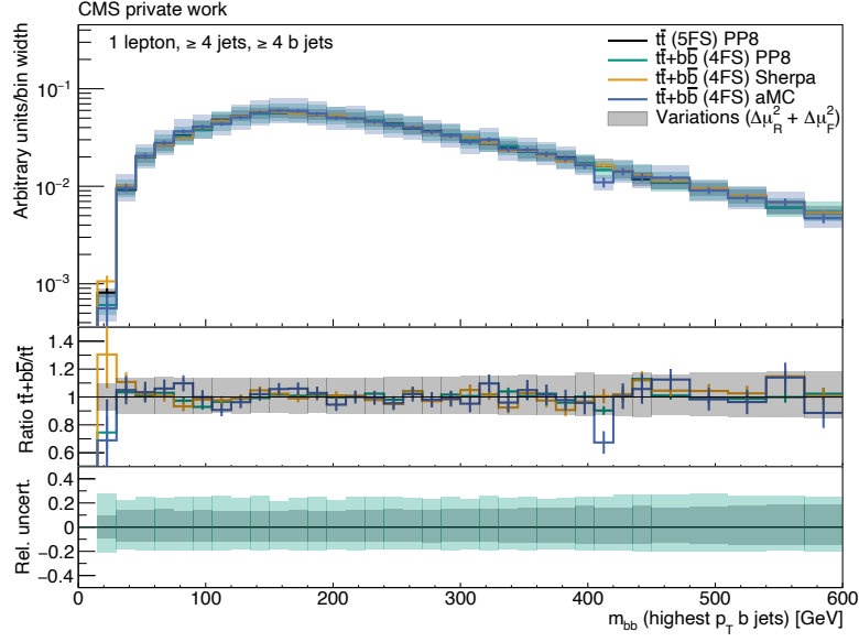
Figure A.25: m(bb) (leading) of the t\bar{t} POWHEG+PYTHIA8 (black), t\bar{t}+b\bar{b} POWHEG+PYTHIA8 (green), t\bar{t}+b\bar{b} SHERPA (orange) and t\bar{t}+b\bar{b} MG5AMC-(NLO) (blue) simulated events. The statistical uncertainties are shown as bars. The quadratically summed variations of \mu_R and \mu_F are visualized as bands. All distributions are normalized to an integral value of 1. All events pass the selection “1 lepton, \geq 4 jets, \geq 4 b jets”.
