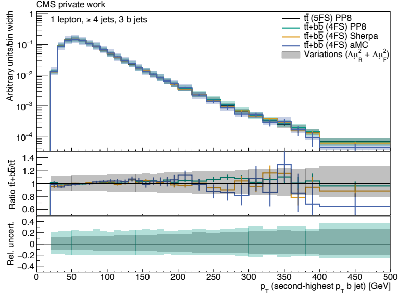
Figure A.5: Sub-leading b jet p_T of the t\bar{t} POWHEG+PYTHIA8 (black), t\bar{t}+b\bar{b} POWHEG+PYTHIA8 (green), t\bar{t}+b\bar{b} SHERPA (orange) and t\bar{t}+b\bar{b} MG5AMC(NLO) (blue) simulated events. The statistical uncertainties are shown as bars. The quadratically summed variations of \mu_R and \mu_F are visualized as bands. All distributions are normalized to an integral value of 1. All events pass the selection “1 lepton, \geq 4 jets, 3 b jets”.
