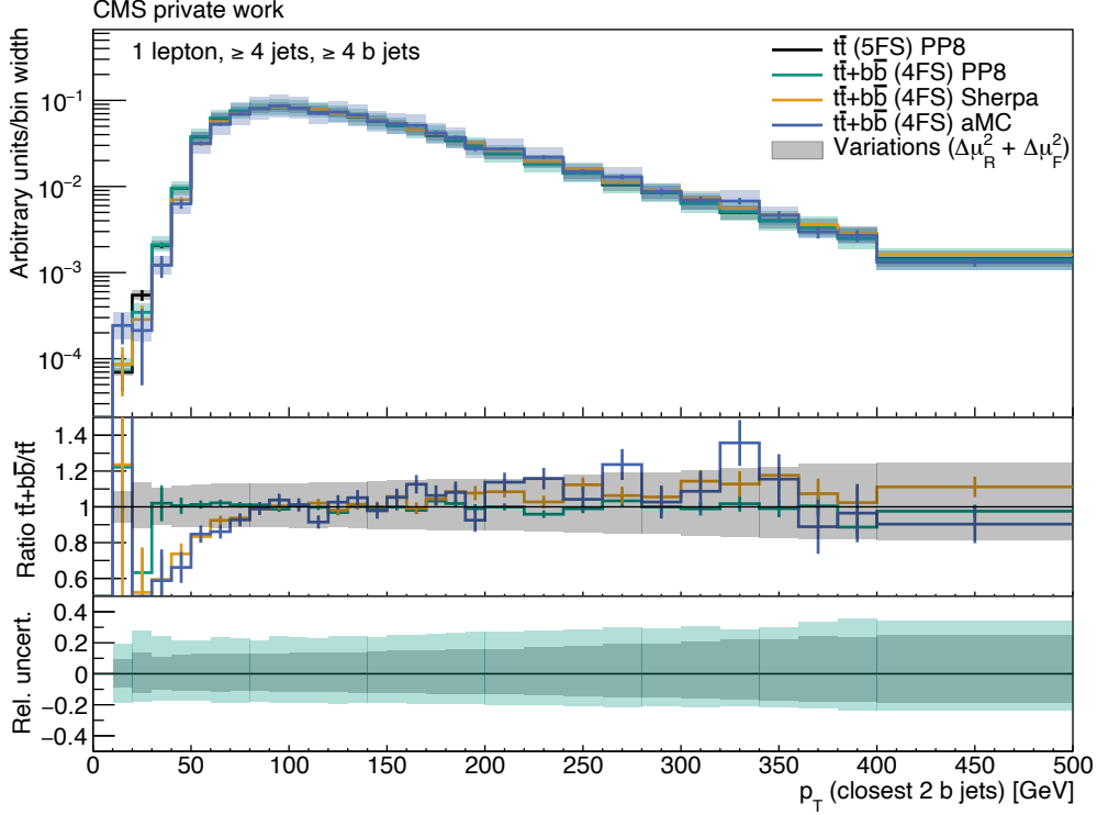
Figure 6.8: p_T (bb) (closest) of the t\bar{t} POWHEG+PYTHIA8 (black), t\bar{t}+b\bar{b} POWHEG+PYTHIA8 (green), t\bar{t}+b\bar{b} SHERPA (orange) and t\bar{t}+b\bar{b} MG5-AMC(NLO) (blue) simulated events. The statistical uncertainties are shown as bars. The quadratically summed variations of \mu_R and \mu_F are visualized as bands. All distributions are normalized to an integral value of 1. All events pass the selection “1 lepton, \geq 4 jets, \geq 4 b jets”.
