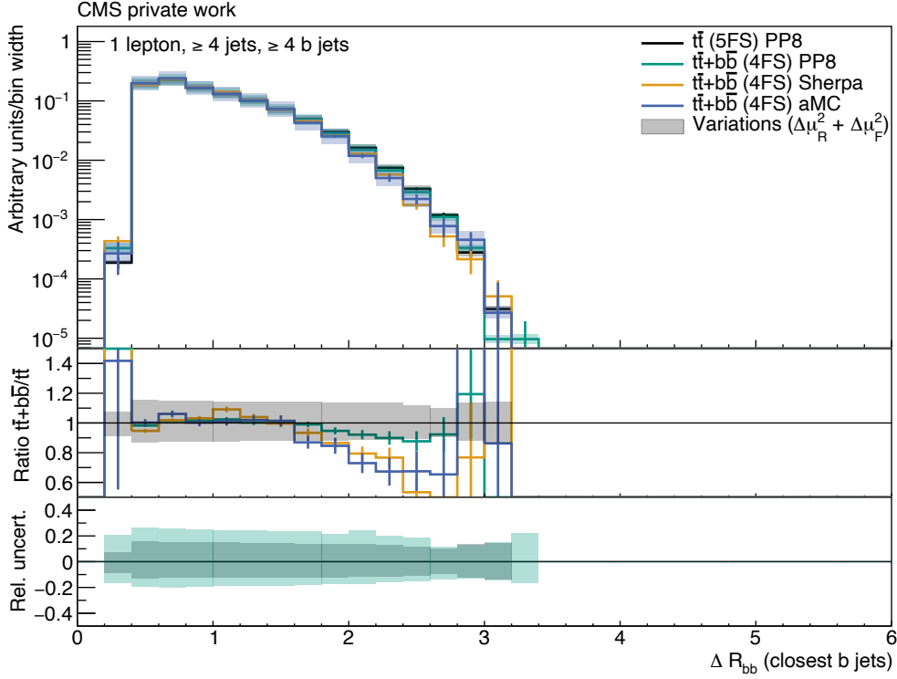
Figure 6.5: \Delta R(bb) (closest) of the t\bar{t} POWHEG+PYTHIA8 (black), t\bar{t}+b\bar{b} POWHEG+PYTHIA8 (green), t\bar{t}+b\bar{b} SHERPA (orange) and t\bar{t}+b\bar{b} MG5-AMC(NLO) (blue) simulated events. The statistical uncertainties are shown as bars. The quadratically summed variations of \mu_R and \mu_F are visualized as bands. All distributions are normalized to an integral value of 1. All events pass the selection “1 lepton, \geq 4 jets, \geq 4 b jets”.
