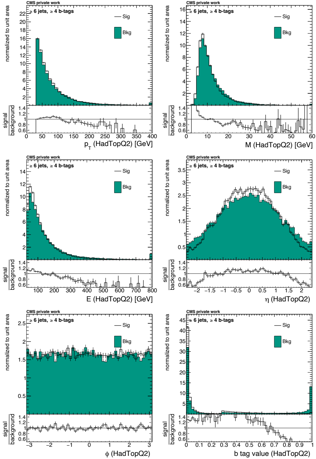
Figure B.30: Input variables of HadTopQ2 for DNN training. The solid line (sig) shows the distribution of the given variable for the correct jet assignment. The histogram (bkg) shows a wrong jet assignment.
