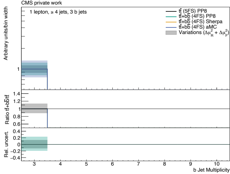
Figure A.2: b jet multiplicity of the t\bar{t} POWHEG+PYTHIA8 (black), t\bar{t}+b\bar{b} POWHEG+PYTHIA8 (green), t\bar{t}+b\bar{b} SHERPA (orange) and t\bar{t}+b\bar{b} MG5AMC-(NLO) (blue) simulated events. The statistical uncertainties are shown as bars. The quadratically summed variations of \mu_R and \mu_F are visualized as bands. All distributions are normalized to an integral value of 1. All events pass the selection “1 lepton, \geq 4 jets, 3 b jets”.
