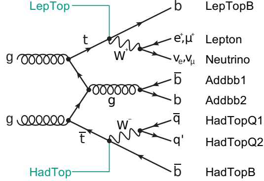
Figure 7.2: Example t\bar{t}+b\bar{b} Feynman diagram with names introduced for the objects.
