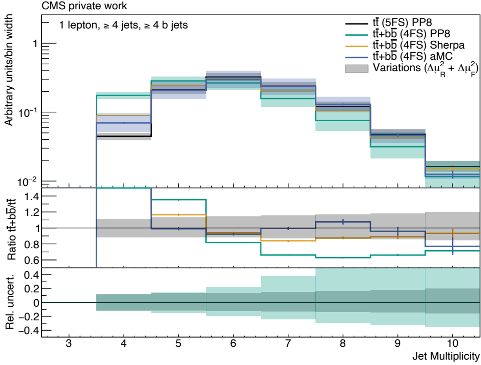
Figure 6.1: Jet multiplicity of the t\bar{t} POWHEG+PYTHIA8 (black), t\bar{t}+b\bar{b} POWHEG+PYTHIA8 (green), t\bar{t}+b\bar{b} SHERPA (orange) and t\bar{t}+b\bar{b} MG5-AMC(NLO) (blue) simulated events. The statistical uncertainties are shown as bars. The quadratically summed variations of \mu_R and \mu_F are visualized as bands. All distributions are normalized to an integral value of 1. All events pass the selection “1 lepton, \geq 4 jets, \geq 4 b jets”.
