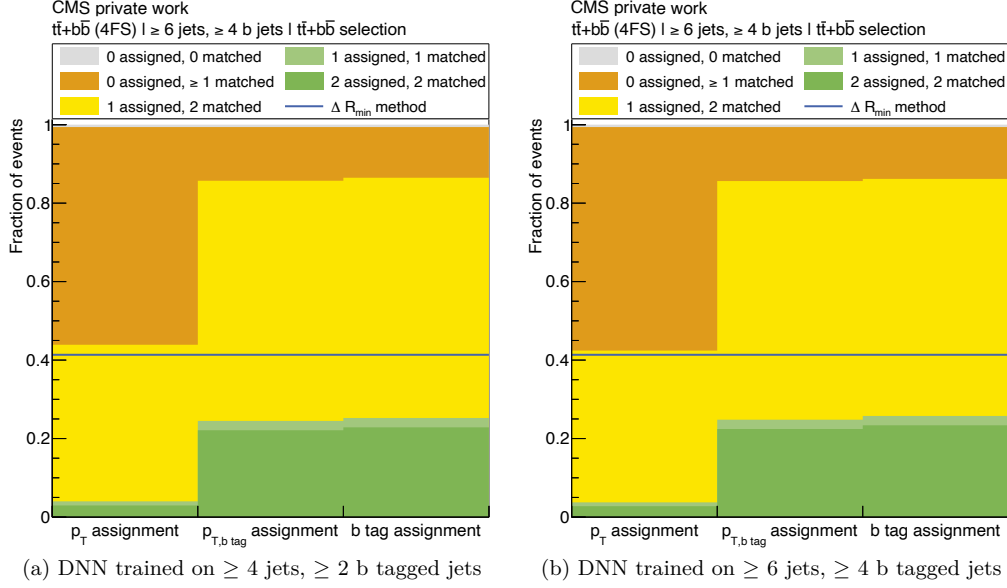
Figure 7.10: Assignment method performance of the b jets from t\bar{t} system reconstruction.
