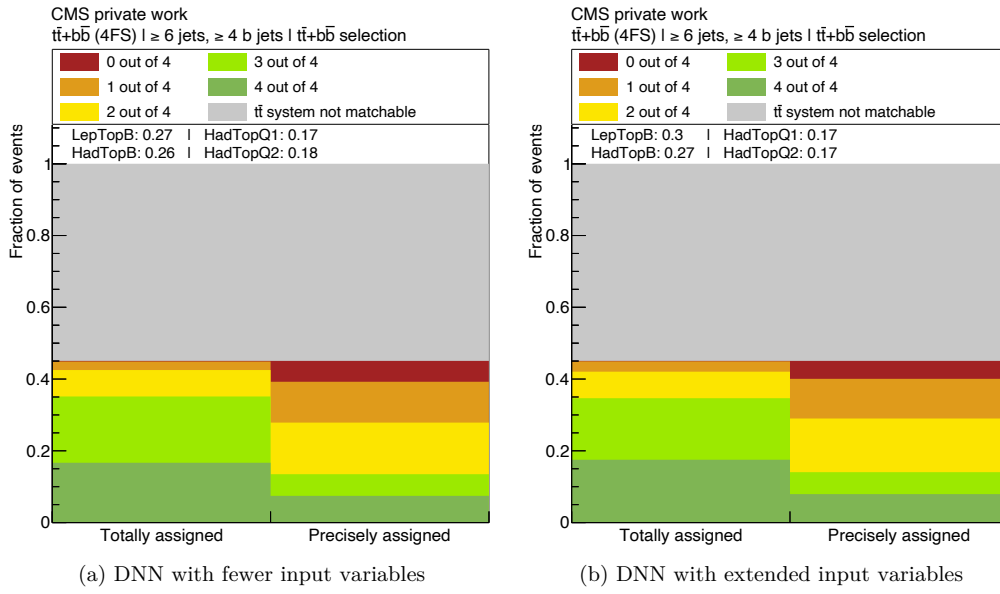
Figure 7.6: DNN performance of the t\bar{t} system reconstruction. It is shown how many jets are correctly assigned by the DNN in which fraction of events. Figure 7.6a shows the DNN performance based on training with the comparably small set of input variables from Table 7.4, Figure 7.6b shows the DNN performance based on the training with the considerably enlarged set of input variables. The label “precisely assigned” denotes the exact assignment of each jet-type, while “totally assigned” is invariant under a permutation of two or more jet-types.
