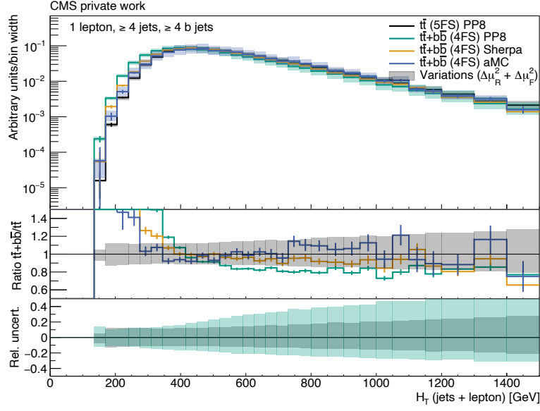
Figure A.21: H_T (jets+lepton) of the t\bar{t} POWHEG+PYTHIA8 (black), t\bar{t}+b\bar{b} POWHEG+PYTHIA8 (green), t\bar{t}+b\bar{b} SHERPA (orange) and t\bar{t}+b\bar{b} MG5AMC-(NLO) (blue) simulated events. The statistical uncertainties are shown as bars. The quadratically summed variations of \mu_R and \mu_F are visualized as bands. All distributions are normalized to an integral value of 1. All events pass the selection “1 lepton, \geq 4 jets, \geq 4 b jets”.
