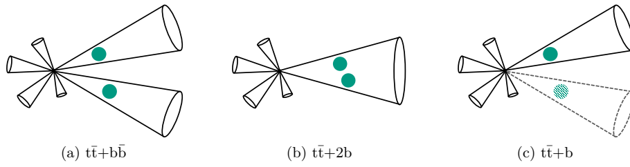
Figure 5.3: Illustration of t\bar{t}+B events. The t\bar{t} system is not shown in this visualization, the differences only pertain to the additional jets. Figure 5.3a shows two separate jets, each of them contains a B hadron (green circle). Figure 5.3b shows both B hadrons very close to each other which are therefore merged into a single jet. Figure 5.3c also shows two separate jets with a B hadron in each jet, but one jet is out of acceptance (dashed).
