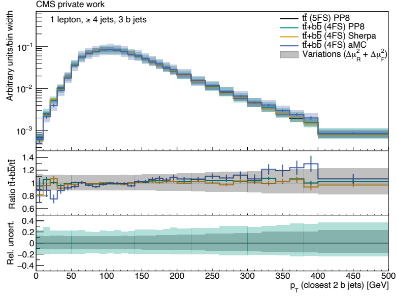
Figure A.15: p_T(\text{bb}) (closest) of the t\bar{t} POWHEG+PYTHIA8 (black), t\bar{t}+b\bar{b} POWHEG+PYTHIA8 (green), t\bar{t}+b\bar{b} SHERPA (orange) and t\bar{t}+b\bar{b} MG5AMC-(NLO) (blue) simulated events. The statistical uncertainties are shown as bars. The quadratically summed variations of \mu_R and \mu_F are visualized as bands. All distributions are normalized to an integral value of 1. All events pass the selection “1 lepton, \geq 4 jets, 3 b jets”.
