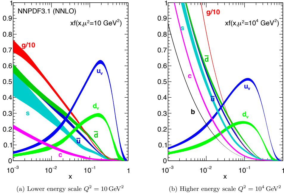
Figure 2.1: Example PDF sets as a function of the momentum fraction x at two different energy scales ( \mu^2 = Q^2 ): in Figure 2.1a at a lower energy scale ( 10 \text{ GeV}^2 ), in Figure 2.1b at a higher energy scale ( 10^4 \text{ GeV}^2 ) [40] are shown. At both energies, the valence quarks dominate the high momentum fractions while the gluons dominate the lower scale. The gluon distributions are divided by a factor of 10 and thus dominate to a significantly stronger extent at low Q^2 than visually represented. However, the distributions are shifting at high energies, the probabilities for finding the valence quarks diminish and the sea quarks as well as the gluons become relevant. In fact, even the b quark can be noticed (black). The PDF sets will be used in Chapter 6.
