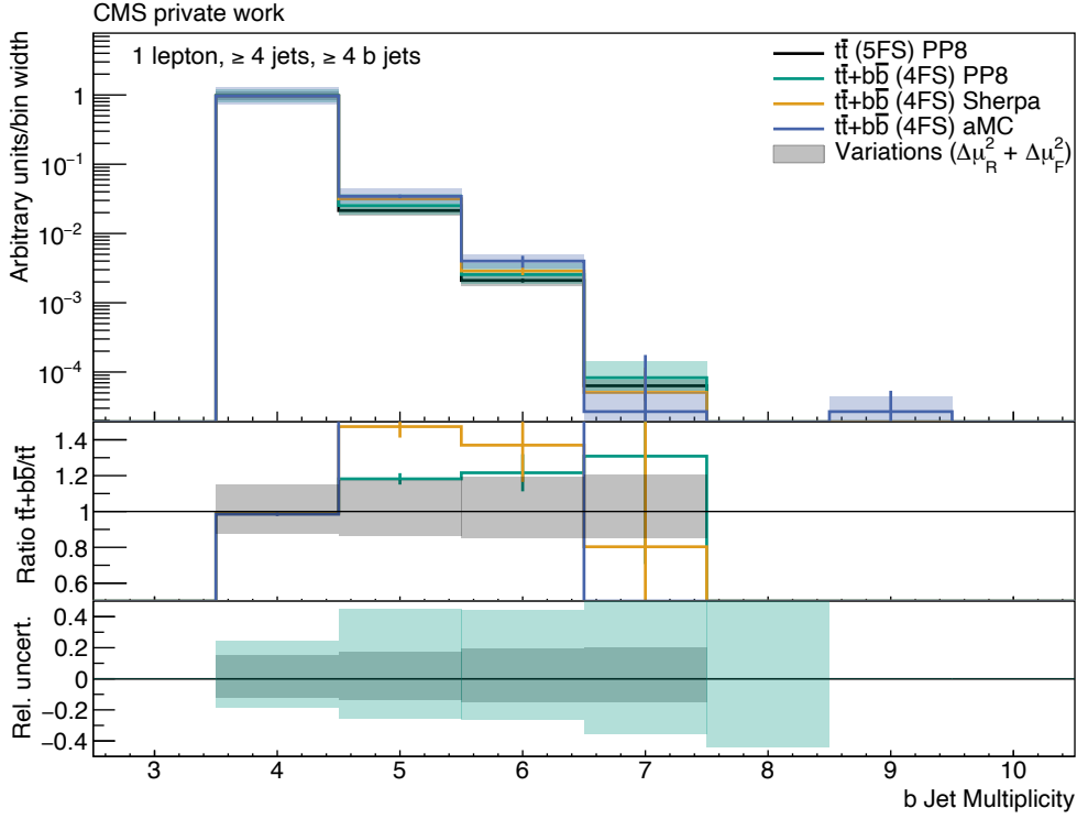
Figure 6.2: b jet multiplicity of the t\bar{t} POWHEG+PYTHIA8 (black), t\bar{t}+b\bar{b} POWHEG+PYTHIA8 (green), t\bar{t}+b\bar{b} SHERPA (orange) and t\bar{t}+b\bar{b} MG5-AMC(NLO) (blue) simulated events. The statistical uncertainties are shown as bars. The quadratically summed variations of \mu_R and \mu_F are visualized as bands. All distributions are normalized to an integral value of 1. All events pass the selection “1 lepton, \geq 4 jets, \geq 4 b jets”.
