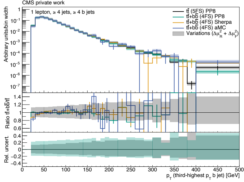
Figure A.19: Third b jet p_T of the t\bar{t} POWHEG+PYTHIA8 (black), t\bar{t}+b\bar{b} POWHEG+PYTHIA8 (green), t\bar{t}+b\bar{b} SHERPA (orange) and t\bar{t}+b\bar{b} MG5AMC-(NLO) (blue) simulated events. The statistical uncertainties are shown as bars. The quadratically summed variations of \mu_R and \mu_F are visualized as bands. All distributions are normalized to an integral value of 1. All events pass the selection “1 lepton, \geq 4 jets, \geq 4 b jets”.
