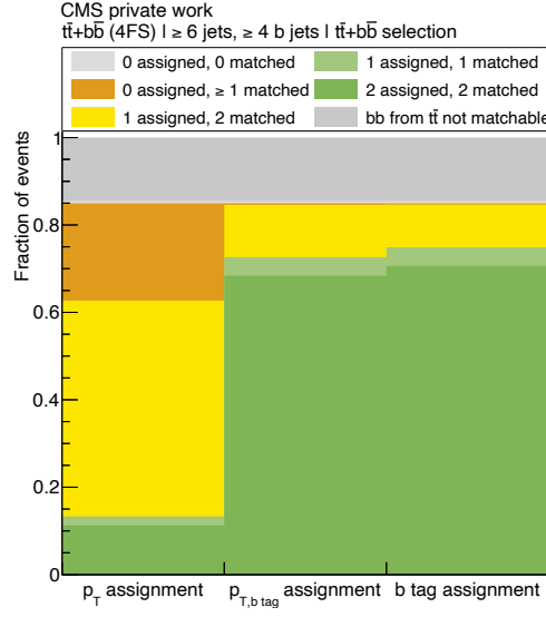
Figure 7.8: Maximum possible efficiency of the p_T , p_{T,b \text{ tag}} and b tag assignment method for the b jets from t\bar{t} system reconstruction strategy assuming a perfect DNN reconstruction. It is shown how many additional b jets are assigned in which fraction of events depending on the number of jets assigned via the matching algorithm.
