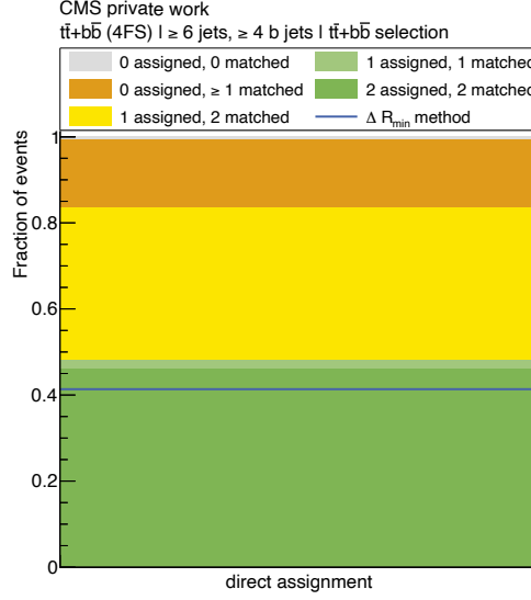
Figure 7.12: Performance of the additional b jet reconstruction with direct DNN training. It is shown how many additional b jets are assigned in which fraction of events depending on the number of jets assigned via the matching algorithm.
