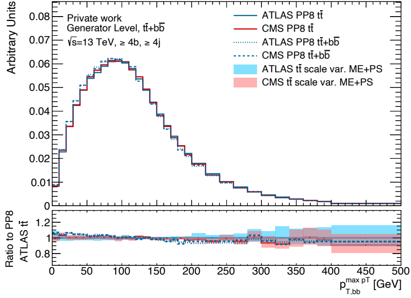
(a) t\bar{t} POWHEG+PYTHIA8 and t\bar{t}+b\bar{b} POWHEG+PYTHIA8 simulations
