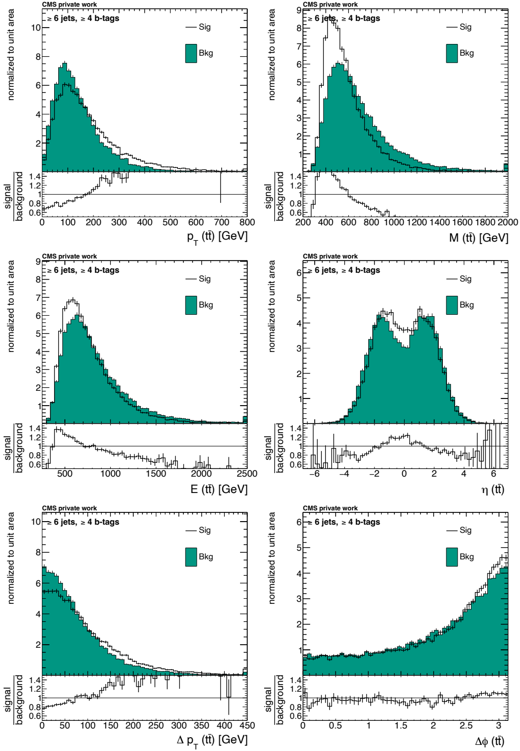
Figure B.33: Input variables of t\bar{t} for DNN training. The solid line (sig) shows the distribution of the given variable for the correct jet assignment. The histogram (bkg) shows a wrong jet assignment.
