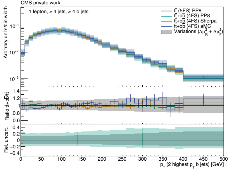
Figure A.26: p_T(bb) (leading) of the t\bar{t} POWHEG+PYTHIA8 (black), t\bar{t}+b\bar{b} POWHEG+PYTHIA8 (green), t\bar{t}+b\bar{b} SHERPA (orange) and t\bar{t}+b\bar{b} MG5AMC-(NLO) (blue) simulated events. The statistical uncertainties are shown as bars. The quadratically summed variations of \mu_R and \mu_F are visualized as bands. All distributions are normalized to an integral value of 1. All events pass the selection “1 lepton, \geq 4 jets, \geq 4 b jets”.
