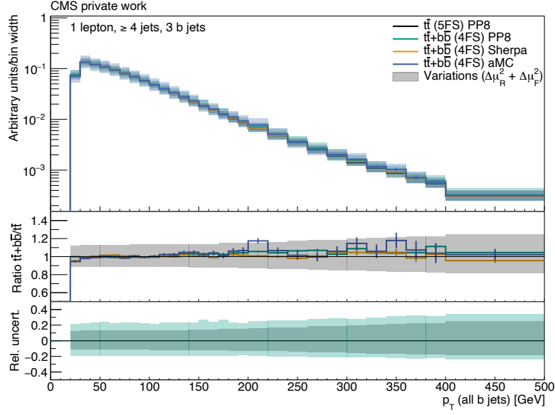
Figure A.3: p_T (all b jets) of the t\bar{t} POWHEG+PYTHIA8 (black), t\bar{t}+b\bar{b} POWHEG+PYTHIA8 (green), t\bar{t}+b\bar{b} SHERPA (orange) and t\bar{t}+b\bar{b} MG5AMC(NLO) (blue) simulated events. The statistical uncertainties are shown as bars. The quadratically summed variations of \mu_R and \mu_F are visualized as bands. All distributions are normalized to an integral value of 1. All events pass the selection “1 lepton, \geq 4 jets, 3 b jets”.
