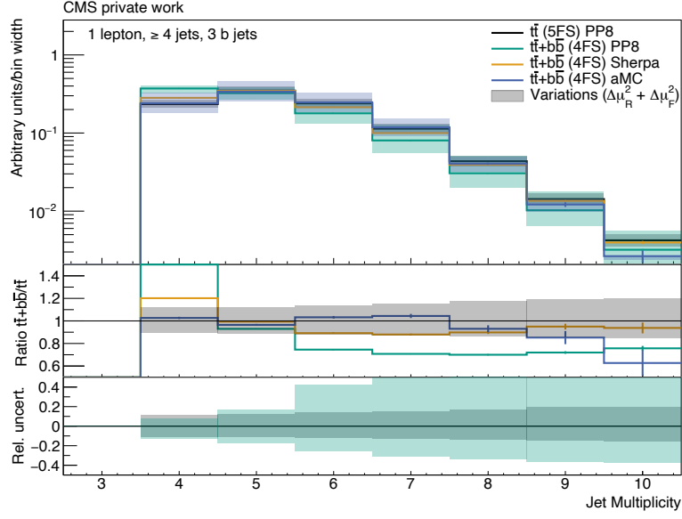
Figure A.1: Jet multiplicity of the t\bar{t} POWHEG+PYTHIA8 (black), t\bar{t}+b\bar{b} POWHEG+PYTHIA8 (green), t\bar{t}+b\bar{b} SHERPA (orange) and t\bar{t}+b\bar{b} MG5AMC-(NLO) (blue) simulated events. The statistical uncertainties are shown as bars. The quadratically summed variations of \mu_R and \mu_F are visualized as bands. All distributions are normalized to an integral value of 1. All events pass the selection “1 lepton, \geq 4 jets, 3 b jets”.
