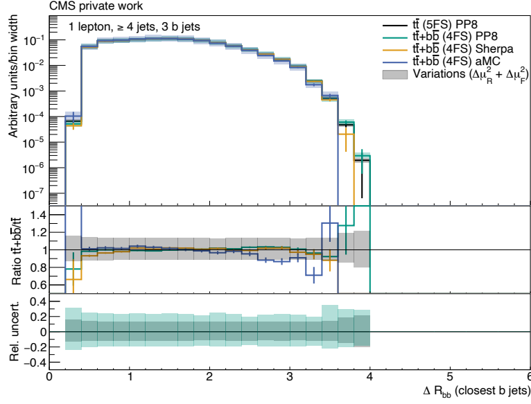
Figure A.11: \Delta R(bb) (closest) of the t\bar{t} POWHEG+PYTHIA8 (black), t\bar{t}+b\bar{b} POWHEG+PYTHIA8 (green), t\bar{t}+b\bar{b} SHERPA (orange) and t\bar{t}+b\bar{b} MG5AMC-(NLO) (blue) simulated events. The statistical uncertainties are shown as bars. The quadratically summed variations of \mu_R and \mu_F are visualized as bands. All distributions are normalized to an integral value of 1. All events pass the selection “1 lepton, \geq 4 jets, 3 b jets”.
