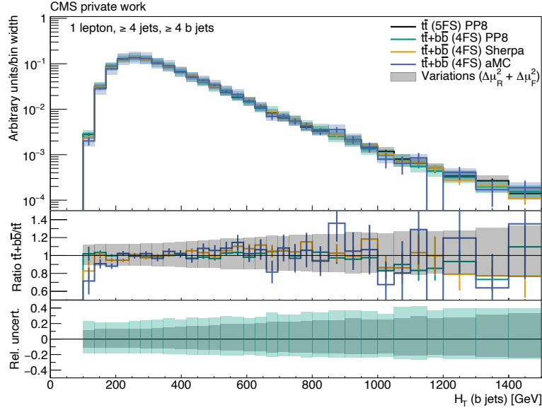
Figure A.22: H_T (b jets) of the t\bar{t} POWHEG+PYTHIA8 (black), t\bar{t}+b\bar{b} POWHEG+PYTHIA8 (green), t\bar{t}+b\bar{b} SHERPA (orange) and t\bar{t}+b\bar{b} MG5AMC(NLO) (blue) simulated events. The statistical uncertainties are shown as bars. The quadratically summed variations of \mu_R and \mu_F are visualized as bands. All distributions are normalized to an integral value of 1. All events pass the selection “1 lepton, \geq 4 jets, \geq 4 b jets”.
