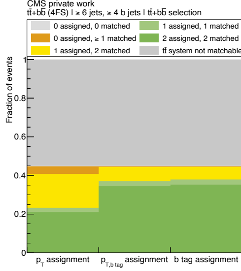
Figure 7.5: Maximum possible efficiency of the p_T , p_{T,b \text{ tag}} and b tag assignment method for the t\bar{t} system reconstruction strategy assuming a perfect DNN reconstruction. It is shown how many additional b jets are assigned in which fraction of events depending on the number of jets assigned via the matching algorithm.
