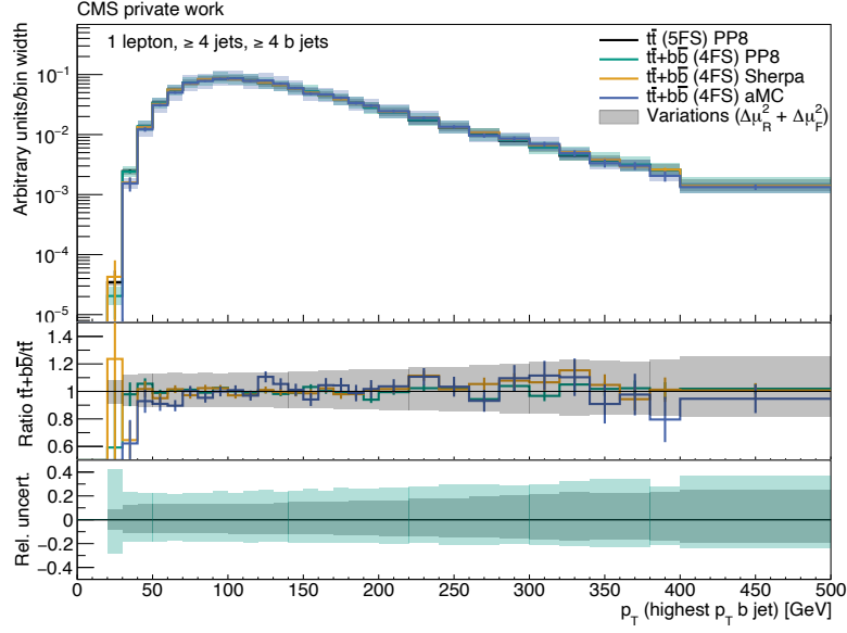
Figure A.17: Leading b jet p_T of the t\bar{t} POWHEG+PYTHIA8 (black), t\bar{t}+b\bar{b} POWHEG+PYTHIA8 (green), t\bar{t}+b\bar{b} SHERPA (orange) and t\bar{t}+b\bar{b} MG5AMC-(NLO) (blue) simulated events. The statistical uncertainties are shown as bars. The quadratically summed variations of \mu_R and \mu_F are visualized as bands. All distributions are normalized to an integral value of 1. All events pass the selection “1 lepton, \geq 4 jets, \geq 4 b jets”.
