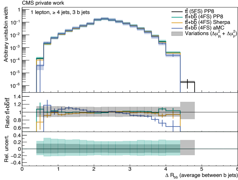
Figure A.10: \Delta R(bb) (average) of the t\bar{t} POWHEG+PYTHIA8 (black), t\bar{t}+b\bar{b} POWHEG+PYTHIA8 (green), t\bar{t}+b\bar{b} SHERPA (orange) and t\bar{t}+b\bar{b} MG5AMC(NLO) (blue) simulated events. The statistical uncertainties are shown as bars. The quadratically summed variations of \mu_R and \mu_F are visualized as bands. All distributions are normalized to an integral value of 1. All events pass the selection “1 lepton, \geq 4 jets, 3 b jets”.
