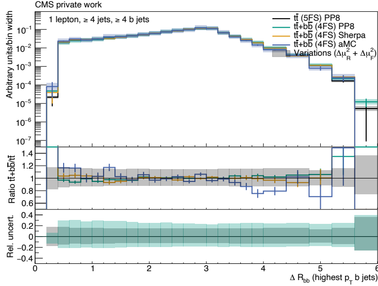
Figure A.24: \Delta R(bb) (leading) of the t\bar{t} POWHEG+PYTHIA8 (black), t\bar{t}+b\bar{b} POWHEG+PYTHIA8 (green), t\bar{t}+b\bar{b} SHERPA (orange) and t\bar{t}+b\bar{b} MG5AMC-(NLO) (blue) simulated events. The statistical uncertainties are shown as bars. The quadratically summed variations of \mu_R and \mu_F are visualized as bands. All distributions are normalized to an integral value of 1. All events pass the selection “1 lepton, \geq 4 jets, \geq 4 b jets”.
