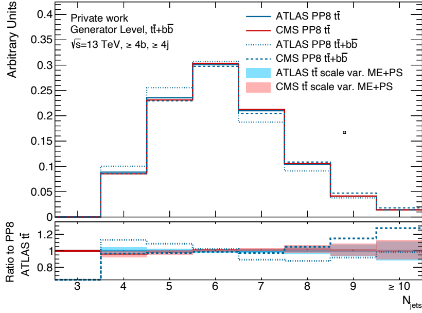
(a) t\bar{t} POWHEG+PYTHIA8 and t\bar{t}+b\bar{b} POWHEG+PYTHIA8 simulations
