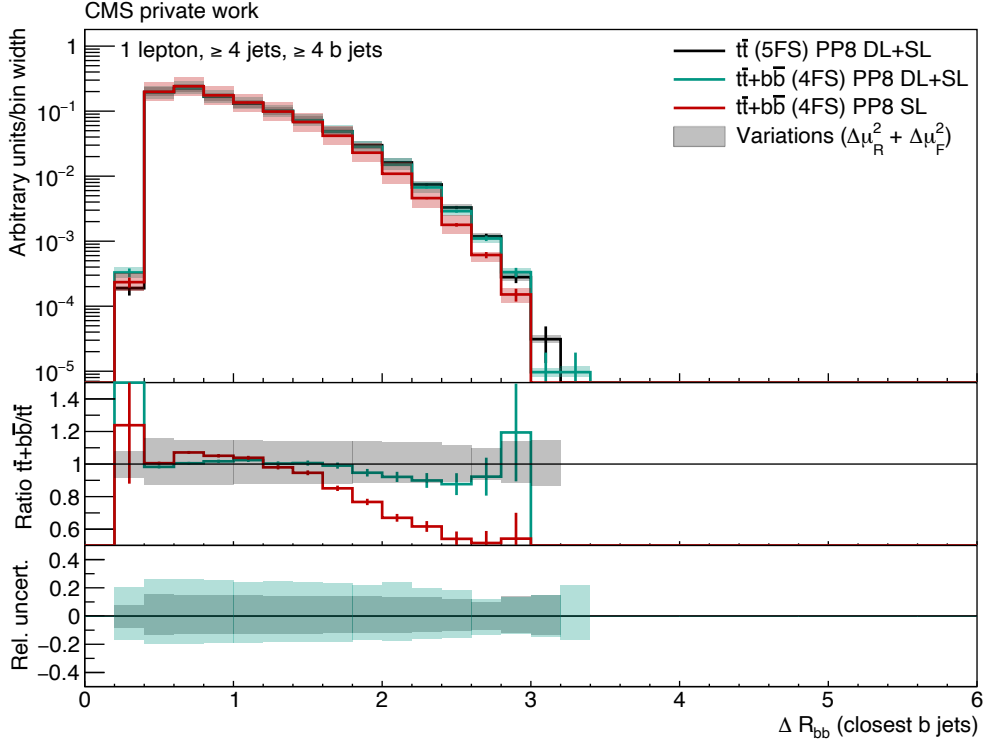
Figure 6.6: \Delta R(bb) (closest) of the t\bar{t} POWHEG+PYTHIA8 (black), t\bar{t}+b\bar{b} POWHEG+PYTHIA8 simulated events in a simulation of the dilepton channel and the single-lepton channel (green), t\bar{t}+b\bar{b} POWHEG+PYTHIA8 simulated events in a simulation of the single-lepton channel only (red). The statistical uncertainties are shown as bars. The quadratically summed variations of \mu_R and \mu_F are visualized as bands. All distributions are normalized to an integral value of 1. All events pass the selection “1 lepton, \geq 4 jets, \geq 4 b jets”.
