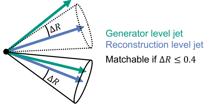
Figure 7.1: Visualization of the matching algorithm between a jet at generator level and a jet at reconstruction level. In the upper case the distance between the two jets is above the \Delta R threshold. In the lower case the distance between the two jets is smaller than the given threshold, therefore these two jets are called matchable.
