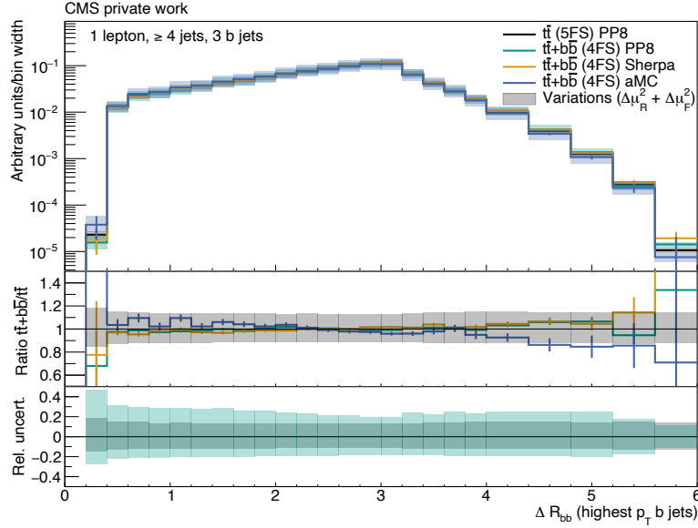
Figure A.12: \Delta R(bb) (leading) of the t\bar{t} POWHEG+PYTHIA8 (black), t\bar{t}+b\bar{b} POWHEG+PYTHIA8 (green), t\bar{t}+b\bar{b} SHERPA (orange) and t\bar{t}+b\bar{b} MG5AMC-(NLO) (blue) simulated events. The statistical uncertainties are shown as bars. The quadratically summed variations of \mu_R and \mu_F are visualized as bands. All distributions are normalized to an integral value of 1. All events pass the selection “1 lepton, \geq 4 jets, 3 b jets”.
