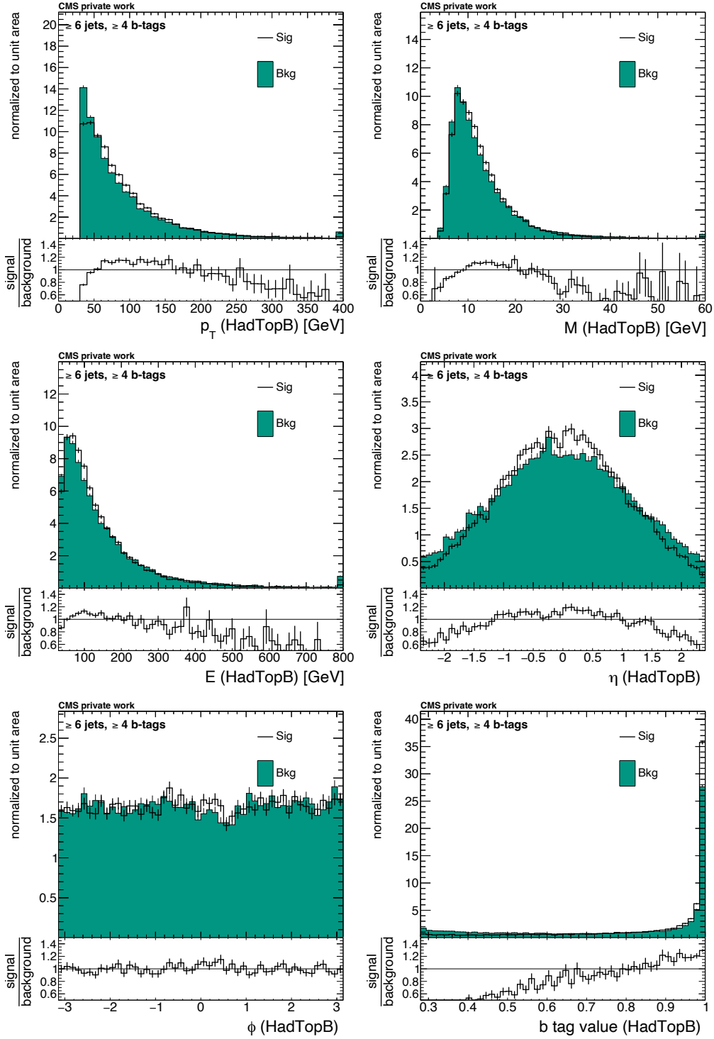
Figure B.27: Input variables of HadTopB for DNN training. The solid line (sig) shows the distribution of the given variable for the correct jet assignment. The histogram (bkg) shows a wrong jet assignment.
