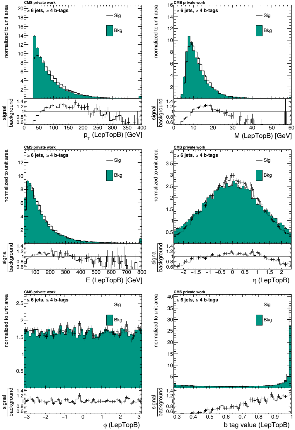
Figure B.28: Input variables of LepTopB for DNN training. The solid line (sig) shows the distribution of the given variable for the correct jet assignment. The histogram (bkg) shows a wrong jet assignment.
