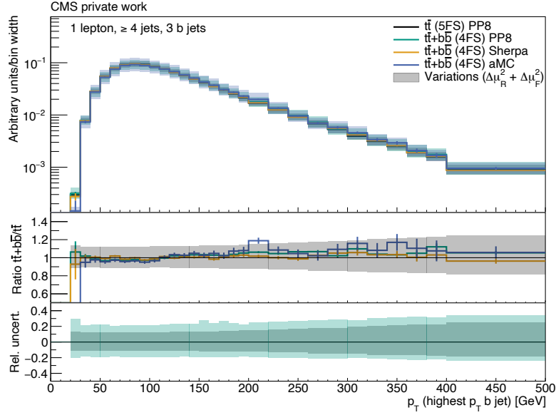
Figure A.4: Leading b jet p_T of the t\bar{t} POWHEG+PYTHIA8 (black), t\bar{t}+b\bar{b} POWHEG+PYTHIA8 (green), t\bar{t}+b\bar{b} SHERPA (orange) and t\bar{t}+b\bar{b} MG5AMC(NLO) (blue) simulated events. The statistical uncertainties are shown as bars. The quadratically summed variations of \mu_R and \mu_F are visualized as bands. All distributions are normalized to an integral value of 1. All events pass the selection “1 lepton, \geq 4 jets, 3 b jets”.
