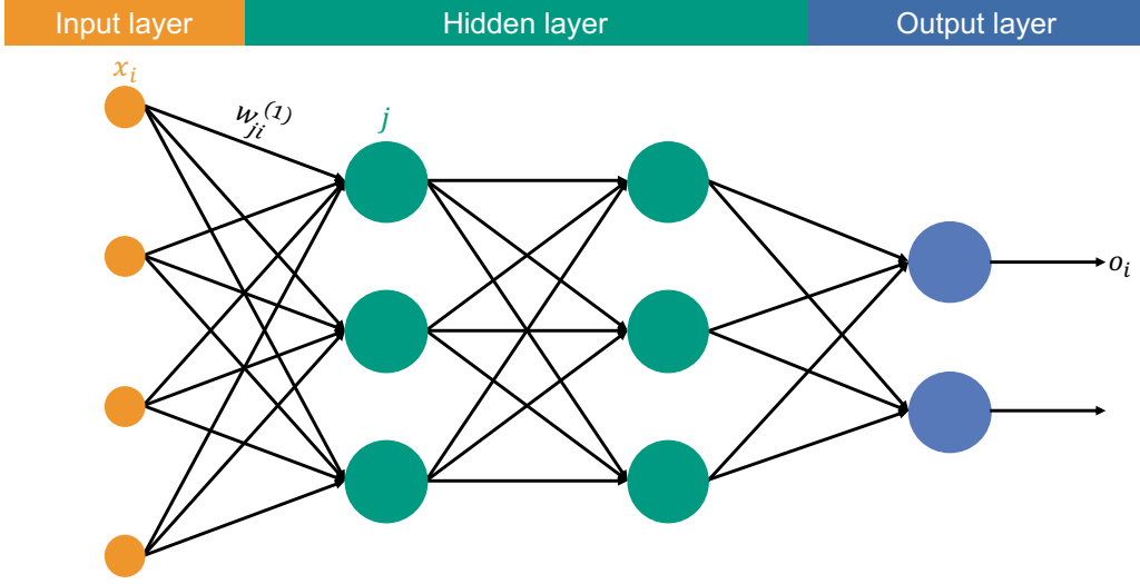
Figure 7.4: Visualization of a deep neural network. On the left side the inputs x_i are shown in the input layer (orange). Two hidden layers are depicted in the center (green). An exemplary weight from the i -th input to the j -th neuron is indicated with w_{ji}^{(1)} . On the right side the output layer with the output value o_i is illustrated (blue).
