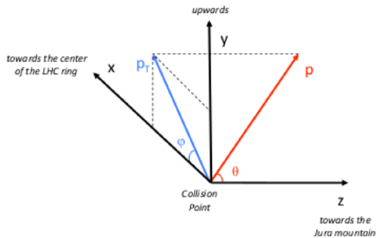
Figure 3.5: The CMS coordinate system.
