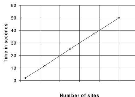
Figure 2: Results of Scalability Tests
