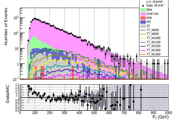
Leading muon p_T distribution after.
