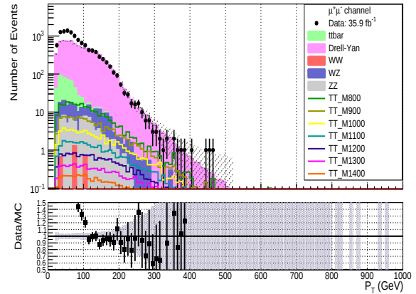
Sub-leading muon p_T distribution after.
