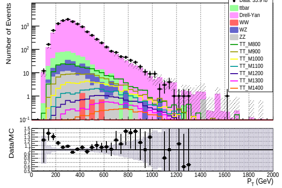
Leading AK4 jet p_T after.
