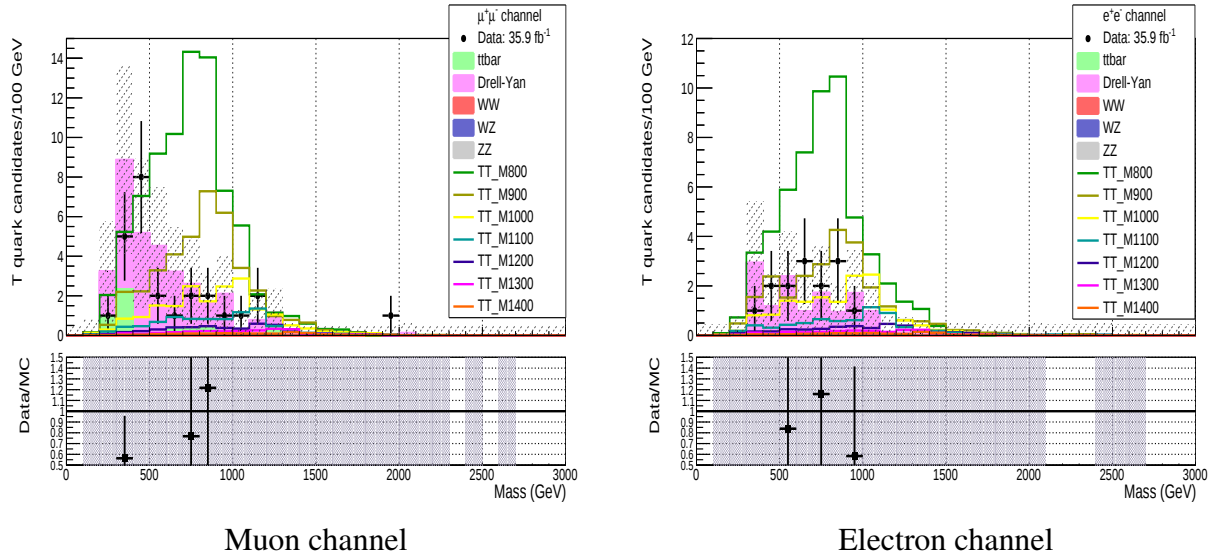
Figure B.1: T mass distribution for \chi^2 < 20 .
