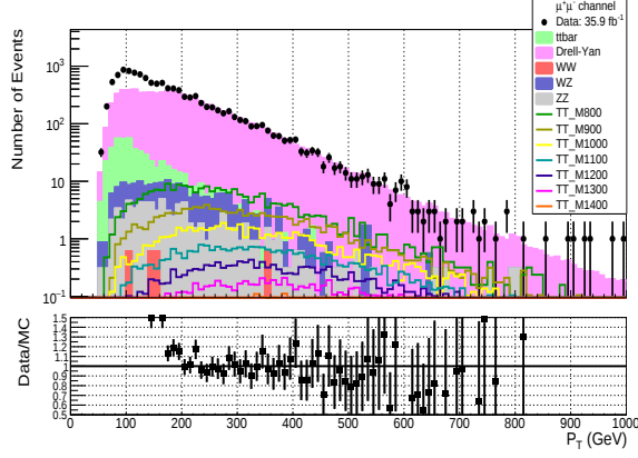
Leading muon p_T distribution before.
