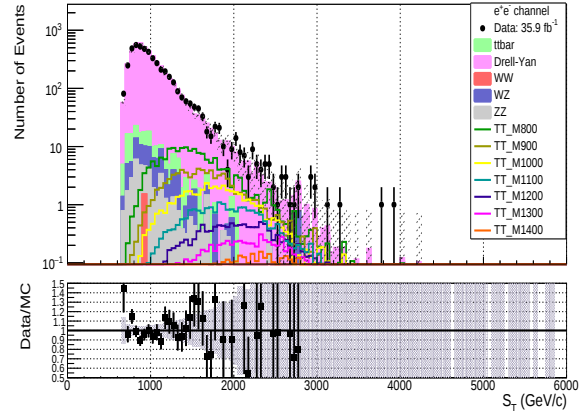
S_T distribution after.
