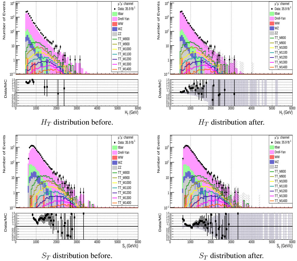
Figure 3.15: (Left) Comparison between the Data and the MC before applying any scale factors. The error bars only reflect the statistical uncertainty. (Right) The Data and MC comparisons after applying the muon identification and isolation scale factors, the trigger scale factors and the Z p_T dependent electroweak correction factors for Drell-Yan. The error band shows both statistical uncertainty as well as the systematic uncertainty on the three scale factors applied along with the theoretical uncertainty on the cross section for the background samples and the uncertainty on the integrated luminosity.
