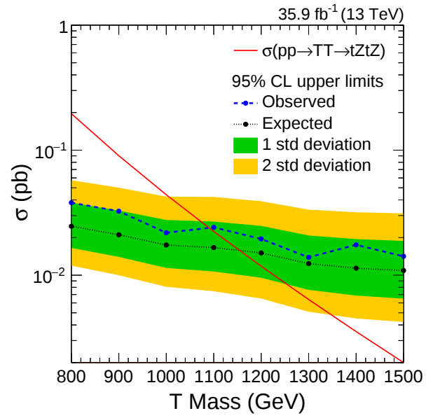
Figure 4.5: The observed and expected limits for TT \rightarrow tZtZ with 100% branching ratio.
