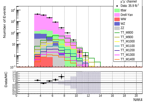
AK4 jet multiplicity after.
