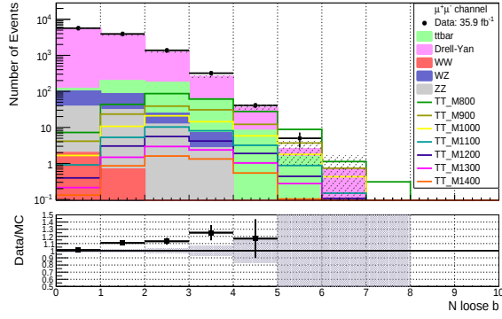
Loose b-jet multiplicity before.
