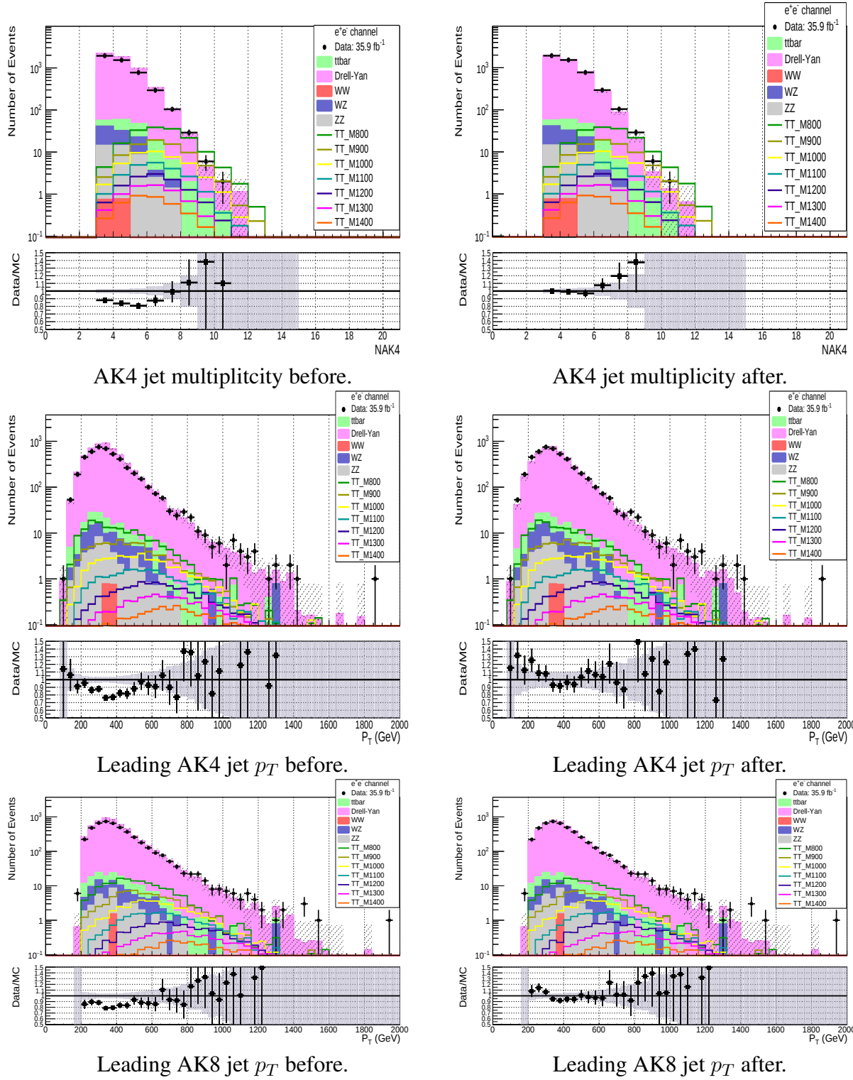
Figure A.3: (Left) The plots show the distribution with just the electron identification and trigger scale factors applied. (Right) The same plots after applying the Z p_T dependent electroweak correction factors to the Drell-Yan sample.
