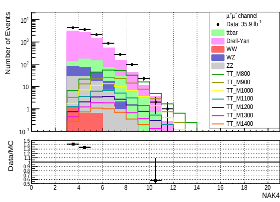
AK4 jet multiplicity before.
