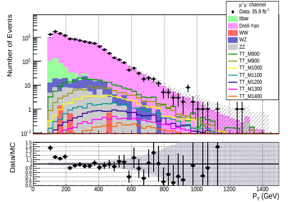
Dimuon p_T distribution after.
