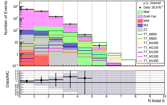
Loose b-jet multiplicity after.
