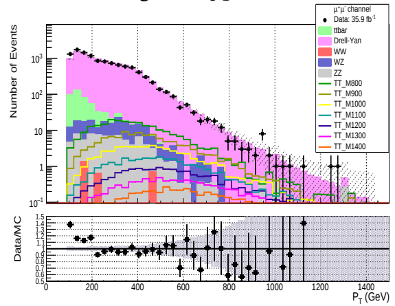
Dimuon p_T distribution after.
