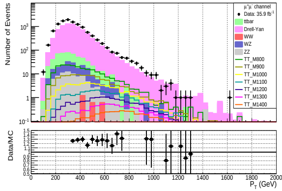
Leading AK4 jet p_T before.
