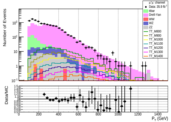
Dimuon p_T distribution before.
