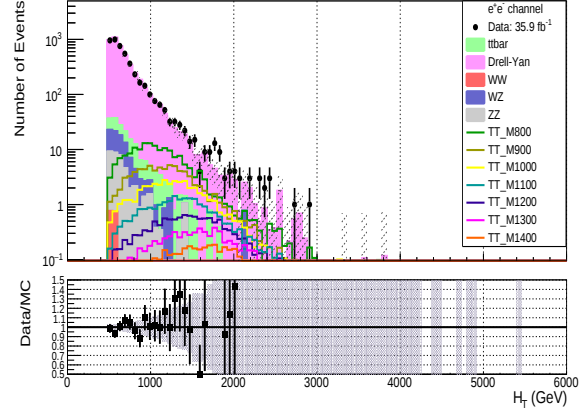
H_T distribution after.
