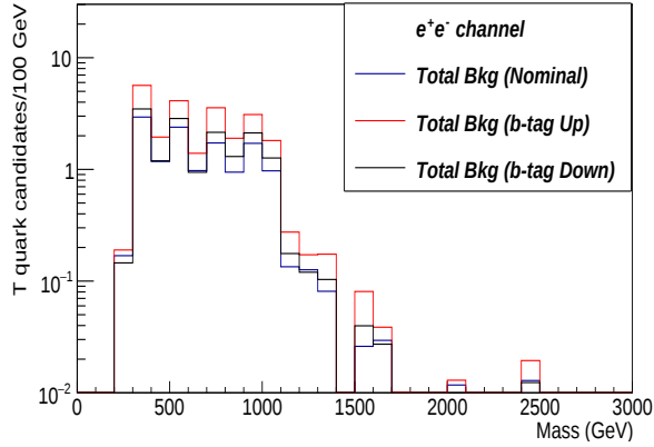
b-tagging systematics for electron channel.
