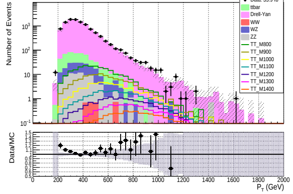
Leading AK8 jet p_T after.
