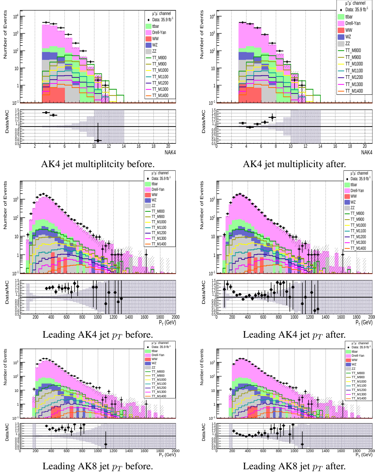
Figure A.7: (Left) The plots show the distribution with just the muon identification and trigger scale factors applied. (Right) The same plots after applying the Z p_T dependent electroweak correction factors to the Drell-Yan sample.
