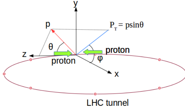
Figure 1.4: Right handed coordinate system used by the CMS.
