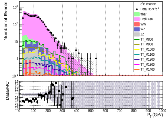
Sub-leading electron p_T distribution after.
