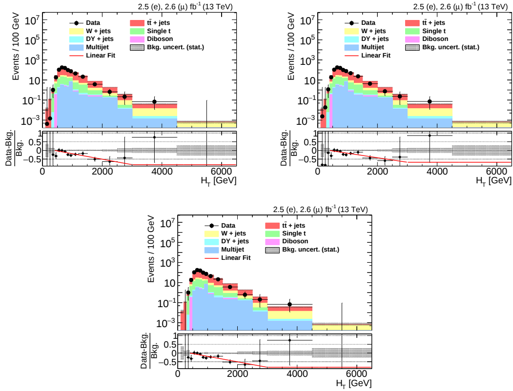
Figure C.8: Comparison of the H_T distributions for three different B\bar{B} hypotheses injected (assuming \mathcal{B}(B \rightarrow tW) = 100\% ): Signal with M(T) = 800\text{ GeV} injected (top left), with M(T) = 1200\text{ GeV} injected (top right) and with M(T) = 1600\text{ GeV} injected (bottom).
