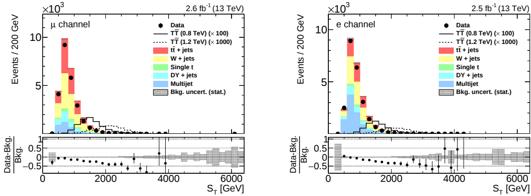
Figure 6.6: N-1 distribution of S_T in the muon (left) and electron (right) channel before applying the S_T > 800 \text{ GeV} requirement. The signal samples are normalised to their theoretically predicted cross section and the intrinsic branching fractions of the samples (33% for each decay mode) are assumed.
