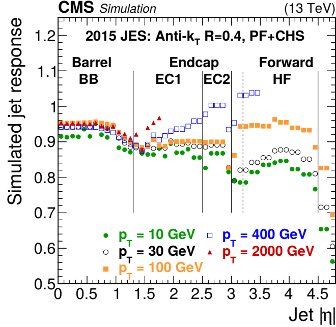
Figure 5.2: Jet response for simulated events at \sqrt{s} = 13 TeV, defined as ratio of the initial parton energy and reconstructed jet energy before any jet energy corrections. The response is shown as a function of the jet |\eta| for jets with varying p_T . Taken from Ref. [184].
