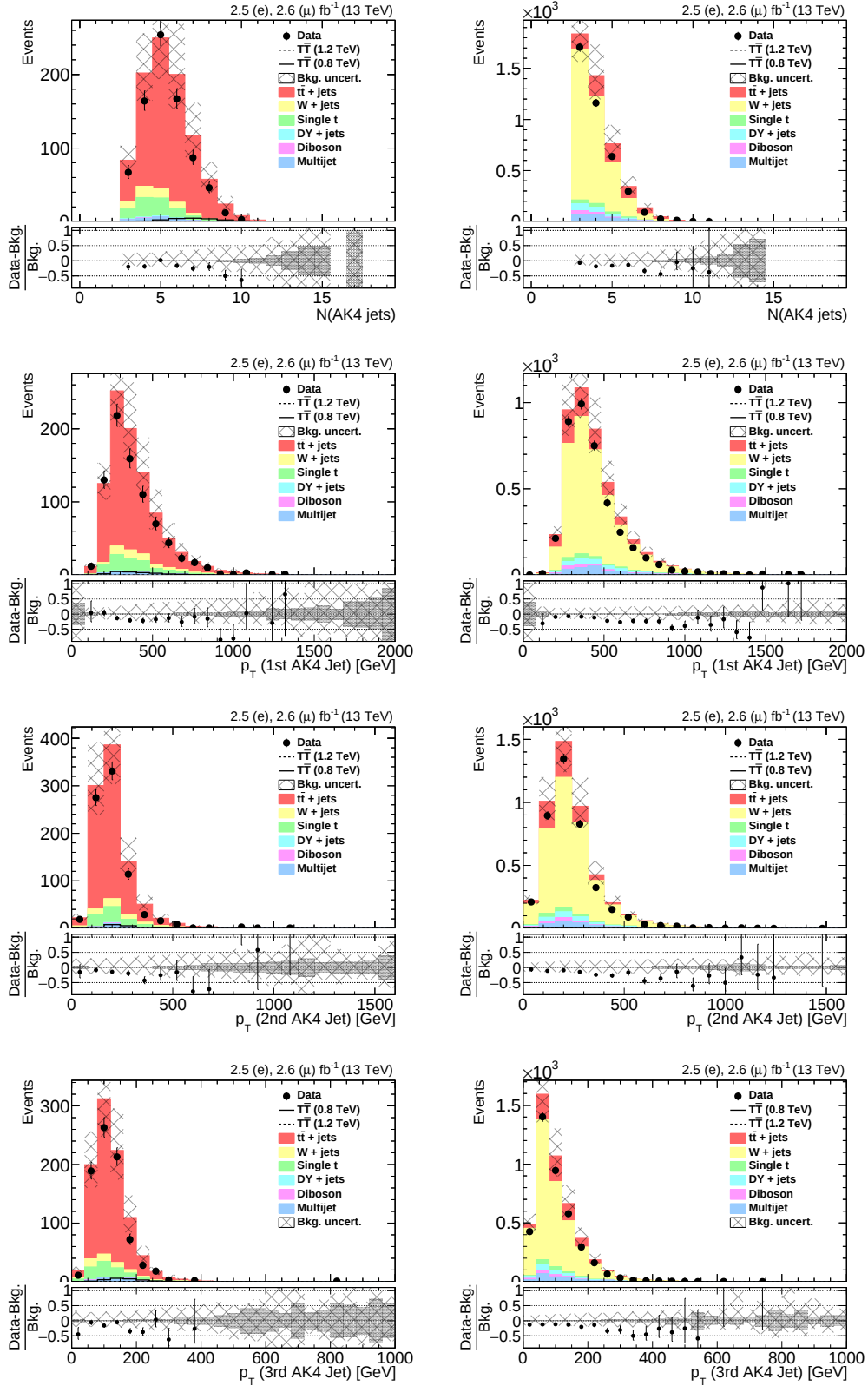
Figure 6.26: Various distributions in the t\bar{t} + jets (left) and W + jets (right) control regions after combining electron and muon channels. From top to bottom the number of AK4 jets and the p_T spectra of the first, second and third AK4 jet (in order of their p_T ) are shown. The statistical uncertainty in the simulation is shown as gray band and the total uncertainty, combining the statistical uncertainty and all systematic uncertainties described in Section 6.4, is shown as hatched band.
