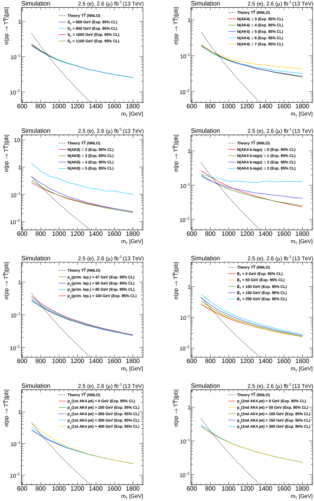
Figure B.2: Expected sensitivities when varying various kinematic variables. From top left to bottom right: S_T , N(\text{AK4 jets}) , N(\text{AK8 jets}) , N(b\text{-tagged AK4 jets}) , p_T(\text{prim. lep.}) , \cancel{E}_T , p_T(1\text{st AK4 jet}) , p_T(2\text{nd AK4 jet}) .
