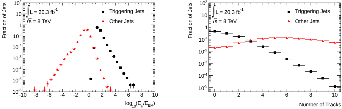
Figure 6.4: Distribution of \log_{10}(E_H/E_{EM}) (left) and the number of tracks with p_T > 1 \text{ GeV} within \Delta R < 0.2 (right) of triggering (black) and non-triggering (red) jets. The offline cut flow requires both jets have \log_{10}(E_H/E_{EM}) > 1.2 and that they are trackless.
