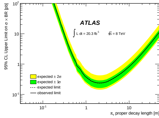
(a) m_\Phi = 300 GeV, m_{\pi_v} = 50 GeV.
