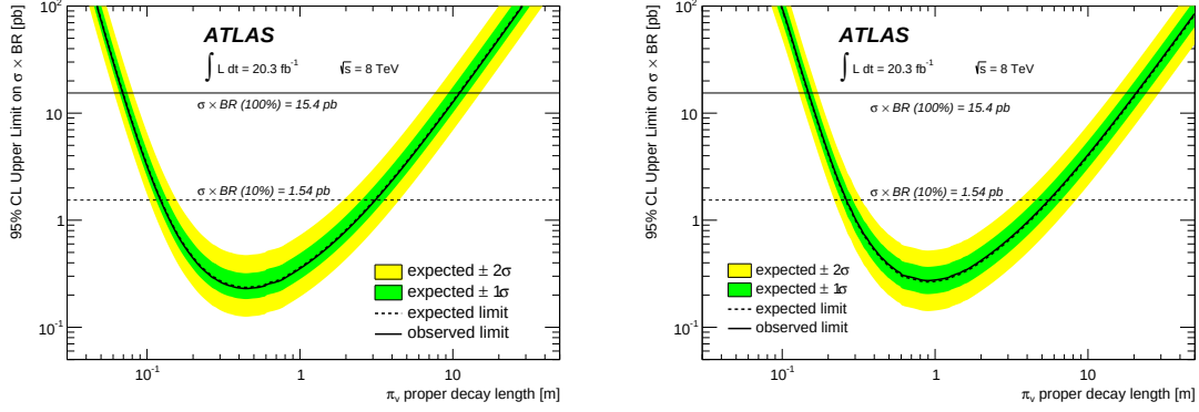
(a) m_\Phi = 140 GeV, m_{\pi_v} = 10 GeV.
