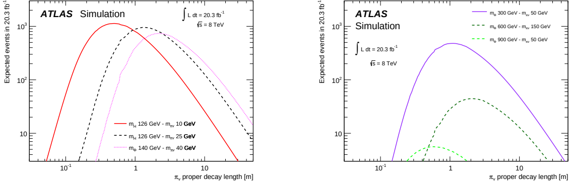
Figure 6.8: The number of events expected to survive the full analysis cut flow for a range of low mass (left) and high mass (right) signal samples. The number of events strongly depends on the proper lifetime of the LLP, which is unconstrained by the signal model.
