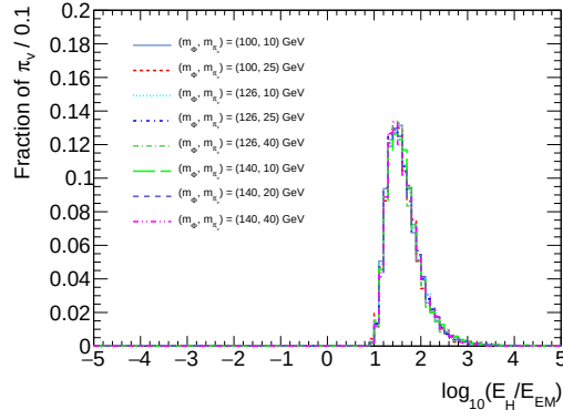
(a) Low \Phi masses, triggering \pi_\nu
