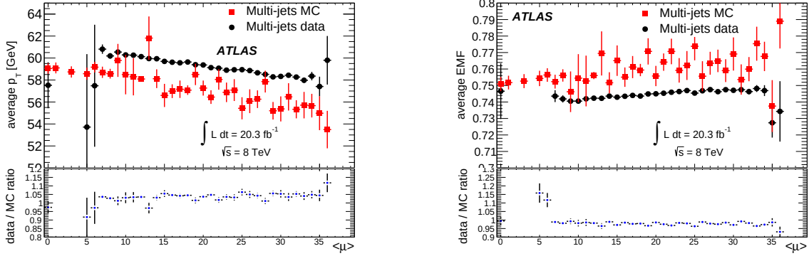
Figure 5.28: The pileup dependence of jet p_T (left) and jet EMF (right). A linear fit is made to the ratio of data to MC and its slope is used to propagate the variation of the parameter in the MC samples.
