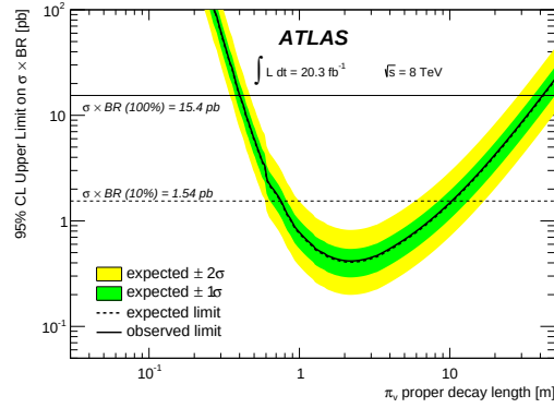
(a) m_\Phi = 140 GeV, m_{\pi_v} = 10 GeV.
