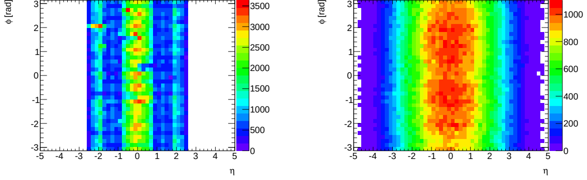
Figure 6.1: Distribution of \phi vs \eta of, on the left, triggering jets and, on the right, non-triggering jets in events with one triggering jet. A jet is identified as a triggering jet if \Delta R < 0.2 between the jet and the CalRatio trigger object. All jets have an E_T > 40 GeV cut applied.
