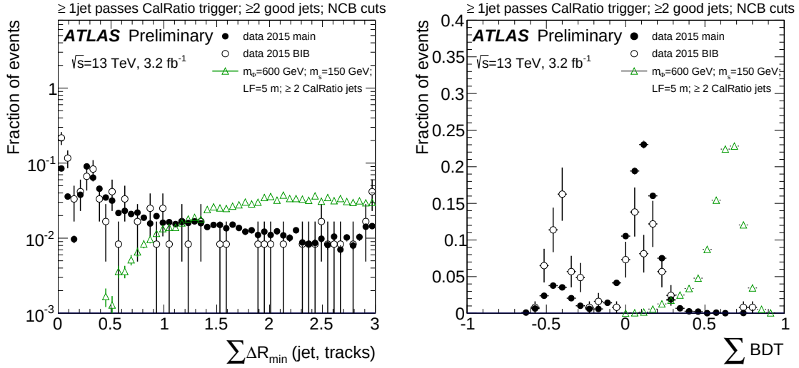
Figure 7.6: The \sum \min \Delta R(jet, tracks) (left) and \sum BDT (right) distributions for jets from the main, BIB and example signal samples. The NCB cuts leave too few events in the cosmic and SM multijet samples to include them in the plots. Only signal MC events with two candidate signal jets are shown.
