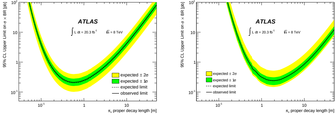
(a) m_\Phi = 900 GeV, m_{\pi_v} = 50 GeV.
