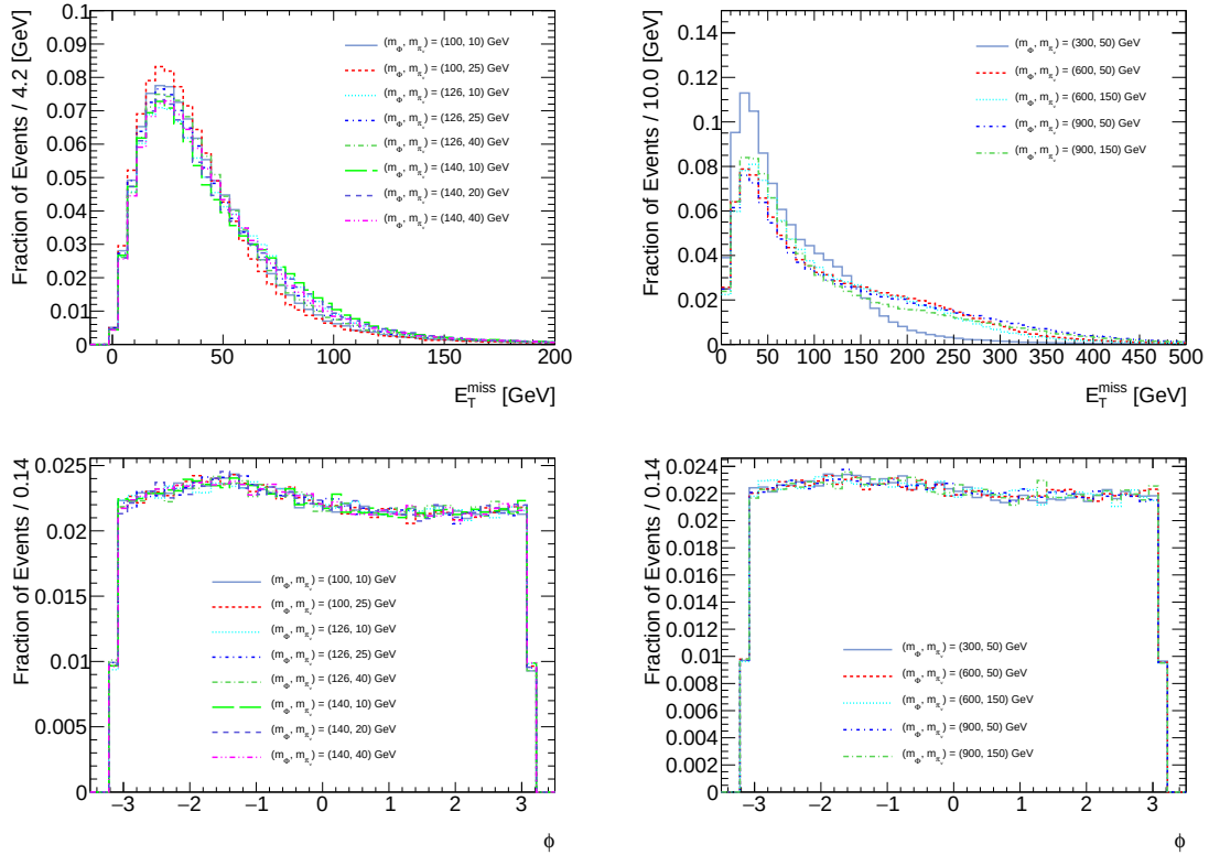
Figure 4.4: The E_T^{\text{miss}} and E_T^{\text{miss}} \phi distributions of the low mass (left) and high mass (right) \Phi samples.
