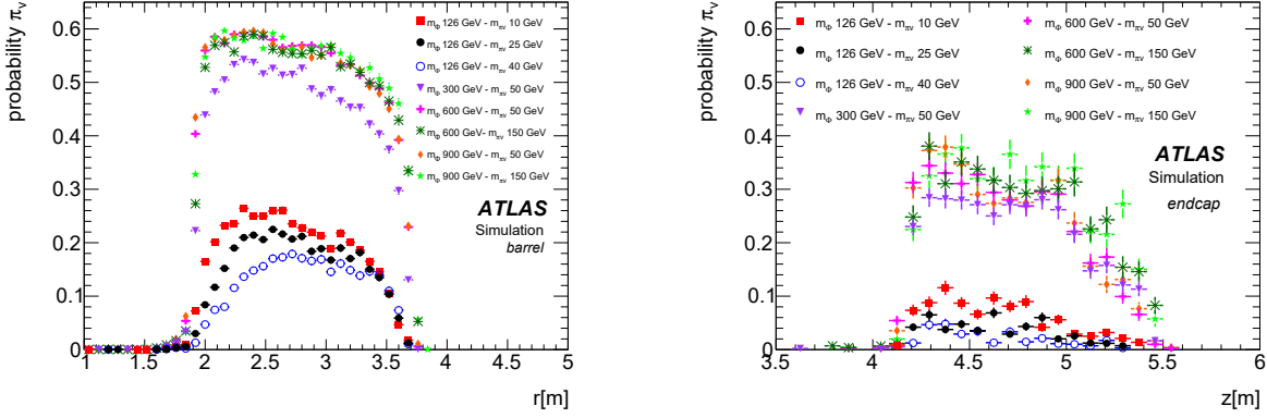
Figure 5.3: Distribution of the probability that a \pi_v decaying in the HCal will fire the CalRatio trigger for decays in (a) the barrel (b) the endcaps for the high mass signal samples. The m_\Phi = 126 GeV samples are shown for comparison.
