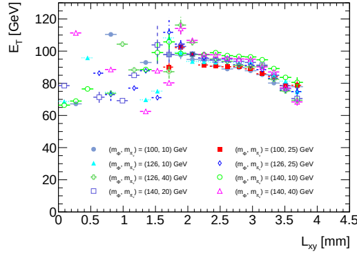
(a) Low \Phi masses, triggering \pi_v
