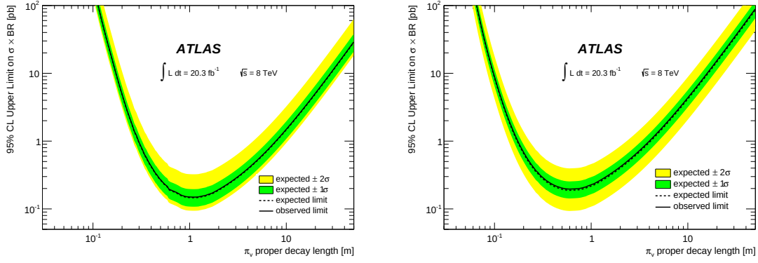
(a) m_\Phi = 300 GeV, m_{\pi_v} = 50 GeV.
