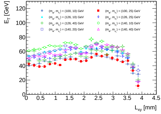
(b) Low \Phi masses, non-triggering \pi_v
