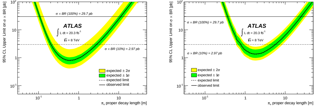
(a) m_\Phi = 100 GeV, m_{\pi_v} = 10 GeV.
