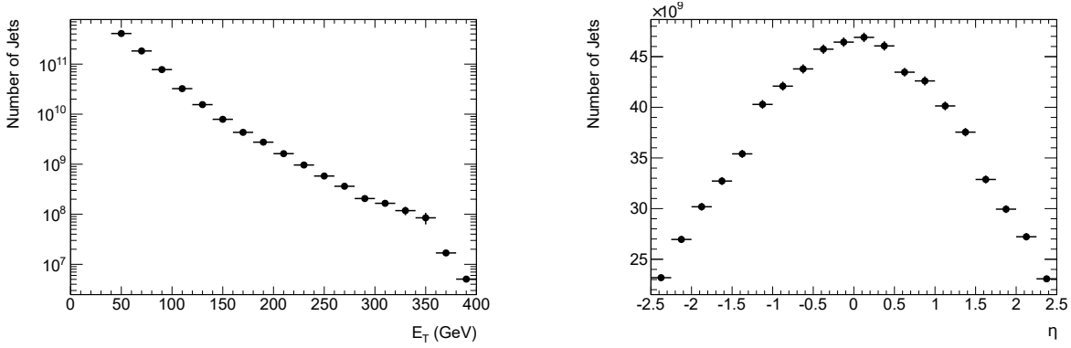
Figure 5.16: Probe jet E_T (left) and \eta (right) after application of the event prescales.
