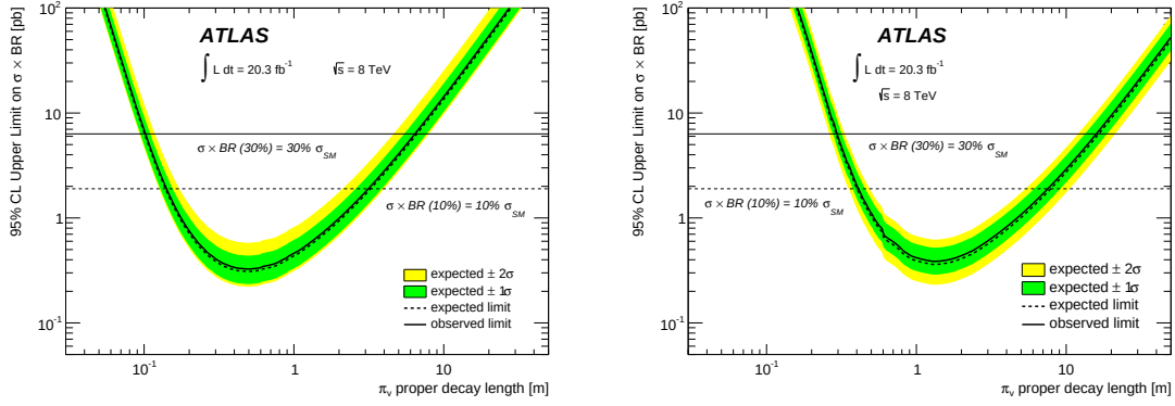
(a) m_\Phi = 126 GeV, m_{\pi_v} = 10 GeV.
