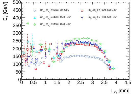
(c) High \Phi masses, triggering \pi_v
