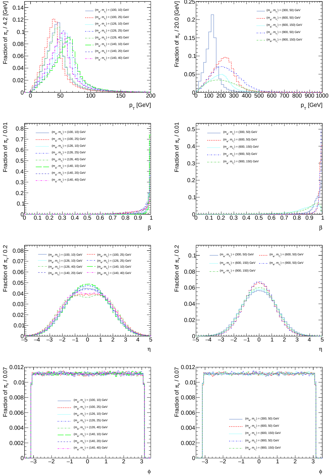
Figure 4.2: Kinematic distributions of the \pi_v produced in the low mass (left) and high mass (right) \Phi samples.
