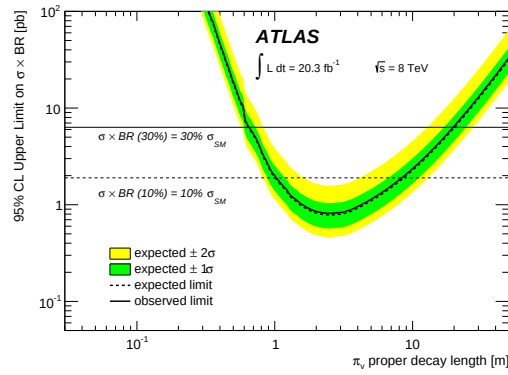
(a) m_\Phi = 126 GeV, m_{\pi_v} = 10 GeV.
