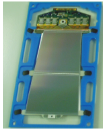
Figure 3.5: A SCT end-cap module
