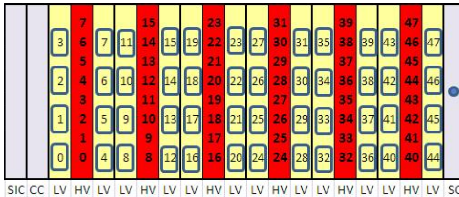
Figure 3.6: The power-supply crate for the SCT.
