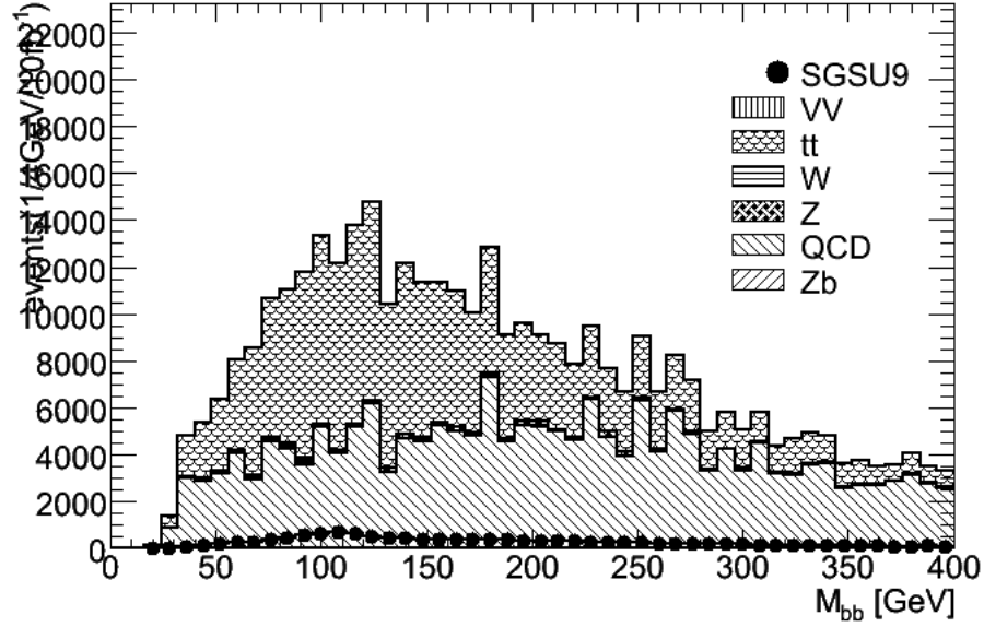
Figure 5.8: Invariant mass of all tagged b -jets for different standard model processes with the cuts in table 5.2 applied and a b -tagging efficiency of 60%.
