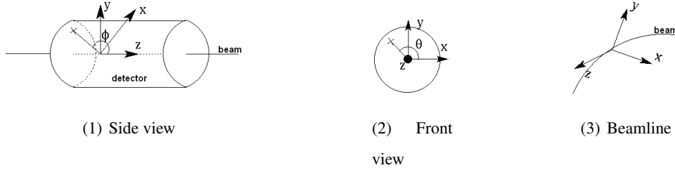
Figure 3.2: The coordinate system used in the detectors at LHC.
