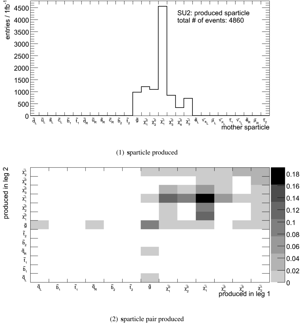
Figure 4.11: (1): The multiplicity of the initially produced sparticles and (2): the various pairs of produced sparticles from each leg per event. Since this scenario has very heavy squarks the production of gauginos dominate, especially \tilde{\chi}_1^\pm pair are produced at high rate.
