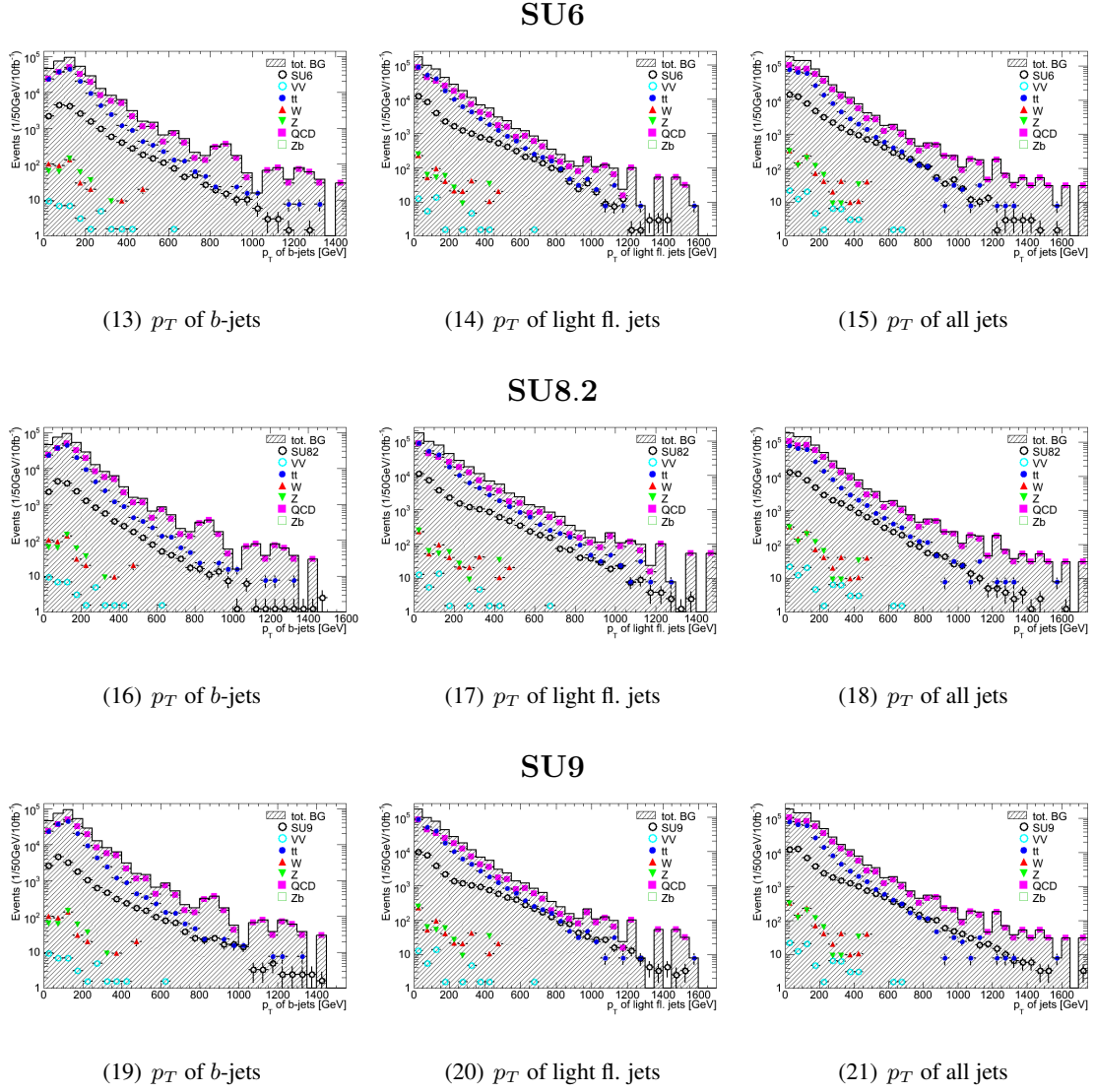
Figure 5.21: The p_T of the different types of jets in each event for the various signal samples and SM backgrounds. The distributions for both signal and SM background (i.e the dominant ones, t\bar{t} and QCD) is very similar. The other SM backgrounds contains much less high p_T jets.
