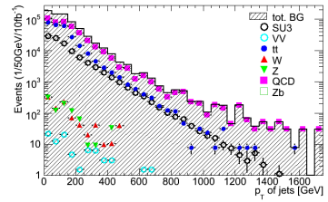
(9) p_T of all jets
