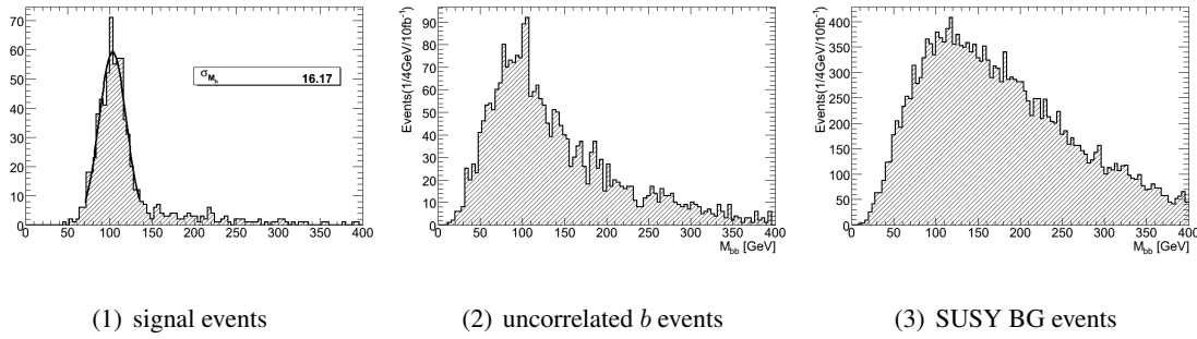
Figure 5.1: Invariant mass of reconstructed b\bar{b} pairs in the different categories of SUSY events in the SU1 scenario.
