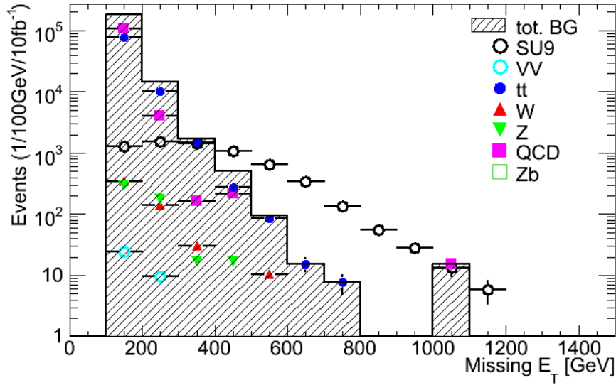
Figure 5.3: The \cancel{E}_T distribution for the SU9 and the Standard Model background. As expected the SU9 peaks at higher values and has longer tails than most of the Standard Model backgrounds. The Standard Model backgrounds with most \cancel{E}_T are the W , Z and t\bar{t} samples, where the decay of the vector bosons and W s from top involves neutrinos.
