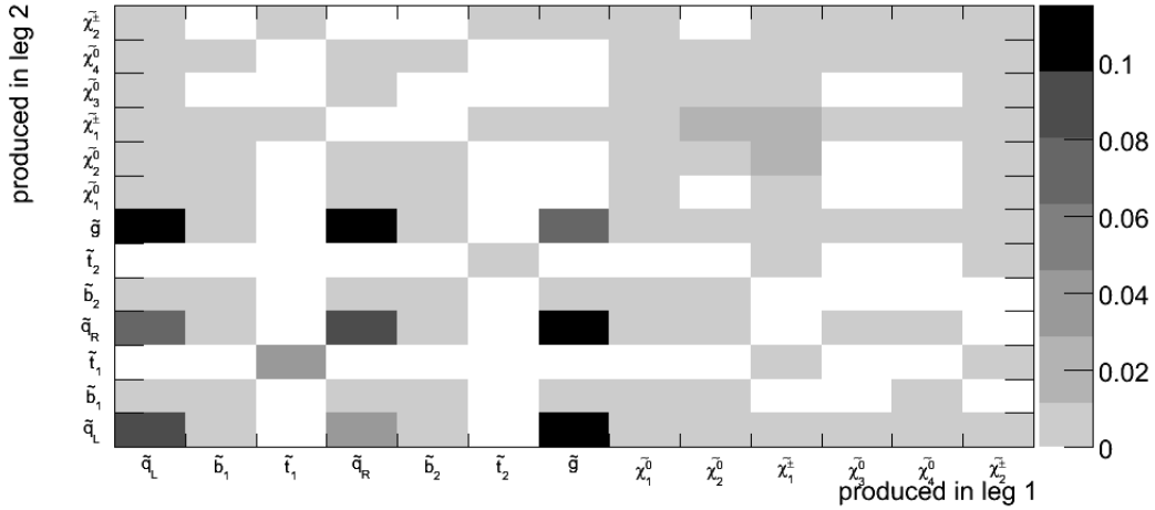
(1) sparticle produced
