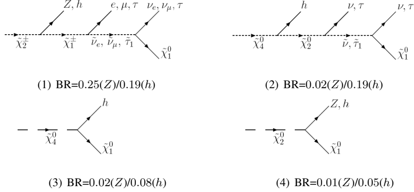
Figure 4.6: The different diagrams for Z and h production in the signal sample SU1 . The branching ratio (BR) for the sparticle to decay into h or Z is presented under the graph.
