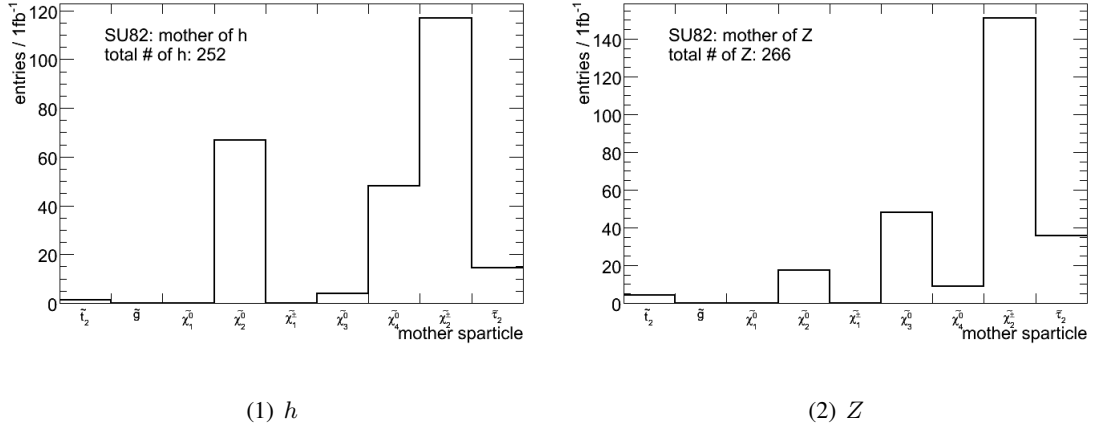
Figure 4.25: The mother of the produced Z and h bosons in the signal sample SU8.2 for 1\text{fb}^{-1} .
