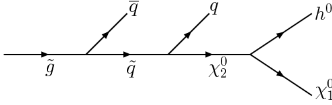
Figure 4.2: A typical cascade of supersymmetric particles producing a Higgs
