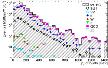
(1) p_T of b -jets
