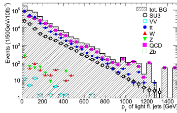
(8) p_T of light fl. jets
