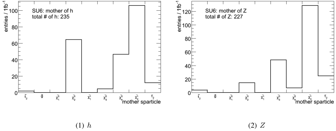
Figure 4.21: The mother of the produced Z and h bosons in the signal sample SU6 for 1\text{fb}^{-1} .
