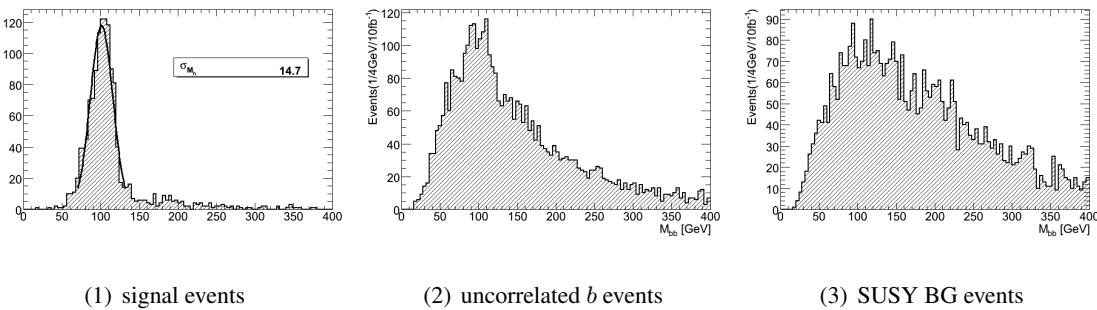
Figure 5.2: Invariant mass of reconstructed b\bar{b} pairs in the different categories of SUSY events in the SU9 scenario.
