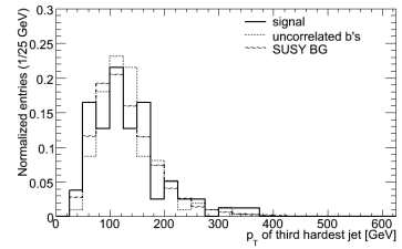
(9) p_T of third hardest jet
