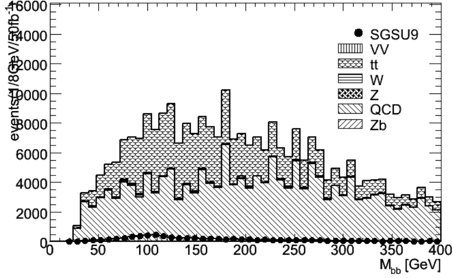
Figure 5.16: Invariant mass of all tagged b -jets for different standard model processes with the cuts in table 5.6 applied and a b -tagging efficiency of 60%. Compared with the corresponding plot in figure 5.13 we see that CUT 4 reduces the SM background. Although CUT 4 is most efficient in removing the combinatorial SUSY background.
