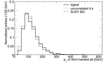
(3) p_T of third hardest jet
