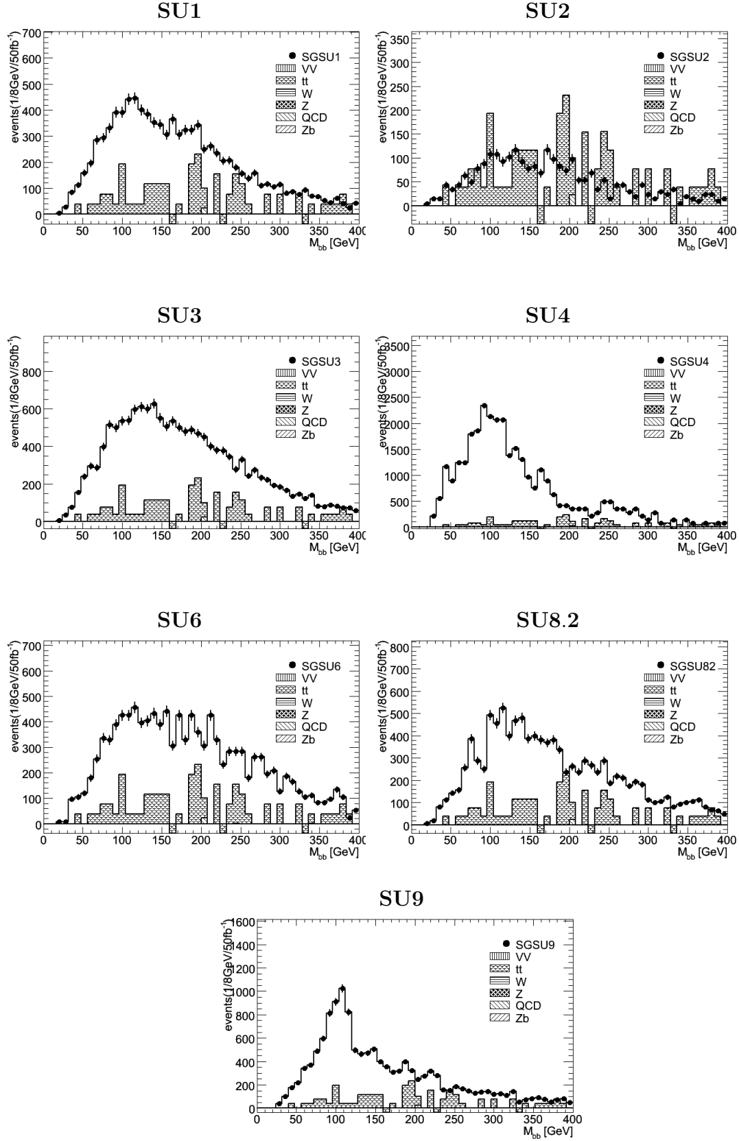
Figure 6.1: The invariant mass plots for the various signal scenarios and SM background with the cuts in table 6.1 applied and requiring both of the additional jets to be light jets.
