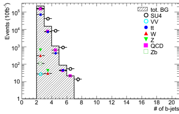
(10) # of b -jets
