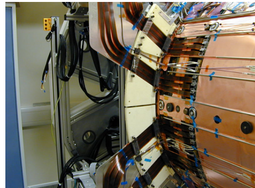
Figure 3.10: the LMTs are connected to the modules of the SCT detector
