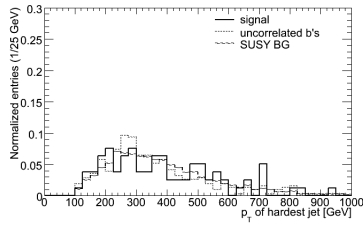
(7) p_T of hardest jet
