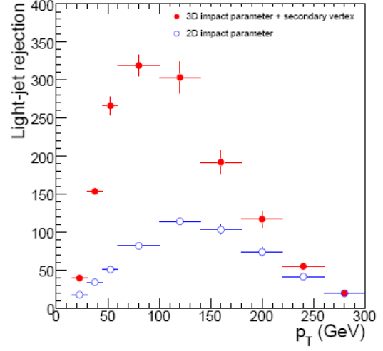
Figure 5.10: The rejection of light jets (not c -jets) as a function of the transverse momentum for two different b -tagging algorithm. Both are showed with a b -tagging efficiency of 60%. The filled dot is the algorithm which is used in this analysis. Sometimes a requirement of the maximum p_T of the b -jets is also used, since the light jet rejection decreases at high p_T . Plot taken from [1]
