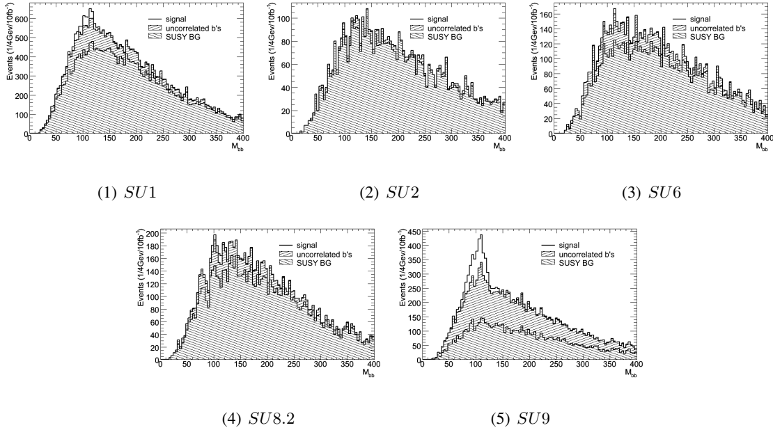
Figure 5.7: Invariant mass of all tagged jets in the different signal scenarios after the cuts in table 5.2 are applied and a b -tagging efficiency of 60%. In SU9 a peak around the Higgs mass is already dominant.
