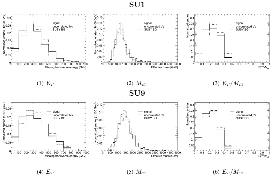
Figure 5.19: The \cancel{E}_T , M_{\text{eff}} and \cancel{E}_T/M_{\text{eff}} for the SU1 (top) and SU9 (bottom) scenarios. Signal and SUSY background shapes are similar. This illustrates the fact that the use of these variables do not improve the significance of the Higgs signal relative to the combinatorial and SUSY backgrounds.
