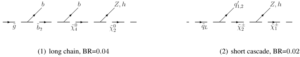
Figure 4.20: Two of the main cascades of supersymmetric particles that lead to a h/Z production in SU4 . The branching ratios for the first decay in each graph is presented. For the short cascade the only possibility is a down squark since the up squark has BR \sim 0
