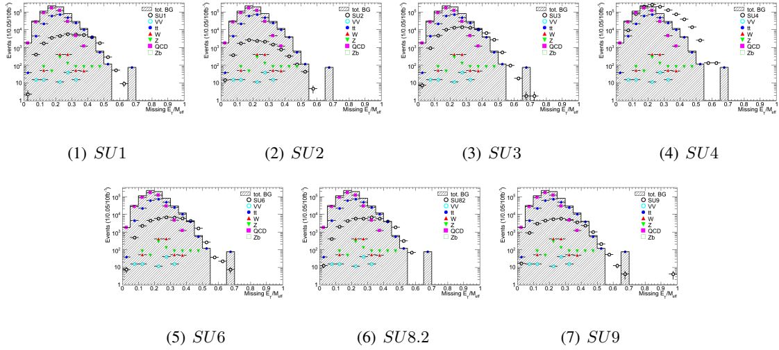
Figure 5.24: \cancel{E}_T/M_{\text{eff}} for the standard model background and signal after the cuts in table 5.11 with an integrated luminosity of \mathcal{L} = 10\text{fb}^{-1} . Again we see a SM background event at high value due to the scaling, as discussed earlier
