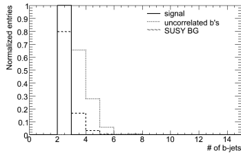
(7) # of b -jets
