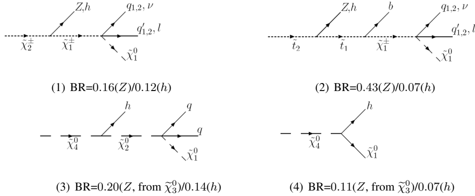
Figure 4.18: The different diagrams for Z and h production in the signal sample SU4 . (1) is probable both for h and Z production while (2) is dominant for Z production. The Z has similar diagrams (3) and (4) as h provided \tilde{\chi}_4^0 is replaced with \tilde{\chi}_3^0
