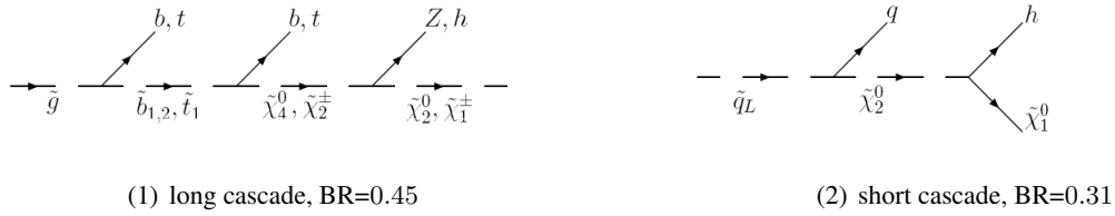
Figure 4.28: Two of the main cascades of supersymmetric particles that lead to a h production in SU8.2 . This is similar cascades as for SU1 and SU6 , but with different branching ratios. The branching ratio for the first decay in each cascade is presented.
