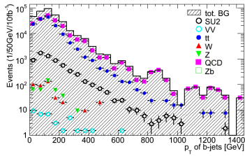
(4) p_T of b -jets
