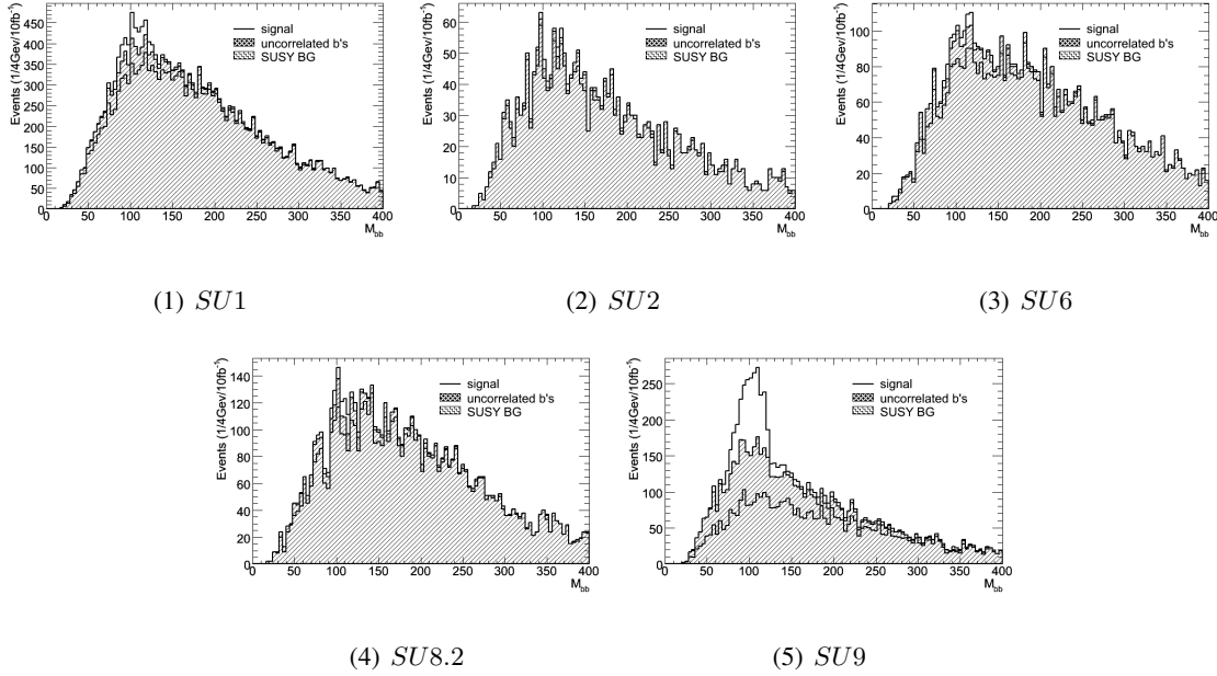
Figure 5.15: Invariant mass of all tagged jets in the different signal scenarios after the cuts in table 5.6 are also applied together with a b -tagging efficiency of 60%. By adding CUT 4 we remove much of the combinatorial background and the uncorrelated SUSY background while the signal stays the same.
