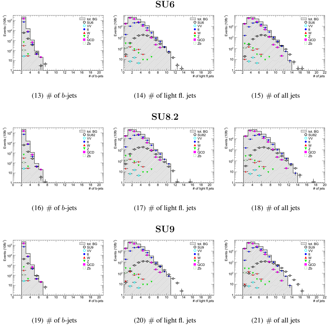
Figure 5.17: The number of b -jets, light jets and the total number of jets in the various signal samples and for the SM backgrounds. The SUSY signals have high jet multiplicity compared with most of the SM background, except t\bar{t} and QCD which also contains many jets. This is after the cuts in table 5.6 are applied. \mathcal{L} = 10fb^{-1}
