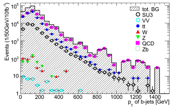
(7) p_T of b -jets
