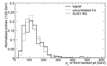
(12) p_T of third hardest jet
