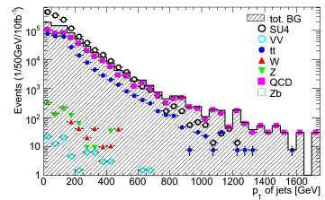
(12) p_T of all jets
