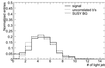
(8) # of light fl. jets
