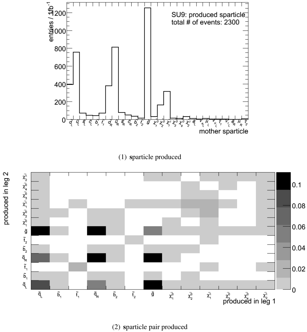
Figure 4.30: (1): The multiplicity of the initially produced sparticles and (2): the various pairs of produced sparticles from each leg per event
