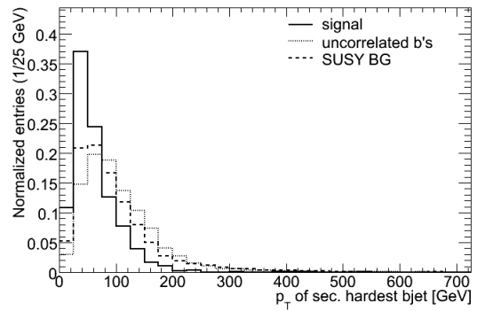
(2) second hardest b -jet
