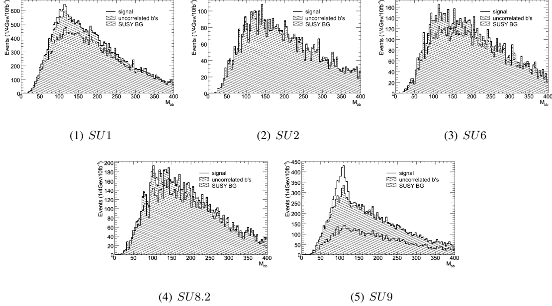
Figure 5.12: Invariant mass of all tagged jets in the different signal scenarios after the cuts in table 5.4 are applied and a b -tagging efficiency of 60%. These plots are very similar to the ones in 5.7, which illustrate that CUT 3 does not remove much of the signal or the other event categories. Although this cut removes a factor of \sim 80\% of the SUSY background, since this background contains many events without b -jets at all (but this will not be clear from these plots, since they only show events with at least two b -jets).
