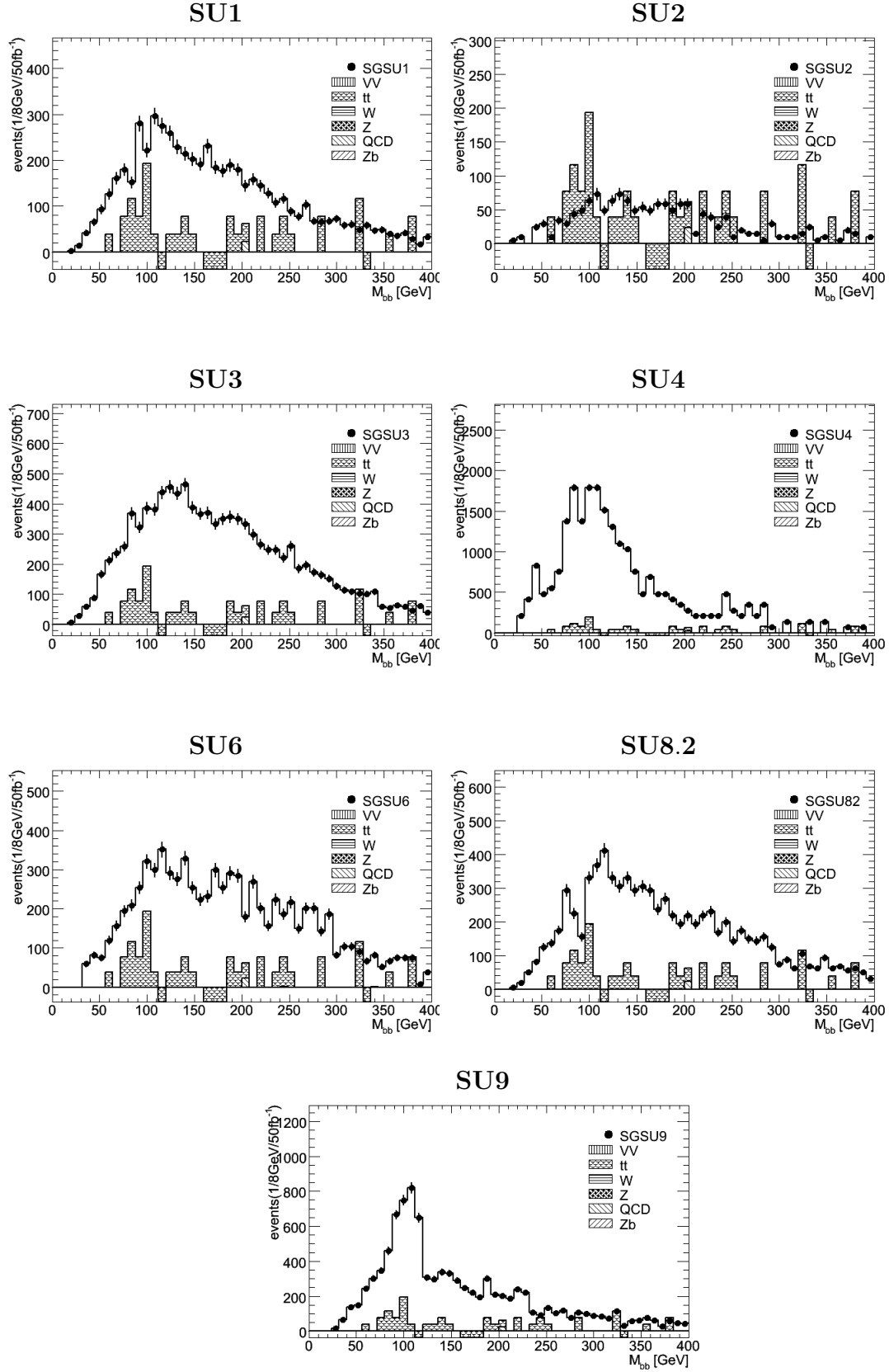
Figure 6.3: The invariant mass plots for the various signal scenarios and SM background with the cuts i table 6.1 requiring both of the additional jets to be a light jet and a lepton veto.
