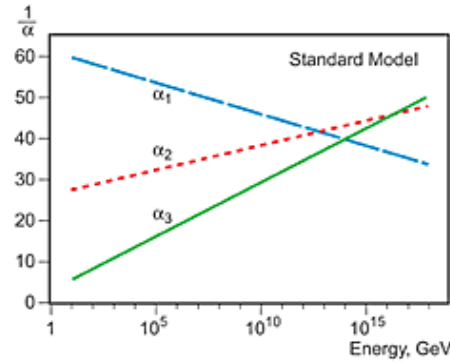
Figure 2.2: The evolution of the coupling constants according to the SM
