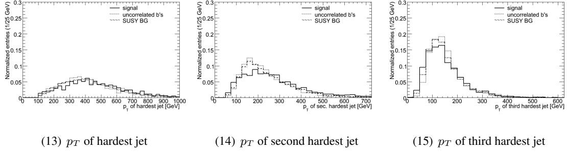
Figure 5.22: The hardest, second hardest and third hardest jet in each event for the different signal samples after the cuts in table 5.7.
