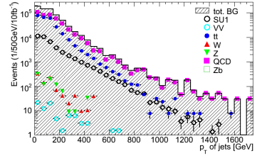
(3) p_T of all jets
