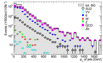
(6) p_T of all jets
