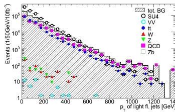
(11) p_T of light fl. jets
