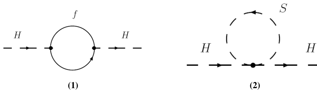
Figure 2.1: Loop corrections to the Higgs mass from fermion loops (1) and scalar loops (2).
