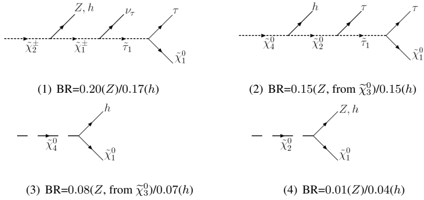
Figure 4.22: The different diagrams for Z and h production in the signal sample SU6 . The Z has similar diagrams (2) and (3) as h provided \tilde{\chi}_4^0 is replaced with \tilde{\chi}_3^0 . The branching ratio for the first decay in each graph is presented.
