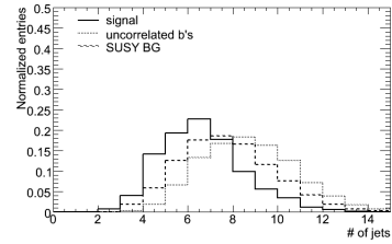
(15) # of all jets
