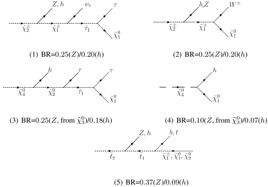
Figure 4.14: The different diagrams for Z and h production in the signal sample SU3 . The Z has similar diagrams (3) and (4) as h provided \tilde{\chi}_4^0 is replaced with \tilde{\chi}_3^0 . Branching ratios for the first decay in each graph is presented
