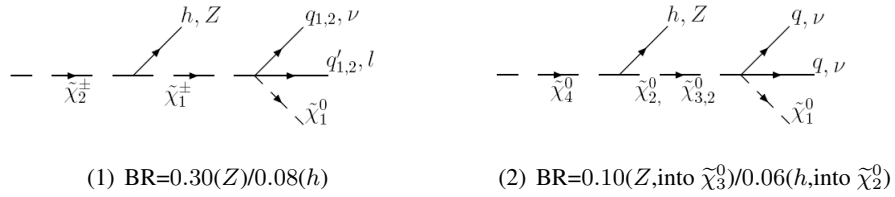
Figure 4.10: The different diagrams for Z and h production in the signal sample SU2 . The branching ratio for the decay is shown under the graph. The decay of \tilde{\chi}_2^0 into \tilde{\chi}_1^0 and h or Z has BR=0.01(Z)/0.002(h)
