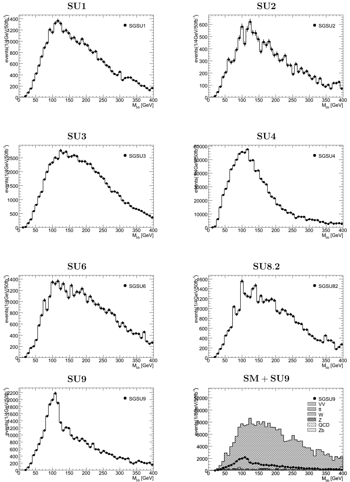
Figure 5.25: The invariant mass of selected b pairs in all the SUSY scenarios after the cuts in 5.11 is applied and with an integrated luminosity of 50 \text{ fb}^{-1} . At the lower right the SU9 signal and SM background is plotted to illustrate that the SM still is dominant.
