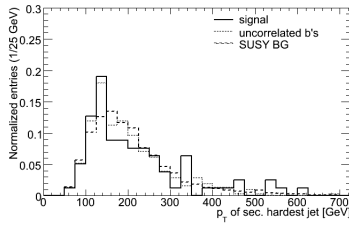
(8) p_T of second hardest jet
