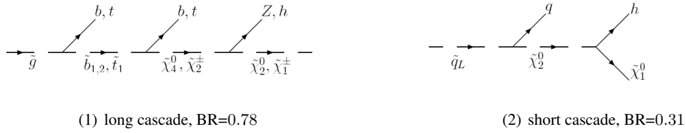
Figure 4.24: Two of the main cascades of supersymmetric particles that lead to a h production in SU6 . This is the same cascades as for SU1 in figure 4.8. The branching ratio for the first decay in each graph is shown.
