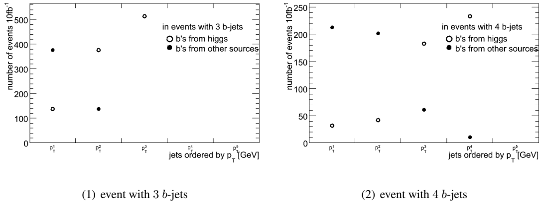
Figure 5.14: Number of b -jets coming from the decay of h compared to that of other b -jets in events with (1): three or (2): four b -jets for the SU9 signal sample. At the x -axis p_T^1, p_T^2, \dots correspond to the hardest, second hardest, ... b -jet in the event. The y -axis shows how many of the hardest, second hardest, ... b -jet in each event that comes from Higgs and from other sources.
