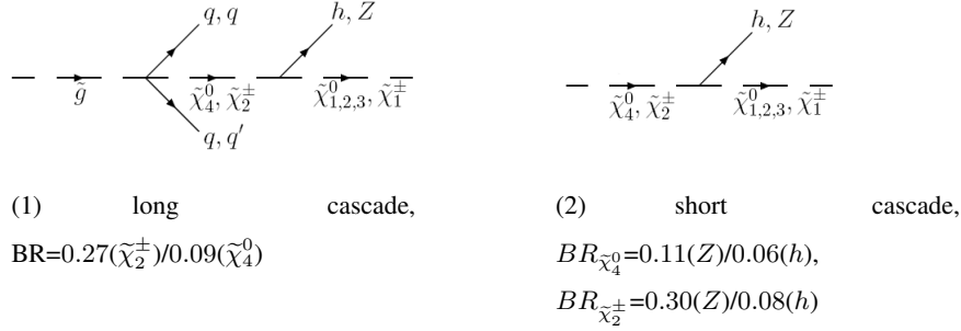
Figure 4.12: Two of the main cascades of supersymmetric particles that lead to a h/Z production in SU2 . The branching ratio for the first decay in each graph is presented.
