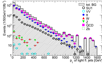
(2) p_T of light fl. jets
