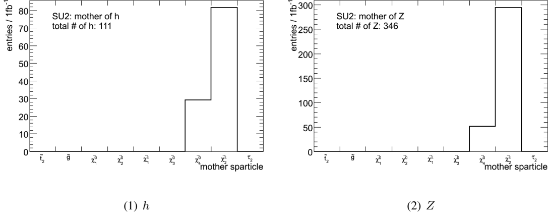
Figure 4.9: The mother of the produced Z and h bosons in the signal sample SU2 for 1fb^{-1} .
