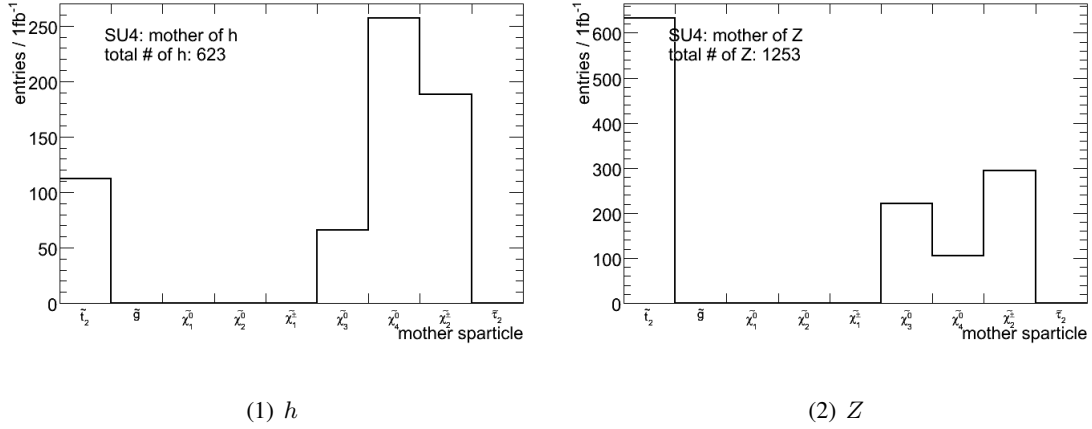
Figure 4.17: The mother of the produced Z and h bosons in the signal sample SU4 for 1\text{fb}^{-1} .
