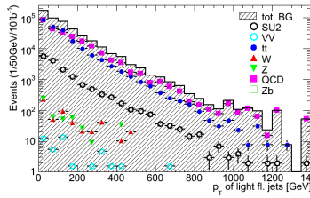
(5) p_T of light fl. jets
