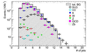
(9) # of all jets
