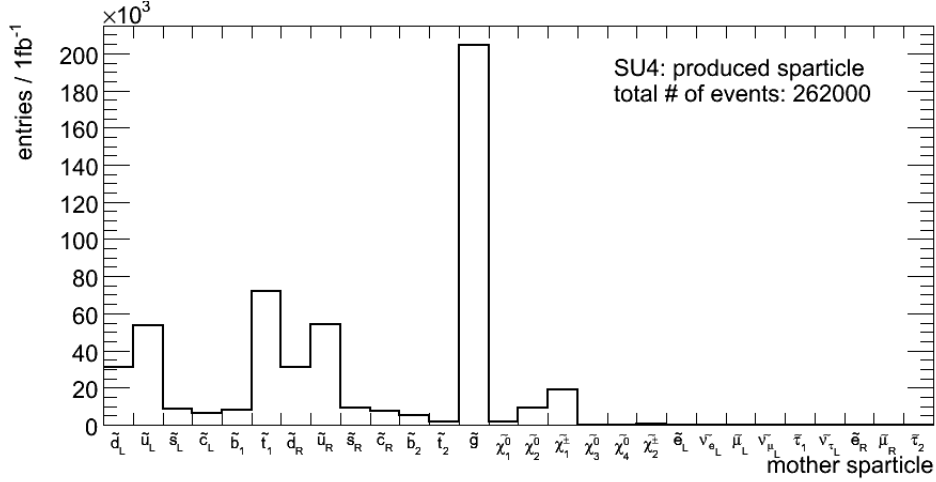
(1) sparticle produced
