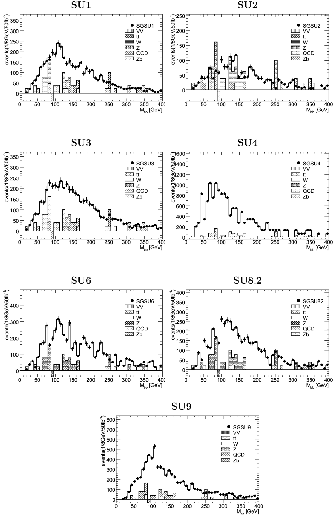
Figure 6.2: The invariant mass plots for the various signal scenarios and SM background with the cuts i table 6.1 requiring one of the additional jets to be a b-jet.
