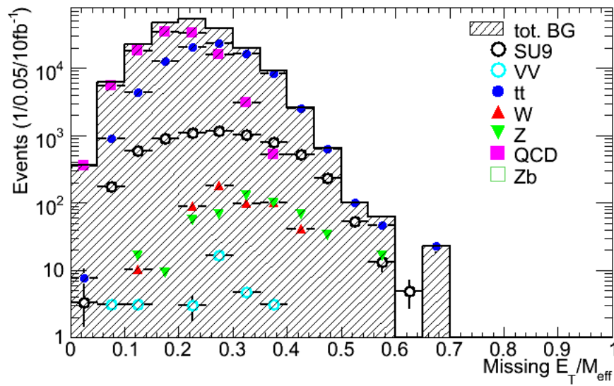
Figure 5.5: The distribution for \cancel{E}_T/M_{\text{eff}} for SU9 and SM background. Only the four hardest jets are used in the M_{\text{eff}} calculation. This variable reflects what is illustrated in figure 5.3 and 5.4. The samples that contain many high p_T jets will peak at low values while the samples which is dominated by \cancel{E}_T will peak at higher values. (Since SUSY events have much of both jets and \cancel{E}_T the distribution is more or less flat between 0.15 – 0.4)
