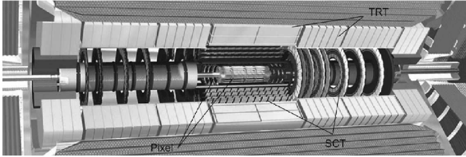
Figure 3.4: The Inner Detector of ATLAS
