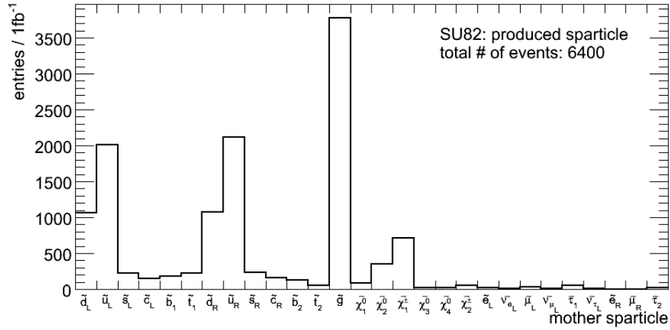
(1) sparticle produced
