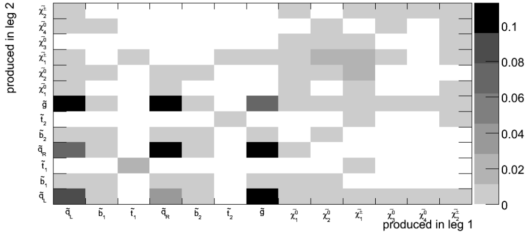
(1) sparticle produced
