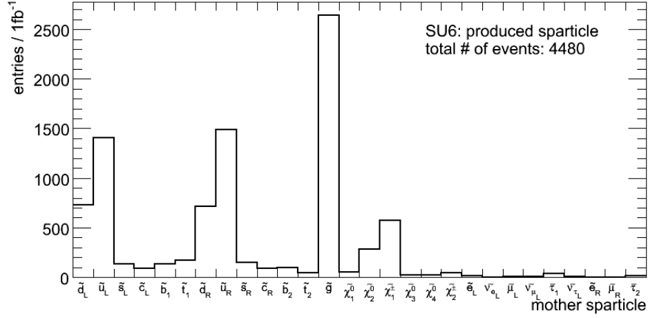
(1) sparticle produced
