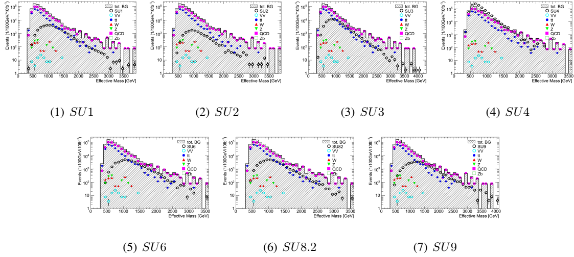
Figure 5.23: M_{\text{eff}} for the standard model background and signal after the cuts in table 5.11 are applied and with an integrated luminosity of \mathcal{L} = 10 fb^{-1} . It is clear that the distribution for the SUSY signals peaks at much higher values than the SM background.
