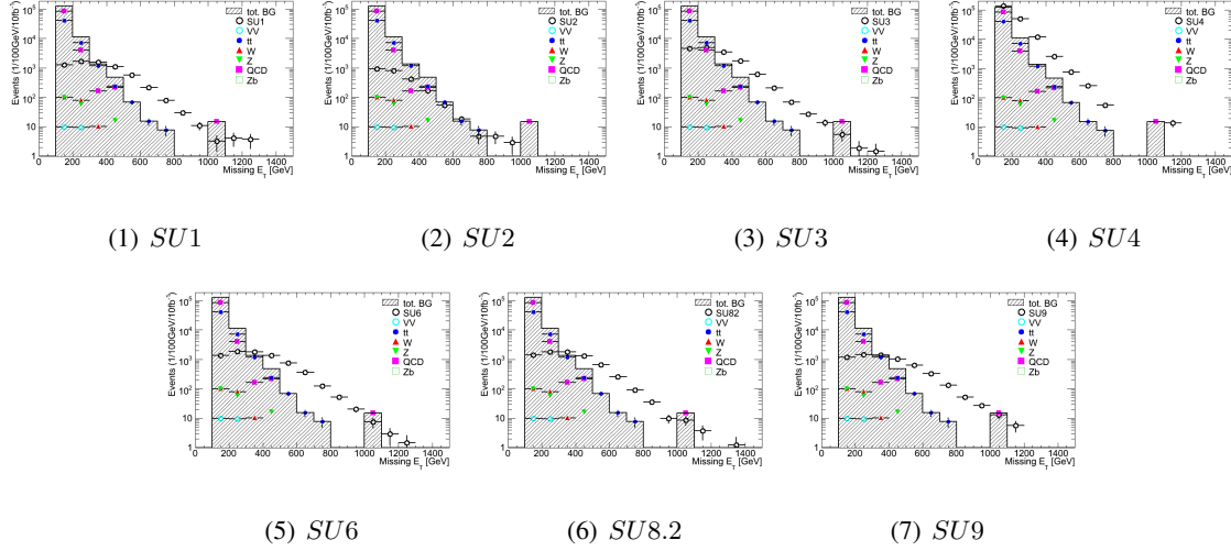
Figure 5.20: \cancel{E}_T for the standard model background and signal after the cuts in table 5.7 are applied. The SUSY signals have different distributions compared with the SM backgrounds, which is dominated by t\bar{t} and QCD. SU2 is special since the \cancel{E}_T is relatively low compared with the other SUSY samples. \mathcal{L} = 10 fb^{-1}
