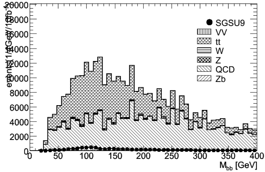
Figure 5.13: Invariant mass of all tagged b -jets for different Standard Model processes with the cuts in table 5.4 applied and a b -tagging efficiency of 60%. For the Standard Model one see a reduction in the number of events compared with 5.8.
