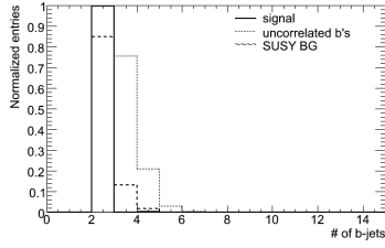
(1) # of b -jets
