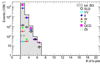
(4) # of b -jets
