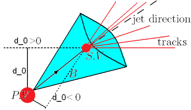
Figure 4.3: The idea of Impact Parameter. PV = primary vertex, SV = secondary vertex and d_0 is the transverse impact parameter.
