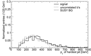
(1) p_T of hardest jet
