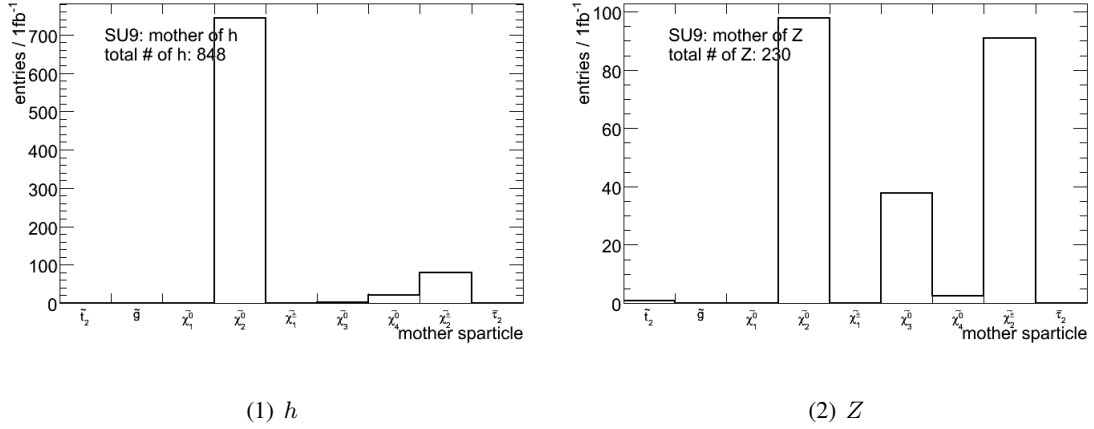
Figure 4.29: The mother of the produced Z and h bosons in the signal sample SU9 for 1\text{fb}^{-1} .
