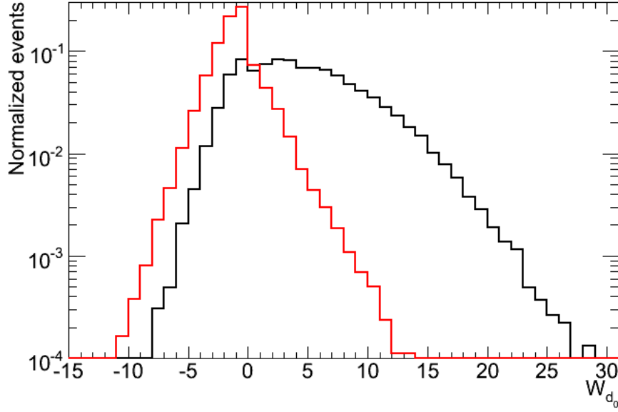
Figure 4.4: The distribution of the transverse IP significance weight (IP2D) for light jets (light) and b -jets (dark).
