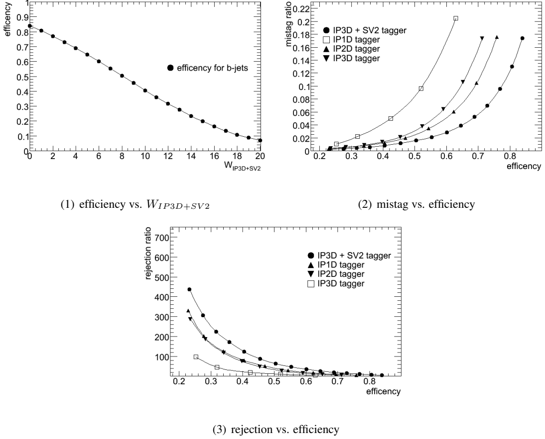
Figure 5.6: (1): The efficiency of b -tagging as a function of the W_{IP3D+SV2} . (2) and (3) the mistag/rejection of light jets as a function of efficiency for different types of taggers. As expected the tagger which combine the IP3D and SV2 tagger has the best performance. These plots are for the SU9 sample, however the same b -tagging performance is achieved with the same value on W_{IP3D+SV2} in the other samples.
