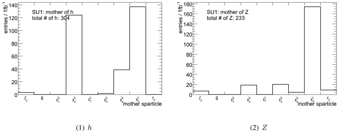
Figure 4.5: The mother of the produced Z and h bosons in the signal sample SU1 for 1fb^{-1} .
