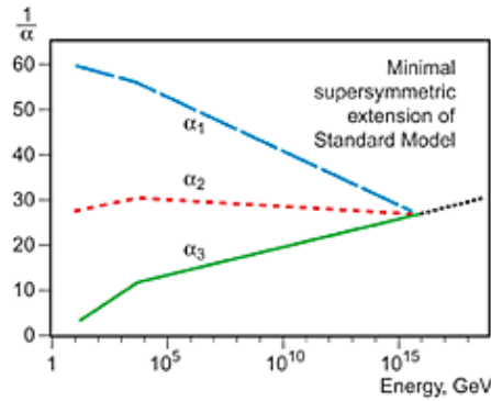
Figure 2.3: The evolution of the coupling constants with a supersymmetric theory at the TeV scale
