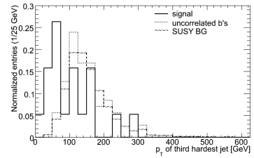
(6) p_T of third hardest jet
