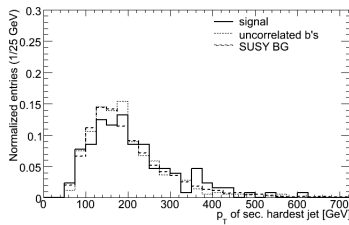
(11) p_T of second hardest jet
