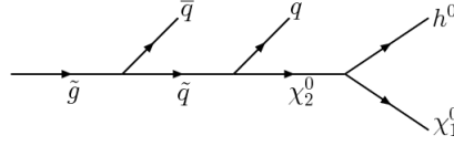
Figure 4.31: The main cascades of supersymmetric particles that lead to h production in SU9 . BR= 0.67 for the gluino to decay into a left handed squark or a third generation squark.
