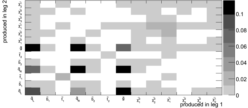
(2) sparticle pair produced
