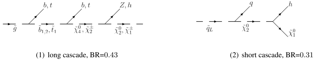
Figure 4.8: Two of the main cascades of supersymmetric particles that lead to a h production in SU1 . The branching ratio for the first decay in the chain is presented under the graph (for the q_L the BR is per left-handed squark).
