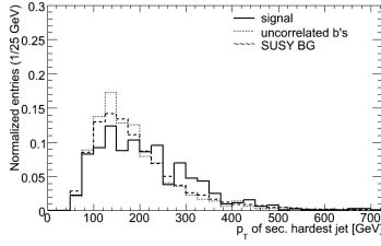
(2) p_T of second hardest jet
