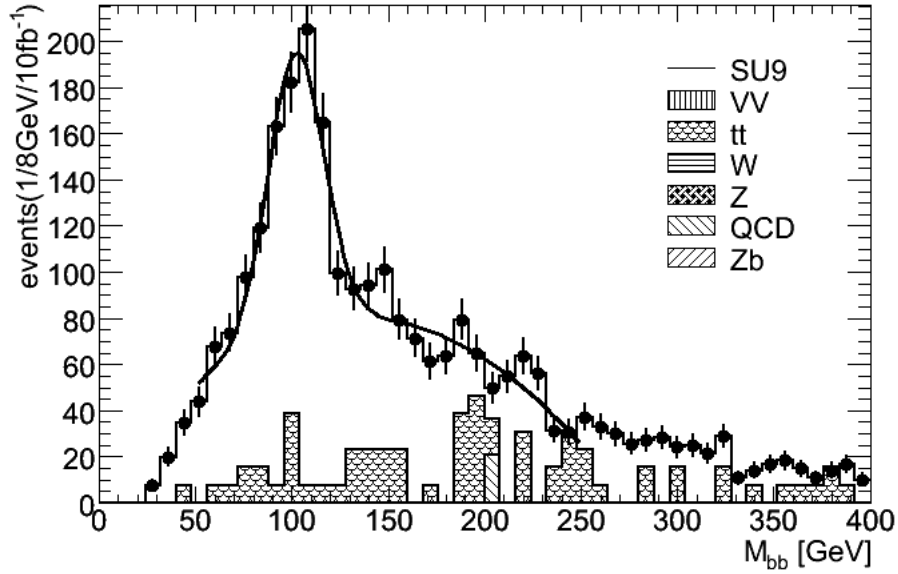
Figure 6.4: Invariant mass of b -jets in SU9 with an integrated luminosity of 10\text{ fb}^{-1} after the cuts in table 6.1 and the requirement of the two additional jets to be light flavored.
