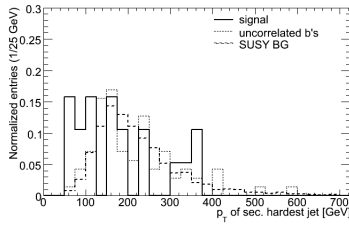
(5) p_T of second hardest jet
