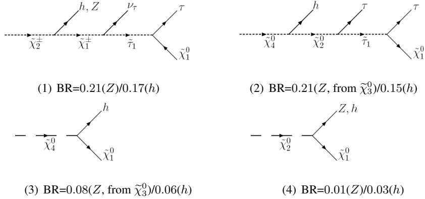
Figure 4.26: The different diagrams for Z and h production in the signal sample SU8.2 . The Z has similar diagrams (2) and (3) as h provided \tilde{\chi}_4^0 is replaced with \tilde{\chi}_3^0 .
