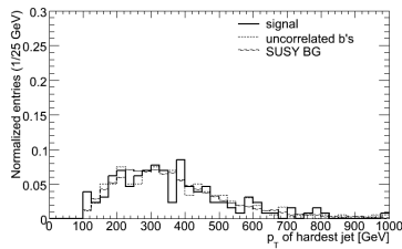
(10) p_T of hardest jet
