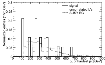
(4) p_T of hardest jet
