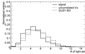
(14) # of light fl. jets
