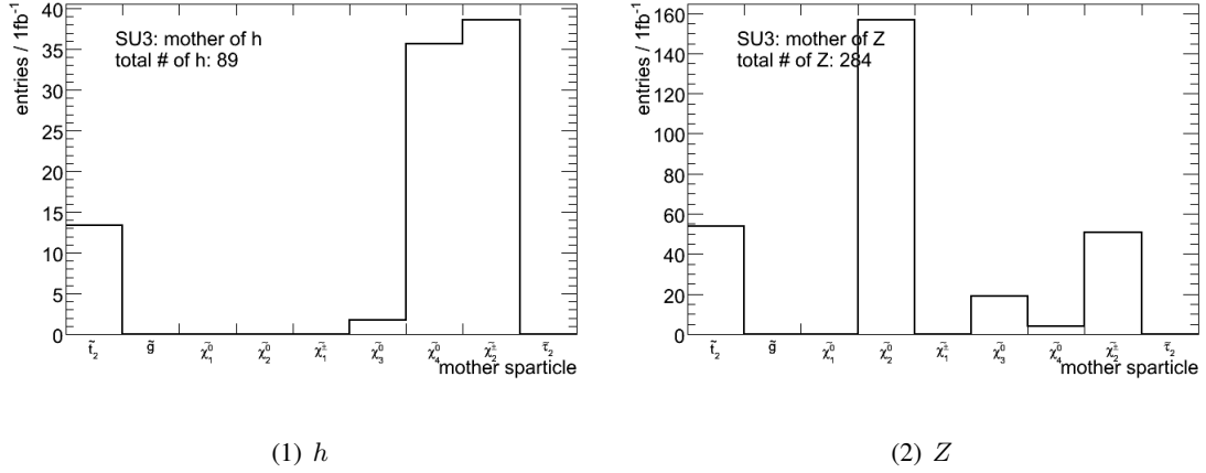
Figure 4.13: The mother of the produced Z and h bosons in the signal sample SU3 for 1\text{fb}^{-1} .
