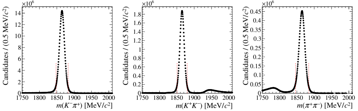
Figure 4.9: Distribution of m(h^+ h^-) after the subtraction of the m(D^0 \pi_{\text{tag}}^+) background for the (left) D^0 \rightarrow K^- \pi^+ , (centre) D^0 \rightarrow K^+ K^- and (right) D^0 \rightarrow \pi^+ \pi^- samples. The signal window is delimited by the vertical dashed lines.
