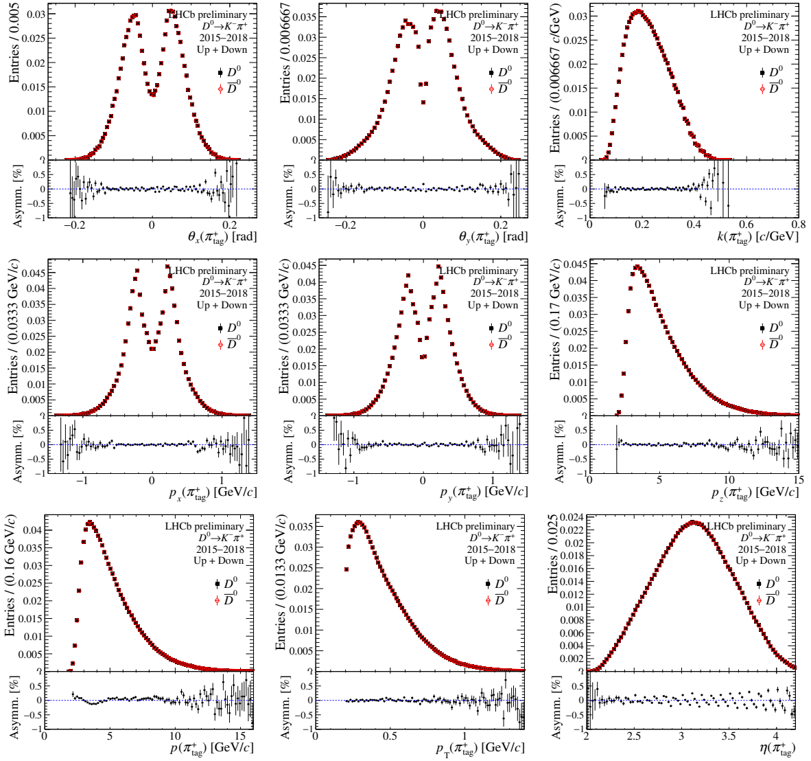
Figure D.10: Distributions and asymmetries of the momentum of the \pi^+ meson for the full D^0 \rightarrow K^- \pi^+ data sample.
