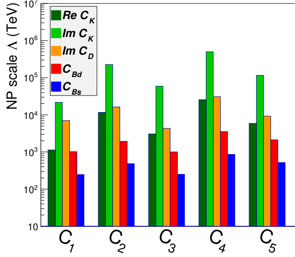
Figure 1.5: Summary of the 95% probability lower bound on the scale of new-physics (NP) interactions beyond the SM, \Delta , for strongly interacting NP. Results from all of the neutral meson systems are shown. Figure taken from Ref. [17].
