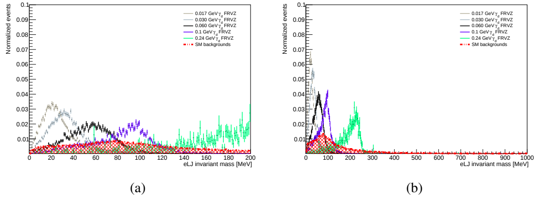
Fig. 6.3 Distributions at pre-selections level of eLJ invariant mass in (a) [0, 200 MeV], and (b) [0, 1000 MeV] range for SM processes, FRVZ and HAHM signal with different \gamma_d mass points.
