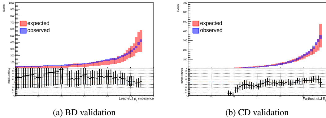
Fig. 7.9 Observed and expected values of the number of events in data in the e\text{LJ-}e\text{LJ} channel BD and CD sub-planes as a function of the cut on p_T^{\text{imb}} and R_\phi , respectively.
