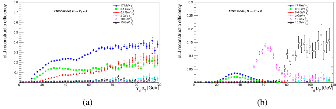
Fig. 5.15 Reconstruction efficiency in the category of (a) 1 electron and (b) 2 electrons inside eLJ as a function of truth p_T of \gamma_d at different \gamma_d mass in the FRVZ benchmark model.
