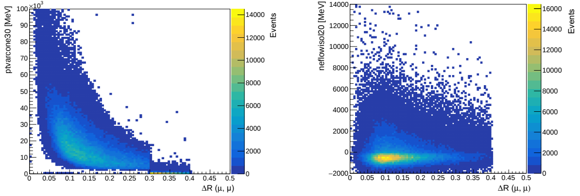
Fig. 5.5 The (a) ptvarcone30 and the (b) neflowisol20 distributions for muons as a function of their truth opening angle \Delta R . Muons are required to be matched to truth muons from \gamma_d , which has a mass of m_{\gamma_d} = 2 GeV.
