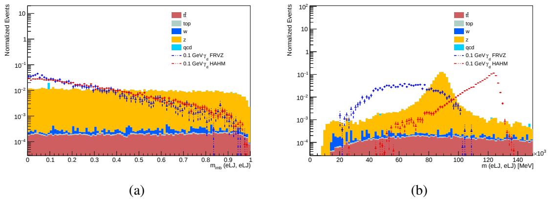
Fig. 6.4 Distributions at pre-selections level of (a) eLJ invariant mass imbalance and (b) eLJ - eLJ invariant mass for SM processes, FRVZ and HAHM signal with \gamma_d = 0.1 GeV.
