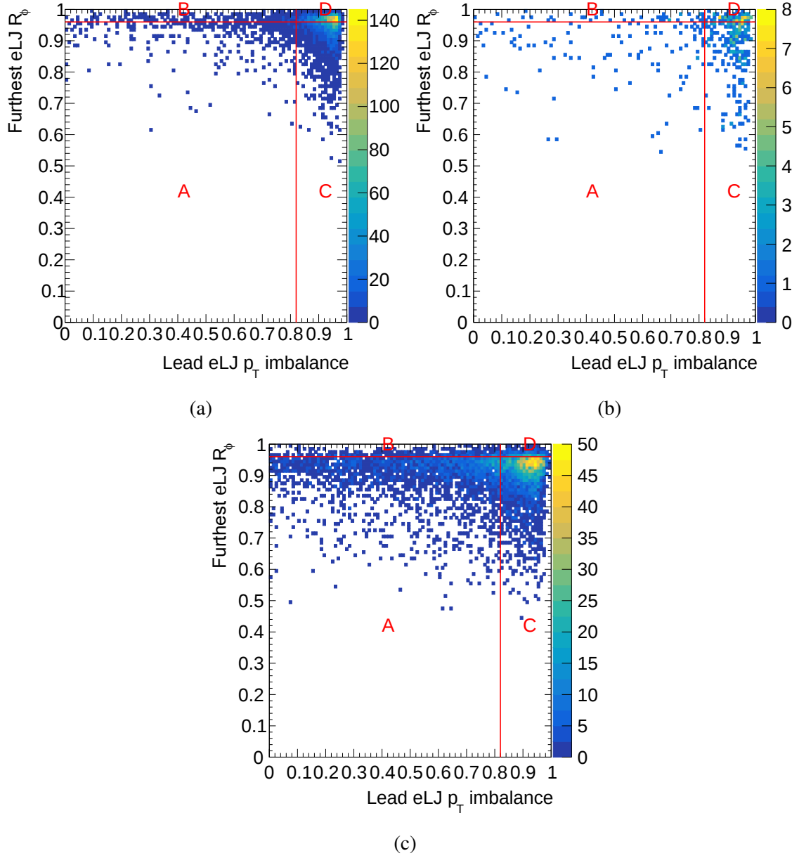
Fig. 7.11 ABCD plane of leading eLJ p_T^{\text{imb}} and furthest eLJ R_\phi for (a) VR1 on-shell Z boson mass window, (b) VR2 |q_{eLJ}| > 0 , and (c) VR3 |\eta| > 1.5 end-cap.
