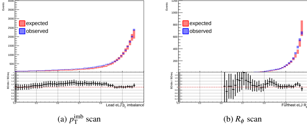
Fig. 7.12 Observed vs. expected values of the number of events in data in the eLJ-eLJ channel on-shell Z boson mass window validation region as a function of the cut on p_T^{\text{imb}} and R_\phi , respectively.
