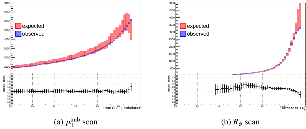
Fig. 7.14 Observed vs. expected values of the number of events in data in the e\text{LJ-}e\text{LJ} channel |\eta| > 1.5 end-cap validation region as a function of the cut on p_T^{\text{imb}} and R_\phi , respectively.
