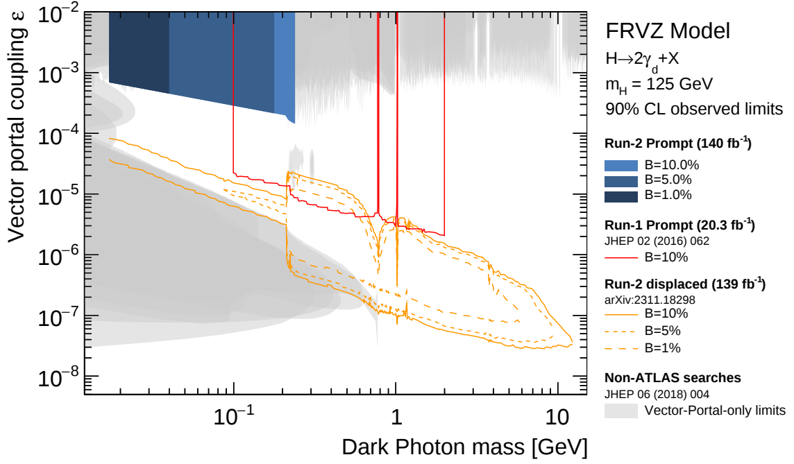
Fig. 9.10 90% exclusion contours as a function of \varepsilon and m_{\gamma_d} for the FRVZ model in the assumption of \gamma_d decay length c\tau < 0.01 mm. The limits are obtained by assuming a decay branching ratio of Higgs boson into \gamma_d s ranging between 10% to 1%, where the darker colors correspond to stronger choices of branching ratio. The figure also shows previous ATLAS Run-1 prompt [4], ATLAS Run-2 displaced [53], and other vector-portal-only limits.
