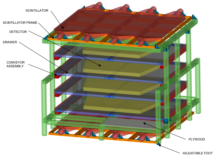
Figure 6.1: Schematic of the cosmic-ray hodoscope. The extruded aluminum parts are colored green and orange. The assemblies of scintillators, waveguides and PMTs are colored red and are located over and under the structure. The flat trapezoid sTGC modules are colored olive and are located over the blue drawers where they are partially seen.
