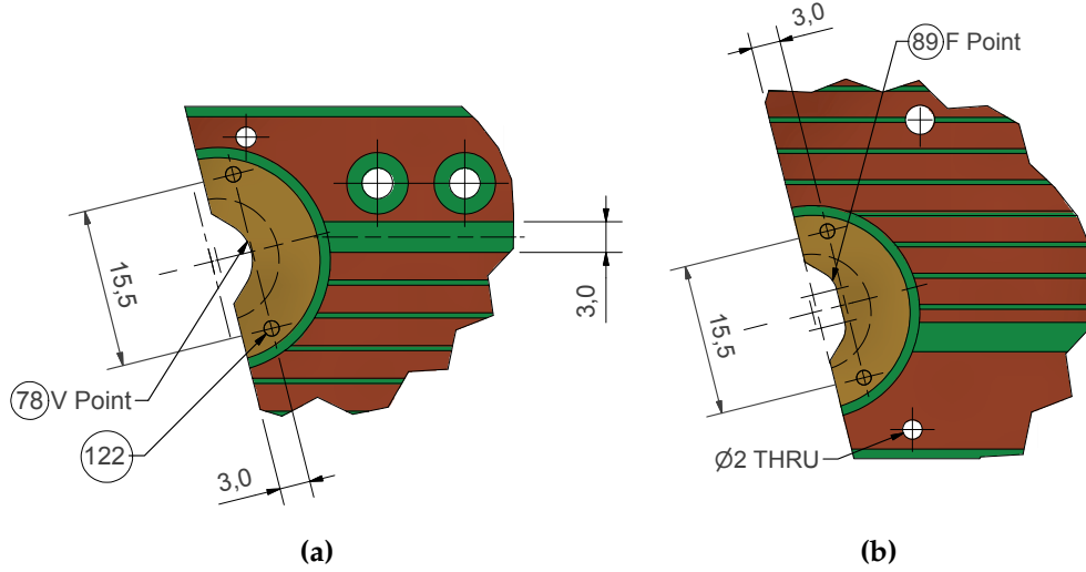
Figure 4.4: Drawing of the strip-board brass inserts as seen in the QL1 quadruplet technical drawings [99]. Units are millimeters. The brass inserts can be either of (a) triangular or (b) trapezoidal type. One brass insert of each type is crimped on one of the angled side of the strip-boards. The triangular brass insert is located on the long base side and the trapezoid brass insert on the short base side.
