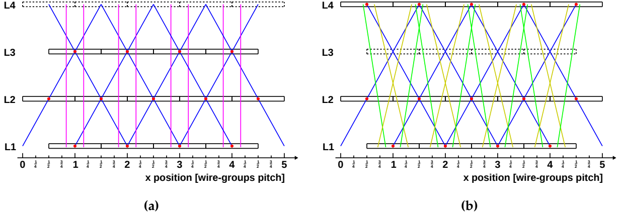
Figure D.3: Sketch of the possible x positions of a reference tracks reconstructed with wire hits in the x - z plane on the tested layer of a sTGC built with half staggering of the wire groups and equal distance between detector planes. The special cases for an (a) outer tested layer (layer 4) and (b) inner tested layer (layer 3) are shown. The wire groups are identified by rectangles. The wire groups of the tested layer have dotted lines. The position of the reconstructed wire space points are marked by a red dot in the middle of the wire groups. The tracks are displayed using lines of different colors. Each color is associated to a value of the x - z track polar angle |\theta_{xz}| .
