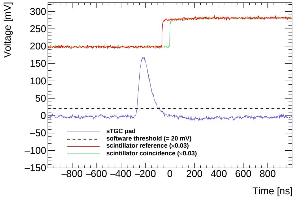
Figure 5.18: Oscilloscope segment of a representative pad analog signal amplified and shaped by the VMM3 ASIC from a cosmic-ray muon. The scintillator detector reference and coincidence signals are digital TTL logic pulses. The digital pulses are scaled by a factor \times 0.03 and offset on the voltage scale for display purposes. The origin of the time axis is the leading edge of the scintillator detector coincidence pulse, which triggers the oscilloscope. The sTGC pulse time measurement is taken as the time when the pulse leading edge crosses the offline software threshold. The reference scintillator detector time measurement is taken as the leading edge of the scintillator detector discriminated pulse (red line).
