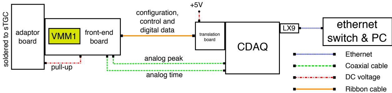
Figure 5.2: Schematic diagram of the data acquisition system associated to a single VMM1 ASIC used to read out wire and strip electrodes. The translation board is used to convert the digital voltage levels for communication between the CDAQ and the front-end board. The translation board also provides power to the CDAQ and the front-end board through the +5V input. The pull-up is a DC voltage level used to bias the signal from sTGC strips and is required by the VMM1 to read out a signal of positive polarity.
