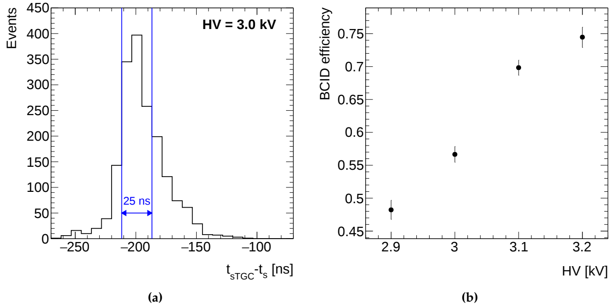
Figure 5.19: (a) Pad time jitter at an operating voltage of 3.0 kV and (b) fraction of hits contained in an optimum 25 ns time window as a function of the operating voltage. The optimal 25 ns time windows, used to calculate the BCID efficiency, is highlighted with blue lines on the (a) distribution.
