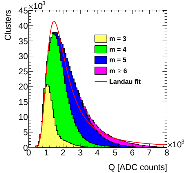
Figure 6.9: Distribution of the strip cluster charge with Landau fit. The contribution of each charge cluster strip multiplicity m corresponds to a different fill color.
