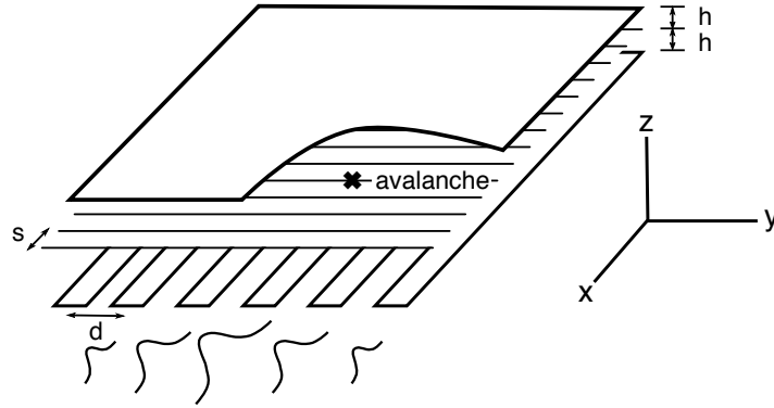
Figure 2.12: Schematic of a multiwire chamber with a segmented cathode. The cross highlights the avalanche position on one of the anode wires. The signal induction on each cathode strip is sketched.
