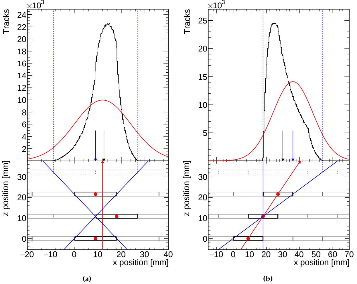
Figure C.1: Results of the wire track extrapolation simulation for the two track types considered. The bottom of the figures shows the pattern of the simulated sTGC module wire groups. The excluded layer is displayed by dotted boxes. Wire groups traversed by the simulated muon track are displayed with bolder lines. The position of the wire space points is indicated by red markers. The red line indicates the reconstructed track obtained from a linear fit to the wire space points. The red arrow indicates the position of the reconstructed track on the excluded layer. The blue lines are muon tracks pointing to extremum positions on the excluded layer. The simulated position distribution is shown as a black line on the top part of the figures. The distribution has the same normalization for both figures. The red curve denotes the Gaussian probability density function of the reconstructed track position assuming that the wire space points have a Gaussian error of width d/\sqrt{12} . The blue dotted lines indicate the extremum track positions for the considered wire groups. The black and blue arrows respectively denote the position of x_{MC} and \bar{x} . The top and the bottom parts of the figures share the same x axis.
