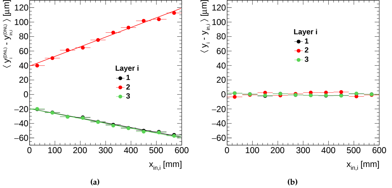
Figure 5.7: Mean of the inclusive reference track y -residuals for each tested layer i , as a function of the reference track x -coordinate on the layer (a) without and (b) with inter-layer misalignments corrections. The differential non linearity corrections are applied in both cases to all space points. The non-corrected y -residuals are fitted to a first order polynomial.
