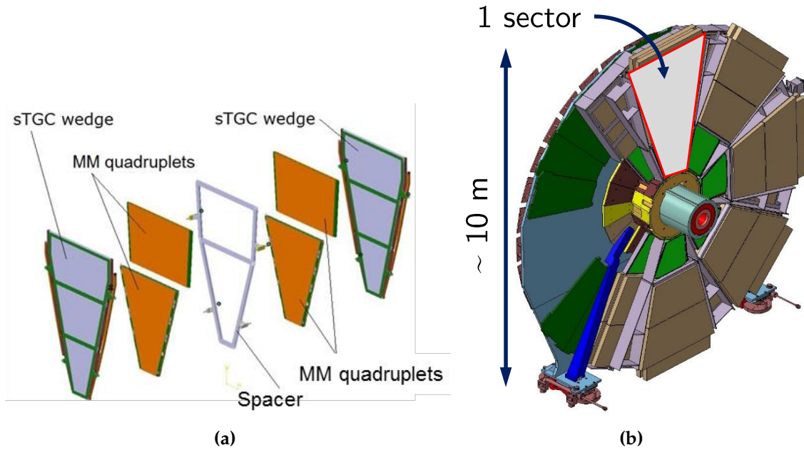
Figure 3.7: (a) Schematic of a disassembled large sector combining sTGC and Micromegas wedges and (b) cutaway drawing of the finished NSW as seen looking towards the interaction point. The sTGC wedges combine 3 modules while Micromegas wedges have 2 modules. The detector modules are made of 4 detector layers. Wedges can be of “large” or “small” type making large and small sectors respectively. The NSW is made of 8 large and 8 small sectors.
