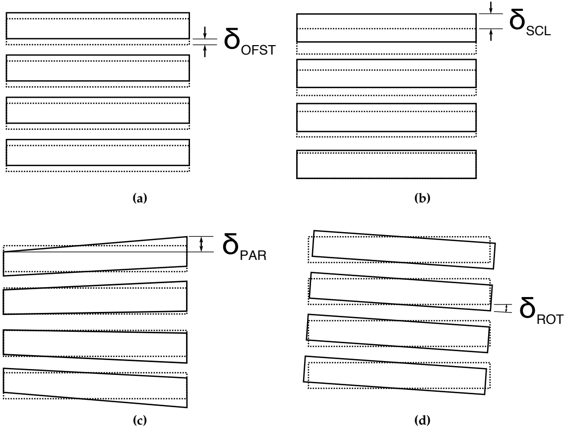
Figure 4.1: Sketch of the strip-board non-conformities considered compared to the nominal strip pattern (dotted lines): (a) constant offset, (b) pitch scale, (c) non-parallelism and (d) rotation. The measurement performed during strip-board dimensional control is shown on each diagram. The values of \delta_{\text{OFST}} , \delta_{\text{SCL}} and \delta_{\text{PAR}} are in units of length while the value of \delta_{\text{ROT}} is an angle. The strips dimensions are not to scale.
