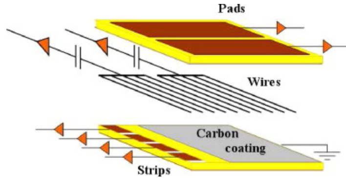
Figure 3.8: Schematic of the pad, strip and wire electrodes of a sTGC gas volume used in the NSW. The wires are ganged in groups of 20 and capacitively coupled to the readout electronics. The strip and pad electrodes are capacitively coupled to the graphite coating.
