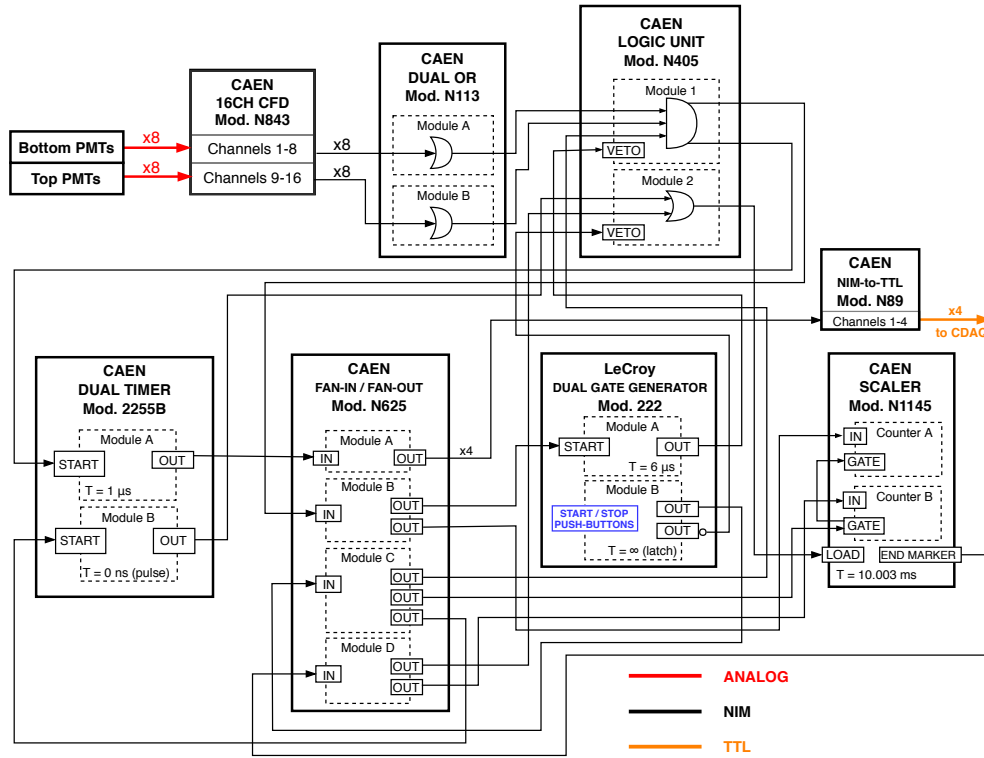
Figure 6.2: Block diagram of the cosmic-ray hodoscope trigger system. The bold rectangles indicate individual NIM modules. The arrows indicate the direction of the signal. The color of the arrows is associated with the logic levels of the signal lines. The CAEN N89 NIM-to-TTL module is used only for the CDAQ prototype boards which require TTL levels. More than 4 independent trigger lines can be used if additional fan-out modules are daisy-chained to the first one.
