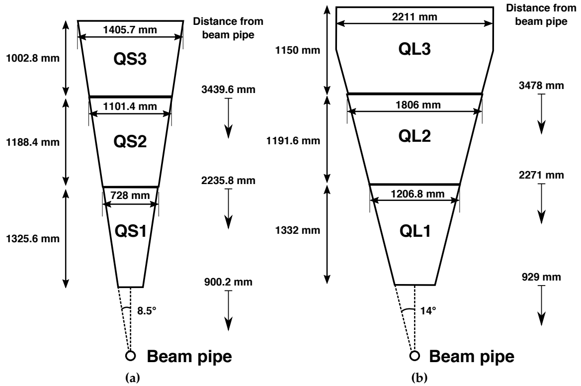
Figure 4.3: Dimensions of the (a) small and (b) large sTGC wedges projected in the x - y plane. The schematics are to scale. The height, width and distance from the beam pipe of each sTGC quadruplet are displayed. The wedges angular coverage in \phi is also shown. There are small gaps between the quadruplets of the order of 1 cm that cannot be resolved on the figure.
