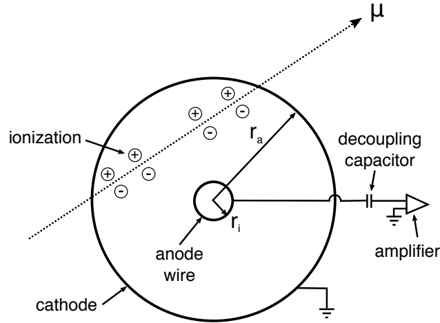
Figure 2.8: Cross section schematic of a cylindrical ionization detector.
