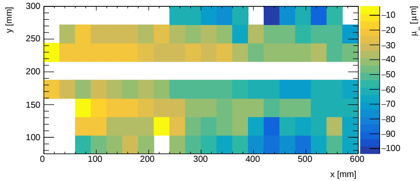
Figure 6.8: Value of the mean obtained from the fitted double Gaussian function to the exclusive y -residual distributions for layer 4 of the 40 \times 60 \text{ cm}^2 sTGC prototype.
