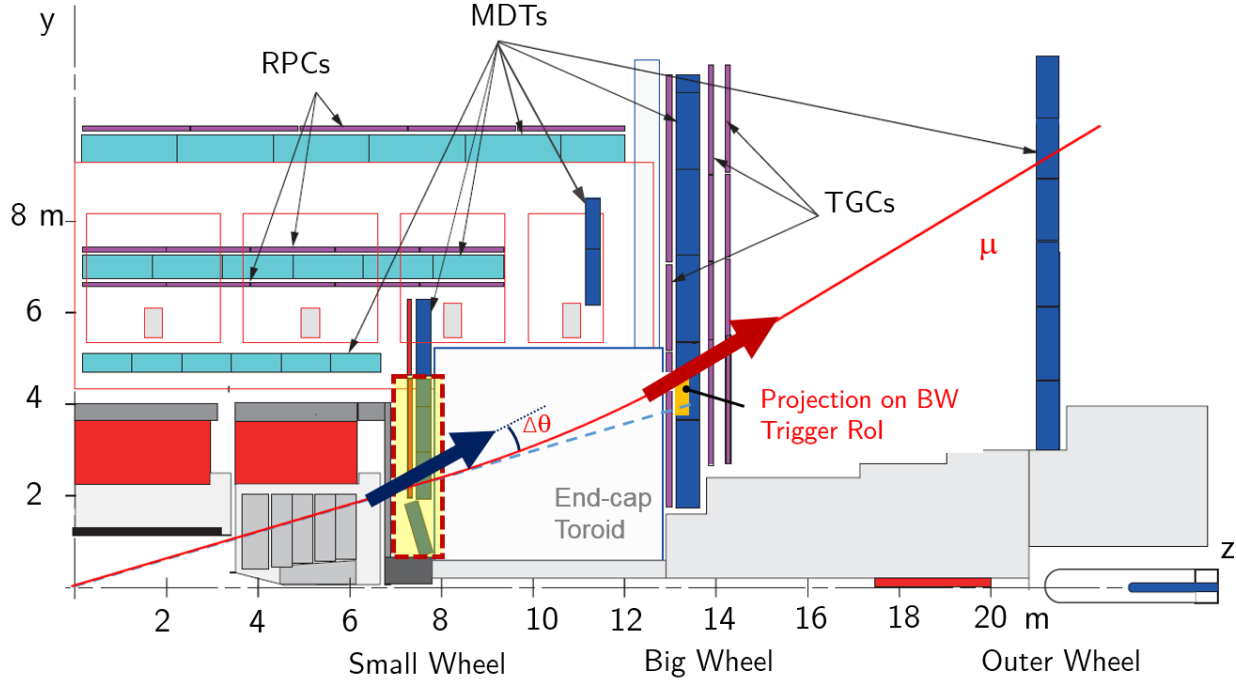
Figure 3.6: Projection of the current ATLAS muon spectrometer on the y - z plane [97]. The yellow shaded rectangle highlights the inner station modules that will be replaced by the NSW as part of the muon spectrometer upgrade. A visual representation of the Level-1 muon trigger algorithm, based on information from the NSW, is shown. A muon originating from the interaction point (red line) traverses the NSW resulting in the reconstruction of a track segment. The NSW measurement is used to confirm whether the reconstructed track segment comes from a particle originating from the interaction point by measuring the angle difference \Delta\theta between the reconstructed track segment and a track segment that would be expected from a muon originating from the interaction point. Then, the NSW track segment is required to be consistent with a second track segment reconstructed by the middle station. Finally, if the NSW trigger conditions are met, the central trigger processor determines if a Level-1 trigger accept shall be issued based on the track segments. The muon transverse momentum p_T is estimated from the muon deviation in the magnetic field of the end-cap toroid which corresponds to angle difference of the track segments of the inner and middle stations.
