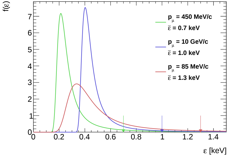
Figure 2.2: Fluctuations of energy loss predicted by Landau's theory for muons traversing a sTGC gas volume. The arrows indicate the mean energy loss \bar{\epsilon} obtained by the Bethe-Bloch formula.
