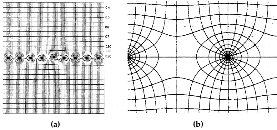
Figure 2.11: (a) Electric field lines and equipotentials in the gas volume of a multiwire chamber. The electric potential relative to the anode wire potential, or value of V_0 , is indicated. The effects of a minor displacement of one anode wire is shown. (b) Enlarged view of the same figure in the vicinity of a wire [14].
