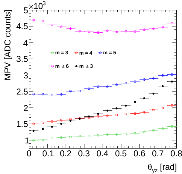
Figure 6.11: Most probable value of the fitted Landau function of the Q values as a function of the muon track angle |\theta_{yz}| for different strip-cluster multiplicities m . The black markers show the MPV values with all strip-cluster multiplicities combined.
