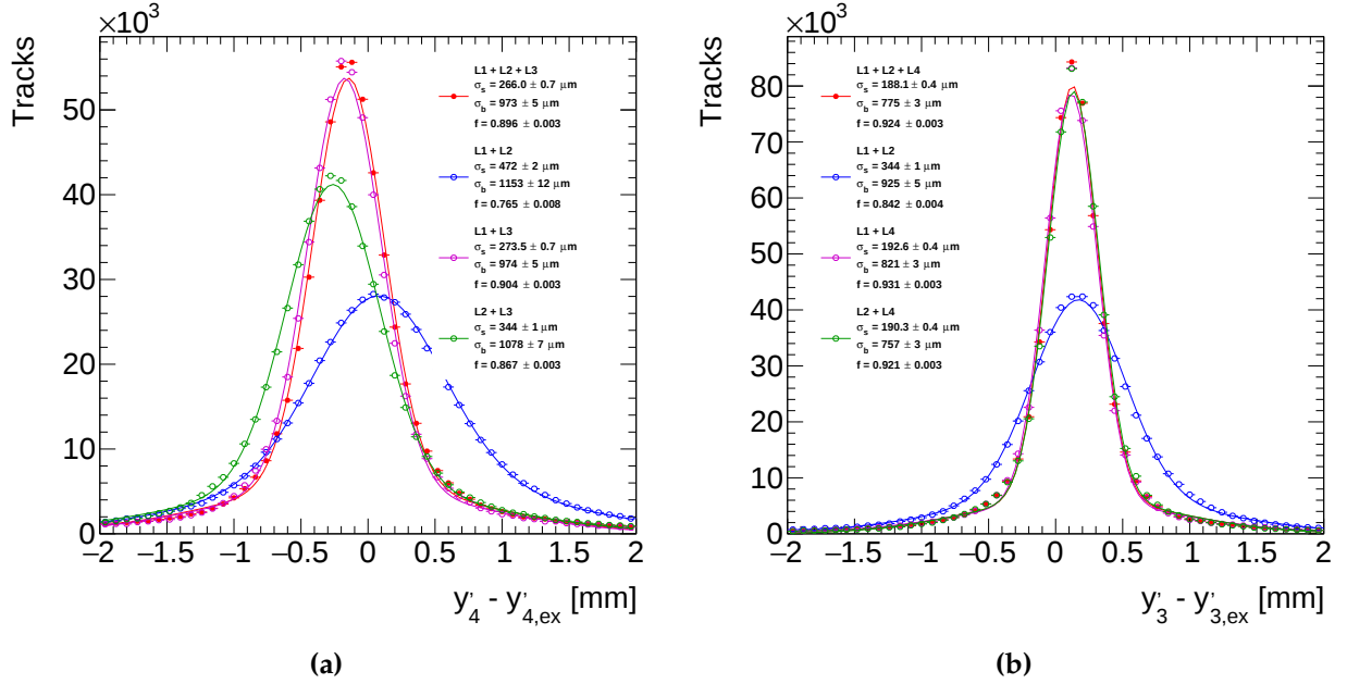
Figure D.1: Exclusive y -residual distributions for (a) an outer tested layer (layer 4) and for (b) and inner tested layer (layer 3). The full red markers denote the track y -residuals from a track reconstructed with all 3 exclusive layers. The other markers indicate tracks reconstructed with only 2 exclusive layers. The distributions have the same normalization. The distributions are fitted to a double Gaussian function. The width of the signal ( \sigma_s ) and background ( \sigma_b ) Gaussians and the signal fraction f are shown.
