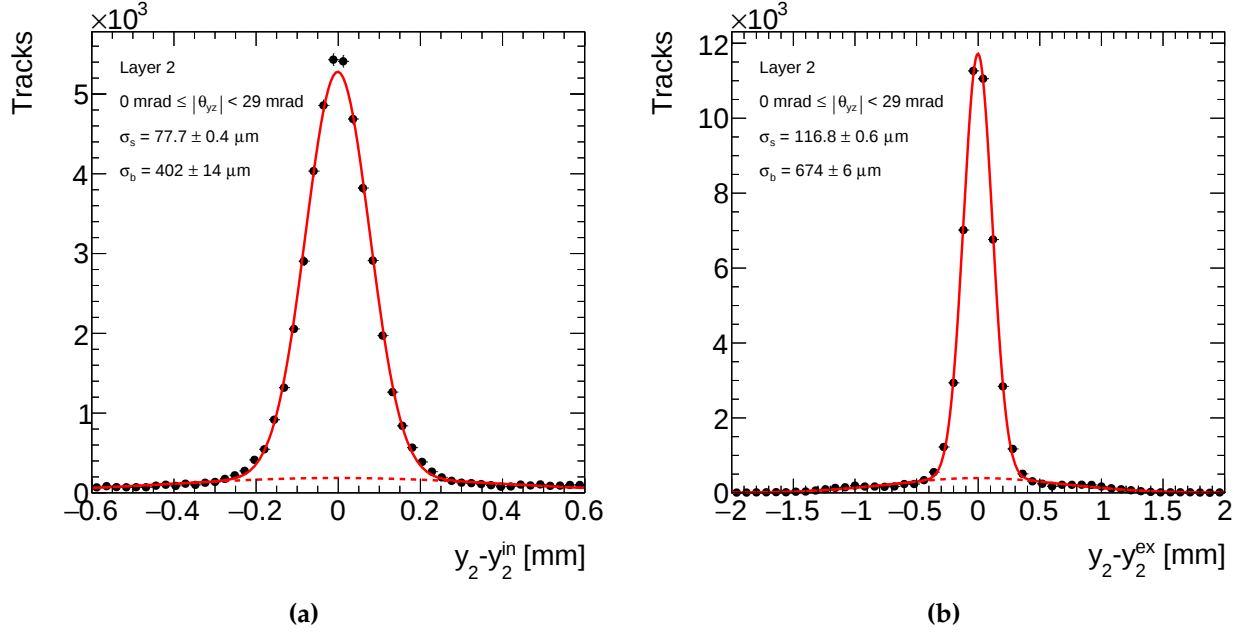
Figure 5.9: Distributions of reference track y -residuals on layer 2 for the (a) inclusive and (b) exclusive cases. The double Gaussian function fitted to the data is drawn on the distributions as a continuous red line. The background term of the fit function is drawn with a dashed line. The signal term accounts for about A_s/(A_s + A_b) = 85\% of the events for both distributions. The signal fraction is approximately constant as a function of the reference track angle.
