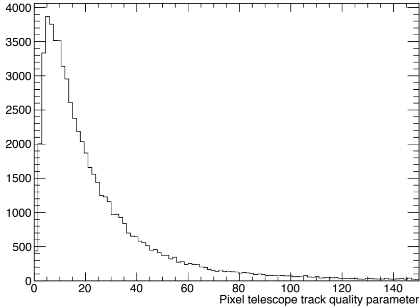
Figure 5.12: Distribution of the track quality parameter for reconstructed tracks from the pixel telescope.
