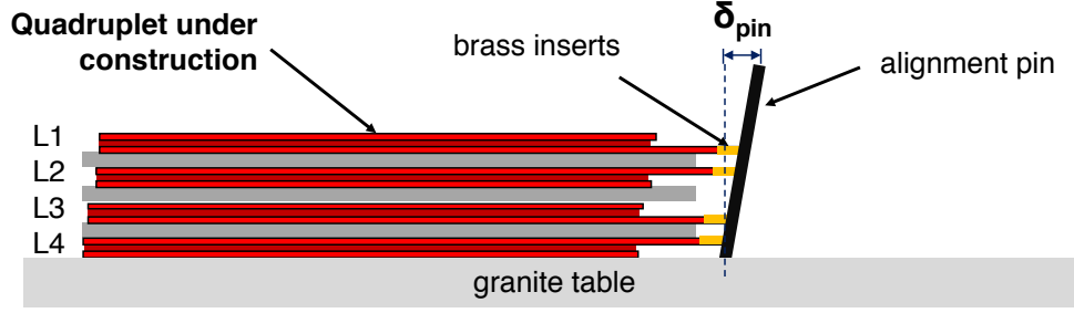
Figure 4.5: Gluing of doublets into a quadruplet on a granite table. The brass inserts are moved away from their nominal positions because of tilted alignment pins.
