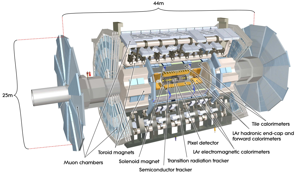
Figure 3.3: Cut-away view of the ATLAS detector. The major subdetector systems are identified.
