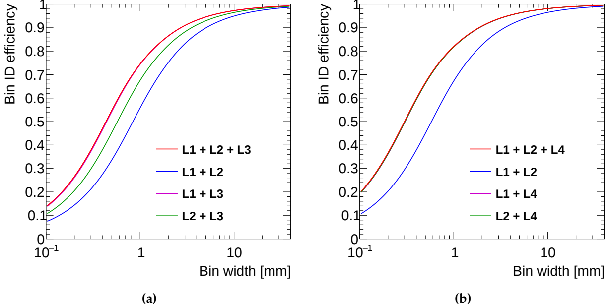
Figure D.2: Calculated BIDA values for (a) an outer tested layer (layer 4) and (b) an inner tested layer (layer 3) based on the double Gaussian fit parameters of the exclusively reconstructed track y -residual distributions shown in Fig. D.1. The layers used for the exclusive track reconstruction are indicated in the legend. The purple and red line coincide for the outer layer case (a). The red, purple and green curves coincidence for the inner layer case (b).
