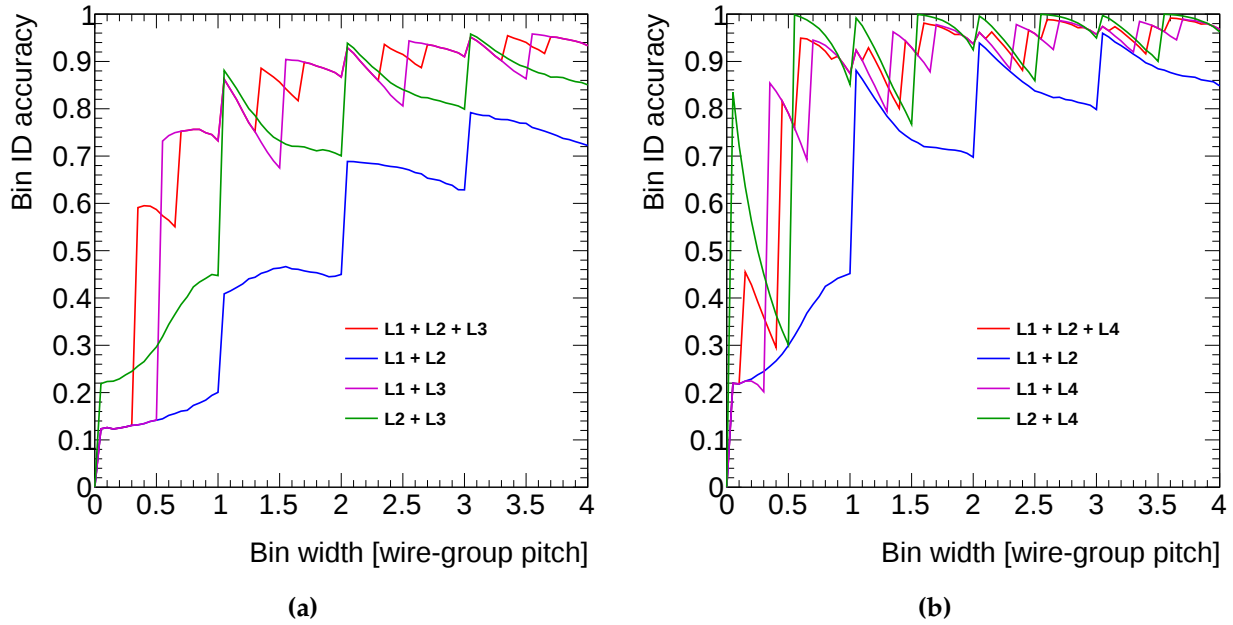
Figure D.5: Simulated BIDA as a function of the bin width for a fixed bin offset equal to half the wire group width when the tested layer is (a) an outer layer and (b) an inner layer. The detector planes used for the reference track reconstruction are indicated in the legend.
