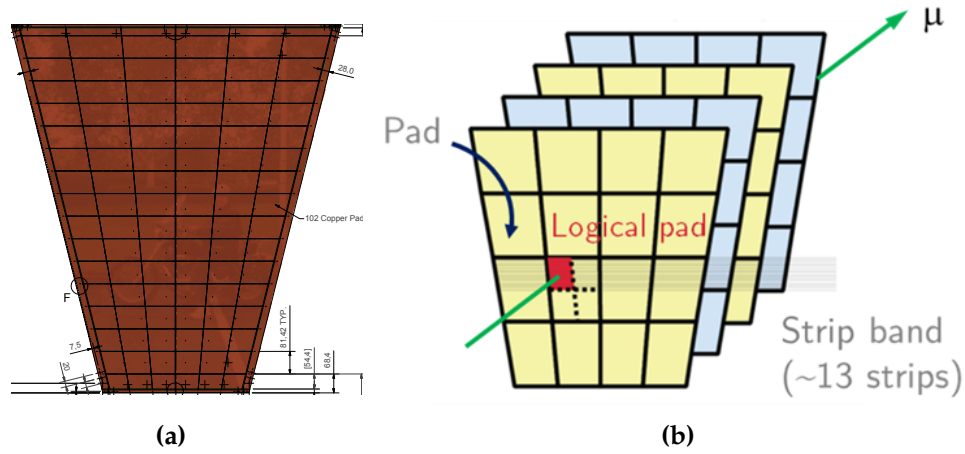
Figure 3.9: (a) Physical readout pads geometry of layer 1 of the QL1 pivot quadruplet [99] and (b) schematic of the readout pads staggering between different sTGC layers of a quadruplet [97]. The area corresponding to a logical pad on a detector plane is approximately four times smaller than the area of a physical pad.
