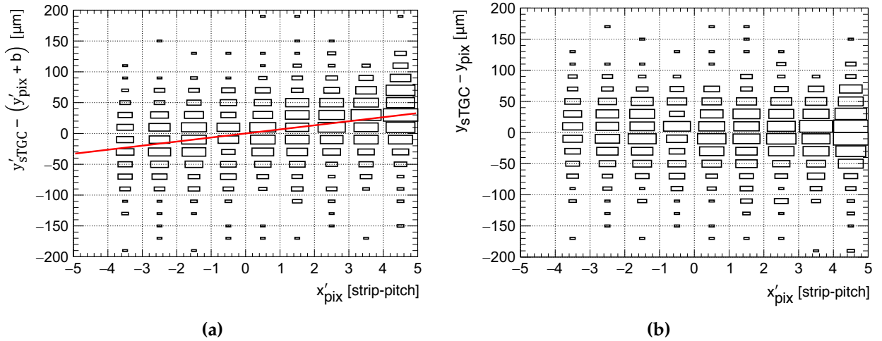
Figure 5.14: Two-dimensional distributions of y -residual as a function of x'_{\text{pix}} for a representative data acquisition run. The rotation correction (red line) has been omitted in (a) for computing the residuals, whereas the corrected y -residual distribution is shown in (b).
