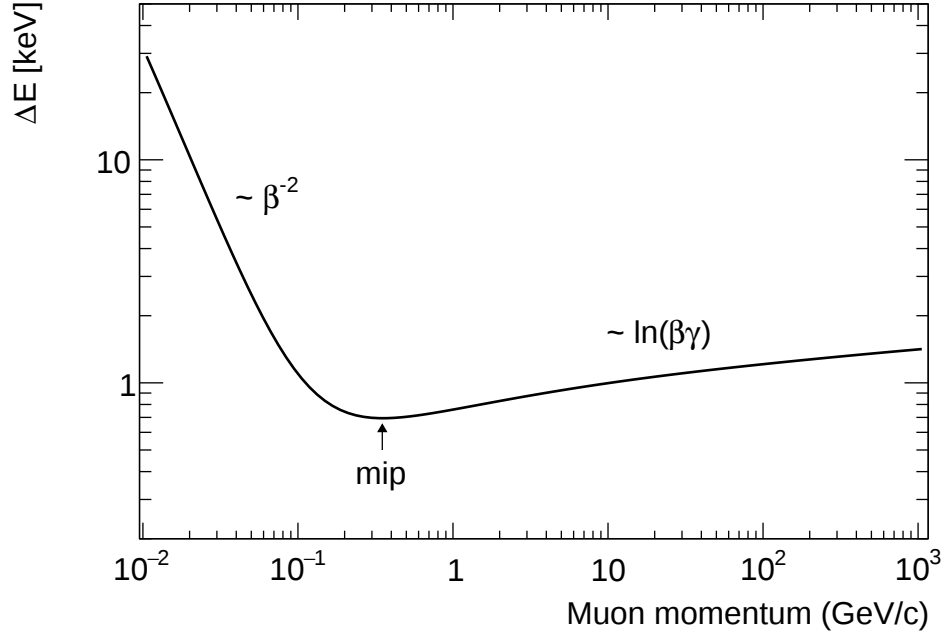
Figure 2.1: Mean energy loss from electronic interactions of a muon traversing the gas volume of a STGC detector.
