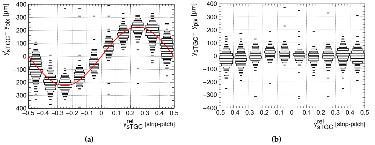
Figure 5.13: Two dimensional distribution of the y -residual as a function the the cluster position y_{\text{sTGC}}^{\text{rel}} relative to the inter-strip spacing for a representative data acquisition run. The differential non linearity correction has been omitted in (a). The red line highlights the universal differential non linearity correction used for correcting all cluster strip multiplicities. The corrected y -residual are shown in (b).
