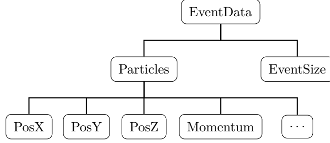
Figure 1: Example TTree.
