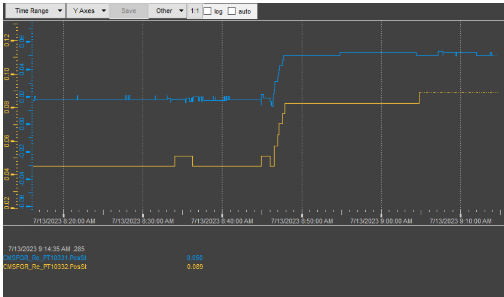
Figure 75: Pressure dependence between the two buffers. Setting the top buffer pressure (blue) to 50 mbar, the bottom buffer pressure (yellow) increases consequently, due to their communication with the connecting pipe.
