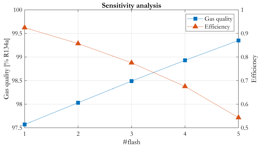
Figure 38: Sensitivity analysis on the multi-flash system. Increasing the number of stages the quality improves despite the efficiency decrement, from 0.92 down to 0.54.
