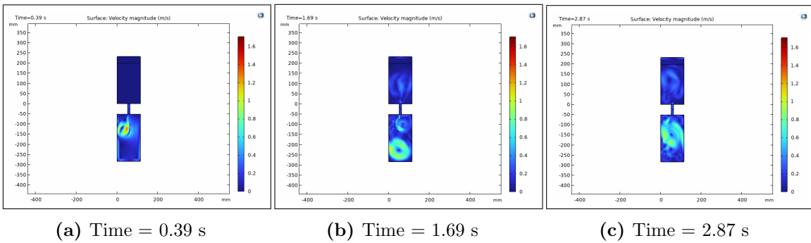
Figure 44: Velocity field time dependent study, with three consecutive frames. The liquid accelerates exiting the connecting pipe and, after touching the walls, it evaporates and the density difference generates the eddies (more evident at 1.69 s). Similar behaviour in top buffer, with the vapour phase encountering liquid mixture and inducing velocity gradients (dark and light blue).
