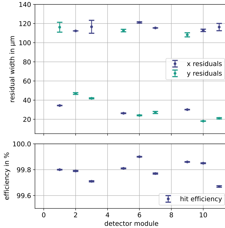
Figure 7.6: Residuals and hit-detection efficiency per detector module for primary protons in single track events. All modules investigated show an efficiency well above 99.6 %. Modules 0, 4 and 8 were not directly illuminated by the beam, thus there is insufficient data for an efficiency and residual measurement.
