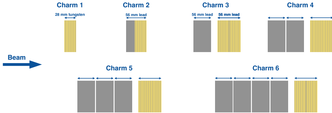
Figure A.3: Schematic layout of the six different target configurations. Adapted from [158, fig. 3].
