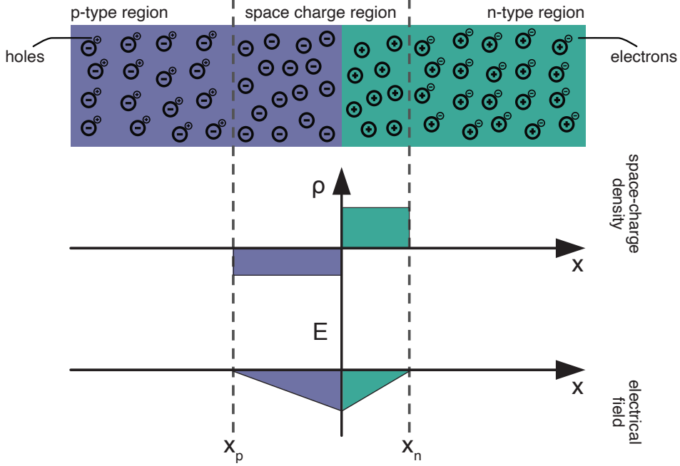
Figure 5.4: Representation of charge carrier density and electric field at an abrupt pn-junction, adapted from [122].
