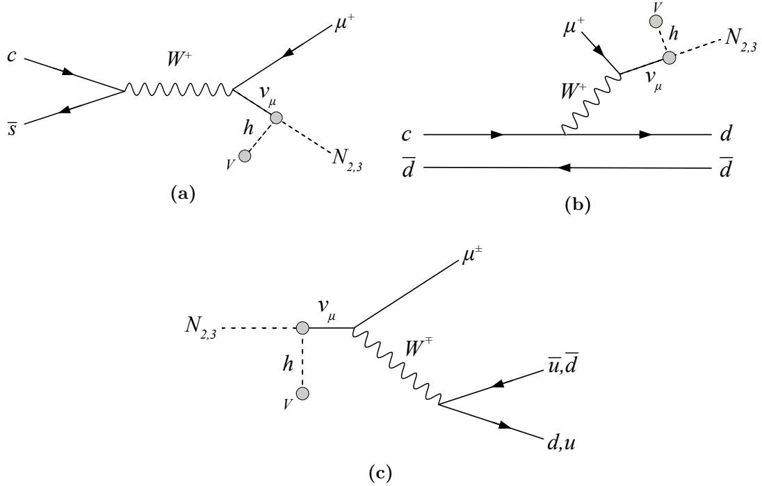
Figure 2.5: Production and decay of HNLs . A D_s meson decays to lepton and neutrino (a), the neutrino is mixing with the HNL , coupling to the Higgs with vacuum expectation value v . The 3-body production (b) is similar, with an additional \pi^0 produced in the D meson decay. In the decay (c) the HNL mixes with a neutrino which subsequently decays to \pi^\pm and \mu^\pm . Also, a 3-body decay N_{2,3} \rightarrow \mu e \nu is possible. Adapted from [56, p. 5; 57]
