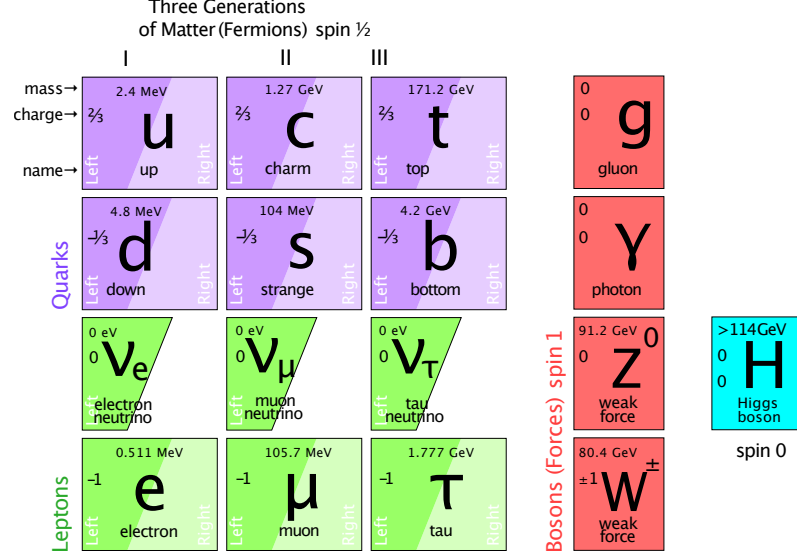
Figure 2.1: Particle content of the SM. Left are the fermions in three generations of quarks and leptons. The neutrinos are the only exclusively left-handed fermions. On the right are the bosons mediating the fundamental interactions, and the Higgs boson [5, p. 2].
