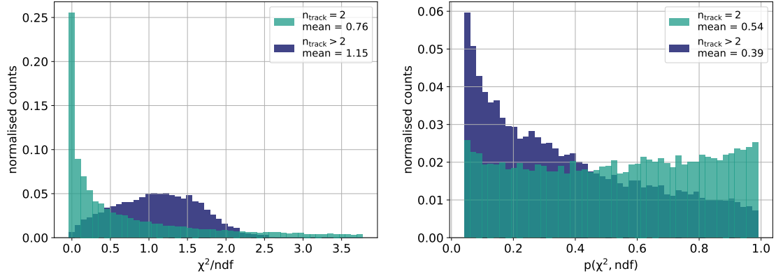
Figure 8.9: The \chi^2/\text{ndf} (left) and p -value (right) distributions in CHARM 2 run 1 for vertices with 2 tracks and more than 2 tracks after vertex finding and fitting. The histograms are normalised to one. The 2-track vertices only have one degree of freedom.
