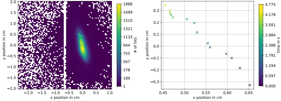
Figure 7.1: Reconstructed cluster centres on the first plane of the pixel detector for a primary proton run (left). The elliptical beam shape is visible. The coordinate system is aligned to the beam centre. Beam centre as a function of spill time for a primary proton spill (right). The colour codes the time relative to the SoS signal. A beam centre drift towards the upper left is visible.
