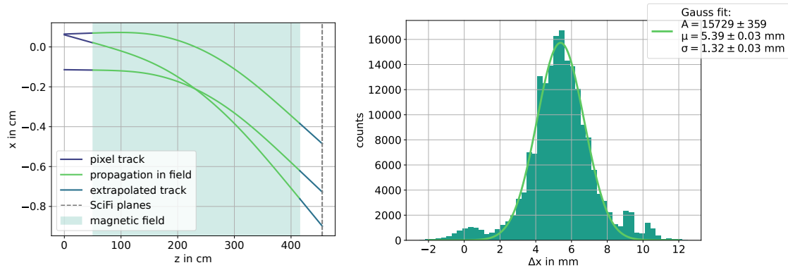
Figure 7.16: Track propagation through the GOLIATH magnetic field for three 400 GeV/ c proton tracks (left). Deflection in x of proton tracks at the first SciFi detector plane for an example run. The right-handed coordinate systems origin is the beam centre on the first pixel detector plane.
