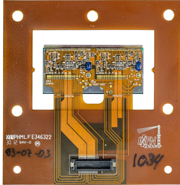
Figure 6.2: An ATLAS IBL DC module with one full size, planar sensor connected to two readout chips [142]. The flex PCB is glued on top of the sensor and electrically connected to the readout chip via wirebonds. The handling frame around is to be cut to shape prior to assembly inside a detector system.
