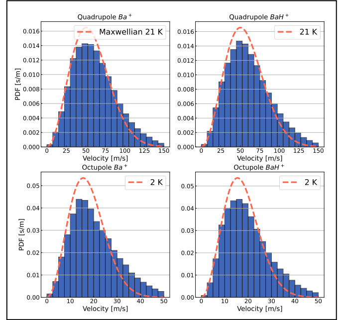
Figure 14. Speed distributions accumulated over the final secular period for simulations without lasers. Every speed histogram approximates Maxwell-Boltzmann distribution with a deviating tail which might be due to hotter particles experiencing larger potential and micromotion.
