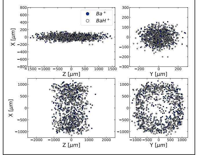
Figure 10. Final positions of 500 \text{Ba}^+ and 500 \text{BaH}^+ ions in quadrupole (top) and octupole (bottom) simulations without laser.
