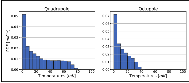
Figure 15. Hydrogen temperature distribution after photodissociating all \text{BaH}^+ ions at once.
