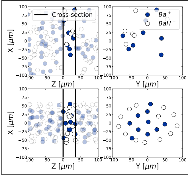
Figure 11. Cross-sections of the initial (top) and final (bottom) positions of ions in the z \in [0\mu\text{m}, 35\mu\text{m}] axial interval in the quadrupole simulation.
