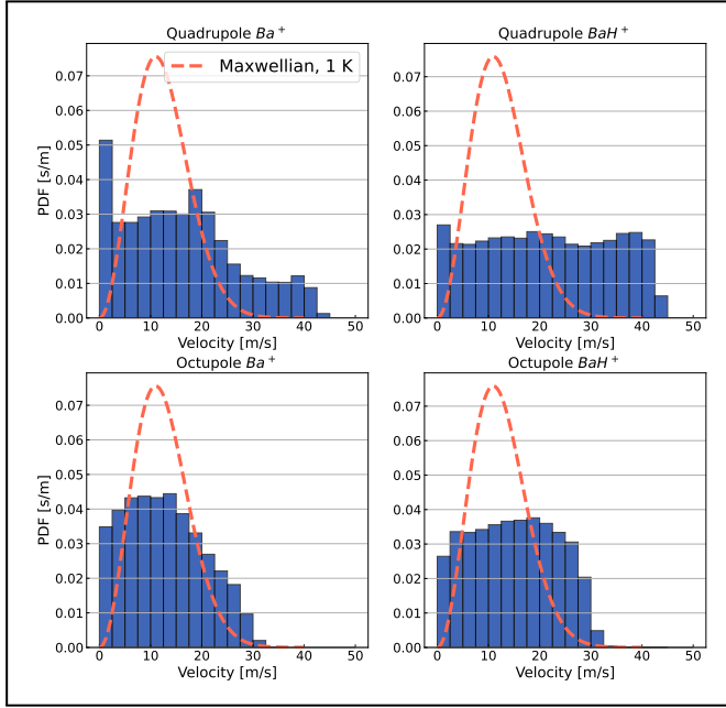
Figure 13. Speed distributions accumulated over the final secular period of the simulation for both the quadrupole and octupole simulations with laser cooling. The accumulated speeds are compared to the initial 1 K Maxwell-Boltzmann distribution.
