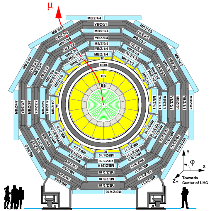
Figure 2.13: Layout of the CMS barrel muon DT chambers in one of the 5 wheels. Each wheel is divided into 12 sectors, each covering a 30° azimuthal angle, and consisting of 4 stations.
