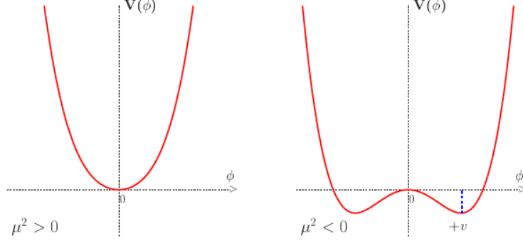
Figure 1.1: The potential V of the scalar field \phi in the case of \mu^2 > 0 , on the left. On the right the Higgs potential described from the last two terms of equation (1.36) with \mu^2 < 0 and \lambda > 0 . The potential minimum is not unique, in the latter case, but there is an infinite number of minimum points located on a continuous ring.
