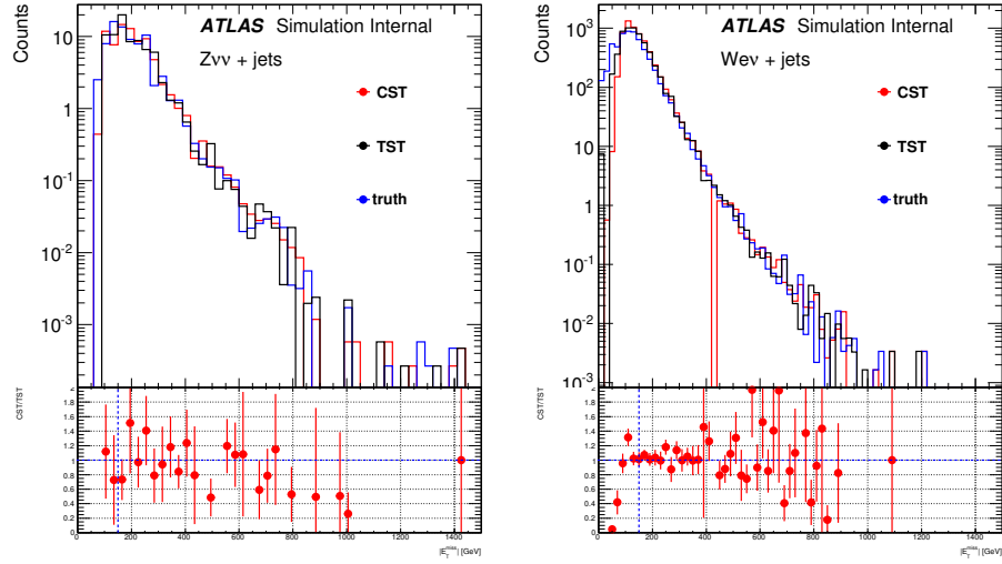
Figure 4.4: Example comparisons of CST and TST E_T^{\text{miss}} distributions in background MC. Left: Z \rightarrow \nu\nu in the signal region (except the E_T^{\text{miss}} cut). Right: W \rightarrow e\nu after the SR jet p_T , \Delta\eta_{jj} , and \Delta\phi_{jj} cuts.
