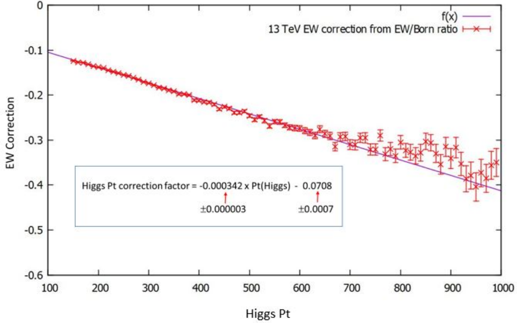
Figure 7.1: NLO electroweak corrections to the VBF signal production, in % of the nominal yield. A linear fit is also shown.
