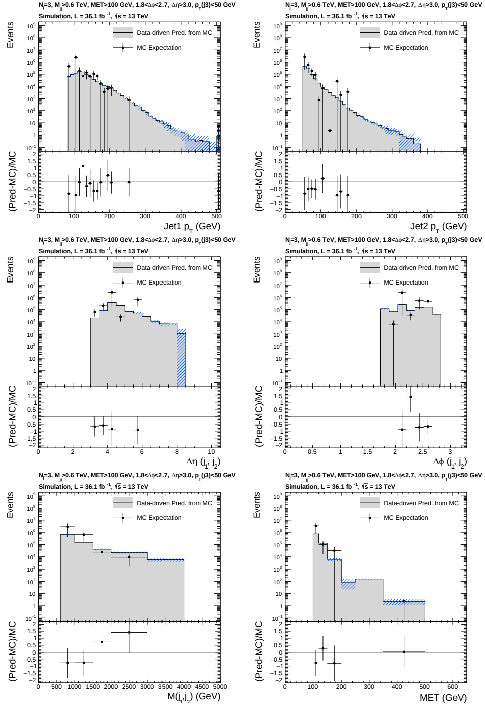
Figure 7.9: Kinematic distributions comparing multijet MC events to the R+S prediction from MC. The selection is the multijet validation region defined in the text.
