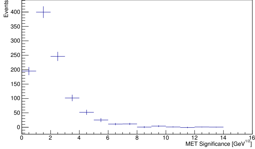
Figure 7.11: E_T^{\text{miss}} \text{sig.} template shape for fake electrons in the inclusive W \rightarrow e\nu control region. In practice, three of these are used (one for each m_{jj} bin).
