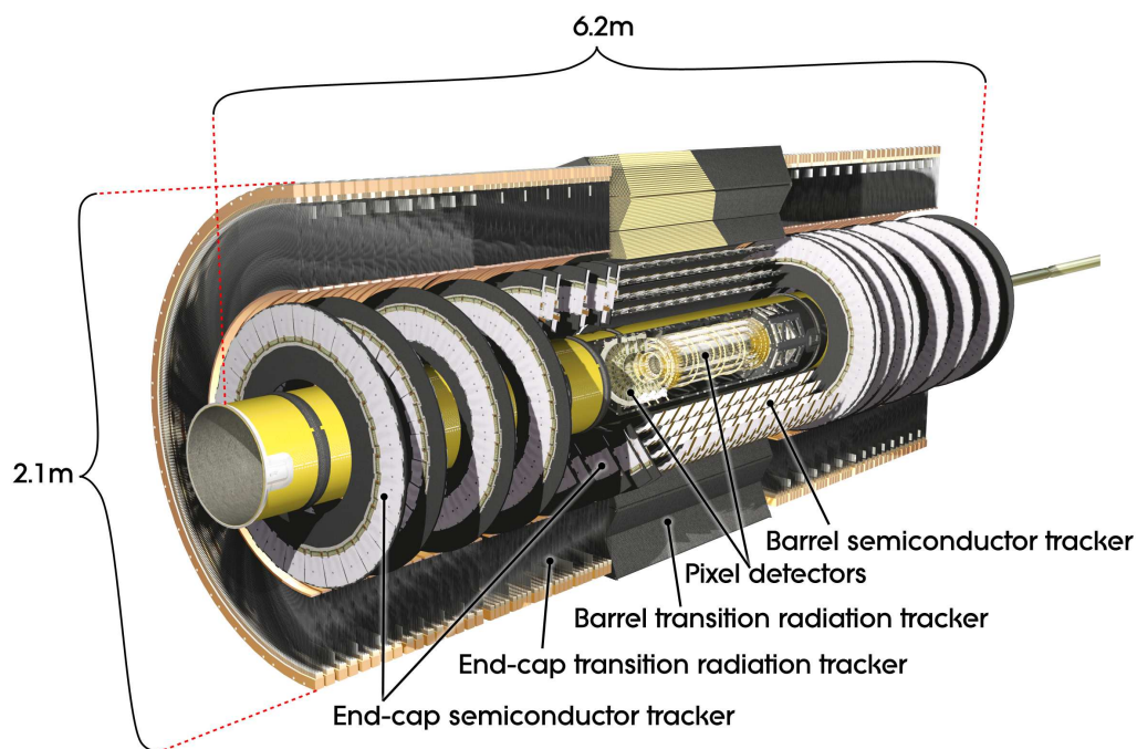
Figure 3.3: General cut-away view of the Inner Detector [55].
