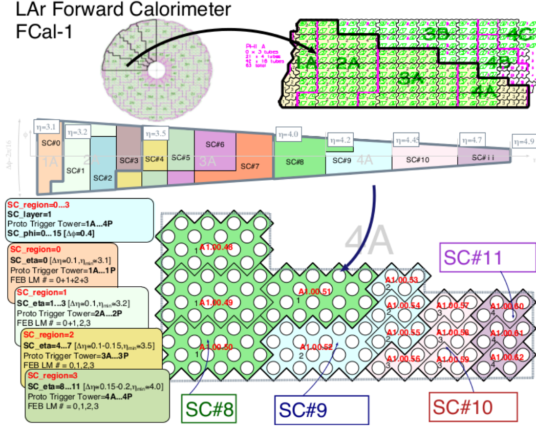
Figure 5.9: Planned supercell layout for FCAL1. Layers 2 and 3 of the FCAL also have 16 wedges in \phi , but are divided into only 8 and 4 supercells in \eta respectively.
