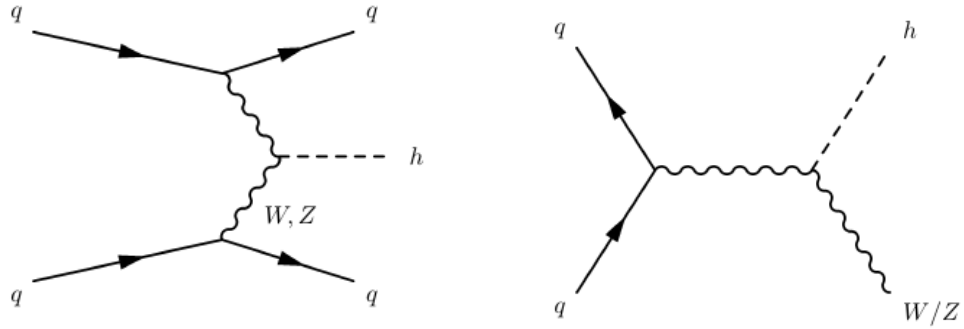
Figure 2.2: Feynman diagrams for Higgs production via weak vector boson fusion ( left ) and W/Z associated production ( right ).
