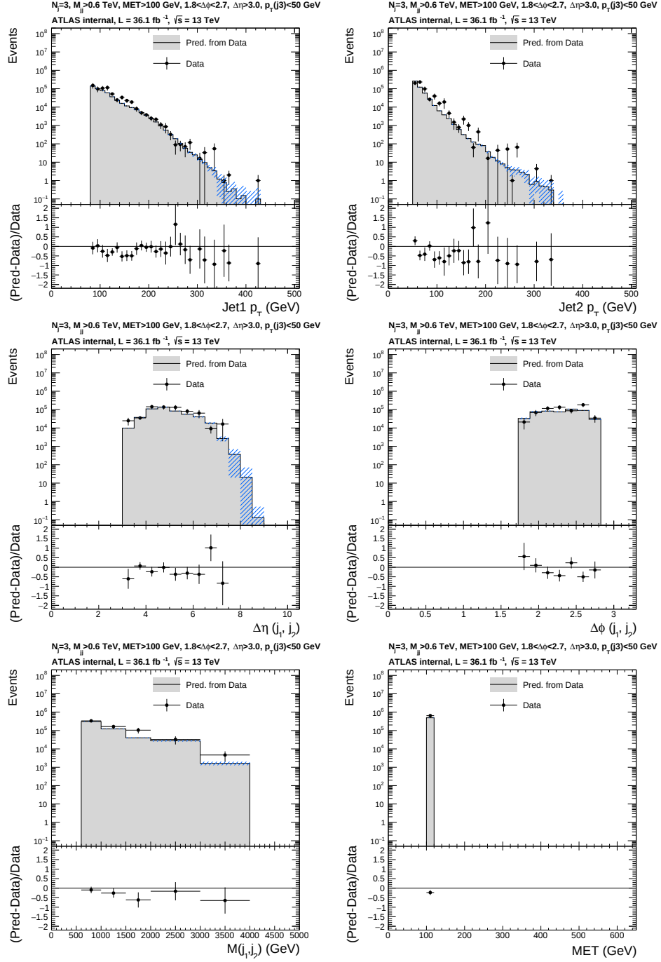
Figure 7.10: Kinematic distributions comparing data events to the R+S prediction from those same events. The selection is the multijet validation region defined in the text. All distributions except E_T^{\text{miss}} have an additional requirement of E_T^{\text{miss}} < 120 GeV to suppress non-multijet backgrounds. Non-multijet backgrounds are not shown.
