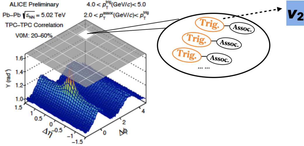
Figure 6.5: The TPC-TPC correlation function is divided into many regions. In each region, particle pairs are found. The v_2 of the trigger particles in TPC-TPC particle pairs is further calculated.
