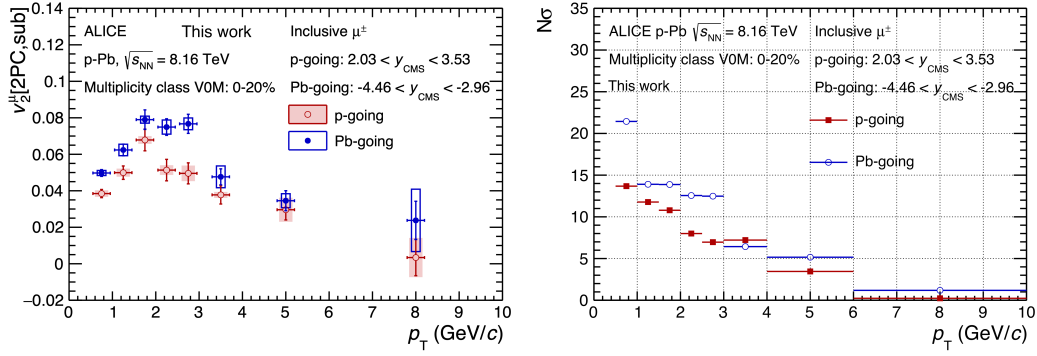
Figure 5.28: Left: comparison between the inclusive muon v_2 with the two-particle correlation method in high-multiplicity p-Pb and Pb-p collisions at \sqrt{s_{NN}} = 8.16 TeV. Right: the significance of a positive muon v_2 as a function of p_T in high-multiplicity p-Pb and Pb-p collisions at \sqrt{s_{NN}} = 8.16 TeV.
