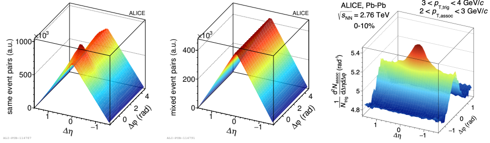
Figure 2.1: Example of the di-hadron correlation yield per trigger particle as a function of \Delta\varphi and \Delta\eta measured in 0–10% most central Pb–Pb collisions at \sqrt{s_{\text{NN}}} = 2.76 TeV, for same (left) and mixed (middle) events. Right: the di-hadron correlation yield per trigger particle after the event mixing correction. Figure taken from [116].
