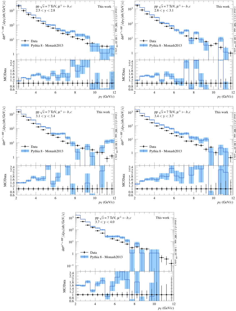
Figure D.8: The comparison of p_T -differential production cross section of muons from heavy-flavour hadron decays in five rapidity regions between the data and PYTHIA8. The data points are from [237].
