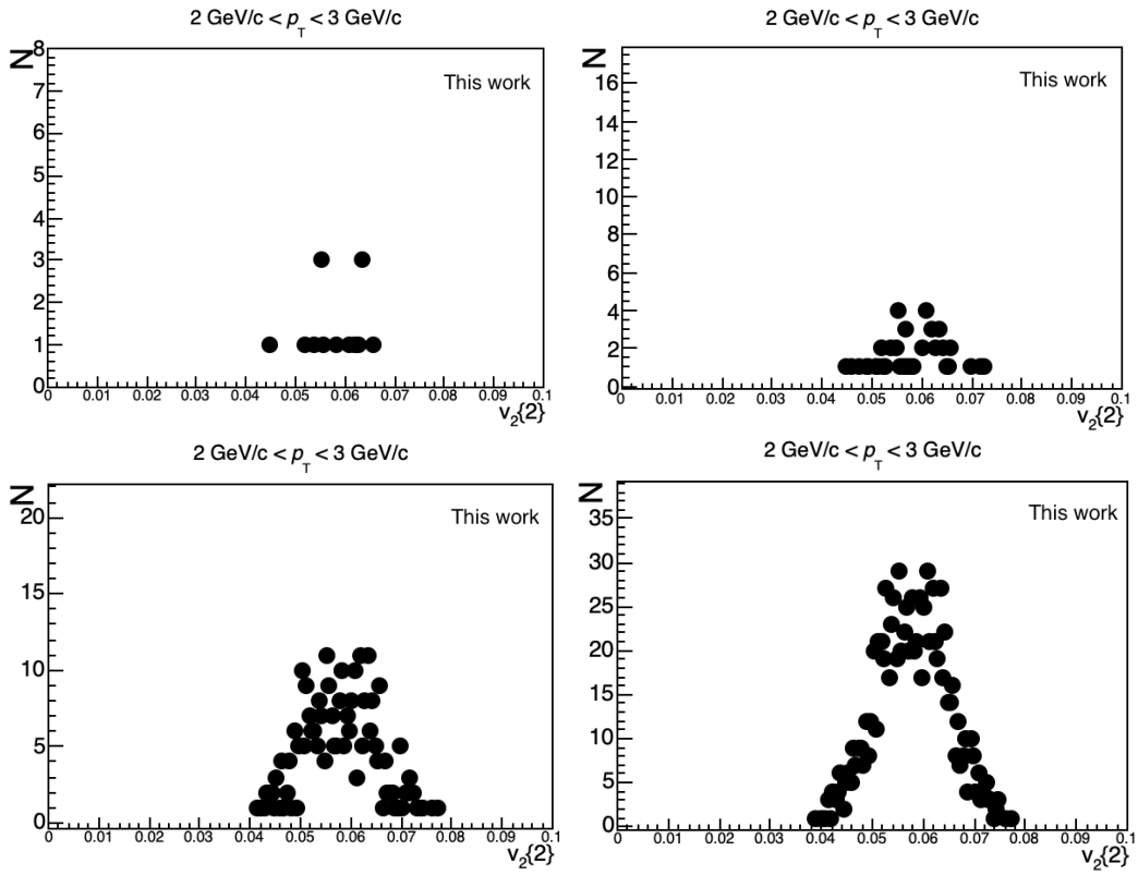
Figure 5.25: The v_2 distribution in 2 < p_T < 3 GeV/c interval with 15 trials (upper left), 50 trials (upper right), 300 trials (lower left) and 900 trials (lower right).
