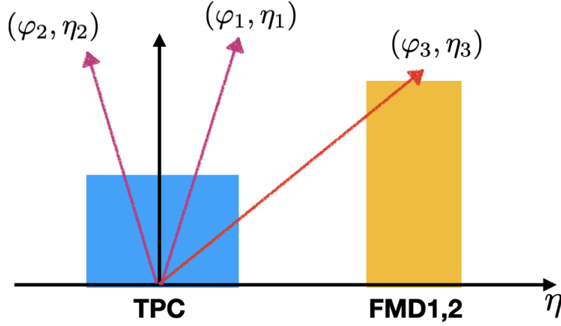
Figure 6.14: The selection of three particles in the jet-particle v_2 measurement in p–Pb collisions at \sqrt{s_{NN}} = 5.02 TeV. Two particles are chosen in the TPC acceptance and the third particle is in FMD1,2.
