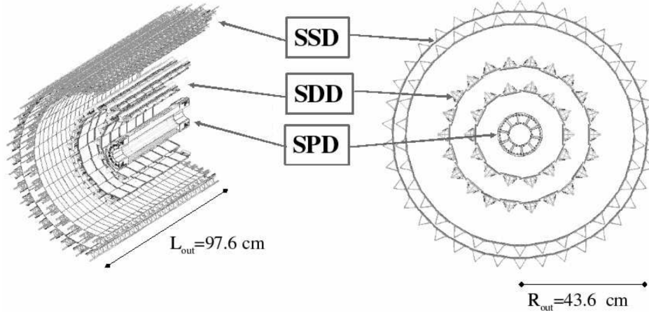
Figure 3.3: The Schematic layout of the ALICE Inner Tracking System. Figure taken from [124].
