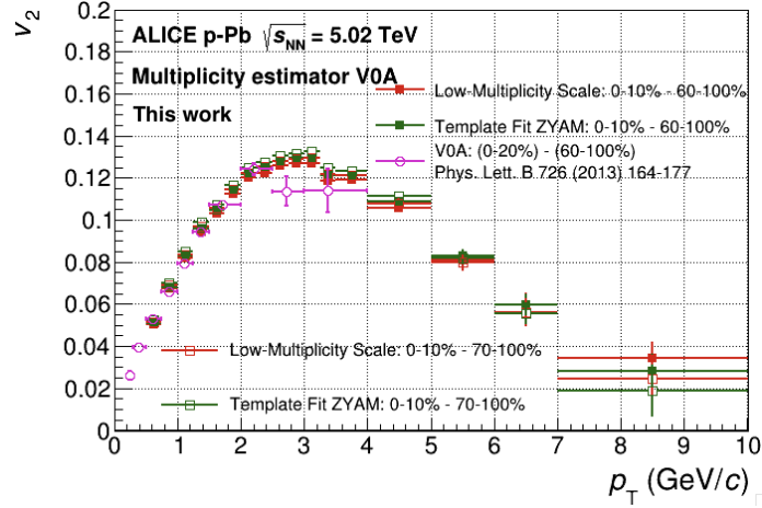
Figure 6.10: Comparison between the inclusive charged-particle v_2 at mid-rapidity obtained with the subtraction method and the template fit 6 method in p-Pb collisions at \sqrt{s_{NN}} = 5.02 TeV and the published same measurement obtained with the subtraction method in 0–20% multiplicity class [93]. The results obtained with the nonflow subtraction methods performed in lower multiplicity (70–100%) collisions are also shown.
