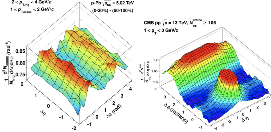
Figure 1.26: Left: associated yield per trigger particle in \Delta\phi and \Delta\eta for hadron-hadron correlations in p-Pb collisions at \sqrt{s_{\text{NN}}} = 5.02 TeV for the 0–20% multiplicity class, after subtraction of the associated yield obtained in the 60–100% event class, measured by ALICE. Right: the associated yield per trigger particle in \Delta\phi and \Delta\eta for hadron-hadron correlations in pp collisions at \sqrt{s} = 13 TeV for a high-multiplicity sample ( N_{\text{trk}}^{\text{offline}} \geq 105 ), measured by CMS. Figures are taken from [92, 93].
