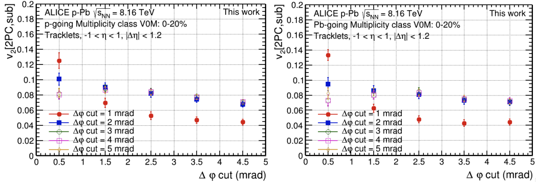
Figure A.1: The v_2 of the SPD tracklets as a function of the \Delta\varphi selections applied on the trigger-particle in p-Pb (left) and Pb-p (right) collisions. Different colors represent the different \Delta\varphi selections for associated SPD tracklets.
