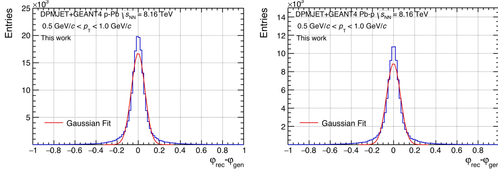
Figure B.1: \varphi_{\text{Rec}} - \varphi_{\text{Gen}} distribution of muon tracks with 0.5 < p_T < 1 GeV/c estimated from MC simulations with the DPMJET event generator and GEANT4 transport code in p-Pb (left) and Pb-p (right) collisions. The lines correspond to the fit with a Gaussian function.
