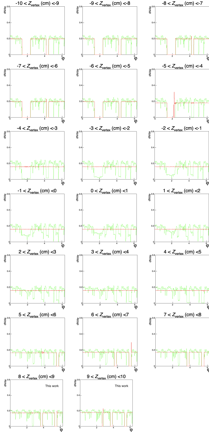
Figure C.7: The \varphi distribution of SPD tracklets before (green lines) and after (red lines) the NUA correction. The same Z_{\text{vertex}} intervals as in Fig. C.4 are employed.
