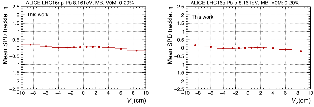
Figure C.5: The average \eta of SPD tracklets as a function of Z_{\text{vertex}} in p-Pb (left) and Pb-p (right) collisions.
