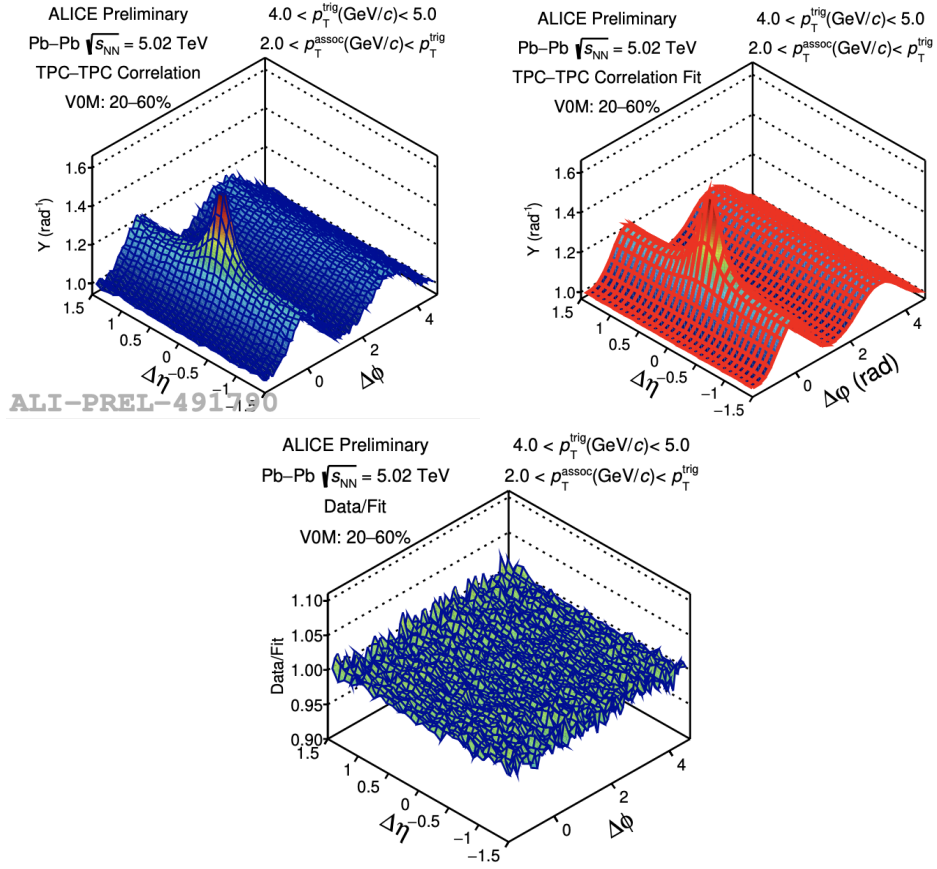
Figure 6.3: Upper left: the associated yield per trigger particle in TPC-TPC correlations for Pb-Pb collisions at \sqrt{s_{NN}} = 5.02 TeV. Upper right: the fit of TPC-TPC correlations. Bottom: the ratio between the data and fit.
