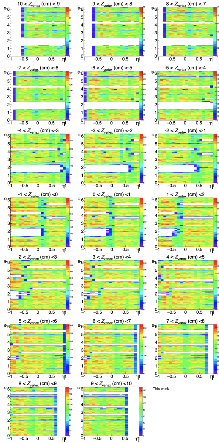
Figure C.4: SPD tracklet \eta - \phi map ( \eta as x -axis, \phi as y -axis) in different Z_{\text{vertex}} bins for MSL-triggered events in the 0–20% high-multiplicity p–Pb collisions selected with the V0M estimator.
