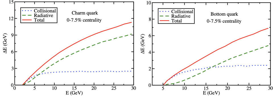
Figure 1.11: Comparison of radiative and collisional energy loss for charm (left) and beauty (right) quarks as a function of the quark energy. Figures are taken from [43].
