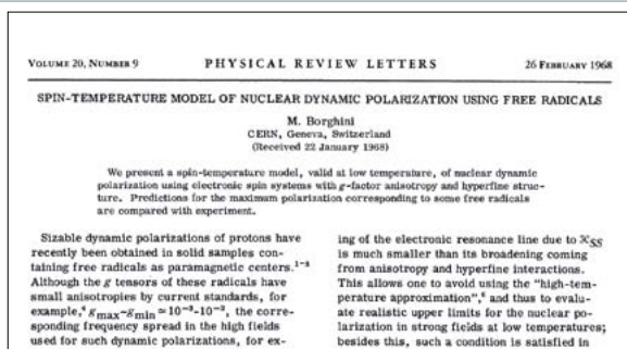
Michel's 1968 paper on his "spin-temperature model".
