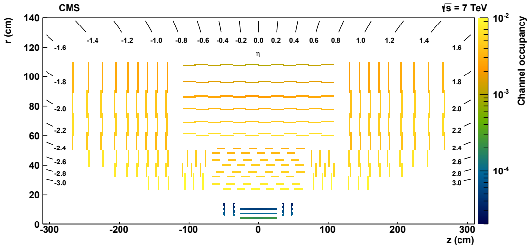
Figure 3.9: Map of typical occupancy across the CMS tracker. Based on measurement at \sqrt{s} = 7 TeV with an average of 9 pp interactions per beam crossing. [14]
