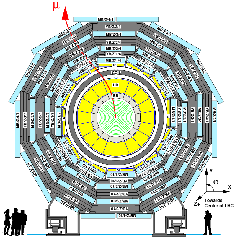
Figure 3.28: Diagram of the muon barrel system, with 4 layers of muon detectors (blue, “MB”) interleaved with the magnet yoke (“YB”) [9].
