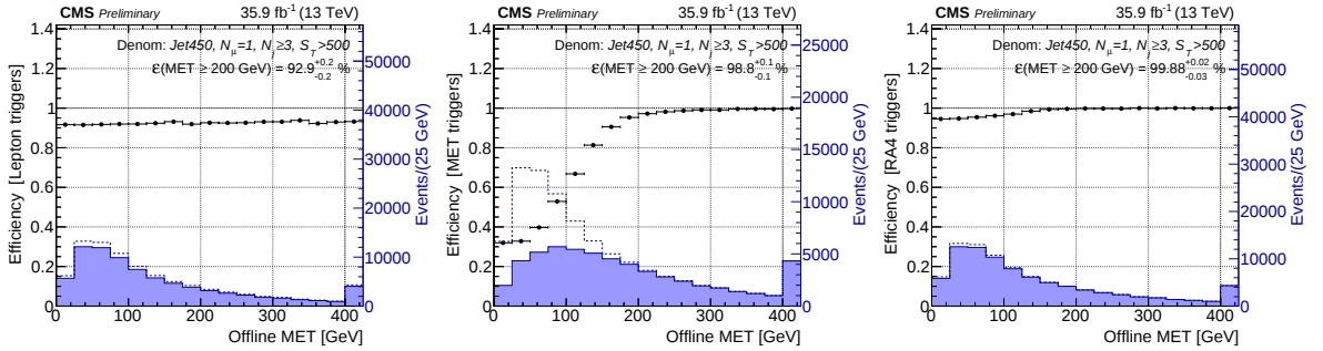
Figure 6.2: Combined trigger efficiencies as a function of E_T^{\text{miss}} in muon events for the OR of all lepton triggers (left), all E_T^{\text{miss}} triggers (center), and all lepton and E_T^{\text{miss}} triggers together (right). The efficiencies are measured using a data sample collected using the HLT_PFJet450 and HLT_AK8PFJet450 triggers, and offline requirements of one muon, 3 or more jets, and S_T > 500 GeV [67].
