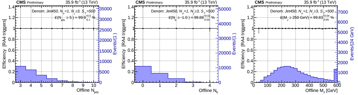
Figure 6.4: Trigger efficiencies in muon events as a function of N_{\text{jets}} (left), N_b (center) and M_J (right). The efficiencies are measured using a data sample collected using the HLT_PFJet450 and HLT_AK8PFJet450 triggers, and offline requirements of one electron, 3 or more jets, and S_T > 500 GeV and E_T^{\text{miss}} > 200 GeV [67].
