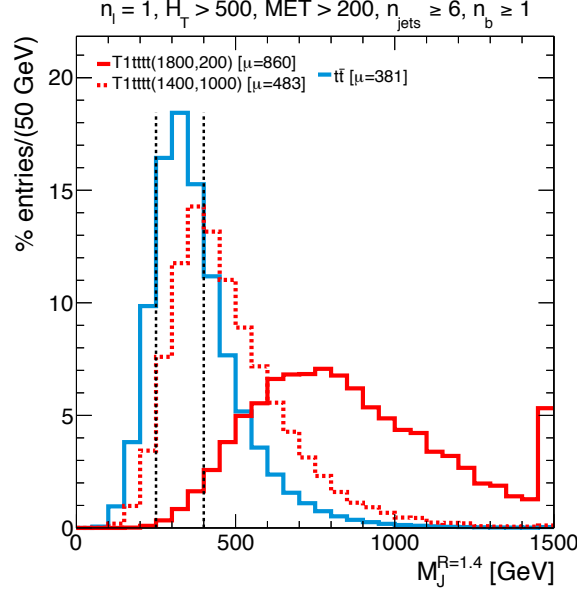
Figure 8.1: Shape comparison of M_J distributions in t\bar{t} events (blue) and T1tttt events (red), for compressed and non-compressed model points (dashed and solid, respectively). The selection is similar to the baseline selection [67].
