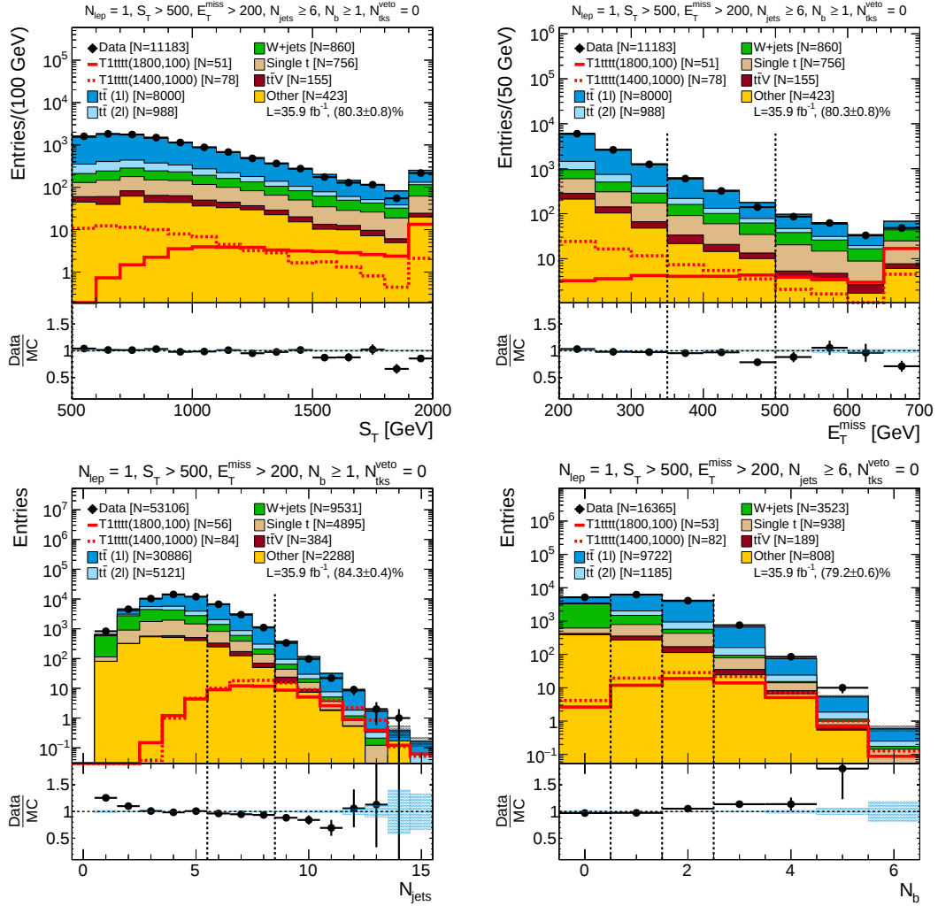
Figure 7.1: Distributions of key variables for the baseline selection, in data (points) and Monte Carlo (stacked histograms). S_T and E_T^{\text{miss}} are shown in the top row; N_{\text{jets}} and N_b in the bottom row. Baseline selection is applied, except for the variable plotted. The blue hatched area in the ratio panel indicates the statistical uncertainty of the simulation. The simulations are normalized to the number of events observed in data for each selection, amounting to approximately 80-85% of the expectation based on luminosity. The precise normalization ratio is shown in parentheses on each frame [67].
