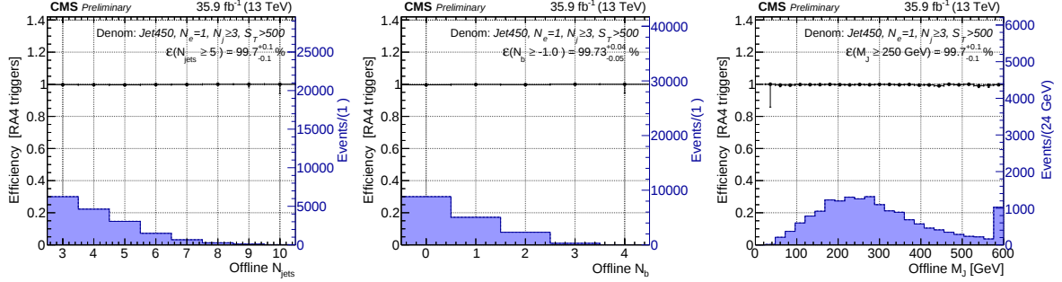
Figure 6.3: Combined trigger efficiencies in electron events as a function of N_{\text{jets}} (left), N_b (center) and M_J (right). The efficiencies are measured using a data sample collected using the HLT_PFJet450 and HLT_AK8PFJet450 triggers, and offline requirements of one electron, 3 or more jets, and S_T > 500 GeV and E_T^{\text{miss}} > 200 GeV [67].
