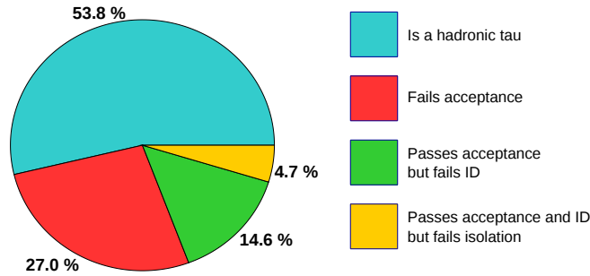
Figure 7.4: Composition of lost leptons by mutually exclusive category. “Failing acceptance” indicates the presence of electrons and muons with p_T < 20 \text{ GeV} [67].
