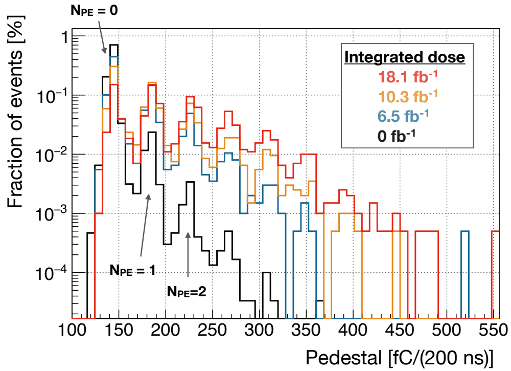
Figure 3.24: Photoelectron charge spectrum from a single SiPM after various exposures in situ in CMS. This SiPM was connected to the scintillator tile at i\text{Eta} = 29 , i\text{Phi} = 63 , and depth = 1. The position of the N_{\text{PE}} = 0 peak is determined by the QIE pedestal current.
