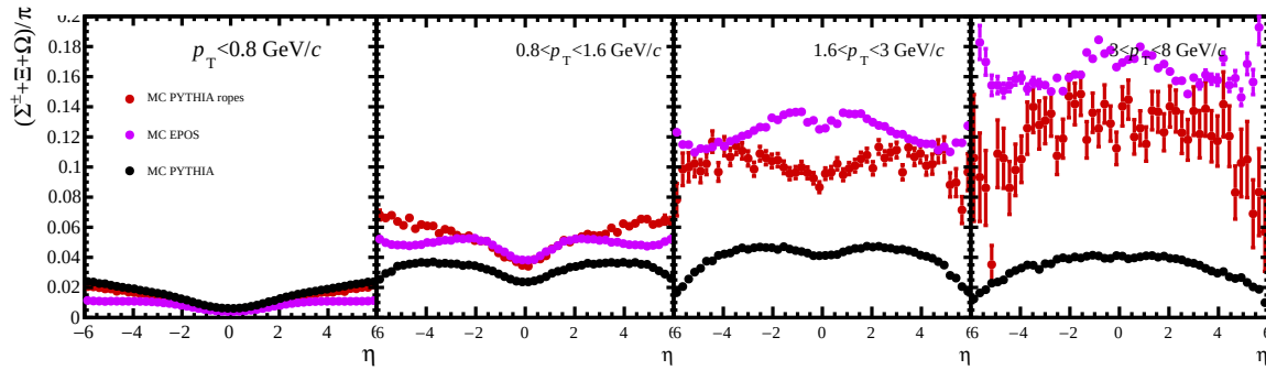
Figure 5.26: (\Sigma^\pm + \Xi^\pm + \Omega^-)/\pi ratios in pp collisions at 5 TeV as predicted by EPOS, PYTHIA with official LHCb tune and PYTHIA with string-string interactions.
