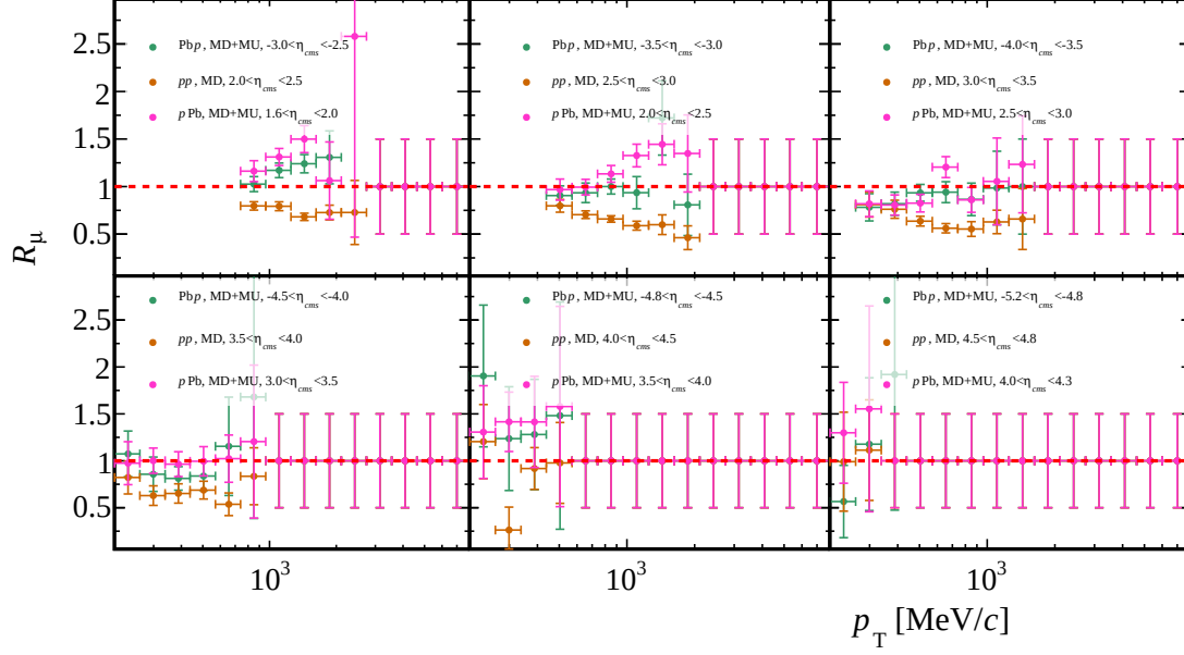
Figure 6.36: Results for R_{X \rightarrow \mu} in Pbp , pPb and pp collisions. The values have been obtained using Eq. 6.17 and considering the criteria of Tab. 6.5.
