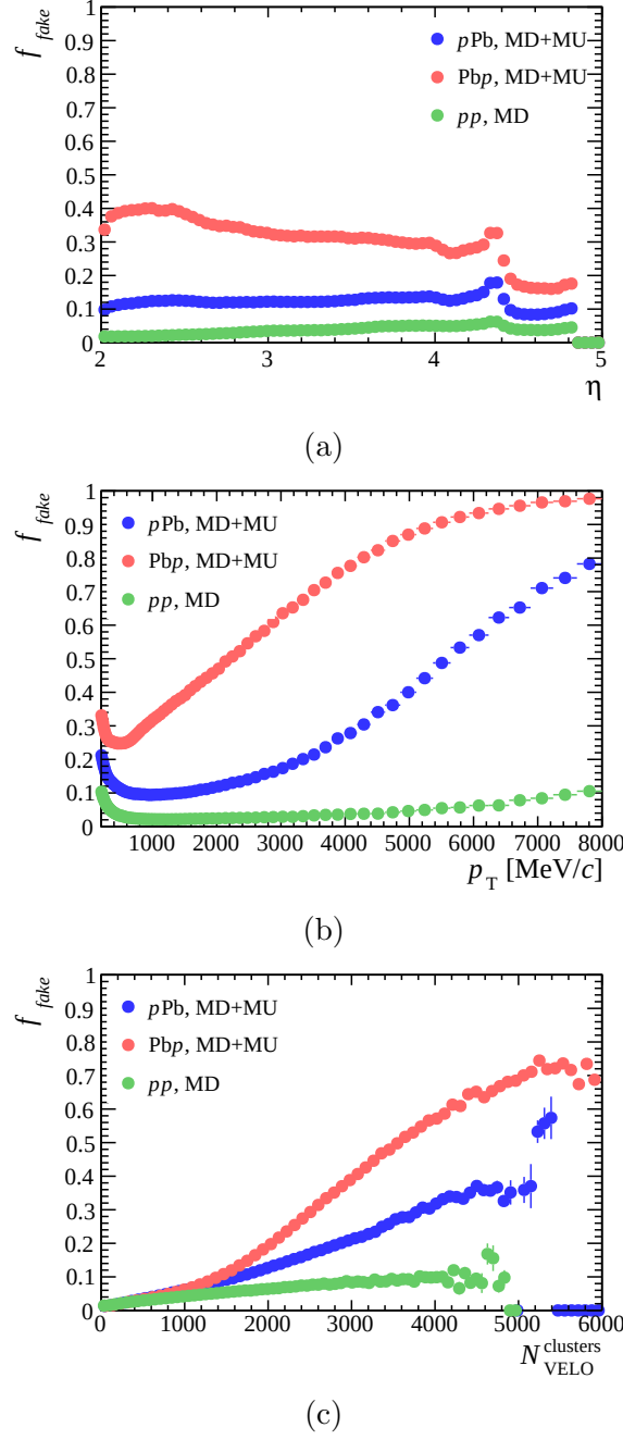
Figure 5.8: Fraction of fake tracks in simulation as a function of \eta (Fig. 5.8a), p_T (Fig. 5.8b) and N_{VELO}^{clusters} (Fig. 5.8c), for the different configurations. The simulation is weighted with set 1 for pPb and Pbp and set 12 for pp , in order to adjust the detector occupancy to data. No track quality selection is applied apart from the requirements at the reconstruction level. Both magnet configurations are merged for proton-lead data as no difference between the two polarities is seen.
