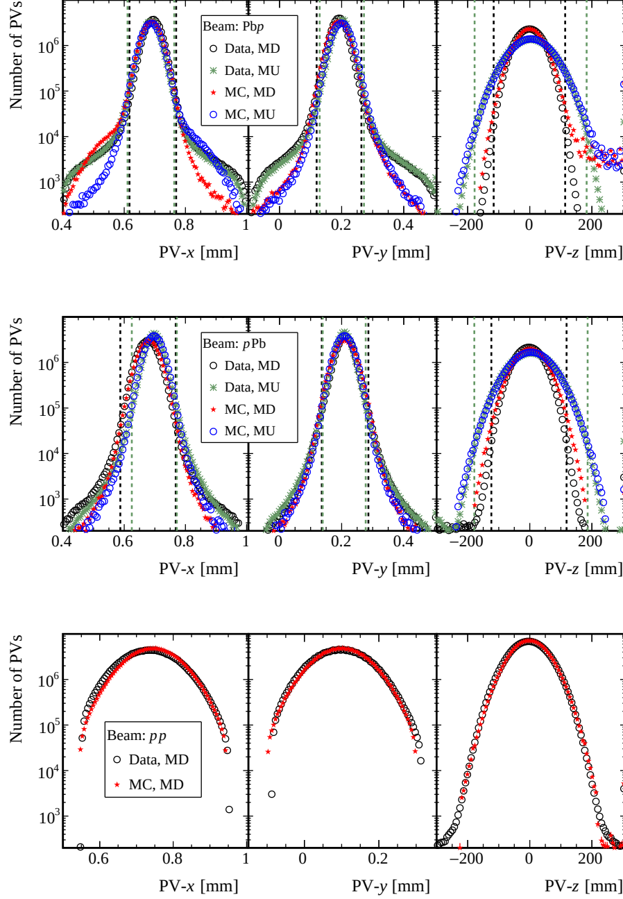
Figure 5.1: Spatial reconstructed primary vertex distribution for Pbp (top), p\text{Pb} (middle) and pp (bottom) configurations. Black and green dots represent data, while red and blue dots represent simulation. Vertical axis are expressed in logarithmic scale, to ease the visualisation of the background. Simulation is scaled to the total number of PVs in data. Dashed vertical bars indicate the boundaries of the luminous region.
