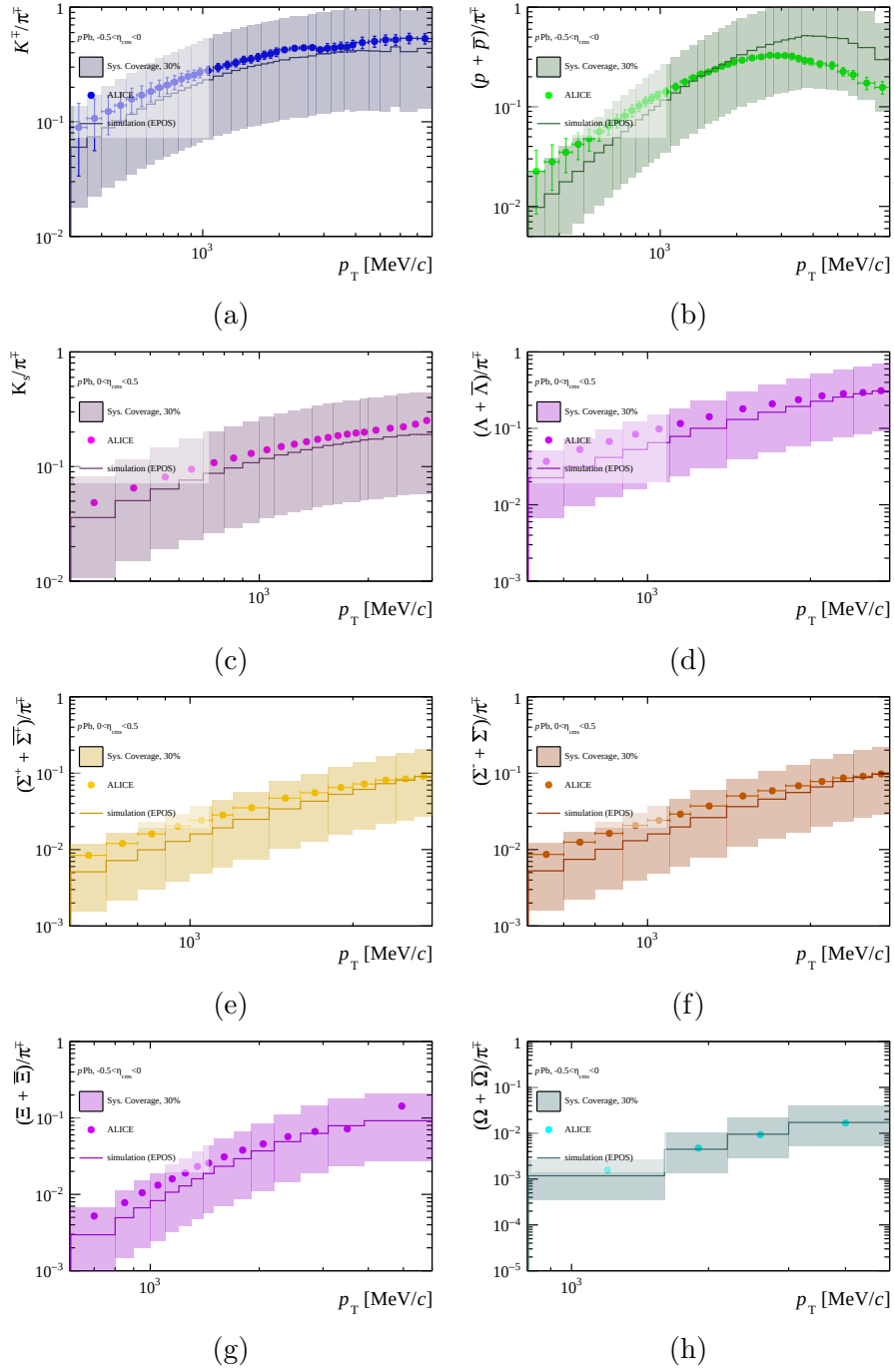
Figure 5.27: Comparison of the hadron/ \pi ratio for Pbp ( -0.5 < \eta_{\text{cms}} < 0.5 ) and pPb ( 0 < \eta_{\text{cms}} < 0.5 ) collisions in simulation (EPOS) and ALICE data [93, 168, 169]. The band corresponds to a 30% variation of the ratio. Error bars in ALICE data represent the systematic and statistical uncertainty added in quadrature, but they are only displayed in the K/\pi and p/\pi ratios.
