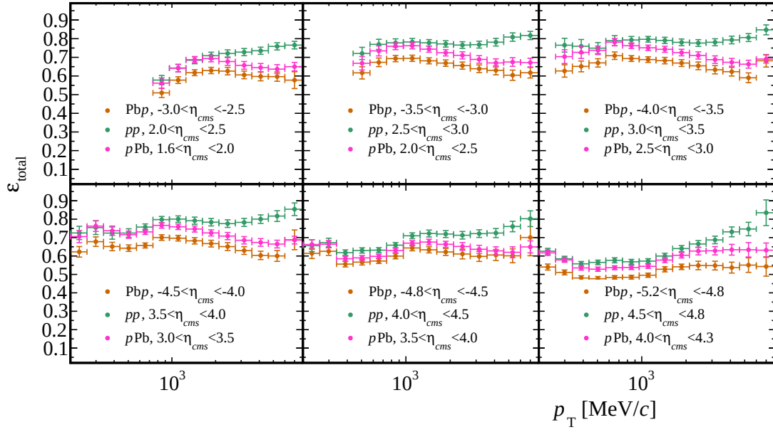
Figure 6.51: \varepsilon_{\text{total}} in PbPb, pPb and pp dataset.
