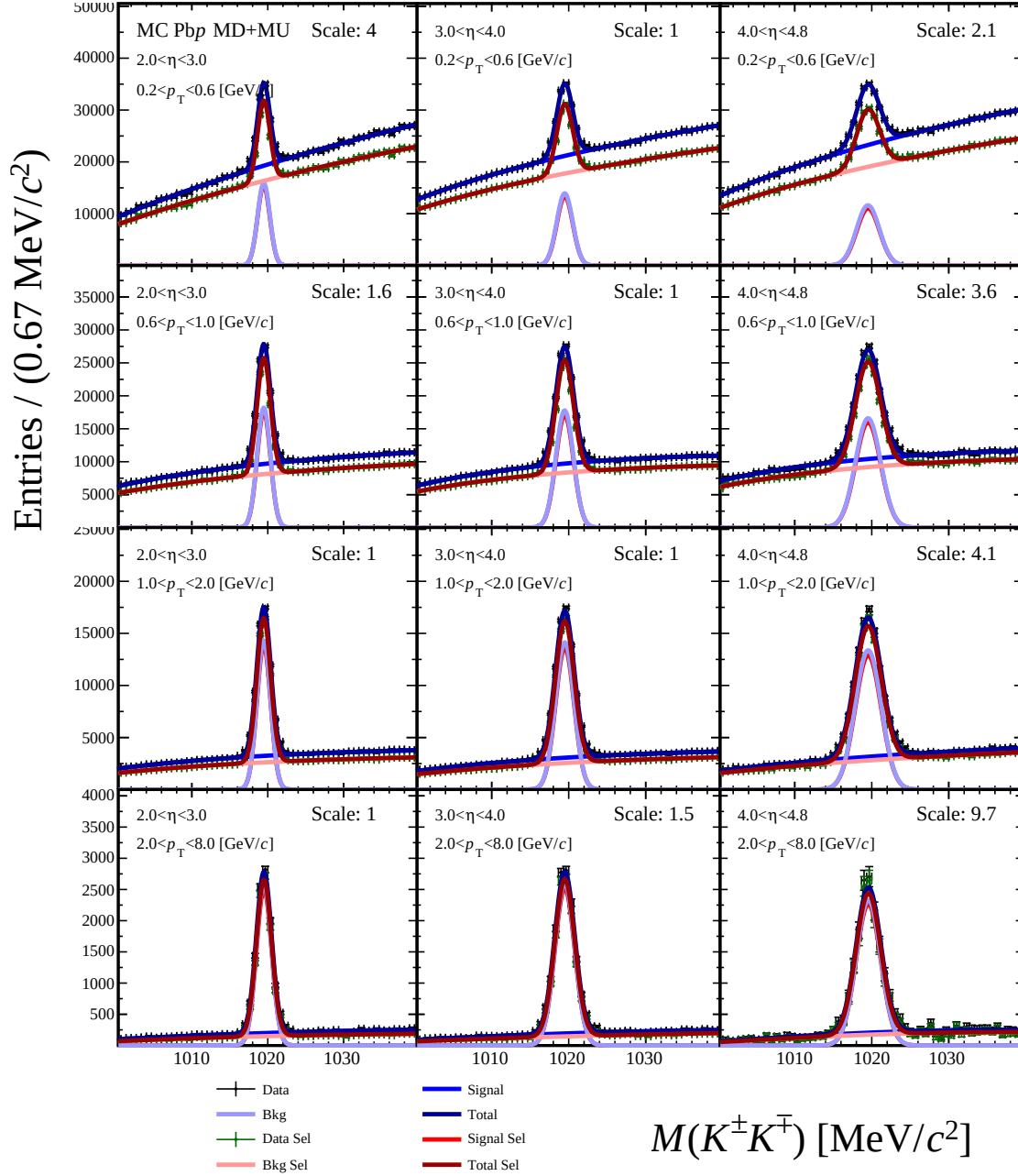
Figure B.8: Signal extraction of \phi \rightarrow K^\pm K^\mp for the simulation sample of the Pbp collisions in the different (\eta, p_T) kinematic bins. The (\eta, p_T) values are indicated in the top left side of each plot. Some plots are re-scaled to make them appear in the centre of the plot, the scale factor is indicated in the top right side.
