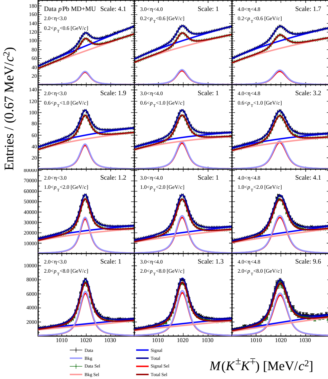
Figure B.12: Signal extraction of \phi \rightarrow K^\pm K^\mp for data sample p\text{Pb} collisions for the different kinematic bins ( \eta, p_T ). The ( \eta, p_T ) values are indicated in the top left side of each plot. Some plots are re-scaled to make them appear in the centre of the plot, the scale factor is indicated in the top right side.
