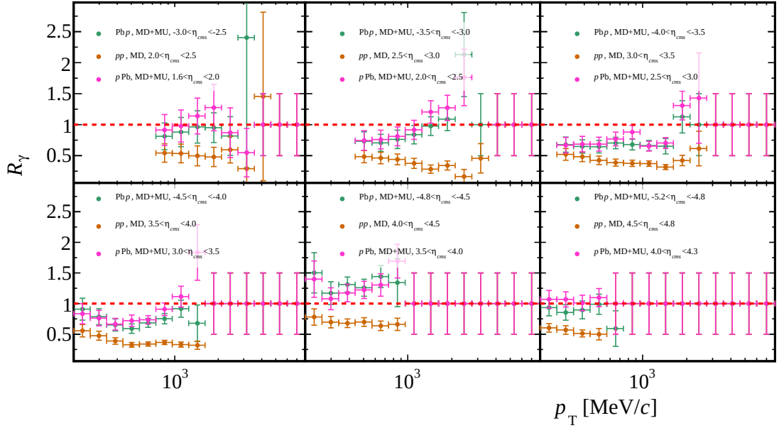
Figure 6.35: Results for R_\gamma in PbPb, pPb and pp collisions. The values have been obtained using Eq. 6.17 and considering the criteria of Tab. 6.5.
