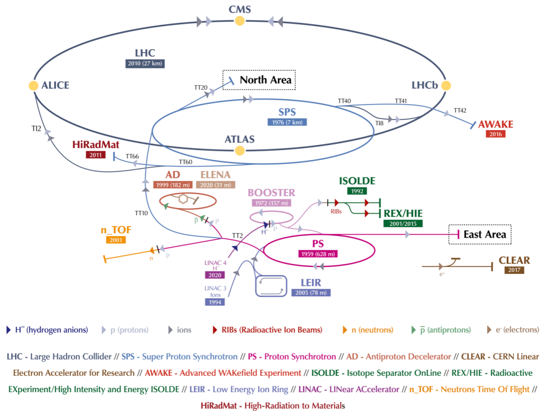
Figure 3.1: Diagram of the CERN accelerator complex in 2019. Note that the new LINAC4 substitutes the LINAC 2, which was operating during Run 1 and Run 2. Figure from [105].
