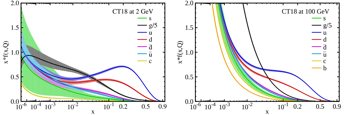
Figure 2.2: Parton distribution functions from the CT18 analysis [23] at Q = 2 GeV (left) and Q = 100 GeV (right), considering natural units, for u , \bar{u} , d , \bar{d} , s = \bar{s} , b = \bar{b} and g . The gluon PDF is scaled as g(x, Q)/5 in all instances, and the charm distribution c(x, Q) is perturbatively generated by evolving from Q_0 = 1.3 and 1.4 GeV. The band around each contribution represents the estimated uncertainty.
