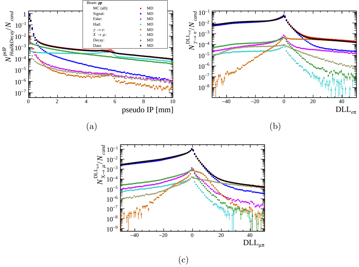
Figure 6.29: pseudoIP , DLL_{e\pi} and DLL_{\mu\pi} distributions for pp . Black markers correspond to real data, while the rest of the colours correspond to simulation, which is weighted with set 12 for pp . Requirements from Tab. 6.5 are applied and each sample is normalised to the number of candidates.
