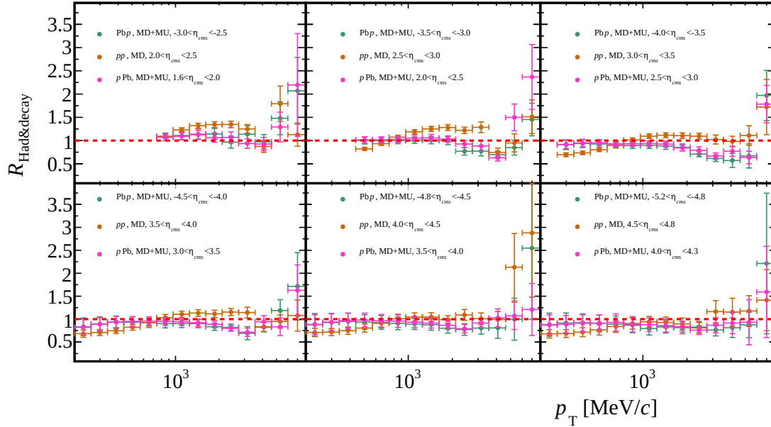
Figure 6.37: Results for R_{\text{had\&decays}} in Pbp , pPb and pp collisions. The values have been obtained using Eq. 6.17 and considering the criteria of Tab. 6.5.
