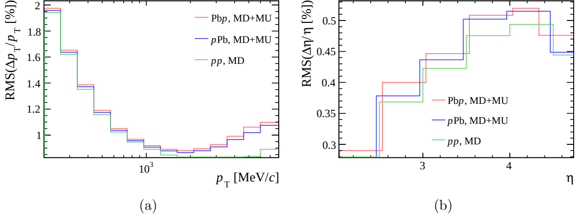
Figure 6.46: Resolution of LHCb in p_T and \eta for matched candidates. The showed bins correspond to the (\eta, p_T) bins covered in the analysis.
