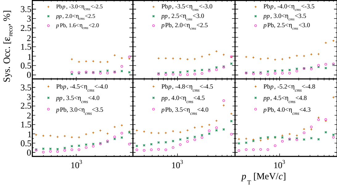
Figure 7.2: Relative systematic uncertainty in \varepsilon_{\text{reco}} from detector occupancy description for PbPb, pPb and pp data.
