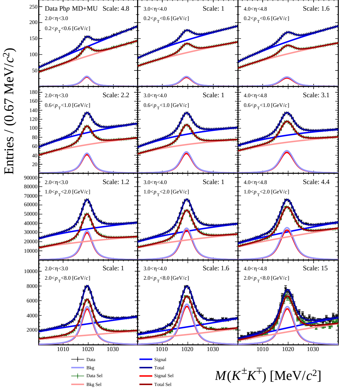
Figure B.11: Signal extraction of \phi \rightarrow K^\pm K^\mp for data sample of Pbp collisions for the different kinematic bins (\eta, p_T) . The (\eta, p_T) values are indicated in the top left side of each plot. Some plots are re-scaled to make them appear in the centre of the plot, the scale factor is indicated in the top right side.
