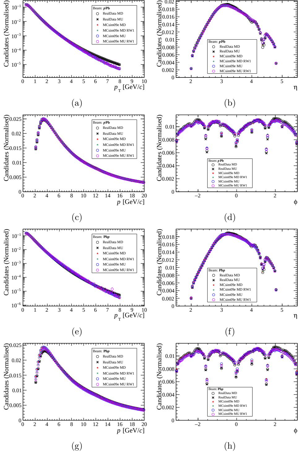
Figure 5.20: Distribution of candidate tracks with respect to p_T , \eta , p and \phi in simulation and data for the p\text{Pb} and \text{PbP} datasets.
