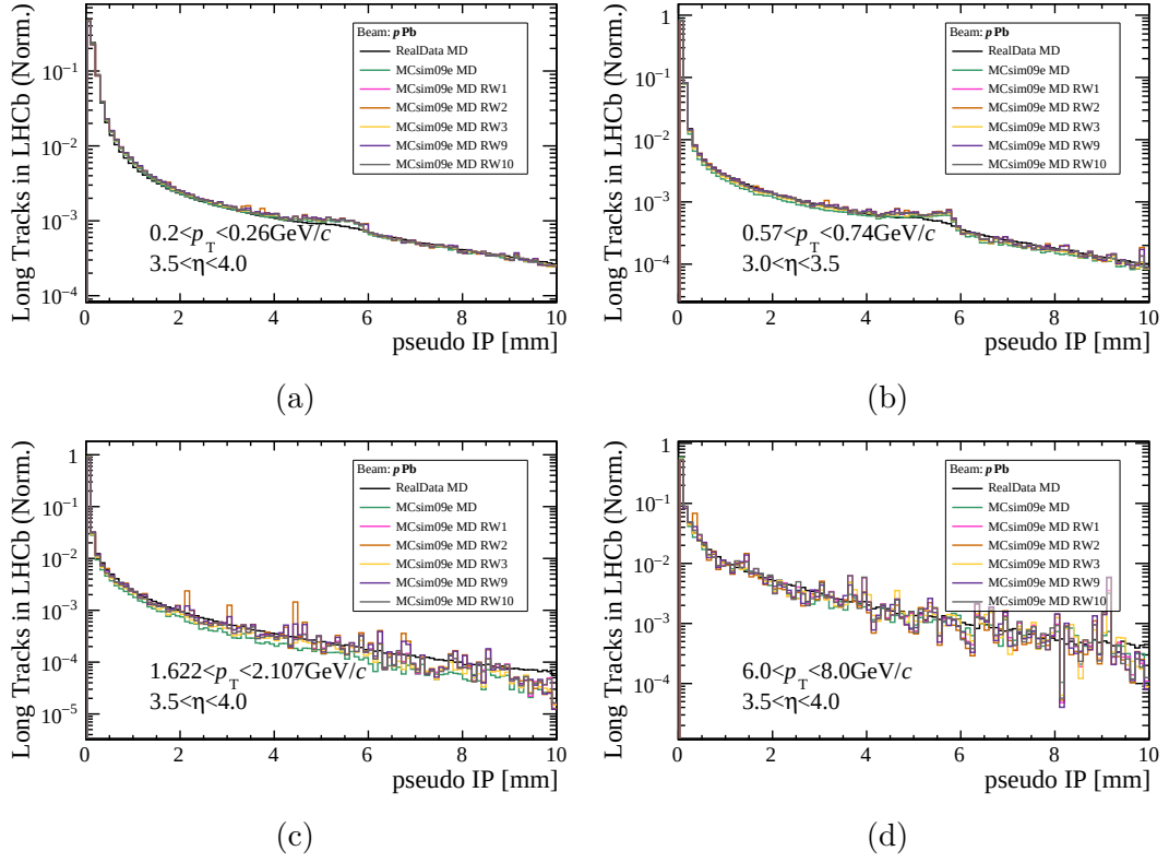
Figure B.3: Distributions of long tracks in the LHCb acceptance with respect to pseudoIP for particular (\eta, p_T) ranges in data and simulation for the pPb dataset.
