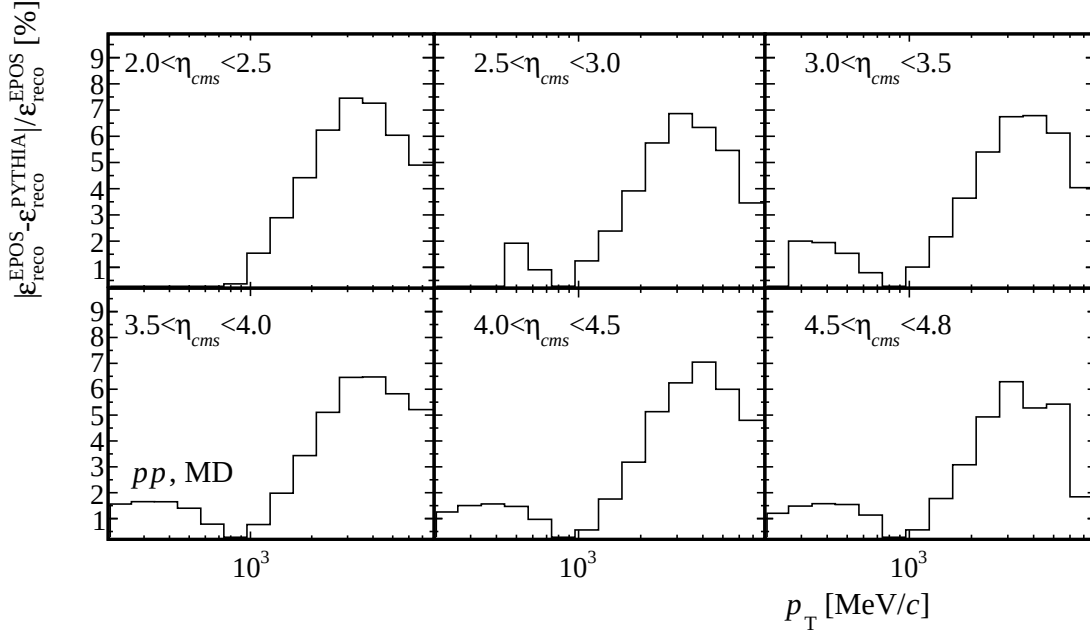
Figure 6.10: Relative difference between \epsilon_{\text{reco}} computed with PYTHIA and EPOS particle fractions ( f_p ).
