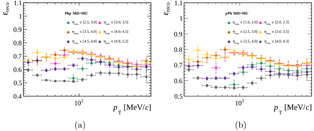
Figure 6.4: Reconstruction efficiency for the Pbp (left) and p Pb (right) configurations for the different (\eta, p_T) bins, computed with Eq. 6.6. Datasets with MD and MU are combined. Error bars include statistical and systematic uncertainty.
