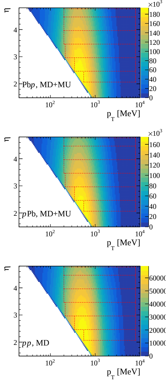
Figure 6.1: Fiducial acceptance of the LHCb spectrometer. In red: pseudorapidity bins and p_T range for the different beam configurations. Figures are prepared with simulation including all prompt charged particles with p > 2 \text{ GeV}/c .
