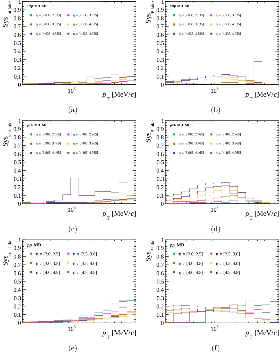
Figure B.23: Relative uncertainty on R_{fake} from sample size (left) and from fake track purity (right) for Pbp, pPb and pp samples.
