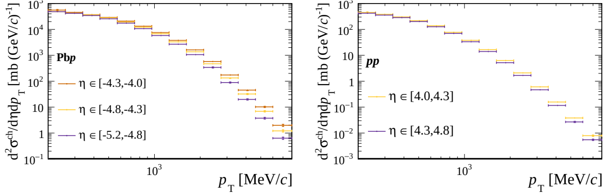
Figure 8.2: Charged particle production cross-section in Pbp (left) and pp (right) collisions at \sqrt{s_{NN}} = 5.02 TeV with the alternative binning as discussed in Sec. 6.1. Error bars account for statistical, systematic and luminosity uncertainties added in quadrature.
