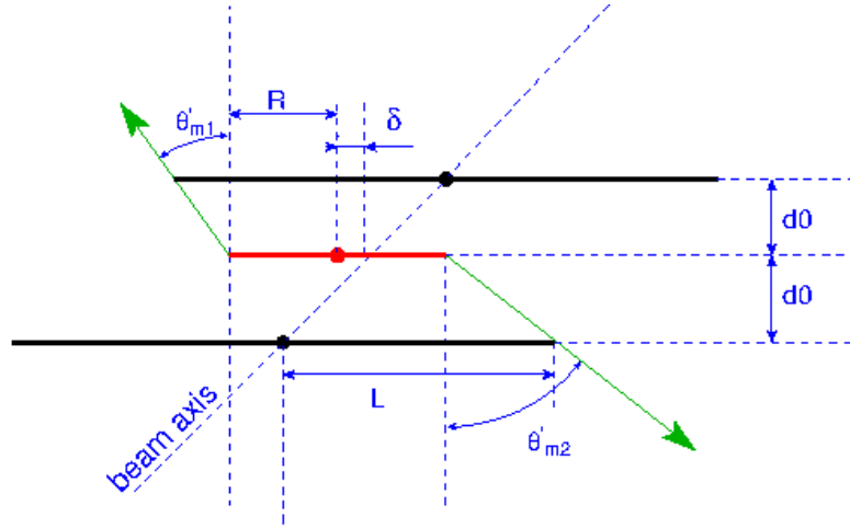
FIGURE 5.12: Top view of 2 detectors and target showing that at small \cos \theta' trajectories emitted from the edge of the target may fall outside the active area. \delta is the horizontal shift of the target, R its radius, L the half length of the active area and d_0 the separation distance.
