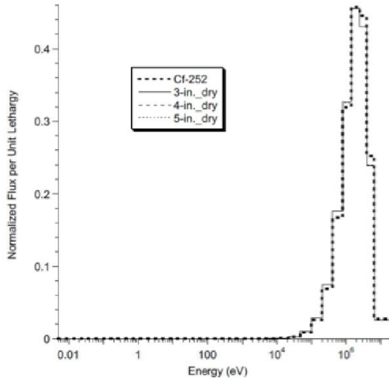
FIGURE 7.15: Difference between original ^{252}\text{Cf} neutron spectrum and spectrum at the sample due to the slight moderation [9].
