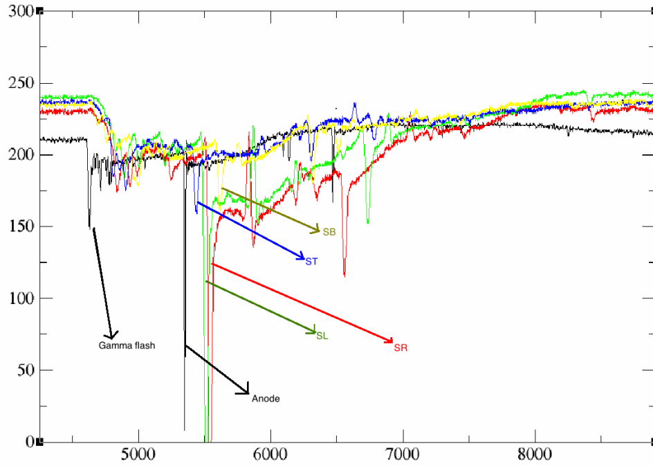
FIGURE 4.16: Signals from the 5 channels of a detector, anode (black), left SL (green), right SR (red), top ST (blue), bottom SB (yellow). The strong peak around 5400 ns in the anode signal is fission a fragment and the corresponding delay line peaks follow around 5500 ns. The time on the horizontal axis starts with the triggering of the DAQ.
