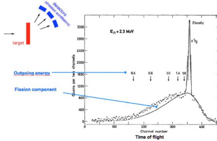
FIGURE 7.11: Knitter experiment: measurement of the outgoing neutrons and subtraction of the fission contribution to get the scattering component.[7]
