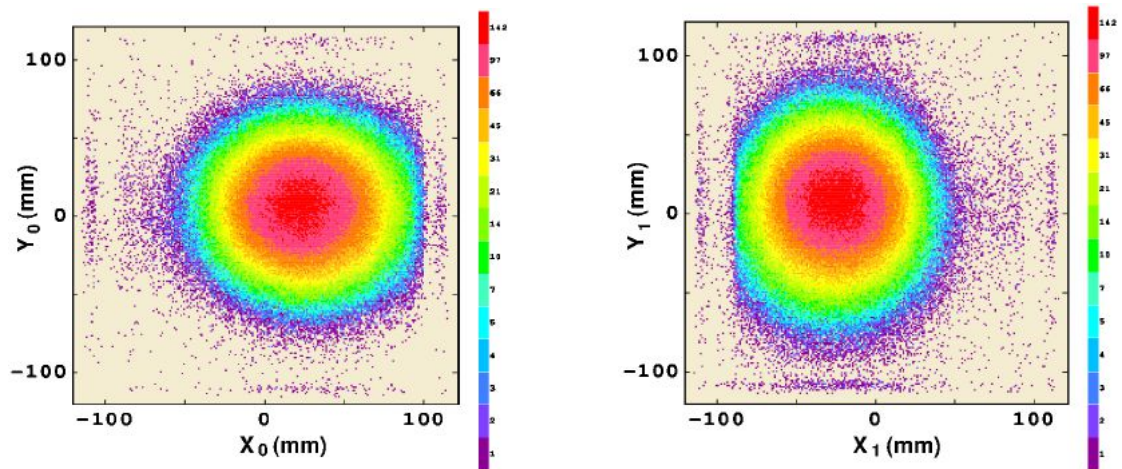
FIGURE 4.25: Distribution of hitting points on the detectors surrounding the ^{235}\text{U} target, the upstream detector is on the left side and the downstream one on the right side. The X axis is horizontal and oriented to the left hand side when travelling along the beam.
