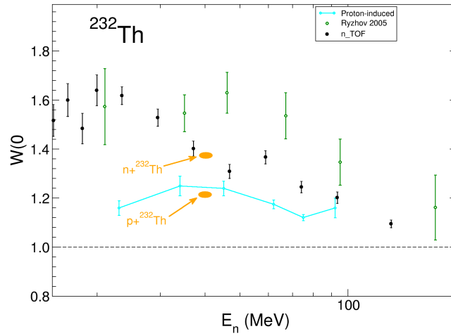
FIGURE 6.7: ^{232}\text{Th} anisotropy with Ryzhov data, n\_TOF data and proton-induced data.
