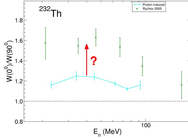
FIGURE 6.5: Comparison between neutron-induced anisotropy from [5] and proton-induced anisotropy collected by [1].
