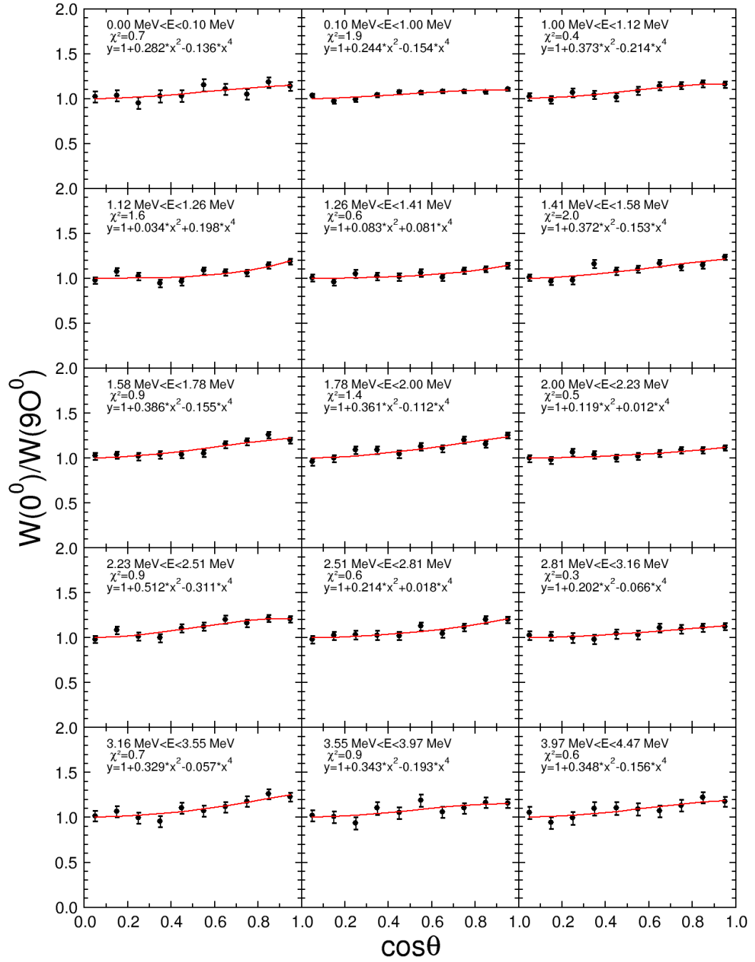
FIGURE C.12: ^{237}\text{Np} angular distributions for E_n < 5.00 MeV
