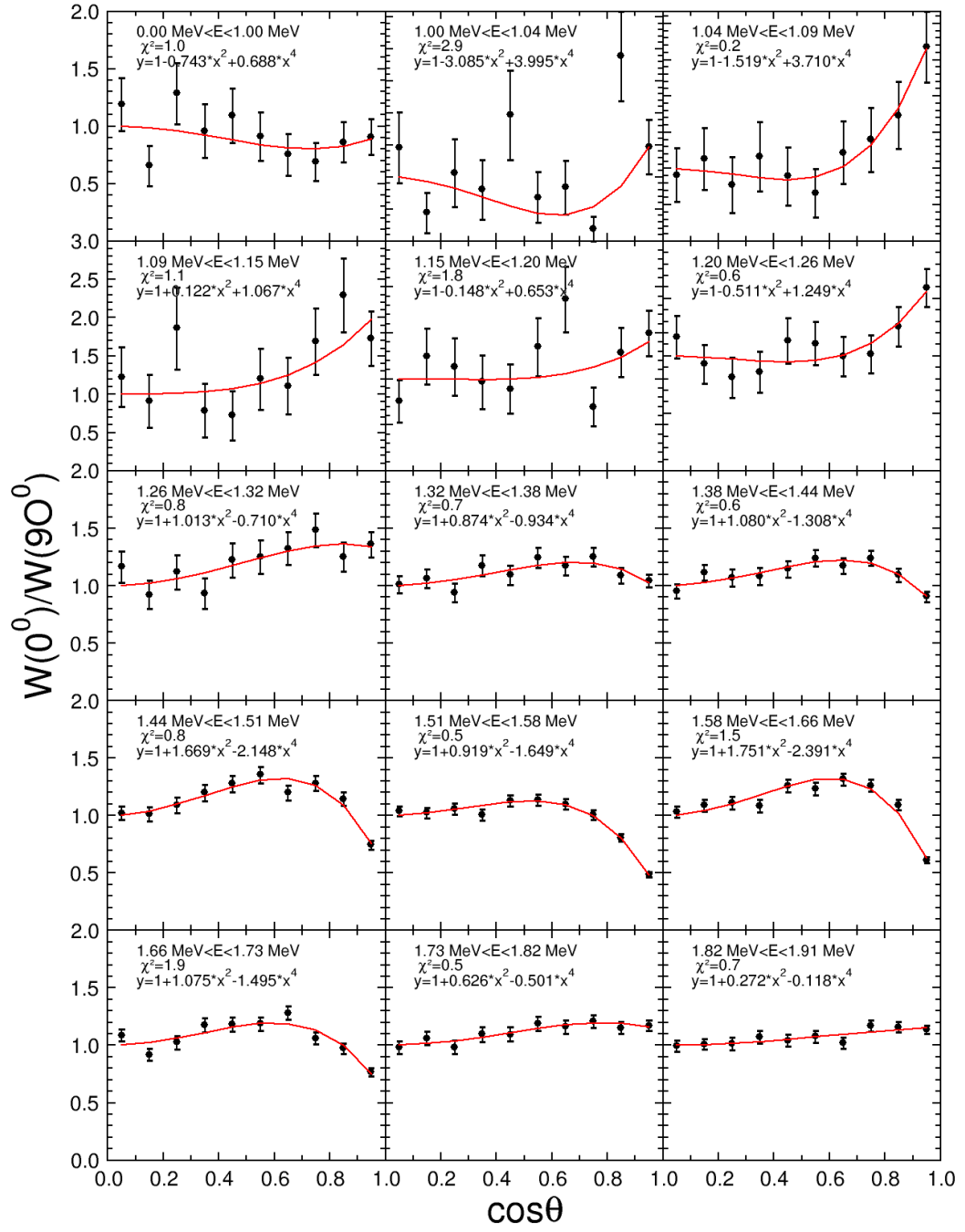
FIGURE C.1: ^{232}\text{Th} angular distributions for E_n < 1.91 MeV
