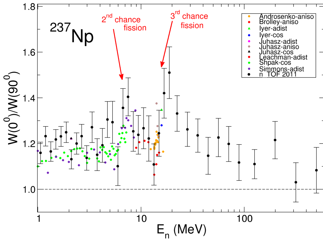
FIGURE 6.11: ^{237}\text{Np} anisotropy compared to the existing data
