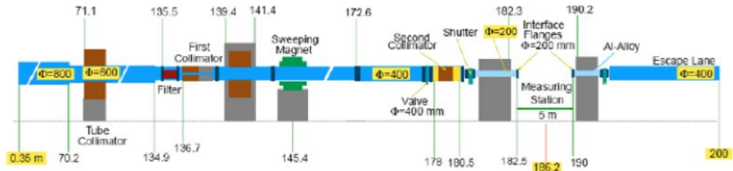
FIGURE 3.2: The 200 m neutron line
