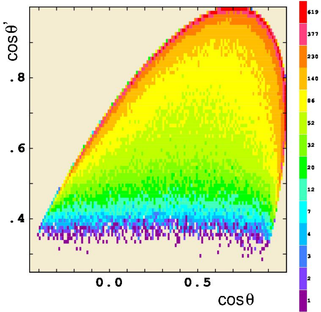
FIGURE 5.8: Distribution of counts in the (\cos \theta, \cos \theta') plane for the ^{235}\text{U} target and E_n < 100 keV.
