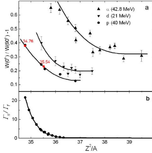
FIGURE 6.6: The dependence of anisotropy coefficient for fission induced by p , d and \alpha -particles with different targets. The curves are fits of the experimental data, from Eismont et al. [6].
