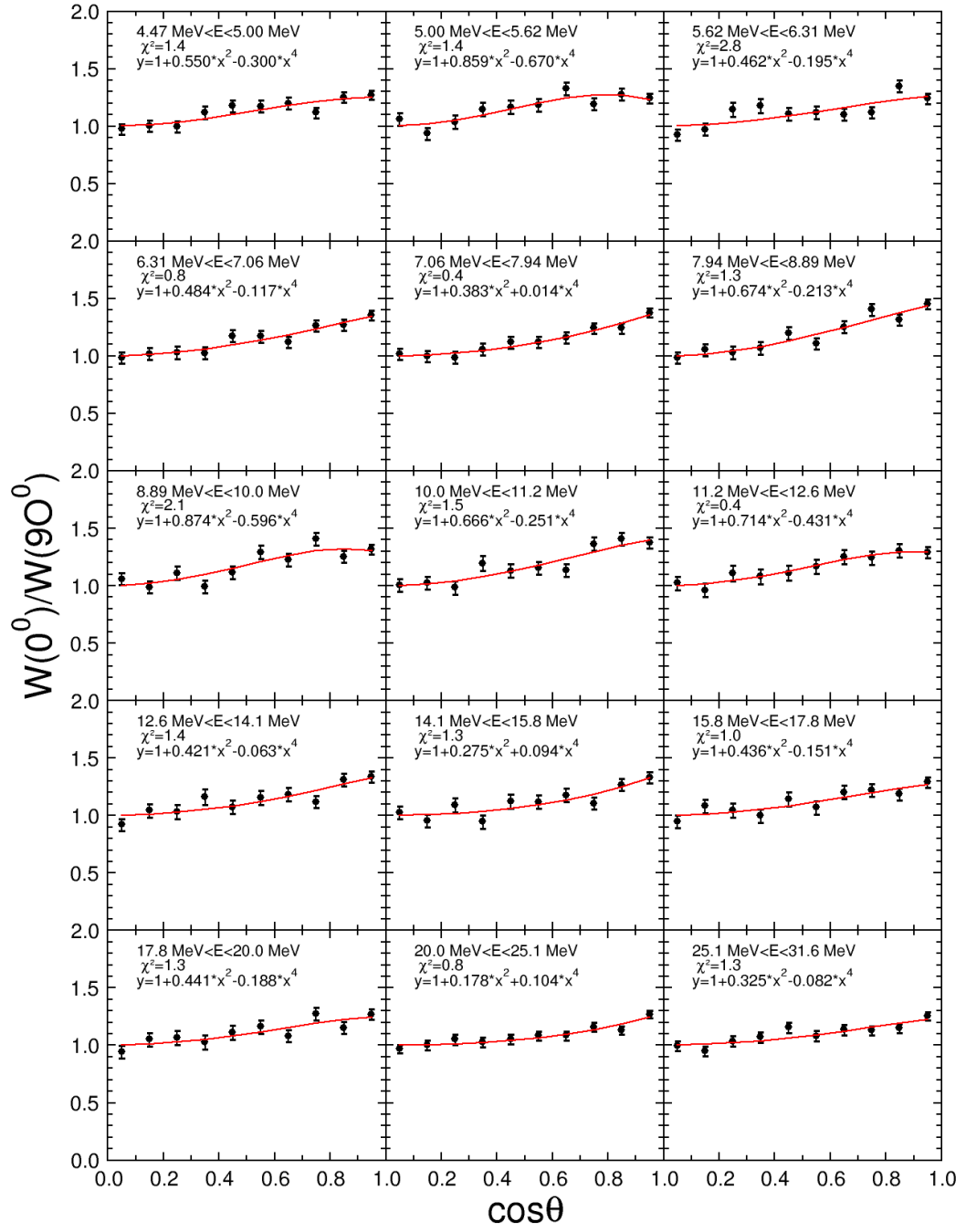
FIGURE C.7: ^{235}\text{U} angular distributions for 4.47 < E_n < 31.6 MeV
