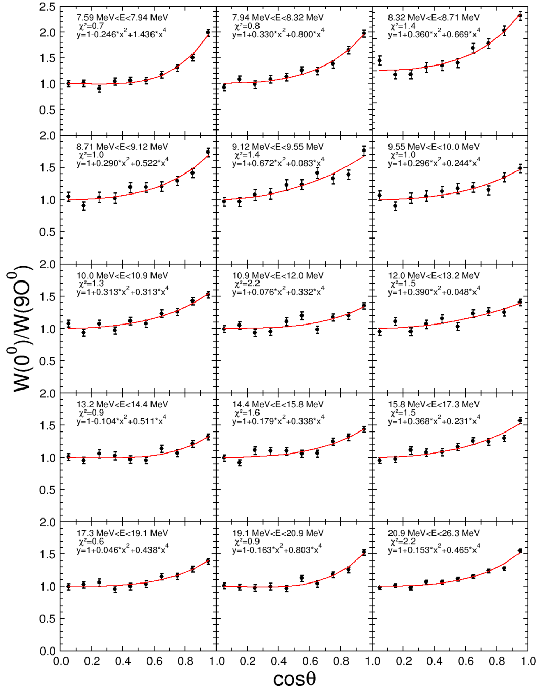
FIGURE C.4: ^{232}\text{Th} angular distributions for 7.59 < E_n < 26.3 MeV
