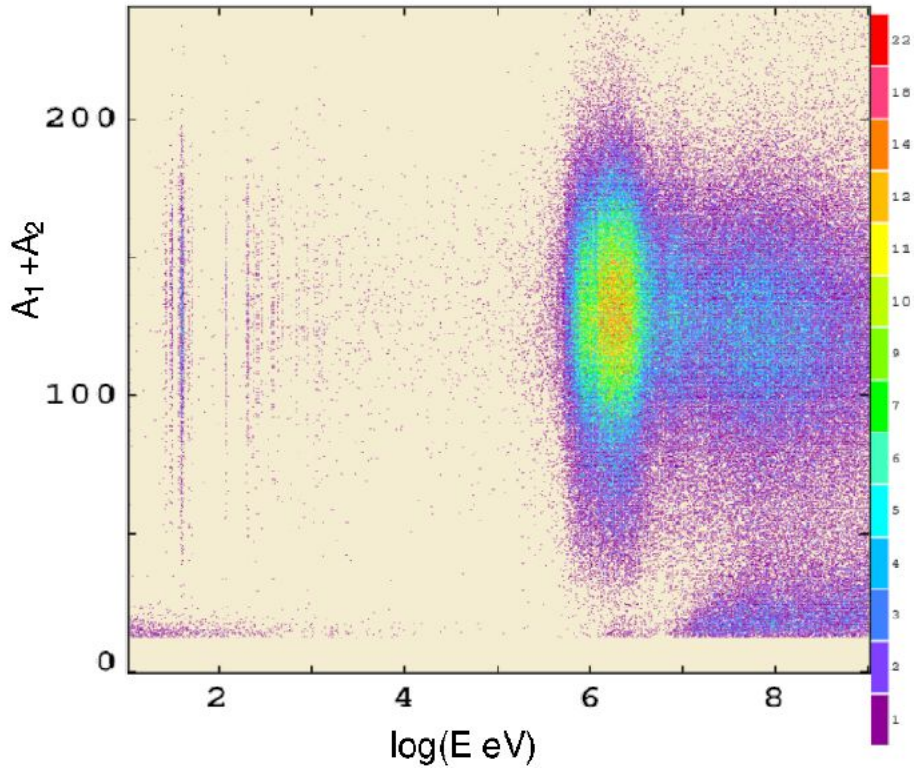
FIGURE 4.13: Distribution of the sum of anode amplitudes in detectors around the ^{237}\text{Np} target, as a function of the neutron energy.
