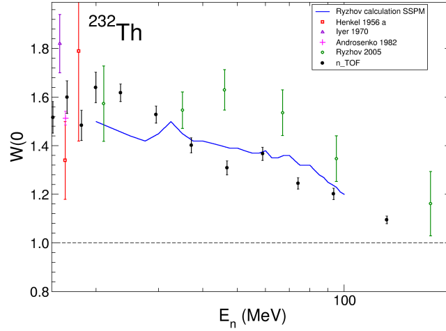
FIGURE 6.4: Comparison between n_TOF data, Ryzhov data and Ryzhov SSPSM calculation (without reduction of K_0^2 ).
