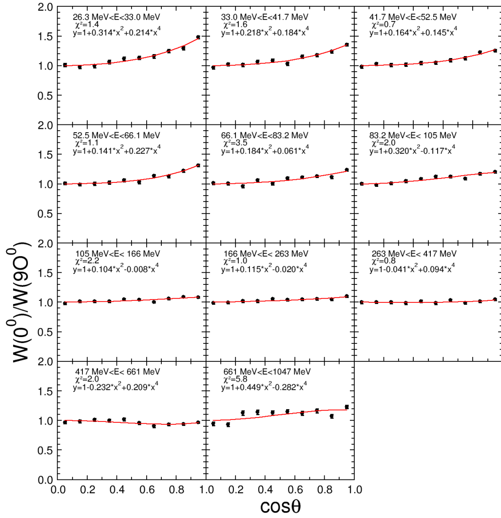
FIGURE C.5: ^{232}\text{Th} angular distributions for 26.3 < E_n < 1047 MeV
