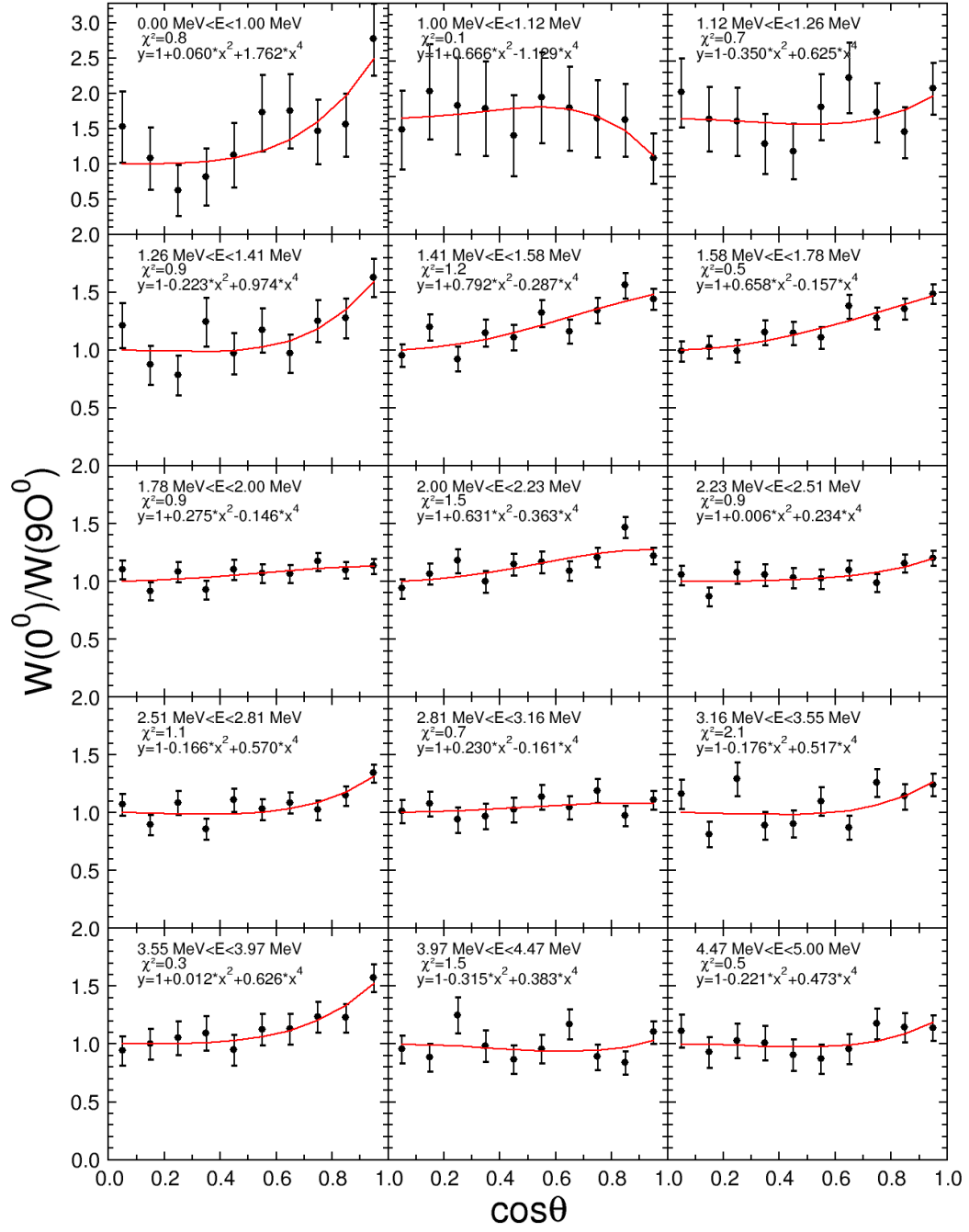
FIGURE C.9: ^{238}\text{U} angular distributions for E_n < 5.00 MeV
