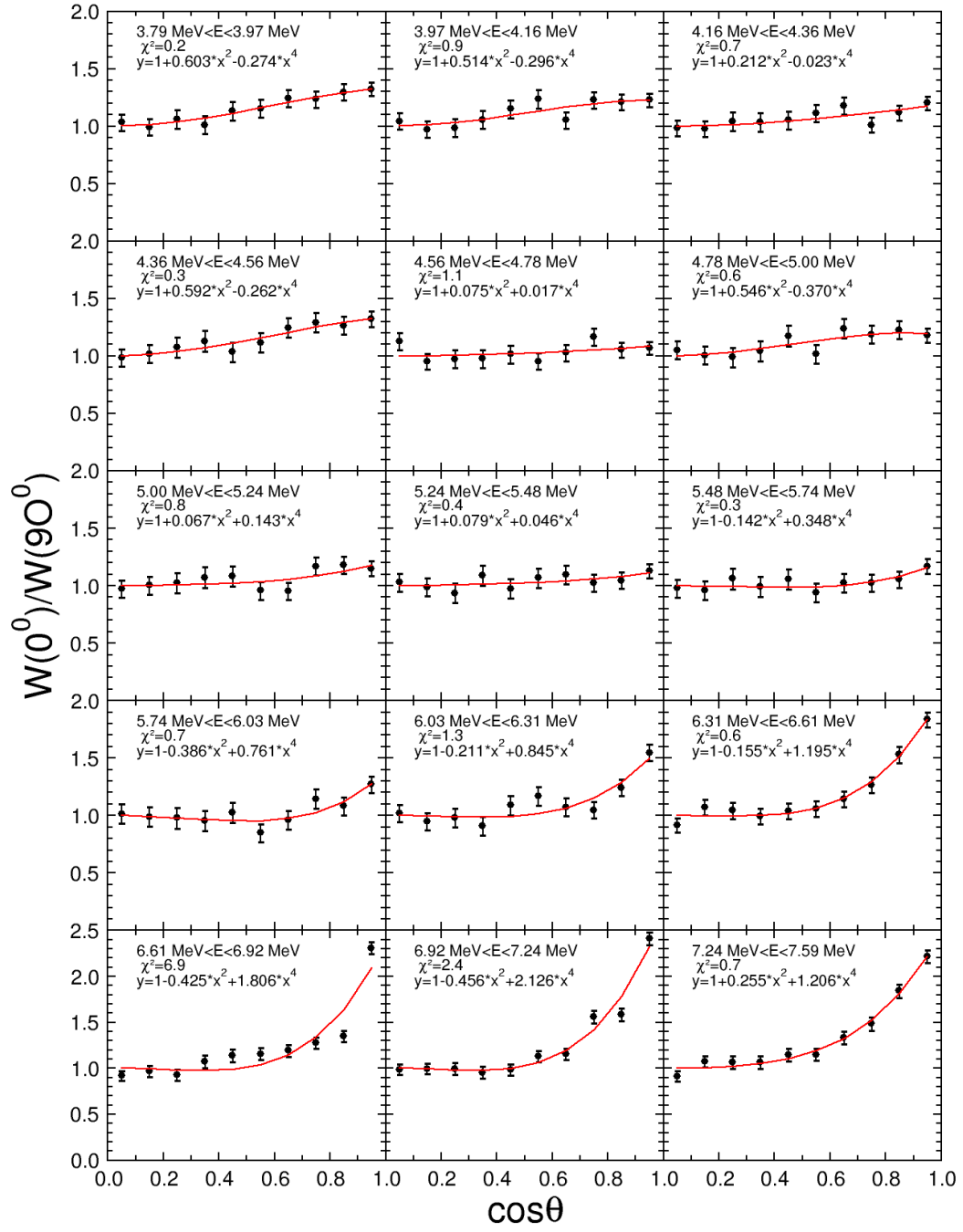
FIGURE C.3: ^{232}\text{Th} angular distributions for 3.79 < E_n < 7.59 MeV
