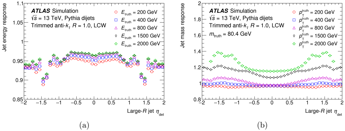
Figure 5.21: Large- R jet calibration. (a) Energy response in bins of E^{\text{true}} and \eta for the absolute energy scale correction. (b) Mass response in bins of p_T^{\text{true}} and \eta for jets with truth mass around m_W \approx 80 GeV. Figures sourced from [82].
