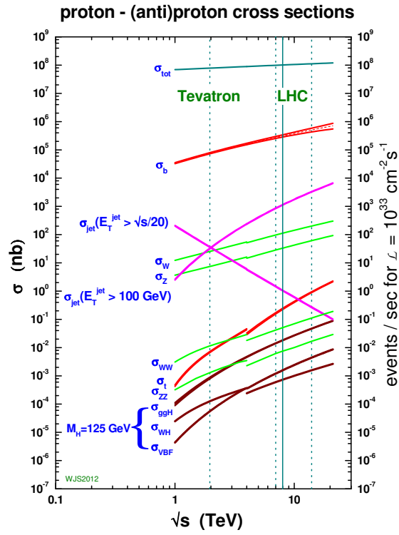
Figure 4.4: Cross sections for pp interactions as a function of \sqrt{s} center-of-mass energy. Figure sourced from [220].
