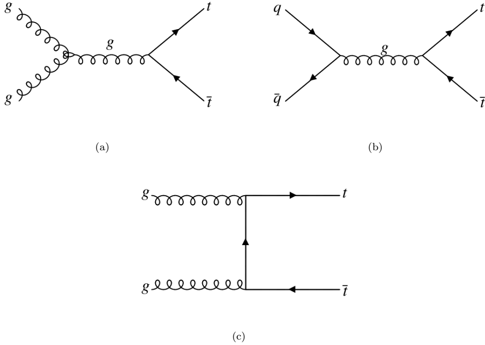
FIGURE 11.8: Tree level Feynman diagrams of t\bar{t} production at the LHC.
