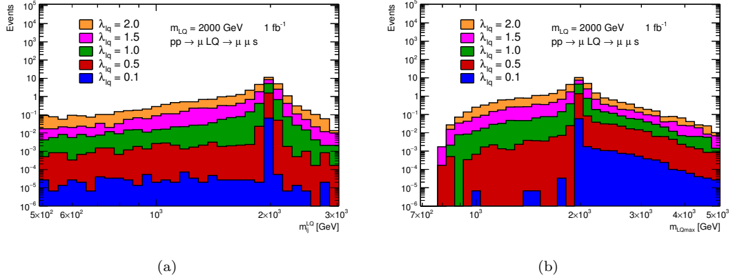
FIGURE 11.5: Predicted 2 TeV LQ signal shape of the process pp \rightarrow \mu LQ \rightarrow \mu \mu s against m_{lj}^{LQ} (a) and the quantity m_{LQmax} (b) on a logarithmic scale for varying \lambda_{lq} coupling values. Signal hypotheses are scaled to an integrated luminosity of 1 \text{ fb}^{-1} .
