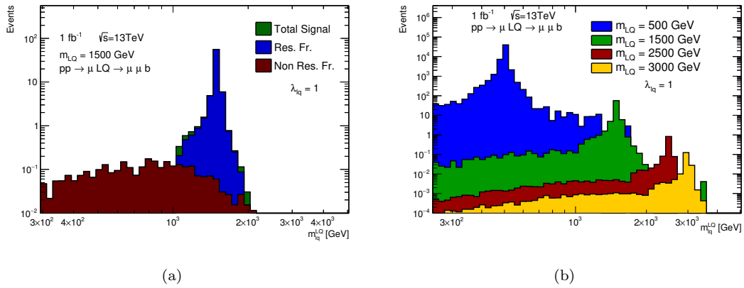
FIGURE 11.4: Predicted LQ signal shape of the process pp \rightarrow \mu LQ \rightarrow \mu \mu b against the invariant mass of the LQ decay products m_{lj}^{LQ} . (a) shows a signal distribution with m_{LQ} = 1500 \text{ GeV} decomposed into resonant and non-resonant fractions and (b) multiple distributions for varying LQ masses m_{LQ} in the range of 500 GeV and 3 TeV under the assumption of \lambda_{lq} = 1 .
