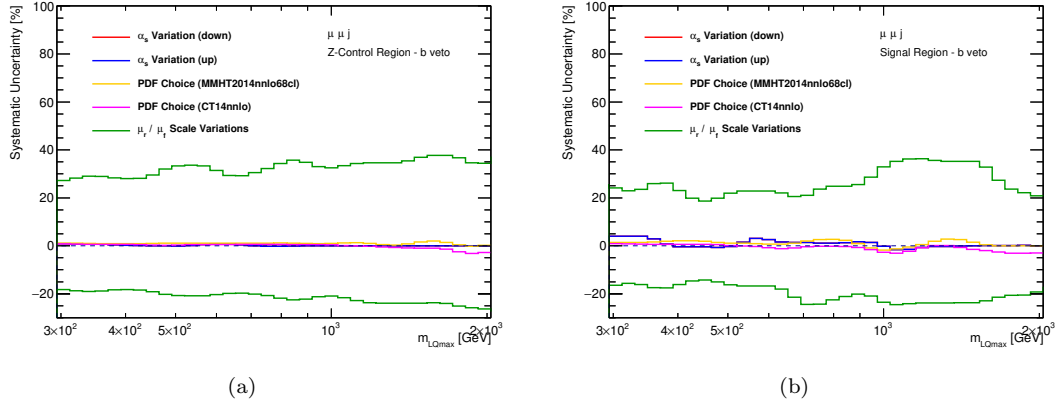
FIGURE 11.22: Theoretical uncertainties on the Z/\gamma^* + \text{jets} background with respect to the contribution itself. Variations are determined on the m_{LQ\text{max}} spectrum in the muon channel b -veto Z/\gamma^* control region (a) and b -veto signal region (b).
