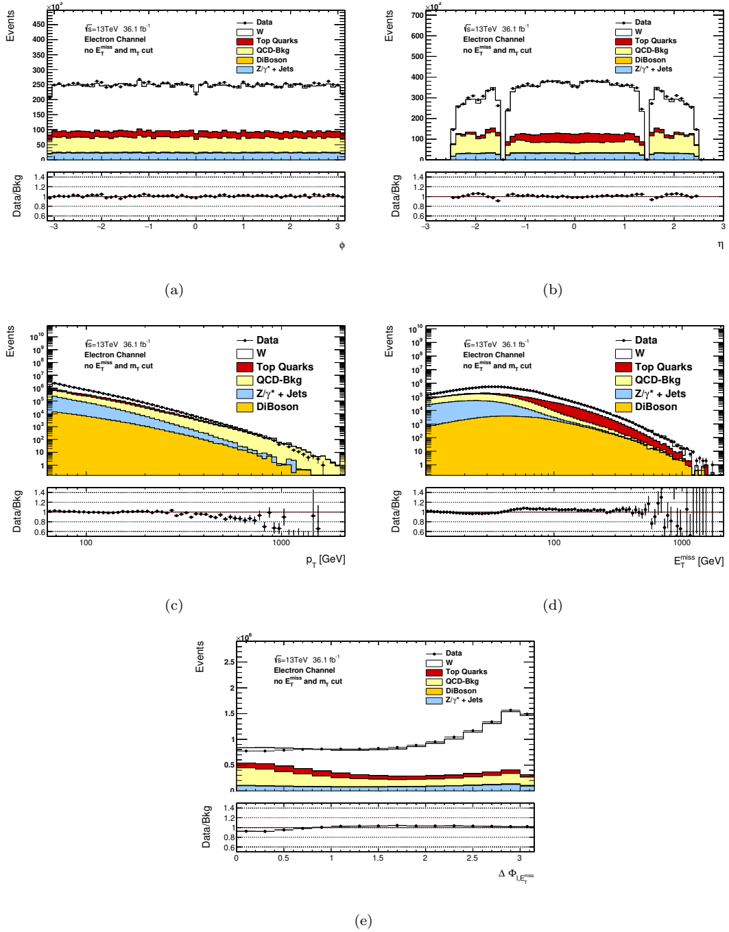
FIGURE 7.23: Lepton candidates' \phi , \eta , p_T and E_T^{\text{miss}} as well as the \Delta \Phi_{l, E_T^{\text{miss}}} - between the lepton and E_T^{\text{miss}} - distributions obtained in the electron channel are shown, while not applying the E_T^{\text{miss}} and m_T cut defined in the signal selection. In each upper panel the measured data as well as the background estimation are shown. Each background contribution is drawn separately but stacked. The lower panel illustrates the agreement by showing the ratio between data and background estimate.
