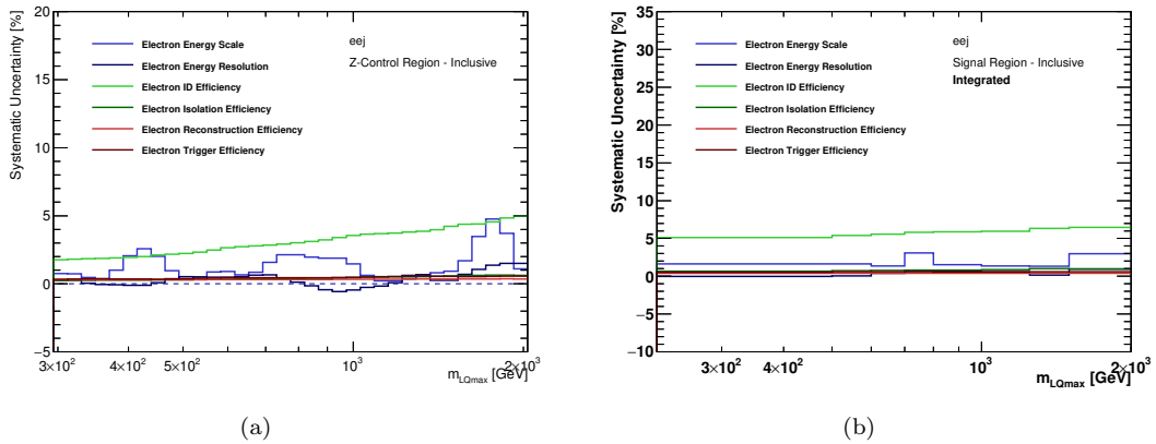
FIGURE 11.20: Uncertainties related to electron reconstruction. Variations in (a) are determined on the m_{LQ_{\max}} spectrum in the electron channel combined Z/\gamma^* control region. In (b) the variation in the tail integral of the combined electron channel signal region is probed. The value in each bin is calculated by considering the tail integrals starting from the lower interval margin.
