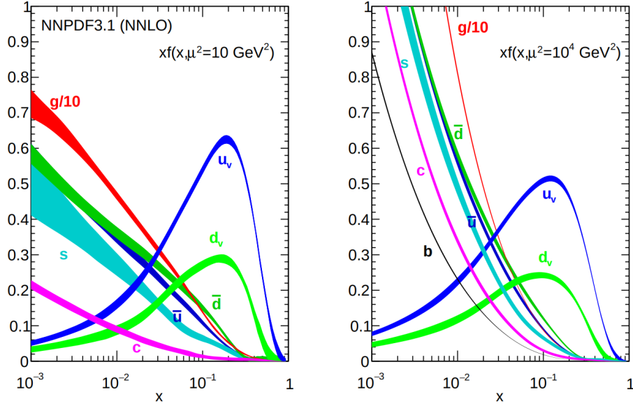
FIGURE 2.3: NNPDF3.1 parton density distributions at a scale of Q^2 = 10 \text{ GeV}^2 and Q^2 = 10^4 \text{ GeV}^2 . Different colors indicate the distributions of different particle types with the width of the line indicating the one \sigma uncertainties. The gluon contribution is scaled by 1/10 for better visibility. [42]
