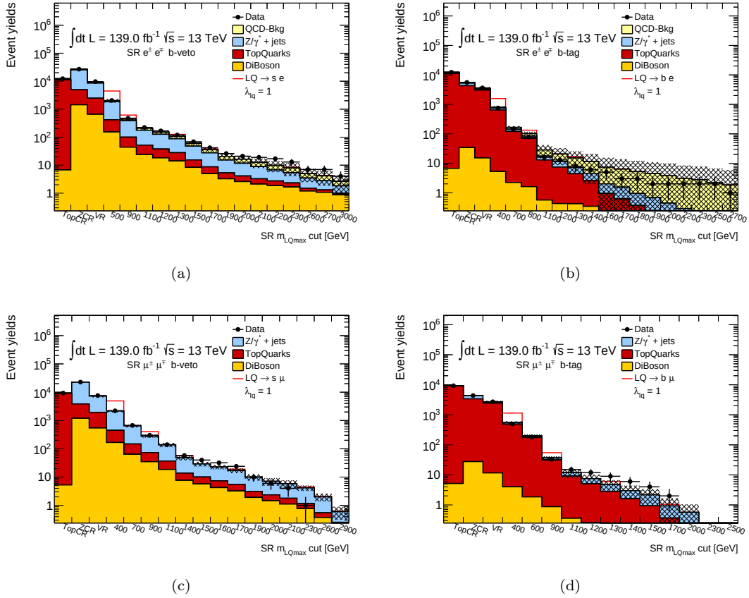
FIGURE 12.2: Data event yields and background expectation in every region per channel. Background expectations are drawn stacked. The shaded area illustrates the background uncertainty. Control regions (TopCR, ZCR) are displayed in the first two bins. The third bin shows the the validation region (VR), which is followed by the signal regions in each channel. These are defined by the m_{LQ\max} cut applied. Signal hypotheses for m_{LQ} = n \cdot 500 GeV with n \in 1, 2, 3, 4, 5, 6, 7 and \lambda_{lq} = 1 are shown as well in the relevant signal regions.
