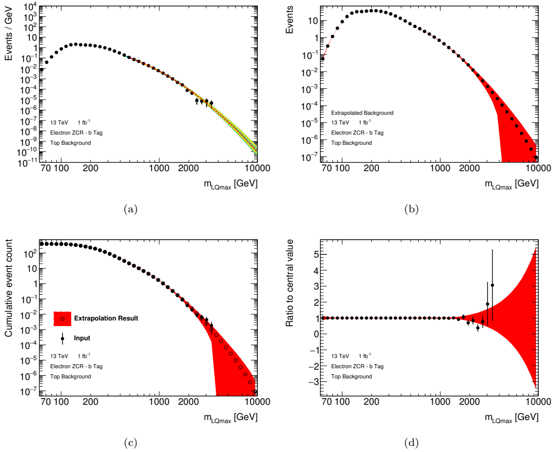
FIGURE 11.19: Diagrams illustrating the fit based procedure to extrapolate the electron channel m_{LQ\max} spectrum in the b -tag Z/\gamma^* control region. (a) shows the ensemble of all fits used to estimate the extrapolation uncertainty and nominal value, which is drawn as a red dashed line. (b) displays the final estimate of this background with its uncertainty indicated as red area. (c) shows the integral over the tail in each mass bin starting from the respective bin with its uncertainty in comparison to the simulated input MC. (d) depicts the ratio of the extrapolation result to the input distribution.
