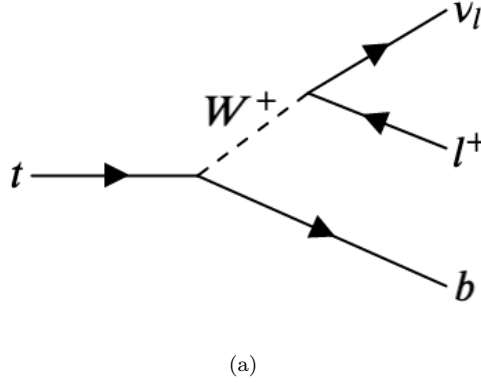
FIGURE 11.9: LO Feynman diagram of the top quark decay with a charged anti-lepton in the final state.
