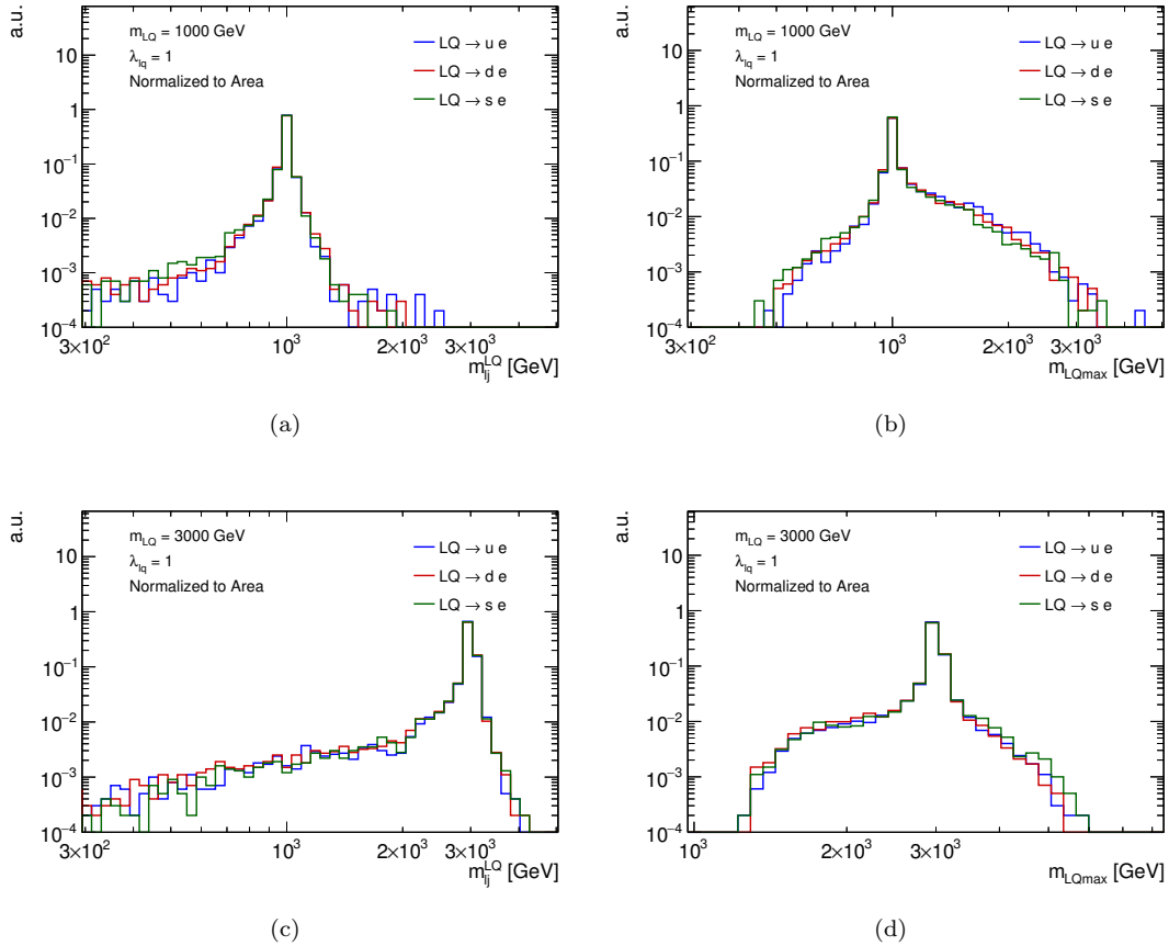
FIGURE B.3: Generator level m_{l_j}^{LQ} and m_{LQmax} distributions for signal processes including different quark types. Each spectrum is normalized to its area. In the top row the signal process pp \rightarrow lLQ \rightarrow ll s with a LQ mass hypothesis of 1 TeV and in the bottom row for 3 TeV were generated. The LQ-lepton-quark coupling is assumed to be \lambda_{lq} = 1 .
