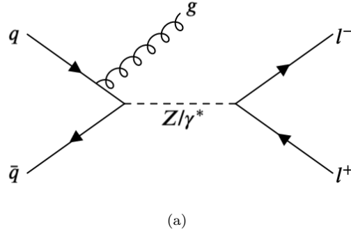
FIGURE 11.7: Tree level (LO) Feynman diagram of the Z/\gamma^* + \text{jets} process. The jet is produced by initial state radiation.
