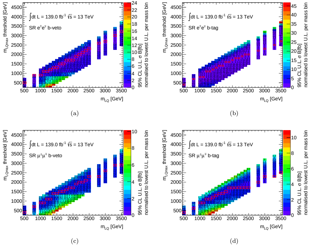
FIGURE 12.1: Threshold scan used to optimize the m_{LQmax} cut applied in each channels signal regions for each mass hypothesis. The x -axis shows the LQ mass of the signal, the y -axis the applied m_{LQmax} threshold and the z -axis the ratio of the 95% CL expected cross-section limit to the best limit obtained for a given mass hypothesis. Red boxes indicate the threshold which gives the best limit and is taken for further analysis.
