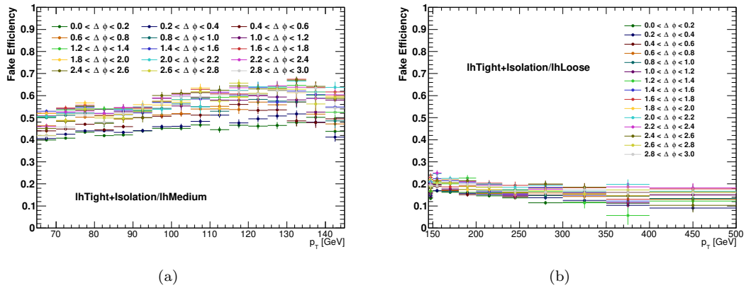
FIGURE 7.17: Electron candidate fake efficiencies against p_T in different \Delta\Phi_{l,E_T^{miss}} intervals. (a) displays the efficiency for candidates with p_T \in [65 \text{ GeV}, 145 \text{ GeV}] while (b) shows the efficiency for candidates with p_T > 145 \text{ GeV} .
