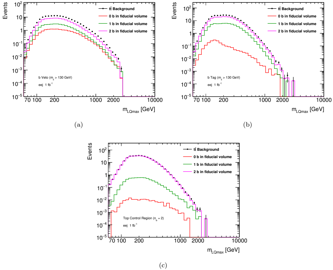
FIGURE B.1: t\bar{t} background m_{LQ\max} distributions in the b -veto (a) and b -tag (b) combined region ( m_t > 130 GeV) as well as the Top control region (c). The total background is illustrated by the black data points. Different contributions classified by the number of b quarks in the fiducial region are given by the purple, green and red line.
