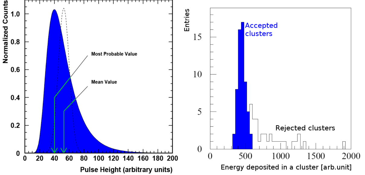
Figure 2.8: Left: Landau shape describing charge distribution in primary ionization clusters (marked with shaded blue area). Gaussian peak of comparable width is shown with dashed line for reference. Right: Sample distribution of measured cluster energy deposits, showing principle of truncation procedure. Small deposit clusters (blue area) are accepted for energy-loss measurement. Figures from Ref. [74].
