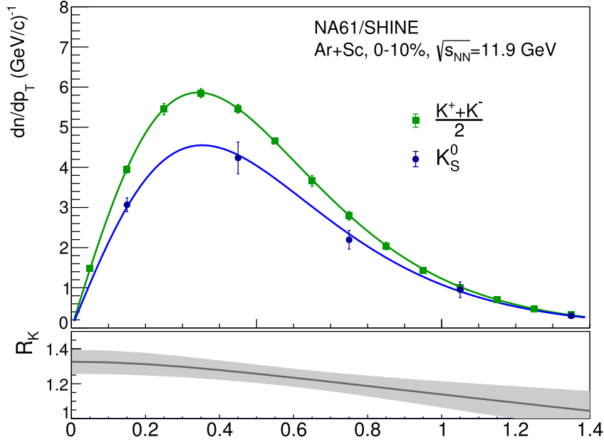
Figure 6.15: Top: Comparison of transverse momentum spectrum of K_S^0 (this analysis) and average spectrum of charged kaons [98] in Ar+Sc collisions at 75 A GeV/c. Total uncertainties are plotted, calculated as square root of sum of squared statistical and systematic uncertainties ( \sqrt{\text{stat}^2 + \text{sys}^2} ). For charged kaons total uncertainties were calculated separately for positively charged and negatively charged kaons and then propagated. Bottom: Transverse momentum dependence of R_K ratio calculated from Eq. (6.4) for fitted functions.
