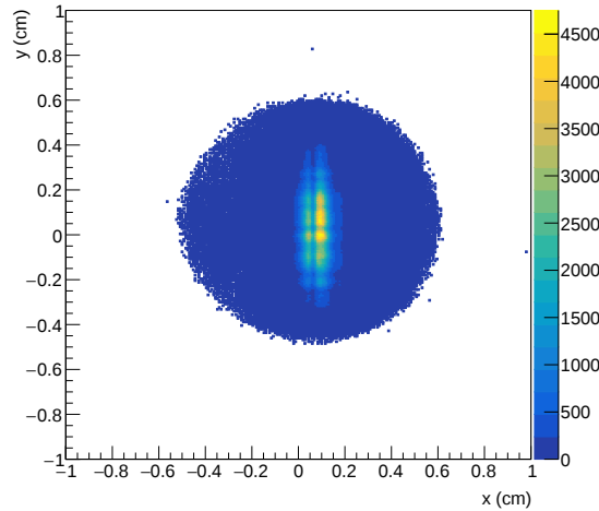
Figure 4.2: Beam profile at target z position in collected Ar+Sc collisions at 75A \text{ GeV}/c .
