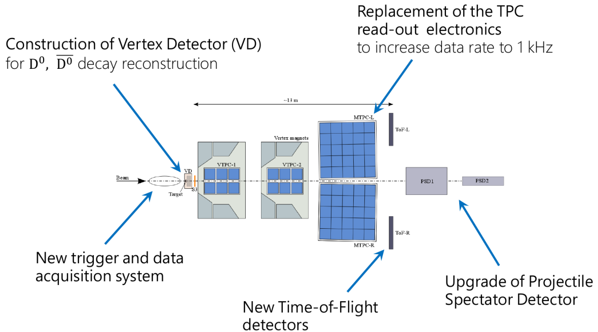
Figure 7.3: Schematic picture of most important upgrades in NA61/SHINE experiment. Figure from Ref. [110].
