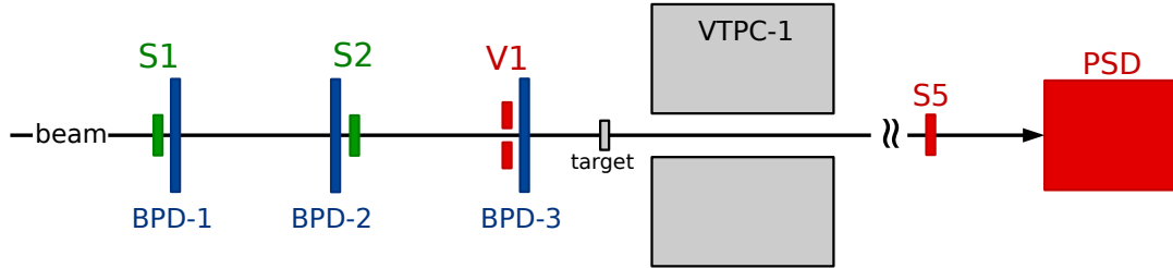
Figure 4.1: Layout of sub-detectors included in trigger during Ar+Sc data-taking campaign.
