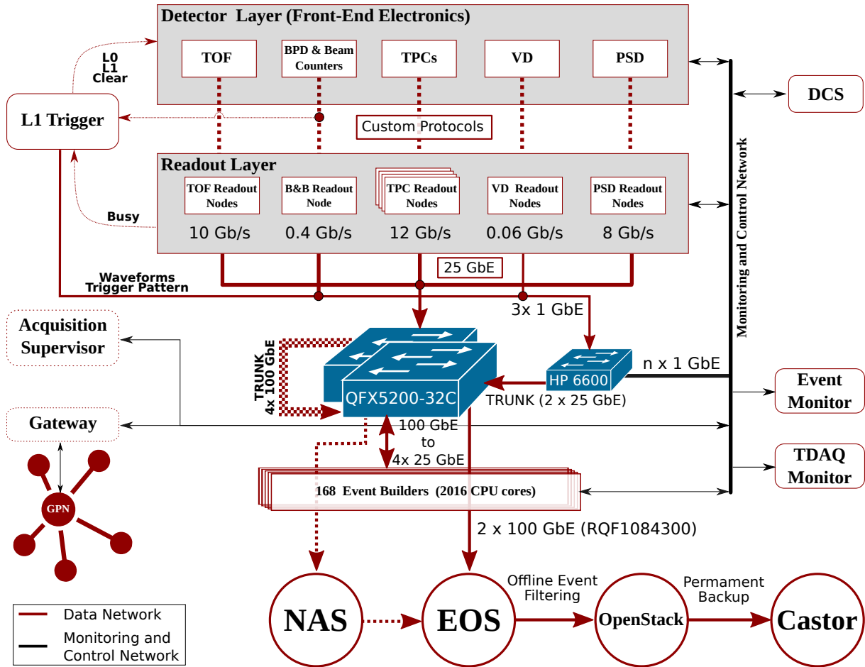
Figure 7.4: Schematic layout of new DAQ system of NA61/SHINE experiment. Figure from Ref. [71].
