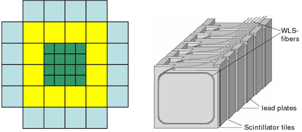
Figure 2.11: Left: Schematic transverse layout of PSD modules. Right: Schematic view of single PSD module. Figures from Ref. [60].
