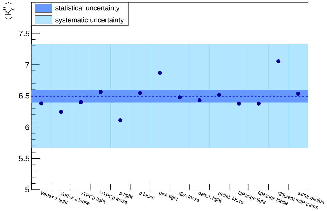
Figure 5.14: Contributions of different biasing selection criteria to final systematic uncertainty of mean multiplicity of K_S^0 mesons produced in Ar+Sc collisions at 75A GeV/c. Dashed line denotes \langle K_S^0 \rangle = 6.49 (see Sec. 6.4).
