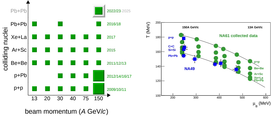
Figure 2.1: Left: Summary of data collected within system size – beam momentum scan performed by NA61/SHINE. Pb+Pb data at 150A GeV/c were partially collected. Right: Coverage of phase diagram of strongly interacting matter by NA61/SHINE data. Figures from Ref. [71].
