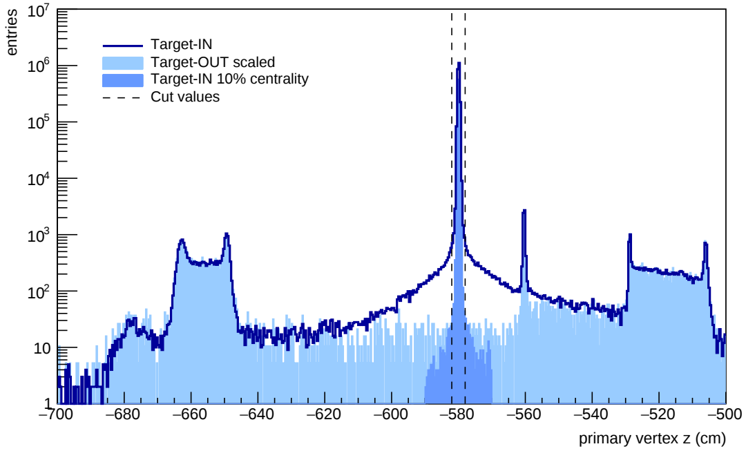
Figure 5.1: Distribution of z position of primary vertex for Ar+Sc collisions at 75A GeV/c. Solid line represents Target-IN data; light blue histogram represents scaled Target-OUT data. Dashed lines correspond to range of values accepted for analysis. Cut selection was based on Target-IN data for 10% most central collisions presented as shaded area on darker blue. Distributions are plotted after beam off-time cut and beam quality cut.
