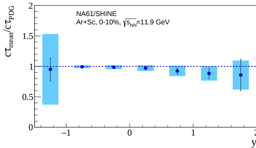
Figure 6.4: Mean lifetime with statistical (vertical bars) and systematic (shaded boxes) uncertainties of K_S^0 mesons compared with PDG value as function of rapidity for Ar+Sc collisions at 75A GeV/ c .
