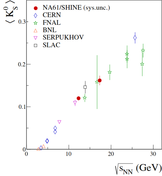
Figure 1.10: Mean multiplicity of K_S^0 mesons produced in p+p collisions as function of energy. Figure from Ref. [59].
