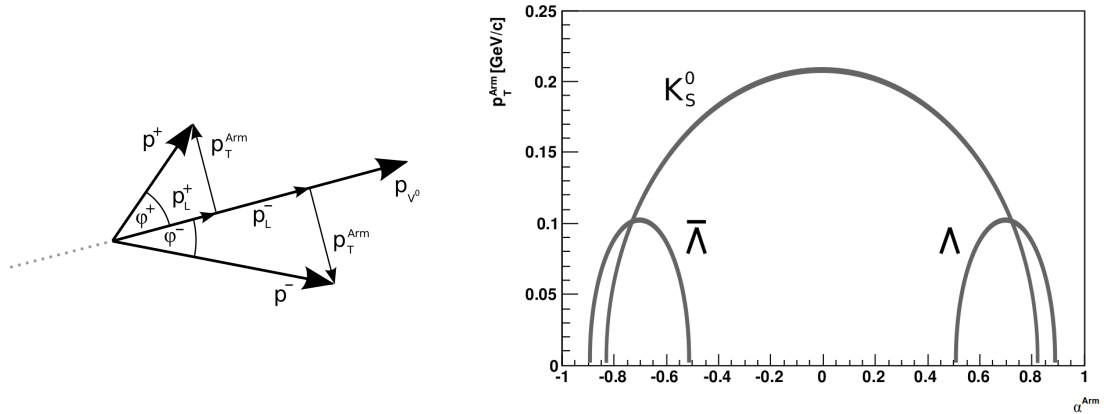
Figure 1.6: Left: Definition of variables used to calculate p_T^{Arm} and \alpha^{Arm} . Right: Theoretically allowed p_T^{Arm} and \alpha^{Arm} values for strange neutral particles. Figures from Ref. [29].
