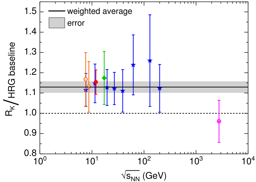
Figure 6.18: Experimental data for charged to neutral kaon ratio divided by HRG baseline as function of collision energy. HRG baseline ( Q/B \neq \text{const.} ) is shown by black dots in Fig. 6.17. Figure from Ref. [106] with later changes.
