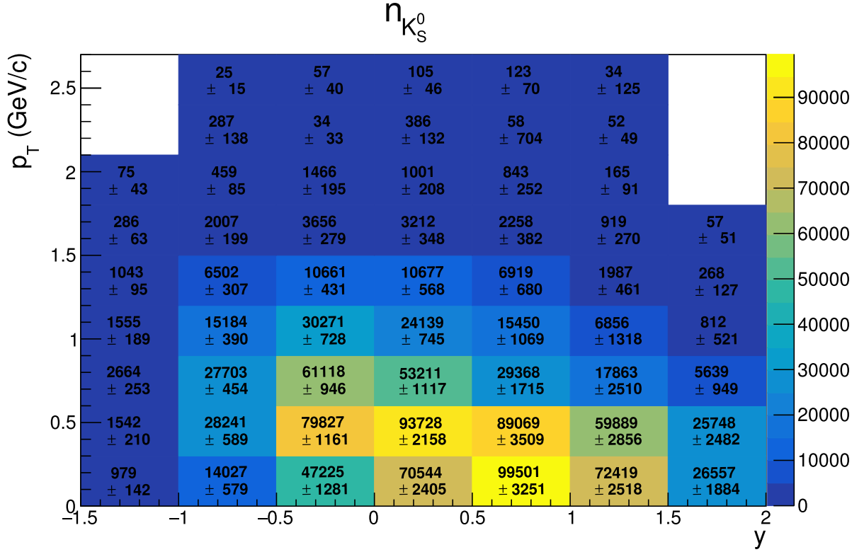
Figure 5.10: Raw (uncorrected) y - p_T yields of K_S^0 mesons in Ar+Sc collisions at 75A GeV/c with statistical uncertainties (see Sec. 5.7.1).
