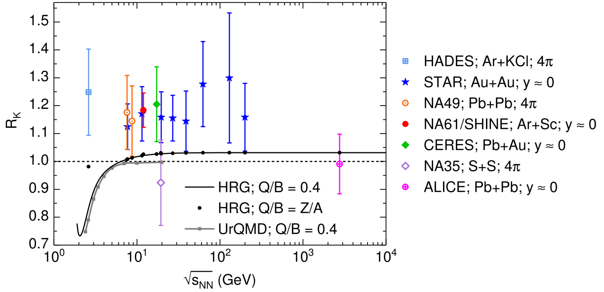
Figure 6.17: Charged to neutral kaon ratio as function of collision energy. Experimental data are shown by symbols with total uncertainties. HRG baseline for electric-to-baryon charge Q/B = 0.4 is shown by black line. HRG baseline for Q/B values specified accordingly to given types of colliding nuclei is represented by black dots. UrQMD model results are shown by gray squares. Figure from Ref. [106] with later changes.
