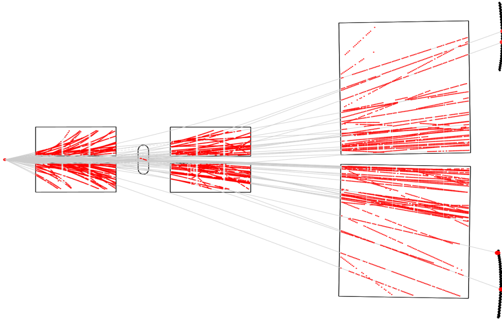
Figure 3.1: Example of reconstructed ^{40}\text{Ar}+^{45}\text{Sc} collision at 75A \text{ GeV}/c . TPC clusters are marked as red points and reconstructed tracks are marked as gray lines.
