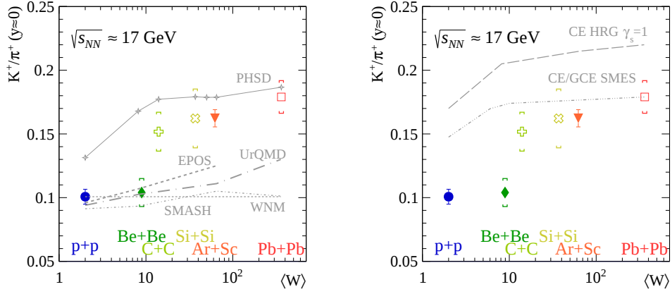
Figure 1.8: System size (mean number of wounded nucleons) dependence of K^+/\pi^+ ratio at mid-rapidity obtained at beam momenta of 150(8)A GeV/c compared with dynamical ( Left ) and statistical ( Right ) models. Figures from Ref. [35, 36].
