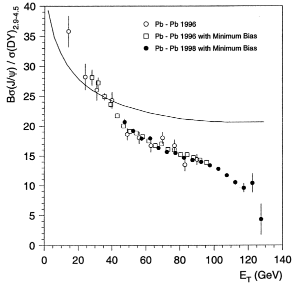
Figure 7.2: Branching ratio (B) multiplied \sigma_{J/\psi} (cross-section – measure of production/reaction probability) and divided by \sigma_{DY} (cross-section for well-known Drell-Yan process – lepton pair production in electromagnetic interaction of hadrons) as function of transverse energy (measure of collision centrality – most central events have highest values of E_T ) in Pb+Pb collisions at 158A GeV/c measured by NA50. Curve represents J/ \psi suppression due to ordinary (“cold”) nuclear matter absorption. Figure from Ref. [117].
