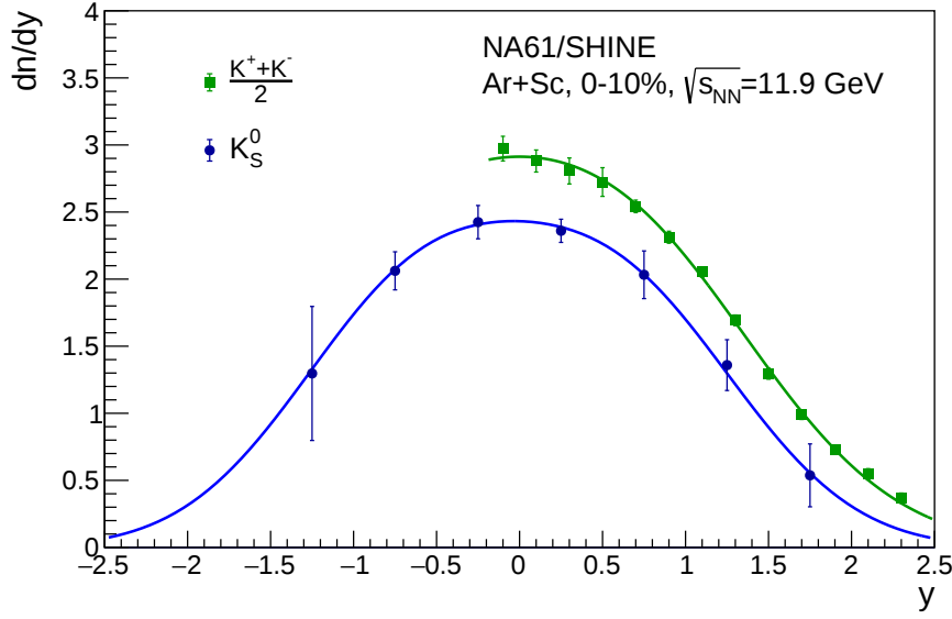
Figure 6.14: Comparison of rapidity spectrum of K_S^0 (this analysis) and average spectrum of charged kaons [98] in Ar+Sc collisions at 75A GeV/c. Total uncertainties are plotted, calculated as square root of sum of squared statistical and systematic uncertainties ( \sqrt{\text{stat}^2 + \text{sys}^2} ). For charged kaons total uncertainties were calculated separately for positively charged and negatively charged kaons, and then propagated.
