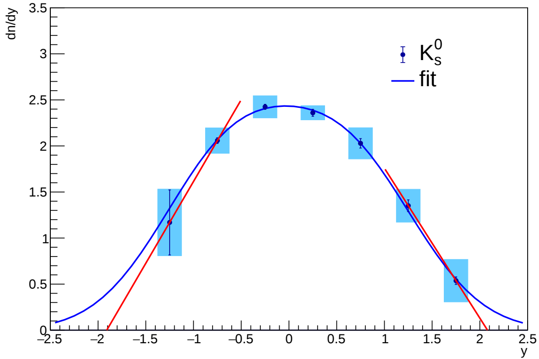
Figure 5.13: Rapidity spectrum of K_S^0 in 10% most central Ar+Sc collisions at 75A GeV/c (see Sec. 6.4). Red lines fitted to most external points of distribution were used to estimate contribution to systematic uncertainty coming from extrapolation of measured rapidity distribution to full phase space.
