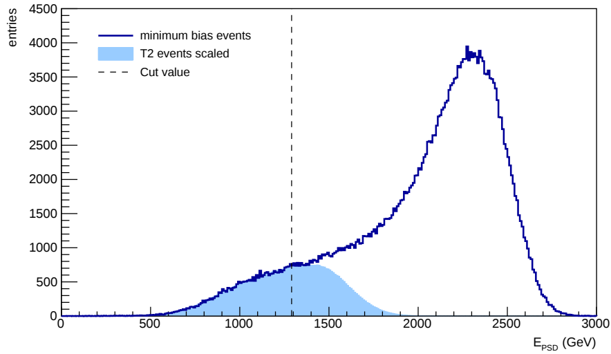
Figure 5.3: Measured distribution of PSD energy deposit for minimum bias events (blue line) and scaled T2 events (shaded blue area) without any event selection for Ar+Sc collisions at 75A GeV/c. Dashed line corresponds to threshold for 10% most central collisions.
