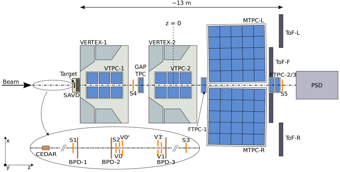
Figure 2.2: Schematic picture of NA61/SHINE detector. S3 detector is placed after target. Figure from Ref. [71].
