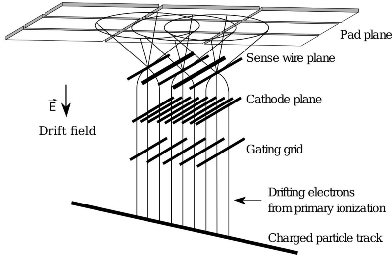
Figure 2.7: Schematic picture of TPC read-out. Figure from Ref. [61].
