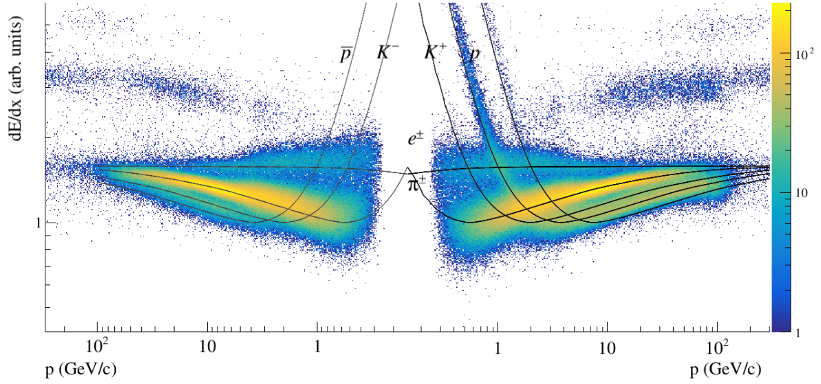
Figure 2.9: Distribution of energy loss versus momentum measured by NA61/SHINE TPCs in Ar+Sc collisions at 75 A GeV/c. Solid lines show nominal Bethe-Bloch functions (Eq. (2.1)) for different particle species. Clouds visible for p > 10 GeV/c above main part of distribution correspond to heavier fragments produced in Ar+Sc interactions. Right part of plot shows positively charged particles while left part negatively charged ones.
