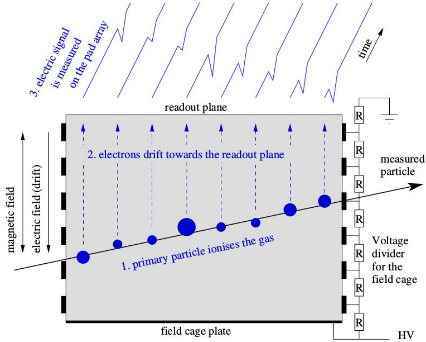
Figure 2.6: Schematic picture presenting principle of operation of Time Projection Chamber. Figure from Ref. [74].
