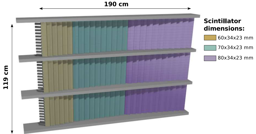
Figure 2.10: Schematic layout of scintillators in ToF-R detector. ToF-L detector layout is mirror reflection of ToF-R with respect to beamline. Figure from Ref. [60].
