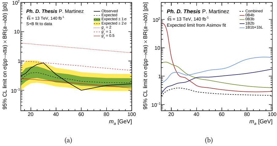
Figure 12.21: (a) Expected and observed 95% CL upper limits of \sigma(t\bar{t}a) \times \text{BR}(a \rightarrow b\bar{b}) as a function of m_a . The red lines correspond to different values of the coupling to the top quark. (b) Expected 95% CL upper limits of \sigma(t\bar{t}a) \times \text{BR}(a \rightarrow b\bar{b}) as a function of m_a for each SR. The dashed line corresponds to the combined expected limit from (a). All limits are calculated for the available signal mass points and smoothed using ROOT for easier visualisation.
