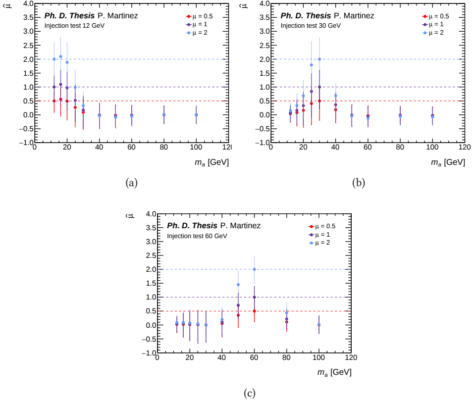
Figure C.38: Fitted signal strength with respect to the a -boson mass from the (a) m_a = 12 GeV, (b) m_a = 30 GeV and (c) m_a = 60 GeV injection tests. The different colours correspond to \mu = 0.5 (red), \mu = 1 (purple) and \mu = 2 (blue).
