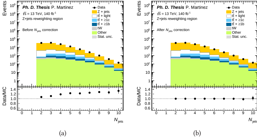
Figure 9.15: Data versus MC comparison of the N_{\text{jets}} distribution (a) before and (b) after applying the N_{\text{jets}} correction to the Z+jets background. Systematic uncertainties are not included.
