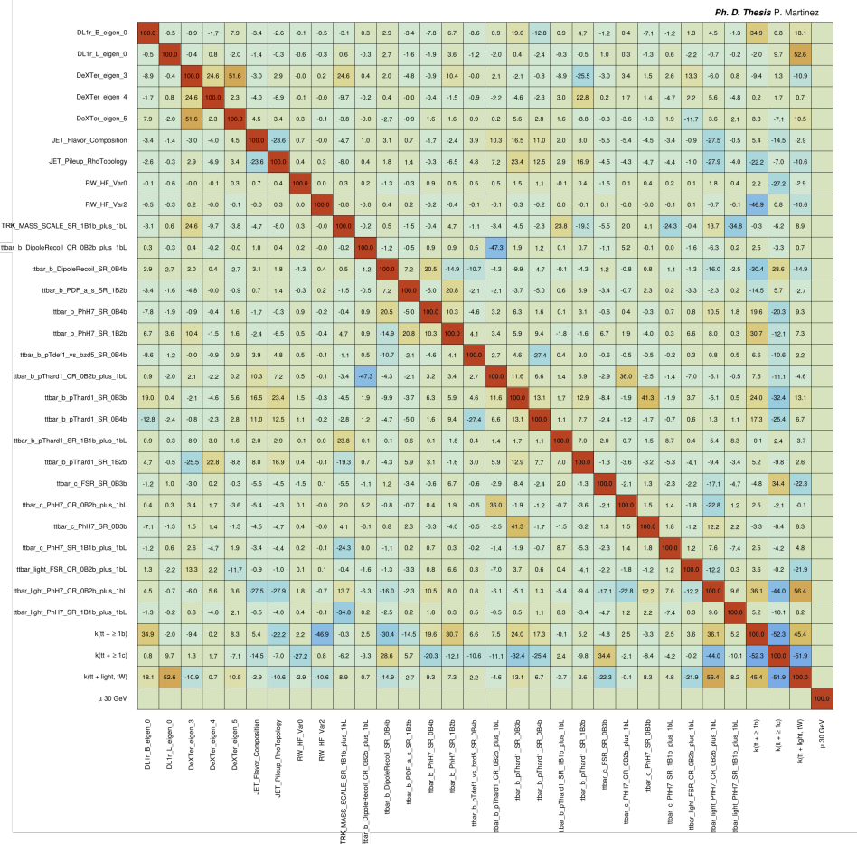
Figure B.34: Correlation matrix for the relevant NPs in the blinded fit to data with m_a = 30 GeV.
