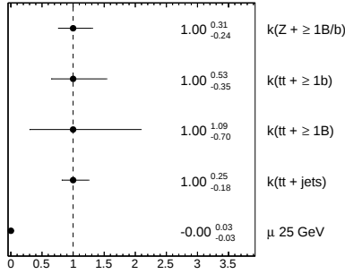
Figure 10.2: Normalisation factors for the Z +jets and t\bar{t} +jets samples in fit to the Asimov dataset with m_a = 25 GeV.
