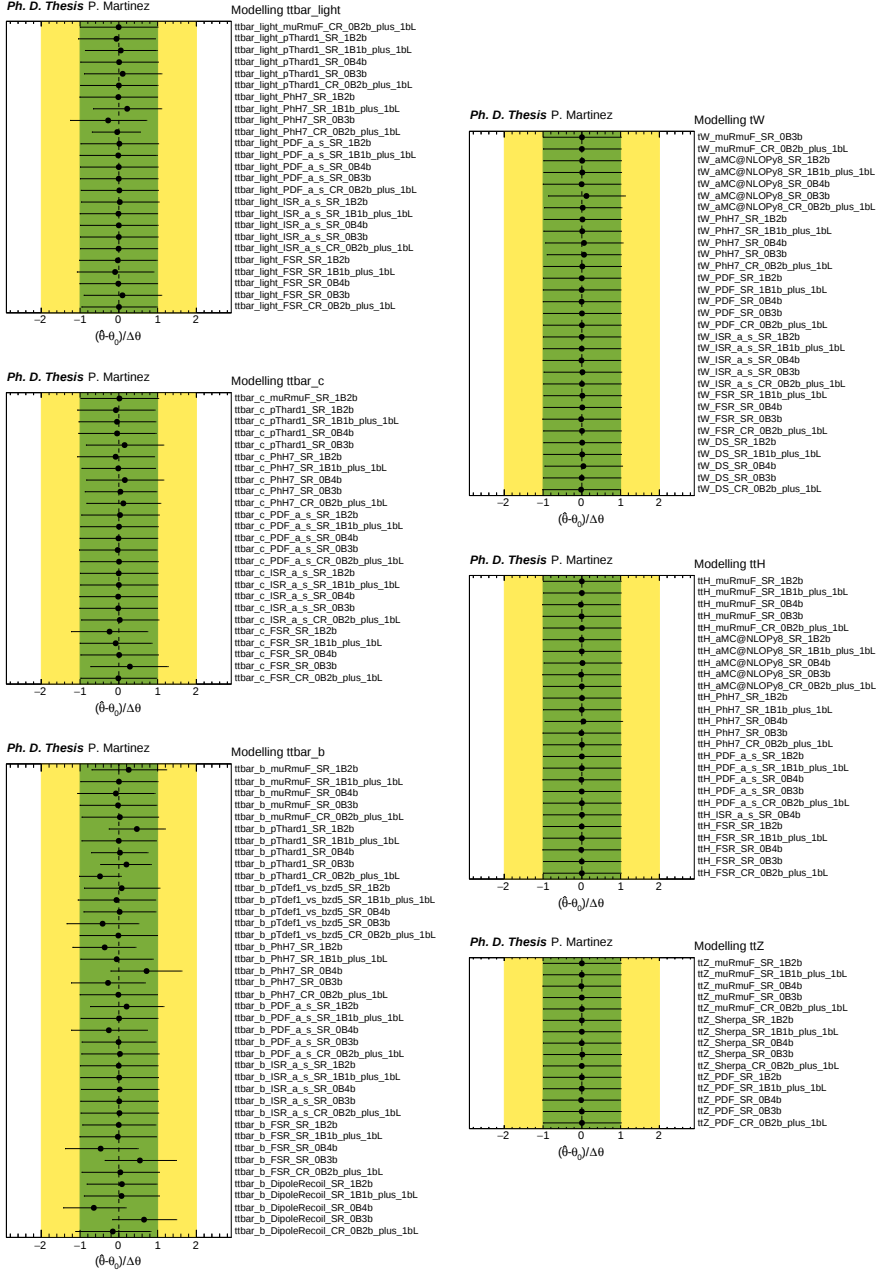
Figure B.36: Fitted nuisance parameters from the blinded fit to data with m_a = 30 GeV (II).
