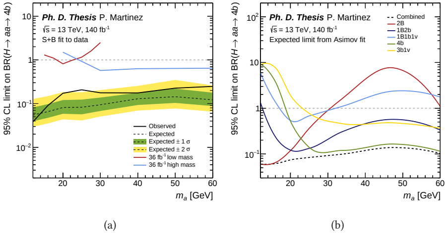
Figure 10.14: (a) Expected and observed 95% CL upper limits of \text{BR}(H \rightarrow aa \rightarrow 4b) as a function of m_a . The red and blue lines correspond to the two previous analyses using 36 \text{ fb}^{-1} of proton-proton collisions at \sqrt{s} = 13 \text{ TeV} . (b) Expected 95% CL upper limits of \text{BR}(H \rightarrow aa \rightarrow 4b) as a function of m_a for each SR. The dashed line corresponds to the combined expected limit from (a). All limits are calculated for the available signal mass points and smoothed using ROOT for easier visualisation.
