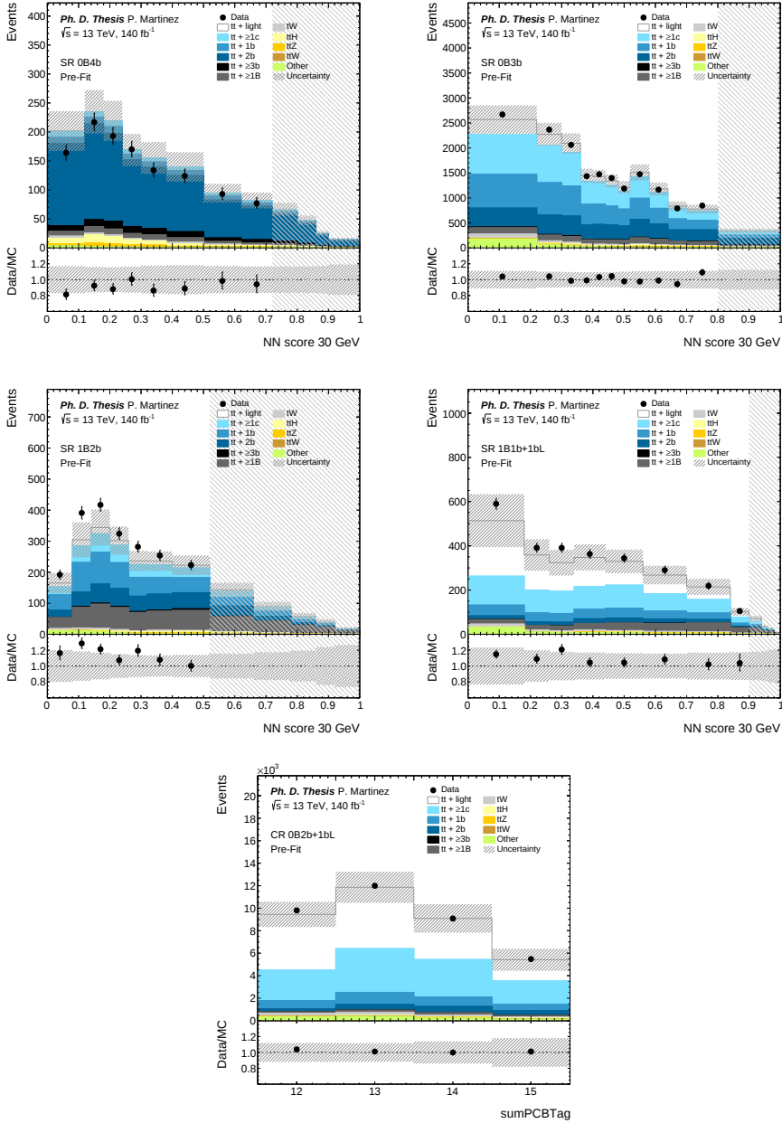
Figure B.31: Pre-fit plots from the blinded fit to data with m_a = 30 GeV.
