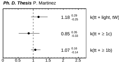
Figure B.33: Normalisation factors for the t\bar{t} +jets samples in the blinded fit to data with m_a = 30 GeV.
