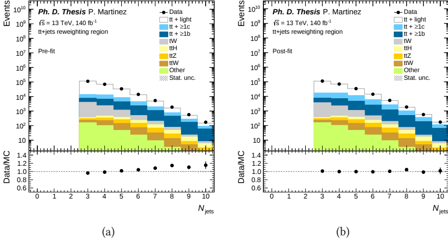
Figure 11.7: Data versus MC comparison of the N_{\text{jets}} distribution (a) before and (b) after applying the tt +jets normalisation correction. Systematic uncertainties are not included.
