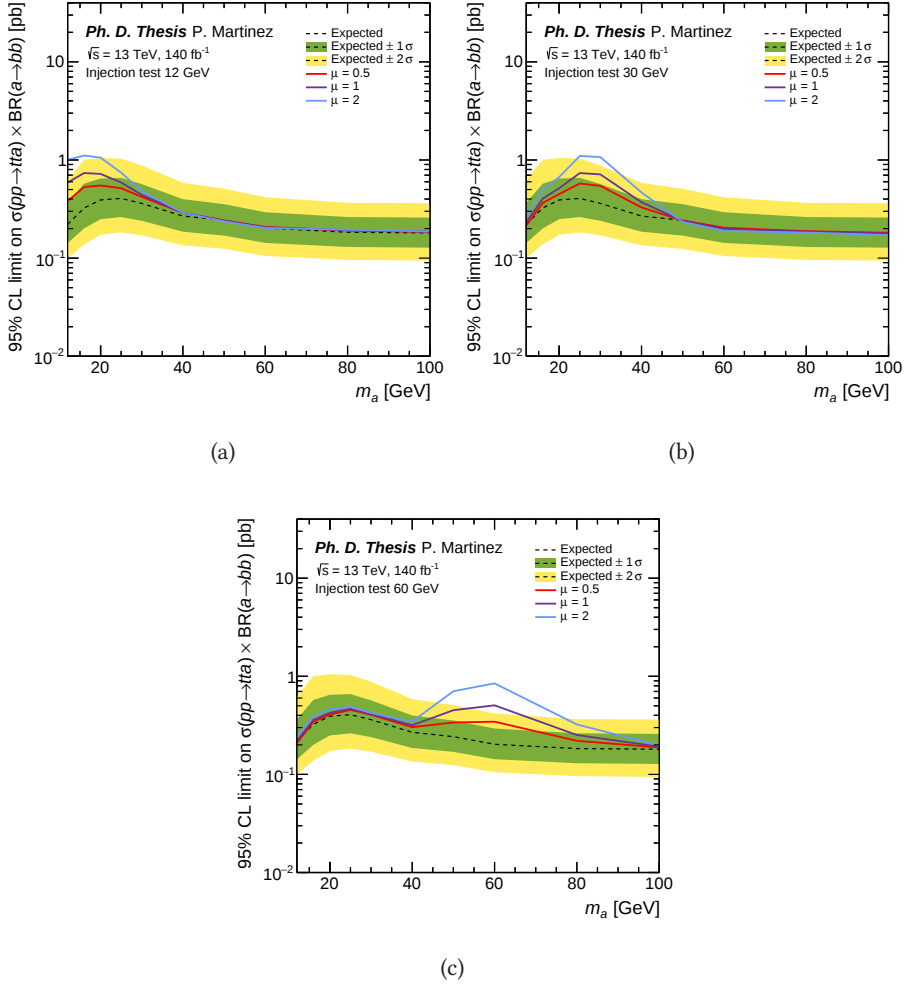
Figure C.37: Expected limits from the (a) m_a = 12 GeV, (b) m_a = 30 GeV and (c) m_a = 60 GeV injection tests. They are computed for \mu = 0 (dashed black line), \mu = 0.5 (solid red line), \mu = 1 (solid purple line) and \mu = 2 (solid blue line).
