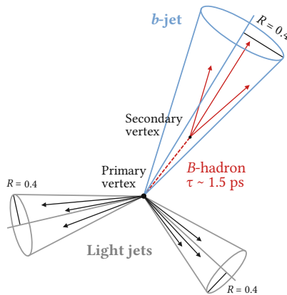
Figure 6.2: Schematic representation of a b -jet.
