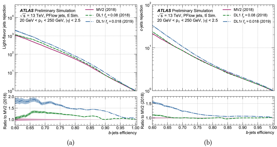
Figure 6.4: DL1r light- and c -flavour rejection with respect to the b -jet efficiency [152].
