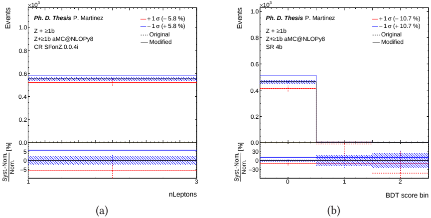
Figure 10.6: Up (red) and down (blue) 1\sigma variation of the MADGRAPH5_aMC@NLO ME uncertainty in the (a) Z + \text{jets} 4b CR and the (b) 4b SR, corresponding to the Z + \geq 1b MC sample.
