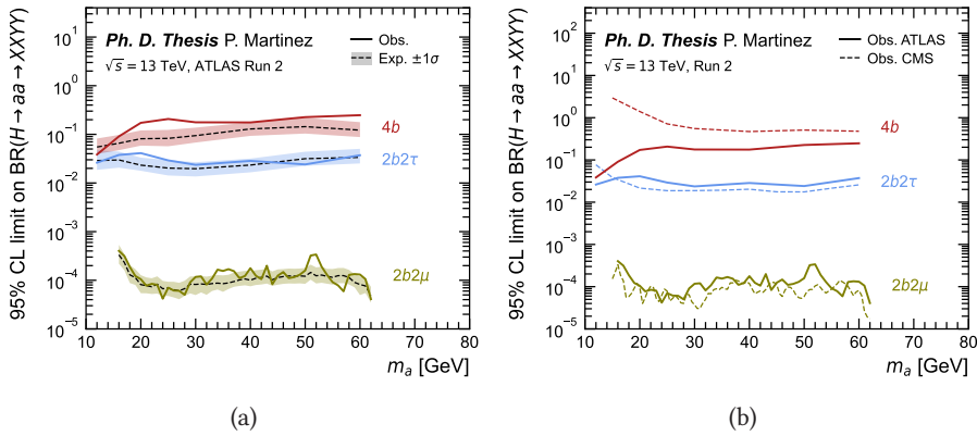
Figure 10.15: (a) Expected and observed 95% CL upper limits of \text{BR}(H \rightarrow aa \rightarrow XYY) as a function of m_a using the full Run 2 dataset recorded by the ATLAS experiment. (b) Observed 95% CL upper limits of \text{BR}(H \rightarrow aa \rightarrow XYY) as a function of m_a using the full Run 2 dataset recorded by the ATLAS and CMS experiments. Only analyses with at least two b -quarks in the final state are included.
