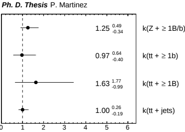
Figure B.28: Normalisation factors for the Z +jets and t\bar{t} +jets samples in the blinded fit to data with m_a = 25 GeV.
