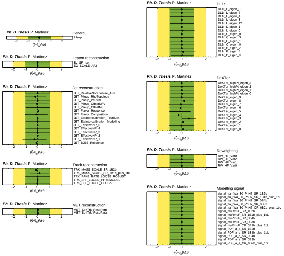
Figure B.35: Fitted nuisance parameters from the blinded fit to data with m_a = 30 GeV (I).
