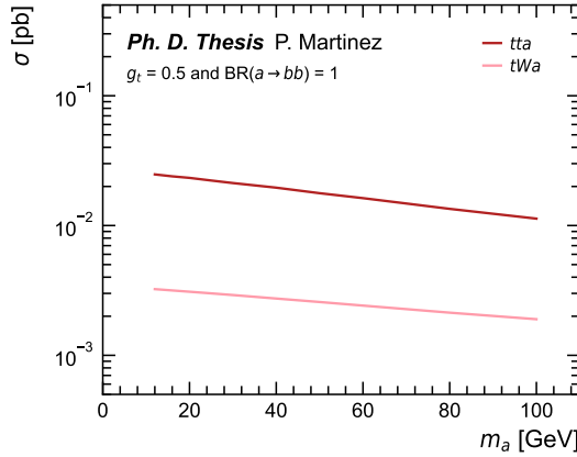
Figure 11.2: Cross sections for the t\bar{t}a and tWa signal processes assuming g_t = 0.5 and \text{BR}(a \rightarrow b\bar{b}) = 1 .
