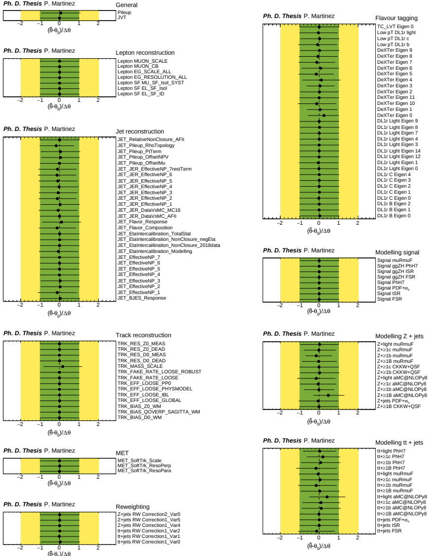
Figure B.30: Fitted nuisance parameters from the blinded fit to data with m_a = 25 GeV.
