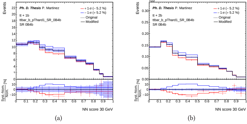
Figure 12.12: Up (red) and down (blue) 1\sigma variation of the p_{T\text{Hard}}=1 uncertainty with respect to the NN score distribution for the (a) t\bar{t}+1b and the (b) t\bar{t}+2b MC samples in the 0B4b SR.
