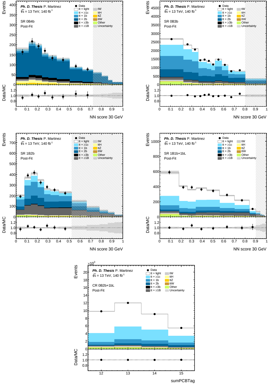
Figure B.32: Post-fit plots from the blinded fit to data with m_a = 30 GeV.
