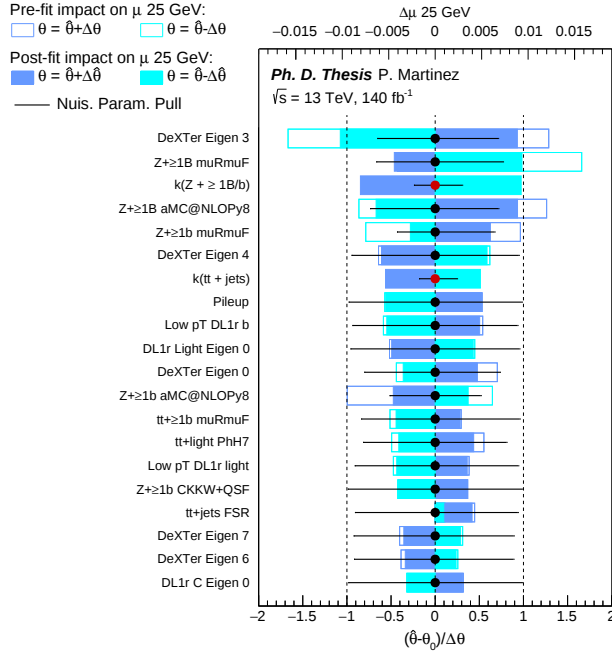
Figure 10.8: Ranked systematic impacts to the signal strength from the B-only fit to the Asimov dataset with m_a = 25 GeV.
