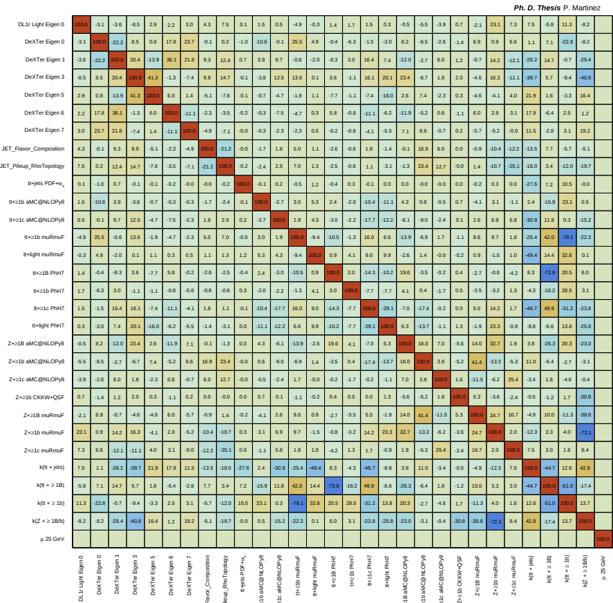
Figure B.29: Correlation matrix for the relevant NPs in the blinded fit to data with m_a = 25 GeV.
