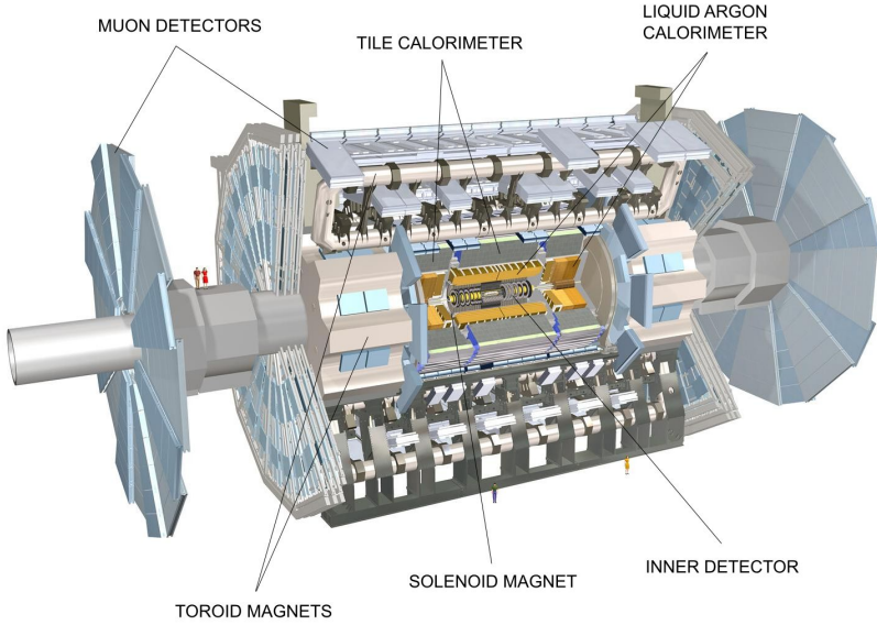
Figure 4.6: The ATLAS detector at CERN [75].
