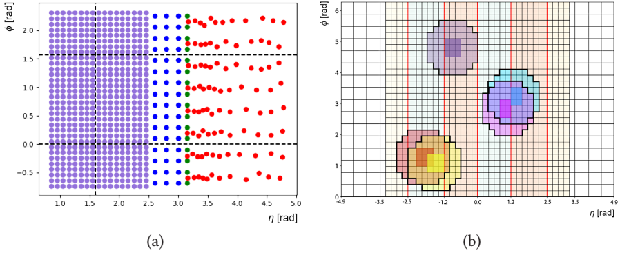
Figure A.24: Granularity of the inputs to (a) jFEX and (b) gFEX in the \Delta\eta \times \Delta\phi plane [240].
