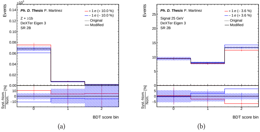
Figure 10.5: Up (red) and down (blue) 1\sigma variation of the third eigenvalue of the DeXTer systematic uncertainty in the 2B SR, corresponding to the (a) Z + \geq 1b MC sample and the (b) 25 GeV signal MC sample.
