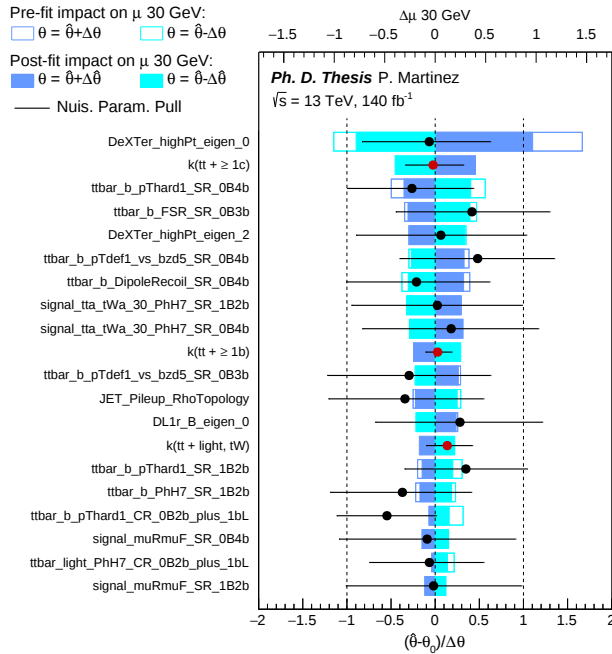
Figure 12.20: Ranked impact of the systematic uncertainties to the signal strength from the S+B fit to data with m_a = 30 GeV.
