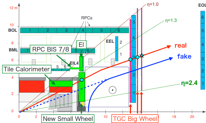
Figure A.25: Phase-I upgrades for the L1Muon trigger [241].
