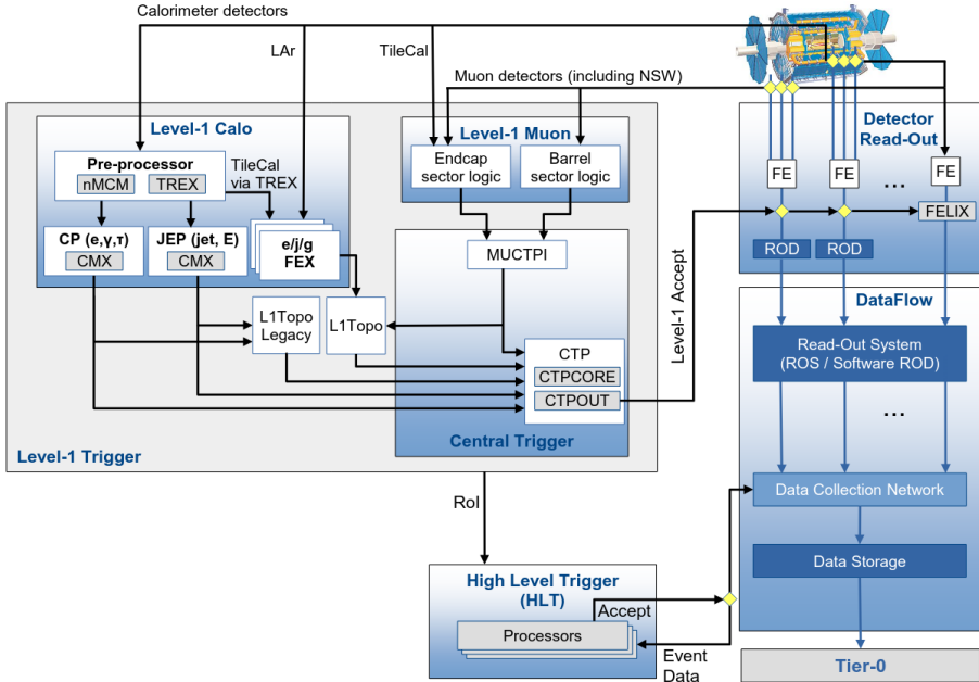
Figure A.22: Schematics of the ATLAS TDAQ system in Run 3.
