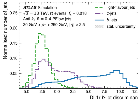
Figure 6.3: Normalised distributions of the DL1r b -jet discriminant corresponding to light-, c - and b -jets for a t\bar{t} test sample using f_c = 0.018 [150].
