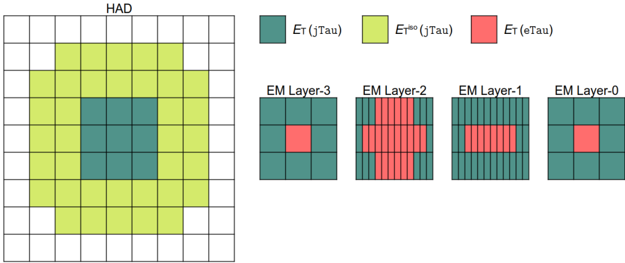
Figure A.26: Visual representation of the trigger towers used to determine E_T(\text{jTau}) , E_T^{\text{iso}}(\text{jTau}) and E_T(\text{eTau}) . Each square corresponds to one trigger tower, some of them containing several SuperCells. HAD and EM refer to the hadronic and EM calorimeters, respectively.
