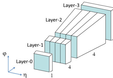
Figure A.23: Trigger tower composed of ten SuperCells after the Phase-I upgrade for the LAr calorimeter [94].
