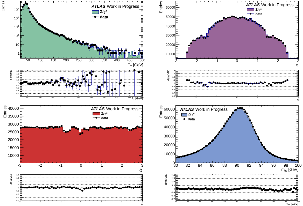
Figure 4.1: Kinematic distributions of selected Z \rightarrow ee electron probes passing the medium and B-layer hit requirements identification cuts for data and MC. Shown are the transverse energy E_T (top left), the pseudorapidity \eta (top right), the azimuthal angle \phi (bottom left). The bottom right plot shows the invariant mass m_{ee} obtained combining all the tag and probe pairs.
