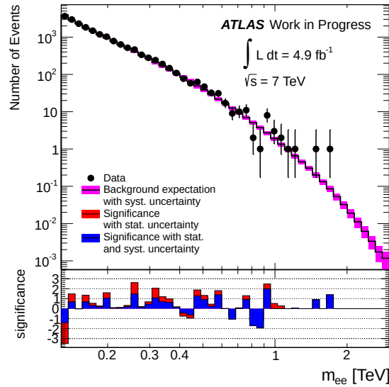
Figure 5.19: Differences between data and expectation in the electron channel. The mass range goes from 130 GeV to 3 TeV.
