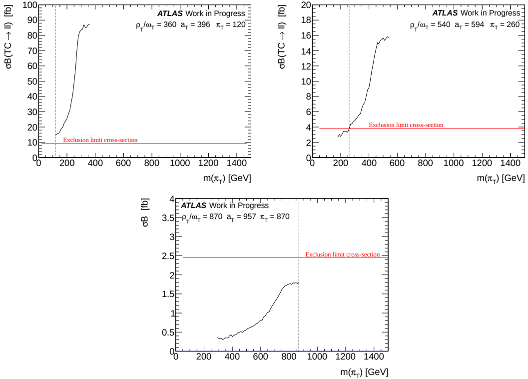
Figure 5.25: The predicted \rho_T/\omega_T \rightarrow l^+l^- cross-section as function as the \pi_T mass for three different points in the m(\rho_T/\omega_T) : m(\pi_T) plane. For each value of m(\rho_T/\omega_T) the m(\pi_T) corresponding to the intersection of the 95% C.L. exclusion cross-section measurement (the red line) with the theoretically predicted \sigma_T is displayed.
