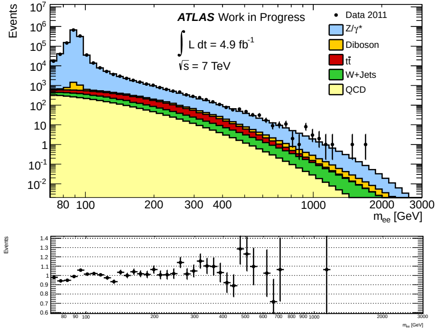
Figure 5.11: Dielectron invariant mass ( m_{ee} ) distribution after event selection for the 2011 data and the SM backgrounds overlaid.
