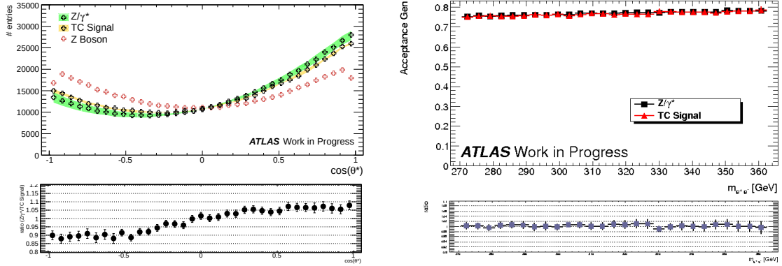
Figure F.1: On the left plot \cos(\theta^*) distribution at generator level for the Z bosons, the Z/\gamma^* , and TC signal process, the colored bands define the variation of the \cos(\theta^*) distribution for different m_{ee} values. On the right plot at generator level the total acceptance as a function of the m(e^+e^-) for the Drell-Yan process and for a TC signal at 300 GeV. Note that Z/\gamma^* process is generated in the same mass range as the TC signal as described in section 5.1.2.
