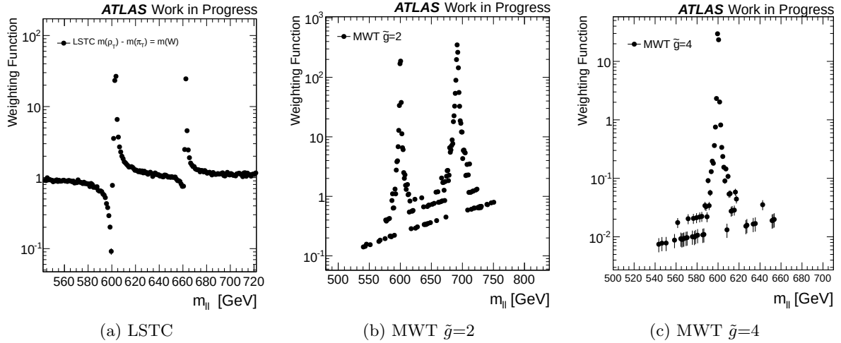
Figure 5.15: For a mass point at = 600 GeV: weighting function used to reshape the dilepton mass distribution in the officially produced Drell-Yan sample to that of a LSTC or MWT samples. (a) The LSTC case where m(\rho_T) = m(\omega_T) = 600 GeV and m(a_T) = 660 GeV. (b) The MWT scenario for \tilde{g}=2 case m(R_1) = 600 and m(R_2) = 692 , and (c) The MWT scenario for \tilde{g}=4 case where m(R_1) = 600 . Note that in the MWT case the two resonances are generated without the Drell-Yan component.
