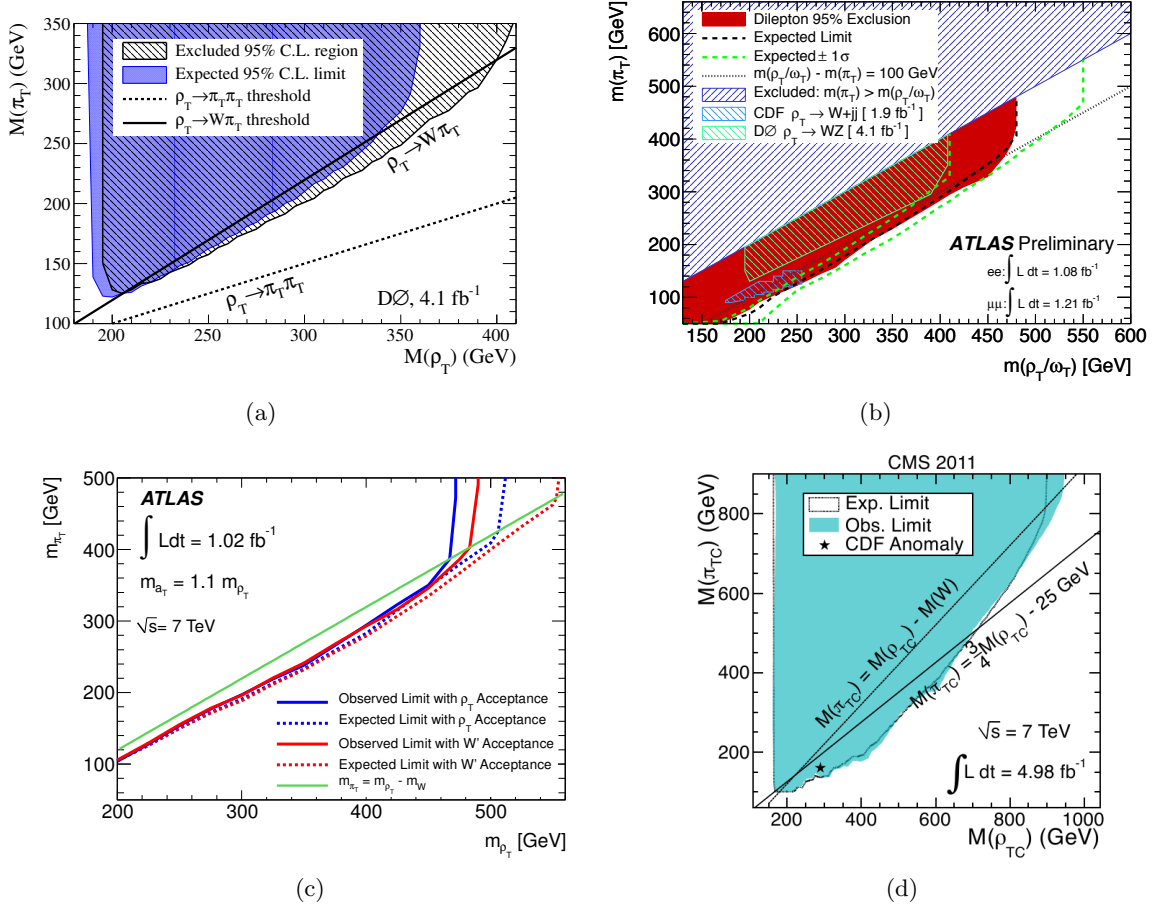
Figure 1.8: Current limits on LSTC. (a) 95% exclusion region in the plane of \rho_T vs. \pi_T masses in WZ \rightarrow lll\nu channel from the DØ collaboration, using 4.1 fb -1 of data [45]. (b) 95% exclusion region in the plane of \rho_T vs. \pi_T masses from the ATLAS collaboration, in \rho_T/\omega_T \rightarrow ll decay channel where the a_T contribution is not taken into account. Are also quoted the previous exclusion limits from CDF and DØ collaborations [36]. (c) The 95% CL expected and observed excluded mass regions in the plane of \rho_T vs. \pi_T masses in WZ \rightarrow lll\nu channel from the ATLAS collaboration using \sim 1 \text{ fb}^{-1} of data [37]. (d) The 95% exclusion region in the plane of \rho_T vs. \pi_T masses in WZ \rightarrow lll\nu channel from the CMS collaboration, using 5 fb -1 of data [38].
