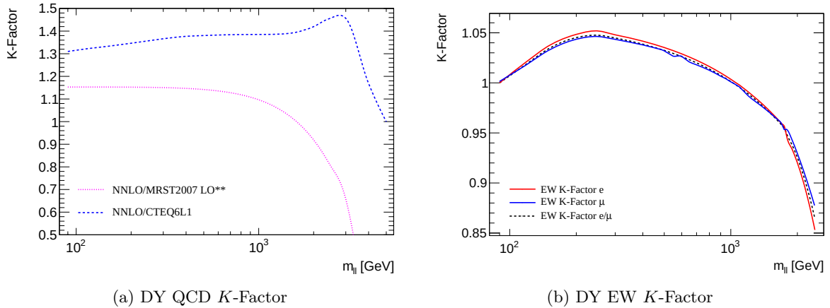
Figure 5.3: Different order QCD K -Factors for Drell-Yan lepton-pair production as function of dilepton invariant mass m_{\ell\ell} (a). The final electroweak mass dependent K -Factor for dielectron and dimuon final state separately and for the dielectron and dimuon case combined (b). The EW K -Factor for electron and muon case combined was considered to be the average of the two.
