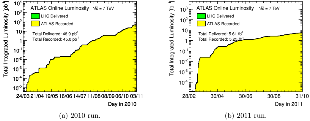
Figure 2.3: Total integrated luminosity recorded by the ATLAS experiment in 2010, and up to October 2011 [56].
