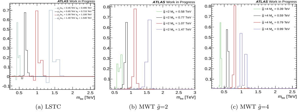
Figure 5.17: Technimesons line shape distribution at reconstruction level in the electron channel. (a) The LSTC case where each signal templates are simulated according with the theoretical cross-section. (b) and (c) In the MWT scenario for \tilde{g}=2 and for \tilde{g}=4 cases, signal template for four different M_A hypothesis. Note that in the MWT case the signal templates are normalized to unity.
