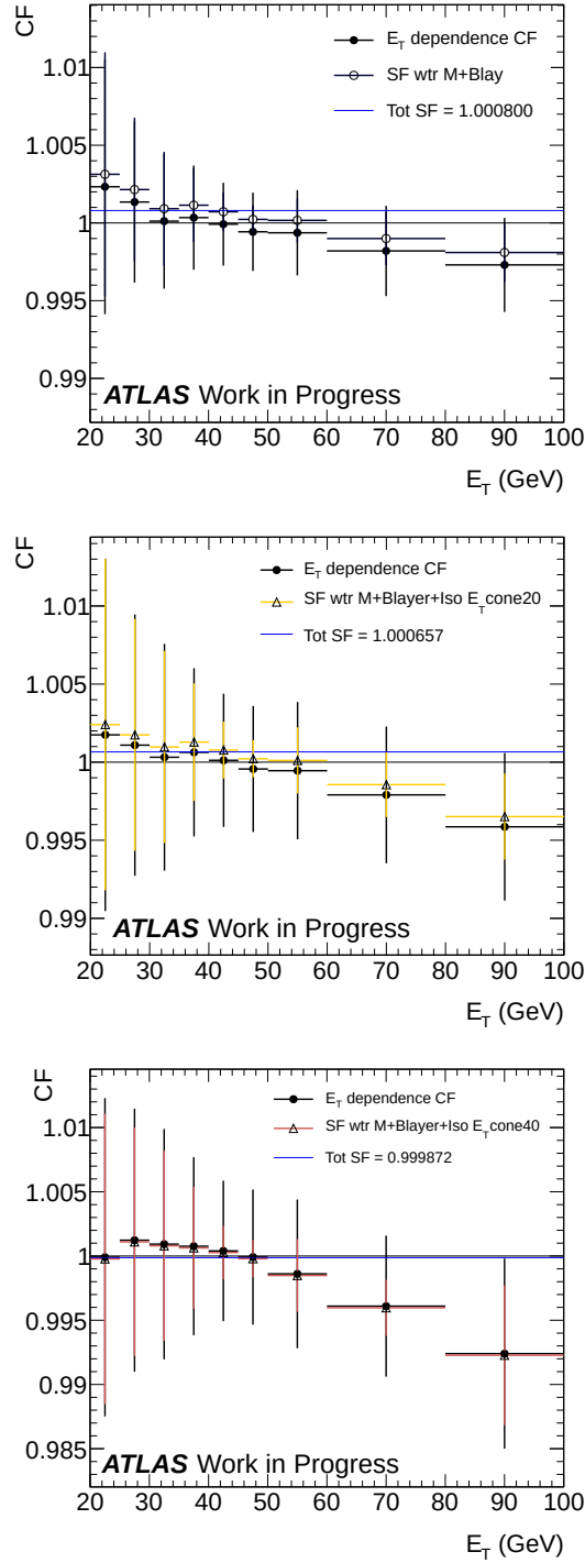
Figure 4.10: Correction factors (CF) of the medium plus B-layer (top left), B-layer plus E_T cone20 isolation (top right), and B-layer plus E_T cone40 isolation requirement (bottom plot). Each bin of the E_T dependent SF is scaled for the data/MC ratio integrated over the full pseudorapidity range |\eta| < 2.47 and over the electron E_T > 25 GeV. The errors evaluated in the plots take into account the statistical and systematic uncertainties.
