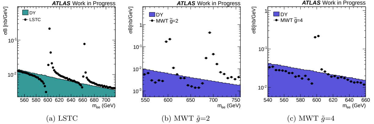
Figure 5.2: Techimesons line-shape distribution at generator level. (a) The LSTC model with m(\rho_T) = m(\omega_T) = 600 GeV and m(a_T) = 660 GeV. (b) The MWT model with \tilde{g}=2 and M_A = 581 GeV, (c) The MWT model with \tilde{g}=4 and M_A = 596 GeV. In all the plots the filled histogram is the SM Drell-Yan distribution.
