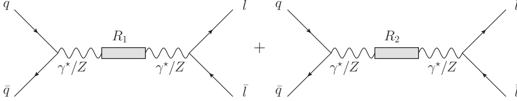
Figure 1.13: Feynman Diagram of the MWT process giving fermion pairs l\bar{l} as a final state.
