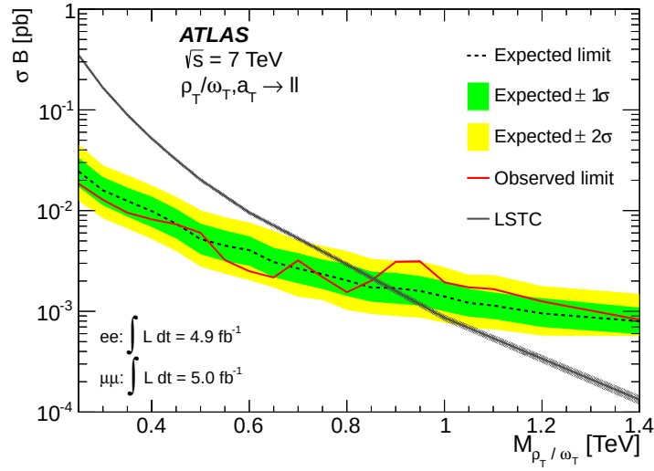
(b) electron and muon combined
