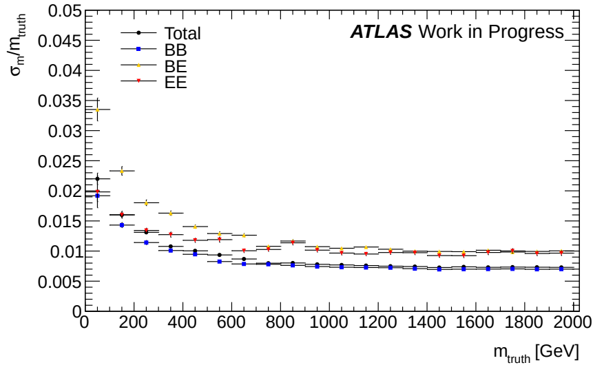
Figure E.3: Mass resolution as function of M_{truth} , showing overall mass resolution and the three possible different event configurations.
