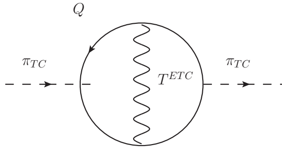
Figure 1.3: Feynman Diagram of the correction to the propagator of a technimeson via the exchange of an ETC gauge boson. This diagram leads to scale up the mass of the technimeson.
