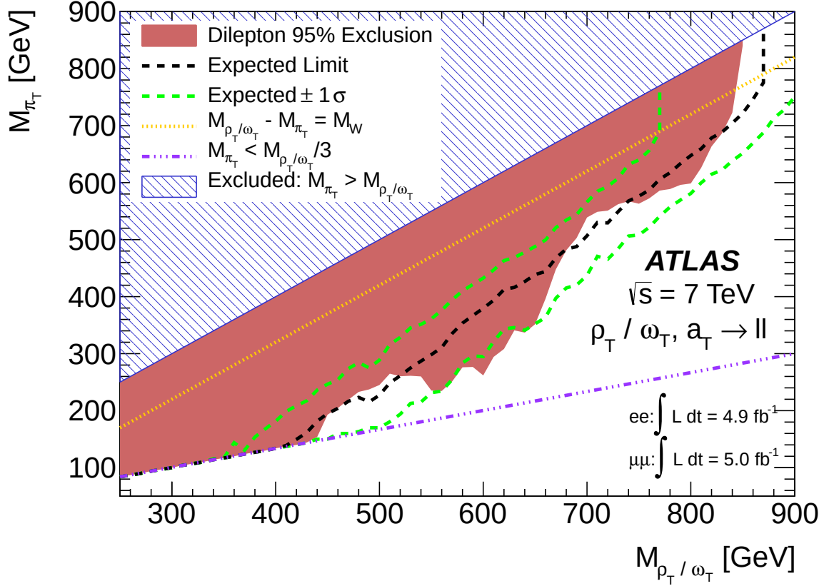
Figure 5.26: The 95% C.L. exclusion region as a function of the \rho_T/\omega_T and \pi_T masses is shown in red, assuming m(a_T) = 1.1 \times m(\rho_T/\omega_T) . The yellow dotted line corresponds to m(\rho_T/\omega_T) - m(\pi_T) = m(W) . The black dashed line shows the expected limit, with the green dashed lines showing the \pm 1\sigma bands. The blue hashed region in which m(\pi_T) > m(\rho_T/\omega_T) is excluded by theory. This search is insensitive in the region below the violet dotted line ( m(\pi_T) < m(\rho_T/\omega_T)/3 ) due to vanishing branching ratio of \rho_T and \omega_T to dileptons, as is explain in the text.
