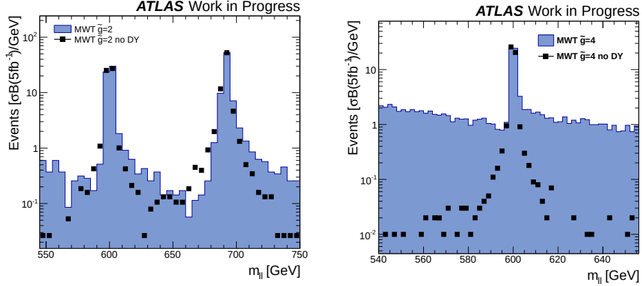
Figure 5.16: On the left plot: The dilepton invariant mass distribution in the MWT scenario for \tilde{g}=2 case, where m(R_1) = 600 and m(R_2) = 692 , the fill histogram is the MWT process with the Drell-Yan component and the points represent the case in which the resonance is generated without the Drell-Yan component. Note that in the latter case only the interference between the two resonance is present.
