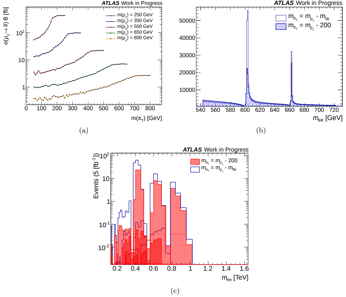
Figure 5.23: (a) The \rho_T/\omega_T dilepton cross-section times the branching fraction as a function of m_{\pi_T} . (b) At generator level, line shape for m_{\rho_T/\omega_T} = 600 GeV generated with two different mass splitting hypothesis: m(\rho_T/\omega_T) - m(\pi_T) = m(W) for the empty histogram and m(\rho_T/\omega_T) - m(\pi_T) = 200 GeV for the filled histogram. (c) LSTC signal templates for m_{\rho_T/\omega_T} = 400, 600, 800 GeV generated with m(\rho_T/\omega_T) - m(\pi_T) = m(W) for the black histograms and m(\rho_T/\omega_T) - m(\pi_T) = 200 GeV for the red histograms. Note that the templates are normalized to the predicted cross-section.
