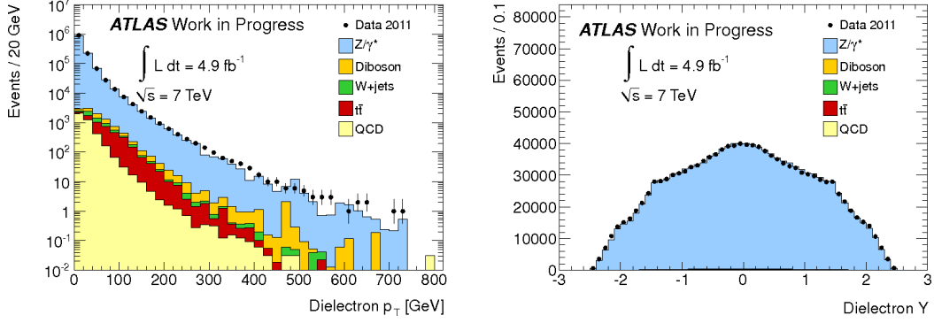
Figure 5.10: Dielectron p_T and rapidity after event selection.
