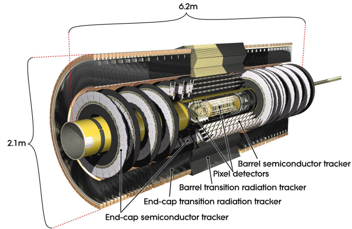
(a) The ATLAS Inner Detector. The central and end caps region are visible.
