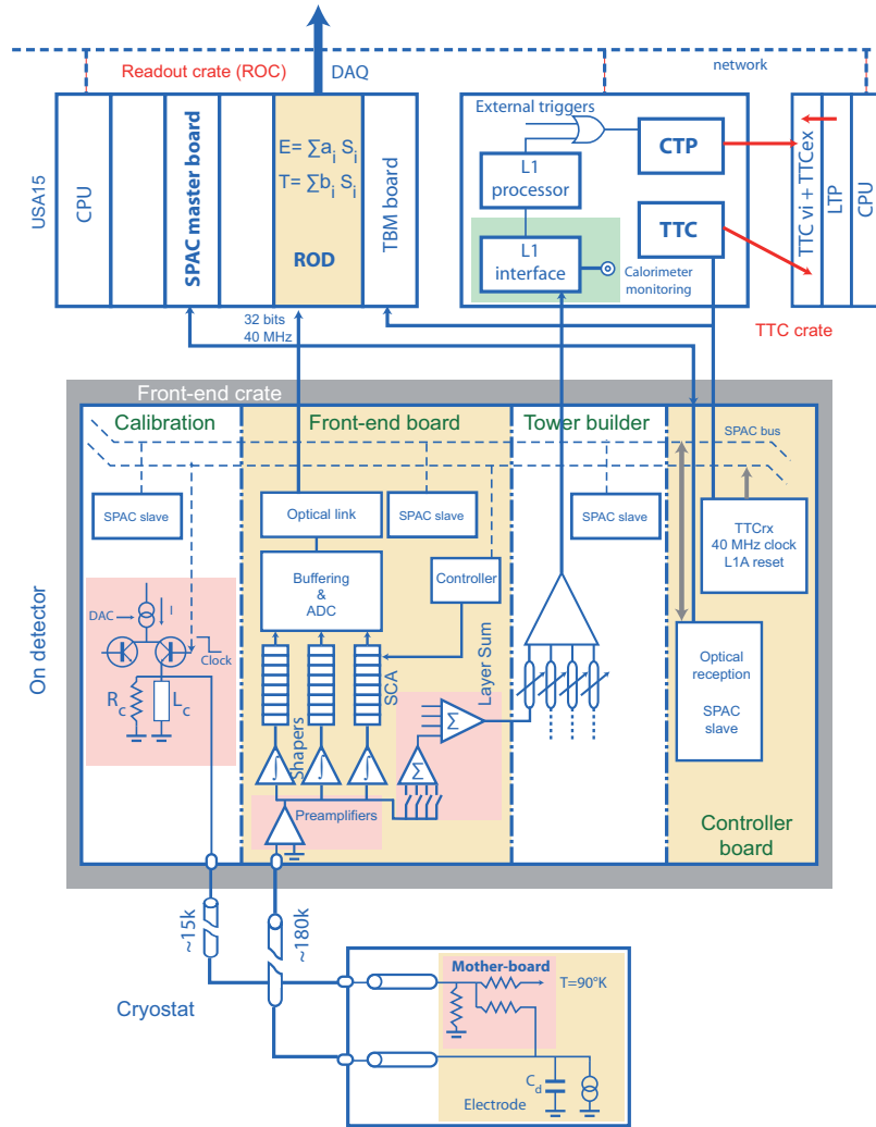
Figure 3.3: Block diagrams showing the architecture of the overall LAr Calorimeter readout electronic.
