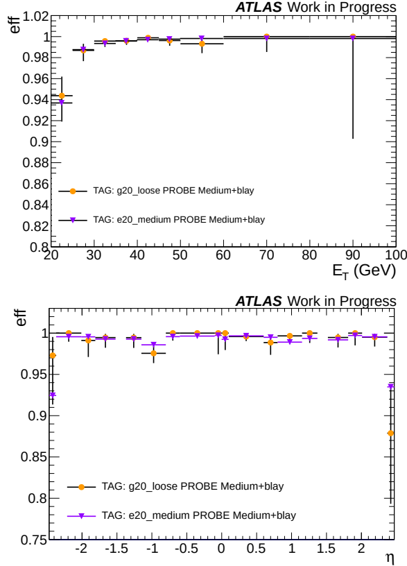
Figure C.1: For the tag electron matched with the g20_{loose} or the e2^*_{medium} trigger items. Data efficiencies comparison with respect to offline medium plus B-layer probe electrons for 2g20_{loose} trigger measured as a function of the offline electron E_T , and the offline electron \eta with |\eta| < 2.47 and E_T > 25 GeV, for both case the transition region between the barrel and endcap EM calorimeters are excluded. Note that about \sim 50\% of the 2011 data are used, corresponding to \sim 2.7fb^{-1} .
