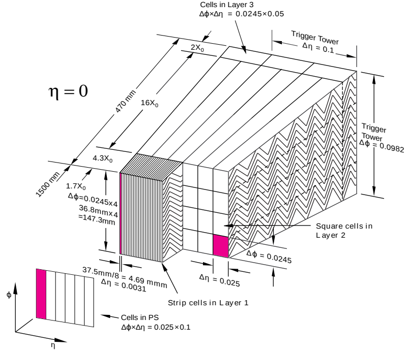
Figure 3.2: Sketch of a barrel module where the different layers are clearly visible with the accordion structure in \phi . The granularity in \eta and \phi of the cells of each layers and of the trigger towers is also shown.
