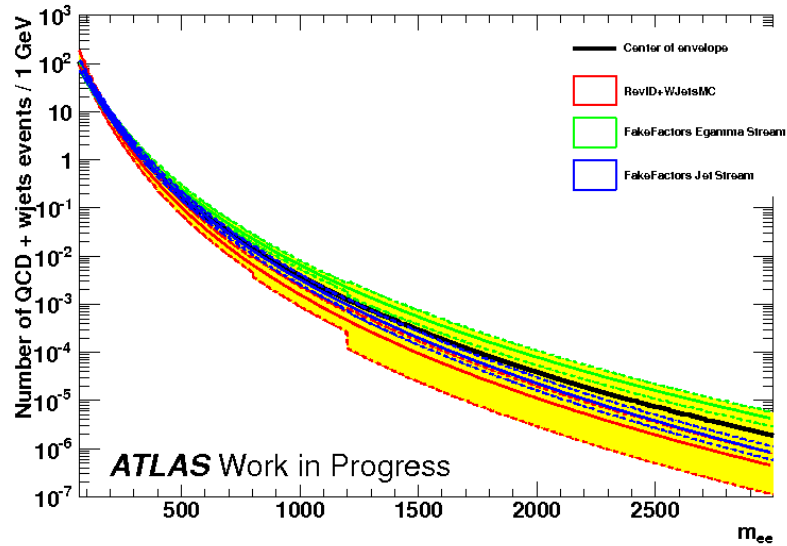
Figure 5.12: Combination of the QCD plus W + \text{jets} via the background envelope method as is done in Reference [83]. The central value of the envelope is shown in black with the yellow error band. The separate methods are shown as colored lines with their uncertainty band shown with dashed lines in the same color.
