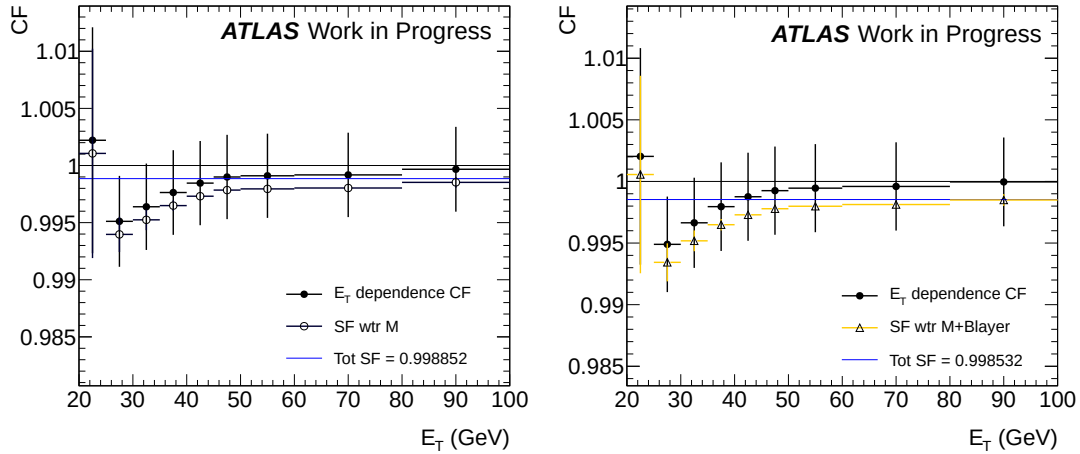
Figure 4.6: Correction factors (CF) of the medium (left) and of the medium plus B-layer hit requirement (right). Each bin of the E_T dependent SF is scaled for the data/MC ratio integrated over the full pseudorapidity range |\eta| < 2.47 and over the electron E_T > 25 GeV. The errors evaluated in the plots take into account the statistical and systematic uncertainties.
