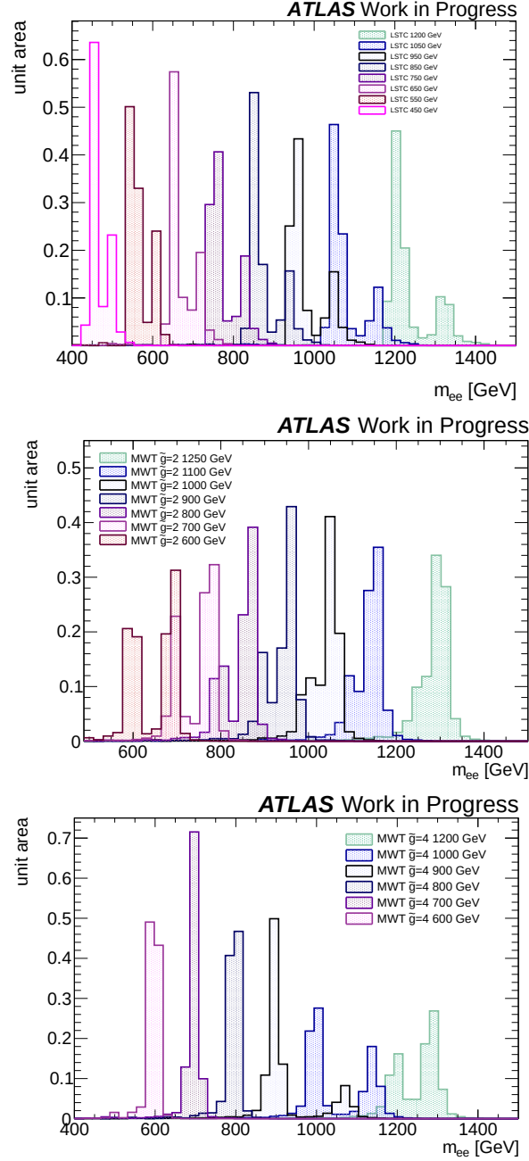
Figure F.2: Dielectron invariant mass ( m_{ee} ) distribution after event selection for a few TC pole masses, for the LSTC and the MWT for \tilde{g}=2 and \tilde{g}=4 . In those plots the dielectron invariant mass ( m_{ee} ) distribution after event selection is shown in linear scale to better see the line shape of the two resonances present in the spectrum.
