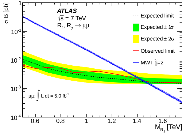
(b) MWT \tilde{g}=2
