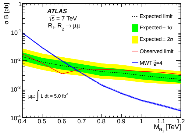
(c) MWT \tilde{g}=4
