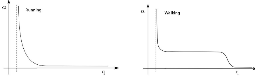
Figure 1.5: (left) QCD-like behavior of the coupling constant as function of the momentum (Running). (right) Walking-like behavior of the coupling constant as function of the momentum (Walking)
