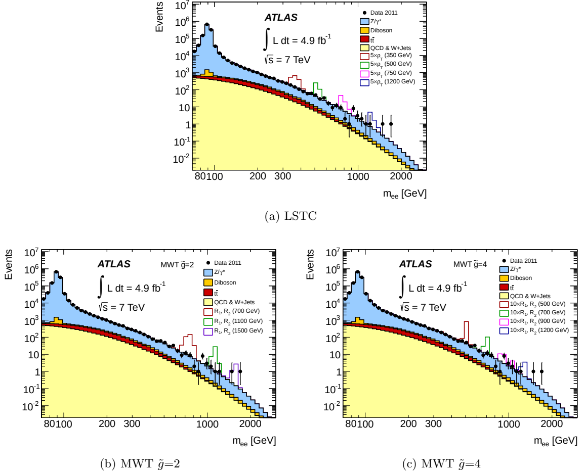
Figure 5.13: Dielectron invariant mass ( m_{ee} ) distribution after event selection for the 2011 data and the SM backgrounds overlaid. (a): m_{ee} distribution where four different LSTC signals are overlaid. (b) and (c): m_{ee} distribution where different MWT signals are overlaid for \tilde{g}=2 and \tilde{g}=4 hypothesis respectively.
