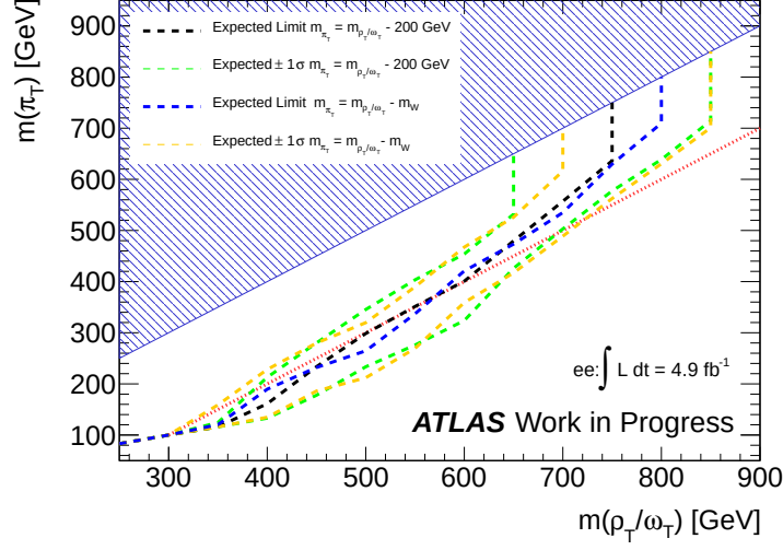
Figure 5.24: For the dielectron channel only, expected exclusion region in the parameter space m(\rho_T/\omega_T) vs m(\pi_T) , obtained with m(\rho_T/\omega_T) - m(\pi_T) = m(W) for the blue dashed line and m(\rho_T/\omega_T) - m(\pi_T) = 200 GeV for the black dashed line. For both hypothesis the \pm 1\sigma bands are also displayed. The dark red dashed line shows the m(\pi_T) = m(\rho_T/\omega_T) - 200 GeV.
