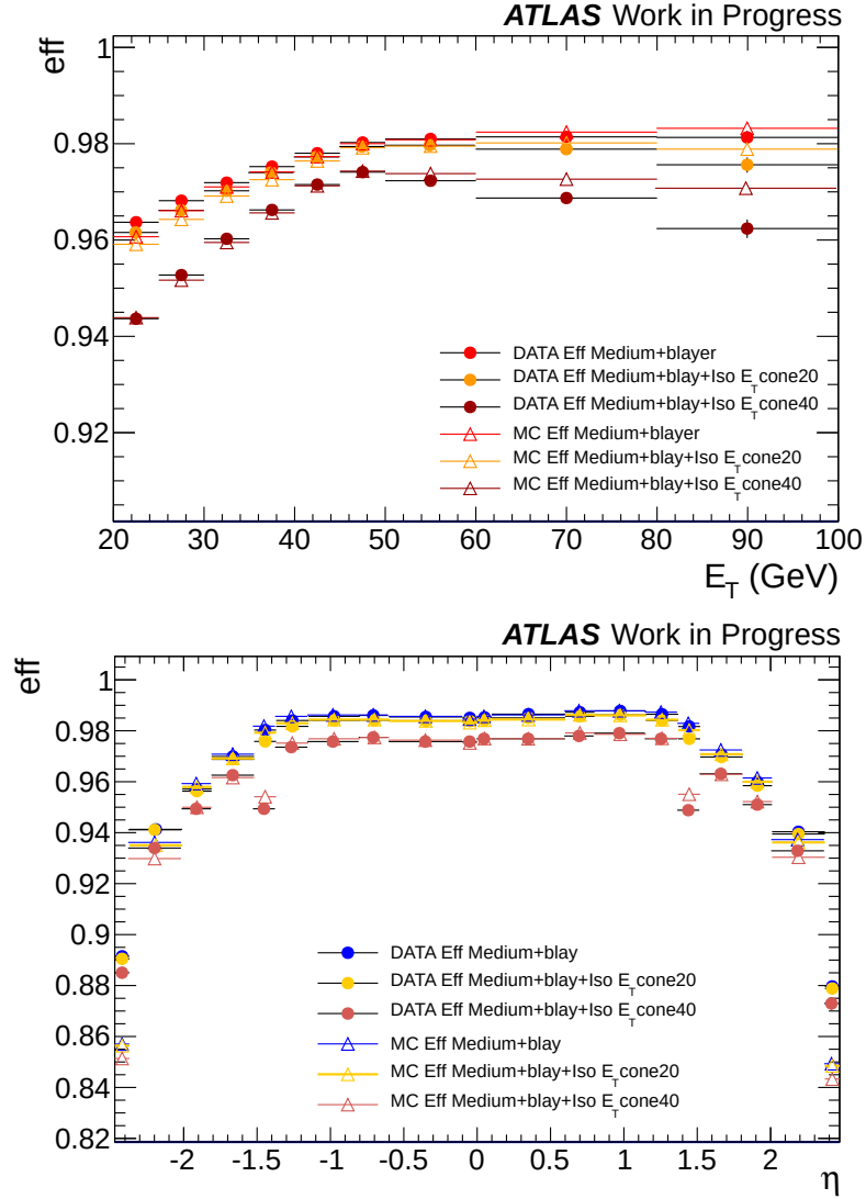
Figure 4.7: Data and MC electron identification efficiencies of the B-layer hit requirement, of the B-layer hit plus E_T cone20 isolation requirement, and of the B-layer hit plus E_T cone40 isolation requirement. Those efficiencies are measured as a function of (top) the electron E_T and (bottom) as a function of \eta for electron with E_T > 25 GeV. The errors evaluated in the plots take into account only the statistical uncertainties.
