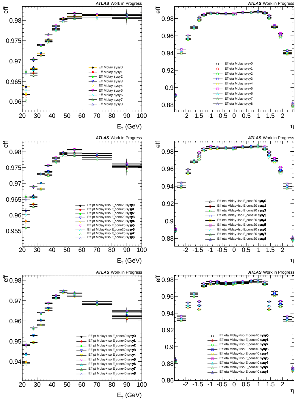
Figure 4.8: Systematic variations on the electron identification efficiencies measured in data with respect to the B-layer hit requirement (top), B-layer hit and E_T cone20 isolation requirement (middle), and B-layer hit and E_T cone40 isolation requirement (bottom). Those efficiencies variations are measured as a function of the electron E_T (left), and as a function of electron \eta (right). The so called sys7 correspond to the configuration with higher background and weaker tag cuts (see Table 4.2 for the details).
