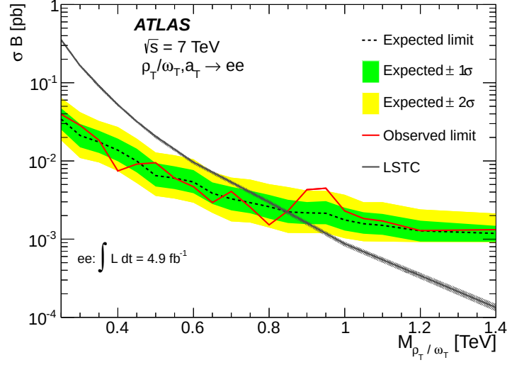
(a) electron channel
