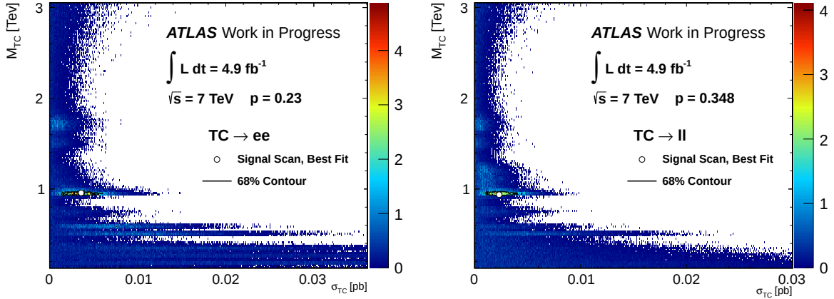
Figure 5.18: The absolute value of the profile LLR test as a function of \sigma_{TC} and M_{TC} for the likelihood fit (left) to ATLAS data in the dielectron channel; (right) to ATLAS data for the combination of the dielectron and dimuon channel.
