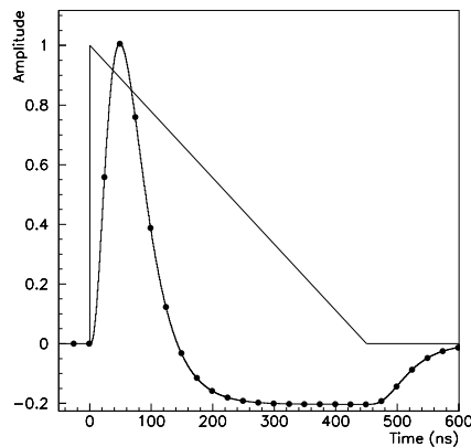
Figure 3.4: Amplitude versus time for triangular pulse of the current in a LAr barrel electromagnetic cell and of the FEB output signal after bi-polar shaping. Also indicated are the sampling points every 25 ns.
