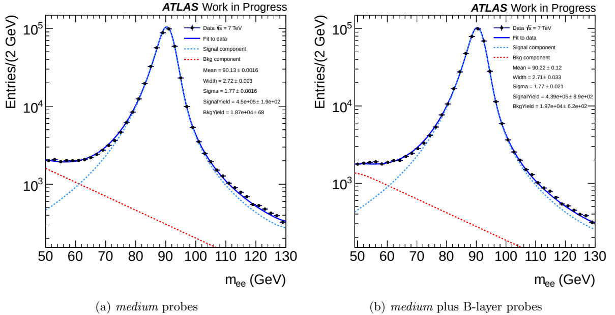
Figure 4.2: The invariant mass distribution in the data of tag and probe candidates passing the selection criteria described in Section 4.2. The probe electrons have to pass either the medium (a) or the medium plus B-layer hit (b) selection respectively. In the plots the invariant mass distribution is shown as well as the fit results for signal and background individually. The fit was done using a Breit-Wigner convoluted with a Crystal-Ball distribution for the signal and a single sided decay function for the background description
