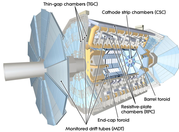
Figure 2.9: Atlas muon spectrometer system [54].
