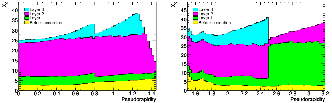
Figure 2.7: Cumulative amounts of material, in units of radiation length ( X_0 ) and as a function of |\eta| , in front of and in the electromagnetic calorimeters [58]. For the barrel (left) and end-cap (right) is shown the thicknesses of each accordion layer as well as the amount of material in front of the accordion.
