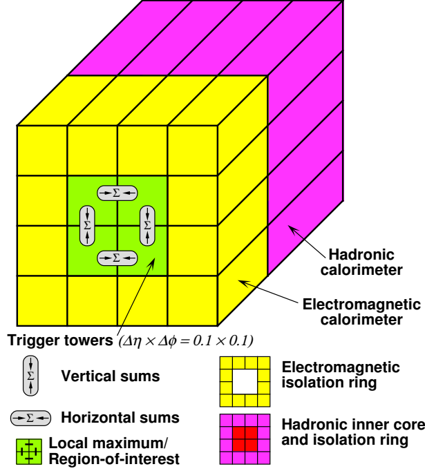
Figure A.2: A scheme of the L1 algorithm to find EM RoIs [58].
