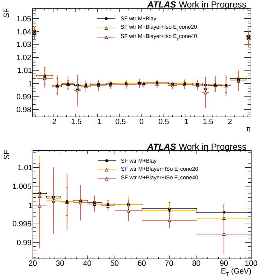
Figure 4.9: SF for the identification efficiencies for medium plus B-layer electrons and medium plus B-layer and E_T cone20 and E_T cone40 isolation requirement as a function of the electron \eta (top) and as a function of E_T (bottom) bins. The errors evaluated in the plots take into account the statistical and systematic uncertainties.
