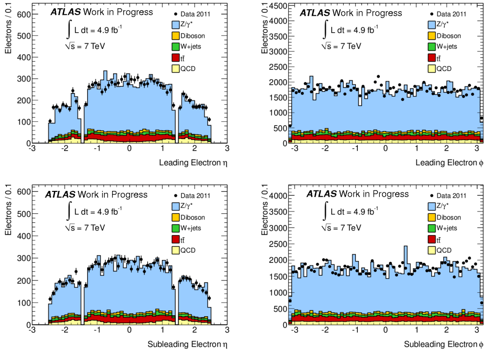
Figure 5.7: \eta and \phi distributions for the leading electron and sub-leading electron after event selection and m_{ee} > 150 GeV.
