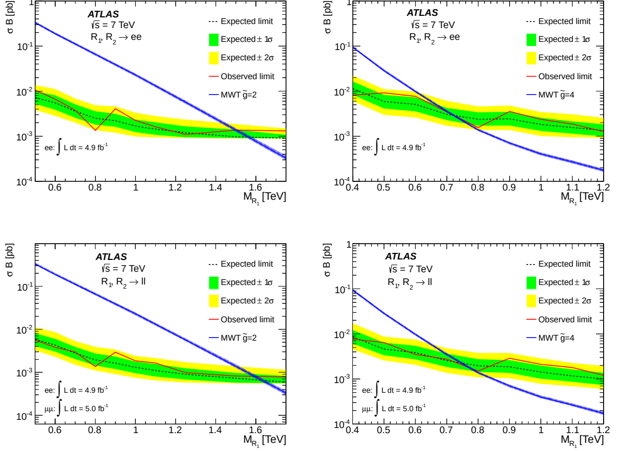
Figure 5.27: Expected and observed 95% C.L. limits on \sigma B for R_{1,2} production as a function of m(R_1) for the electron channel (top) and for the combination of the dielectron and the dimuon decay channels (bottom). On the left side MWT limits for the benchmark coupling point \tilde{g}=2 and on the right side for \tilde{g}=4 . In the plots the thickness of the theoretical curve represents the systematic uncertainties on the signal cross-section.
