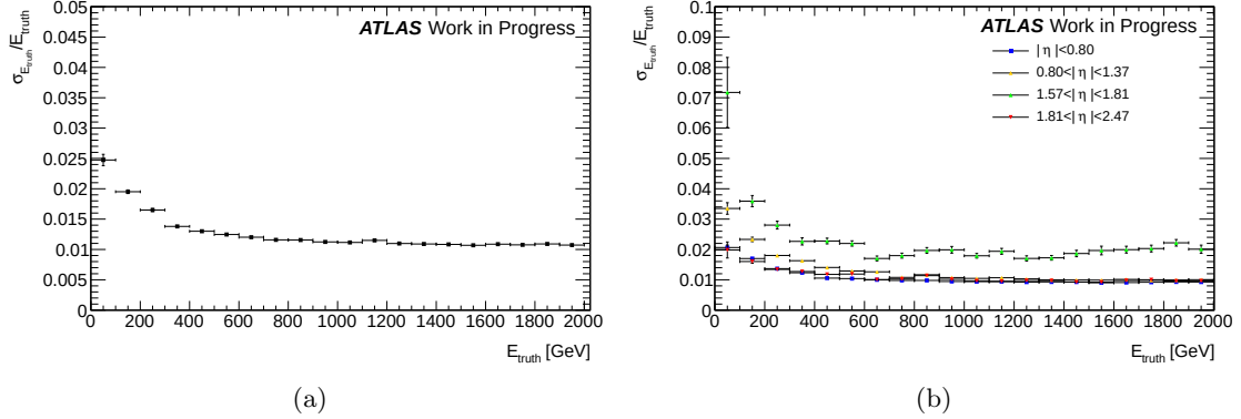
Figure E.2: Energy resolution as a function of E_{truth} . (a) energy resolution over full \eta -range; (b) energy resolution in \eta bins. The points in the plots correspond to the width of the \frac{\sigma_e}{E_{truth}} distribution obtained with a gaussian fit.
