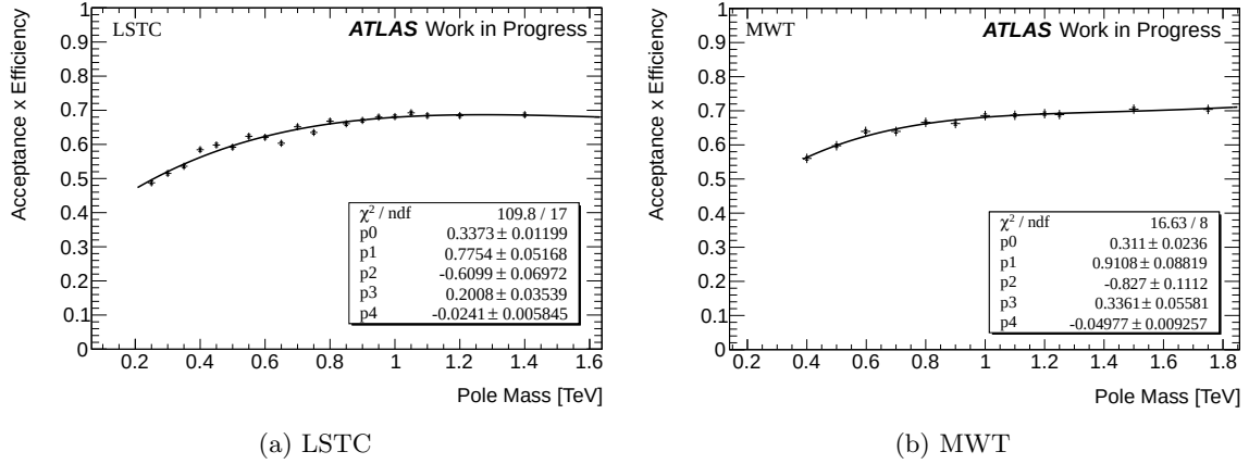
Figure 5.20: Electron channel: total acceptance times efficiency as a function of the pole mass for the technicolor models: LSTC (left), MWT (right).
