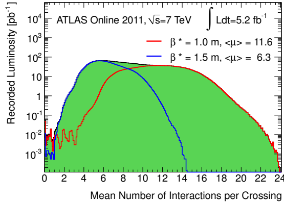
Figure 5.1: The luminosity-weighted distribution of the mean number of interactions per crossing ( \langle \mu \rangle ) for 2011 data, taken with two different LHC setup
