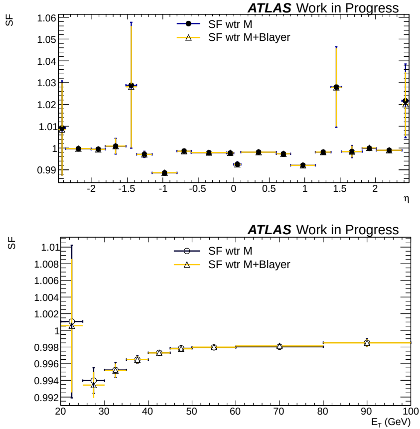
Figure 4.5: Trigger efficiency SF with respect to medium and medium plus B-layer hit requirements for 2g20\_loose trigger measured as a function of (top) the electron \eta and (bottom) as a function of the electron E_T . The errors evaluated in the plots take into account the statistical and systematic uncertainties.
