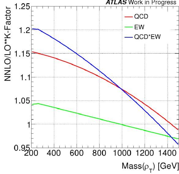
Figure 5.4: Cross section ratios for different \rho_T/\omega_T mass giving the QCD, EW and full QCD times EW K -Factors.
