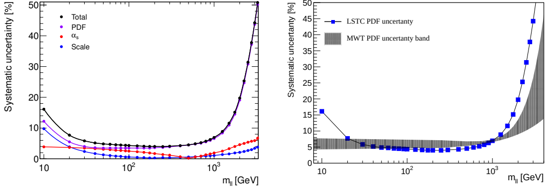
Figure 5.14: Left: PDF uncertainties on the NNLO Drell-Yan lepton-pair production cross-section as function of dilepton mass m_{\ell+\ell-} . The PDF and \alpha_s uncertainties are evaluated using the MSTW2008 PDF error sets. Right: PDF uncertainties on the LSTC and MWT lepton-pair signal production cross-section as function of dilepton mass m_{\ell+\ell-} . The PDF uncertainty for MWT model are evaluated using the CTEQ6.6 PDF error sets, as a function of the resonance mass and for different hypothesis on the coupling \tilde{g} .
