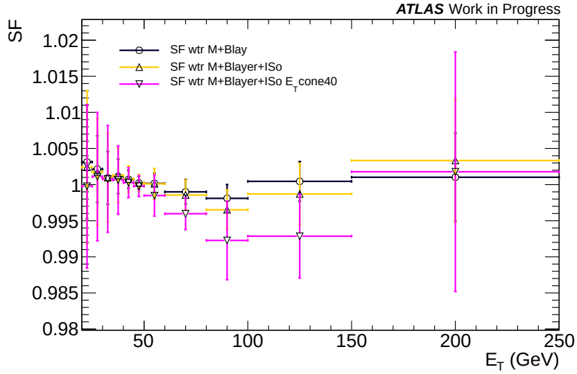
Figure D.4: SF for the identification efficiencies for medium plus B-layer electrons and medium plus B-layer and E_{T\text{cone}20} and E_{T\text{cone}40} isolation requirement as a function of the electron E_T bins. The errors evaluated in the plots take into account the statistical and systematic uncertainties.
