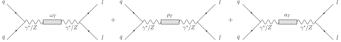
Figure 1.6: Feynman Diagram of the LSTC process giving fermion pairs l\bar{l} as a final state.
