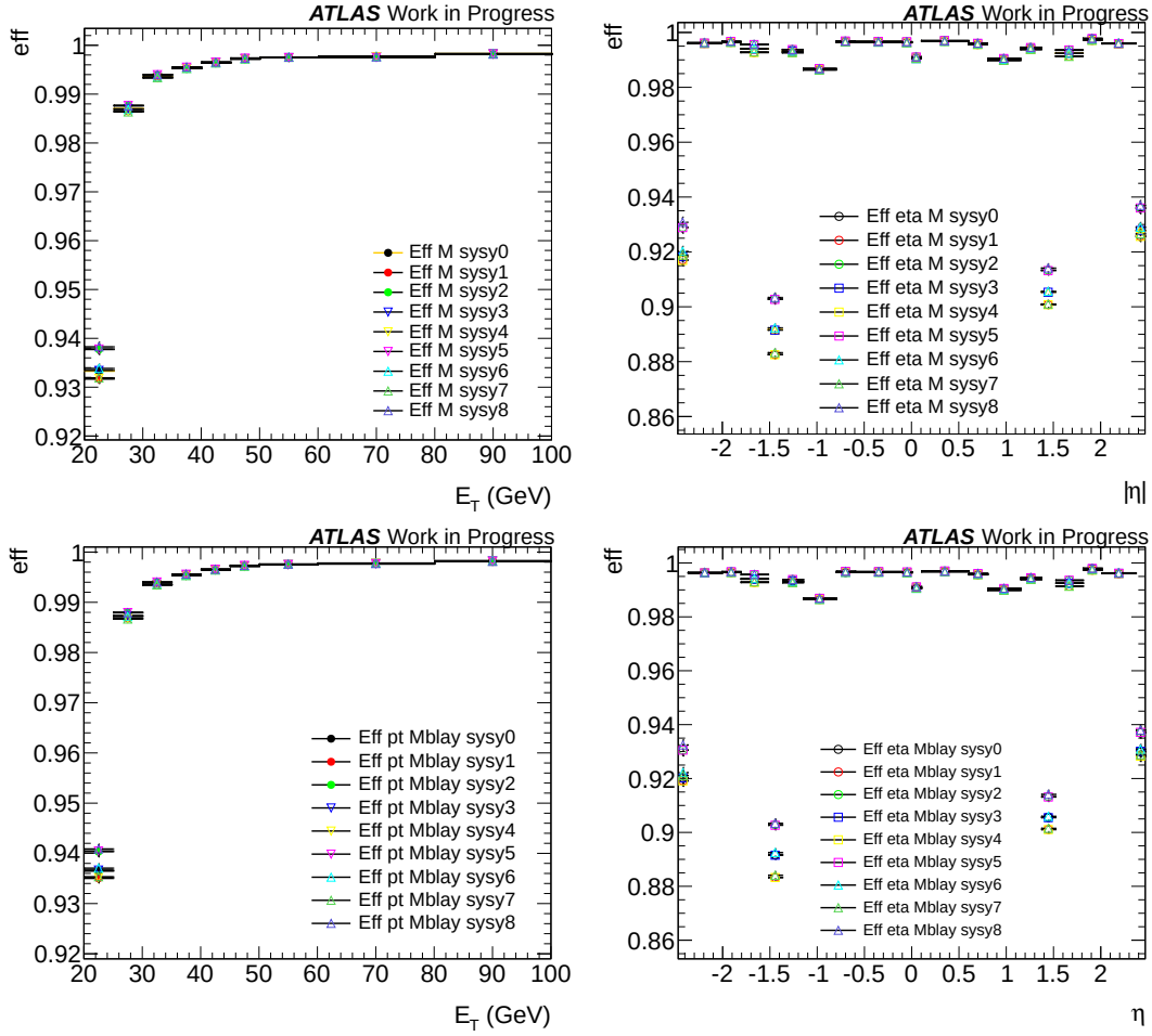
Figure 4.4: Systematic variations on the 2g20\_loose trigger efficiencies measured on data with respect to medium (top) and medium plus B-layer (bottom) probe electrons. Those efficiencies variations are measured as a function of the electron E_T (left) and as a function of the electron \eta (right). The so called sys7 correspond to the configuration with higher background and weaker tag cuts (see Table 4.2 for the details).
