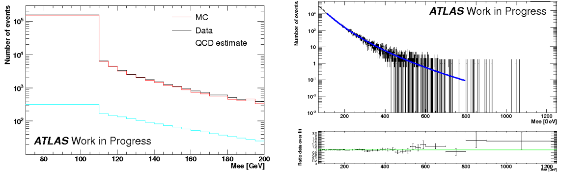
Figure 5.5: Left plot: Results of the normalization template fit performed on the data and on the QCD and non-QCD background templates. The red line represent the non-QCD backgrounds, the black one the data and the blue line the QCD template. Right plot: The QCD data template obtained with a fail- medium requirement corrected for the non-QCD backgrounds, fitted in the range 110 to 800 GeV with the ratio data over fit in a coarser binning.
