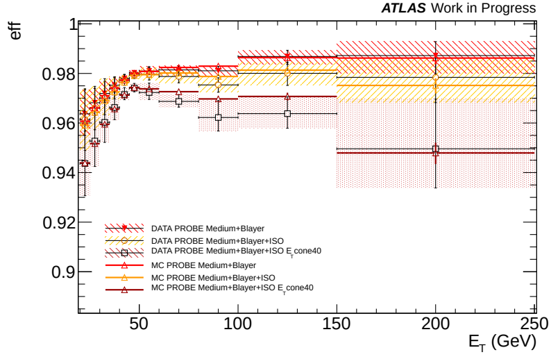
Figure D.3: Data and MC electron identification efficiencies of the B-layer hit requirement, of the B-layer hit plus E_{T\text{cone}20} isolation requirement, and of the B-layer hit plus E_{T\text{cone}40} isolation requirement. For the data points the errors evaluated in the plot take into account both the statistical and the systematic uncertainties.
