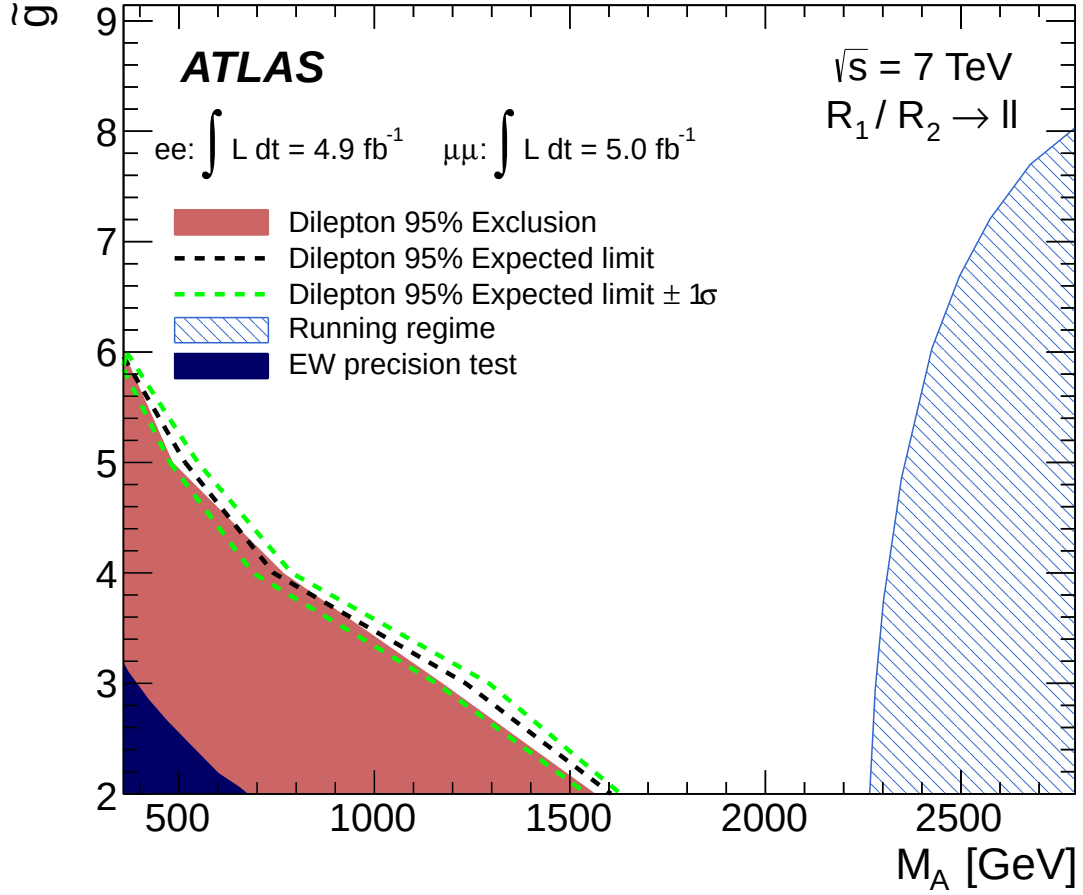
Figure 5.29: Bounds in the (M_A, \tilde{g}) plane of the MWT parameter space: (i) The 95% C.L. measurement of the electroweak precision parameters W and Y excludes the area in the left bottom corner. (ii) Imposing the modified Weinberg Sum Rules excludes the uniformly shaded area in the right corner (Running Regime). (iii) The shaded red area (dashed black line) shows the observed (expected) exclusion at 95% C.L. in dilepton channel, with m_H = 200 \text{ GeV} and s = 0 .
