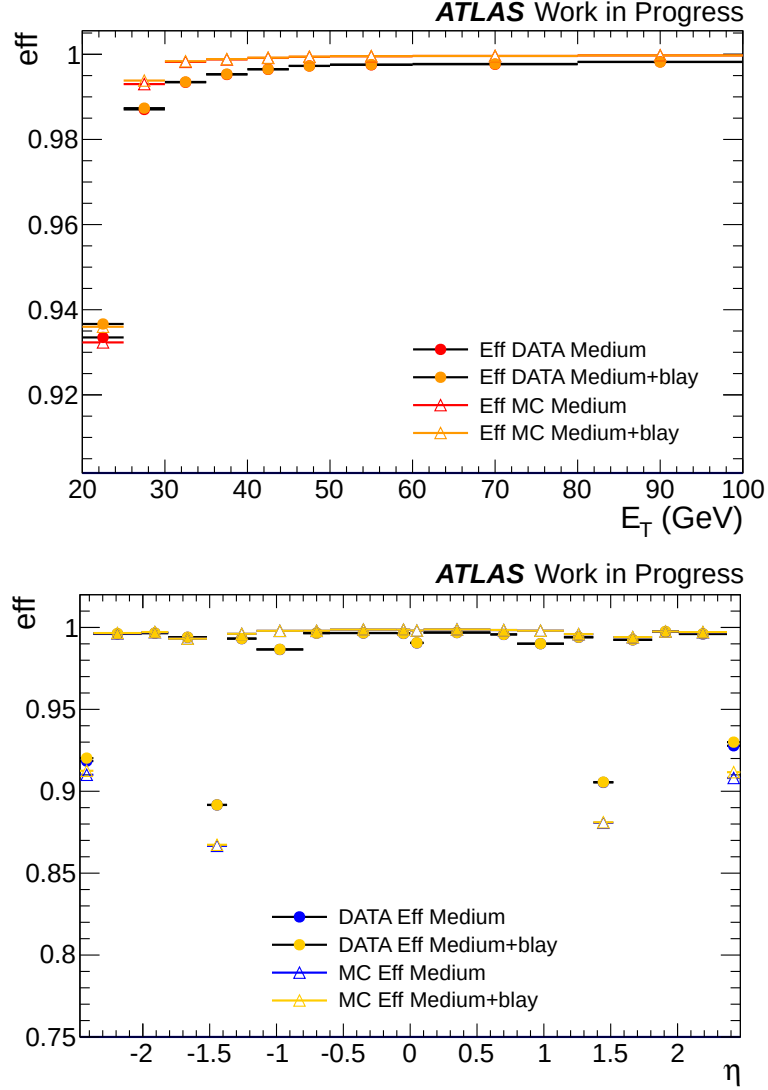
Figure 4.3: Trigger efficiency in data and in MC simulation with respect to medium and medium plus B-layer hit requirements for 2g20_loose trigger measured as a function of (top) the electron E_T and (bottom) as a function of \eta for electron with E_T > 25 GeV. The errors evaluated in the plots take into account only the statistical uncertainties.
